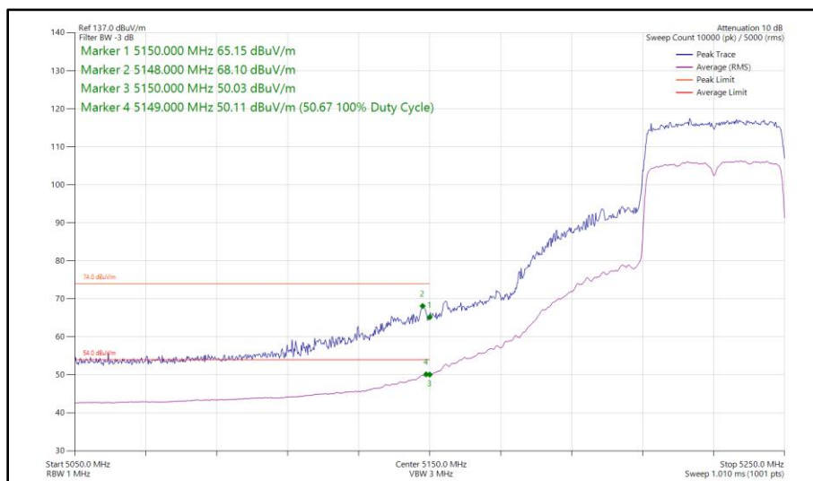
Figure 111 - 802.11ax HE40, SU, SISO, Core 1 - 5230 MHz Band Edge Frequency 5150 MHz
