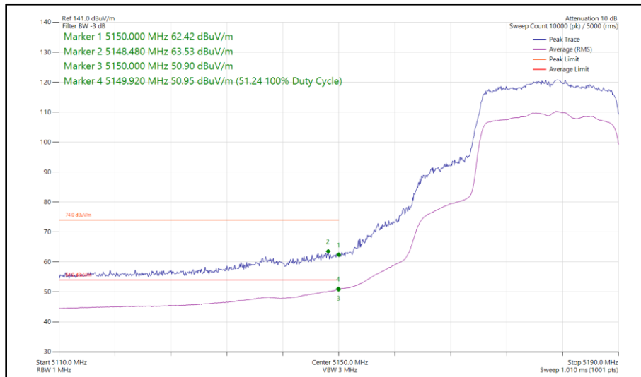
Figure 68 - 802.11ax HE20, SU, SDM, Core 0 - Core 1 - 5180 MHz Band Edge Frequency 5150 MHz
