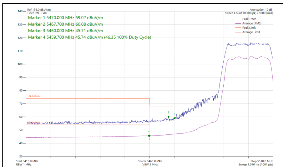
Figure 77 - 802.11n HT20, SDM, Core 0 - Core 1 - 5500 MHz Band Edge Frequency 5460 MHz
