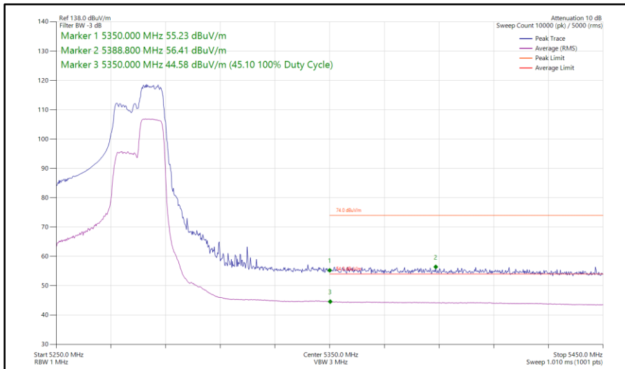
Figure 98 - 802.11ax HE40, RU 106-56, SISO, Core 0 - 5270 MHz Band Edge Frequency 5350 MHz
