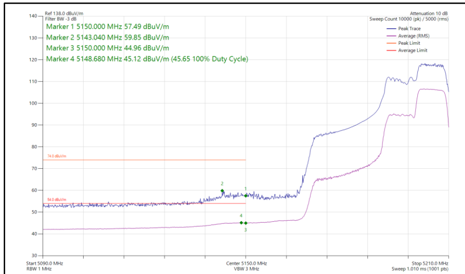
Figure 110 - 802.11ax HE40, RU 106-56, SISO, Core 1 - 5190 MHz Band Edge Frequency 5150 MHz
