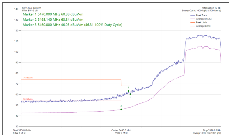
Figure 105 - 802.11ax HE40, SU, SISO, Core 0 - 5550 MHz Band Edge Frequency 5460 MHz
