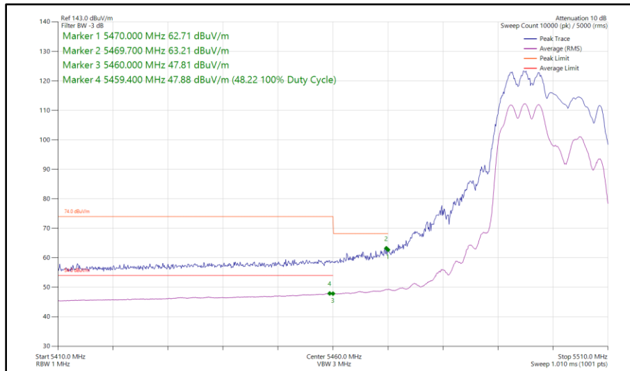
Figure 80 - 802.11ax HE20, RU 106-53, SDM, Core 0 - Core 1 - 5500 MHz Band Edge Frequency 5460 MHz
