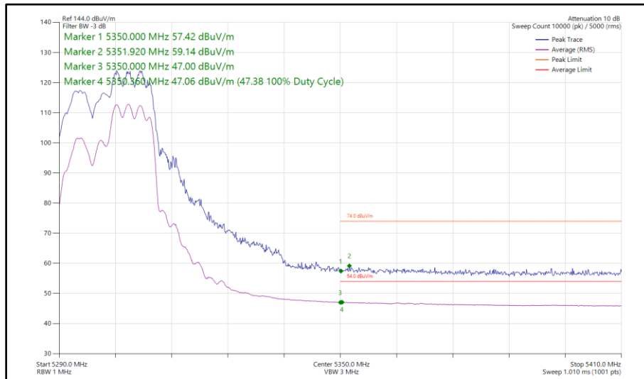
Figure 74 - 802.11ax HE20, RU 106-54, SDM, Core 0 - Core 1 - 5300 MHz Band Edge Frequency 5350 MHz
