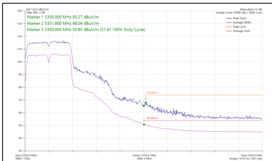
Figure 113 - 802.11n HT40, SISO, Core 1 - 5270 MHz Band Edge Frequency 5350 MHz
