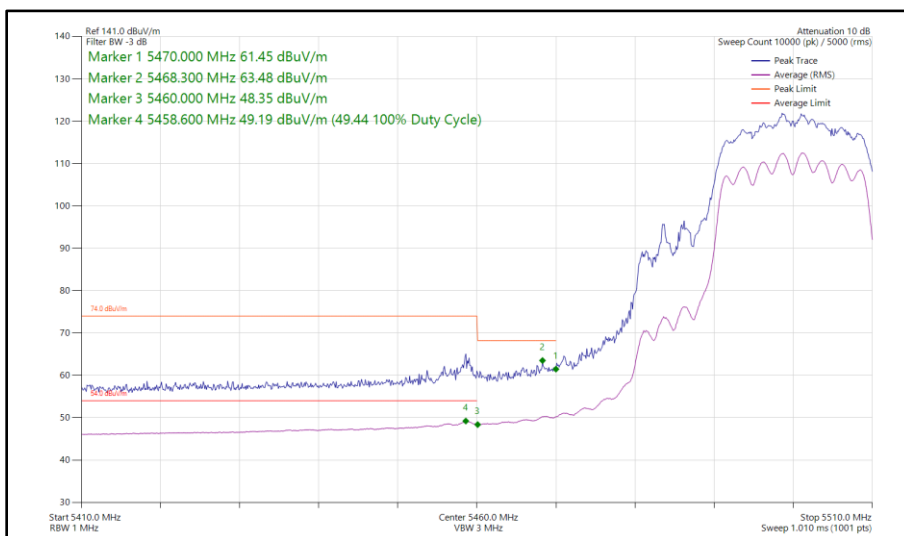
Figure 61 - 802.11n HT20, CDD, Core 0 - Core 1 - 5500 MHz Band Edge Frequency 5460 MHz
