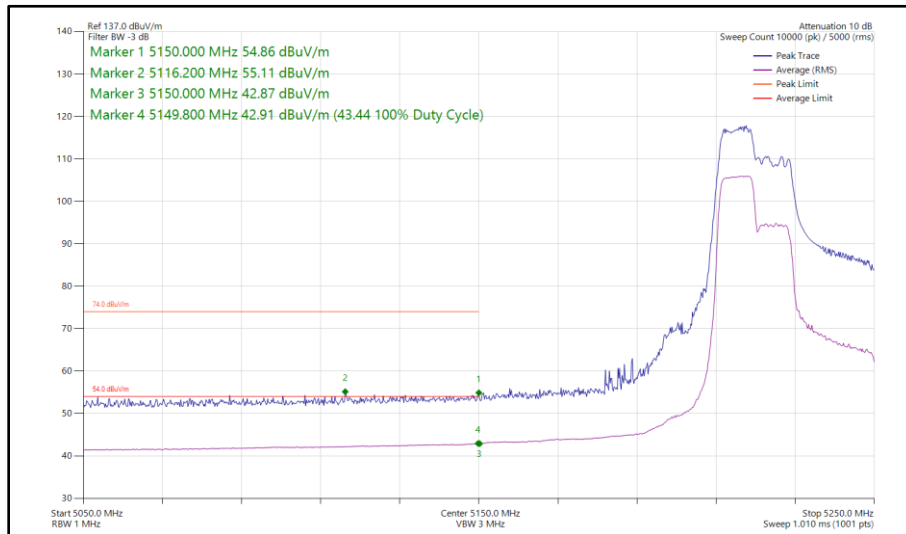
Figure 94 - 802.11ax HE40, RU 106-53, SISO, Core 0 - 5230 MHz Band Edge Frequency 5150 MHz
