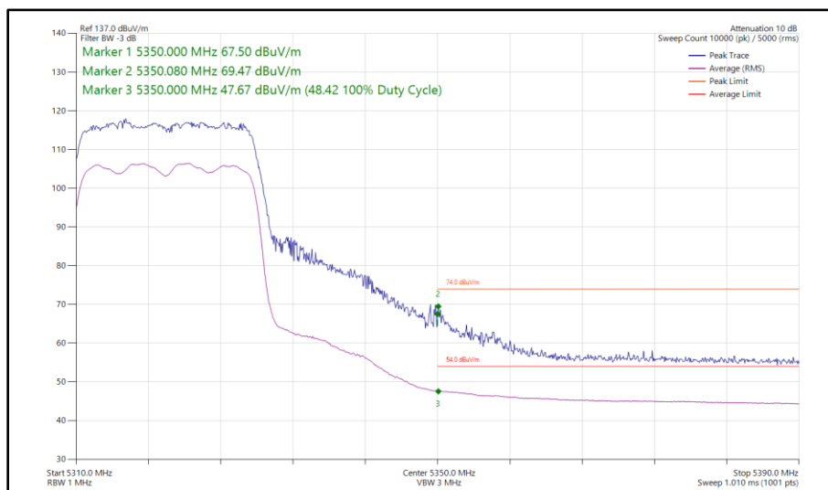
Figure 75 - 802.11ax HE20, SU, SDM, Core 0 - Core 1 - 5320 MHz Band Edge Frequency 5350 MHz
