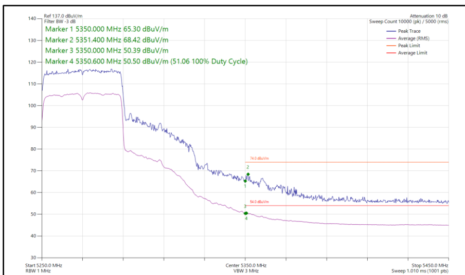
Figure 115 - 802.11ax HE40, SU, SISO, Core 1 - 5270 MHz Band Edge Frequency 5350 MHz
