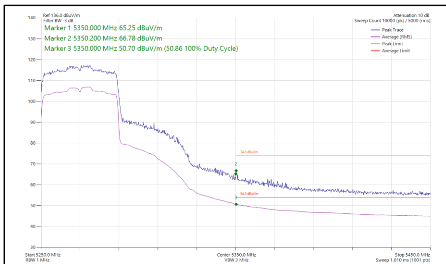
Figure 97 - 802.11ax HE40, SU, SISO, Core 0 - 5270 MHz Band Edge Frequency 5350 MHz
