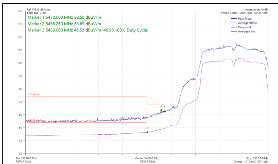
Figure 119 - 802.11n HT40, SISO, Core 1 - 5510 MHz Band Edge Frequency 5460 MHz
