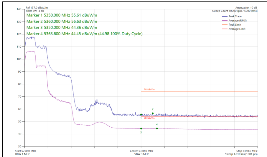
Figure 116 - 802.11ax HE40, RU 106-53, SISO, Core 1 - 5270 MHz Band Edge Frequency 5350 MHz
