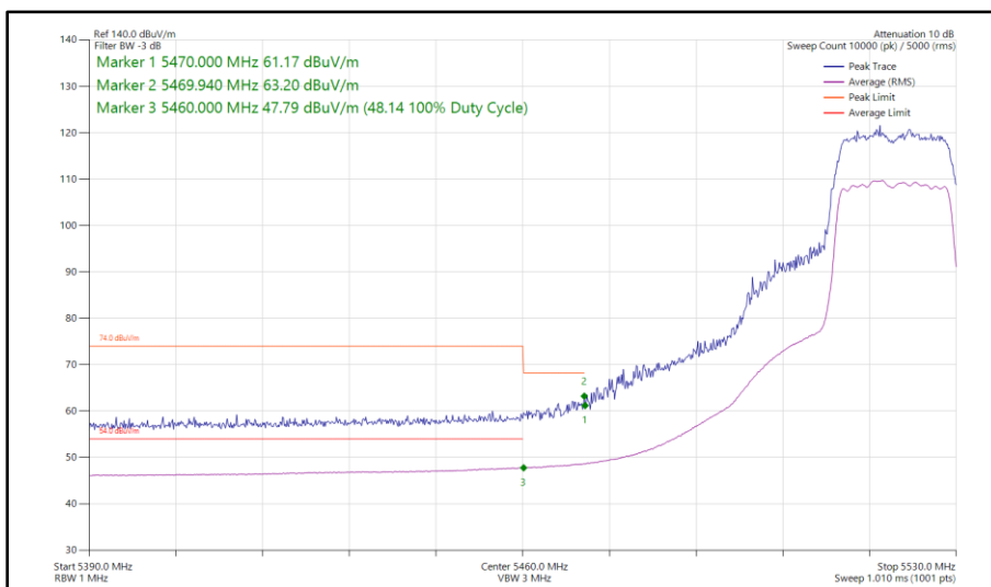
Figure 88 - 802.11ac VHT20, TxBF, Core 0 - Core 1 - 5520 MHz Band Edge Frequency 5460 MHz
