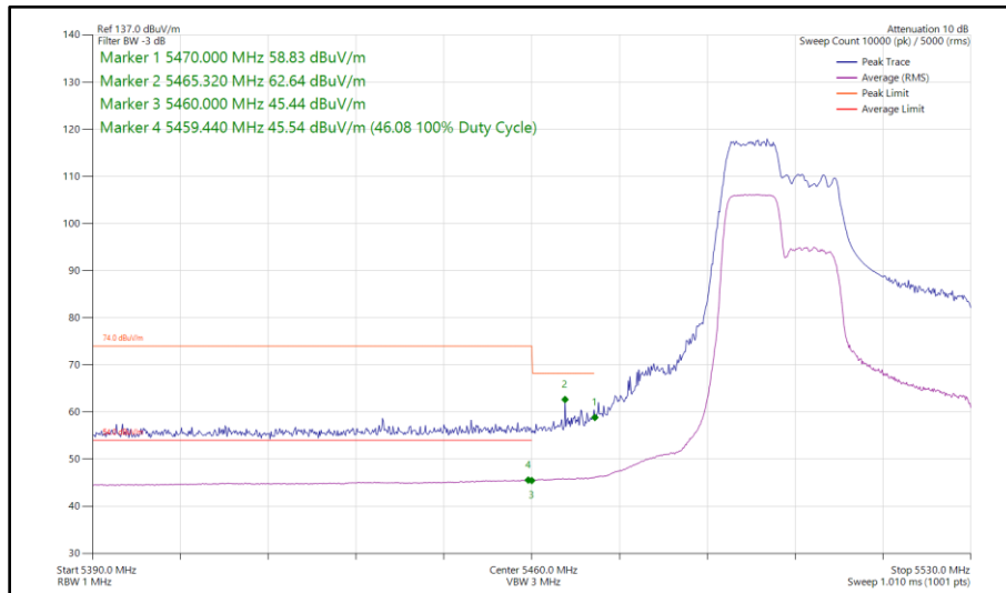
Figure 104 - 802.11ax HE40, RU 106-53, SISO, Core 0 - 5510 MHz Band Edge Frequency 5460 MHz
