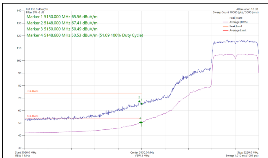
Figure 93 - 802.11ax HE40, SU, SISO, Core 0 - 5230 MHz Band Edge Frequency 5150 MHz
