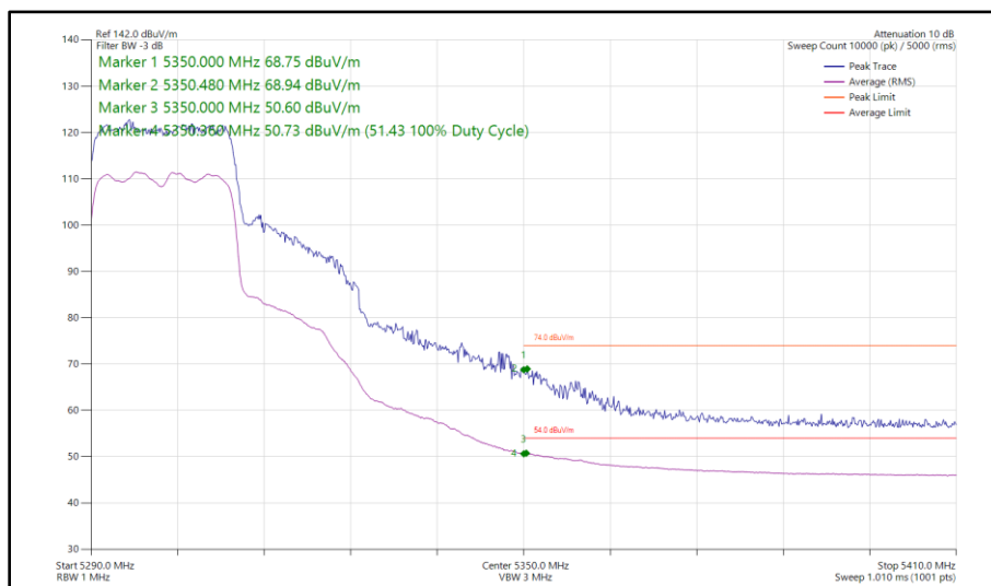
Figure 73 - 802.11ax HE20, SU, SDM, Core 0 - Core 1 - 5300 MHz Band Edge Frequency 5350 MHz
