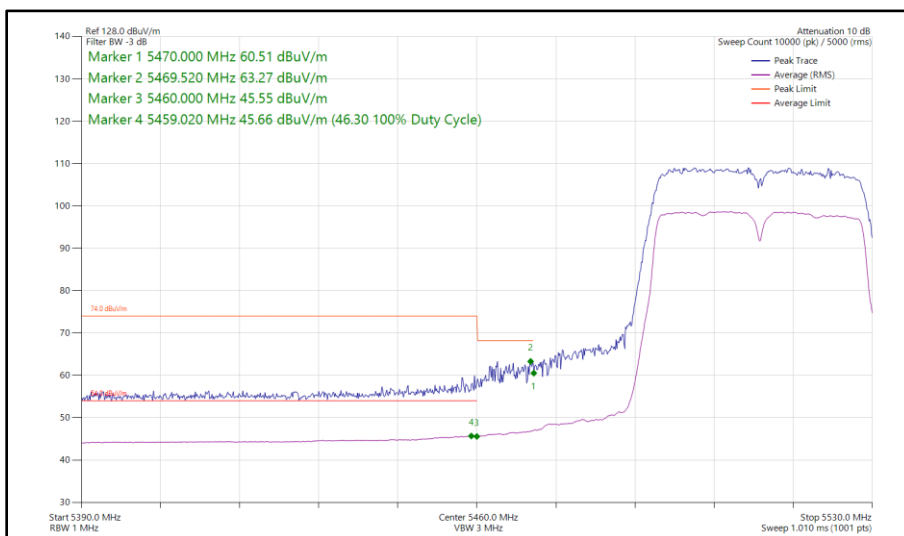
Figure 101 - 802.11n HT40, SISO, Core 0 - 5510 MHz Band Edge Frequency 5460 MHz
