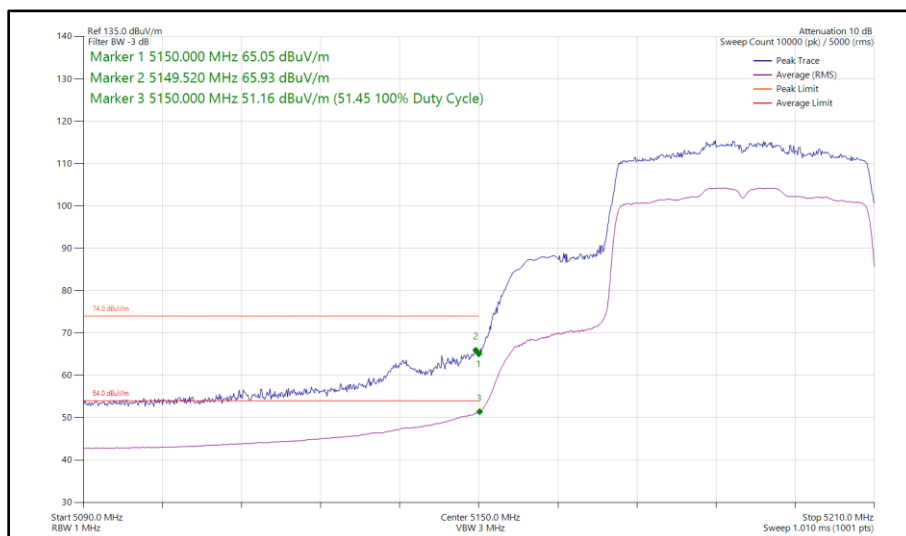
Figure 109 - 802.11ax HE40, SU, SISO, Core 1 - 5190 MHz Band Edge Frequency 5150 MHz
