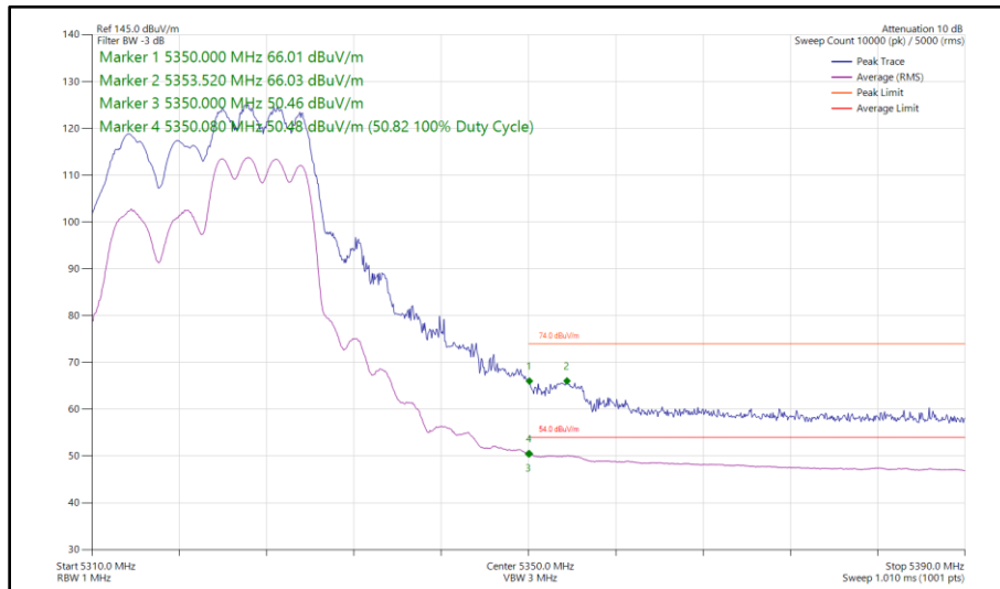
Figure 76 - 802.11ax HE20, RU 106-54, SDM, Core 0 - Core 1 - 5320 MHz Band Edge Frequency 5350 MHz
