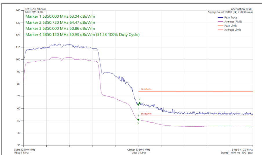
Figure 99 - 802.11ax HE40, SU, SISO, Core 0 - 5310 MHz Band Edge Frequency 5350 MHz
