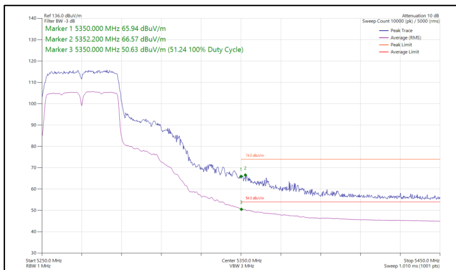
Figure 95 - 802.11n HT40, SISO, Core 0 - 5270 MHz Band Edge Frequency 5350 MHz
