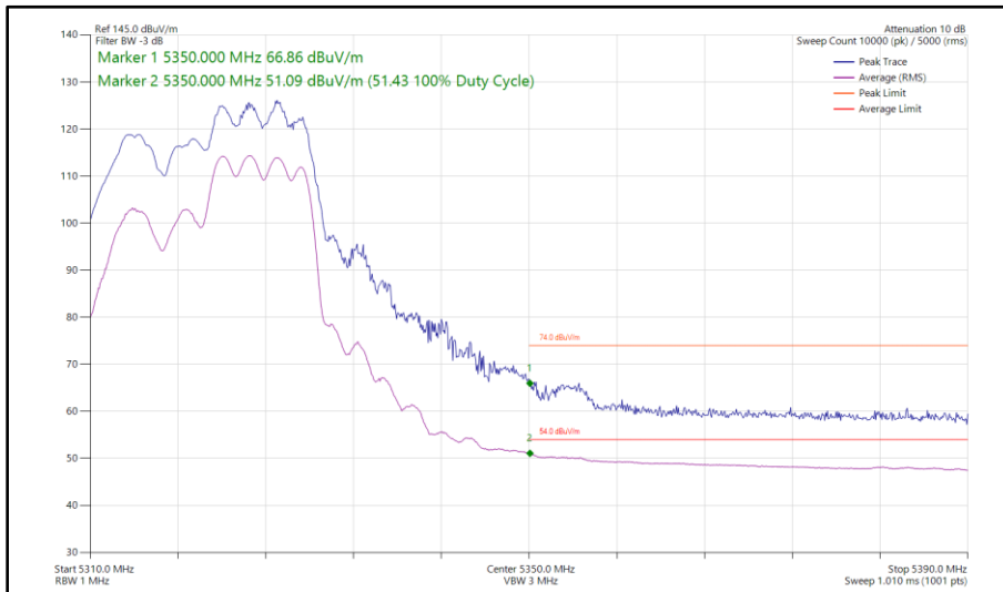
Figure 60 - 802.11ax HE20, RU 106-54, CDD, Core 0 - Core 1 - 5320 MHz Band Edge Frequency 5350 MHz
