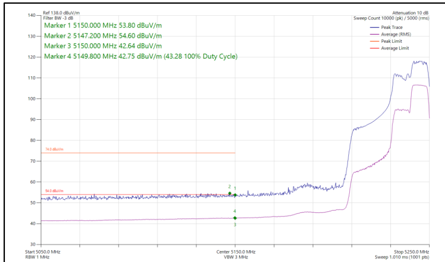
Figure 112 - 802.11ax HE40, RU 106-56, SISO, Core 1 - 5230 MHz Band Edge Frequency 5150 MHz
