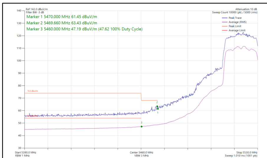
Figure 81 - 802.11ax HE20, SU, SDM, Core 0 - Core 1 - 5520 MHz Band Edge Frequency 5460 MHz
