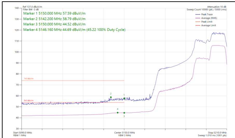
Figure 92 - 802.11ax HE40, RU 106-56, SISO, Core 0 - 5190 MHz Band Edge Frequency 5150 MHz
