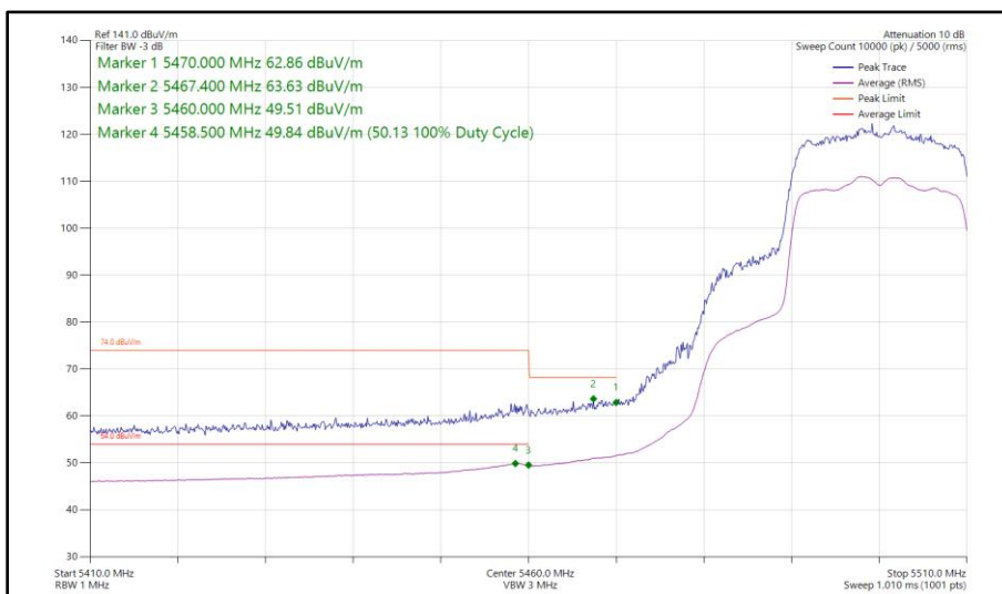
Figure 79 - 802.11ax HE20, SU, SDM, Core 0 - Core 1 - 5500 MHz Band Edge Frequency 5460 MHz
