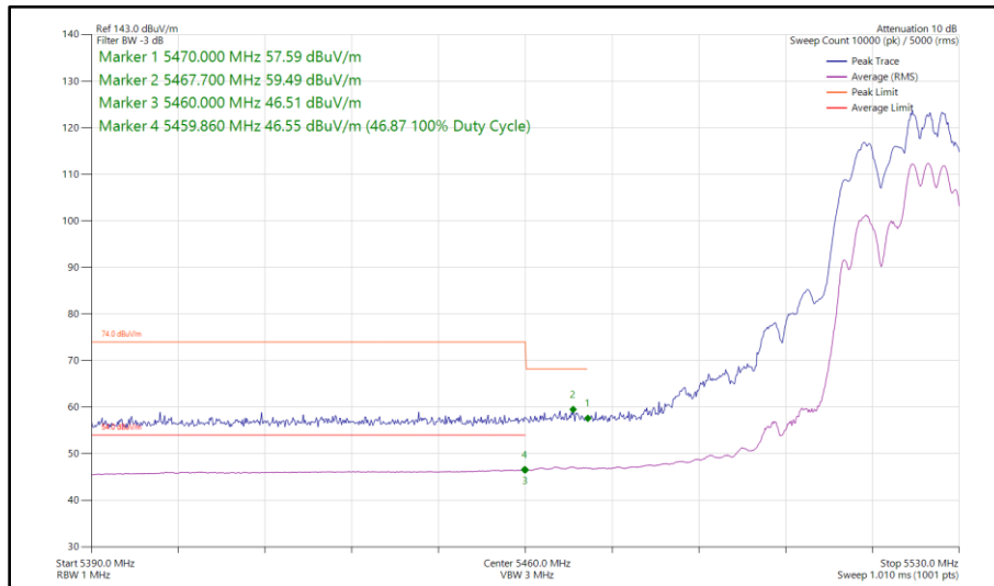
Figure 82 - 802.11ax HE20, RU 106-54, SDM, Core 0 - Core 1 - 5520 MHz Band Edge Frequency 5460 MHz
