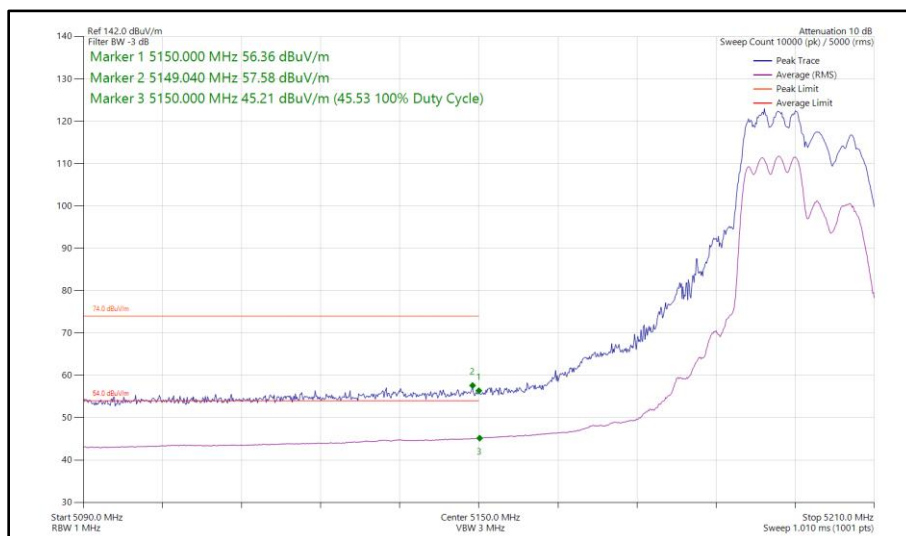
Figure 71 - 802.11ax HE20, RU 106-53, SDM, Core 0 - Core 1 - 5200 MHz Band Edge Frequency 5150 MHz
