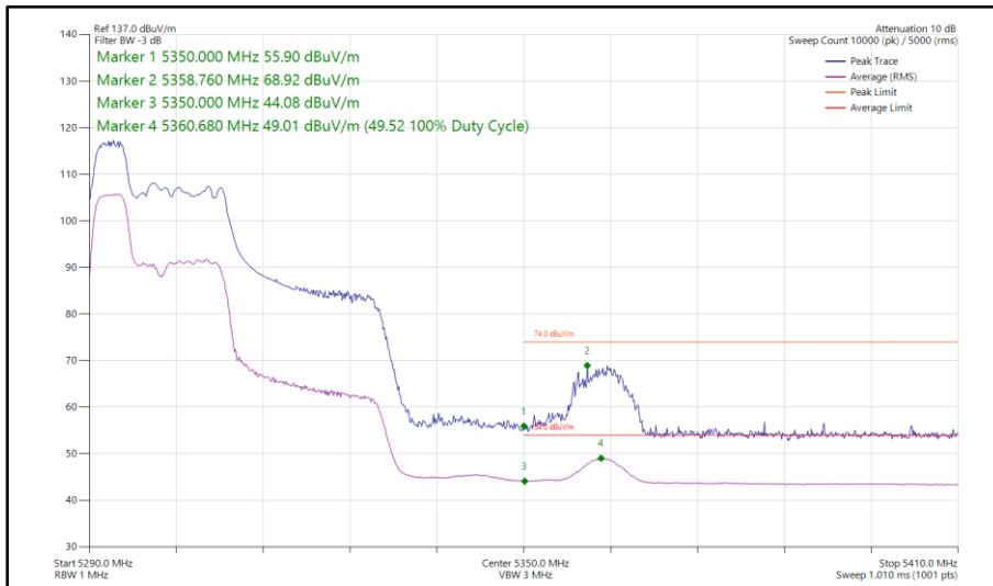
Figure 100 - 802.11ax HE40, RU 52-37, SISO, Core 0 - 5310 MHz Band Edge Frequency 5350 MHz
