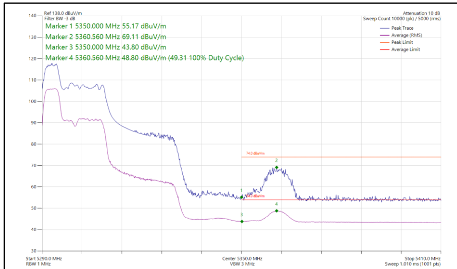
Figure 118 - 802.11ax HE40, RU 52-37, SISO, Core 1 - 5310 MHz Band Edge Frequency 5350 MHz
