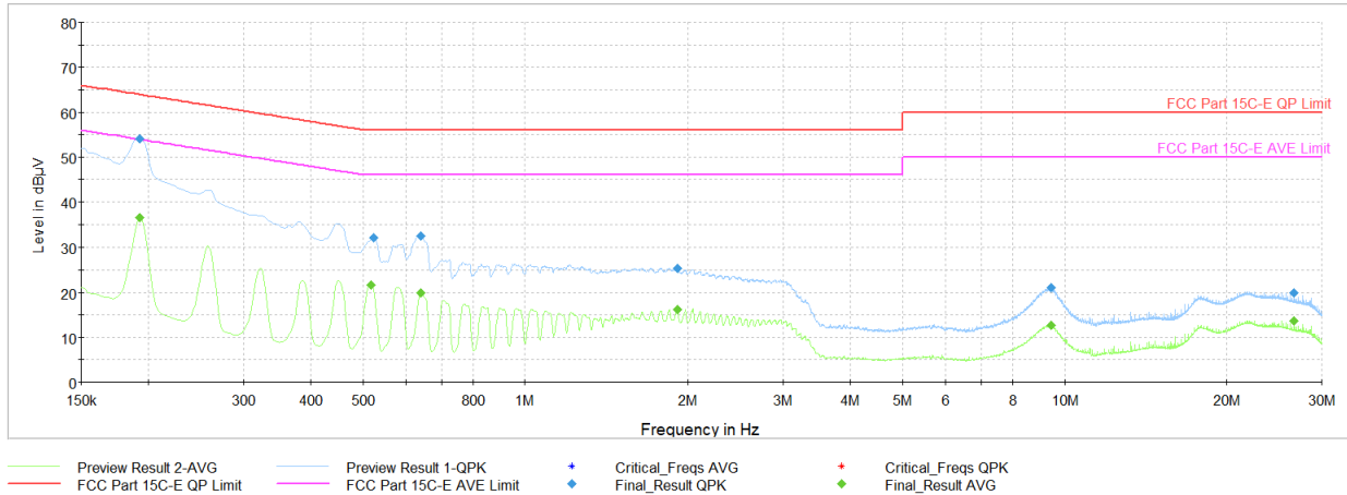
Plot 7-32. AC Line Conducted Plot with Bluetooth LE (L1, 1Mbps – Ch.0 with charging case and AC/DC Adapter)
