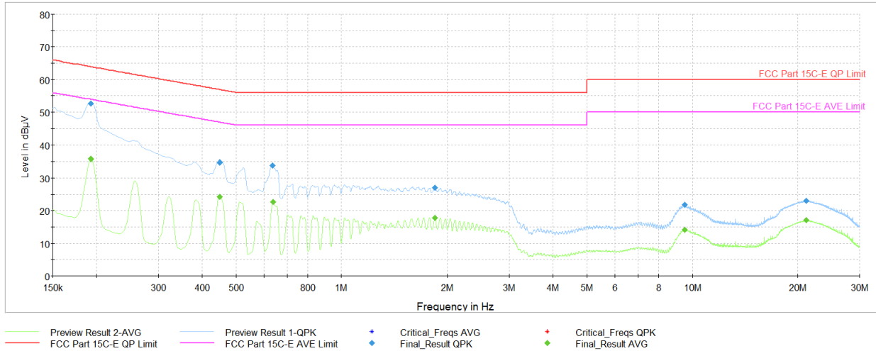
Plot 7-33. AC Line Conducted Plot with Bluetooth LE (N, 1Mbps – Ch.0, with charging case and AC/DC Adapter)
