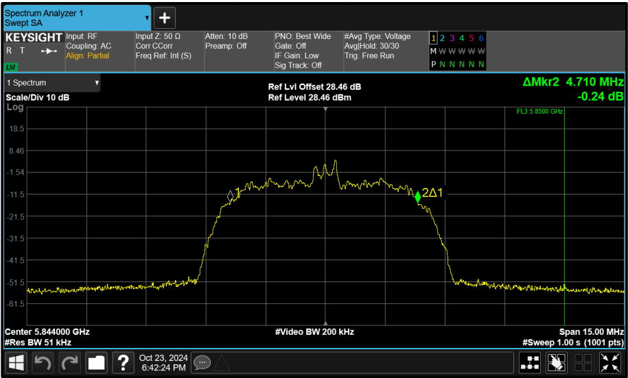
Figure 132 - Core 0 (A) 5844 MHz (CH119) 99% Bandwidth
