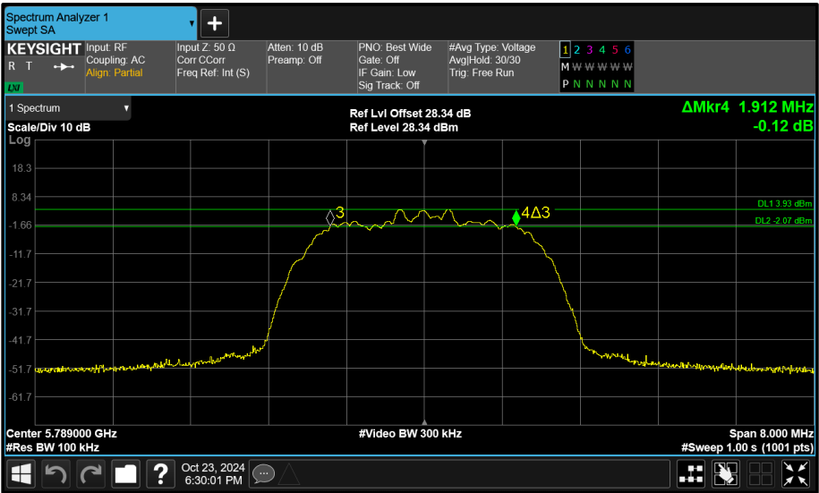
Figure 117 - Core 0 (A) 5789 MHz (CH64) 6 dB Bandwidth
