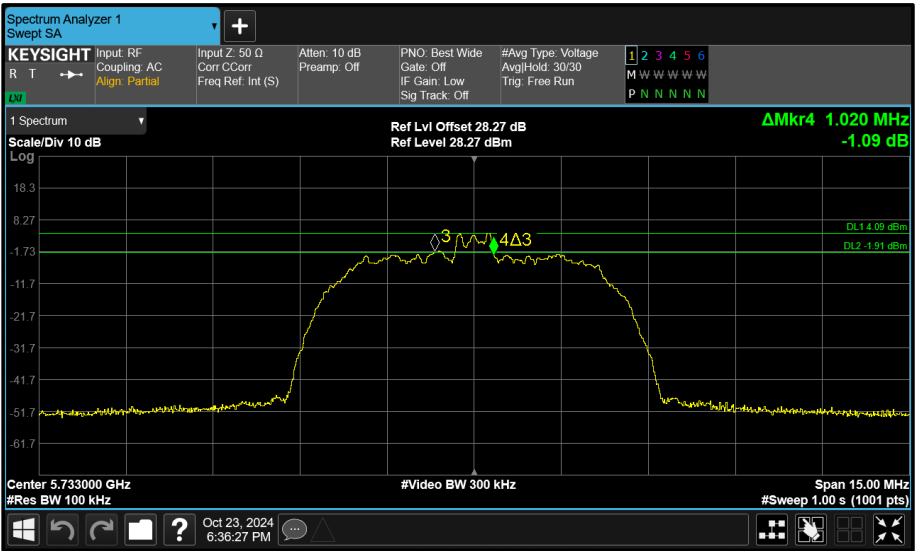
Figure 125 - Core 0 (A) 5733 MHz (CH8) 6 dB Bandwidth
