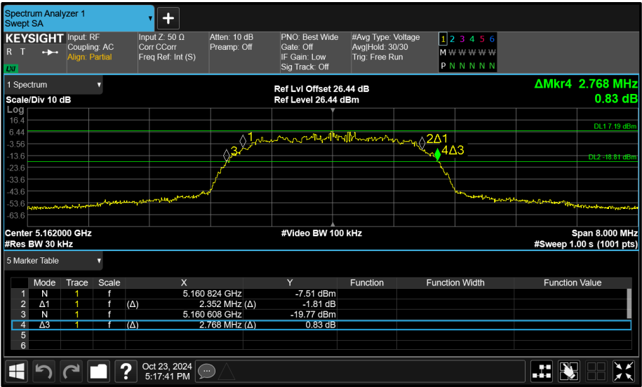
Figure 64 - Core 1 (B) 5162 MHz (CH12) 26 dB and 99% Bandwidth
