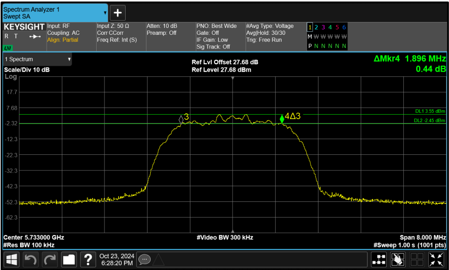
Figure 115 - Core 1 (B) 5733 MHz (CH8) 6 dB Bandwidth
