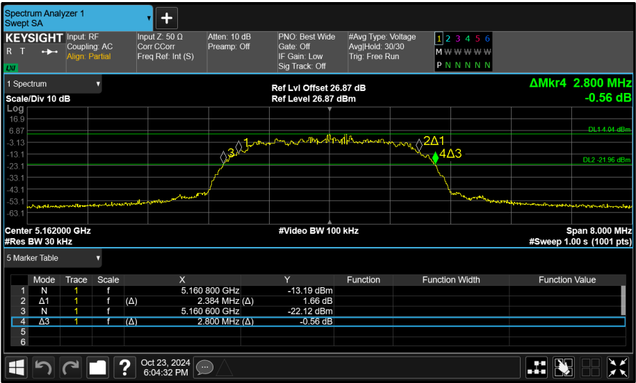
Figure 136 - Core 0 (A) 5162 MHz (CH12) 26 dB and 99% Bandwidth
