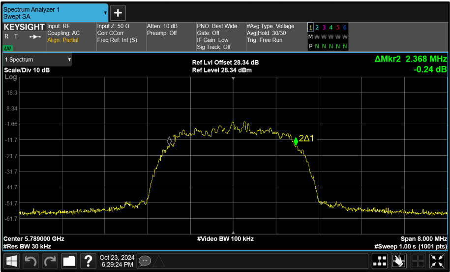
Figure 116 - Core 0 (A) 5789 MHz (CH64) 99% Bandwidth
