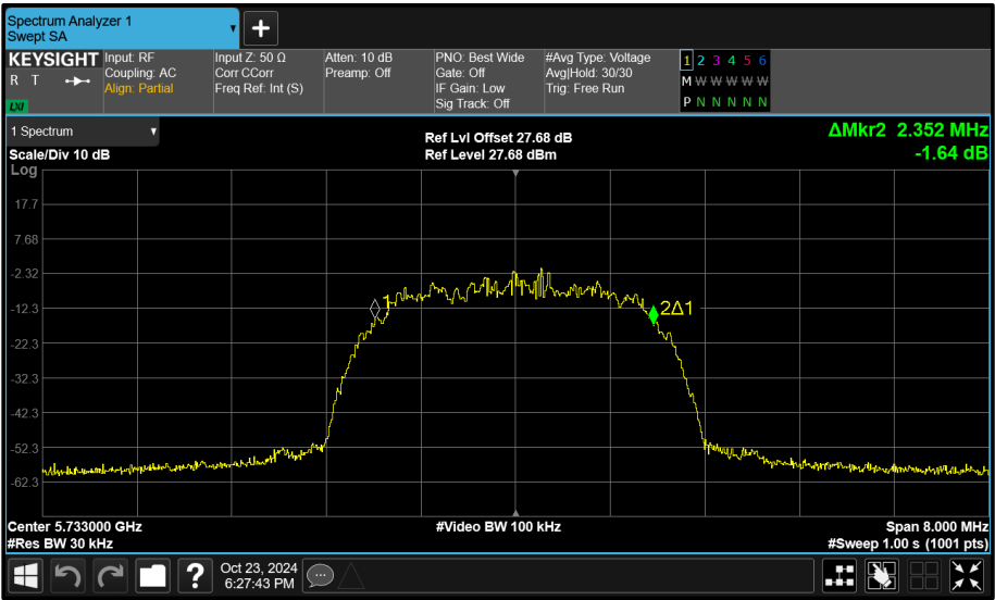
Figure 114 - Core 1 (B) 5733 MHz (CH8) 99% Bandwidth
