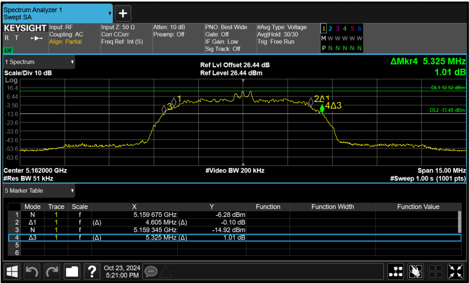
Figure 67 - Core 1 (B) 5162 MHz (CH12) 26 dB and 99% Bandwidth
