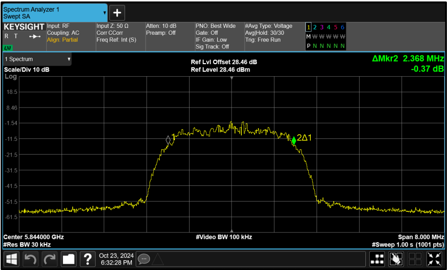
Figure 120 - Core 0 (A) 5844 MHz (CH119) 99% Bandwidth
