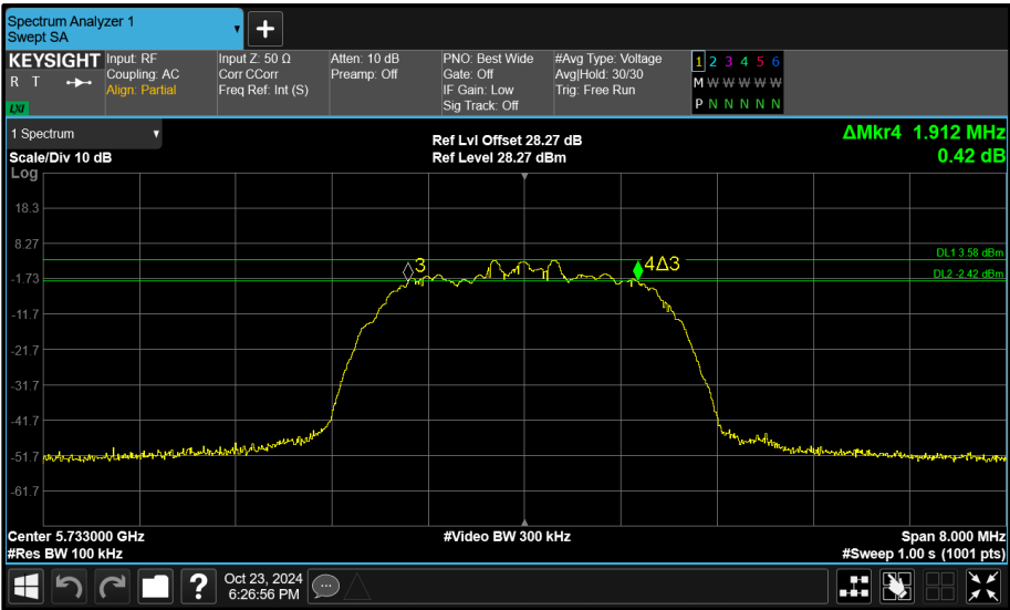
Figure 113 - Core 0 (A) 5733 MHz (CH8) 6 dB Bandwidth
