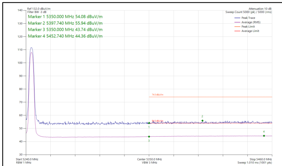
Figure 35 - Bluetooth HDR4, MIMO, Core 0 - Core 1 - 5245 MHz Band Edge Frequency 5350 MHz
