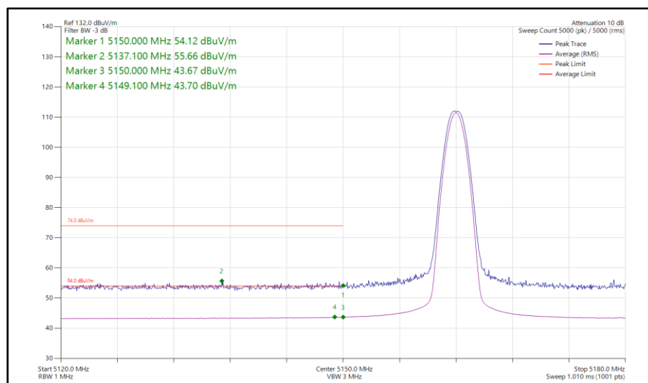
Figure 19 - Bluetooth DH5, SISO, Core 0 - 5162 MHz Band Edge Frequency 5150 MHz
