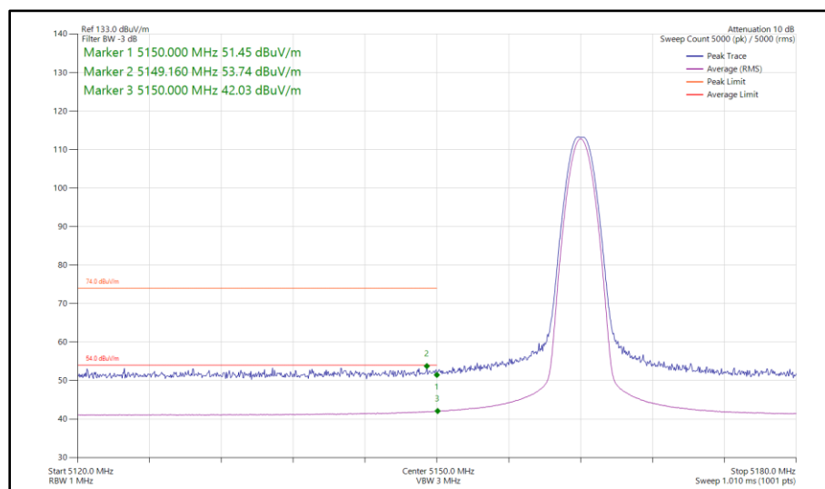
Figure 25 - Bluetooth DH5, SISO, Core 1 - 5162 MHz Band Edge Frequency 5150 MHz
