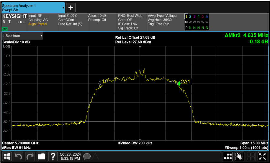
Figure 58 - Core 1 (B) 5733 MHz (CH8) 99% Bandwidth
