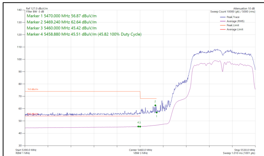
Figure 599 - 802.11ac VHT40, TxBF, Core 0 - Core 1 - 5510 MHz Band Edge Frequency 5470 MHz
