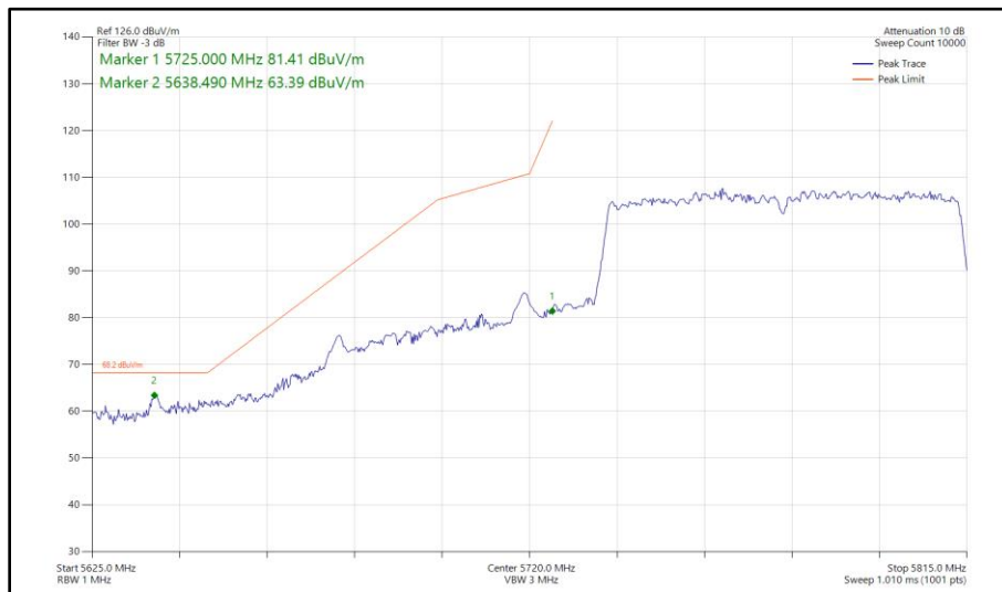
Figure 639 - 802.11ac VHT80, CDD, Core 0 - Core 1 - 5775 MHz Band Edge Frequency 5725 MHz
