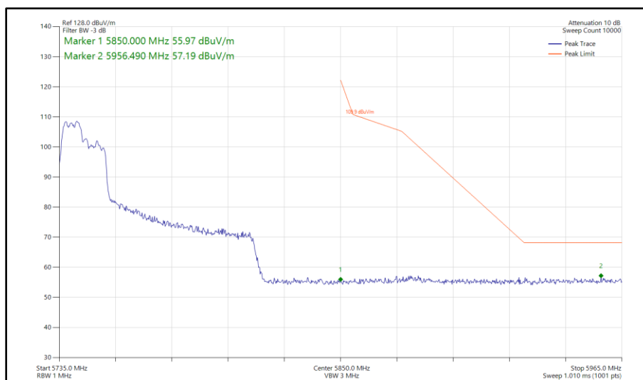
Figure 665 - 802.11ax HE80, RU 106-53, SDM, Core 0 - Core 1 - 5775 MHz Band Edge Frequency 5850 MHz
