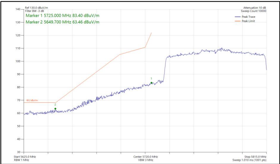
Figure 655 - 802.11ax HE80, SU, SDM, Core 0 - Core 1 - 5775 MHz Band Edge Frequency 5725 MHz
