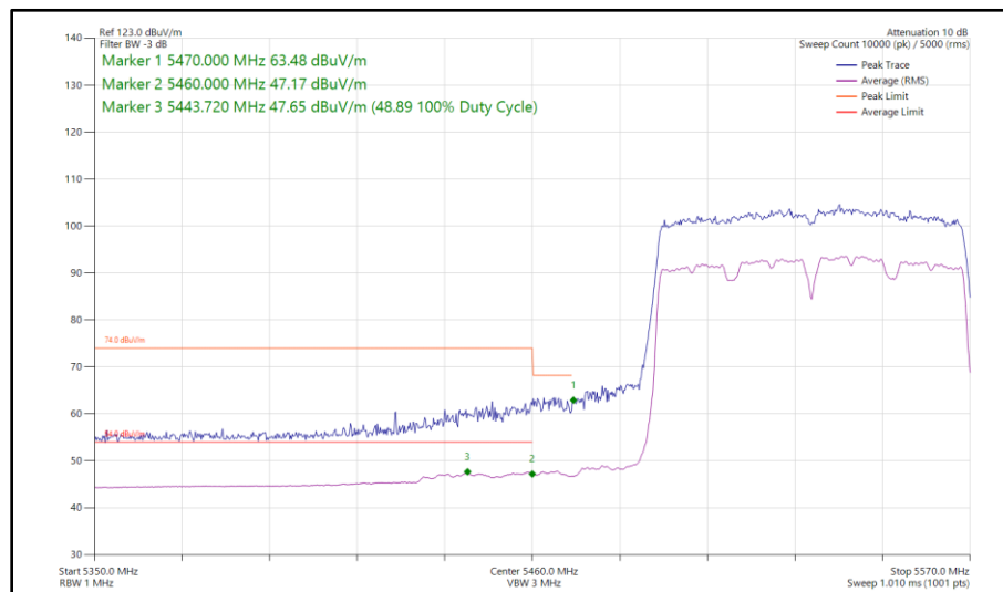
Figure 651 - 802.11ac VHT80, SDM, Core 0 - Core 1 - 5530 MHz Band Edge Frequency 5470 MHz
