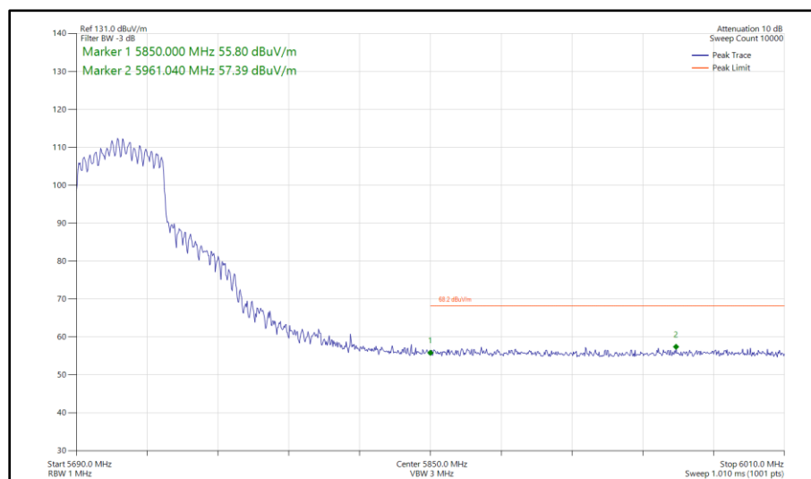
Figure 574 - 802.11ax HE40, SU, CDD, Core 0 - Core 1 - 5710 MHz Band Edge Frequency 5850 MHz
