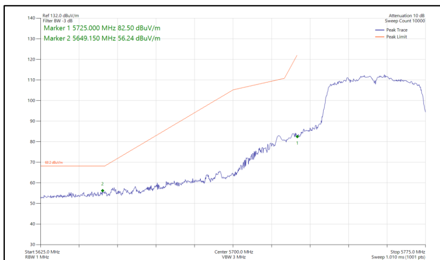
Figure 584 - 802.11n HT40, SDM, Core 0 - Core 1 - 5755 MHz Band Edge Frequency 5725 MHz
