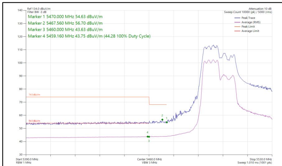
Figure 561 - 802.11ax HE40, RU 106-53, CDD, Core 0 - Core 1 - 5510 MHz Band Edge Frequency 5470 MHz
