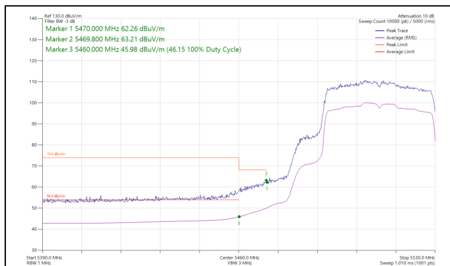
Figure 539 - 802.11ax HE40, SU, SISO, Core 1 - 5510 MHz Band Edge Frequency 5470 MHz
