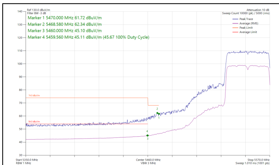
Figure 541 - 802.11ax HE40, SU, SISO, Core 1 - 5550 MHz Band Edge Frequency 5470 MHz
