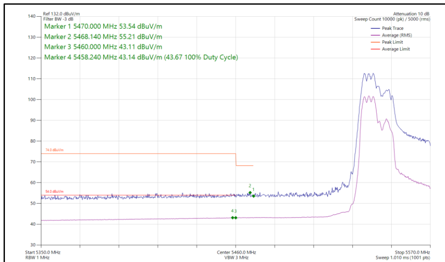
Figure 583 - 802.11ax HE40, RU 106-53, SDM, Core 0 - Core 1 - 5550 MHz Band Edge Frequency 5470 MHz
