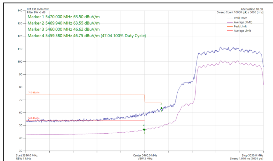
Figure 560 - 802.11ax HE40, SU, CDD, Core 0 - Core 1 - 5510 MHz Band Edge Frequency 5470 MHz
