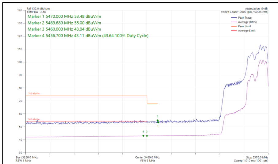
Figure 563 - 802.11ax HE40, RU 106-56, CDD, Core 0 - Core 1 - 5550 MHz Band Edge Frequency 5470 MHz
