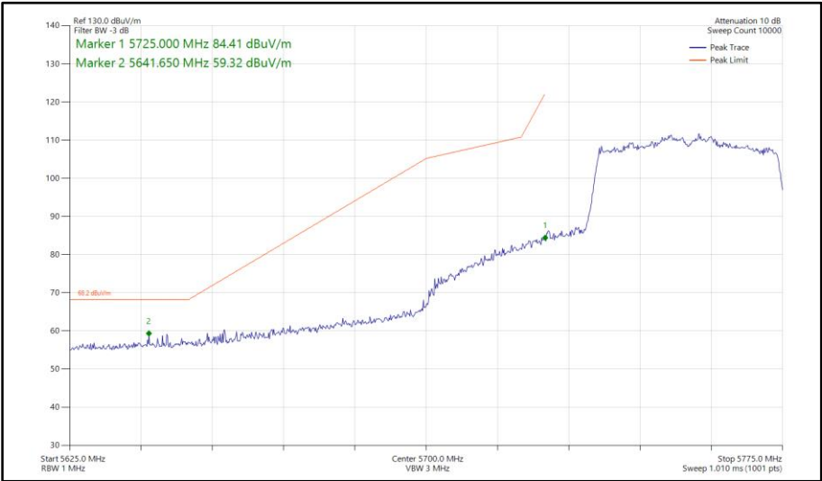
Figure 585 - 802.11ax HE40, SU, SDM, Core 0 - Core 1 - 5755 MHz Band Edge Frequency 5725 MHz
