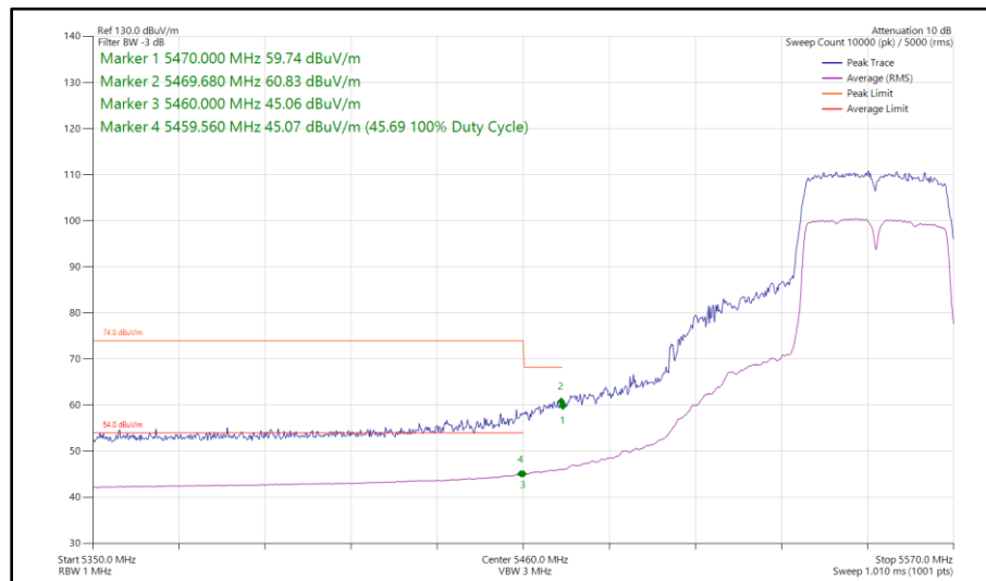
Figure 517 - 802.11n HT40, SISO, Core 0 - 5550 MHz Band Edge Frequency 5470 MHz
