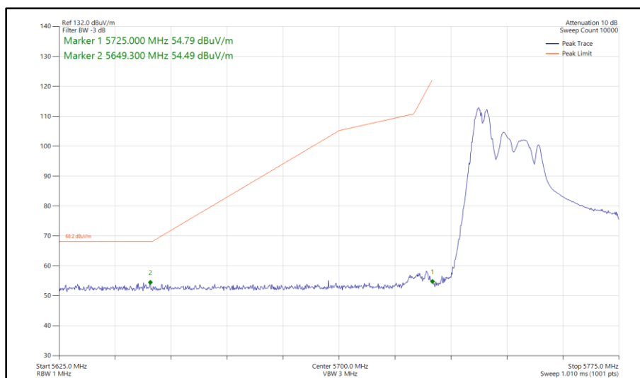
Figure 566 - 802.11ax HE40, RU 52-37, CDD, Core 0 - Core 1 - 5755 MHz Band Edge Frequency 5725 MHz
