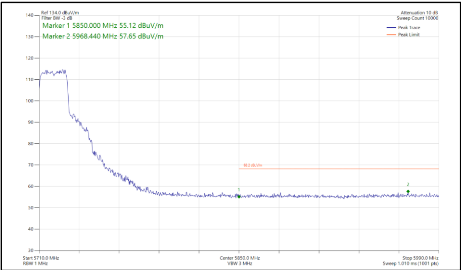
Figure 504 - 802.11ax HE20, SU, SDM, Core 0 - Core 1 - 5720 MHz Band Edge Frequency 5850 MHz
