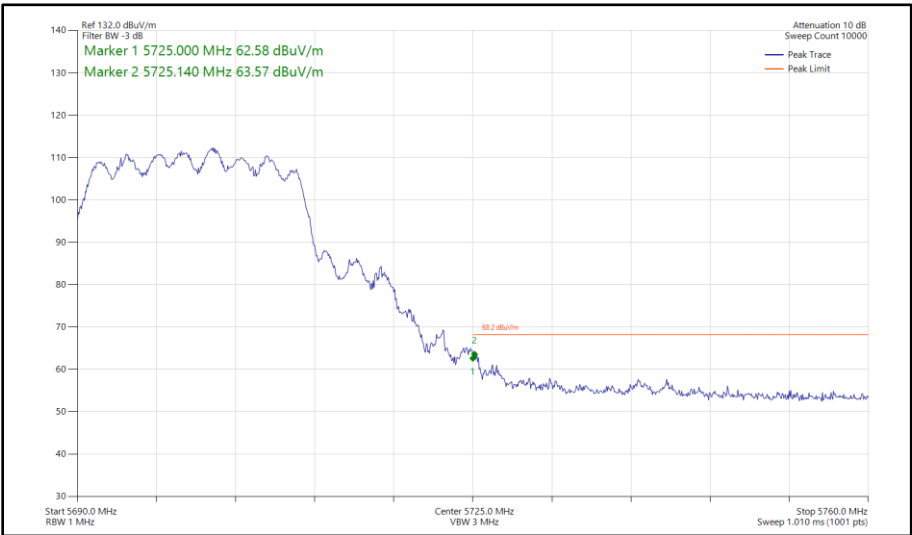
Figure 475 - 802.11ax HE20, SU, CDD, Core 0 - Core 1 - 5700 MHz Band Edge Frequency 5725 MHz
