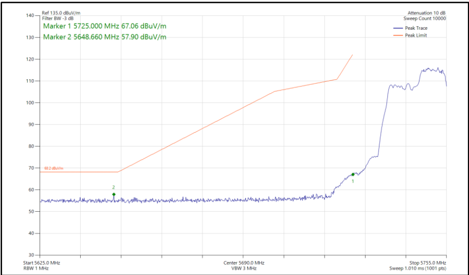
Figure 439 - 802.11ax HE20, RU 106-54, SISO, Core 1 - 5745 MHz Band Edge Frequency 5725 MHz
