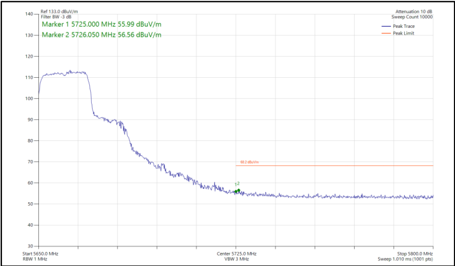
Figure 495 - 802.11n HT20, SDM, Core 0 - Core 1 - 5660 MHz Band Edge Frequency 5725 MHz
