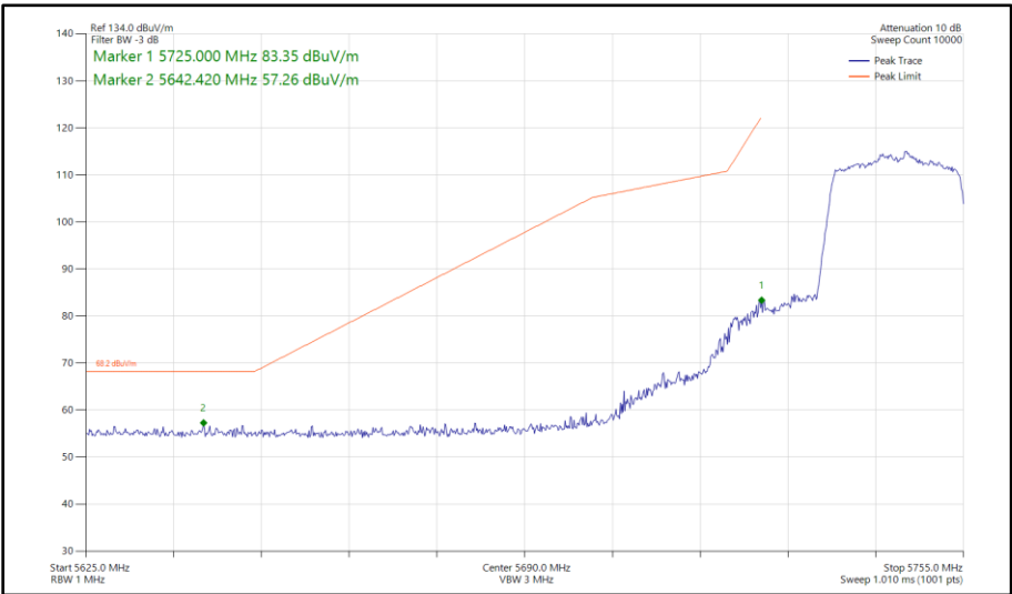
Figure 492 - 802.11ax HE20, SU, SDM, Core 0 - Core 1 - 5745 MHz Band Edge Frequency 5725 MHz
