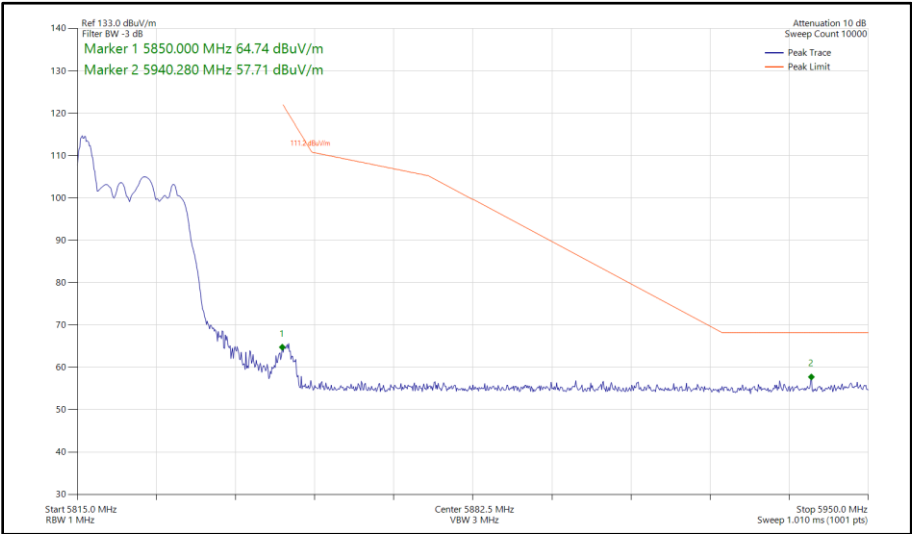
Figure 484 - 802.11ax HE20, RU 26-0, CDD, Core 0 - Core 1 - 5825 MHz Band Edge Frequency 5850 MHz
