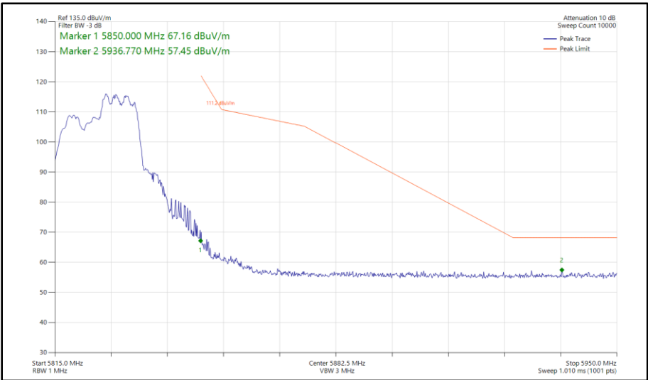
Figure 508 - 802.11ax HE20, RU 106-54, SDM, Core 0 - Core 1 - 5825 MHz Band Edge Frequency 5850 MHz
