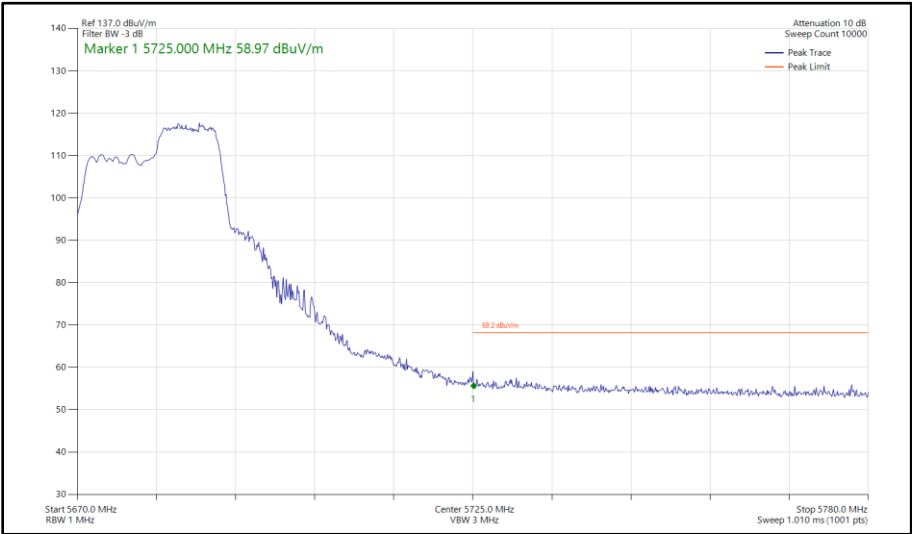
Figure 446 - 802.11ax HE20, RU 106-54, SISO, Core 1 - 5680 MHz Band Edge Frequency 5725 MHz
