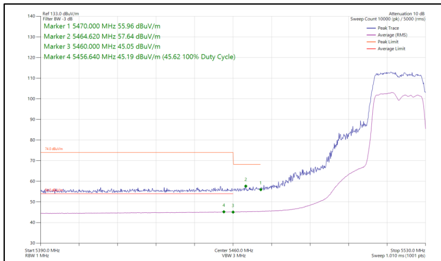
Figure 510 - 802.11ac VHT20, TxBF, Core 0 - Core 1 - 5520 MHz Band Edge Frequency 5470 MHz
