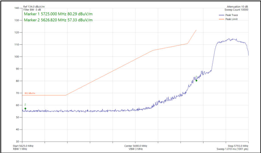
Figure 436 - 802.11n HT20, SISO, Core 1 - 5745 MHz Band Edge Frequency 5725 MHz
