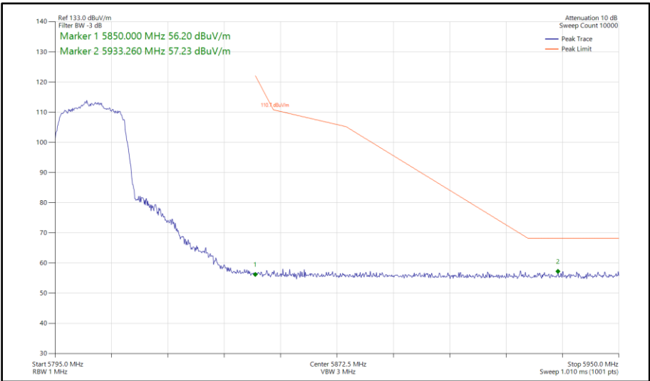
Figure 453 - 802.11n HT20, SISO, Core 1 - 5805 MHz Band Edge Frequency 5850 MHz
