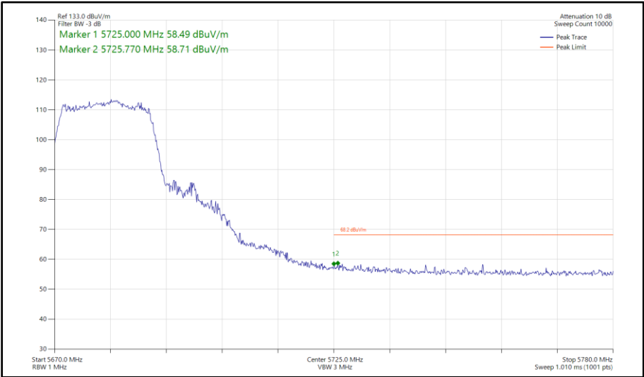
Figure 512 - 802.11ac VHT20, TxBF, Core 0 - Core 1 - 5680 MHz Band Edge Frequency 5725 MHz
