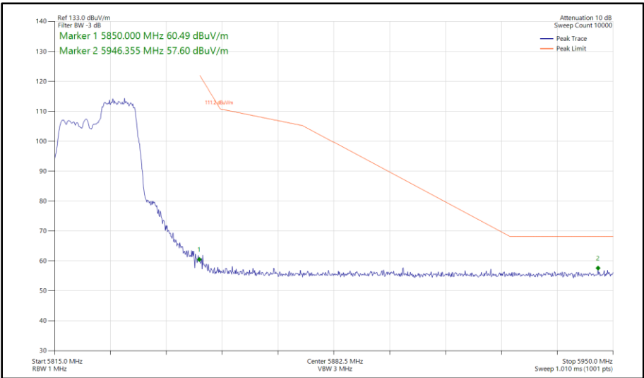
Figure 459 - 802.11ax HE20, RU 106-54, SISO, Core 1 - 5825 MHz Band Edge Frequency 5850 MHz
