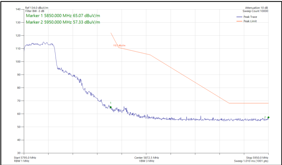
Figure 506 - 802.11ax HE20, SU, SDM, Core 0 - Core 1 - 5805 MHz Band Edge Frequency 5850 MHz
