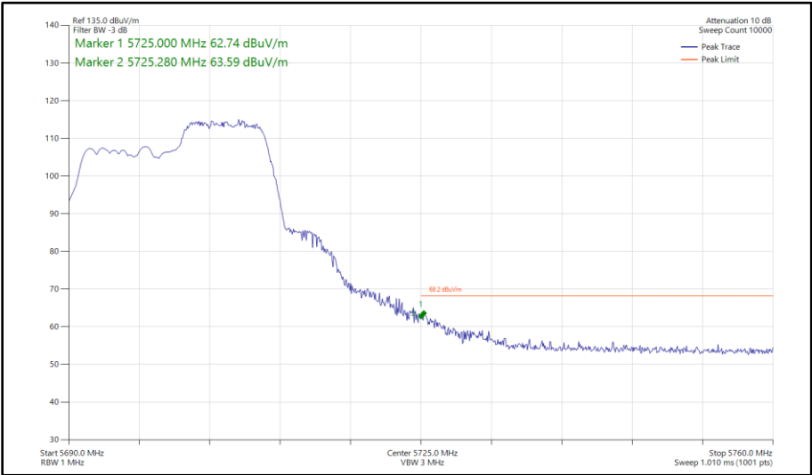
Figure 448 - 802.11ax HE20, RU 106-54, SISO, Core 1 - 5700 MHz Band Edge Frequency 5725 MHz
