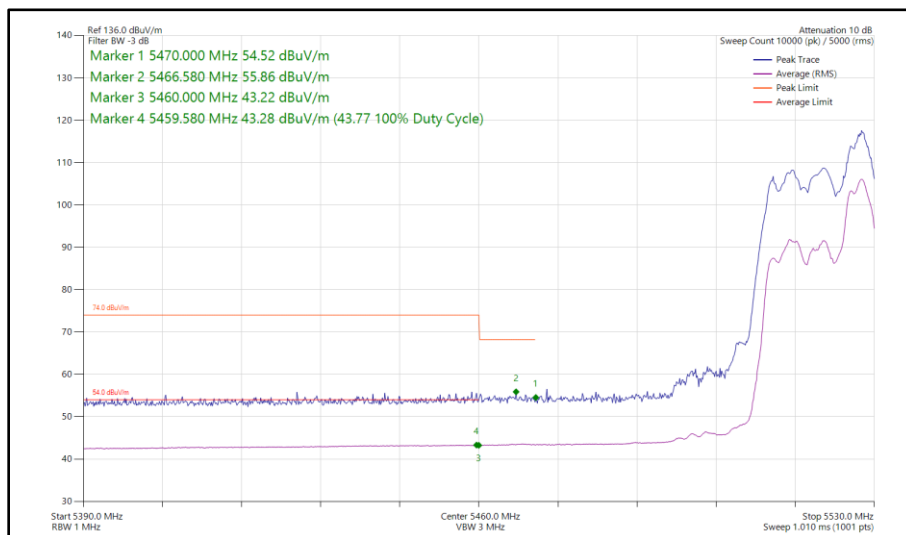
Figure 465 - 802.11ax HE20, RU 52-40, CDD, Core 0 - Core 1 - 5520 MHz Band Edge Frequency 5470 MHz
