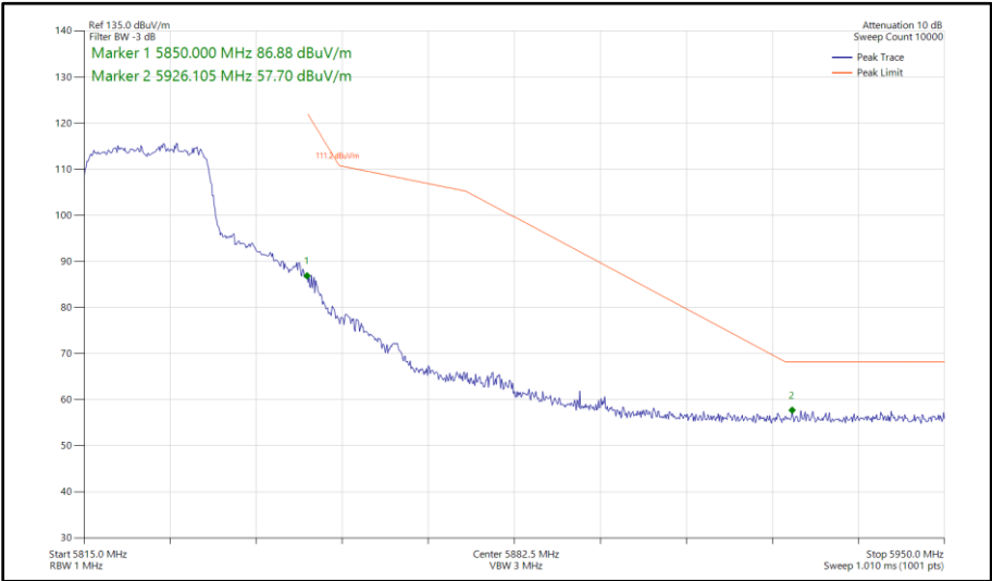
Figure 507 - 802.11ax HE20, SU, SDM, Core 0 - Core 1 - 5825 MHz Band Edge Frequency 5850 MHz
