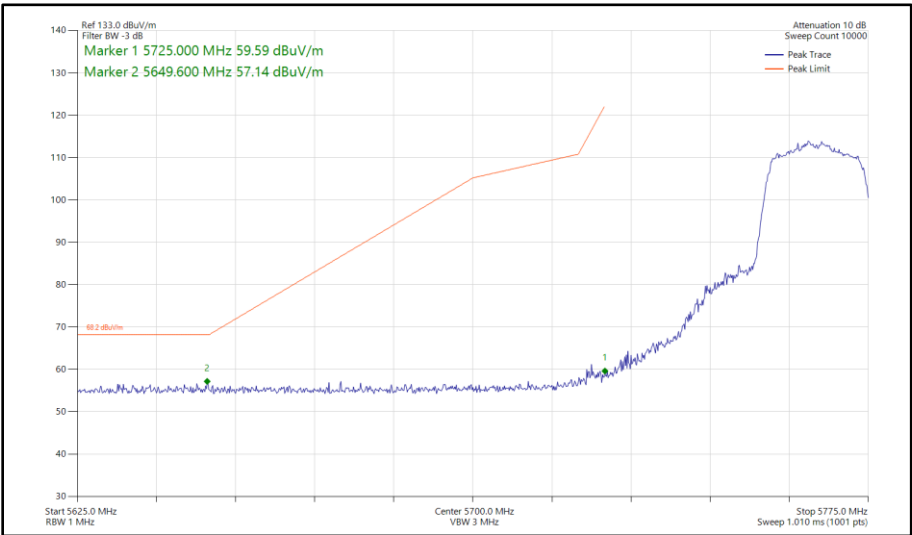
Figure 437 - 802.11n HT20, SISO, Core 1 - 5765 MHz Band Edge Frequency 5725 MHz
