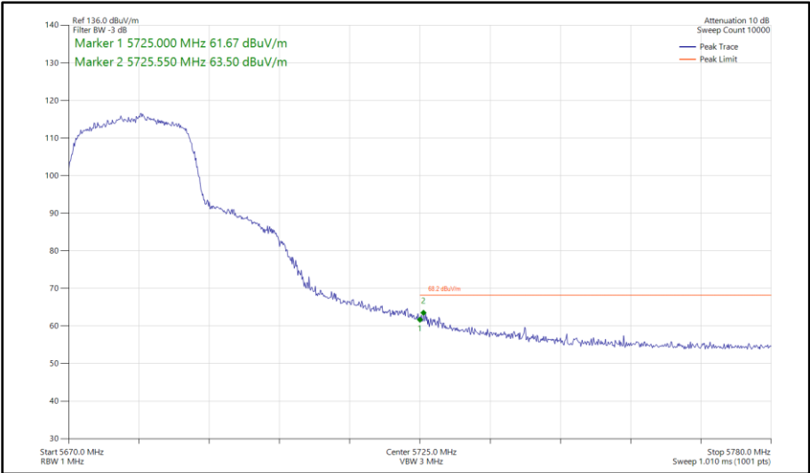
Figure 443 - 802.11n HT20, SISO, Core 1 - 5680 MHz Band Edge Frequency 5725 MHz
