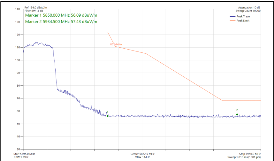
Figure 457 - 802.11ax HE20, SU, SISO, Core 1 - 5805 MHz Band Edge Frequency 5850 MHz
