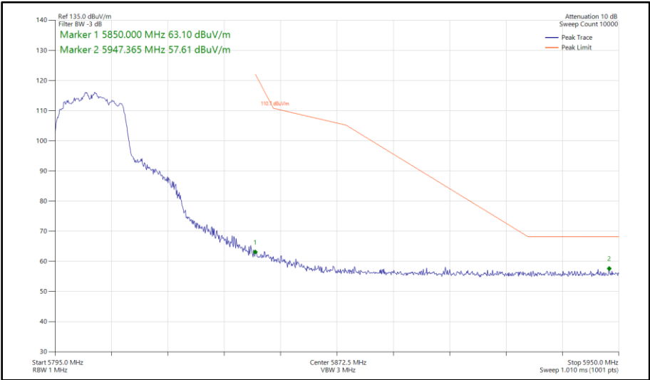
Figure 478 - 802.11n HT20, CDD, Core 0 - Core 1 - 5805 MHz Band Edge Frequency 5850 MHz
