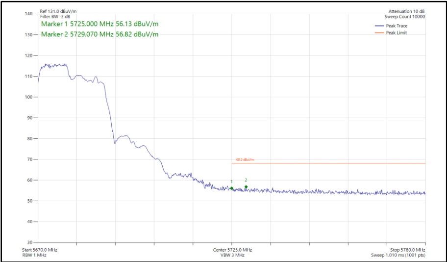
Figure 499 - 802.11ax HE20, RU 106-53, SDM, Core 0 - Core 1 - 5680 MHz Band Edge Frequency 5725 MHz
