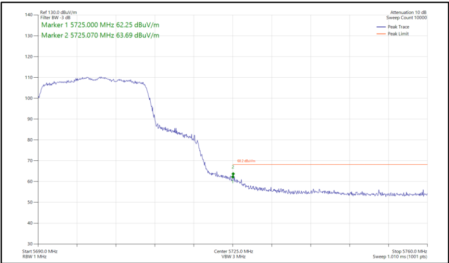
Figure 447 - 802.11ax HE20, SU, SISO, Core 1 - 5700 MHz Band Edge Frequency 5725 MHz
