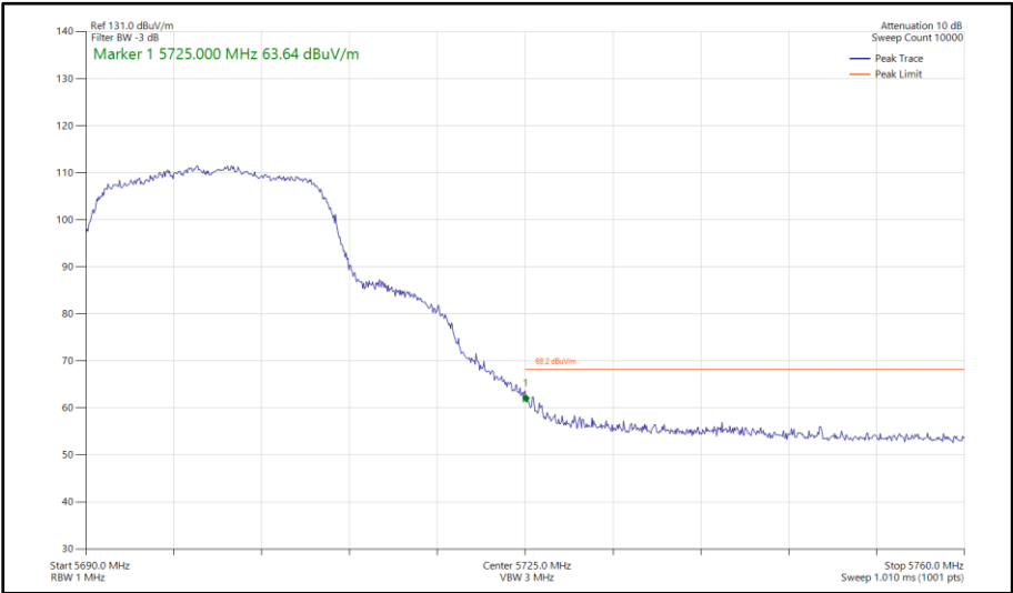
Figure 472 - 802.11n HT20, CDD, Core 0 - Core 1 - 5700 MHz Band Edge Frequency 5725 MHz
