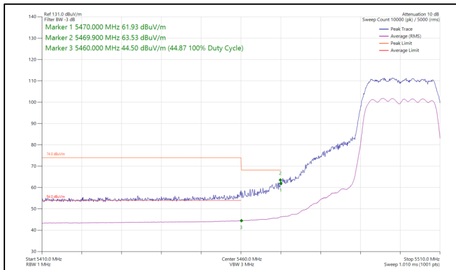
Figure 460 - 802.11n HT20, CDD, Core 0 - Core 1 - 5500 MHz Band Edge Frequency 5470 MHz
