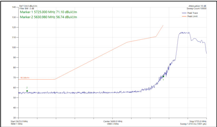
Figure 469 - 802.11ax HE20, RU 106-53, CDD, Core 0 - Core 1 - 5745 MHz Band Edge Frequency 5725 MHz
