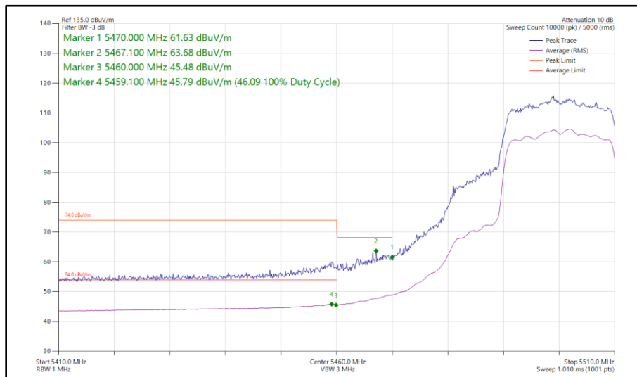
Figure 462 - 802.11ax HE20, SU, CDD, Core 0 - Core 1 - 5500 MHz Band Edge Frequency 5470 MHz
