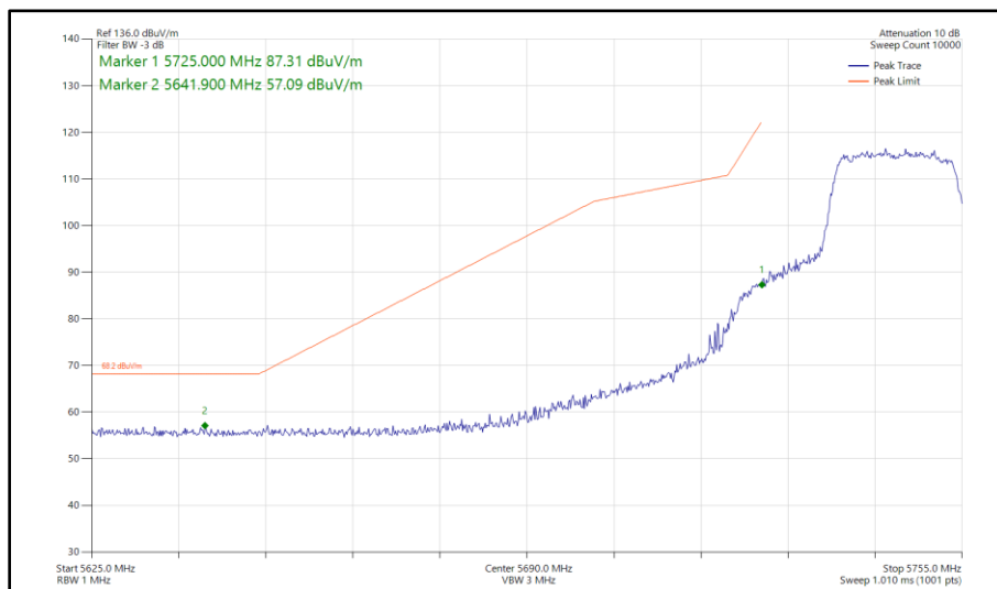
Figure 511 - 802.11ac VHT20, TxBF, Core 0 - Core 1 - 5745 MHz Band Edge Frequency 5725 MHz
