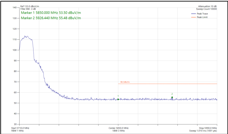
Figure 502 - 802.11n HT20, SDM, Core 0 - Core 1 - 5720 MHz Band Edge Frequency 5850 MHz
