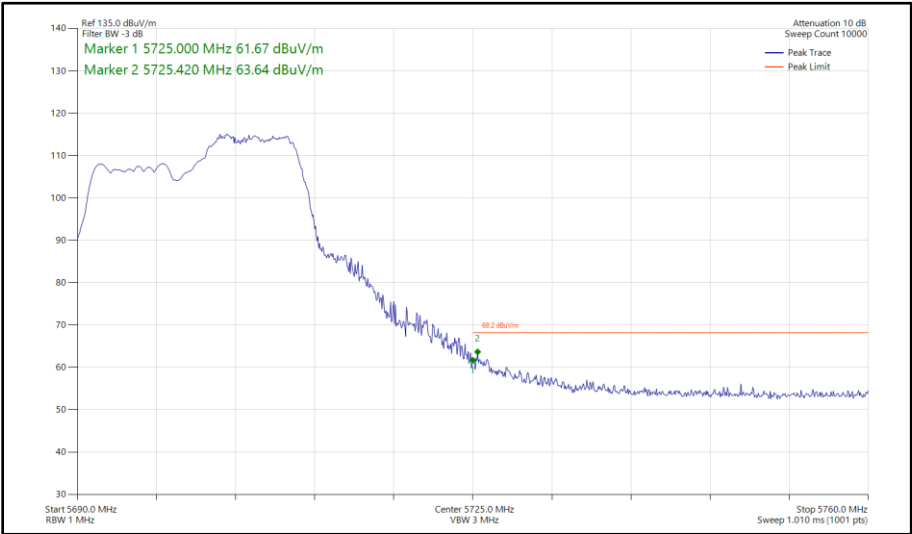
Figure 476 - 802.11ax HE20, RU 106-54, CDD, Core 0 - Core 1 - 5700 MHz Band Edge Frequency 5725 MHz
