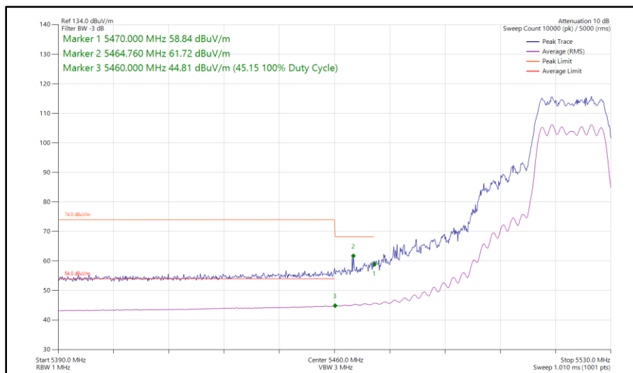
Figure 461 - 802.11n HT20, CDD, Core 0 - Core 1 - 5520 MHz Band Edge Frequency 5470 MHz
