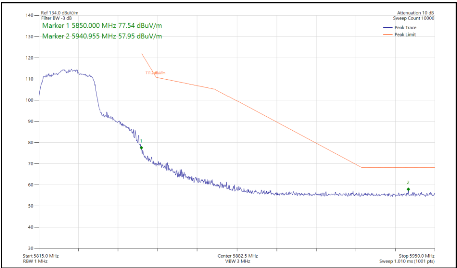
Figure 479 - 802.11n HT20, CDD, Core 0 - Core 1 - 5825 MHz Band Edge Frequency 5850 MHz
