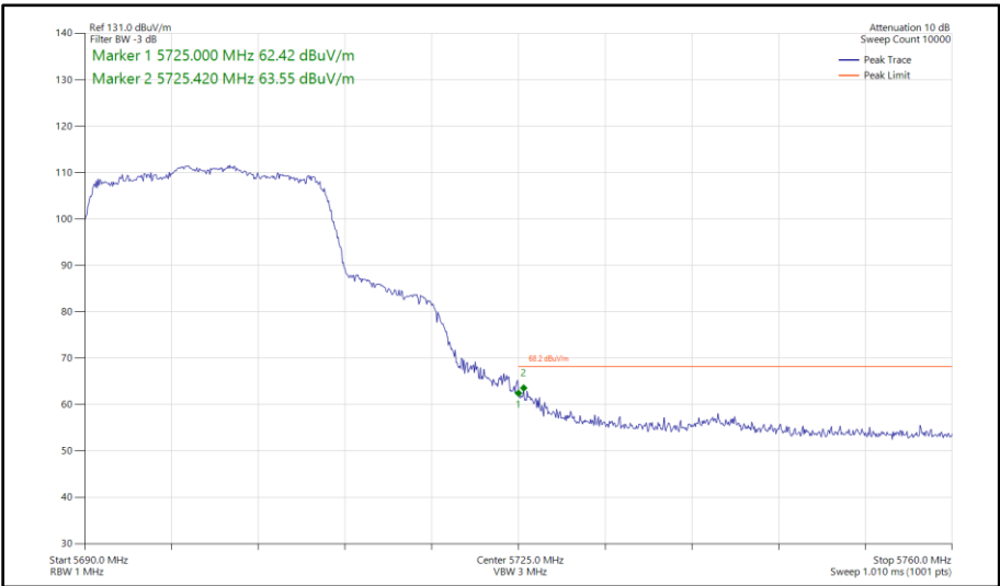
Figure 500 - 802.11ax HE20, SU, SDM, Core 0 - Core 1 - 5700 MHz Band Edge Frequency 5725 MHz
