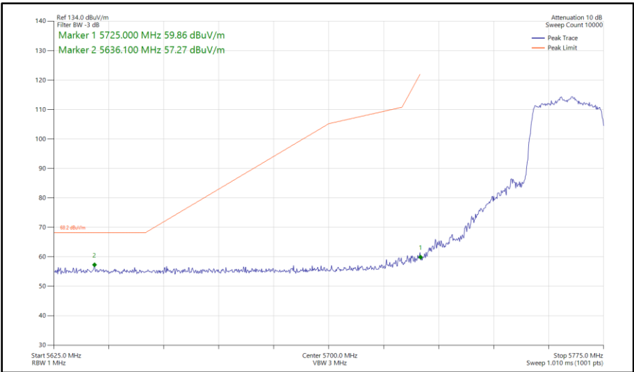
Figure 494 - 802.11ax HE20, SU, SDM, Core 0 - Core 1 - 5765 MHz Band Edge Frequency 5725 MHz
