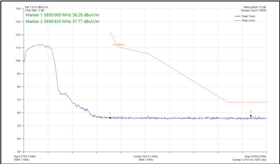
Figure 450 - 802.11a, SISO, Core 1 - 5805 MHz Band Edge Frequency 5850 MHz
