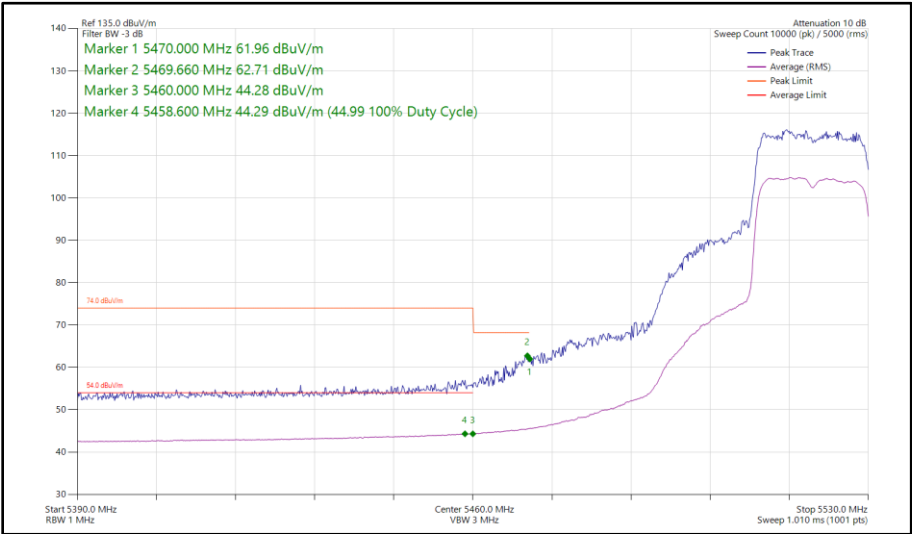
Figure 489 - 802.11ax HE20, SU, SDM, Core 0 - Core 1 - 5520 MHz Band Edge Frequency 5470 MHz
