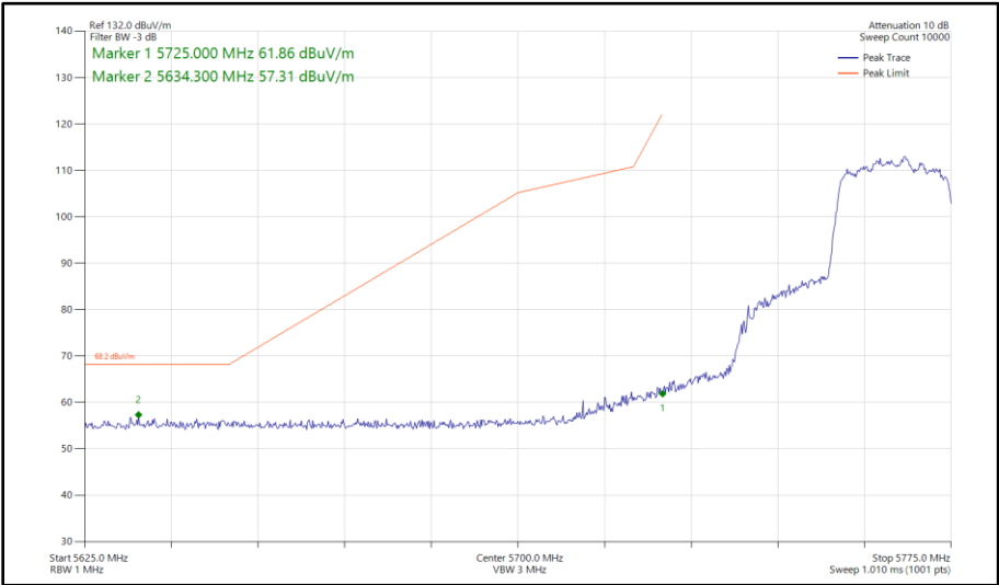
Figure 470 - 802.11ax HE20, SU, CDD, Core 0 - Core 1 - 5765 MHz Band Edge Frequency 5725 MHz
