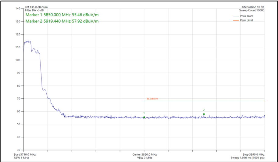
Figure 456 - 802.11ax HE20, RU 106-53, SISO, Core 1 - 5720 MHz Band Edge Frequency 5850 MHz
