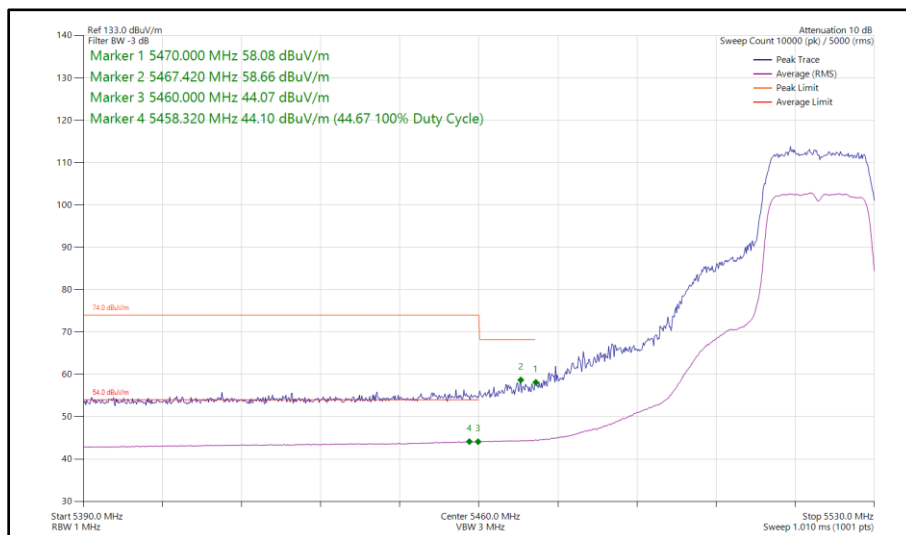
Figure 486 - 802.11n HT20, SDM, Core 0 - Core 1 - 5520 MHz Band Edge Frequency 5470 MHz
