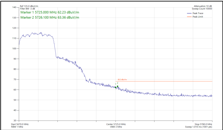
Figure 473 - 802.11ax HE20, SU, CDD, Core 0 - Core 1 - 5680 MHz Band Edge Frequency 5725 MHz
