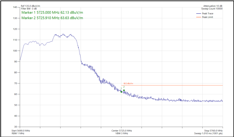
Figure 501 - 802.11ax HE20, RU 106-54, SDM, Core 0 - Core 1 - 5700 MHz Band Edge Frequency 5725 MHz
