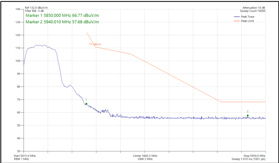
Figure 451 - 802.11a, SISO, Core 1 - 5825 MHz Band Edge Frequency 5850 MHz
