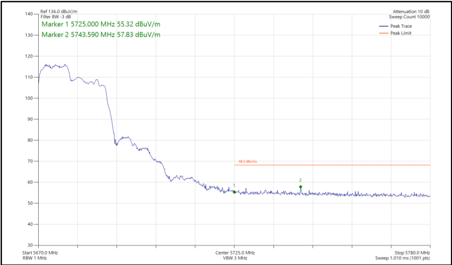
Figure 474 - 802.11ax HE20, RU 106-53, CDD, Core 0 - Core 1 - 5680 MHz Band Edge Frequency 5725 MHz
