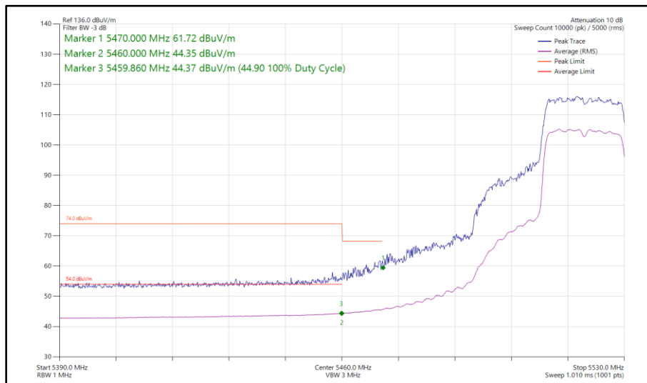
Figure 464 - 802.11ax HE20, SU, CDD, Core 0 - Core 1 - 5520 MHz Band Edge Frequency 5470 MHz
