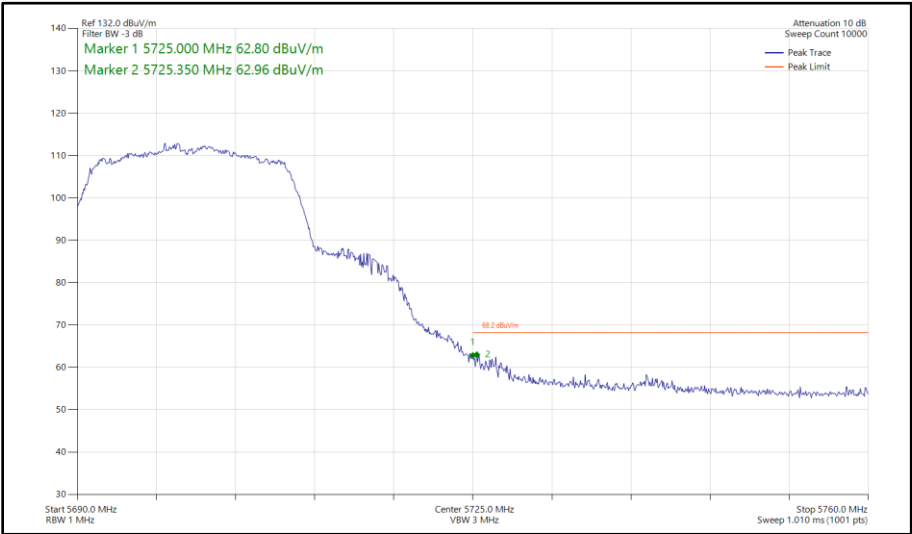
Figure 497 - 802.11n HT20, SDM, Core 0 - Core 1 - 5700 MHz Band Edge Frequency 5725 MHz
