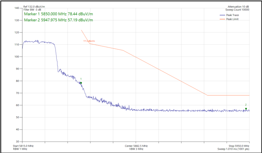
Figure 458 - 802.11ax HE20, SU, SISO, Core 1 - 5825 MHz Band Edge Frequency 5850 MHz
