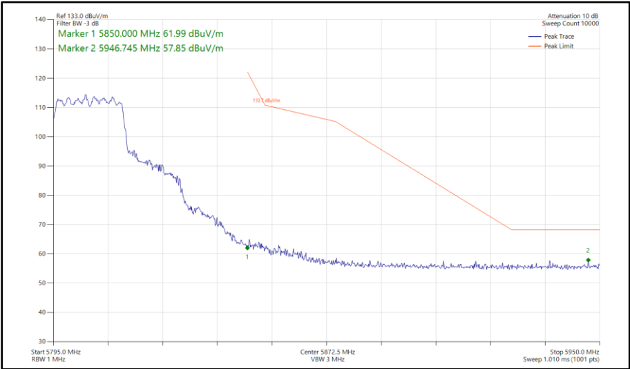
Figure 482 - 802.11ax HE20, SU, CDD, Core 0 - Core 1 - 5805 MHz Band Edge Frequency 5850 MHz
