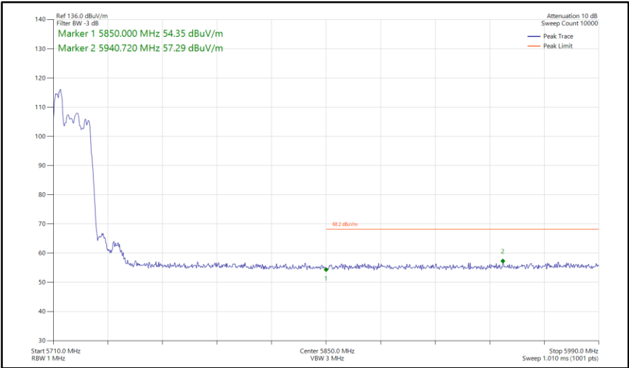
Figure 505 - 802.11ax HE20, RU 52-37, SDM, Core 0 - Core 1 - 5720 MHz Band Edge Frequency 5850 MHz
