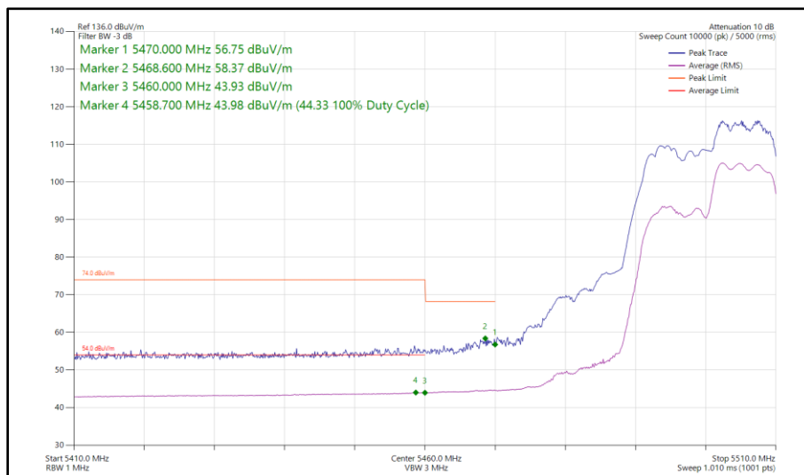
Figure 488 - 802.11ax HE20, RU 106-54, SDM, Core 0 - Core 1 - 5500 MHz Band Edge Frequency 5470 MHz
