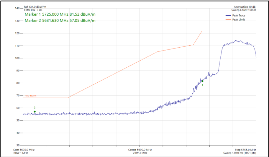
Figure 466 - 802.11n HT20, CDD, Core 0 - Core 1 - 5745 MHz Band Edge Frequency 5725 MHz
