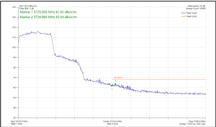
Figure 498 - 802.11ax HE20, SU, SDM, Core 0 - Core 1 - 5680 MHz Band Edge Frequency 5725 MHz
