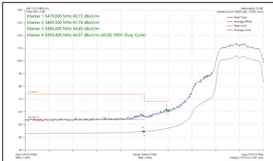
Figure 485 - 802.11n HT20, SDM, Core 0 - Core 1 - 5500 MHz Band Edge Frequency 5470 MHz
