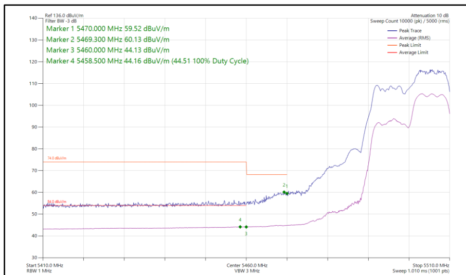
Figure 463 - 802.11ax HE20, RU 106-54, CDD, Core 0 - Core 1 - 5500 MHz Band Edge Frequency 5470 MHz
