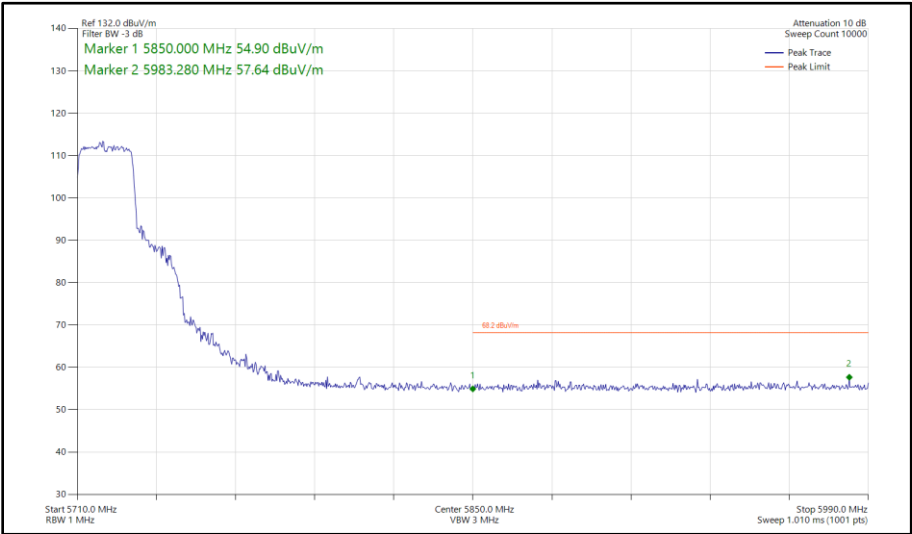
Figure 480 - 802.11ax HE20, SU, CDD, Core 0 - Core 1 - 5720 MHz Band Edge Frequency 5850 MHz
