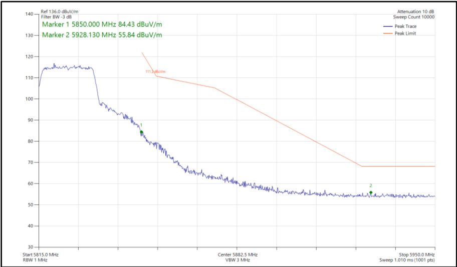
Figure 503 - 802.11n HT20, SDM, Core 0 - Core 1 - 5825 MHz Band Edge Frequency 5850 MHz
