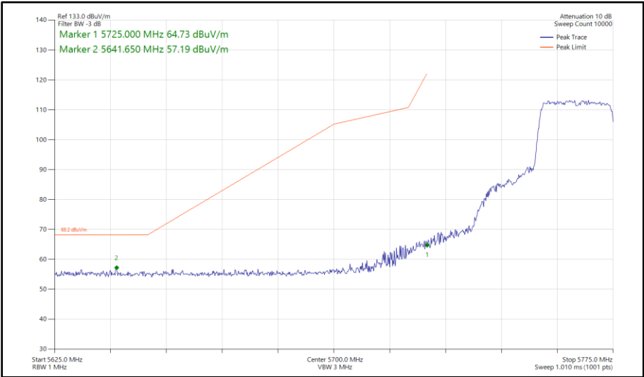
Figure 440 - 802.11ax HE20, SU, SISO, Core 1 - 5765 MHz Band Edge Frequency 5725 MHz
