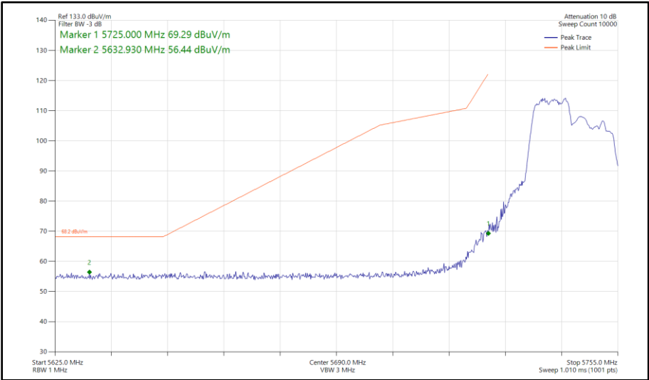
Figure 493 - 802.11ax HE20, RU 106-53, SDM, Core 0 - Core 1 - 5745 MHz Band Edge Frequency 5725 MHz
