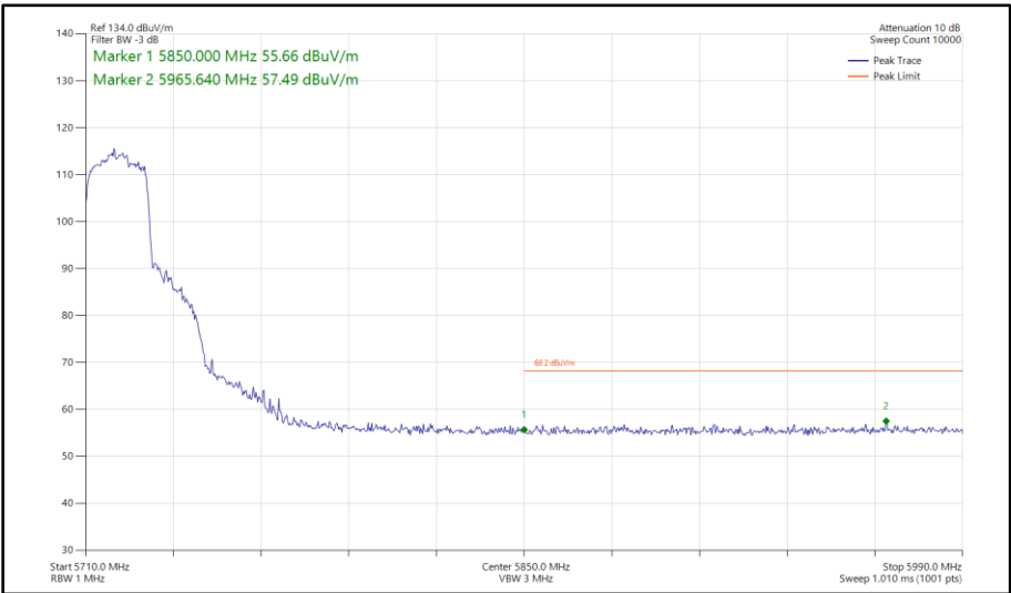
Figure 455 - 802.11ax HE20, SU, SISO, Core 1 - 5720 MHz Band Edge Frequency 5850 MHz
