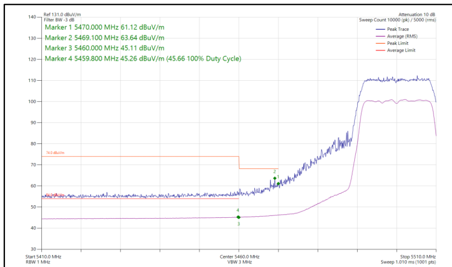
Figure 509 - 802.11ac VHT20, TxBF, Core 0 - Core 1 - 5500 MHz Band Edge Frequency 5470 MHz
