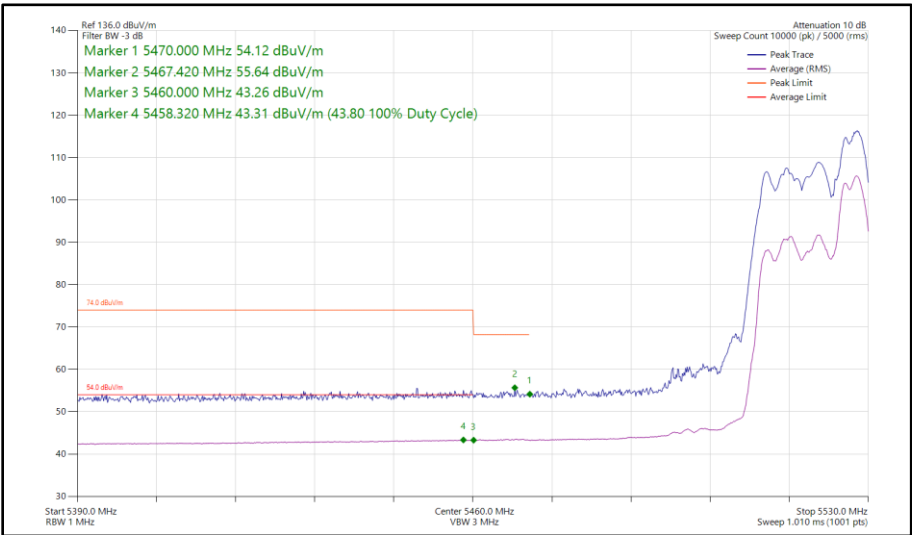
Figure 490 - 802.11ax HE20, RU 52-40, SDM, Core 0 - Core 1 - 5520 MHz Band Edge Frequency 5470 MHz
