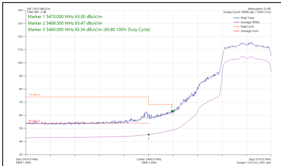
Figure 487 - 802.11ax HE20, SU, SDM, Core 0 - Core 1 - 5500 MHz Band Edge Frequency 5470 MHz
