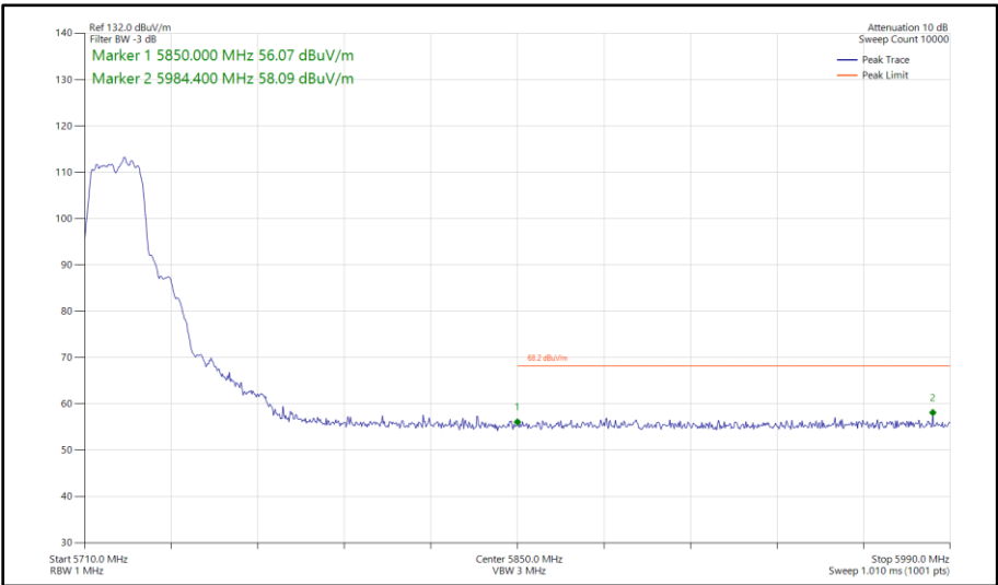
Figure 449 - 802.11a, SISO, Core 1 - 5720 MHz Band Edge Frequency 5850 MHz
