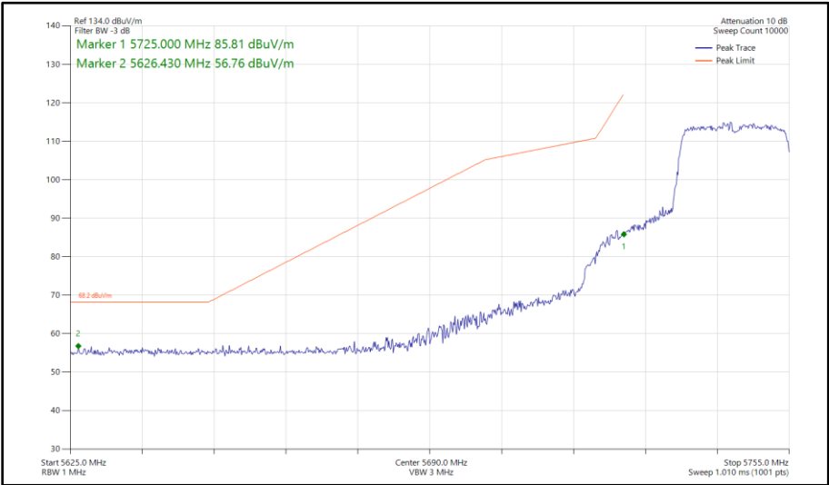
Figure 438 - 802.11ax HE20, SU, SISO, Core 1 - 5745 MHz Band Edge Frequency 5725 MHz
