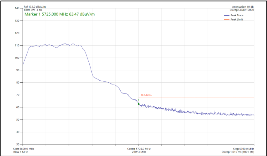
Figure 442 - 802.11a, SISO, Core 1 - 5700 MHz Band Edge Frequency 5725 MHz
