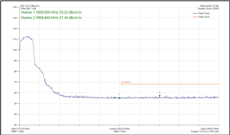
Figure 452 - 802.11n HT20, SISO, Core 1 - 5720 MHz Band Edge Frequency 5850 MHz
