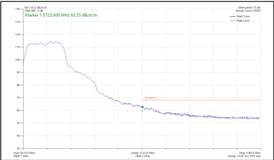
Figure 441 - 802.11a, SISO, Core 1 - 5680 MHz Band Edge Frequency 5725 MHz
