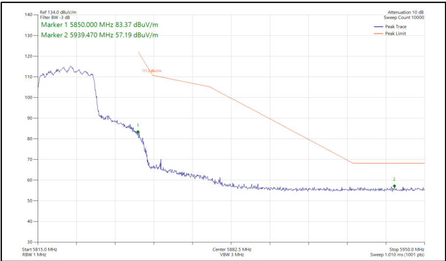
Figure 483 - 802.11ax HE20, SU, CDD, Core 0 - Core 1 - 5825 MHz Band Edge Frequency 5850 MHz
