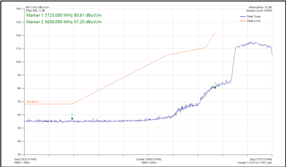
Figure 468 - 802.11ax HE20, SU, CDD, Core 0 - Core 1 - 5745 MHz Band Edge Frequency 5725 MHz
