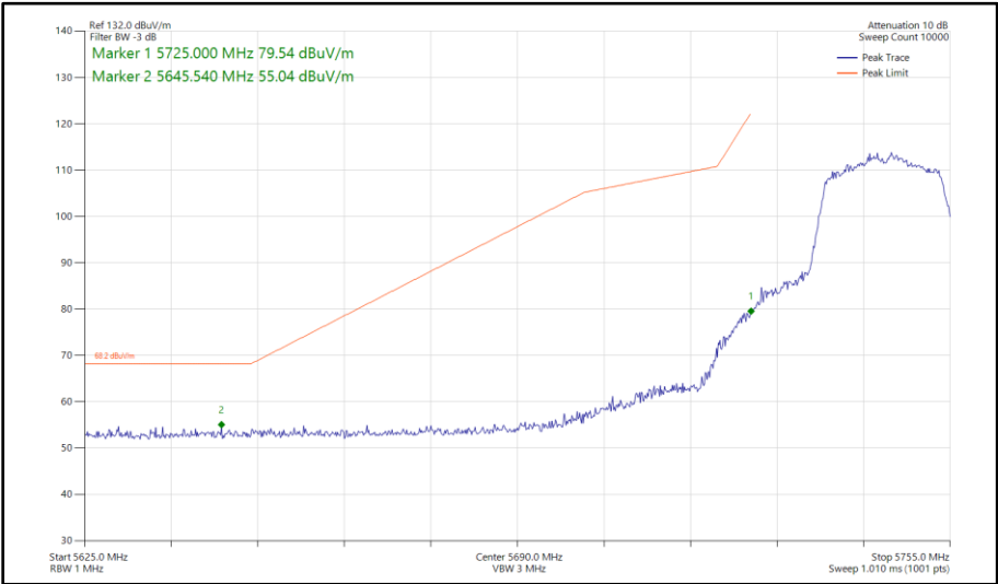
Figure 491 - 802.11n HT20, SDM, Core 0 - Core 1 - 5745 MHz Band Edge Frequency 5725 MHz
