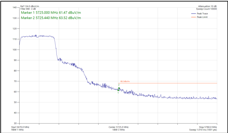
Figure 445 - 802.11ax HE20, SU, SISO, Core 1 - 5680 MHz Band Edge Frequency 5725 MHz
