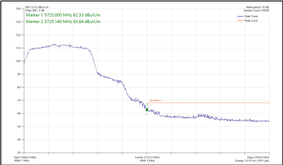
Figure 444 - 802.11n HT20, SISO, Core 1 - 5700 MHz Band Edge Frequency 5725 MHz
