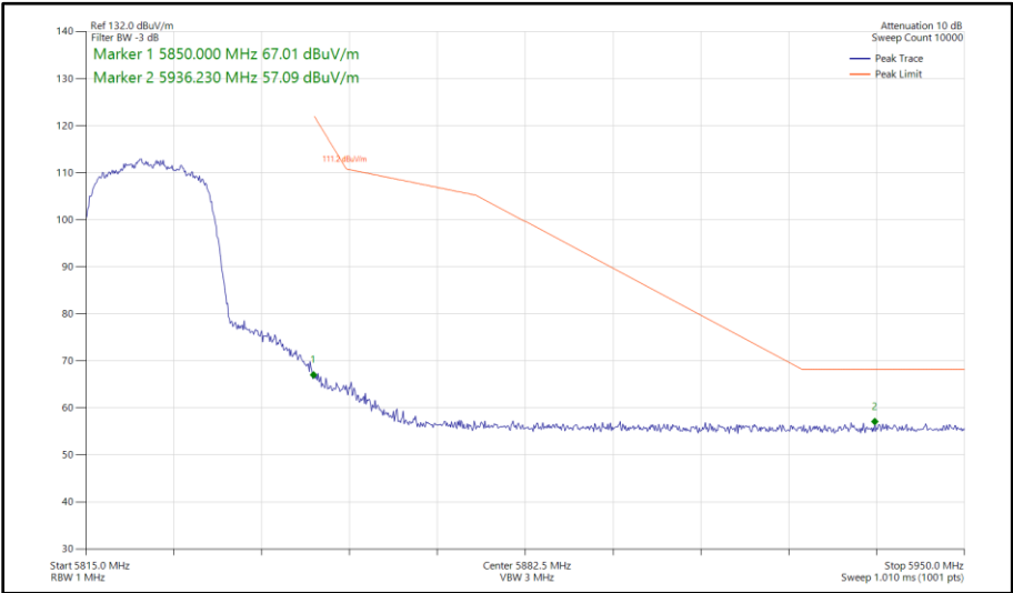
Figure 454 - 802.11n HT20, SISO, Core 1 - 5825 MHz Band Edge Frequency 5850 MHz
