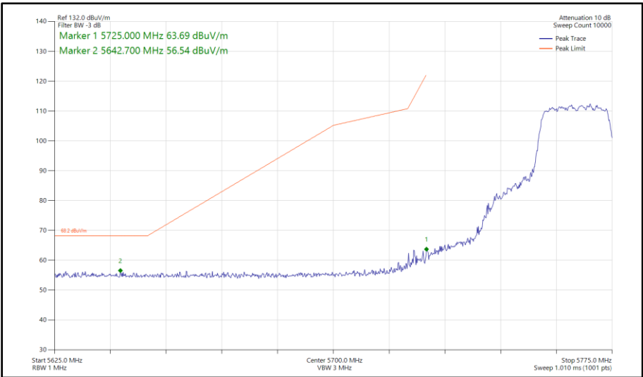
Figure 467 - 802.11n HT20, CDD, Core 0 - Core 1 - 5765 MHz Band Edge Frequency 5725 MHz
