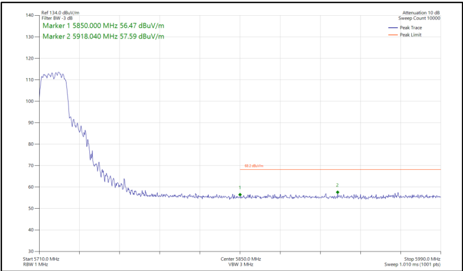
Figure 477 - 802.11n HT20, CDD, Core 0 - Core 1 - 5720 MHz Band Edge Frequency 5850 MHz
