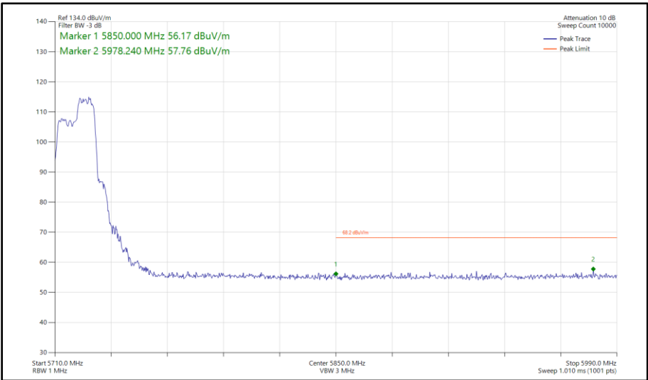
Figure 481 - 802.11ax HE20, RU 106-54, CDD, Core 0 - Core 1 - 5720 MHz Band Edge Frequency 5850 MHz
