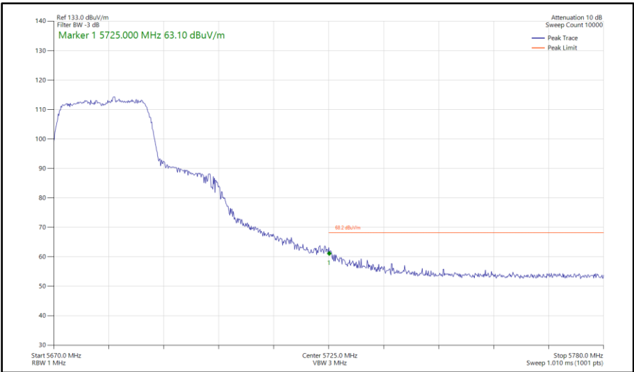
Figure 496 - 802.11n HT20, SDM, Core 0 - Core 1 - 5680 MHz Band Edge Frequency 5725 MHz
