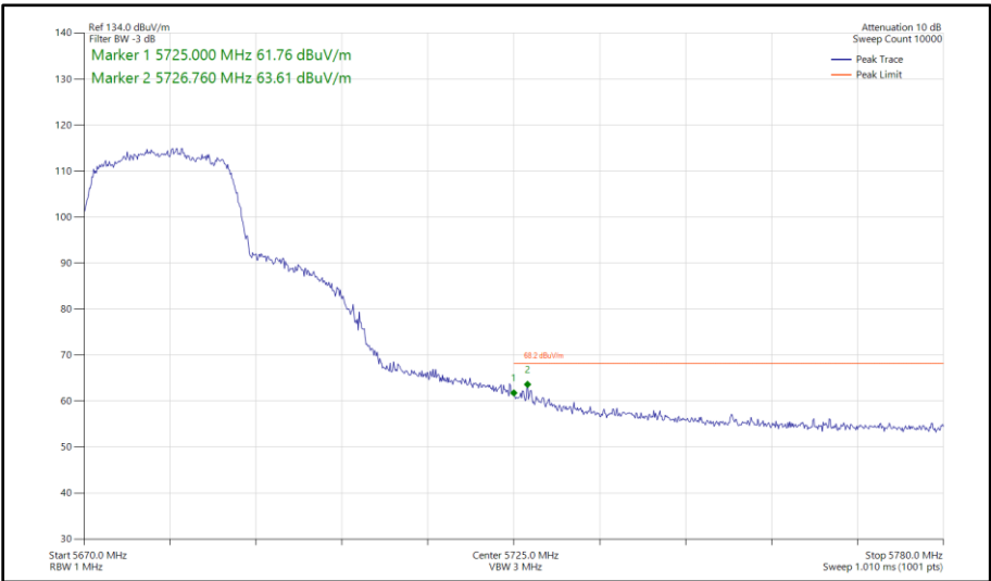
Figure 471 - 802.11n HT20, CDD, Core 0 - Core 1 - 5680 MHz Band Edge Frequency 5725 MHz
