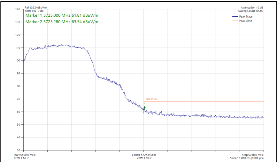
Figure 513 - 802.11ac VHT20, TxBF, Core 0 - Core 1 - 5700 MHz Band Edge Frequency 5725 MHz
