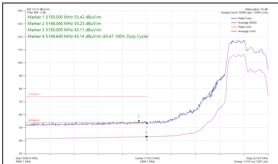
Figure 71 - 802.11ax HE20, RU 106-53, SDM, Core 0 - Core 1 - 5200 MHz Band Edge Frequency 5150 MHz
