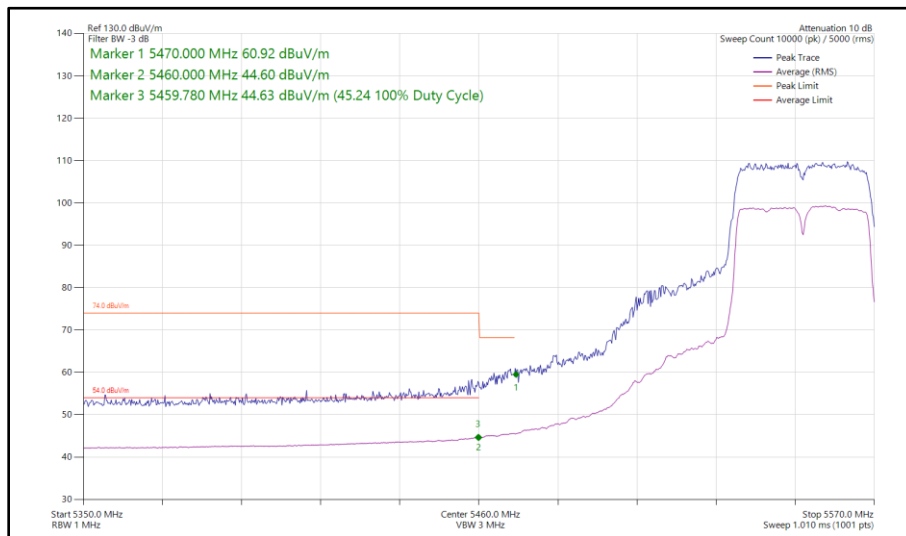
Figure 120 - 802.11n HT40, SISO, Core 1 - 5550 MHz Band Edge Frequency 5460 MHz
