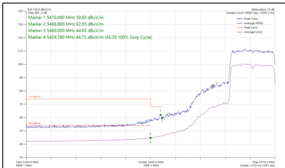
Figure 105 - 802.11ax HE40, SU, SISO, Core 0 - 5550 MHz Band Edge Frequency 5460 MHz
