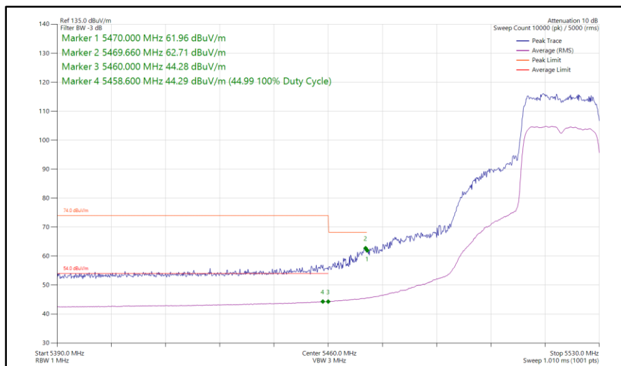
Figure 81 - 802.11ax HE20, SU, SDM, Core 0 - Core 1 - 5520 MHz Band Edge Frequency 5460 MHz
