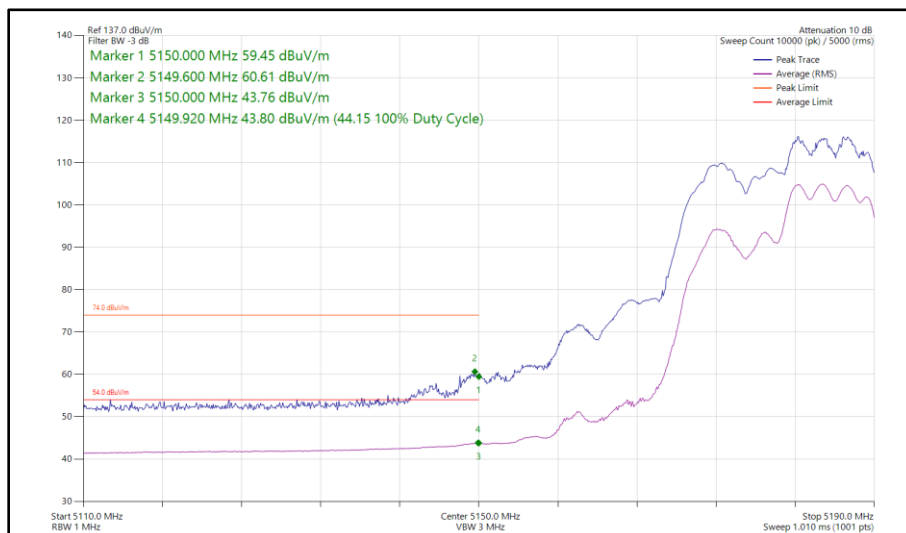
Figure 69 - 802.11ax HE20, RU 106-54, SDM, Core 0 - Core 1 - 5180 MHz Band Edge Frequency 5150 MHz
