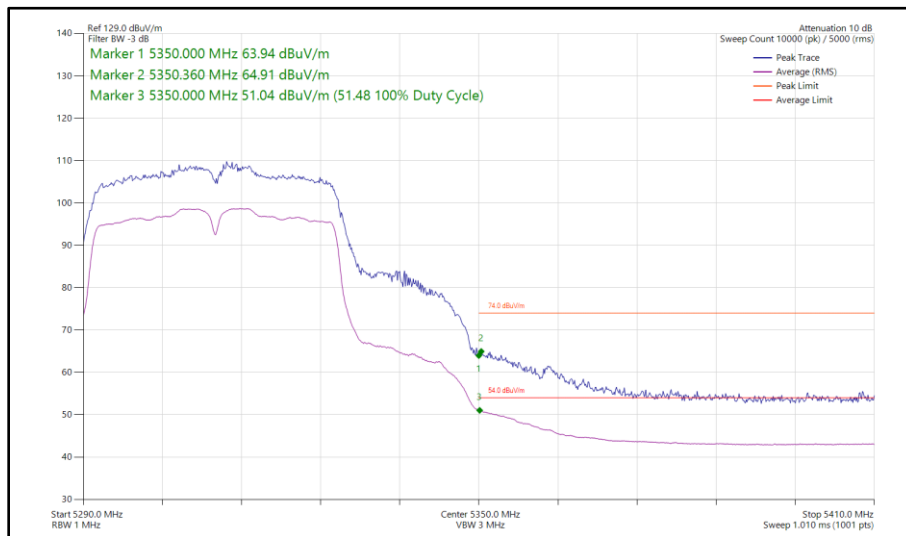
Figure 96 - 802.11n HT40, SISO, Core 0 - 5310 MHz Band Edge Frequency 5350 MHz
