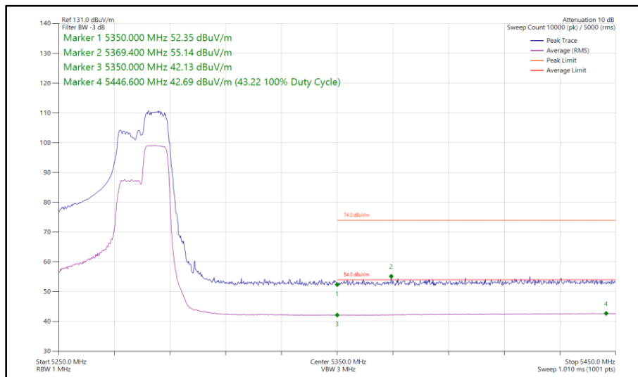
Figure 98 - 802.11ax HE40, RU 106-56, SISO, Core 0 - 5270 MHz Band Edge Frequency 5350 MHz
