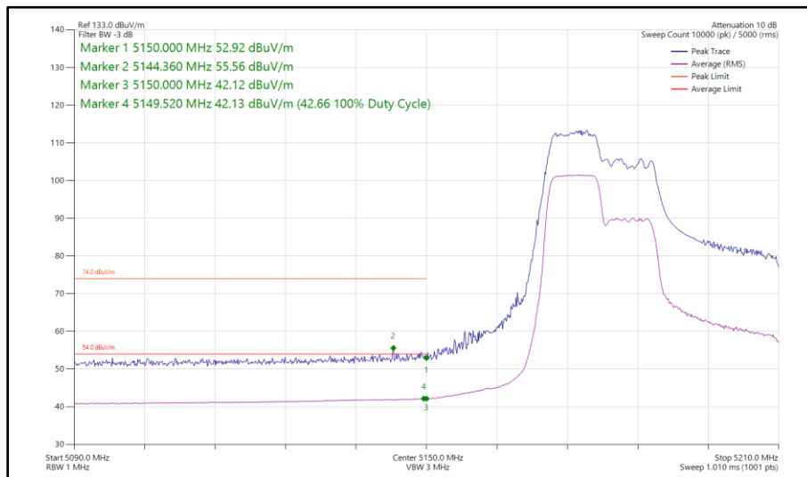
Figure 110 - 802.11ax HE40, RU 106-53, SISO, Core 1 - 5190 MHz Band Edge Frequency 5150 MHz
