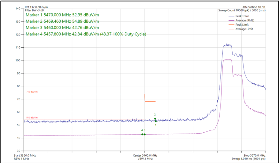
Figure 106 - 802.11ax HE40, RU 106-53, SISO, Core 0 - 5550 MHz Band Edge Frequency 5460 MHz
