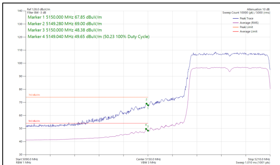
Figure 109 - 802.11ax HE40, SU, SISO, Core 1 - 5190 MHz Band Edge Frequency 5150 MHz
