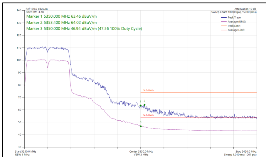
Figure 113 - 802.11n HT40, SISO, Core 1 - 5270 MHz Band Edge Frequency 5350 MHz
