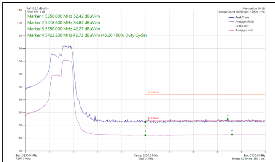
Figure 116 - 802.11ax HE40, RU 106-56, SISO, Core 1 - 5270 MHz Band Edge Frequency 5350 MHz
