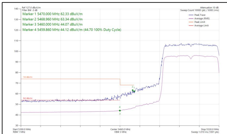
Figure 103 - 802.11ax HE40, SU, SISO, Core 0 - 5510 MHz Band Edge Frequency 5460 MHz
