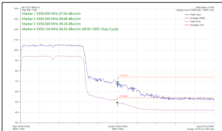
Figure 117 - 802.11ax HE40, SU, SISO, Core 1 - 5310 MHz Band Edge Frequency 5350 MHz
