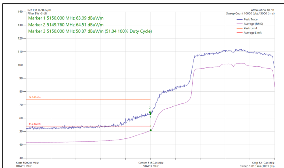
Figure 91 - 802.11ax HE40, SU, SISO, Core 0 - 5190 MHz Band Edge Frequency 5150 MHz
