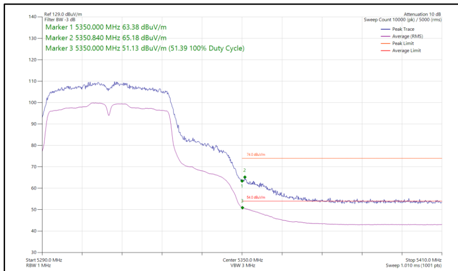
Figure 114 - 802.11n HT40, SISO, Core 1 - 5310 MHz Band Edge Frequency 5350 MHz
