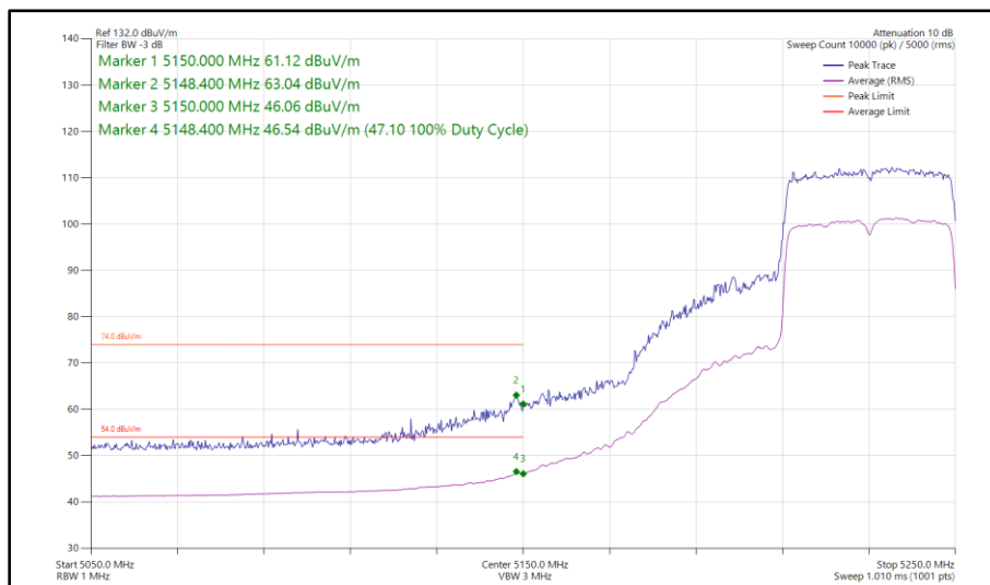
Figure 111 - 802.11ax HE40, SU, SISO, Core 1 - 5230 MHz Band Edge Frequency 5150 MHz
