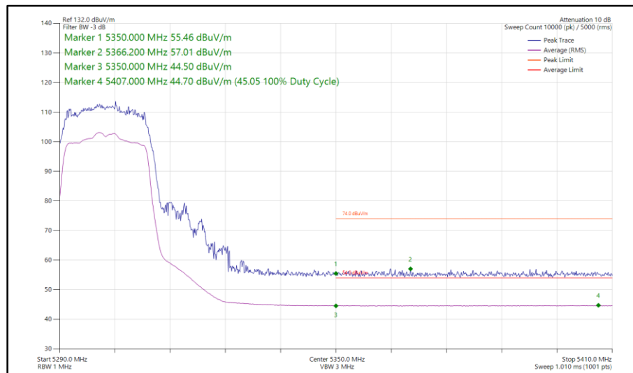
Figure 85 - 802.11ac VHT20, TxBF, Core 0 - Core 1 - 5300 MHz Band Edge Frequency 5350 MHz
