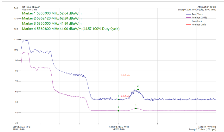
Figure 100 - 802.11ax HE40, RU 52-37, SISO, Core 0 - 5310 MHz Band Edge Frequency 5350 MHz
