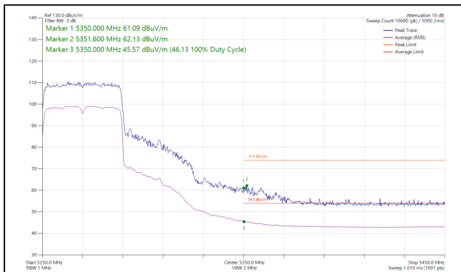
Figure 97 - 802.11ax HE40, SU, SISO, Core 0 - 5270 MHz Band Edge Frequency 5350 MHz
