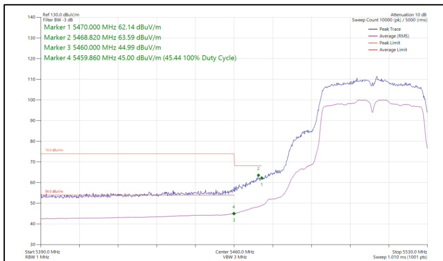
Figure 101 - 802.11n HT40, SISO, Core 0 - 5510 MHz Band Edge Frequency 5460 MHz
