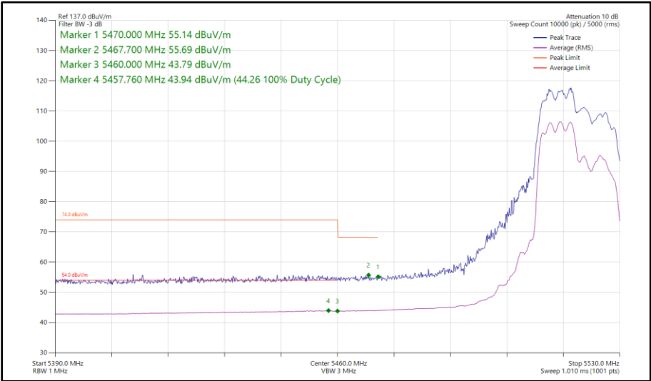
Figure 66 - 802.11ax HE20, RU 106-53, CDD, Core 0 - Core 1 - 5520 MHz Band Edge Frequency 5460 MHz
