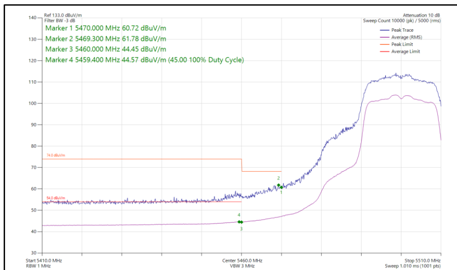
Figure 77 - 802.11n HT20, SDM, Core 0 - Core 1 - 5500 MHz Band Edge Frequency 5460 MHz
