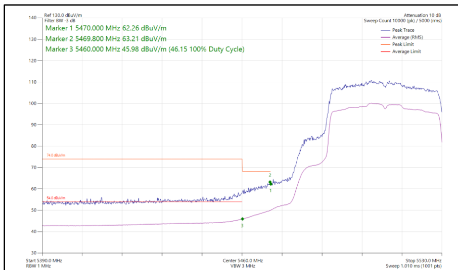
Figure 121 - 802.11ax HE40, SU, SISO, Core 1 - 5510 MHz Band Edge Frequency 5460 MHz
