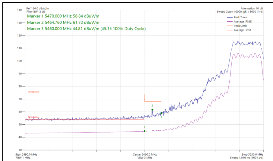
Figure 62 - 802.11n HT20, CDD, Core 0 - Core 1 - 5520 MHz Band Edge Frequency 5460 MHz
