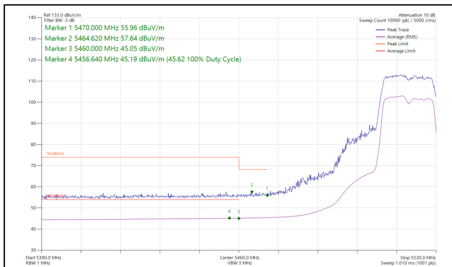
Figure 88 - 802.11ac VHT20, TxBF, Core 0 - Core 1 - 5520 MHz Band Edge Frequency 5460 MHz
