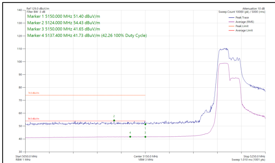
Figure 94 - 802.11ax HE40, RU 106-53, SISO, Core 0 - 5230 MHz Band Edge Frequency 5150 MHz
