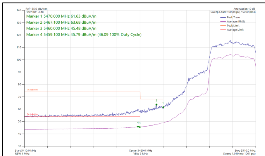
Figure 63 - 802.11ax HE20, SU, CDD, Core 0 - Core 1 - 5500 MHz Band Edge Frequency 5460 MHz
