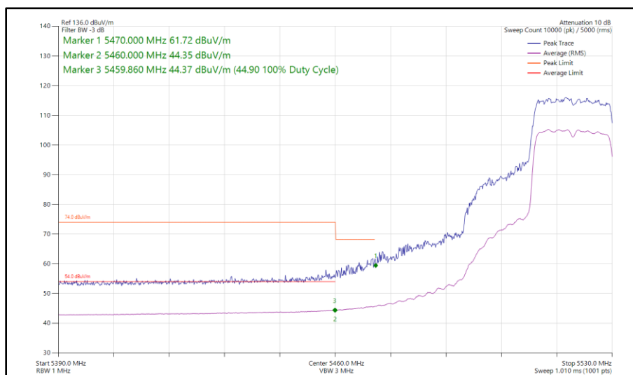
Figure 65 - 802.11ax HE20, SU, CDD, Core 0 - Core 1 - 5520 MHz Band Edge Frequency 5460 MHz
