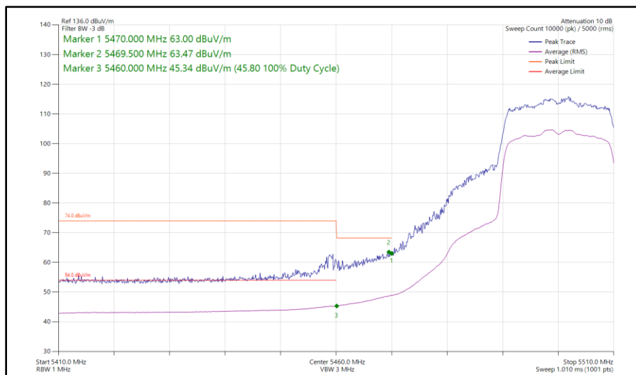
Figure 79 - 802.11ax HE20, SU, SDM, Core 0 - Core 1 - 5500 MHz Band Edge Frequency 5460 MHz
