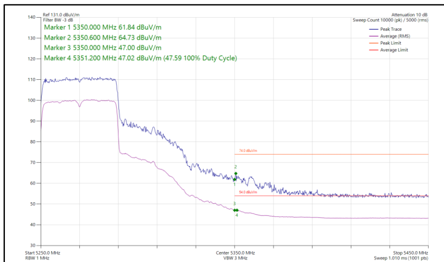
Figure 115 - 802.11ax HE40, SU, SISO, Core 1 - 5270 MHz Band Edge Frequency 5350 MHz
