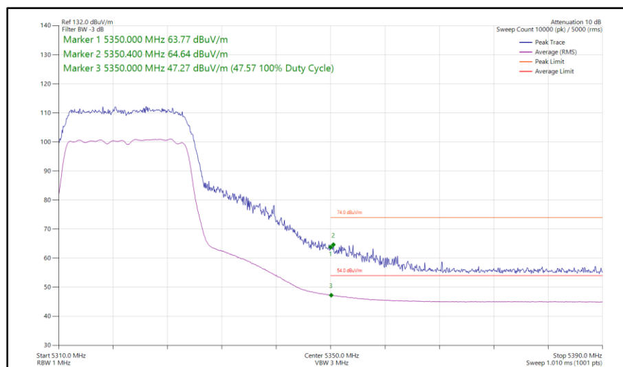
Figure 86 - 802.11ac VHT20, TxBF, Core 0 - Core 1 - 5320 MHz Band Edge Frequency 5350 MHz
