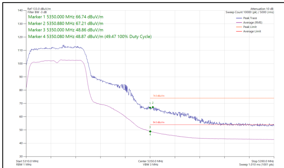
Figure 72 - 802.11n HT20, SDM, Core 0 - Core 1 - 5320 MHz Band Edge Frequency 5350 MHz
