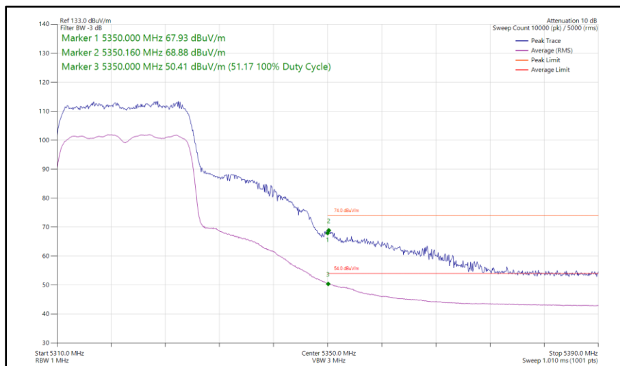
Figure 75 - 802.11ax HE20, SU, SDM, Core 0 - Core 1 - 5320 MHz Band Edge Frequency 5350 MHz
