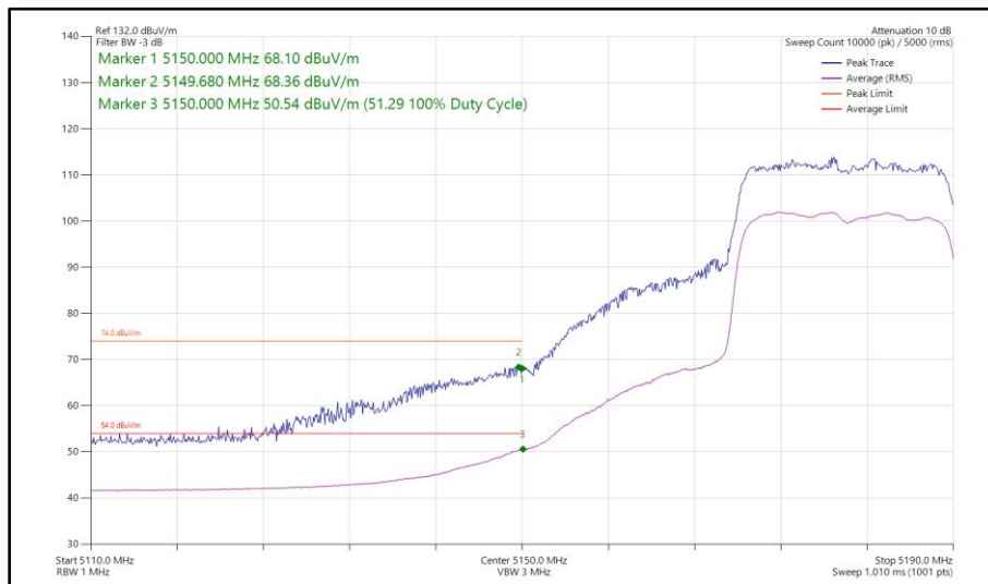
Figure 68 - 802.11ax HE20, SU, SDM, Core 0 - Core 1 - 5180 MHz Band Edge Frequency 5150 MHz
