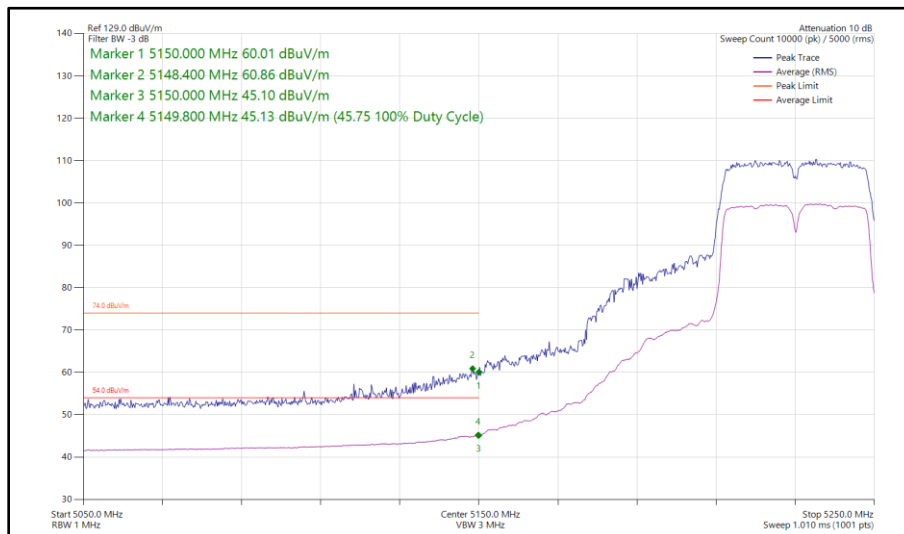
Figure 90 - 802.11n HT40, SISO, Core 0 - 5230 MHz Band Edge Frequency 5150 MHz
