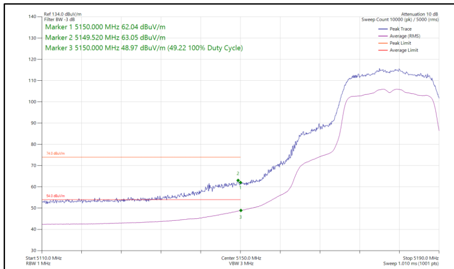
Figure 67 - 802.11n HT20, SDM, Core 0 - Core 1 - 5180 MHz Band Edge Frequency 5150 MHz
