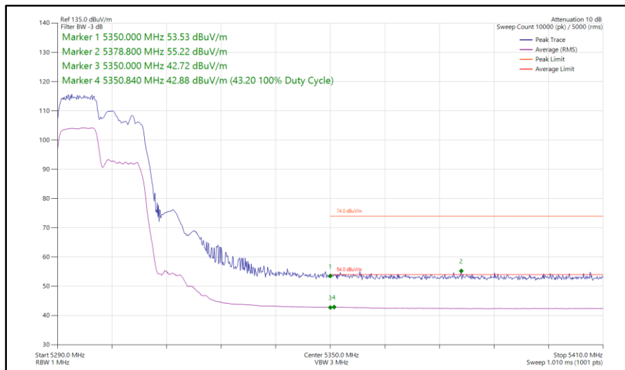
Figure 74 - 802.11ax HE20, RU 106-53, SDM, Core 0 - Core 1 - 5300 MHz Band Edge Frequency 5350 MHz
