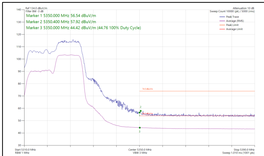
Figure 60 - 802.11ax HE20, RU 106-54, CDD, Core 0 - Core 1 - 5320 MHz Band Edge Frequency 5350 MHz
