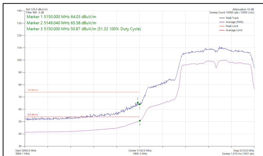
Figure 89 - 802.11n HT40, SISO, Core 0 - 5190 MHz Band Edge Frequency 5150 MHz
