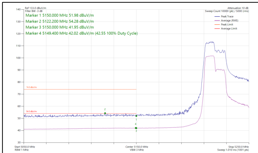
Figure 112 - 802.11ax HE40, RU 106-53, SISO, Core 1 - 5230 MHz Band Edge Frequency 5150 MHz
