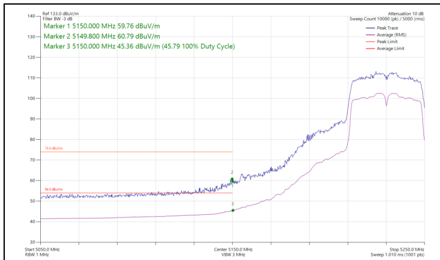
Figure 108 - 802.11n HT40, SISO, Core 1 - 5230 MHz Band Edge Frequency 5150 MHz
