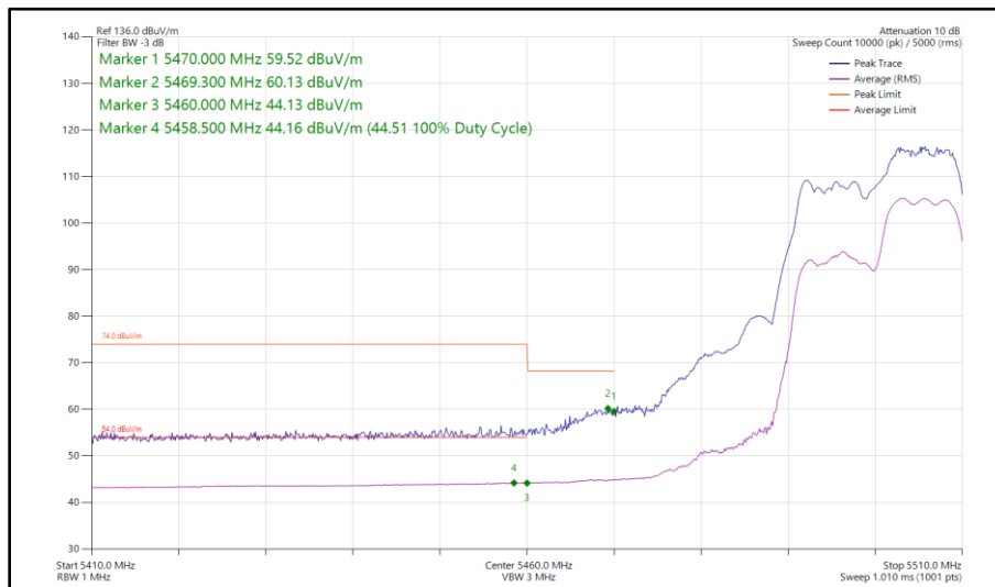
Figure 64 - 802.11ax HE20, RU 106-54, CDD, Core 0 - Core 1 - 5500 MHz Band Edge Frequency 5460 MHz
