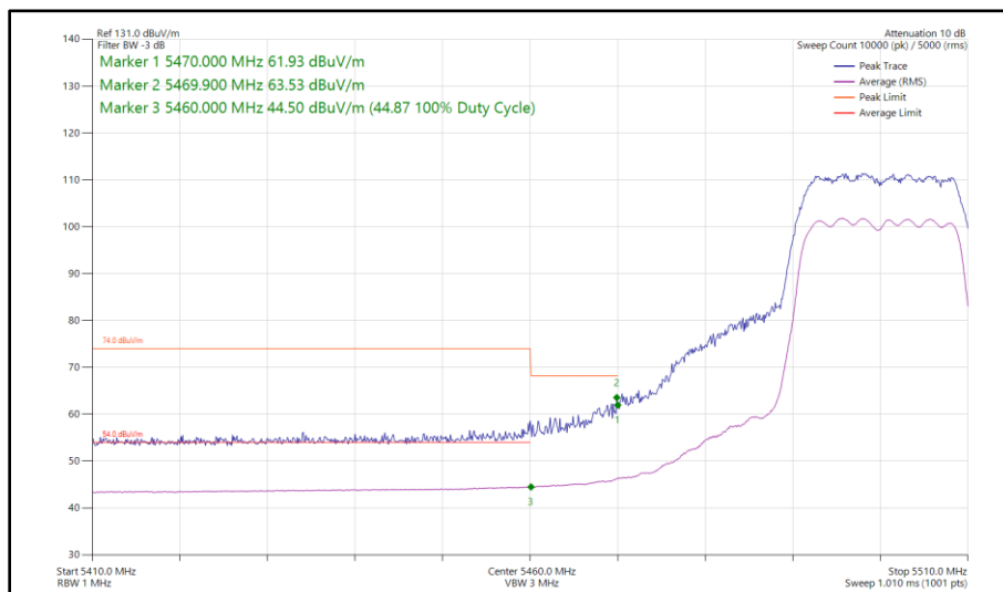
Figure 61 - 802.11n HT20, CDD, Core 0 - Core 1 - 5500 MHz Band Edge Frequency 5460 MHz
