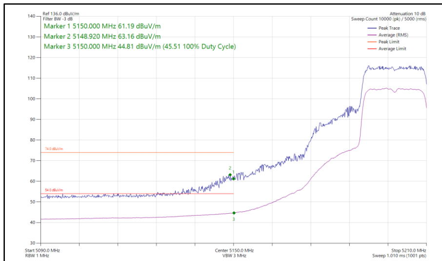
Figure 70 - 802.11ax HE20, SU, SDM, Core 0 - Core 1 - 5200 MHz Band Edge Frequency 5150 MHz
