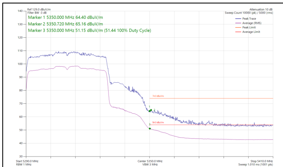
Figure 99 - 802.11ax HE40, SU, SISO, Core 0 - 5310 MHz Band Edge Frequency 5350 MHz
