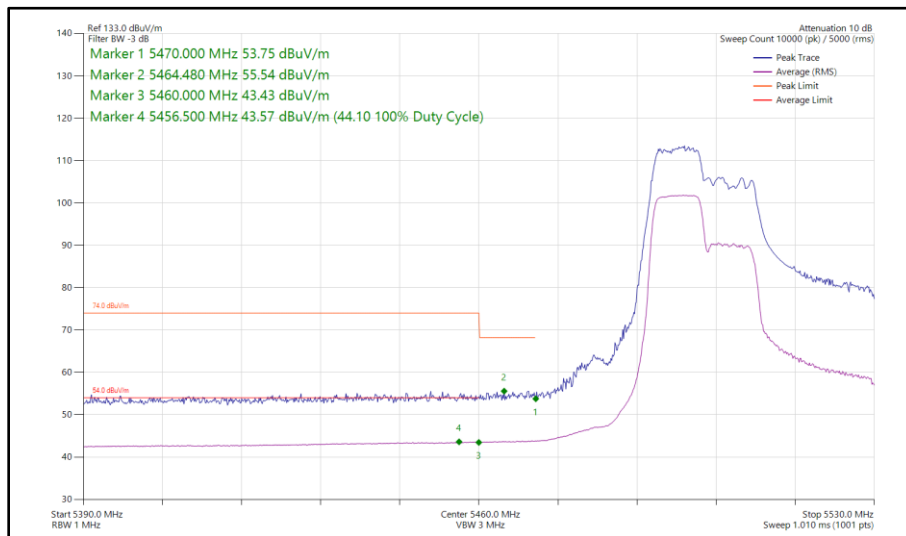
Figure 104 - 802.11ax HE40, RU 106-53, SISO, Core 0 - 5510 MHz Band Edge Frequency 5460 MHz
