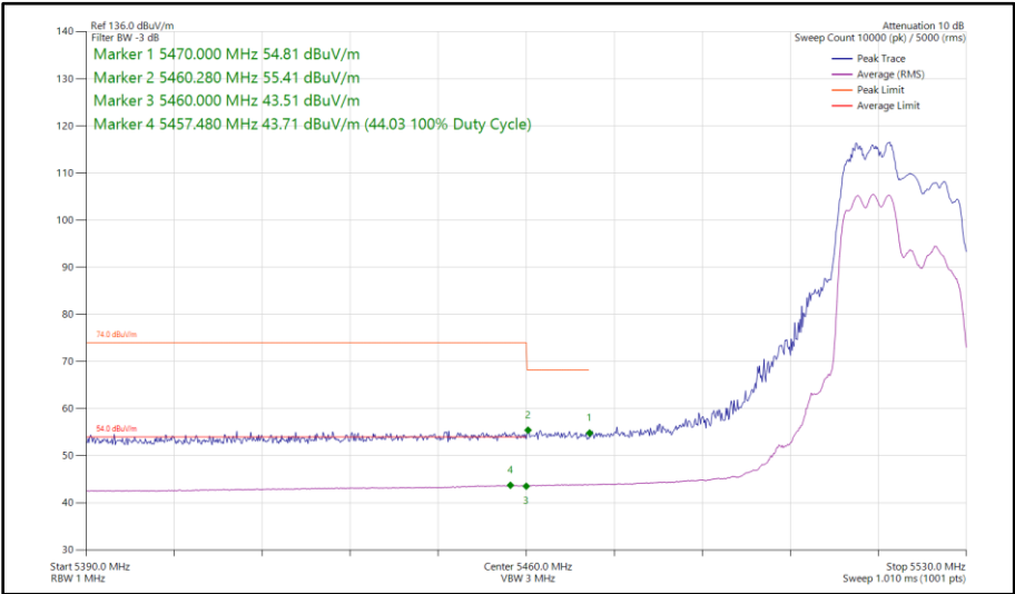
Figure 82 - 802.11ax HE20, RU 106-53, SDM, Core 0 - Core 1 - 5520 MHz Band Edge Frequency 5460 MHz
