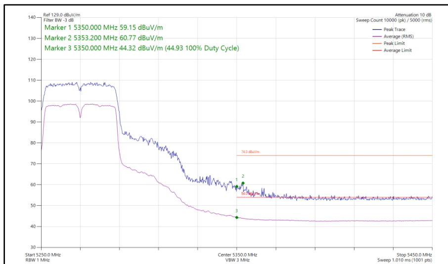
Figure 95 - 802.11n HT40, SISO, Core 0 - 5270 MHz Band Edge Frequency 5350 MHz
