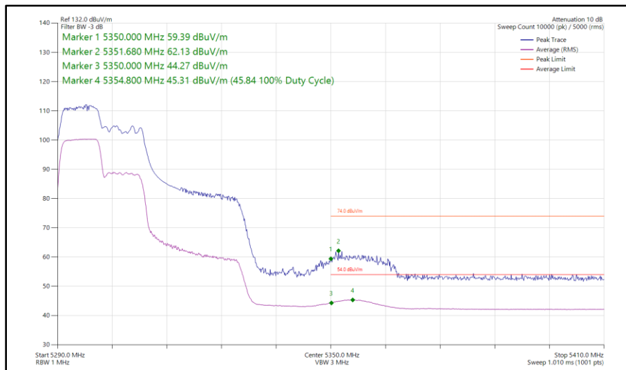
Figure 118 - 802.11ax HE40, RU 106-53, SISO, Core 1 - 5310 MHz Band Edge Frequency 5350 MHz
