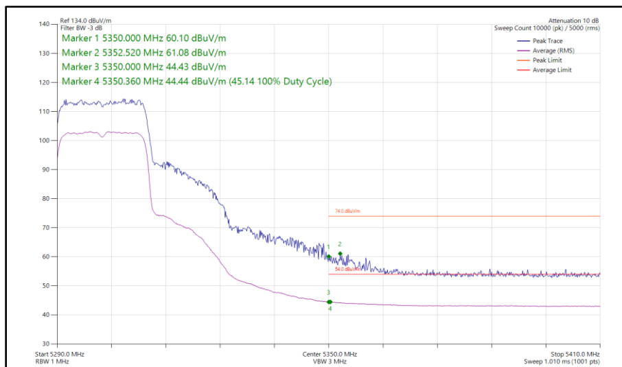
Figure 73 - 802.11ax HE20, SU, SDM, Core 0 - Core 1 - 5300 MHz Band Edge Frequency 5350 MHz
