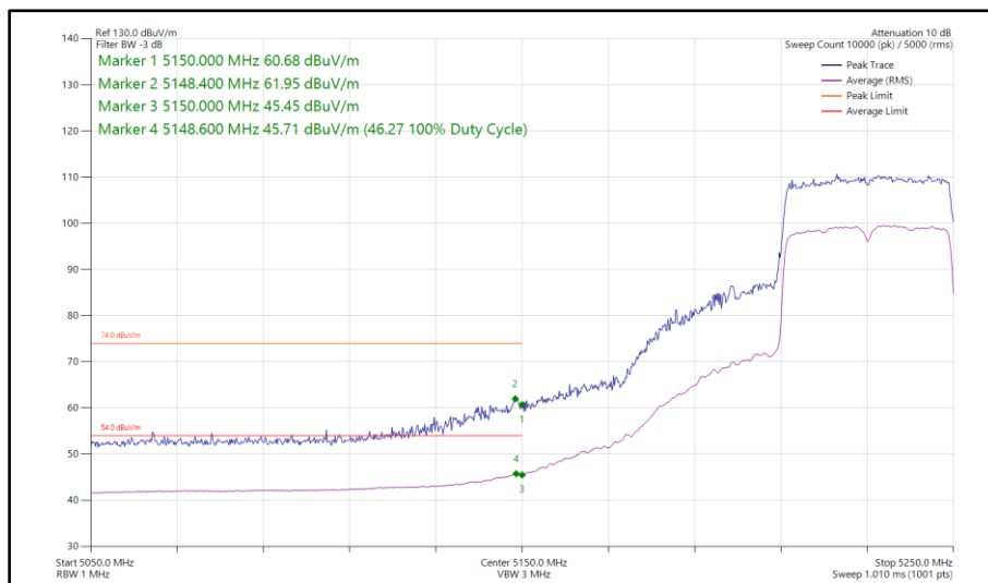
Figure 93 - 802.11ax HE40, SU, SISO, Core 0 - 5230 MHz Band Edge Frequency 5150 MHz
