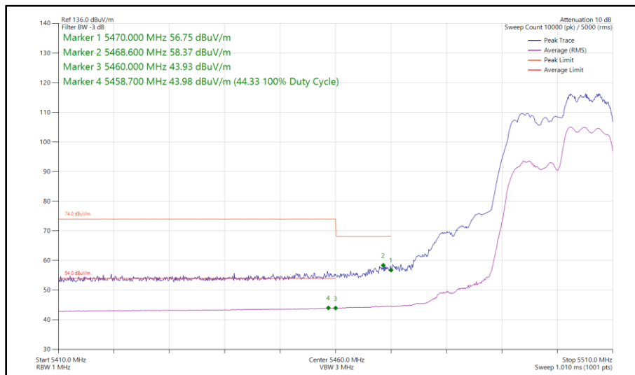
Figure 80 - 802.11ax HE20, RU 106-54, SDM, Core 0 - Core 1 - 5500 MHz Band Edge Frequency 5460 MHz
