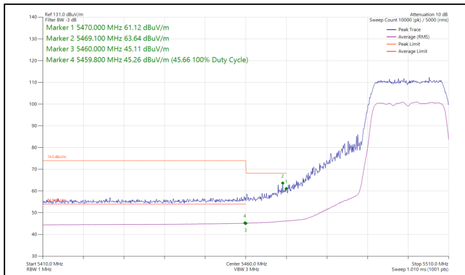
Figure 87 - 802.11ac VHT20, TxBF, Core 0 - Core 1 - 5500 MHz Band Edge Frequency 5460 MHz
