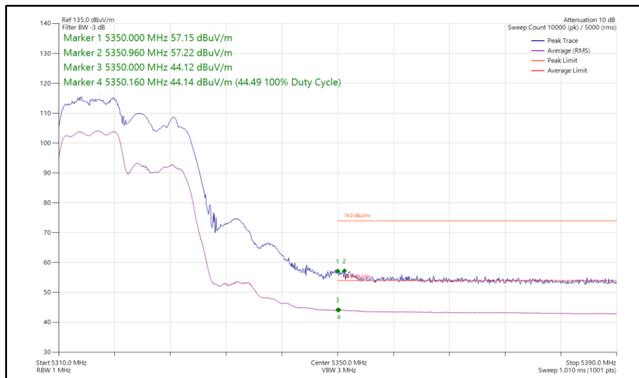
Figure 76 - 802.11ax HE20, RU 106-53, SDM, Core 0 - Core 1 - 5320 MHz Band Edge Frequency 5350 MHz
