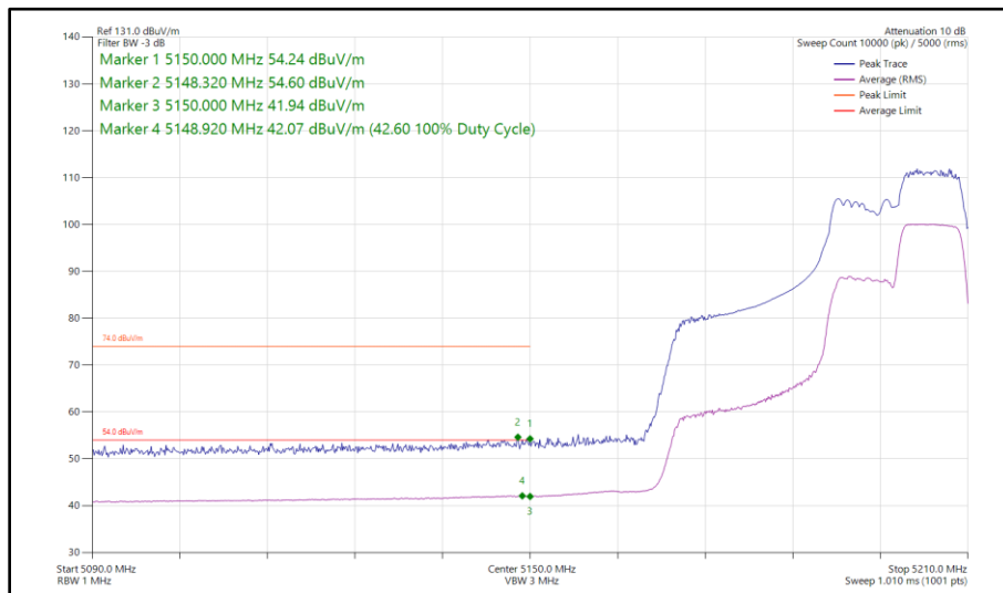
Figure 92 - 802.11ax HE40, RU 106-56, SISO, Core 0 - 5190 MHz Band Edge Frequency 5150 MHz
