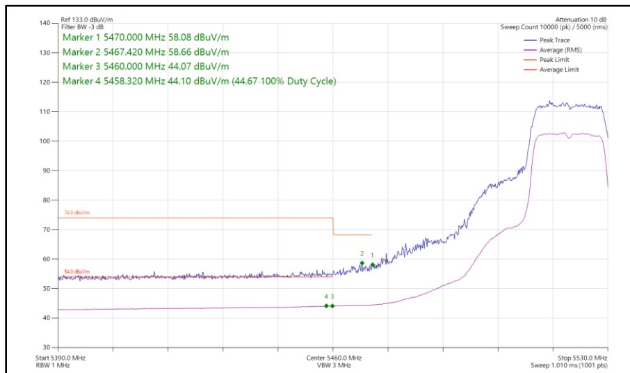
Figure 78 - 802.11n HT20, SDM, Core 0 - Core 1 - 5520 MHz Band Edge Frequency 5460 MHz
