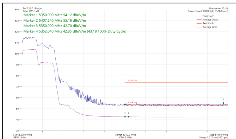
Figure 38 - 802.11ax HE20, RU 106-53, SISO, Core 1 - 5300 MHz Band Edge Frequency 5350 MHz
