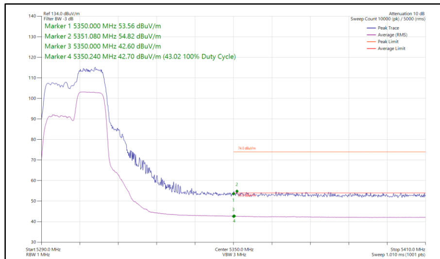
Figure 58 - 802.11ax HE20, RU 106-54, CDD, Core 0 - Core 1 - 5300 MHz Band Edge Frequency 5350 MHz
