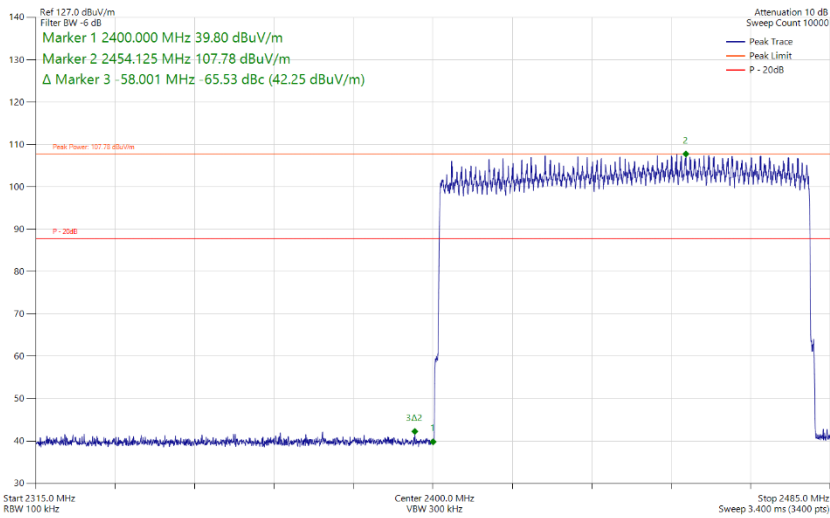
Figure 206 - Bluetooth 2-DH5, MIMO, Core 0 - Core 1 - Hopping Band Edge Frequency 2400 MHz
