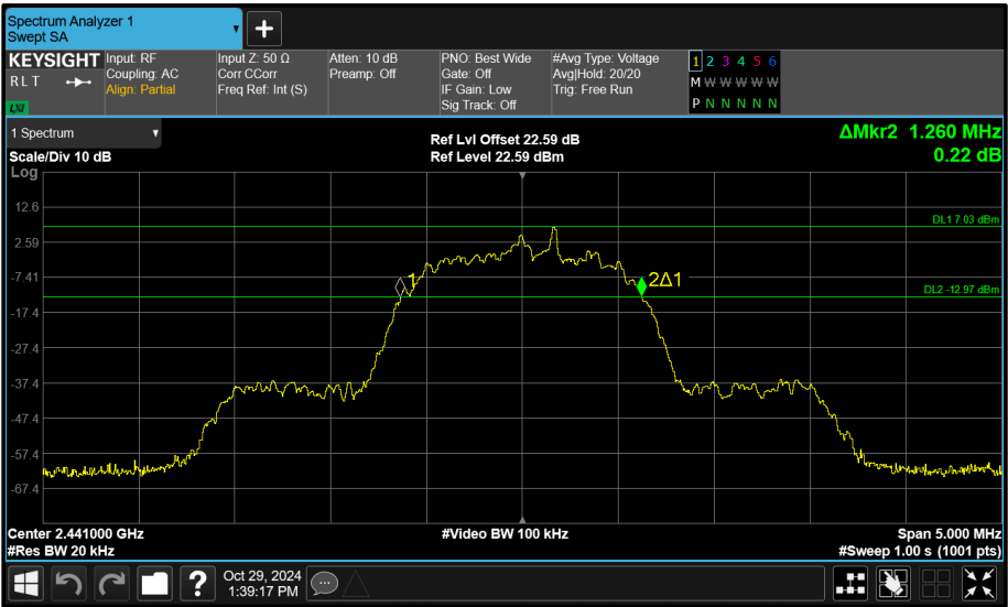
Figure 151 - Core 1 (B) 2441 MHz (CH39) 20 dB Bandwidth
