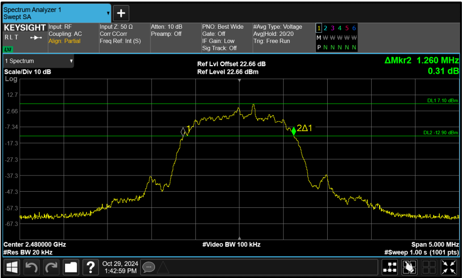
Figure 153 - Core 1 (B) 2480 MHz (CH78) 20 dB Bandwidth
