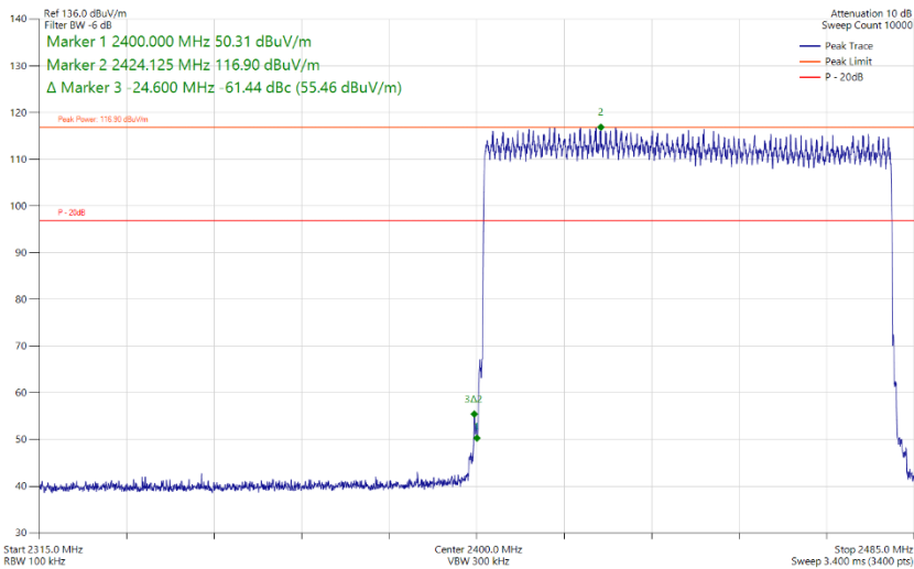
Figure 207 - Bluetooth 3-DH5, MIMO, Core 0 - Core 1 - Hopping Band Edge Frequency 2400 MHz
