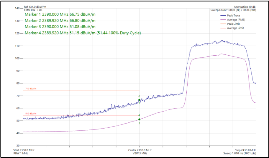
Figure 13 - 802.11ax HE20, SU, SISO, Core 0 - 2417 MHz Band Edge Frequency 2390 MHz
