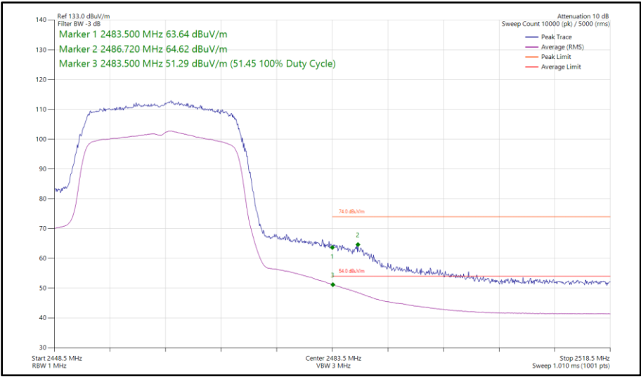
Figure 33 - 802.11ax HE20, SU, SISO, Core 0 - 2462 MHz Band Edge Frequency 2483.5 MHz
