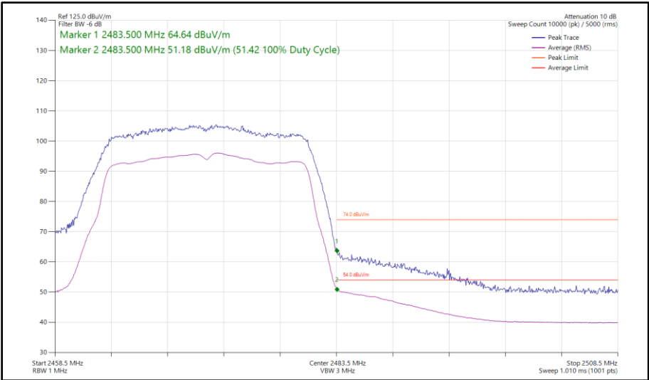
Figure 29 - 802.11n HT20, SISO, Core 0 - 2472 MHz Band Edge Frequency 2483.5 MHz
