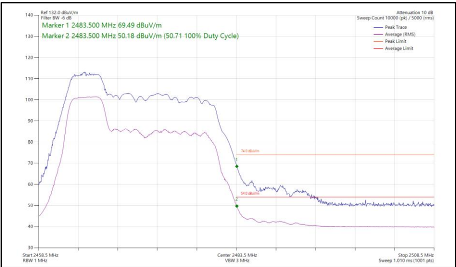
Figure 38 - 802.11ax HE20, RU 52-37, SISO, Core 0 - 2472 MHz Band Edge Frequency 2483.5 MHz
