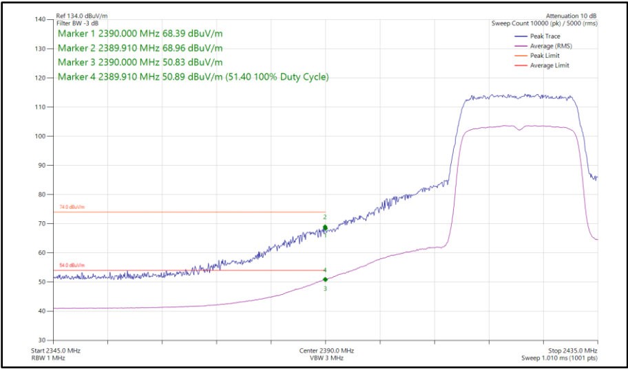
Figure 53 - 802.11ax HE20, SU, SISO, Core 1 - 2422 MHz Band Edge Frequency 2390 MHz
