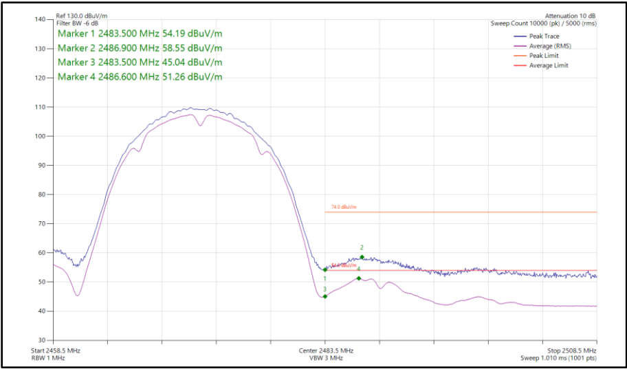
Figure 57 - 802.11b, SISO, Core 1 - 2472 MHz Band Edge Frequency 2483.5 MHz
