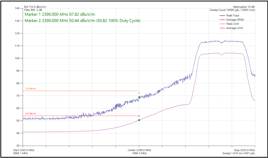
Figure 47 - 802.11n HT20, SISO, Core 1 - 2422 MHz Band Edge Frequency 2390 MHz
