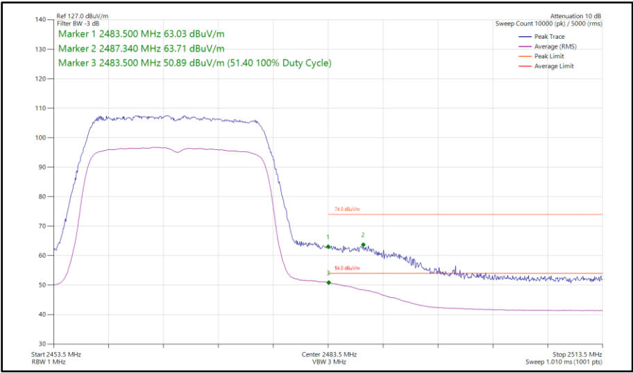
Figure 35 - 802.11ax HE20, SU, SISO, Core 0 - 2467 MHz Band Edge Frequency 2483.5 MHz
