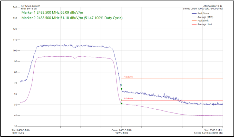
Figure 37 - 802.11ax HE20, SU, SISO, Core 0 - 2472 MHz Band Edge Frequency 2483.5 MHz
