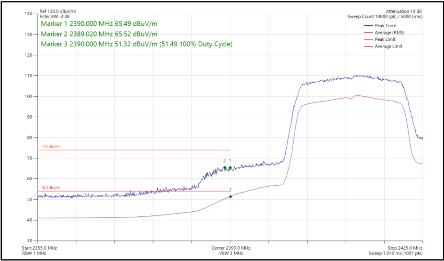
Figure 11 - 802.11ax HE20, SU, SISO, Core 0 - 2412 MHz Band Edge Frequency 2390 MHz
