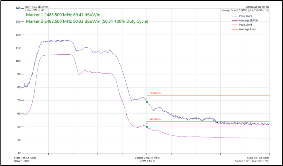
Figure 36 - 802.11ax HE20, RU 106-53, SISO, Core 0 - 2467 MHz Band Edge Frequency 2483.5 MHz
