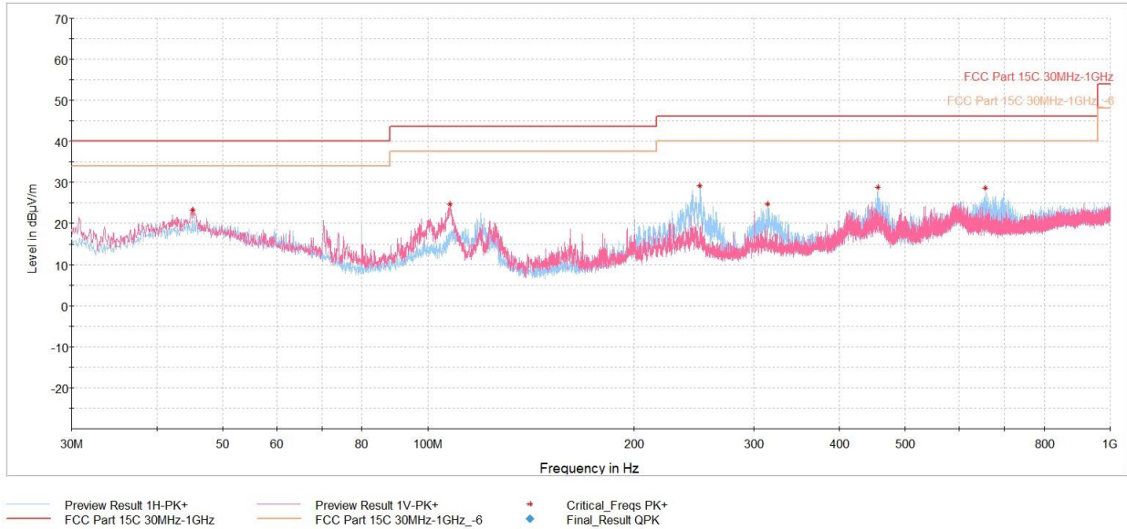
Plot 7-31. Radiated Spurious Emissions Below 1GHz (1Mbps – Ch19, Pol. H & V, with Laptop)
