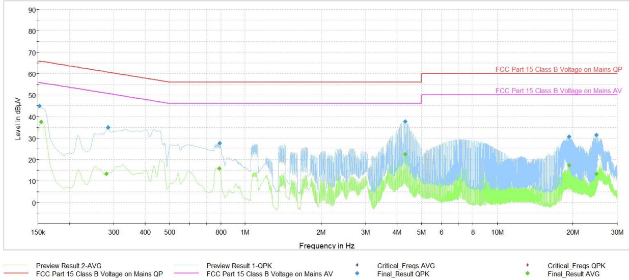
Plot 7-33. AC Line Conducted Plot with Bluetooth LE (N, 1Mbps – Ch.19, with Laptop)
