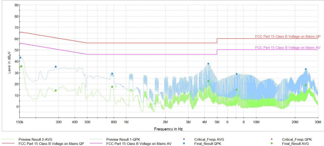
Plot 7-32. AC Line Conducted Plot with Bluetooth LE (L1, 1Mbps – Ch.19 with Laptop)
