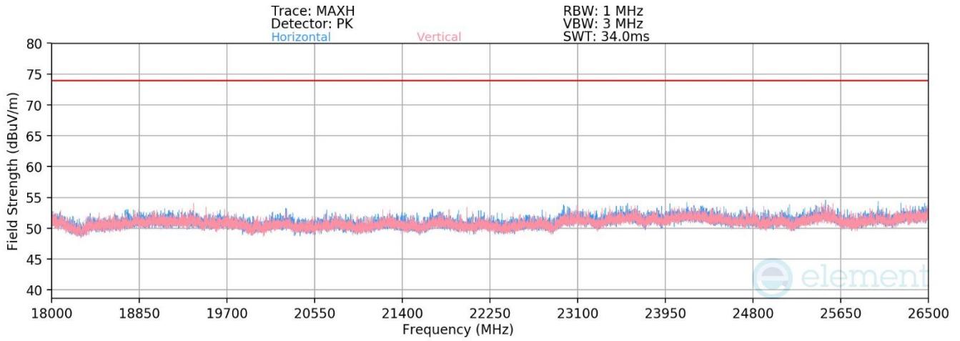
Plot 7-26. Radiated Spurious Emissions Above 18GHz (1Mbps – Ch. 19)
