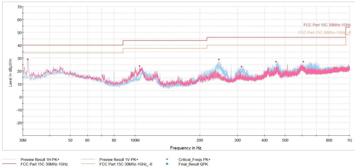
Plot 7-37. Radiated Spurious Emissions Below 1GHz (GFSK – Ch.78, with Laptop)
