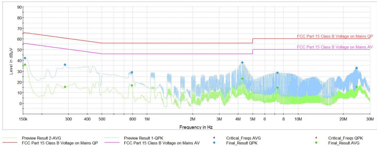
Plot 7-38. AC Line-Conducted Test Plot (L1, GFSK – Ch.78, with Laptop)
