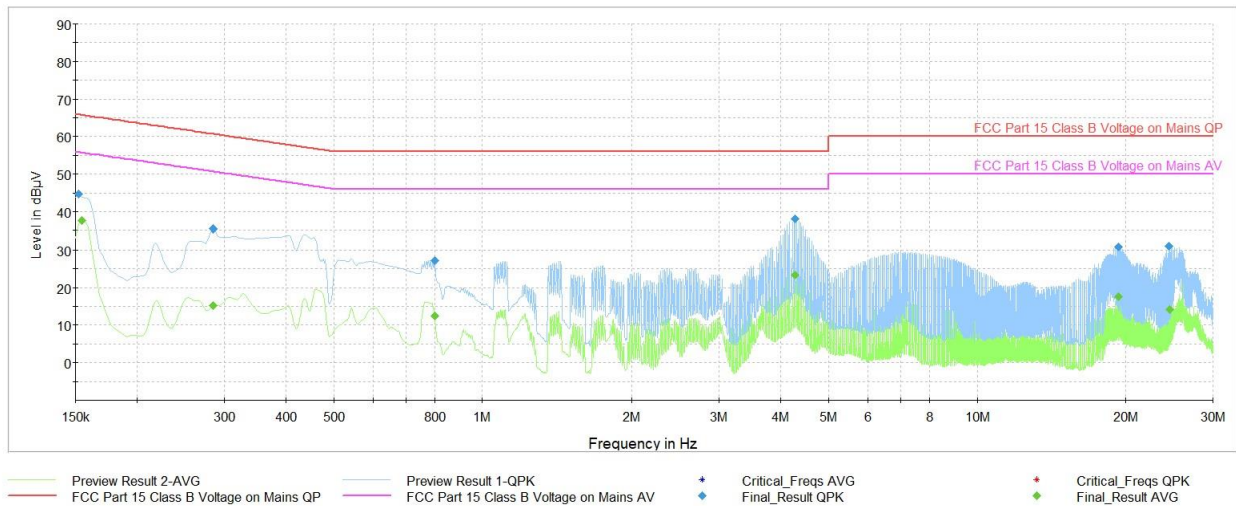
Plot 7-39. AC Line-Conducted Test Plot (N, GFSK – Ch.78, with Laptop)
