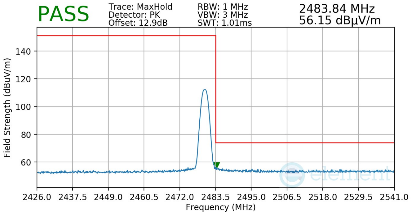
Plot 7-35. Radiated Restricted Upper Band Edge Measurement
