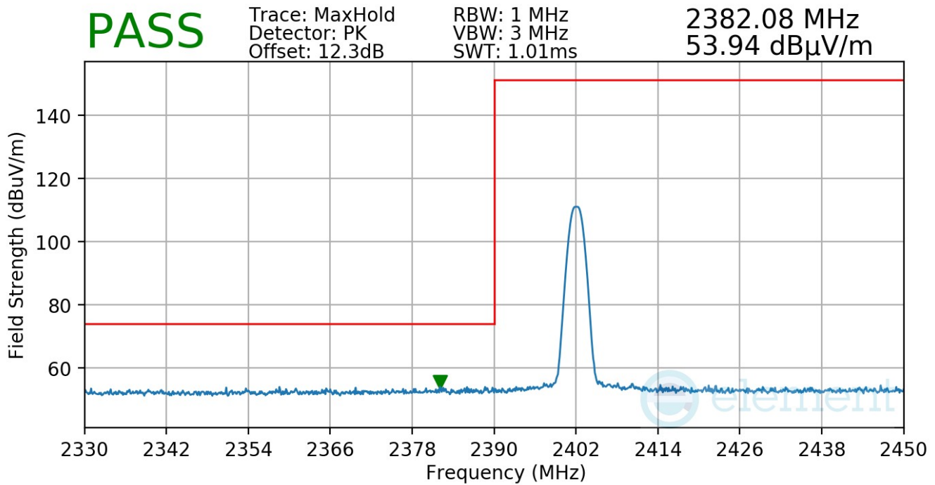
Plot 7-33. Radiated Restricted Lower Band Edge Measurement
