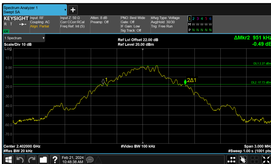
Figure 16 - Core 0 (A) 2402 MHz (CH0) 20 dB Bandwidth
