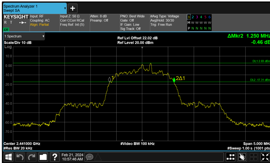
Figure 29 - Core 0 (A) 2441 MHz (CH39) 20 dB Bandwidth
