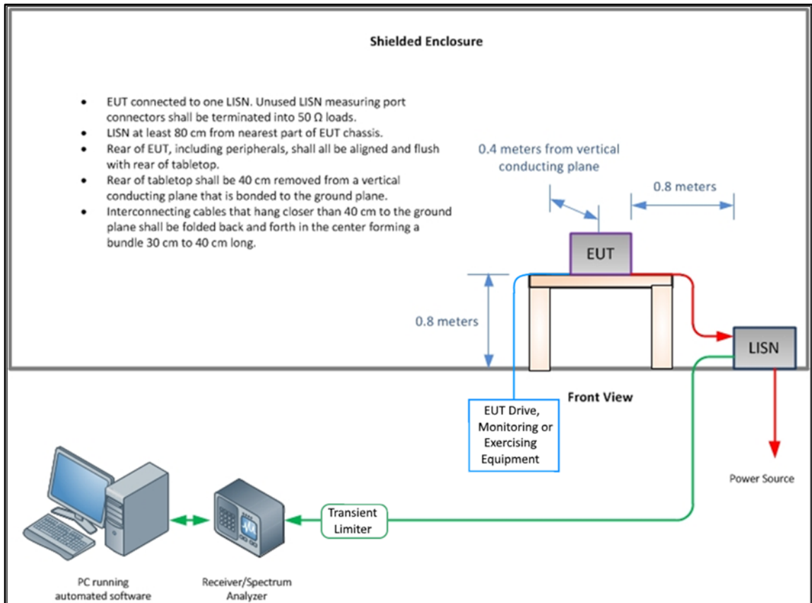
Figure 1 - Conducted Disturbance
