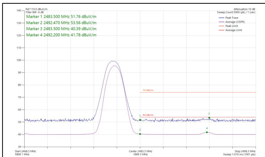
Figure 5 - Bluetooth 2-DH5, SISO, Core 0 - 2480 MHz Band Edge Frequency 2483.5 MHz
