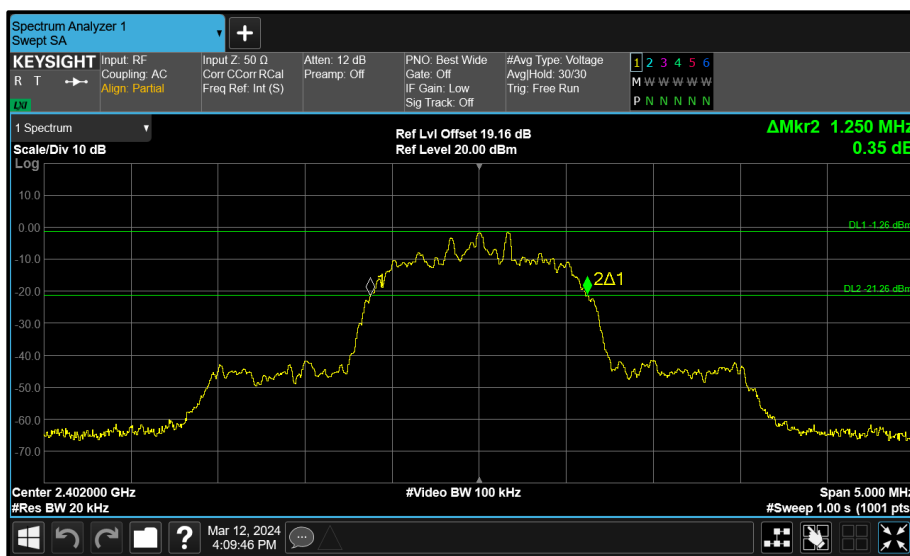
Figure 22 - Core 0 (A) 2402 MHz (CH0) 20 dB Bandwidth
