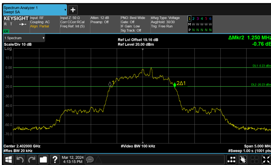
Figure 28 - Core 0 (A) 2402 MHz (CH0) 20 dB Bandwidth
