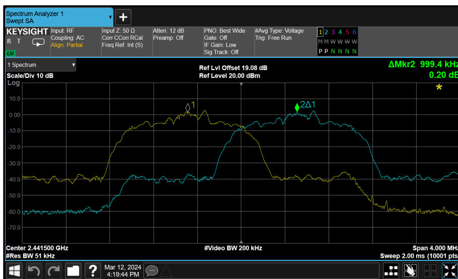
Figure 12 - 8-DPSK - 2441 MHz (CH39)
