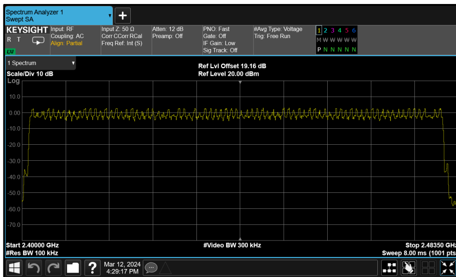
Figure 15 - 8-DPSK (3-DH5) - Number of Hopping Channels
