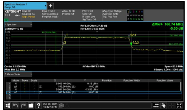
Figure 52 - 802.11ax HE160 SU SP Maximum 99% OBW
