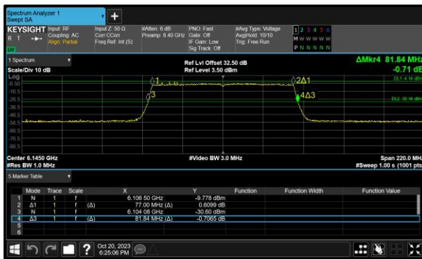
Figure 53 - 802.11ax HE80 SU Minimum 99% OBW
