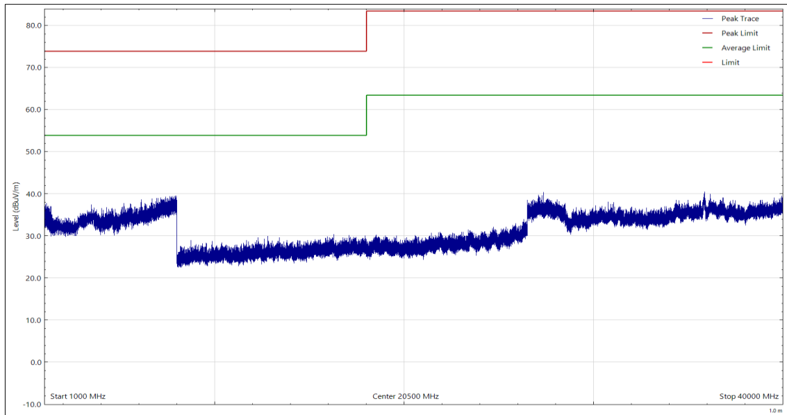
Figure 7 - 1 GHz to 40 GHz, Peak & Average, Vertical
