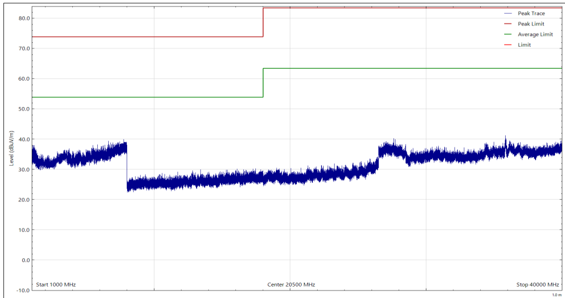
Figure 8 - 1 GHz to 40 GHz, Peak & Average, Horizontal
