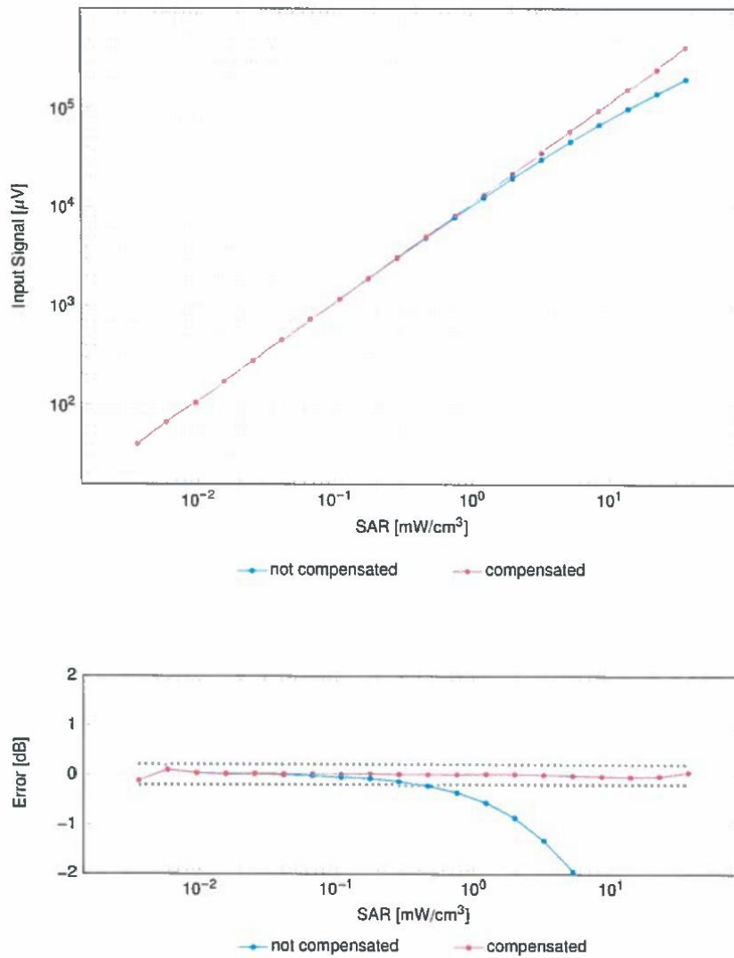
Dynamic Range f(SAR_{head}) (TEM cell, f_{eval} = 1900\text{MHz} )
