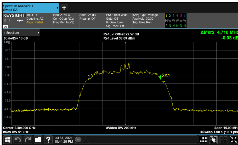
Figure 125 - Core 0 (A) 2404 MHz (CH2) 99% Bandwidth
