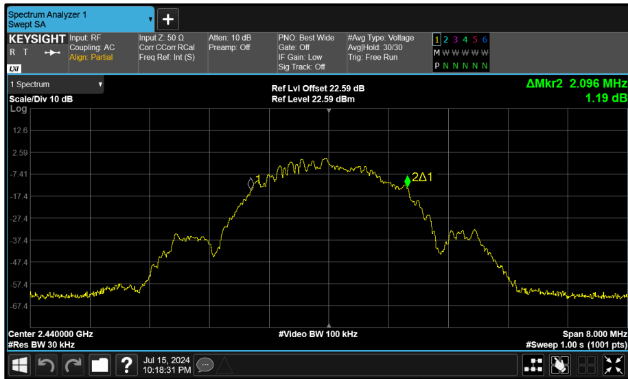
Figure 109 - Core 0 (A) 2440 MHz (CH17) 99% Bandwidth
