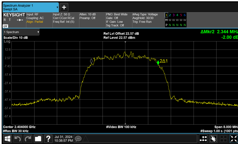
Figure 119 - Core 0 (A) 2404 MHz (CH2) 99% Bandwidth
