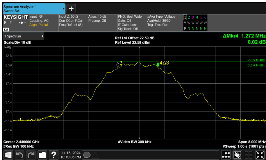
Figure 110 - Core 0 (A) 2440 MHz (CH17) 6 dB Bandwidth
