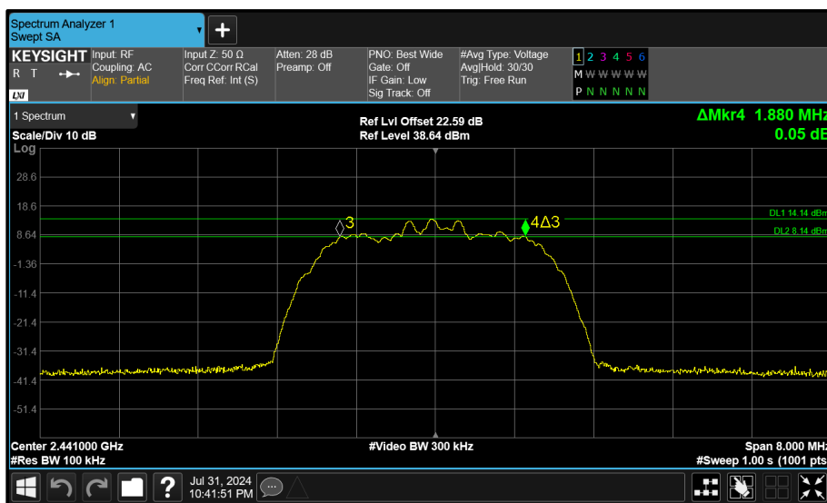
Figure 122 - Core 0 (A) 2441 MHz (CH39) 6 dB Bandwidth
