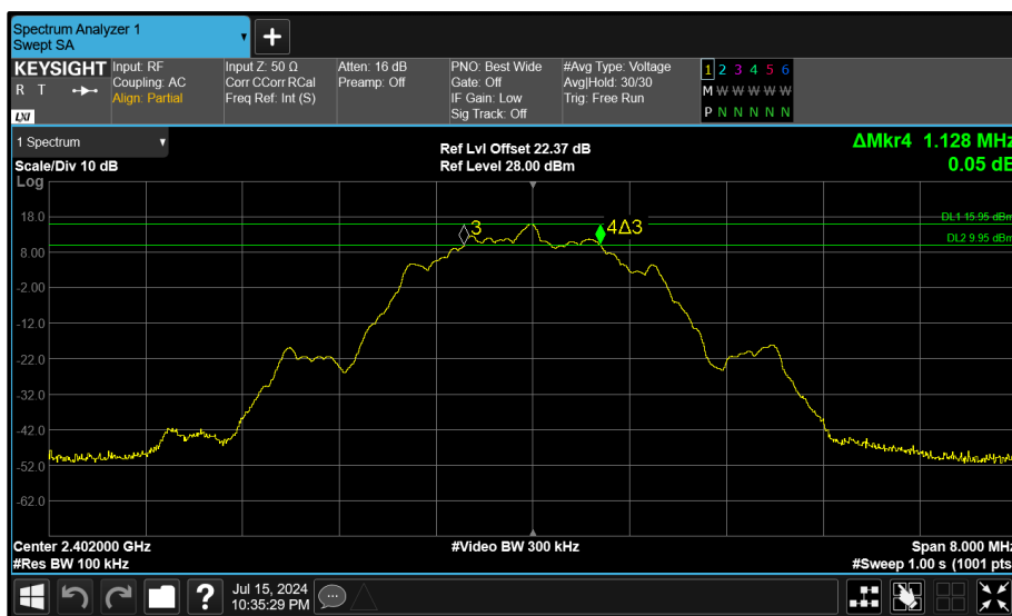
Figure 138 - Core 1 (B) 2402 MHz (CH37) 6 dB Bandwidth
