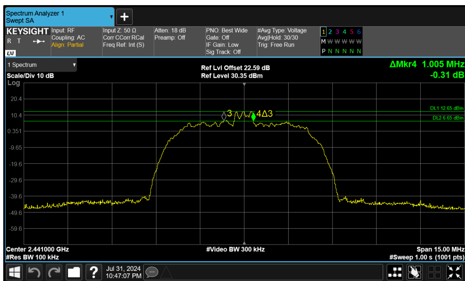
Figure 128 - Core 0 (A) 2441 MHz (CH39) 6 dB Bandwidth
