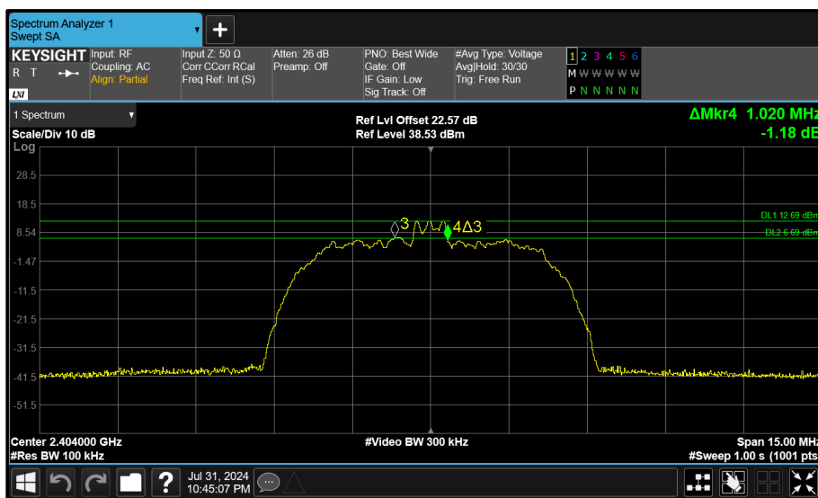
Figure 126 - Core 0 (A) 2404 MHz (CH2) 6 dB Bandwidth
