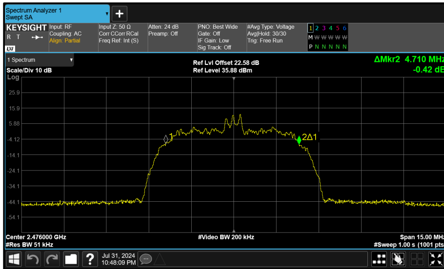
Figure 129 - Core 0 (A) 2476 MHz (CH74) 99% Bandwidth
