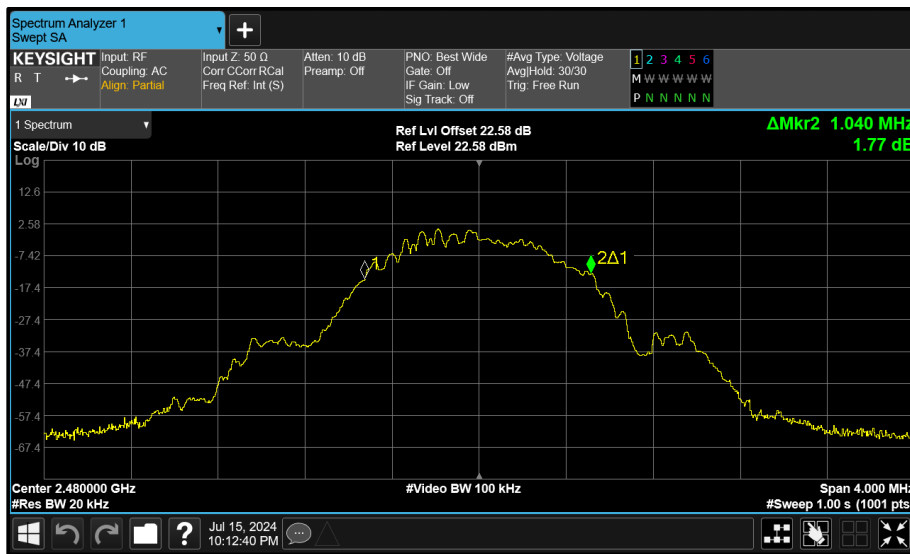
Figure 99 - Core 0 (A) 2480 MHz (CH39) 99% Bandwidth
