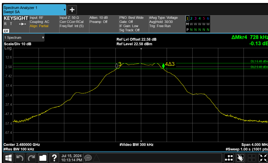
Figure 100 - Core 0 (A) 2480 MHz (CH39) 6 dB Bandwidth
