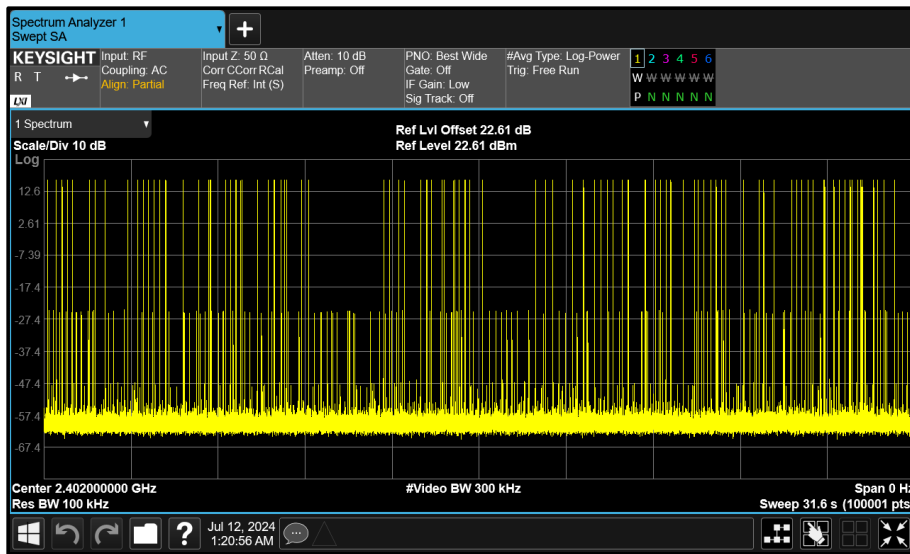
Figure 44 - 8-DPSK - 2402 MHz Accumulated Transmit Time
