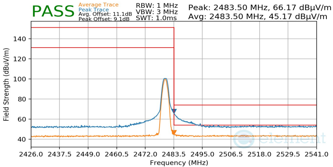
Plot 7-29. Radiated Restricted Upper Band Edge Measurement (Average & Peak)
