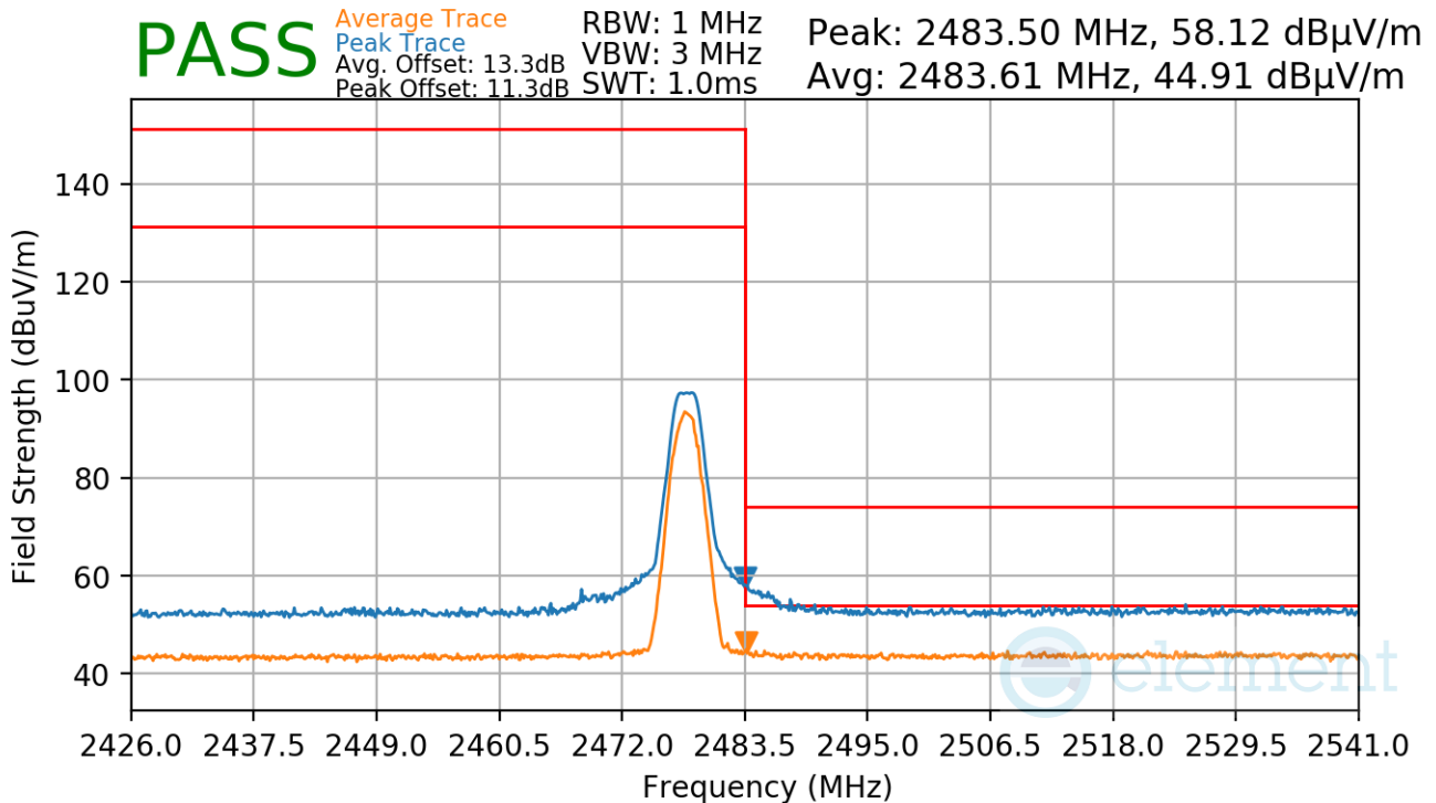
Plot 7-31. Radiated Restricted Upper Band Edge Measurement (Average & Peak)
