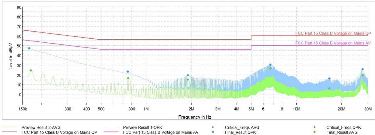
Plot 7-34. AC Line Conducted Plot with Bluetooth LE (N, 1Mbps – Ch.0, with Laptop)
