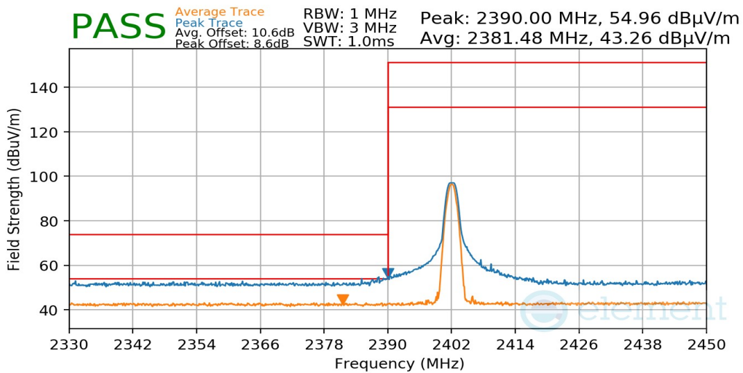
Plot 7-28. Radiated Restricted Lower Band Edge Measurement (Average & Peak)
