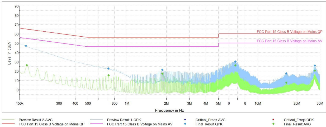
Plot 7-33. AC Line Conducted Plot with Bluetooth LE (L1, 1Mbps – Ch.0 with Laptop)
