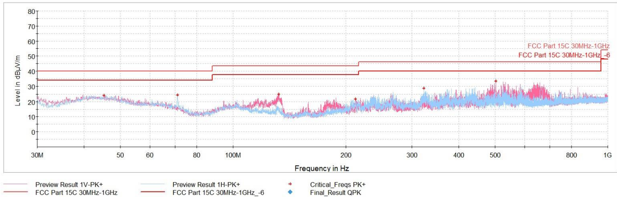
Plot 7-32. Radiated Spurious Emissions Below 1GHz (1Mbps – Ch.0, Pol. H & V, with AC/DC Adapter and Laptop)
