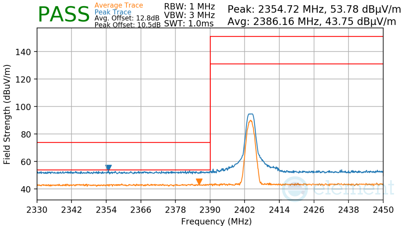
Plot 7-30. Radiated Restricted Lower Band Edge Measurement (Average & Peak)
