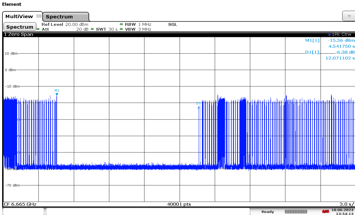
Plot 7-1881. LPI Contention Based Protocol Timing Plot – UNII 7 – 160MHz Channel 143 – Low
