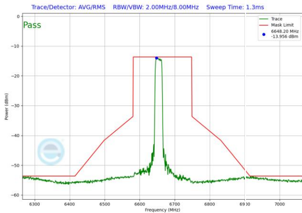
Plot 7-1827. VLP In-Band Emission Plot SDM Antenna 3b (160MHz 802.11ax RU242 (UNII Band 7) – Ch. 143)
