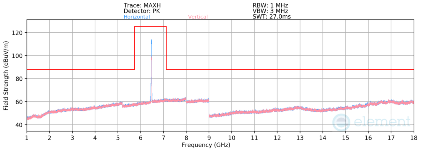
Plot 7-1916. Radiated Spurious Emissions above 1GHz Antenna 5T (802.11ax – Ch. 105 – RU242)
