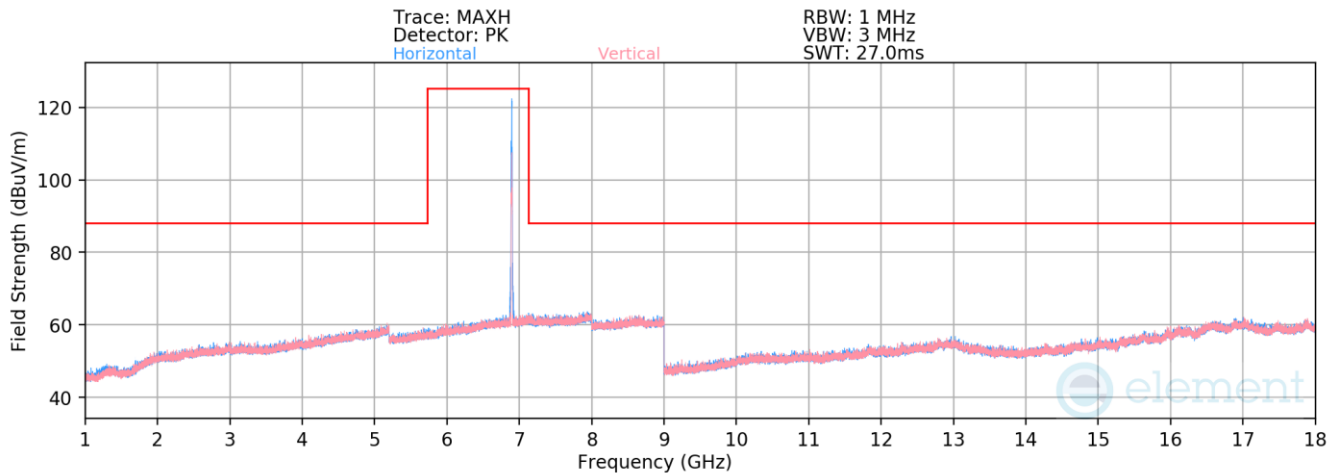
Plot 7-1909. Radiated Spurious Emissions above 1GHz Antenna 5T (802.11ax – Ch. 189 – RU26)
