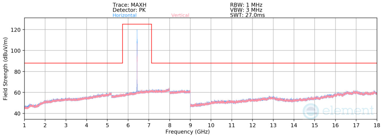
Plot 7-1903. Radiated Spurious Emissions above 1GHz Antenna 5T (802.11ax – Ch. 97 – RU26)
