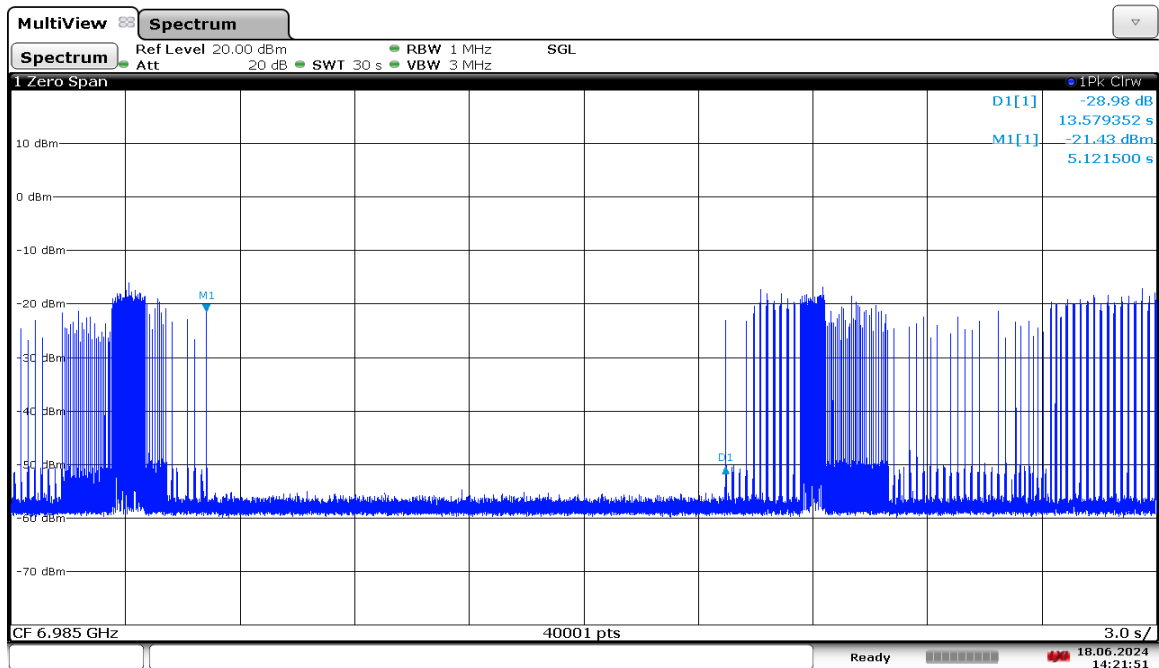
Plot 7-1887. LPI Contention Based Protocol Timing Plot – UNII 8 – 160MHz Channel 207 – High
