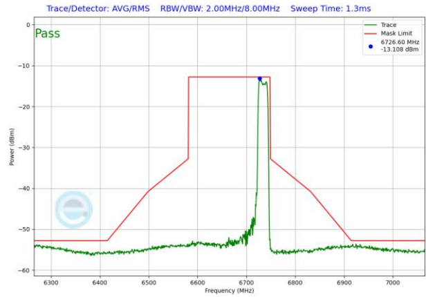
Plot 7-1829. VLP In-Band Emission Plot SDM Antenna 3b (160MHz 802.11ax RU242 (UNII Band 7) – Ch. 143)
