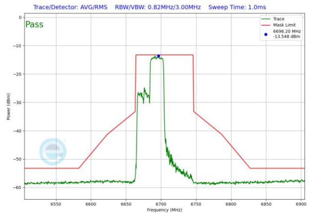
Plot 7-1818. VLP In-Band Emission Plot SDM Antenna WF5T (80MHz 802.11ax RU242 (UNII Band 7) – Ch. 151)
