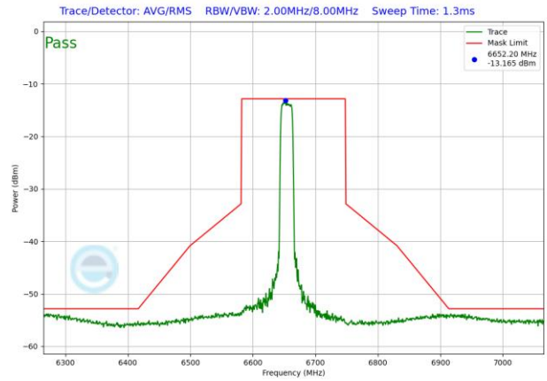
Plot 7-1853. VLP In-Band Emission Plot SDM Diversity Antenna 1b (160MHz 802.11ax RU242 (UNII Band 7) – Ch. 143)
