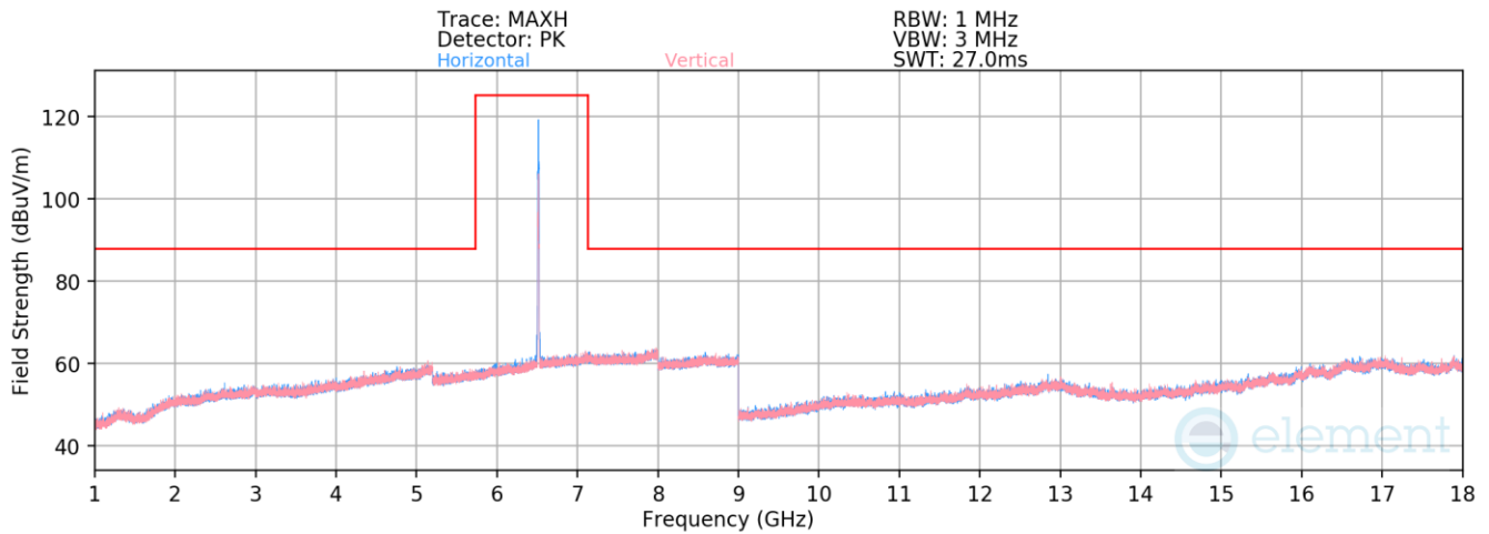
Plot 7-1905. Radiated Spurious Emissions above 1GHz Antenna 5T (802.11ax – Ch. 113 – RU26)
