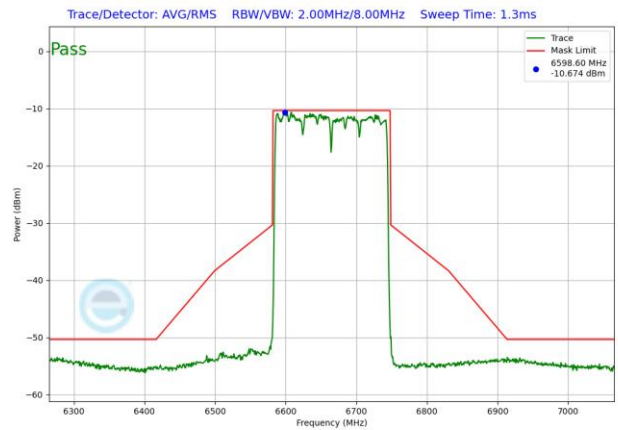
Plot 7-1855. VLP In-Band Emission Plot SDM Diversity Antenna 1b (160MHz 802.11ax RU996x2 (UNII Band 7) – Ch. 143)
