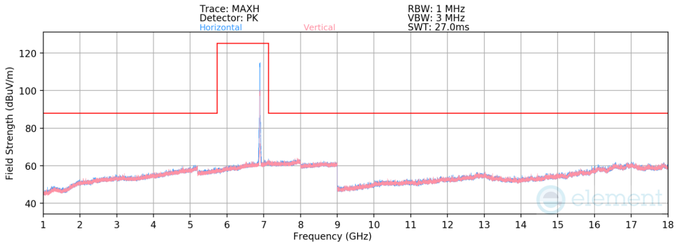
Plot 7-1921. Radiated Spurious Emissions above 1GHz Antenna 5T (802.11ax – Ch. 189 – RU242)
