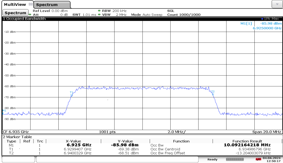
Plot 7-1868. AWGN Signal – UNII 8 – 20MHz
