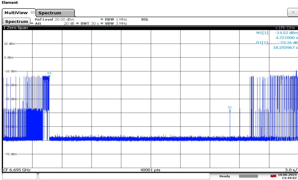
Plot 7-1880. LPI Contention Based Protocol Timing Plot – UNII 7 – 20MHz Channel 149
