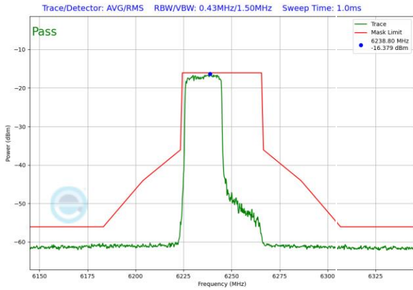
Plot 7-1833. VLP In-Band Emission Plot SDM Diversity Antenna 1b (40MHz 802.11ax RU242 (UNII Band 5) – Ch. 59)
