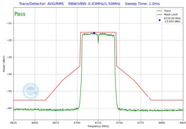
Plot 7-1814. VLP In-Band Emission Plot SDM Antenna WF5T (40MHz 802.11ax RU484 (UNII Band 7) – Ch. 155)
