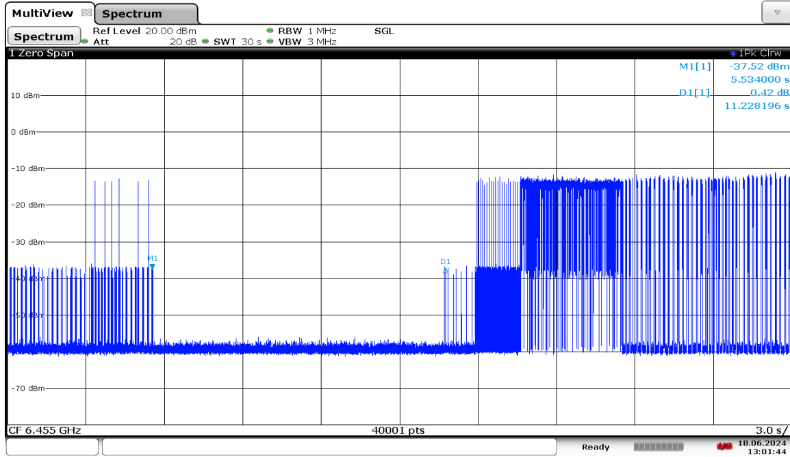
Plot 7-1876. LPI Contention Based Protocol Timing Plot – UNII 6 – 20MHz Channel 101
