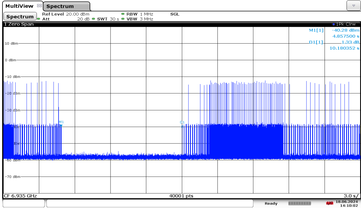
Plot 7-1884. LPI Contention Based Protocol Timing Plot – UNII 8 – 20MHz Channel 197
