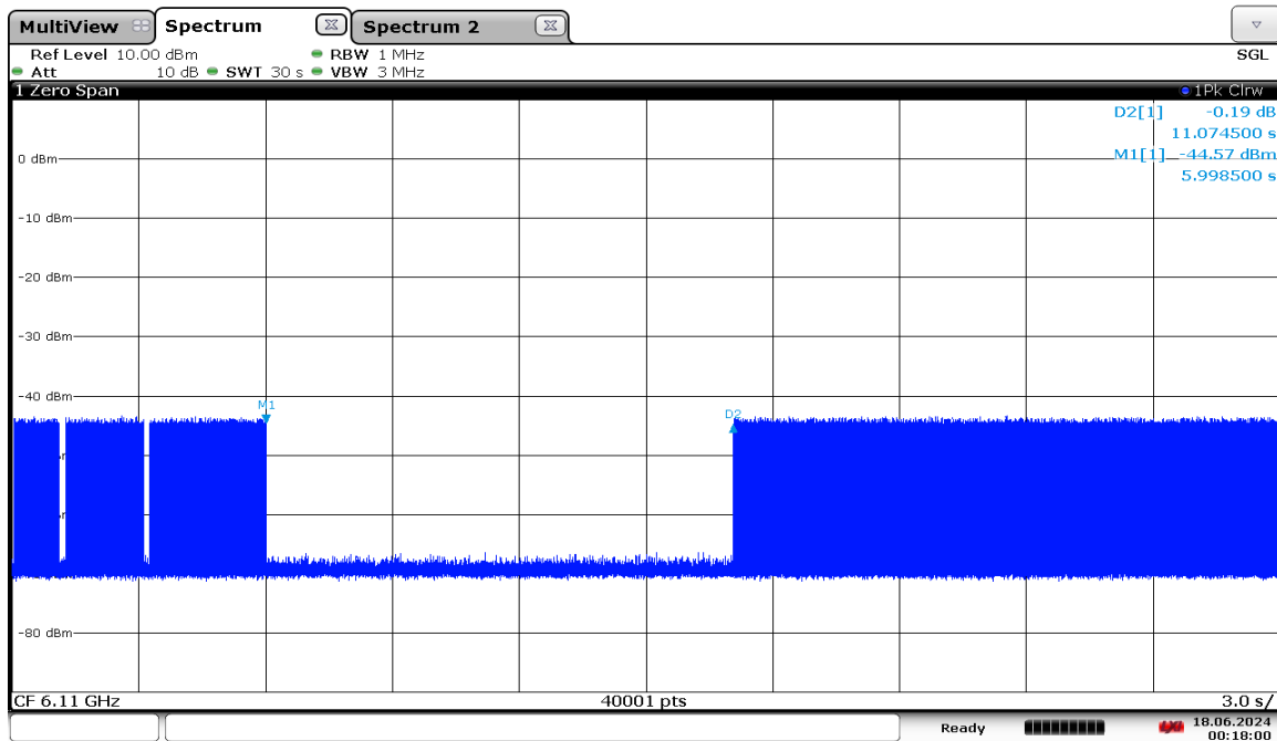
Plot 7-1889. VLP Contention Based Protocol Timing Plot – UNII 5 – 160MHz Channel 47 – Low
