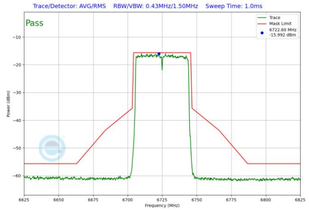
Plot 7-1847. VLP In-Band Emission Plot SDM Diversity Antenna 1b (40MHz 802.11ax RU484 (UNII Band 7) – Ch. 155)
