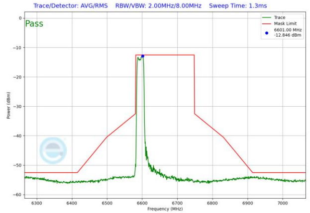
Plot 7-1824. VLP In-Band Emission Plot SDM Antenna WF5T (160MHz 802.11ax RU242 (UNII Band 7) – Ch. 143)
