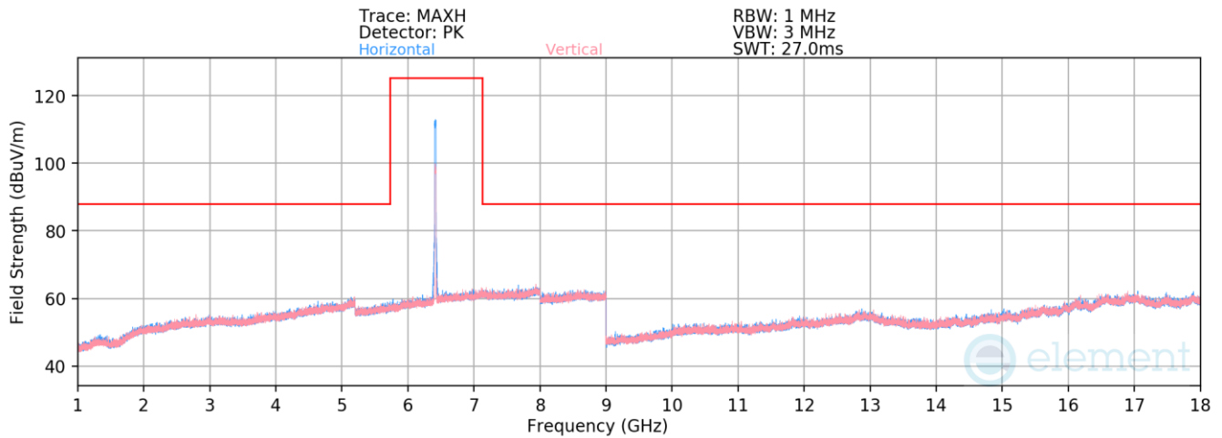
Plot 7-1914. Radiated Spurious Emissions above 1GHz Antenna 5T (802.11ax – Ch. 93 – RU242)
