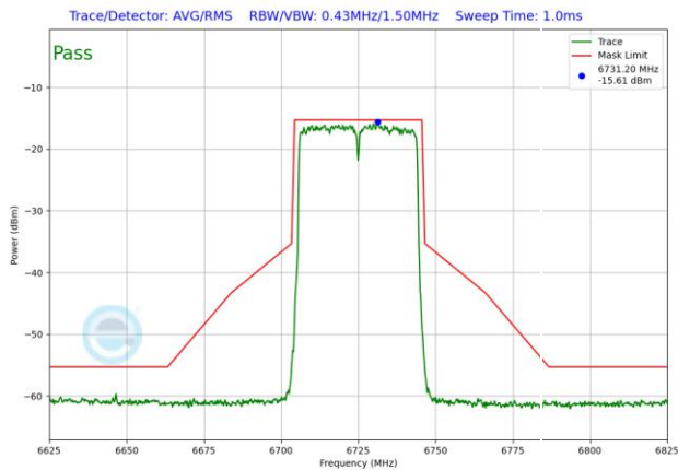
Plot 7-1815. VLP In-Band Emission Plot SDM Antenna 3b (40MHz 802.11ax RU484 (UNII Band 7) – Ch. 155)
