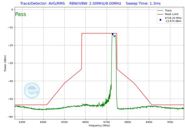
Plot 7-1854. VLP In-Band Emission Plot SDM Diversity Antenna 1b (160MHz 802.11ax RU242 (UNII Band 7) – Ch. 143)
