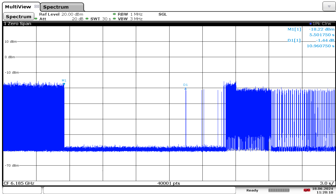
Plot 7-1875. LPI Contention Based Protocol Timing Plot – UNII 5 – 160MHz Channel 47 – High
