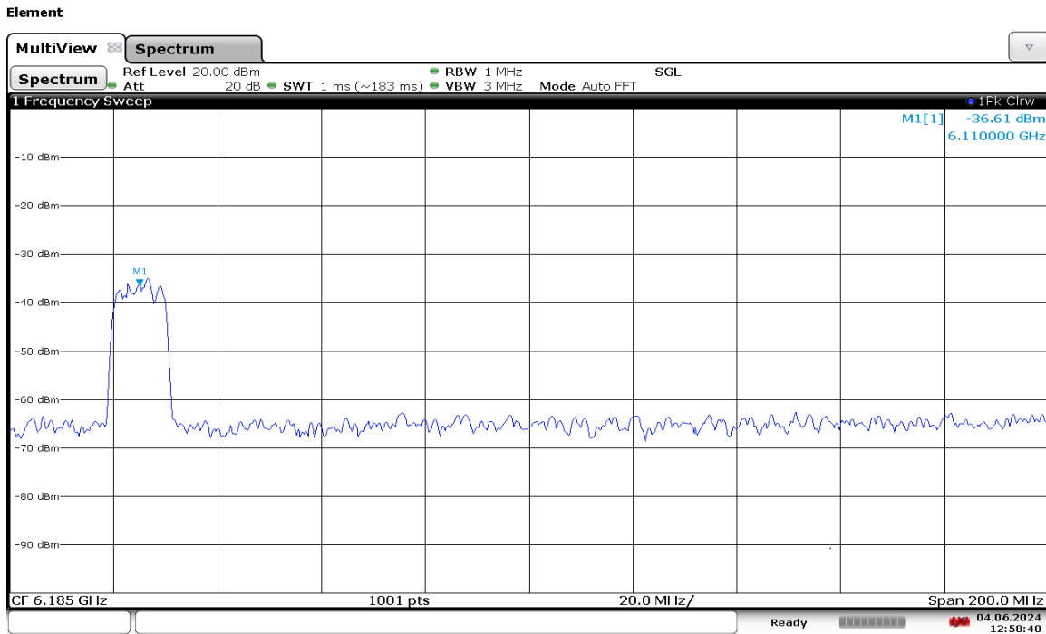
Plot 7-1897. 160MHz Bandwidth – AWGN Signal Injected at Low End – Channel 47
