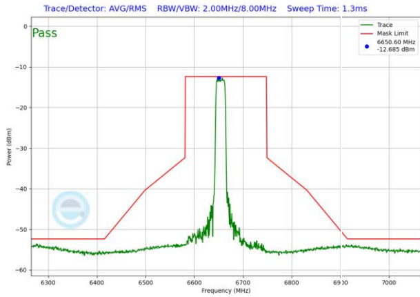
Plot 7-1826. VLP In-Band Emission Plot SDM Antenna WF5T (160MHz 802.11ax RU242 (UNII Band 7) – Ch. 143)
