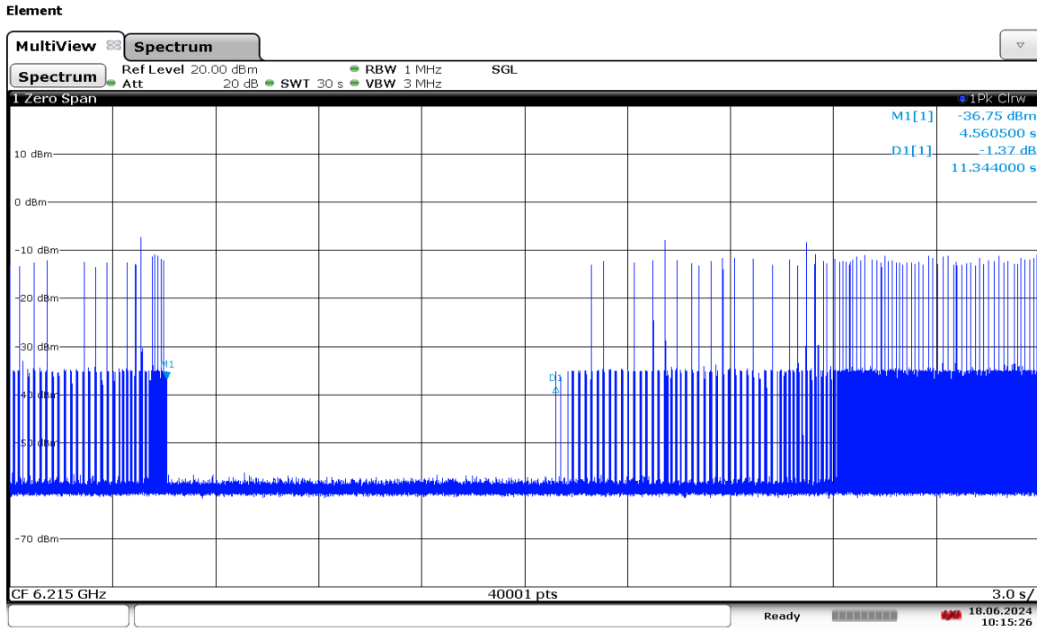
Plot 7-1872. LPI Contention Based Protocol Timing Plot – UNII 5 – 20MHz Channel 53
