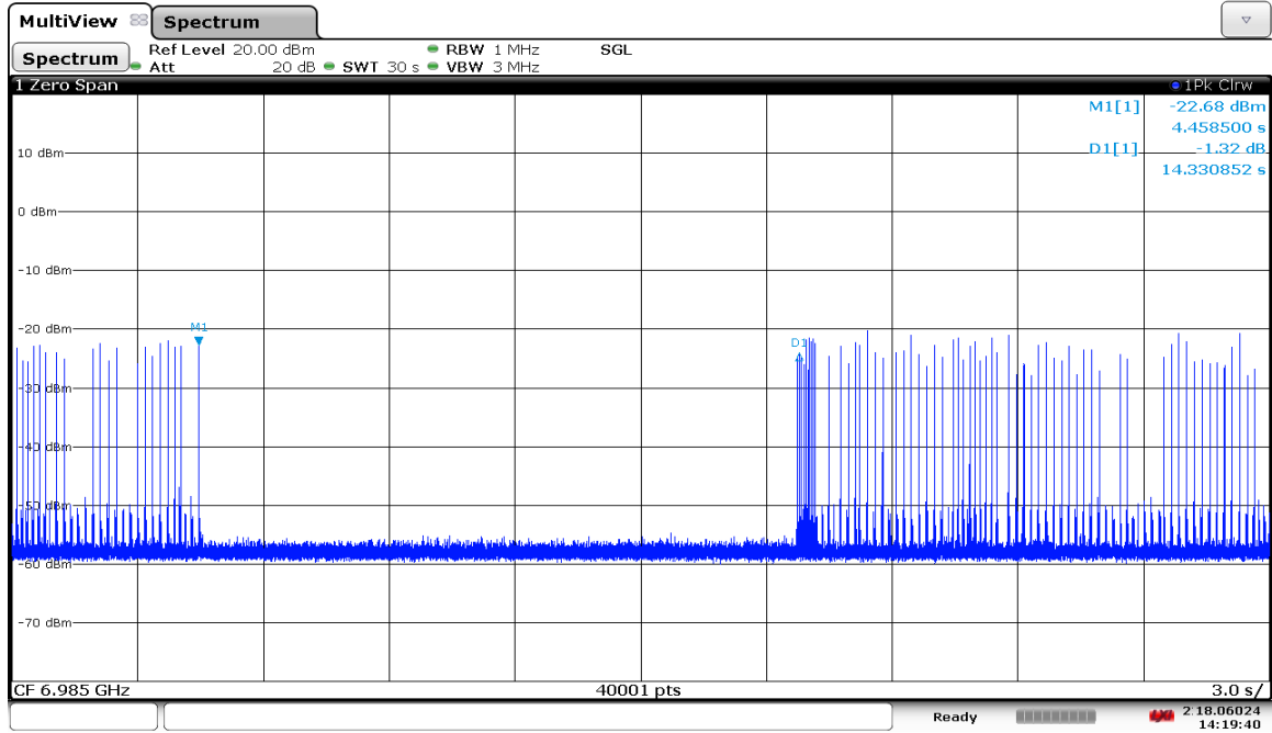
Plot 7-1886. LPI Contention Based Protocol Timing Plot – UNII 8 – 160MHz Channel 207 – Mid
