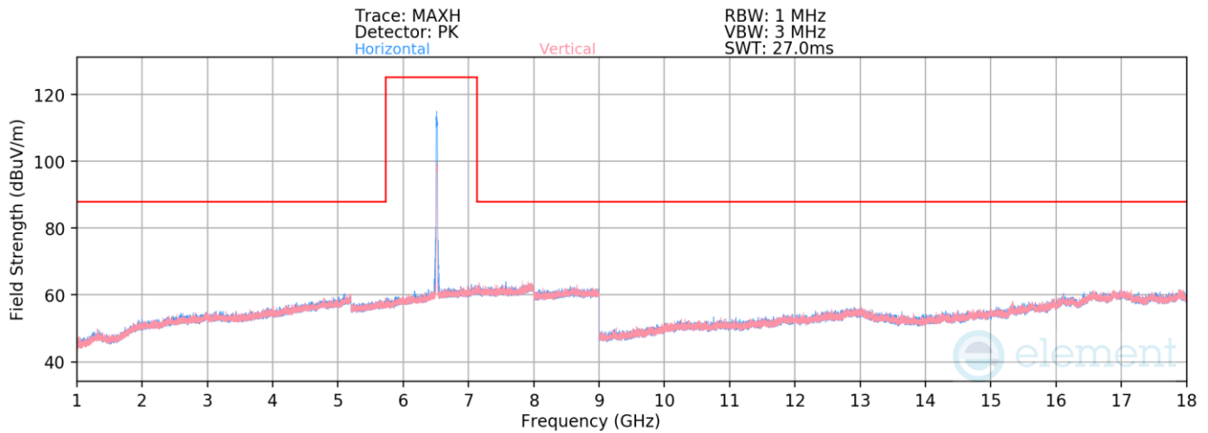
Plot 7-1917. Radiated Spurious Emissions above 1GHz Antenna 5T (802.11ax – Ch. 113 – RU242)
