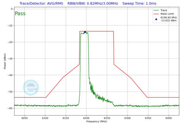
Plot 7-1836. VLP In-Band Emission Plot SDM Diversity Antenna 1b (80MHz 802.11ax RU242 (UNII Band 5) – Ch. 55)
