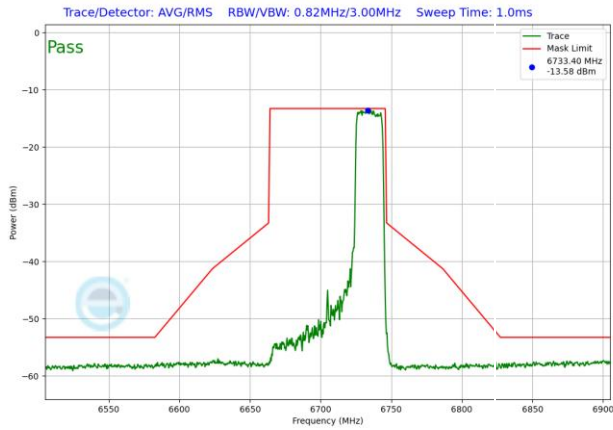
Plot 7-1820. VLP In-Band Emission Plot SDM Antenna WF5T (80MHz 802.11ax RU242 (UNII Band 7) – Ch. 151)
