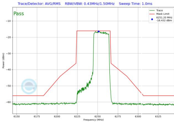
Plot 7-1834. VLP In-Band Emission Plot SDM Diversity Antenna 1b (40MHz 802.11ax RU242 (UNII Band 5) – Ch. 59)
