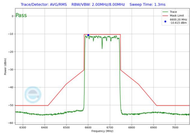
Plot 7-1830. VLP In-Band Emission Plot SDM Antenna WF5T (160MHz 802.11ax RU996x2 (UNII Band 7) – Ch. 143)
