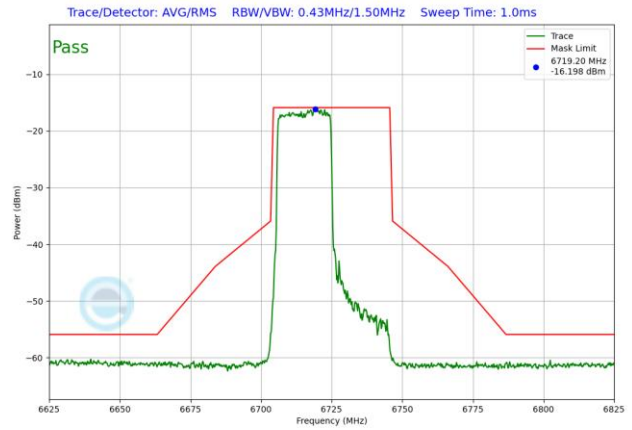
Plot 7-1811. VLP In-Band Emission Plot SDM Antenna 3b (40MHz 802.11ax RU242 (UNII Band 7) – Ch. 155)
