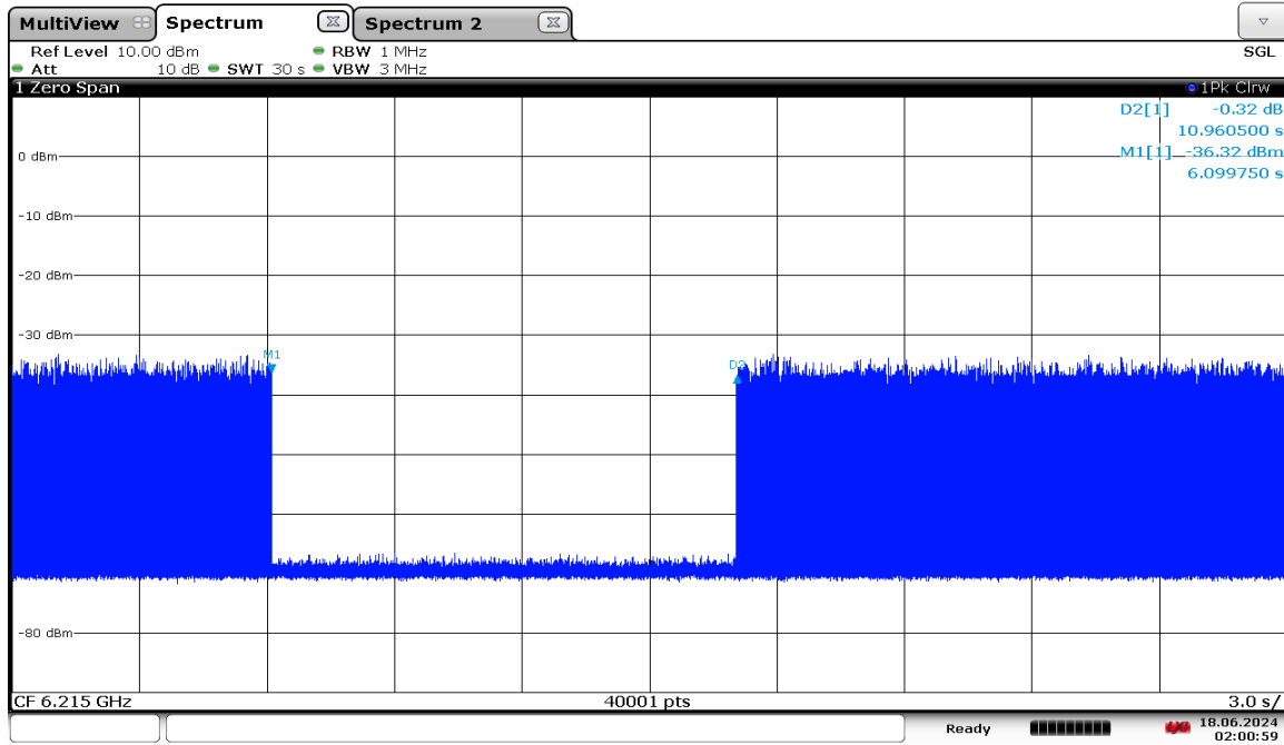
Plot 7-1888. VLP Contention Based Protocol Timing Plot – UNII 5 – 20MHz Channel 53
