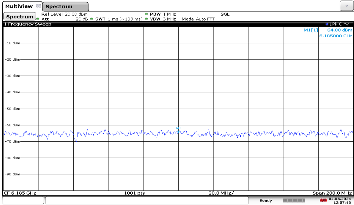
Plot 7-1898. 160MHz Bandwidth – AWGN Signal Injected at Center – Channel 47
