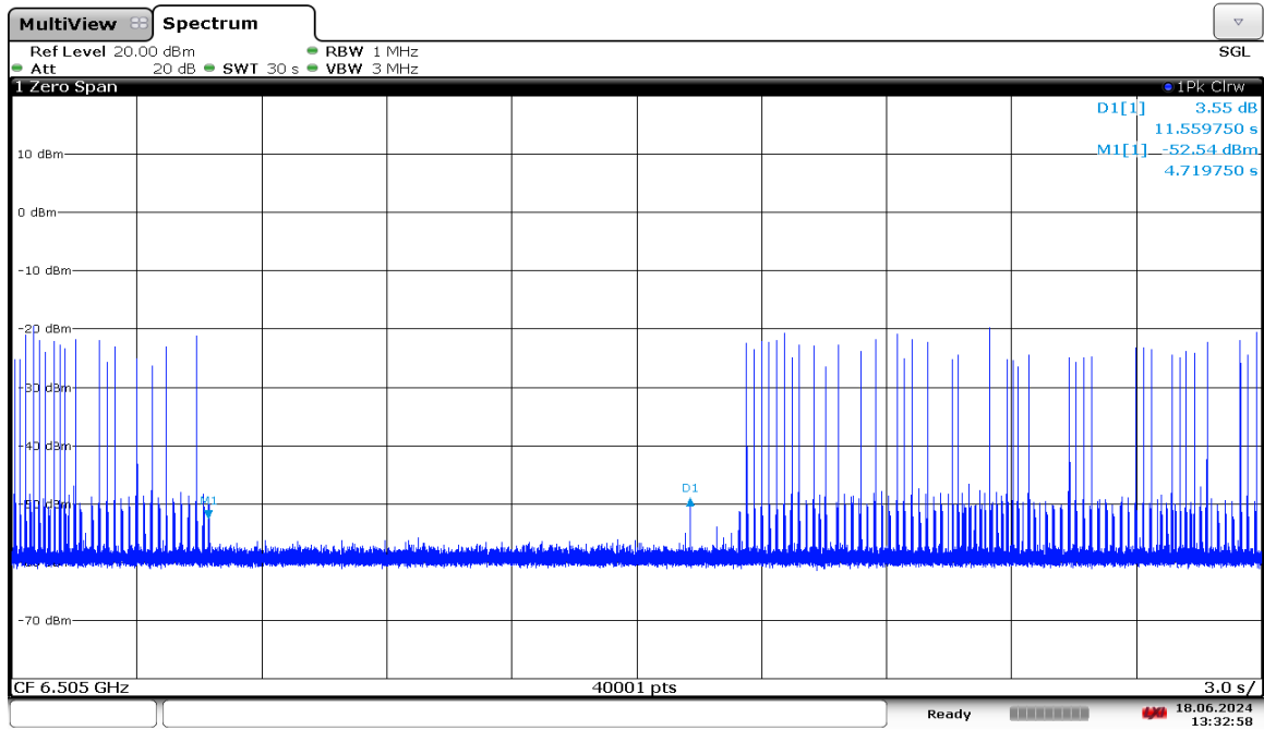
Plot 7-1878. LPI Contention Based Protocol Timing Plot – UNII 6 – 160MHz Channel 111 – Mid
