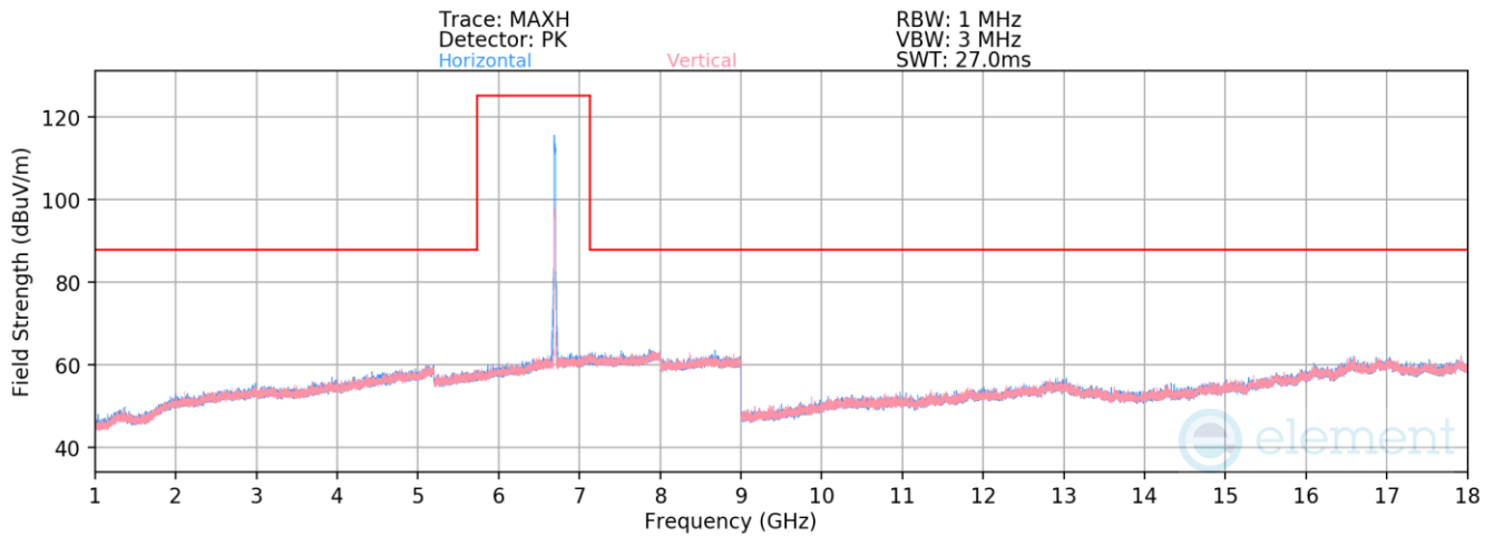
Plot 7-1919. Radiated Spurious Emissions above 1GHz Antenna 5T (802.11ax – Ch. 149 – RU242)
