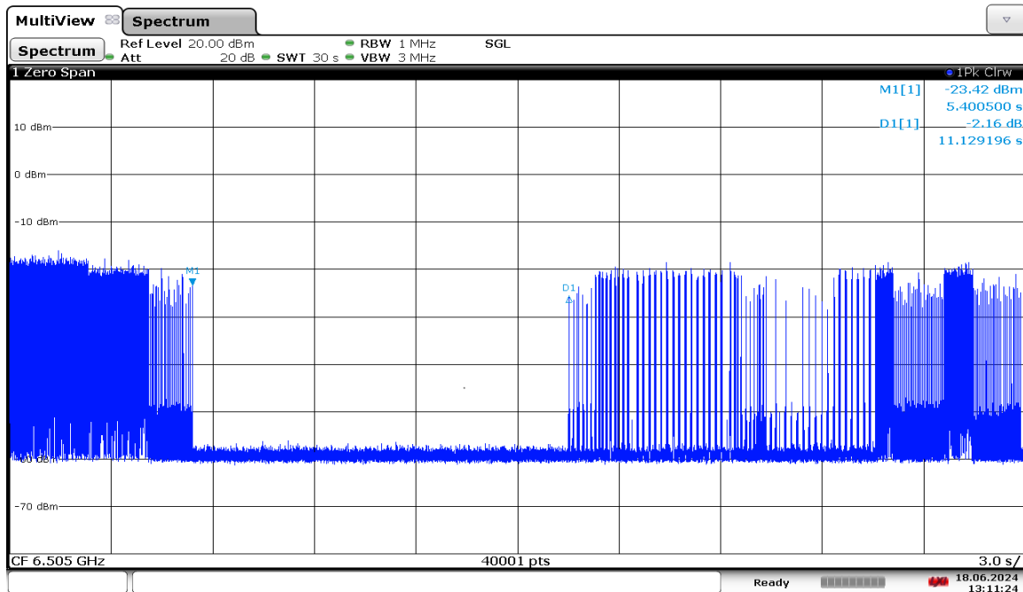
Plot 7-1877. LPI Contention Based Protocol Timing Plot – UNII 6 – 160MHz Channel 111 – Low
