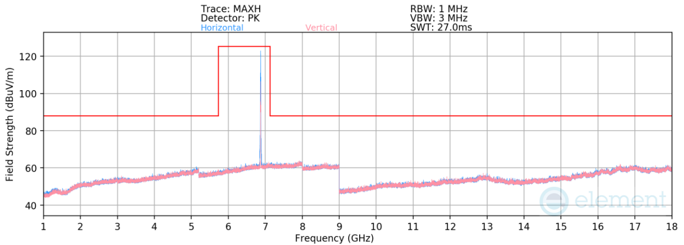
Plot 7-1908. Radiated Spurious Emissions above 1GHz Antenna 5T (802.11ax – Ch. 185 – RU26)
