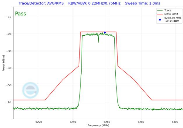
Plot 7-1832. VLP In-Band Emission Plot SDM Diversity Antenna 1b (20MHz 802.11ax RU242 (UNII Band 5) – Ch. 61)
