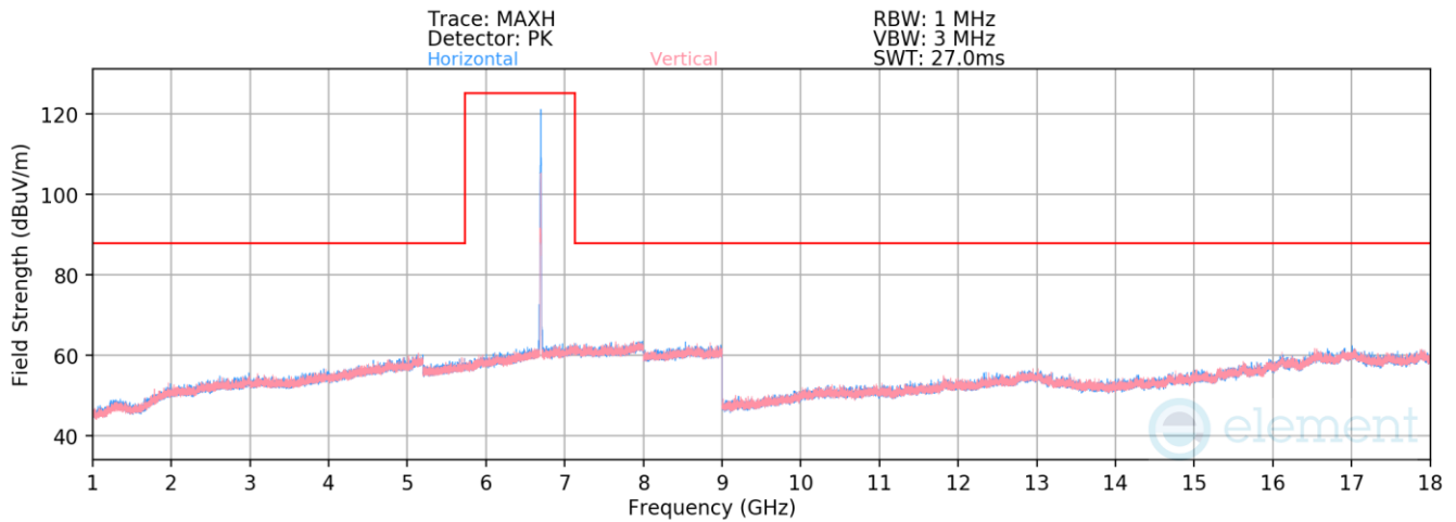
Plot 7-1907. Radiated Spurious Emissions above 1GHz Antenna 5T (802.11ax – Ch. 149 – RU26)
