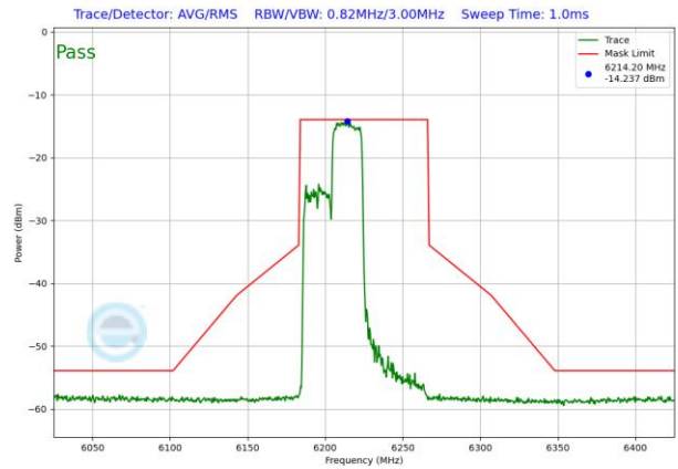
Plot 7-1837. VLP In-Band Emission Plot SDM Diversity Antenna 1b (80MHz 802.11ax RU242 (UNII Band 5) – Ch. 55)
