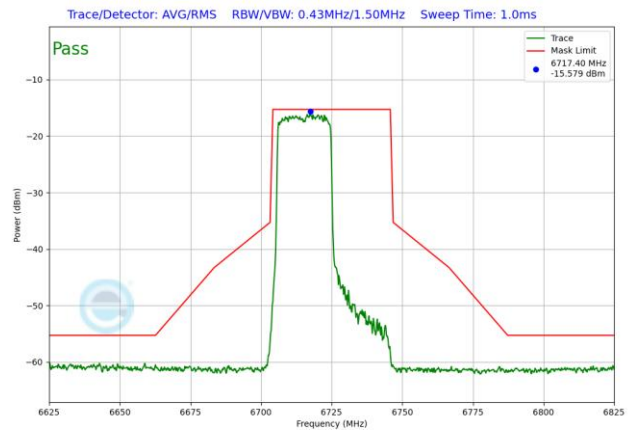
Plot 7-1812. VLP In-Band Emission Plot SDM Antenna WF5T (40MHz 802.11ax RU242 (UNII Band 7) – Ch. 155)
