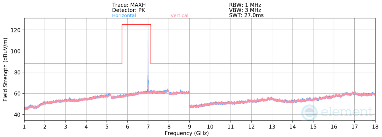
Plot 7-1910. Radiated Spurious Emissions above 1GHz Antenna 5T (802.11ax – Ch. 209 – RU26)
