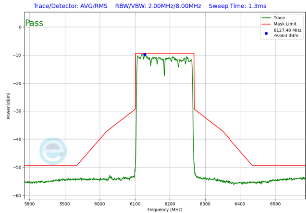
Plot 7-1843. VLP In-Band Emission Plot SDM Diversity Antenna 1b (160MHz 802.11ax RU996x2 (UNII Band 5) – Ch. 47)
