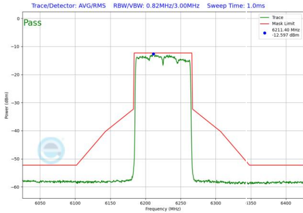
Plot 7-1839. VLP In-Band Emission Plot SDM Diversity Antenna 1b (80MHz 802.11ax RU996 (UNII Band 5) – Ch. 55)
