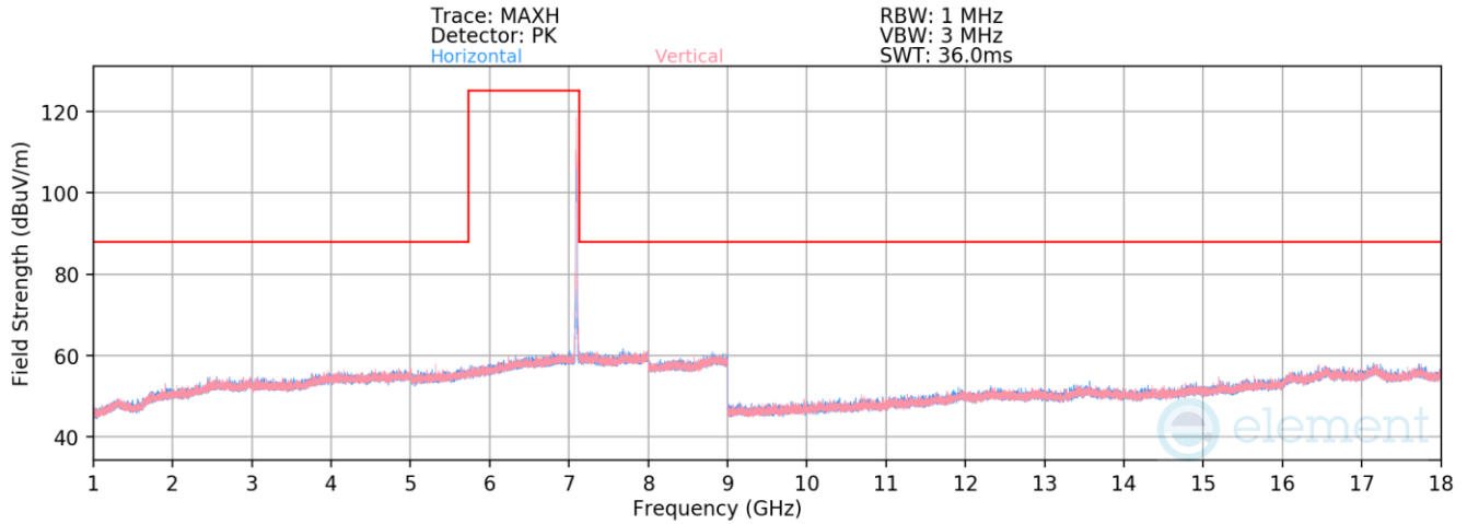
Plot 7-1911. Radiated Spurious Emissions above 1GHz Antenna 5T (802.11ax – Ch. 229 – RU26)
