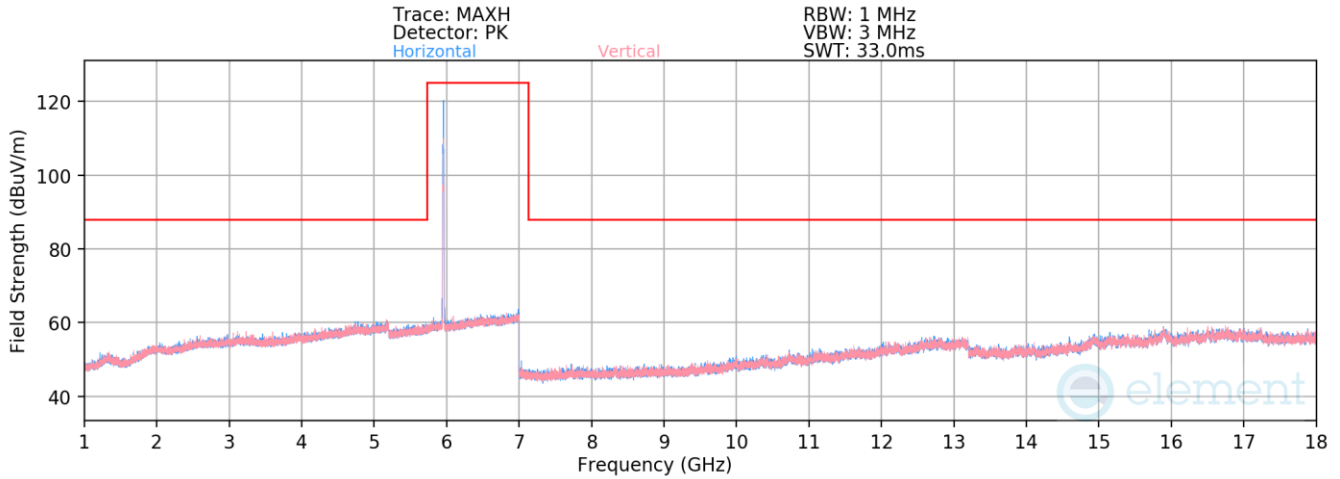
Plot 7-1900. Radiated Spurious Emissions above 1GHz Antenna 5T (802.11ax – Ch. 1 – RU26)
