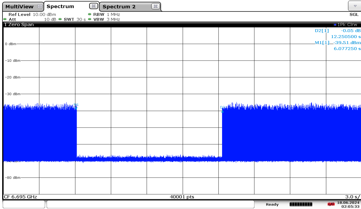
Plot 7-1892. VLP Contention Based Protocol Timing Plot – UNII 7 – 20MHz Channel 149
