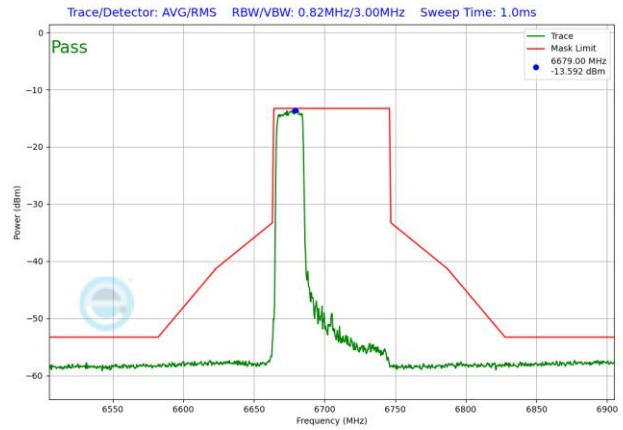
Plot 7-1817. VLP In-Band Emission Plot SDM Antenna 3b (80MHz 802.11ax RU242 (UNII Band 7) – Ch. 151)
