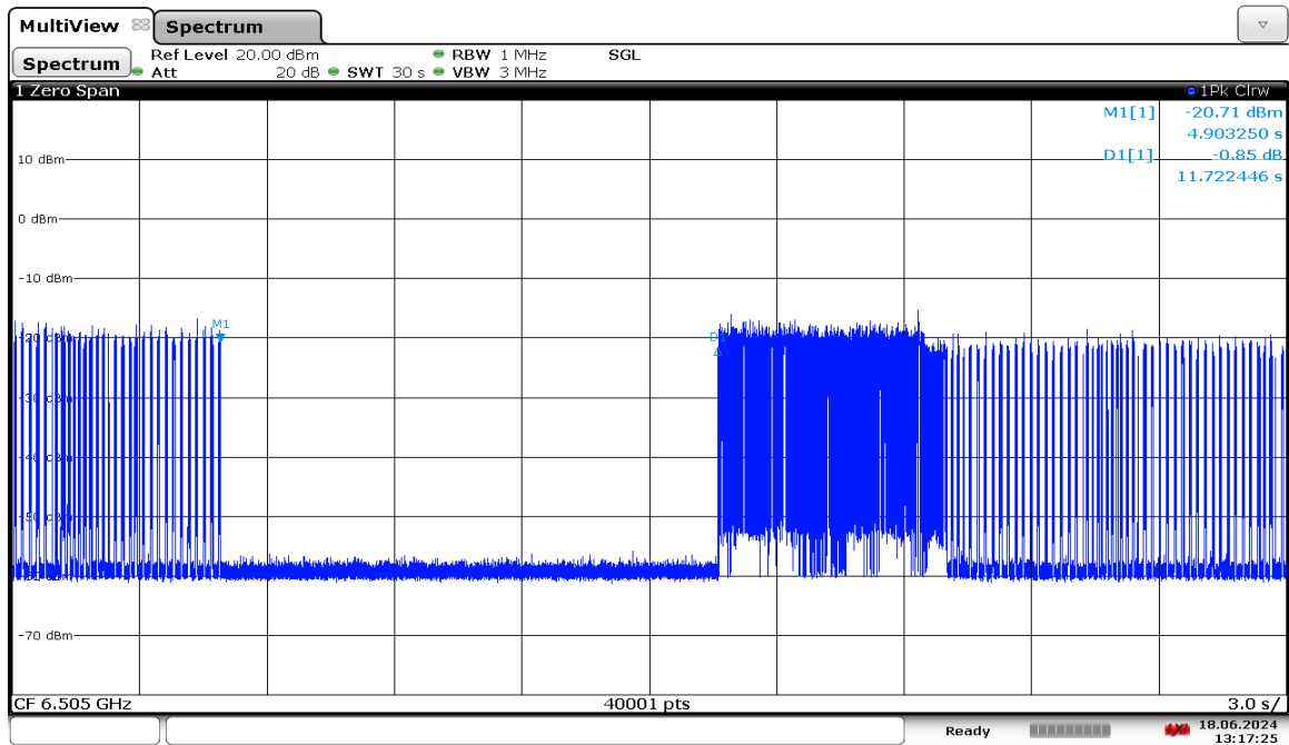
Plot 7-1879. LPI Contention Based Protocol Timing Plot – UNII 6 – 160MHz Channel 111 – High
