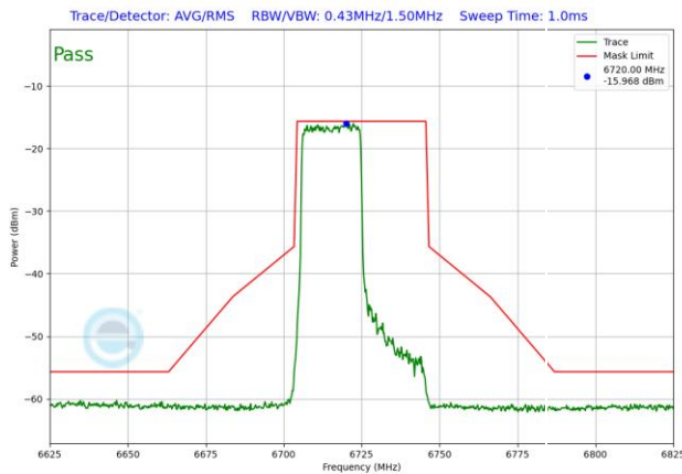
Plot 7-1845. VLP In-Band Emission Plot SDM Diversity Antenna 1b (40MHz 802.11ax RU242 (UNII Band 7) – Ch. 155)
