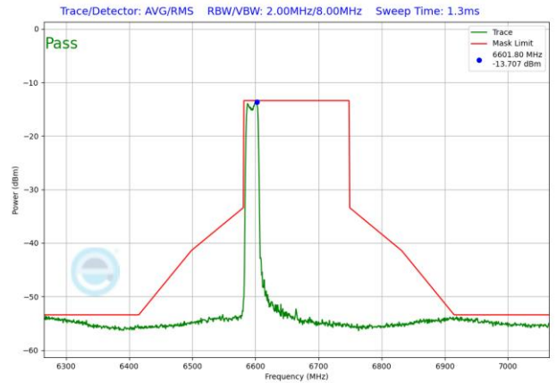
Plot 7-1825. VLP In-Band Emission Plot SDM Antenna 3b (160MHz 802.11ax RU242 (UNII Band 7) – Ch. 143)
