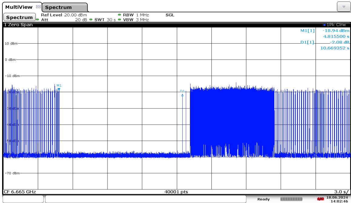
Plot 7-1883. LPI Contention Based Protocol Timing Plot – UNII 7 – 160MHz Channel 143 – High
