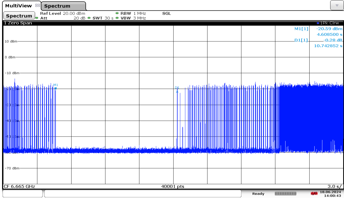
Plot 7-1882. LPI Contention Based Protocol Timing Plot – UNII 7 – 160MHz Channel 143 – Mid
