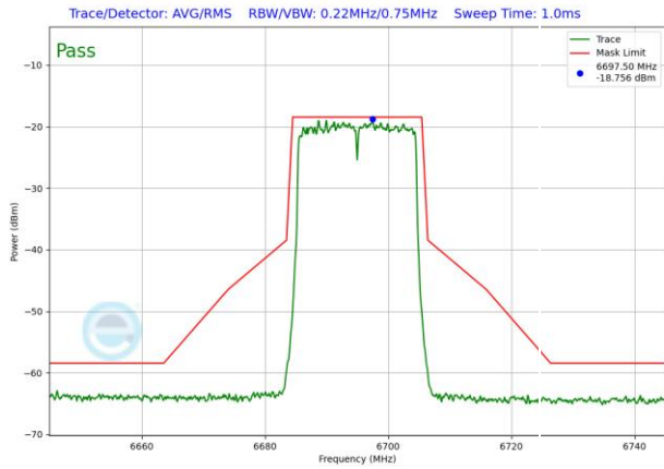
Plot 7-1844. VLP In-Band Emission Plot SDM Diversity Antenna 1b (20MHz 802.11ax RU242 (UNII Band 7) – Ch. 149)
