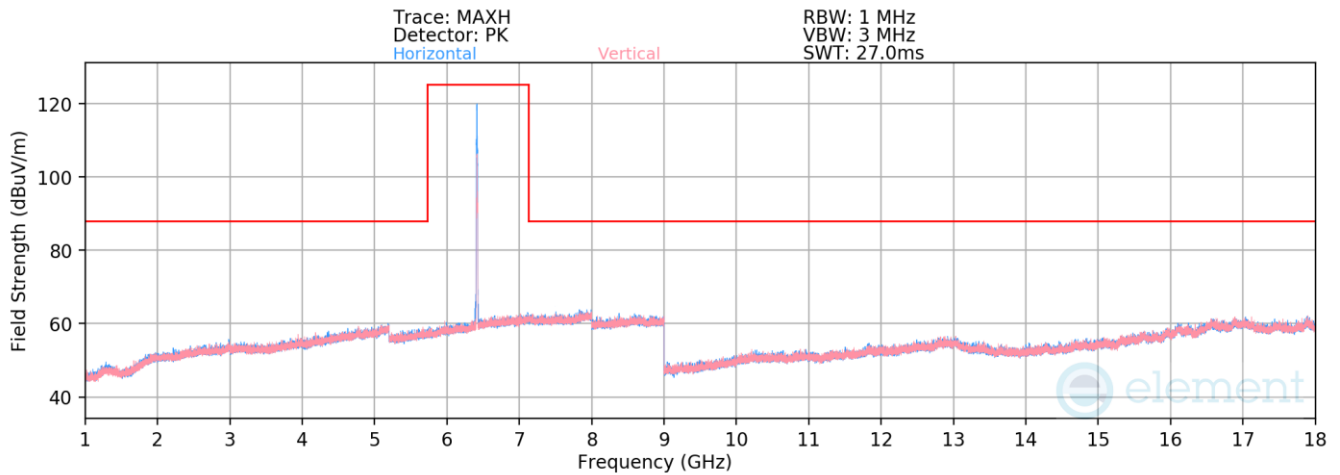
Plot 7-1902. Radiated Spurious Emissions above 1GHz Antenna 5T (802.11ax – Ch. 93 – RU26)
