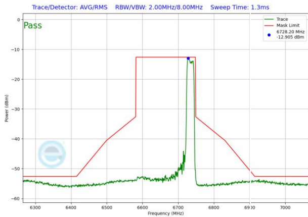
Plot 7-1828. VLP In-Band Emission Plot SDM Antenna WF5T (160MHz 802.11ax RU242 (UNII Band 7) – Ch. 143)
