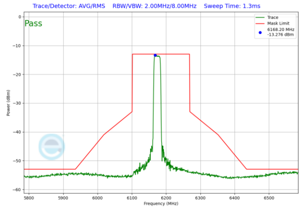
Plot 7-1841. VLP In-Band Emission Plot SDM Diversity Antenna 1b (160MHz 802.11ax RU242 (UNII Band 5) – Ch. 47)
