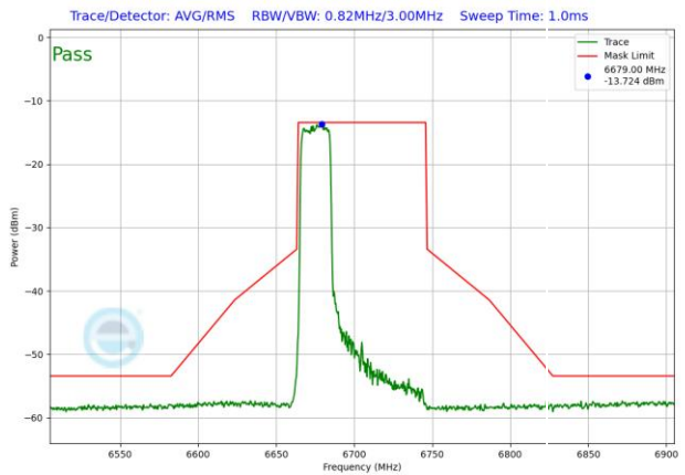
Plot 7-1816. VLP In-Band Emission Plot SDM Antenna WF5T (80MHz 802.11ax RU242 (UNII Band 7) – Ch. 151)
