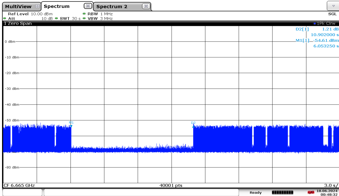
Plot 7-1893. VLP Contention Based Protocol Timing Plot – UNII 7 – 160MHz Channel 143 – Low
