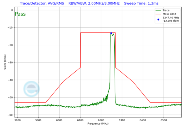
Plot 7-1842. VLP In-Band Emission Plot SDM Diversity Antenna 1b (160MHz 802.11ax RU242 (UNII Band 5) – Ch. 47)
