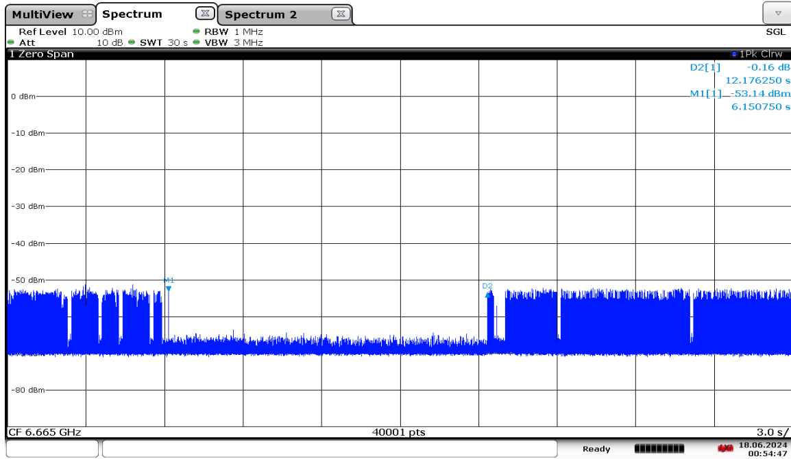
Plot 7-1894. VLP Contention Based Protocol Timing Plot – UNII 7 – 160MHz Channel 143 – Mid
