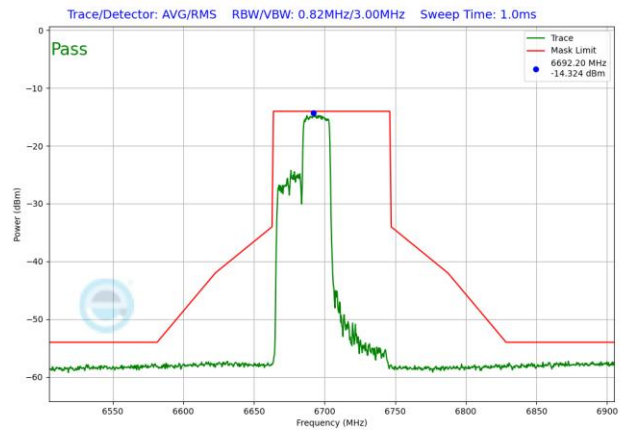
Plot 7-1849. VLP In-Band Emission Plot SDM Diversity Antenna 1b (80MHz 802.11ax RU242 (UNII Band 7) – Ch. 151)
