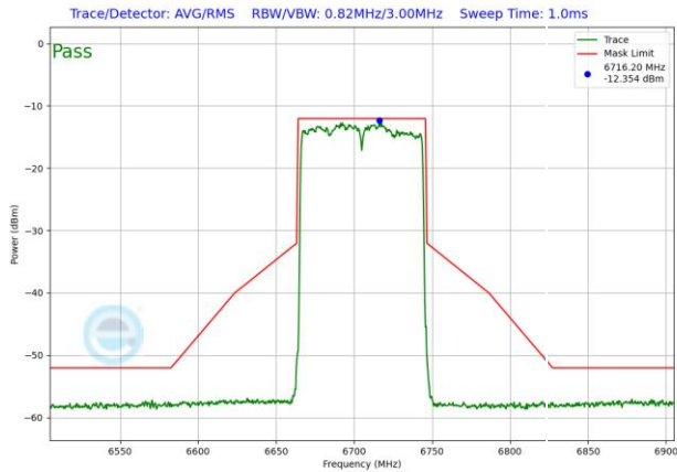
Plot 7-1822. VLP In-Band Emission Plot SDM Antenna WF5T (80MHz 802.11ax RU996 (UNII Band 7) – Ch. 151)
