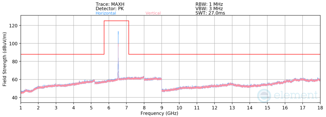
Plot 7-1918. Radiated Spurious Emissions above 1GHz Antenna 5T (802.11ax – Ch. 117 – RU242)
