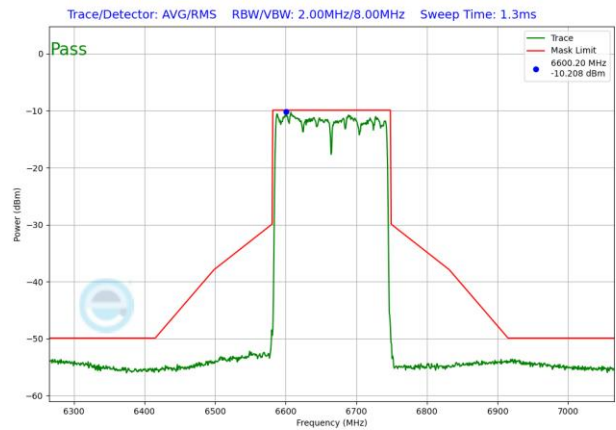
Plot 7-1831. VLP In-Band Emission Plot SDM Antenna 3b (160MHz 802.11ax RU996x2 (UNII Band 7) – Ch. 143)
