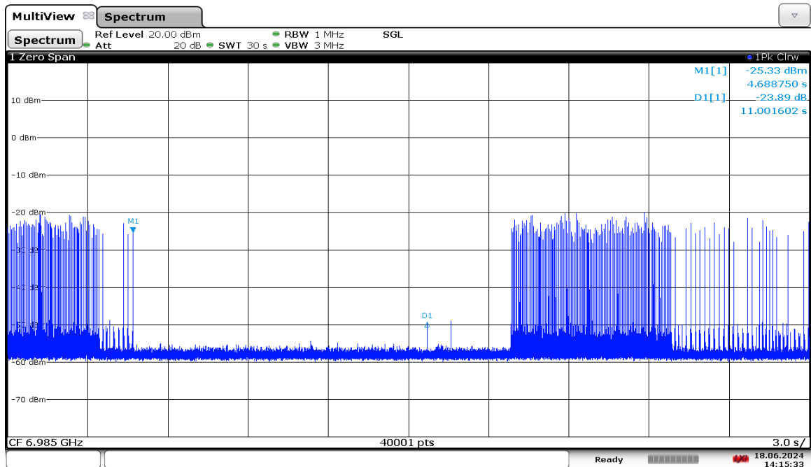
Plot 7-1885. LPI Contention Based Protocol Timing Plot – UNII 8 – 160MHz Channel 207 – Low
