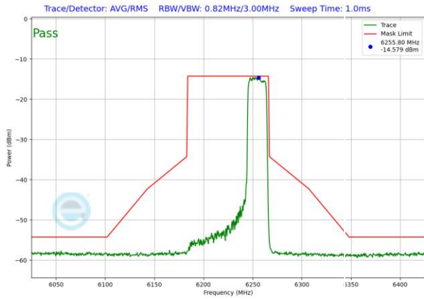
Plot 7-1838. VLP In-Band Emission Plot SDM Diversity Antenna 1b (80MHz 802.11ax RU242 (UNII Band 5) – Ch. 55)
