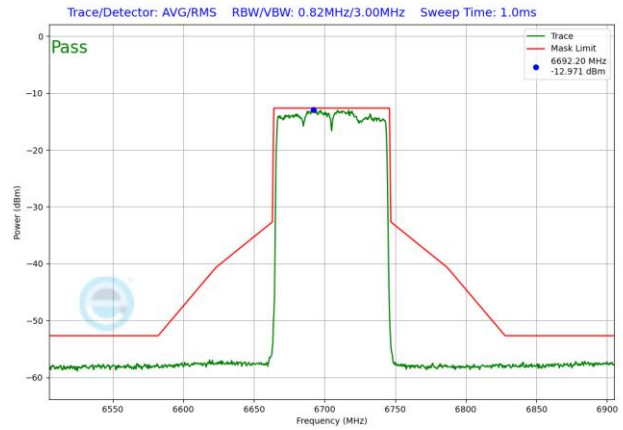
Plot 7-1823. VLP In-Band Emission Plot SDM Antenna 3b (80MHz 802.11ax RU996 (UNII Band 7) – Ch. 151)
