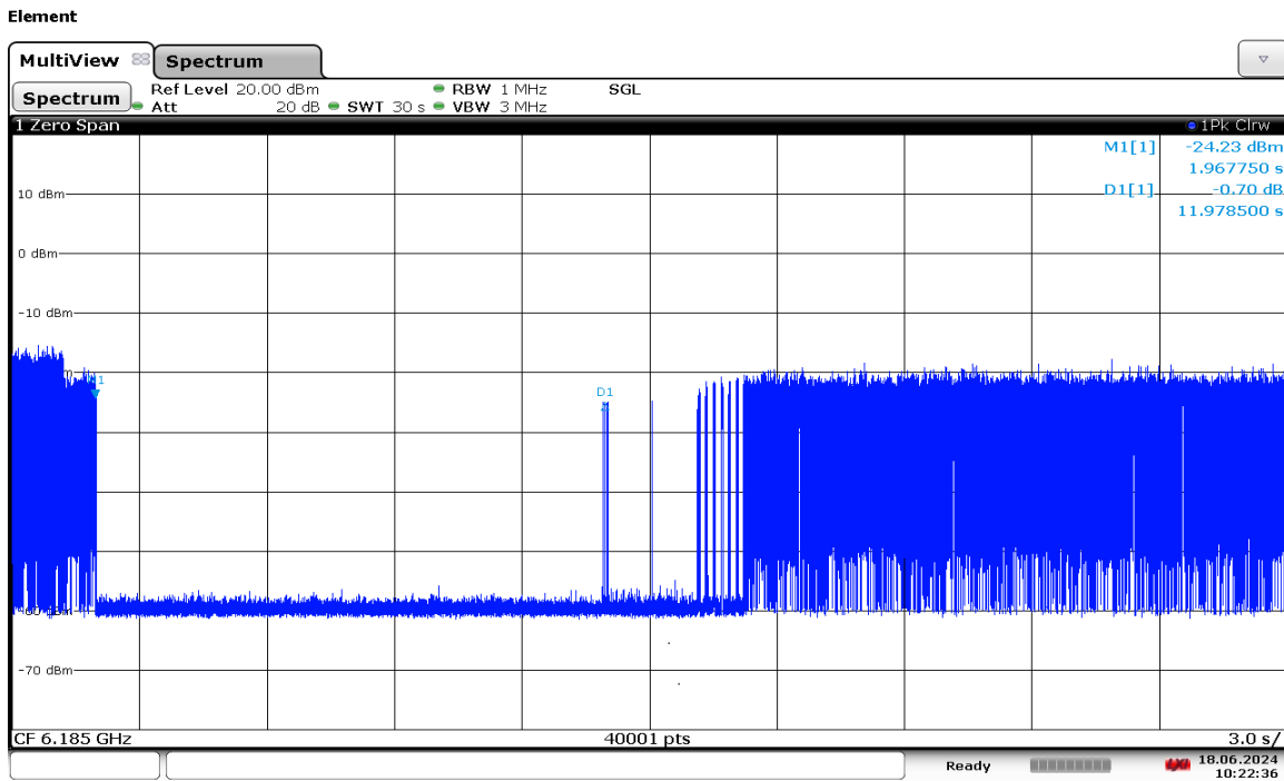
Plot 7-1873. LPI Contention Based Protocol Timing Plot – UNII 5 – 160MHz Channel 47 – Low
