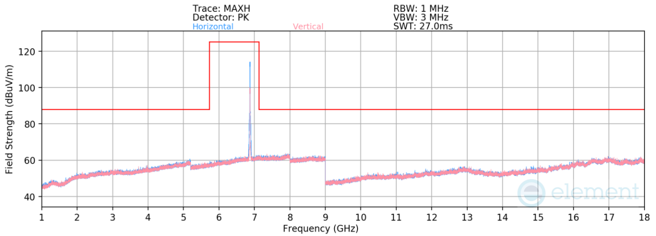
Plot 7-1920. Radiated Spurious Emissions above 1GHz Antenna 5T (802.11ax – Ch. 185 – RU242)
