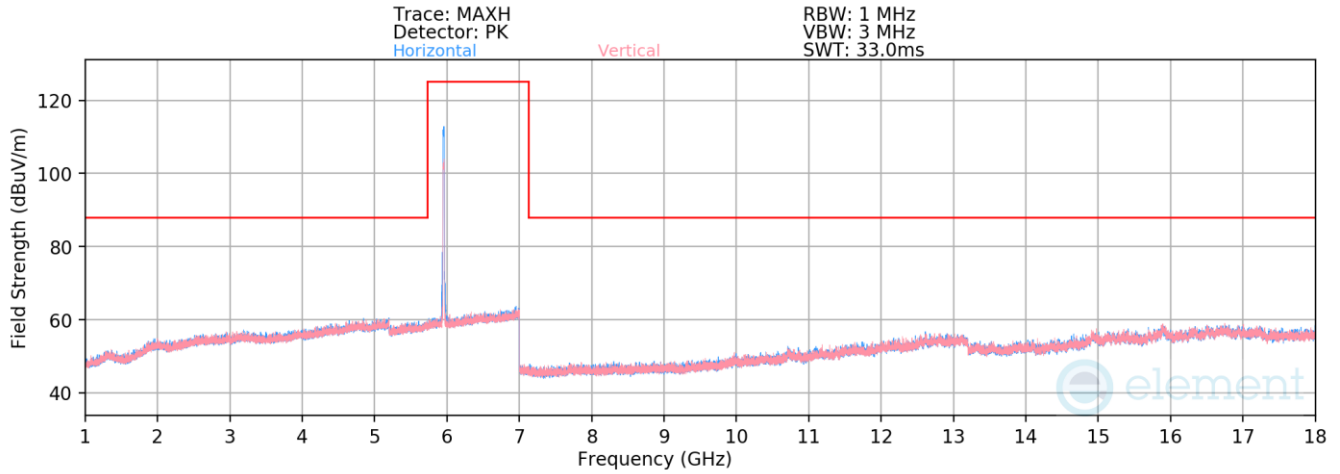
Plot 7-1912. Radiated Spurious Emissions above 1GHz Antenna 5T (802.11ax – Ch. 1 – RU242)
