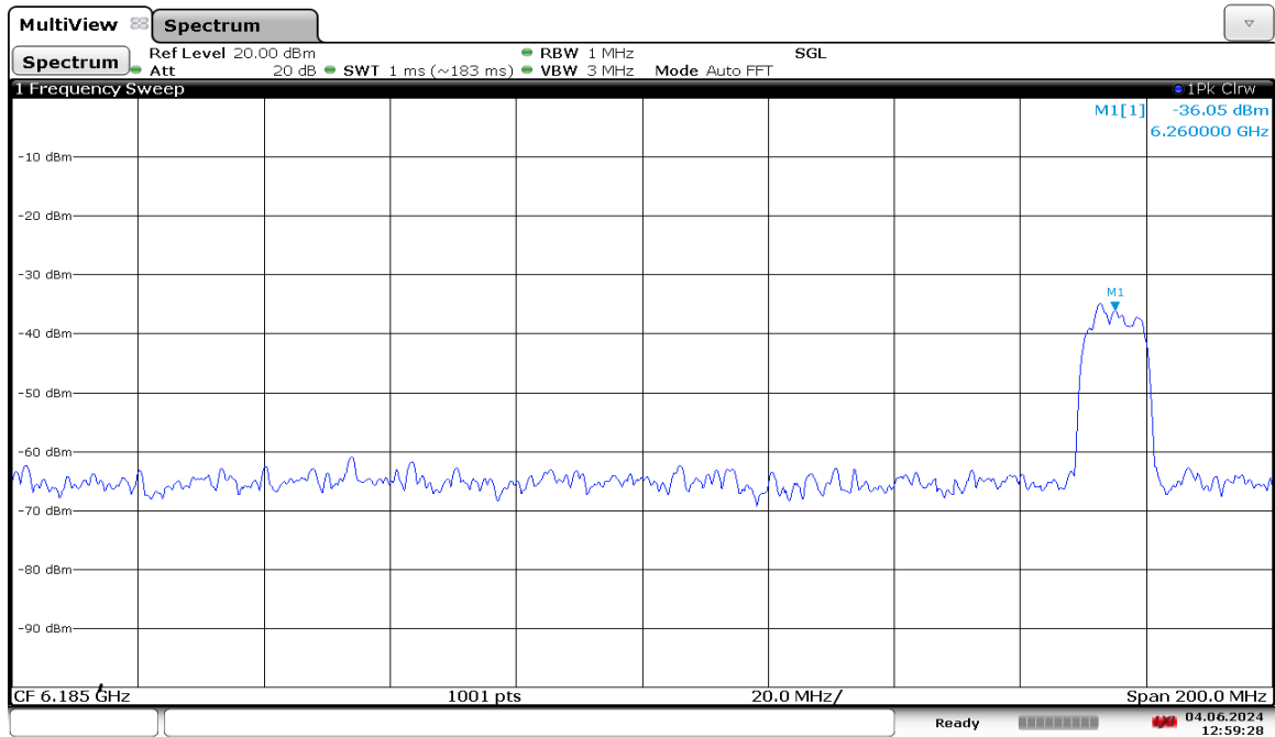
Plot 7-1899. 160MHz Bandwidth – AWGN Signal Injected at High End – Channel 47
