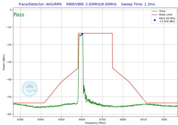
Plot 7-1852. VLP In-Band Emission Plot SDM Diversity Antenna 1b (160MHz 802.11ax RU242 (UNII Band 7) – Ch. 143)
