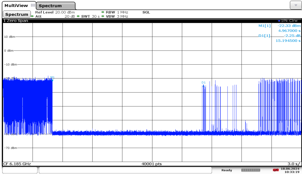
Plot 7-1874. LPI Contention Based Protocol Timing Plot – UNII 5 – 160MHz Channel 47 – Mid
