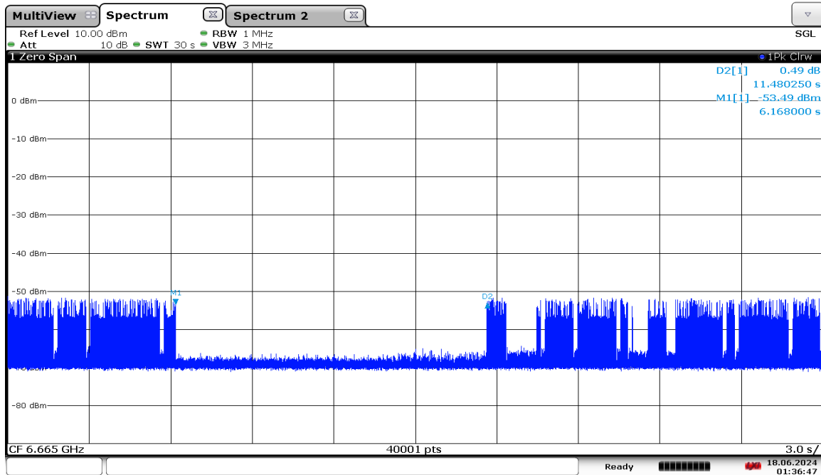
Plot 7-1895. VLP Contention Based Protocol Timing Plot – UNII 7 – 160MHz Channel 143 – High
