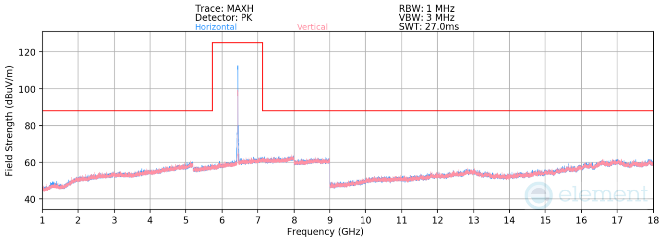
Plot 7-1915. Radiated Spurious Emissions above 1GHz Antenna 5T (802.11ax – Ch. 97 – RU242)
