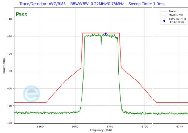
Plot 7-1808. VLP In-Band Emission Plot SDM Antenna WF5T (20MHz 802.11ax RU242 (UNII Band 7) – Ch. 149)
