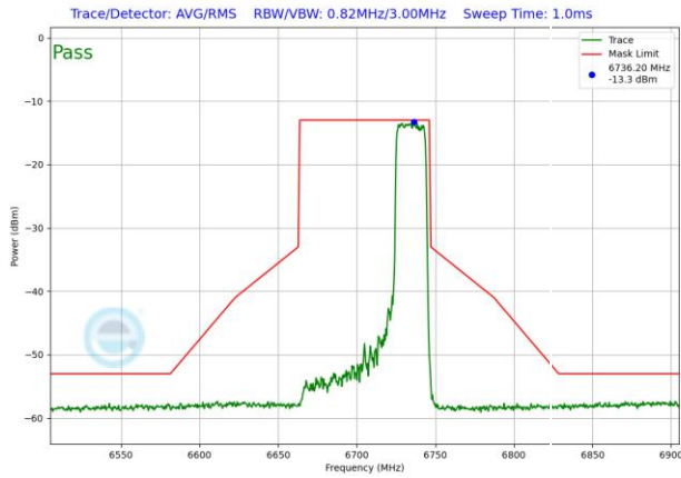
Plot 7-1850. VLP In-Band Emission Plot SDM Diversity Antenna 1b (80MHz 802.11ax RU242 (UNII Band 7) – Ch. 151)
