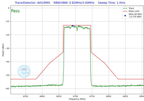
Plot 7-1851. VLP In-Band Emission Plot SDM Diversity Antenna 1b (80MHz 802.11ax RU996 (UNII Band 7) – Ch. 151)
