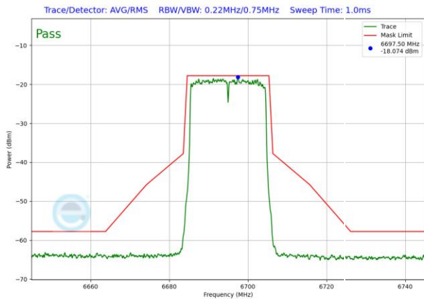
Plot 7-1809. VLP In-Band Emission Plot SDM Antenna 3b (20MHz 802.11ax RU242 (UNII Band 7) – Ch. 149)
