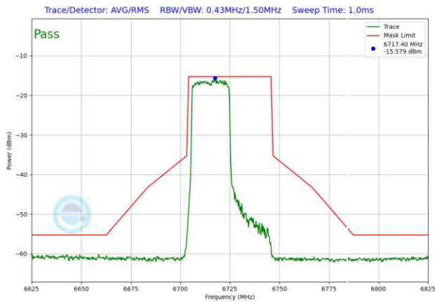
Plot 7-1810. VLP In-Band Emission Plot SDM Antenna WF5T (40MHz 802.11ax RU242 (UNII Band 7) – Ch. 155)
