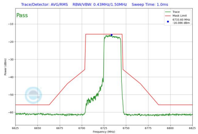
Plot 7-1813. VLP In-Band Emission Plot SDM Antenna 3b (40MHz 802.11ax RU242 (UNII Band 7) – Ch. 155)
