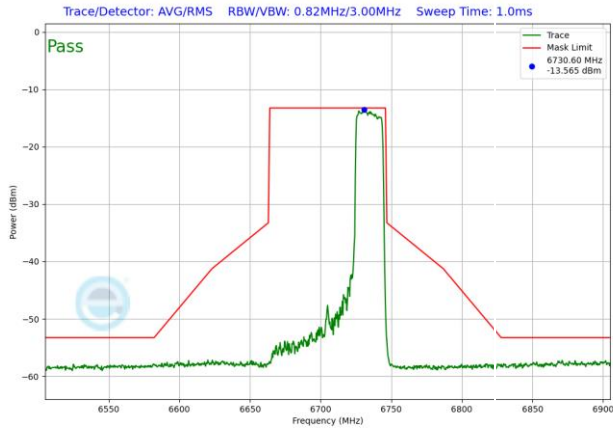
Plot 7-1821. VLP In-Band Emission Plot SDM Antenna 3b (80MHz 802.11ax RU242 (UNII Band 7) – Ch. 151)
