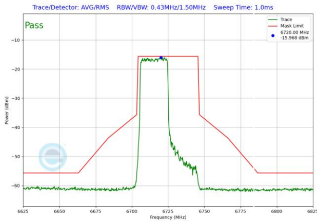
Plot 7-1846. VLP In-Band Emission Plot SDM Diversity Antenna 1b (40MHz 802.11ax RU242 (UNII Band 7) – Ch. 155)
