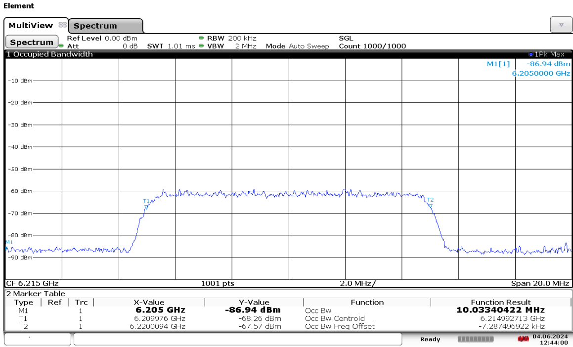
Plot 7-1856. AWGN Signal – UNII 5 – 20MHz
