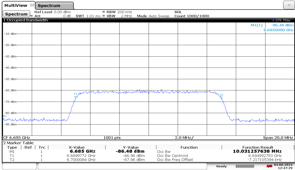
Plot 7-1864. AWGN Signal – UNII 7 – 20MHz
