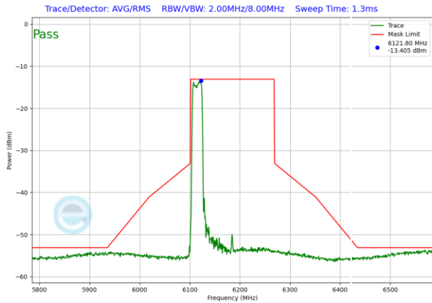
Plot 7-1840. VLP In-Band Emission Plot SDM Diversity Antenna 1b (160MHz 802.11ax RU242 (UNII Band 5) – Ch. 47)
