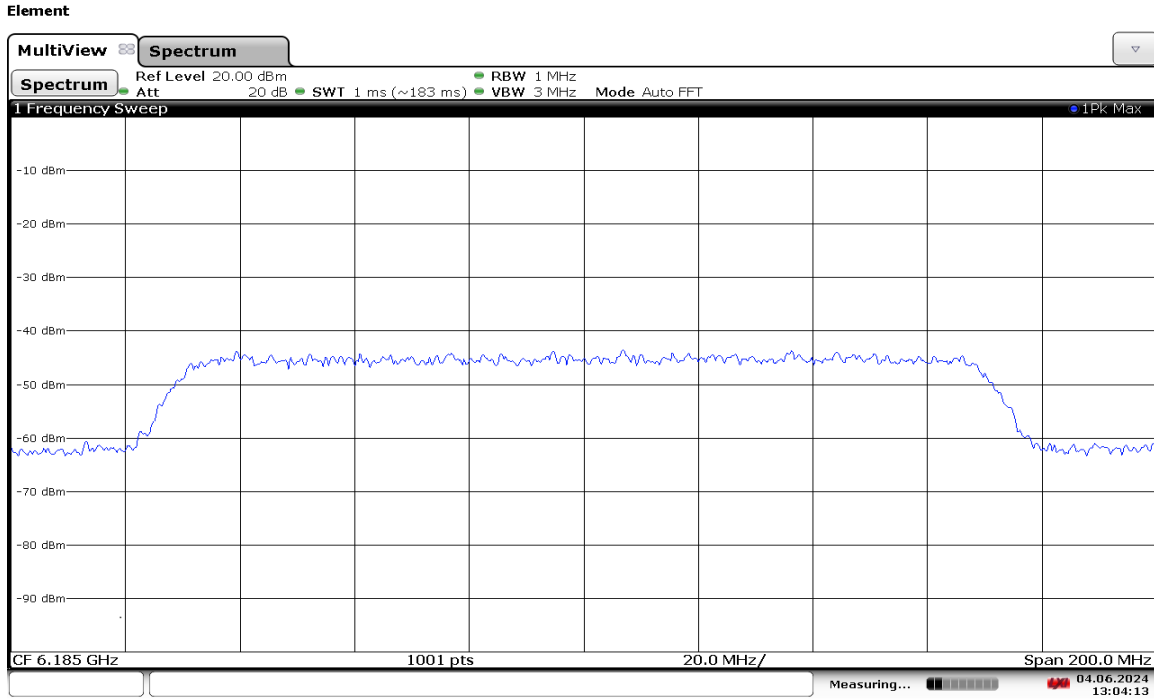
Plot 7-1896. 160MHz Bandwidth – Before AWGN Signal Injected – Channel 47
