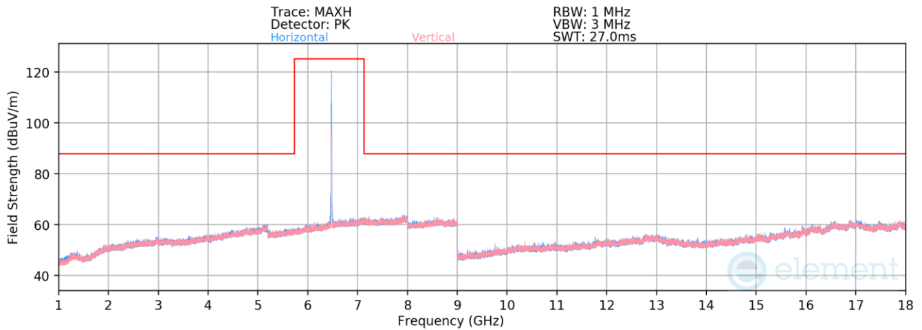
Plot 7-1904. Radiated Spurious Emissions above 1GHz Antenna 5T (802.11ax – Ch. 105 – RU26)
