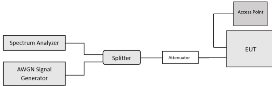
Figure 2. Contention-based protocol, Conducted Setup
