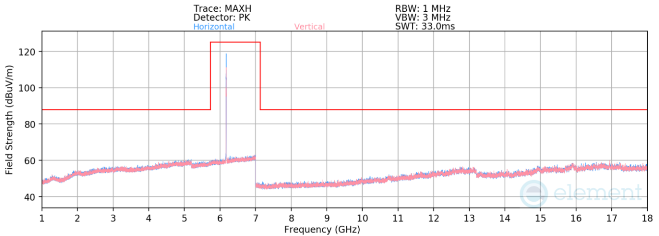
Plot 7-1901. Radiated Spurious Emissions above 1GHz Antenna 5T (802.11ax – Ch. 45 – RU26)
