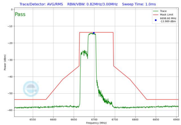
Plot 7-1819. VLP In-Band Emission Plot SDM Antenna 3b (80MHz 802.11ax RU242 (UNII Band 7) – Ch. 151)
