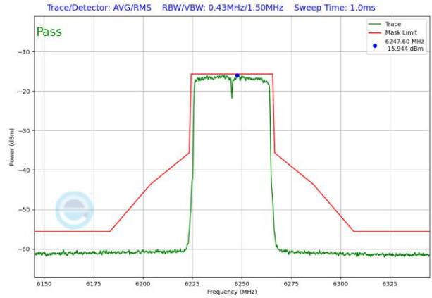
Plot 7-1835. VLP In-Band Emission Plot SDM Diversity Antenna 1b (40MHz 802.11ax RU484 (UNII Band 5) – Ch. 59)
