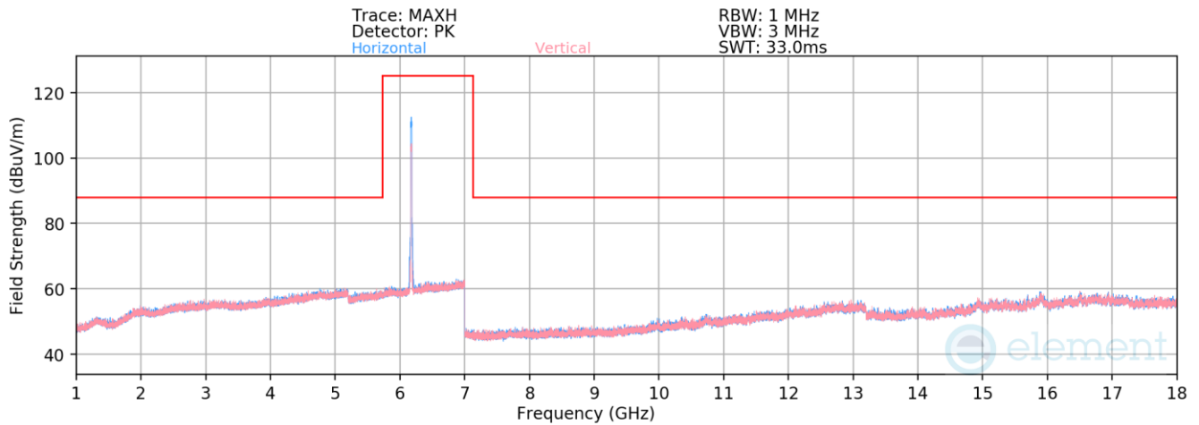
Plot 7-1913. Radiated Spurious Emissions above 1GHz Antenna 5T (802.11ax – Ch. 45 – RU242)
