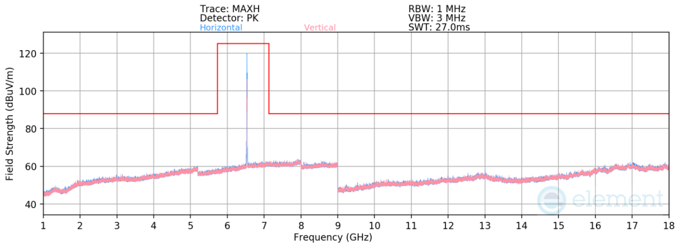
Plot 7-1906. Radiated Spurious Emissions above 1GHz Antenna 5T (802.11ax – Ch. 117 – RU26)
