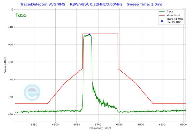
Plot 7-1848. VLP In-Band Emission Plot SDM Diversity Antenna 1b (80MHz 802.11ax RU242 (UNII Band 7) – Ch. 151)
