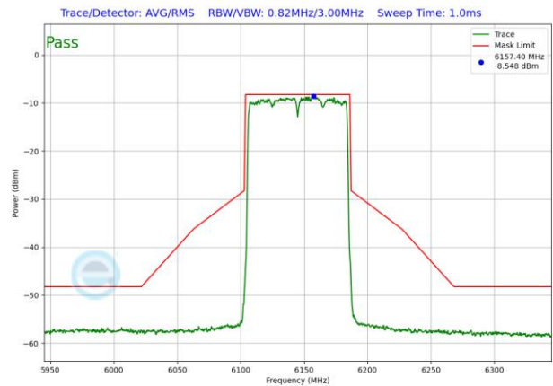
Plot 7-1523. LPI In-Band Emission Plot SDM Antenna WF5T (80MHz 802.11ax RU996 (UNII Band 5) – Ch. 39)
