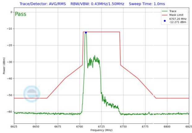
Plot 7-1573. LPI In-Band Emission Plot SDM Antenna WF5T (40MHz 802.11ax RU26 (UNII Band 7) – Ch. 155)
