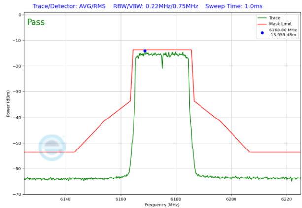
Plot 7-1632. LPI In-Band Emission Plot SDM Diversity Antenna 1b (20MHz 802.11ax RU242 (UNII Band 5) – Ch. 45)
