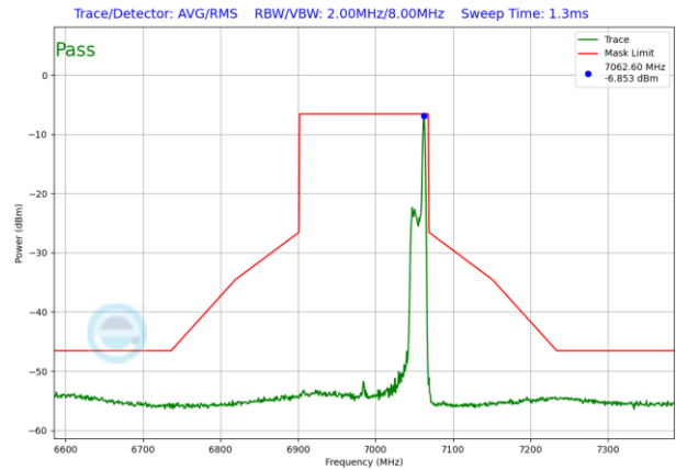
Plot 7-1626. LPI In-Band Emission Plot SDM Antenna 3b (160MHz 802.11ax RU26 (UNII Band 8) – Ch. 207)
