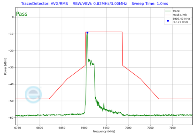
Plot 7-1613. LPI In-Band Emission Plot SDM Antenna WF5T (80MHz 802.11ax RU26 (UNII Band 8) – Ch. 199)
