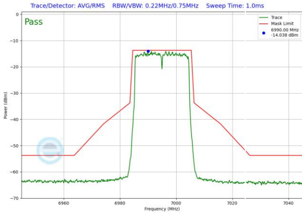
Plot 7-1604. LPI In-Band Emission Plot SDM Antenna 3b (20MHz 802.11ax RU242 (UNII Band 8) – Ch. 209)
