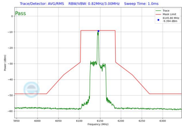
Plot 7-1638. LPI In-Band Emission Plot SDM Diversity Antenna 1b (80MHz 802.11ax RU26 (UNII Band 5) – Ch. 39)
