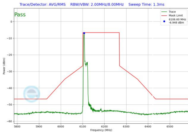
Plot 7-1526. LPI In-Band Emission Plot SDM Antenna 3b (160MHz 802.11ax RU26 (UNII Band 5) – Ch. 47)
