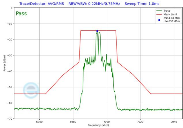
Plot 7-1600. LPI In-Band Emission Plot SDM Antenna 3b (20MHz 802.11ax RU26 (UNII Band 8) – Ch. 209)
