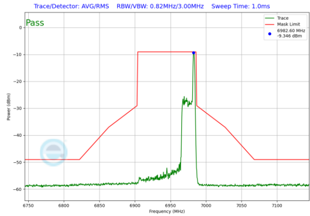
Plot 7-1618. LPI In-Band Emission Plot SDM Antenna 3b (80MHz 802.11ax RU26 (UNII Band 8) – Ch. 199)
