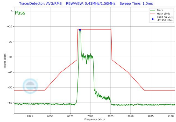
Plot 7-1606. LPI In-Band Emission Plot SDM Antenna 3b (40MHz 802.11ax RU26 (UNII Band 8) – Ch. 211)
