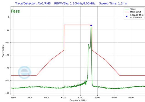
Plot 7-1643. LPI In-Band Emission Plot SDM Diversity Antenna 1b (160MHz 802.11ax RU26 (UNII Band 5) – Ch. 47)
