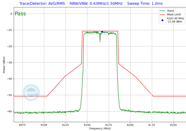
Plot 7-1636. LPI In-Band Emission Plot SDM Diversity Antenna 1b (40MHz 802.11ax RU484 (UNII Band 5) – Ch. 43)
