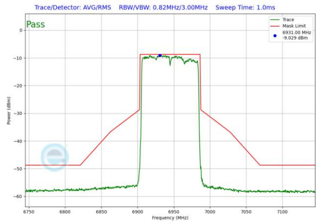
Plot 7-1619. LPI In-Band Emission Plot SDM Antenna WF5T (80MHz 802.11ax RU996 (UNII Band 8) – Ch. 199)
