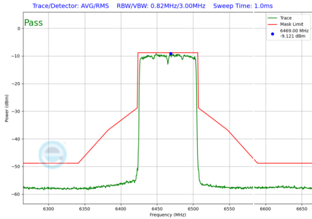
Plot 7-1556. LPI In-Band Emission Plot SDM Antenna 3b (80MHz 802.11ax RU996 (UNII Band 6) – Ch. 103)
