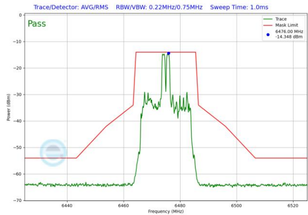
Plot 7-1646. LPI In-Band Emission Plot SDM Diversity Antenna 1b (20MHz 802.11ax RU26 (UNII Band 6) – Ch. 105)
