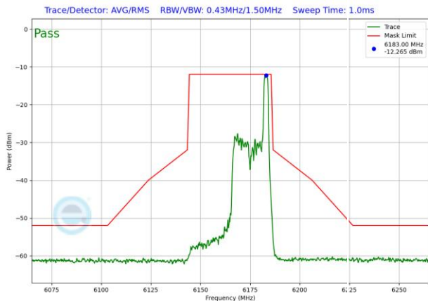
Plot 7-1514. LPI In-Band Emission Plot SDM Antenna 3b (40MHz 802.11ax RU26 (UNII Band 5) – Ch. 43)
