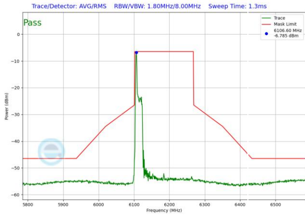
Plot 7-1641. LPI In-Band Emission Plot SDM Diversity Antenna 1b (160MHz 802.11ax RU26 (UNII Band 5) – Ch. 47)
