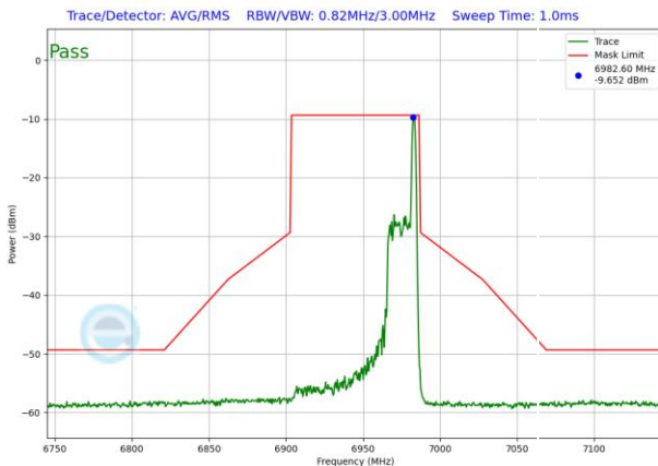
Plot 7-1617. LPI In-Band Emission Plot SDM Antenna WF5T (80MHz 802.11ax RU26 (UNII Band 8) – Ch. 199)
