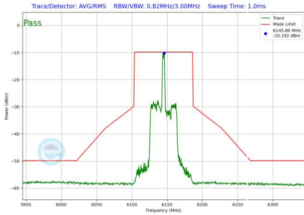
Plot 7-1519. LPI In-Band Emission Plot SDM Antenna WF5T (80MHz 802.11ax RU26 (UNII Band 5) – Ch. 39)
