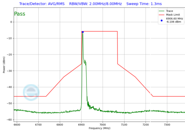
Plot 7-1621. LPI In-Band Emission Plot SDM Antenna WF5T (160MHz 802.11ax RU26 (UNII Band 8) – Ch. 207)
