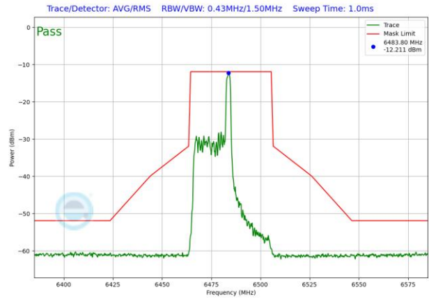
Plot 7-1650. LPI In-Band Emission Plot SDM Diversity Antenna 1b (40MHz 802.11ax RU26 (UNII Band 6) – Ch. 107)
