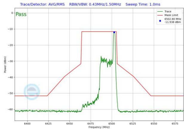
Plot 7-1651. LPI In-Band Emission Plot SDM Diversity Antenna 1b (40MHz 802.11ax RU26 (UNII Band 6) – Ch. 107)
