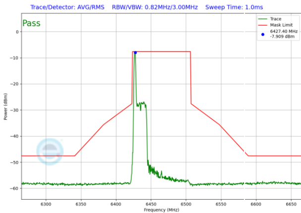
Plot 7-1550. LPI In-Band Emission Plot SDM Antenna 3b (80MHz 802.11ax RU26 (UNII Band 6) – Ch. 103)
