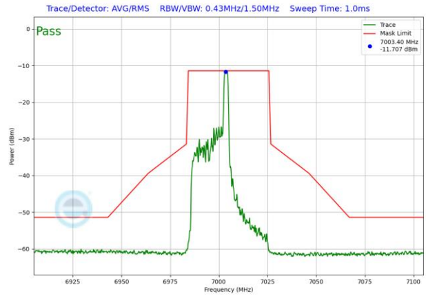
Plot 7-1608. LPI In-Band Emission Plot SDM Antenna 3b (40MHz 802.11ax RU26 (UNII Band 8) – Ch. 211)
