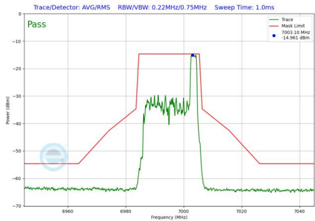
Plot 7-1602. LPI In-Band Emission Plot SDM Antenna 3b (20MHz 802.11ax RU26 (UNII Band 8) – Ch. 209)
