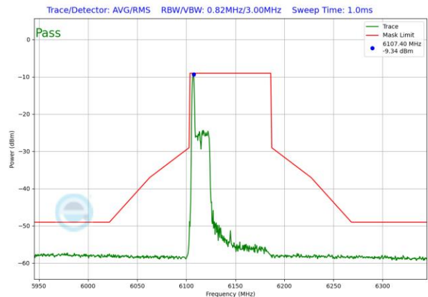
Plot 7-1517. LPI In-Band Emission Plot SDM Antenna WF5T (80MHz 802.11ax RU26 (UNII Band 5) – Ch. 39)
