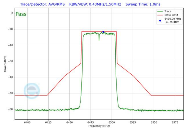
Plot 7-1652. LPI In-Band Emission Plot SDM Diversity Antenna 1b (40MHz 802.11ax RU484 (UNII Band 6) – Ch. 107)
