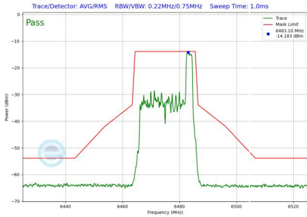
Plot 7-1647. LPI In-Band Emission Plot SDM Diversity Antenna 1b (20MHz 802.11ax RU26 (UNII Band 6) – Ch. 105)
