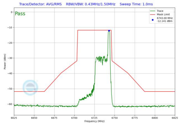
Plot 7-1577. LPI In-Band Emission Plot SDM Antenna WF5T (40MHz 802.11ax RU26 (UNII Band 7) – Ch. 155)
