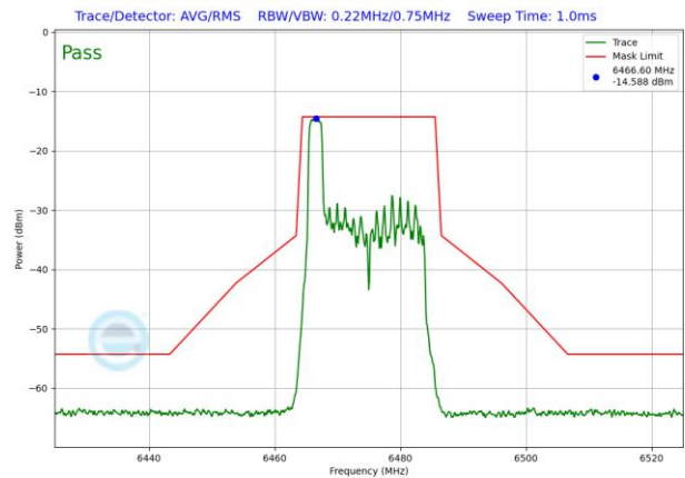
Plot 7-1645. LPI In-Band Emission Plot SDM Diversity Antenna 1b (20MHz 802.11ax RU26 (UNII Band 6) – Ch. 105)
