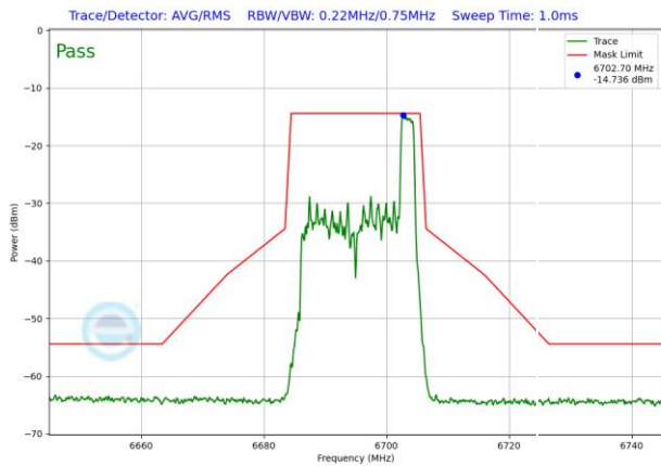
Plot 7-1569. LPI In-Band Emission Plot SDM Antenna WF5T (20MHz 802.11ax RU26 (UNII Band 7) – Ch. 149)
