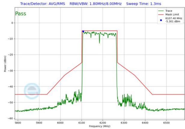
Plot 7-1644. LPI In-Band Emission Plot SDM Diversity Antenna 1b (160MHz 802.11ax RU996x2 (UNII Band 5) – Ch. 47)
