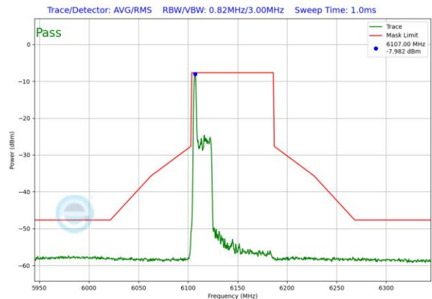
Plot 7-1518. LPI In-Band Emission Plot SDM Antenna 3b (80MHz 802.11ax RU26 (UNII Band 5) – Ch. 39)
