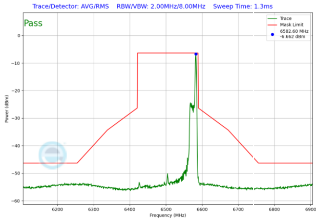
Plot 7-1561. LPI In-Band Emission Plot SDM Antenna WF5T (160MHz 802.11ax RU26 (UNII Band 6) – Ch. 111)
