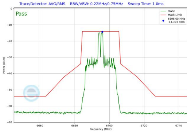
Plot 7-1567. LPI In-Band Emission Plot SDM Antenna WF5T (20MHz 802.11ax RU26 (UNII Band 7) – Ch. 149)
