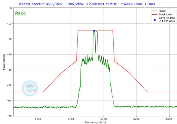
Plot 7-1630. LPI In-Band Emission Plot SDM Diversity Antenna 1b (20MHz 802.11ax RU26 (UNII Band 5) – Ch. 45)
