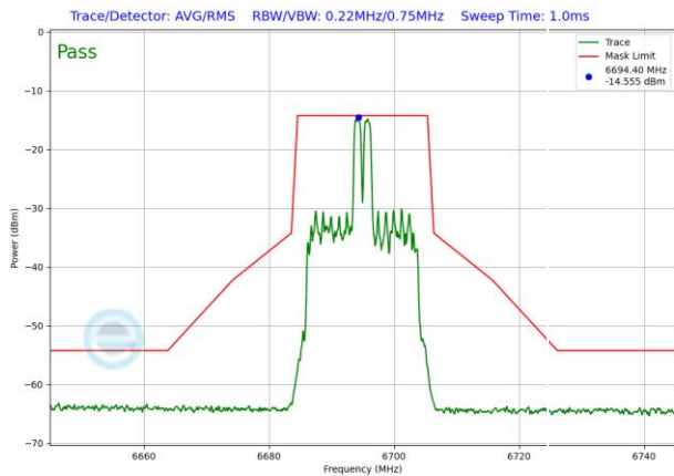
Plot 7-1568. LPI In-Band Emission Plot SDM Antenna 3b (20MHz 802.11ax RU26 (UNII Band 7) – Ch. 149)
