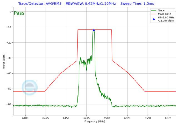
Plot 7-1543. LPI In-Band Emission Plot SDM Antenna WF5T (40MHz 802.11ax RU26 (UNII Band 6) – Ch. 107)
