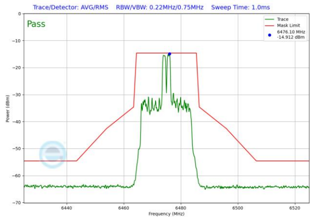
Plot 7-1535. LPI In-Band Emission Plot SDM Antenna WF5T (20MHz 802.11ax RU26 (UNII Band 6) – Ch. 105)
