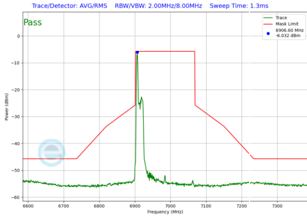
Plot 7-1622. LPI In-Band Emission Plot SDM Antenna 3b (160MHz 802.11ax RU26 (UNII Band 8) – Ch. 207)
