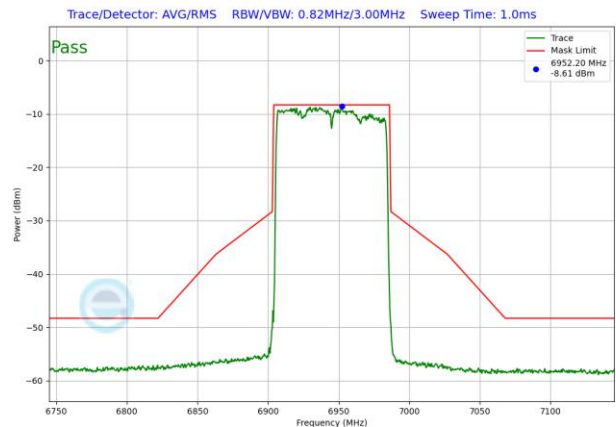
Plot 7-1620. LPI In-Band Emission Plot SDM Antenna 3b (80MHz 802.11ax RU996 (UNII Band 8) – Ch. 199)
