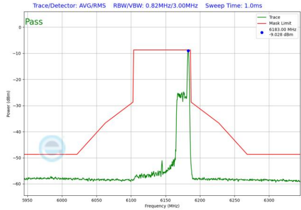
Plot 7-1639. LPI In-Band Emission Plot SDM Diversity Antenna 1b (80MHz 802.11ax RU26 (UNII Band 5) – Ch. 39)
