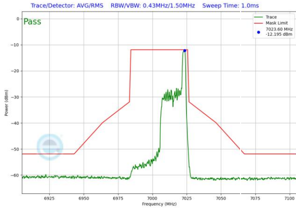
Plot 7-1610. LPI In-Band Emission Plot SDM Antenna 3b (40MHz 802.11ax RU26 (UNII Band 8) – Ch. 211)
