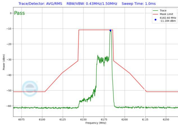
Plot 7-1513. LPI In-Band Emission Plot SDM Antenna WF5T (40MHz 802.11ax RU26 (UNII Band 5) – Ch. 43)
