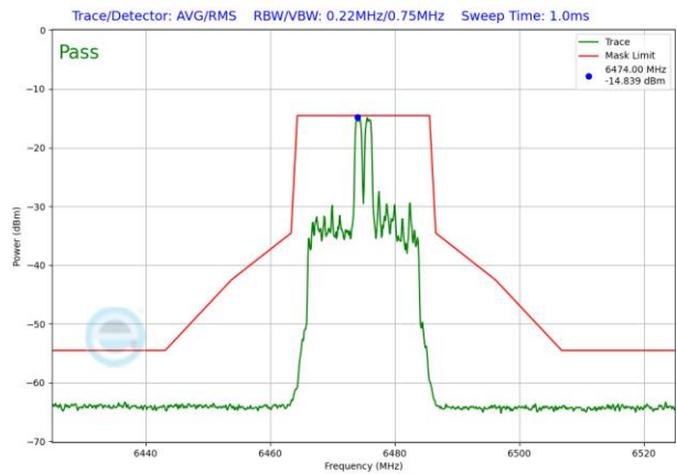
Plot 7-1536. LPI In-Band Emission Plot SDM Antenna 3b (20MHz 802.11ax RU26 (UNII Band 6) – Ch. 105)
