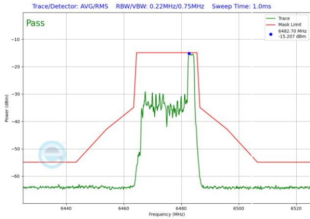
Plot 7-1537. LPI In-Band Emission Plot SDM Antenna WF5T (20MHz 802.11ax RU26 (UNII Band 6) – Ch. 105)
