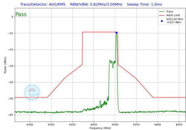
Plot 7-1553. LPI In-Band Emission Plot SDM Antenna WF5T (80MHz 802.11ax RU26 (UNII Band 6) – Ch. 103)
