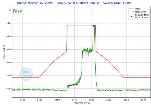
Plot 7-1546. LPI In-Band Emission Plot SDM Antenna 3b (40MHz 802.11ax RU26 (UNII Band 6) – Ch. 107)
