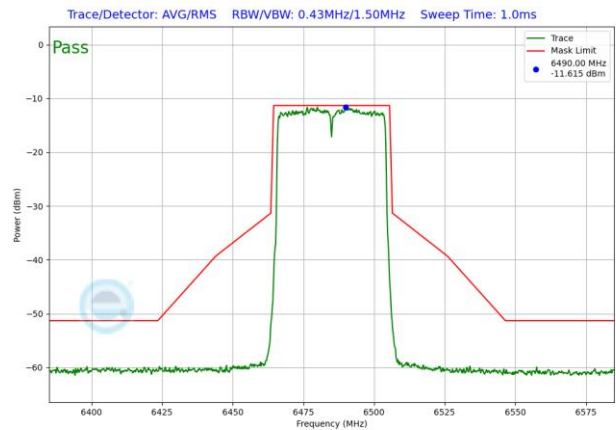
Plot 7-1547. LPI In-Band Emission Plot SDM Antenna WF5T (40MHz 802.11ax RU484 (UNII Band 6) – Ch. 107)
