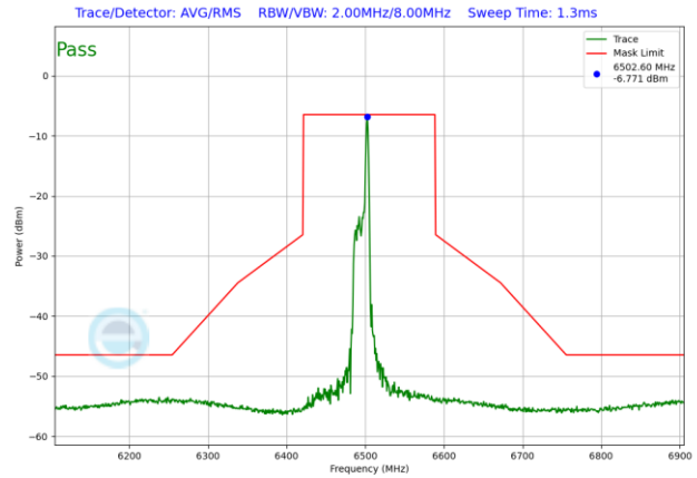
Plot 7-1559. LPI In-Band Emission Plot SDM Antenna WF5T (160MHz 802.11ax RU26 (UNII Band 6) – Ch. 111)
