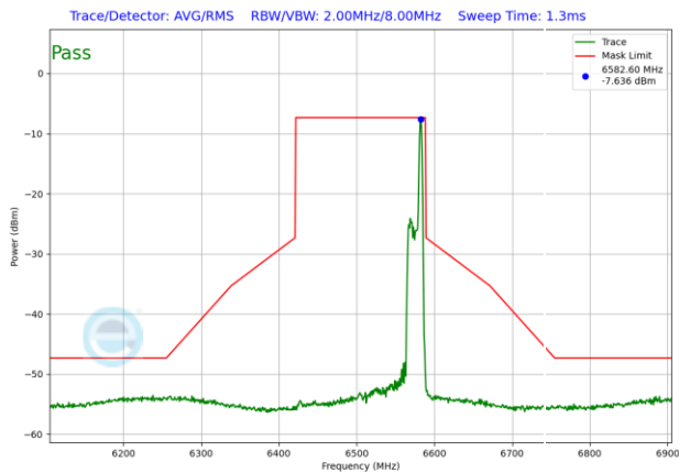
Plot 7-1562. LPI In-Band Emission Plot SDM Antenna 3b (160MHz 802.11ax RU26 (UNII Band 6) – Ch. 111)
