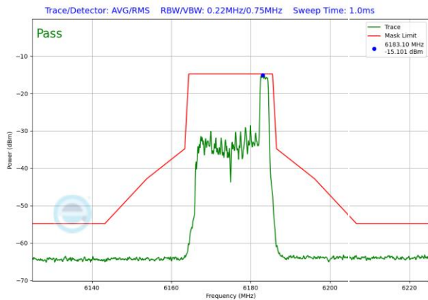
Plot 7-1631. LPI In-Band Emission Plot SDM Diversity Antenna 1b (20MHz 802.11ax RU26 (UNII Band 5) – Ch. 45)
