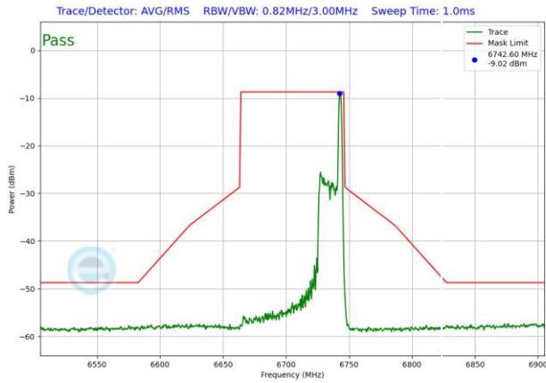
Plot 7-1585. LPI In-Band Emission Plot SDM Antenna WF5T (80MHz 802.11ax RU26 (UNII Band 7) – Ch. 151)
