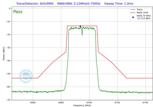
Plot 7-1571. LPI In-Band Emission Plot SDM Antenna WF5T (20MHz 802.11ax RU242 (UNII Band 7) – Ch. 149)
