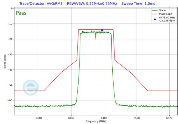
Plot 7-1540. LPI In-Band Emission Plot SDM Antenna 3b (20MHz 802.11ax RU242 (UNII Band 6) – Ch. 105)
