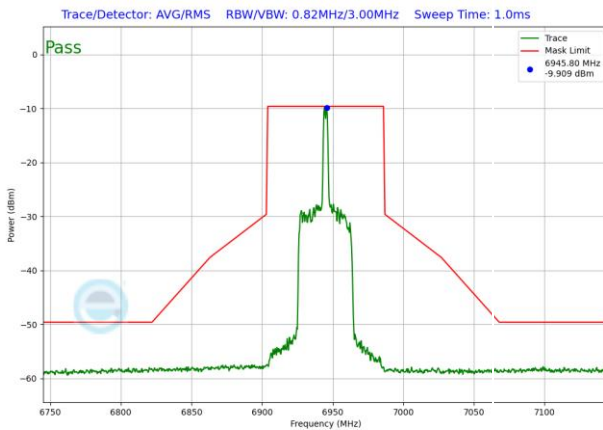
Plot 7-1616. LPI In-Band Emission Plot SDM Antenna 3b (80MHz 802.11ax RU26 (UNII Band 8) – Ch. 199)
