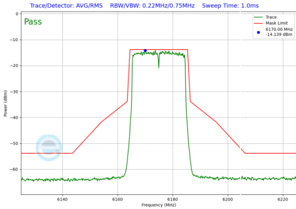
Plot 7-1508. LPI In-Band Emission Plot SDM Antenna 3b (20MHz 802.11ax RU242 (UNII Band 5) – Ch. 45)
