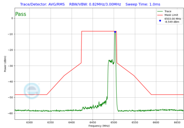
Plot 7-1554. LPI In-Band Emission Plot SDM Antenna 3b (80MHz 802.11ax RU26 (UNII Band 6) – Ch. 103)
