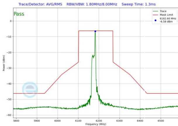
Plot 7-1642. LPI In-Band Emission Plot SDM Diversity Antenna 1b (160MHz 802.11ax RU26 (UNII Band 5) – Ch. 47)
