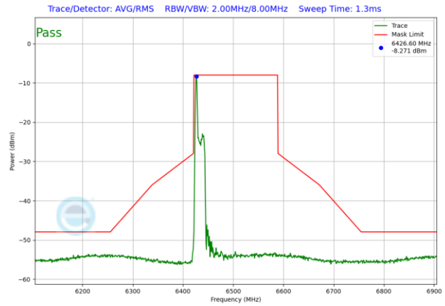
Plot 7-1558. LPI In-Band Emission Plot SDM Antenna 3b (160MHz 802.11ax RU26 (UNII Band 6) – Ch. 111)
