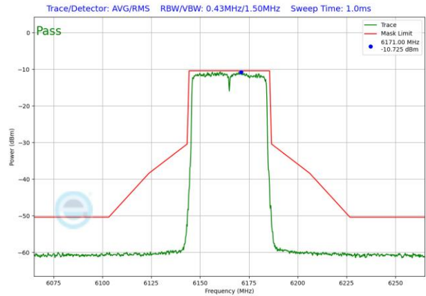
Plot 7-1516. LPI In-Band Emission Plot SDM Antenna 3b (40MHz 802.11ax RU484 (UNII Band 5) – Ch. 43)
