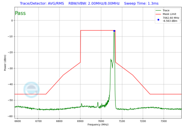
Plot 7-1625. LPI In-Band Emission Plot SDM Antenna WF5T (160MHz 802.11ax RU26 (UNII Band 8) – Ch. 207)
