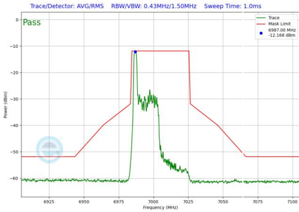
Plot 7-1605. LPI In-Band Emission Plot SDM Antenna WF5T (40MHz 802.11ax RU26 (UNII Band 8) – Ch. 211)
