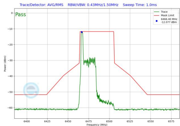
Plot 7-1542. LPI In-Band Emission Plot SDM Antenna 3b (40MHz 802.11ax RU26 (UNII Band 6) – Ch. 107)
