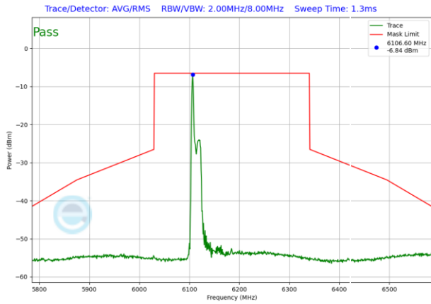
Plot 7-1525. LPI In-Band Emission Plot SDM Antenna WF5T (160MHz 802.11ax RU26 (UNII Band 5) – Ch. 47)
