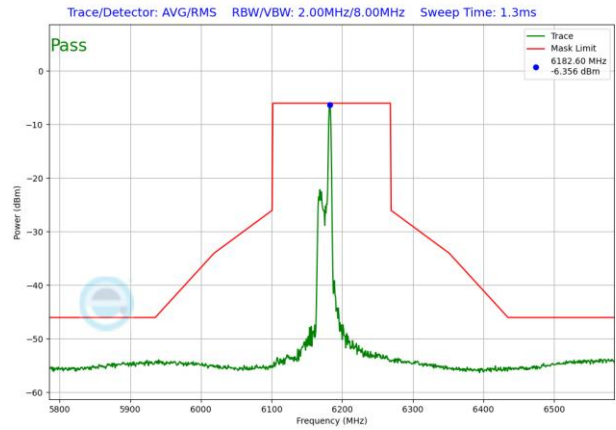
Plot 7-1528. LPI In-Band Emission Plot SDM Antenna 3b (160MHz 802.11ax RU26 (UNII Band 5) – Ch. 47)
