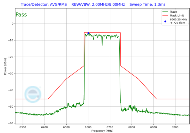
Plot 7-1596. LPI In-Band Emission Plot SDM Antenna 3b (160MHz 802.11ax RU996x2 (UNII Band 7) – Ch. 143)
