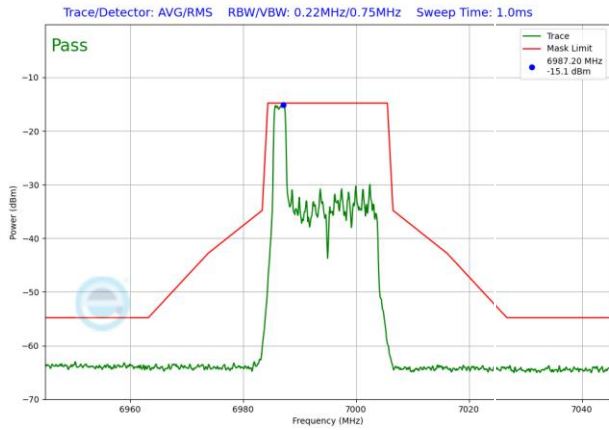
Plot 7-1597. LPI In-Band Emission Plot SDM Antenna WF5T (20MHz 802.11ax RU26 (UNII Band 8) – Ch. 209)
