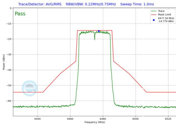
Plot 7-1648. LPI In-Band Emission Plot SDM Diversity Antenna 1b (20MHz 802.11ax RU242 (UNII Band 6) – Ch. 105)
