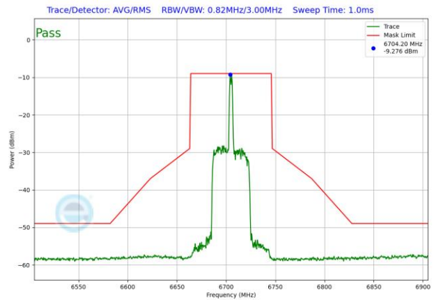
Plot 7-1584. LPI In-Band Emission Plot SDM Antenna 3b (80MHz 802.11ax RU26 (UNII Band 7) – Ch. 151)
