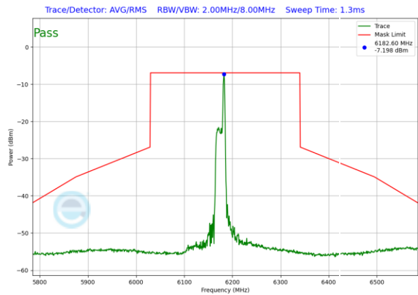
Plot 7-1527. LPI In-Band Emission Plot SDM Antenna WF5T (160MHz 802.11ax RU26 (UNII Band 5) – Ch. 47)
