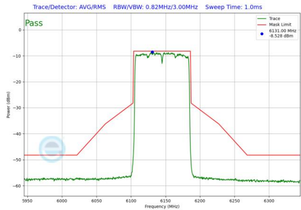
Plot 7-1524. LPI In-Band Emission Plot SDM Antenna 3b (80MHz 802.11ax RU996 (UNII Band 5) – Ch. 39)
