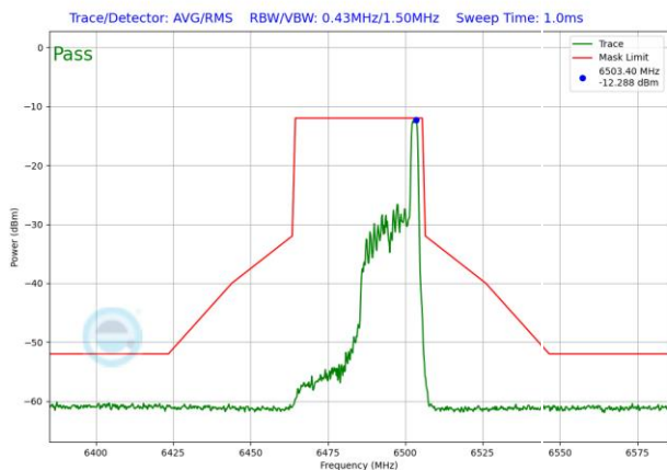
Plot 7-1545. LPI In-Band Emission Plot SDM Antenna WF5T (40MHz 802.11ax RU26 (UNII Band 6) – Ch. 107)
