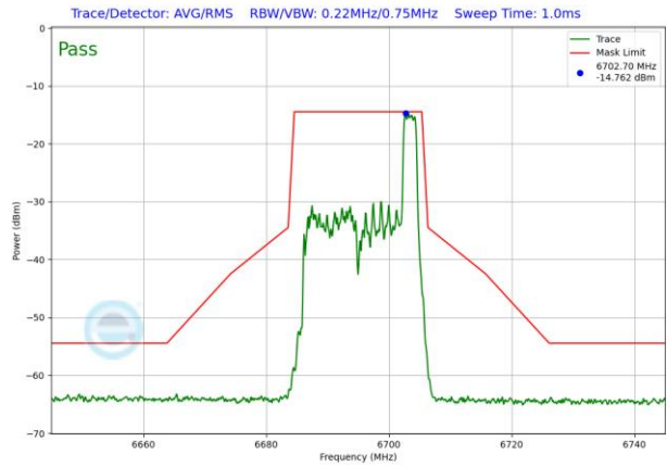
Plot 7-1570. LPI In-Band Emission Plot SDM Antenna 3b (20MHz 802.11ax RU26 (UNII Band 7) – Ch. 149)
