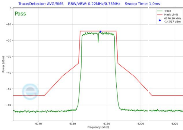
Plot 7-1507. LPI In-Band Emission Plot SDM Antenna WF5T (20MHz 802.11ax RU242 (UNII Band 5) – Ch. 45)
