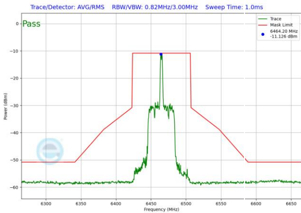
Plot 7-1551. LPI In-Band Emission Plot SDM Antenna WF5T (80MHz 802.11ax RU26 (UNII Band 6) – Ch. 103)
