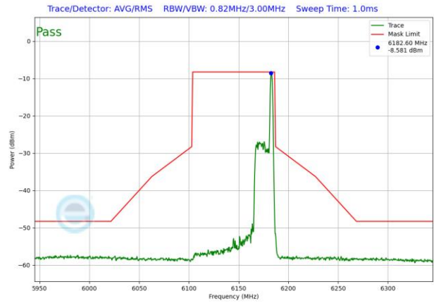
Plot 7-1522. LPI In-Band Emission Plot SDM Antenna 3b (80MHz 802.11ax RU26 (UNII Band 5) – Ch. 39)
