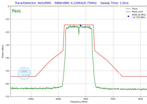
Plot 7-1603. LPI In-Band Emission Plot SDM Antenna WF5T (20MHz 802.11ax RU242 (UNII Band 8) – Ch. 209)
