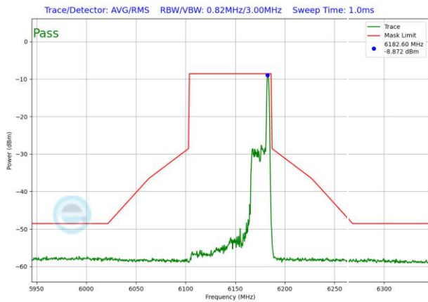
Plot 7-1521. LPI In-Band Emission Plot SDM Antenna WF5T (80MHz 802.11ax RU26 (UNII Band 5) – Ch. 39)
