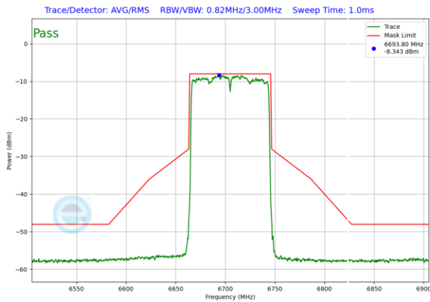
Plot 7-1587. LPI In-Band Emission Plot SDM Antenna WF5T (80MHz 802.11ax RU996 (UNII Band 7) – Ch. 151)
