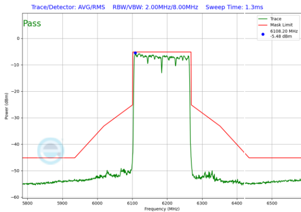
Plot 7-1532. LPI In-Band Emission Plot SDM Antenna 3b (160MHz 802.11ax RU996x2 (UNII Band 5) – Ch. 47)
