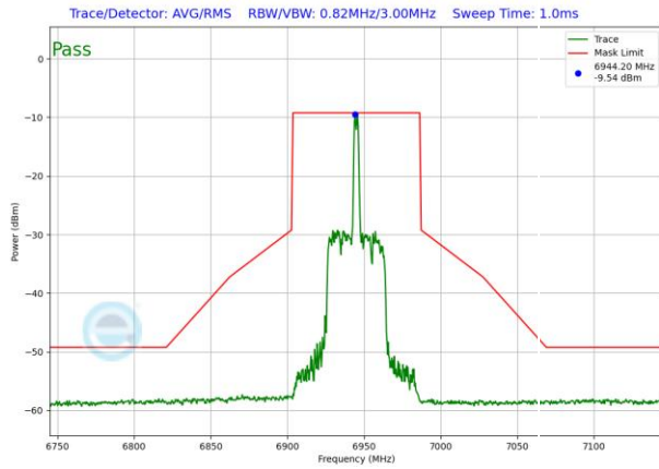
Plot 7-1615. LPI In-Band Emission Plot SDM Antenna WF5T (80MHz 802.11ax RU26 (UNII Band 8) – Ch. 199)
