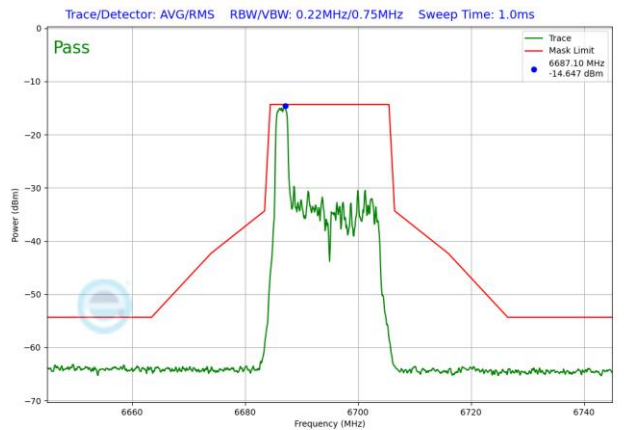
Plot 7-1565. LPI In-Band Emission Plot SDM Antenna WF5T (20MHz 802.11ax RU26 (UNII Band 7) – Ch. 149)
