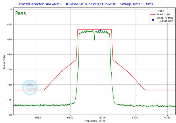
Plot 7-1572. LPI In-Band Emission Plot SDM Antenna 3b (20MHz 802.11ax RU242 (UNII Band 7) – Ch. 149)
