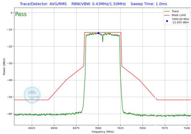
Plot 7-1611. LPI In-Band Emission Plot SDM Antenna WF5T (40MHz 802.11ax RU484 (UNII Band 8) – Ch. 211)
