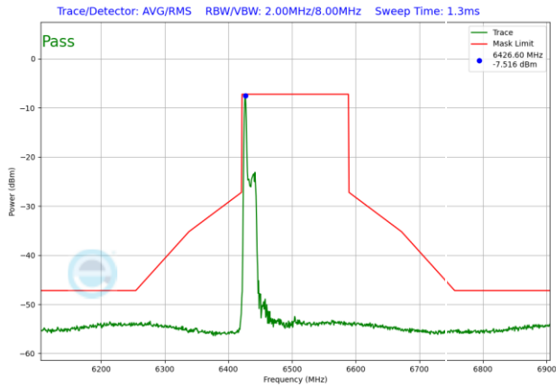
Plot 7-1557. LPI In-Band Emission Plot SDM Antenna WF5T (160MHz 802.11ax RU26 (UNII Band 6) – Ch. 111)
