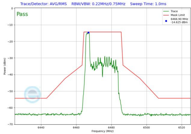
Plot 7-1534. LPI In-Band Emission Plot SDM Antenna 3b (20MHz 802.11ax RU26 (UNII Band 6) – Ch. 105)
