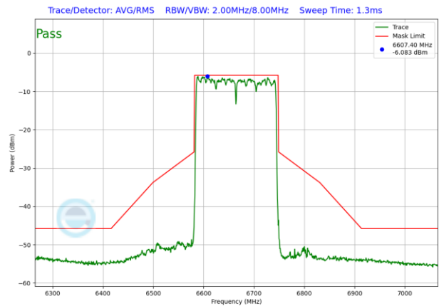
Plot 7-1595. LPI In-Band Emission Plot SDM Antenna WF5T (160MHz 802.11ax RU996x2 (UNII Band 7) – Ch. 143)
