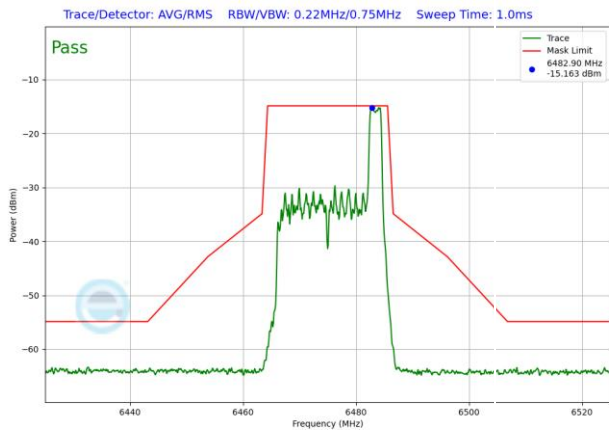
Plot 7-1538. LPI In-Band Emission Plot SDM Antenna 3b (20MHz 802.11ax RU26 (UNII Band 6) – Ch. 105)
