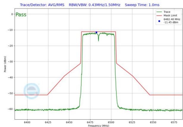
Plot 7-1548. LPI In-Band Emission Plot SDM Antenna 3b (40MHz 802.11ax RU484 (UNII Band 6) – Ch. 107)
