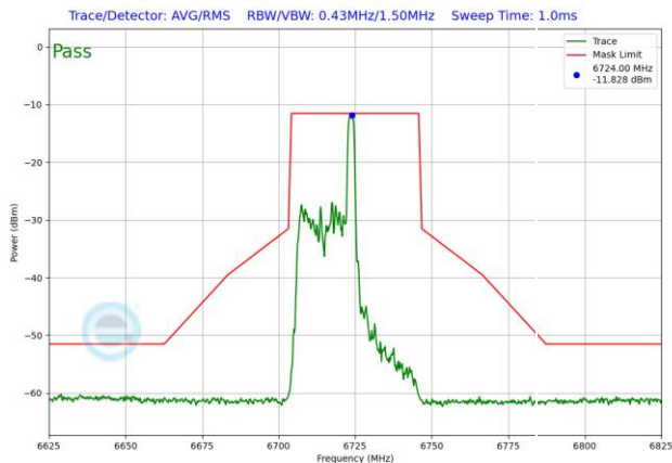
Plot 7-1575. LPI In-Band Emission Plot SDM Antenna WF5T (40MHz 802.11ax RU26 (UNII Band 7) – Ch. 155)
