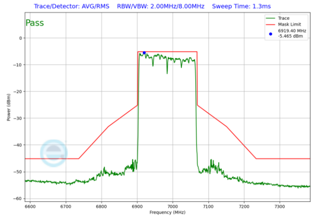
Plot 7-1628. LPI In-Band Emission Plot SDM Antenna 3b (160MHz 802.11ax RU996x2 (UNII Band 8) – Ch. 207)
