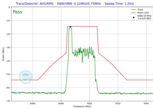
Plot 7-1598. LPI In-Band Emission Plot SDM Antenna 3b (20MHz 802.11ax RU26 (UNII Band 8) – Ch. 209)
