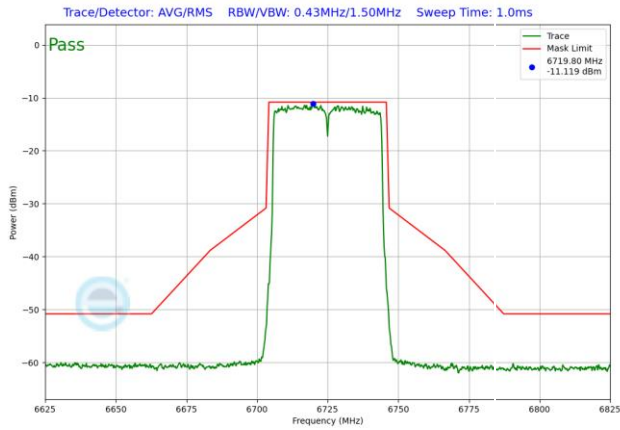
Plot 7-1579. LPI In-Band Emission Plot SDM Antenna WF5T (40MHz 802.11ax RU484 (UNII Band 7) – Ch. 155)
