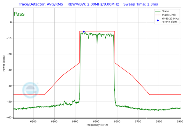
Plot 7-1563. LPI In-Band Emission Plot SDM Antenna WF5T (160MHz 802.11ax RU996x2 (UNII Band 6) – Ch. 111)
