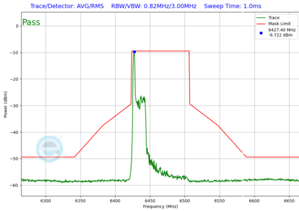
Plot 7-1549. LPI In-Band Emission Plot SDM Antenna WF5T (80MHz 802.11ax RU26 (UNII Band 6) – Ch. 103)
