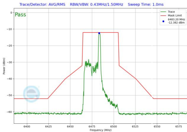
Plot 7-1544. LPI In-Band Emission Plot SDM Antenna 3b (40MHz 802.11ax RU26 (UNII Band 6) – Ch. 107)
