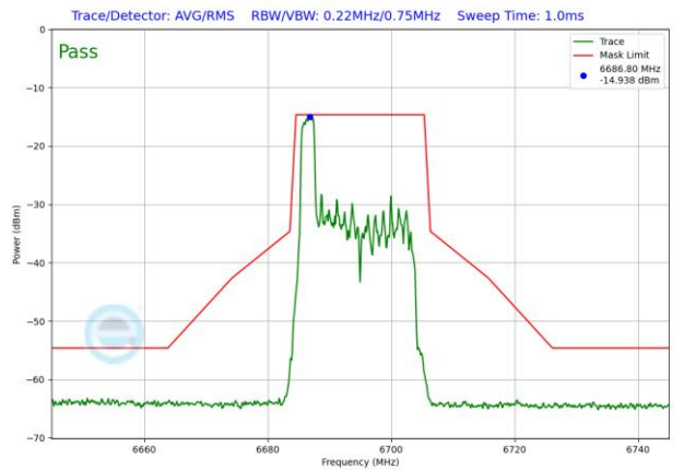
Plot 7-1566. LPI In-Band Emission Plot SDM Antenna 3b (20MHz 802.11ax RU26 (UNII Band 7) – Ch. 149)
