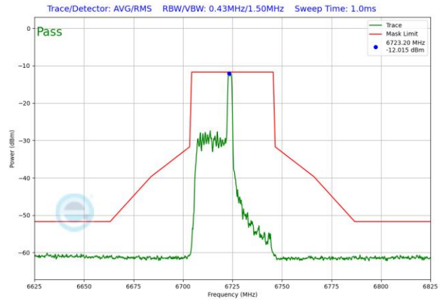
Plot 7-1576. LPI In-Band Emission Plot SDM Antenna 3b (40MHz 802.11ax RU26 (UNII Band 7) – Ch. 155)
