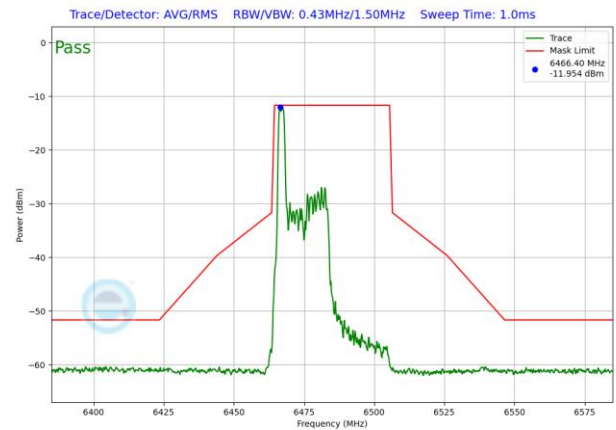
Plot 7-1541. LPI In-Band Emission Plot SDM Antenna WF5T (40MHz 802.11ax RU26 (UNII Band 6) – Ch. 107)
