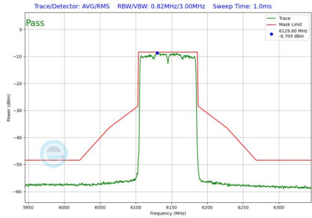
Plot 7-1640. LPI In-Band Emission Plot SDM Diversity Antenna 1b (80MHz 802.11ax RU996 (UNII Band 5) – Ch. 39)
