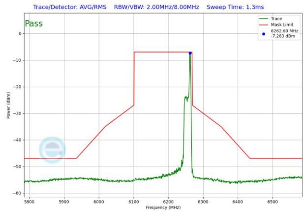
Plot 7-1530. LPI In-Band Emission Plot SDM Antenna 3b (160MHz 802.11ax RU26 (UNII Band 5) – Ch. 47)
