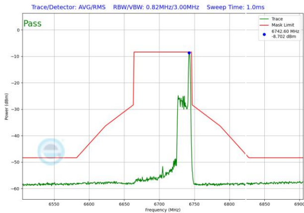
Plot 7-1586. LPI In-Band Emission Plot SDM Antenna 3b (80MHz 802.11ax RU26 (UNII Band 7) – Ch. 151)
