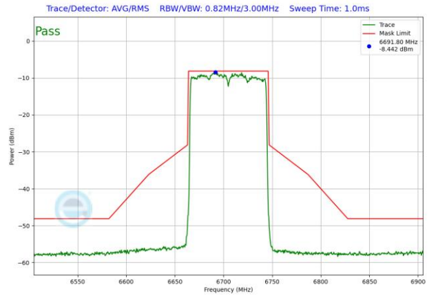
Plot 7-1588. LPI In-Band Emission Plot SDM Antenna 3b (80MHz 802.11ax RU996 (UNII Band 7) – Ch. 151)
