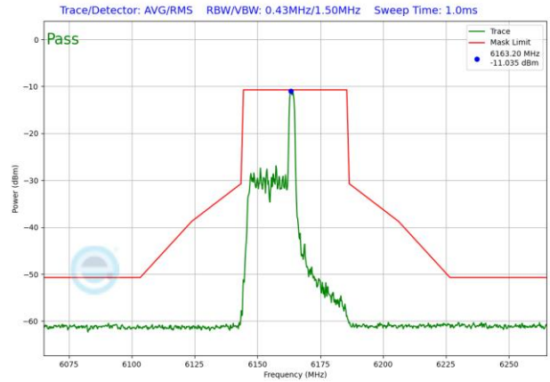
Plot 7-1511. LPI In-Band Emission Plot SDM Antenna WF5T (40MHz 802.11ax RU26 (UNII Band 5) – Ch. 43)
