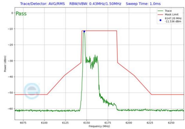
Plot 7-1510. LPI In-Band Emission Plot SDM Antenna 3b (40MHz 802.11ax RU26 (UNII Band 5) – Ch. 43)
