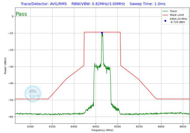
Plot 7-1552. LPI In-Band Emission Plot SDM Antenna 3b (80MHz 802.11ax RU26 (UNII Band 6) – Ch. 103)
