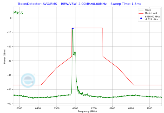
Plot 7-1589. LPI In-Band Emission Plot SDM Antenna WF5T (160MHz 802.11ax RU26 (UNII Band 7) – Ch. 143)
