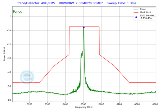
Plot 7-1560. LPI In-Band Emission Plot SDM Antenna 3b (160MHz 802.11ax RU26 (UNII Band 6) – Ch. 111)
