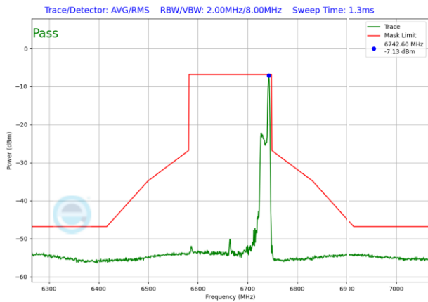
Plot 7-1593. LPI In-Band Emission Plot SDM Antenna WF5T (160MHz 802.11ax RU26 (UNII Band 7) – Ch. 143)
