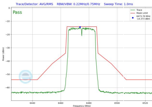
Plot 7-1539. LPI In-Band Emission Plot SDM Antenna WF5T (20MHz 802.11ax RU242 (UNII Band 6) – Ch. 105)
