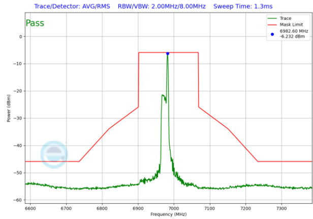
Plot 7-1624. LPI In-Band Emission Plot SDM Antenna 3b (160MHz 802.11ax RU26 (UNII Band 8) – Ch. 207)
