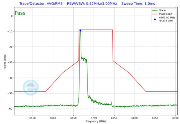
Plot 7-1582. LPI In-Band Emission Plot SDM Antenna 3b (80MHz 802.11ax RU26 (UNII Band 7) – Ch. 151)
