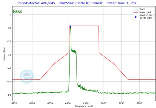
Plot 7-1614. LPI In-Band Emission Plot SDM Antenna 3b (80MHz 802.11ax RU26 (UNII Band 8) – Ch. 199)
