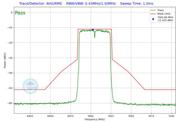
Plot 7-1612. LPI In-Band Emission Plot SDM Antenna 3b (40MHz 802.11ax RU484 (UNII Band 8) – Ch. 211)
