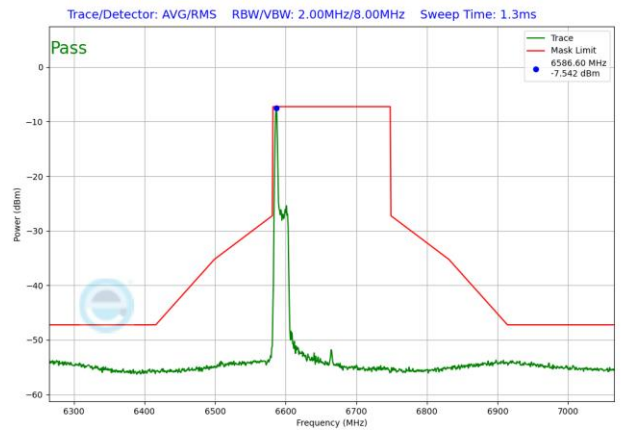
Plot 7-1590. LPI In-Band Emission Plot SDM Antenna 3b (160MHz 802.11ax RU26 (UNII Band 7) – Ch. 143)
