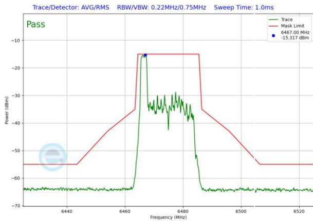
Plot 7-1533. LPI In-Band Emission Plot SDM Antenna WF5T (20MHz 802.11ax RU26 (UNII Band 6) – Ch. 105)
