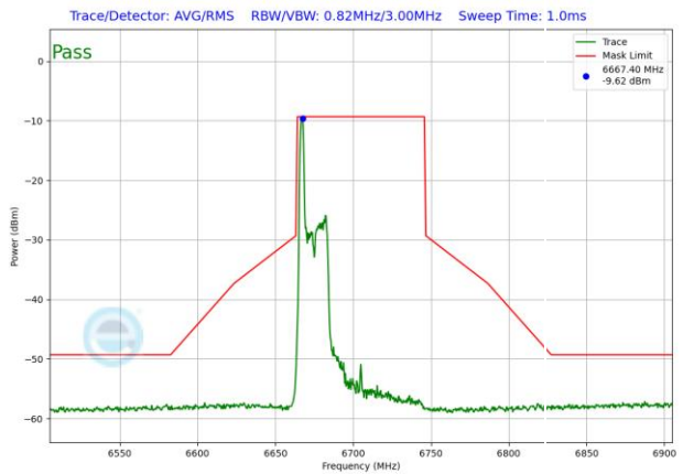
Plot 7-1581. LPI In-Band Emission Plot SDM Antenna WF5T (80MHz 802.11ax RU26 (UNII Band 7) – Ch. 151)
