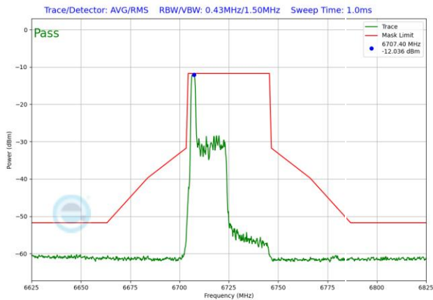
Plot 7-1574. LPI In-Band Emission Plot SDM Antenna 3b (40MHz 802.11ax RU26 (UNII Band 7) – Ch. 155)
