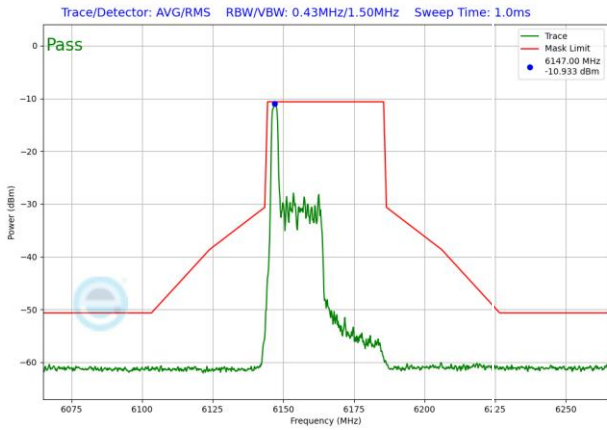
Plot 7-1509. LPI In-Band Emission Plot SDM Antenna WF5T (40MHz 802.11ax RU26 (UNII Band 5) – Ch. 43)
