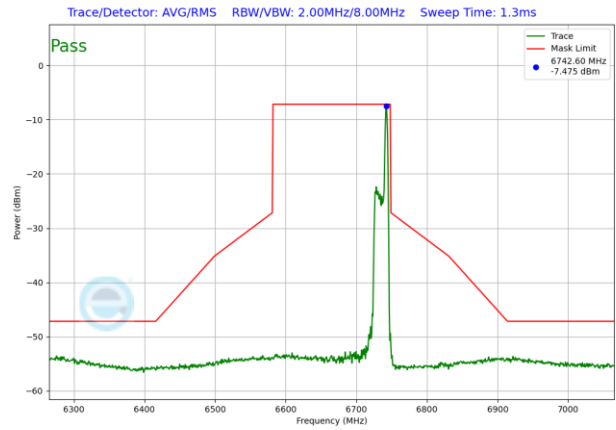
Plot 7-1594. LPI In-Band Emission Plot SDM Antenna 3b (160MHz 802.11ax RU26 (UNII Band 7) – Ch. 143)
