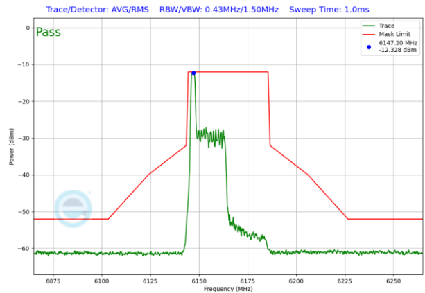
Plot 7-1633. LPI In-Band Emission Plot SDM Diversity Antenna 1b (40MHz 802.11ax RU26 (UNII Band 5) – Ch. 43)
