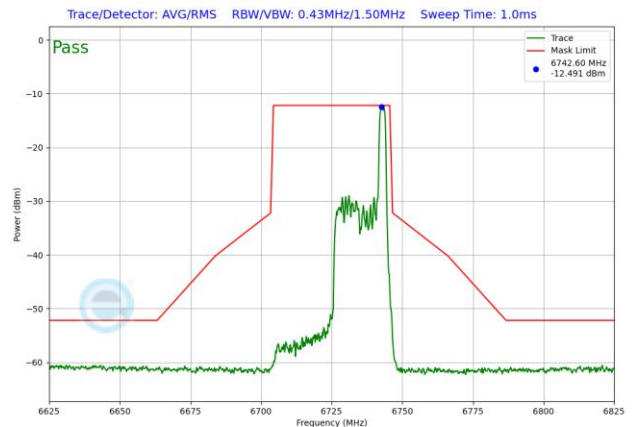
Plot 7-1578. LPI In-Band Emission Plot SDM Antenna 3b (40MHz 802.11ax RU26 (UNII Band 7) – Ch. 155)
