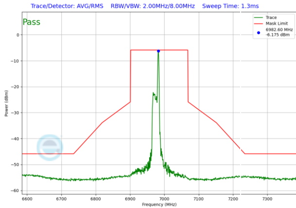
Plot 7-1623. LPI In-Band Emission Plot SDM Antenna WF5T (160MHz 802.11ax RU26 (UNII Band 8) – Ch. 207)
