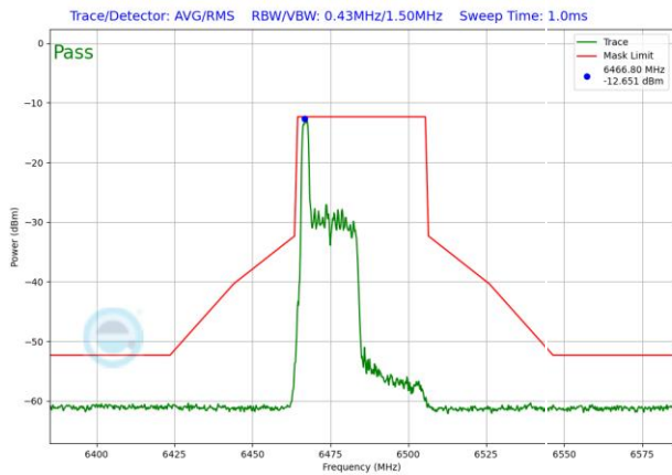
Plot 7-1649. LPI In-Band Emission Plot SDM Diversity Antenna 1b (40MHz 802.11ax RU26 (UNII Band 6) – Ch. 107)
