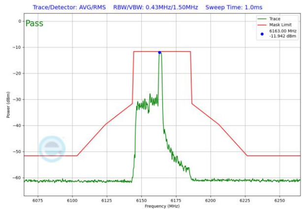
Plot 7-1634. LPI In-Band Emission Plot SDM Diversity Antenna 1b (40MHz 802.11ax RU26 (UNII Band 5) – Ch. 43)
