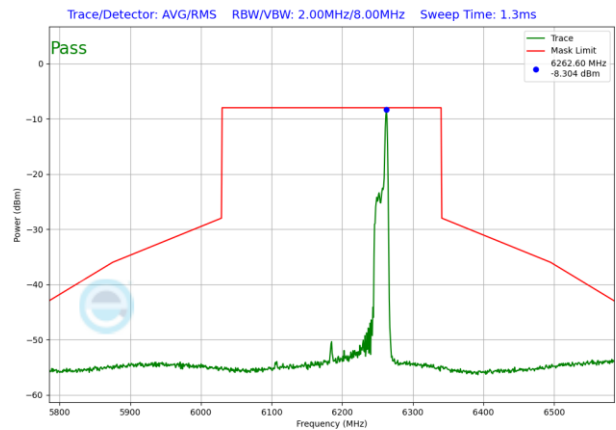
Plot 7-1529. LPI In-Band Emission Plot SDM Antenna WF5T (160MHz 802.11ax RU26 (UNII Band 5) – Ch. 47)
