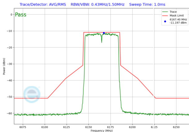
Plot 7-1515. LPI In-Band Emission Plot SDM Antenna WF5T (40MHz 802.11ax RU484 (UNII Band 5) – Ch. 43)
