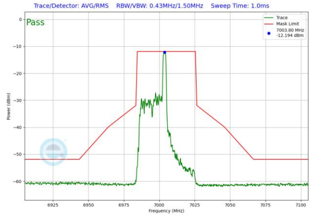
Plot 7-1607. LPI In-Band Emission Plot SDM Antenna WF5T (40MHz 802.11ax RU26 (UNII Band 8) – Ch. 211)
