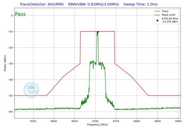
Plot 7-1583. LPI In-Band Emission Plot SDM Antenna WF5T (80MHz 802.11ax RU26 (UNII Band 7) – Ch. 151)
