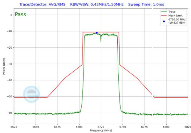
Plot 7-1580. LPI In-Band Emission Plot SDM Antenna 3b (40MHz 802.11ax RU484 (UNII Band 7) – Ch. 155)
