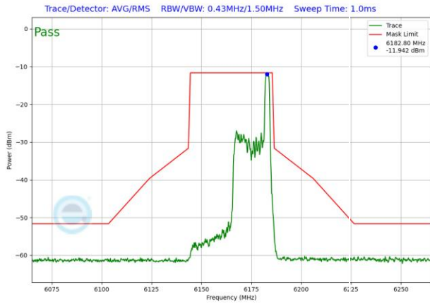
Plot 7-1635. LPI In-Band Emission Plot SDM Diversity Antenna 1b (40MHz 802.11ax RU26 (UNII Band 5) – Ch. 43)
