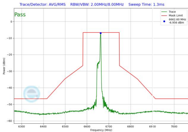
Plot 7-1592. LPI In-Band Emission Plot SDM Antenna 3b (160MHz 802.11ax RU26 (UNII Band 7) – Ch. 143)
