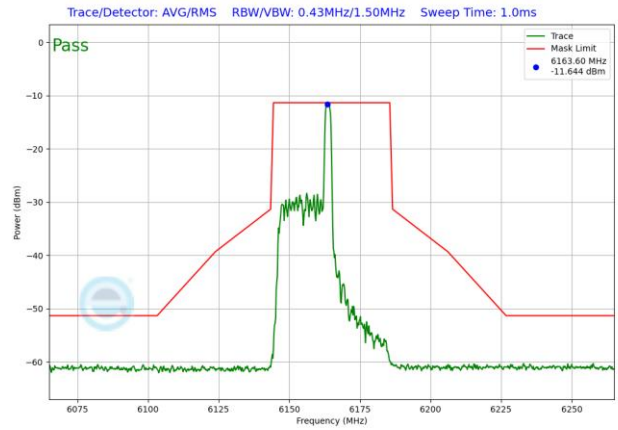
Plot 7-1512. LPI In-Band Emission Plot SDM Antenna 3b (40MHz 802.11ax RU26 (UNII Band 5) – Ch. 43)
