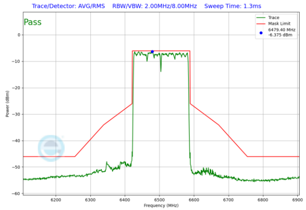
Plot 7-1564. LPI In-Band Emission Plot SDM Antenna 3b (160MHz 802.11ax RU996x2 (UNII Band 6) – Ch. 111)
