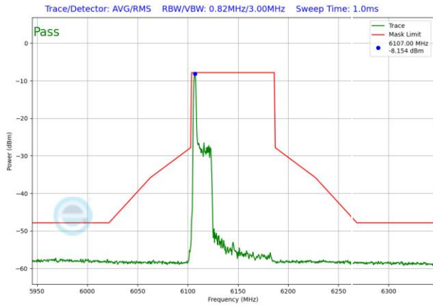
Plot 7-1637. LPI In-Band Emission Plot SDM Diversity Antenna 1b (80MHz 802.11ax RU26 (UNII Band 5) – Ch. 39)
