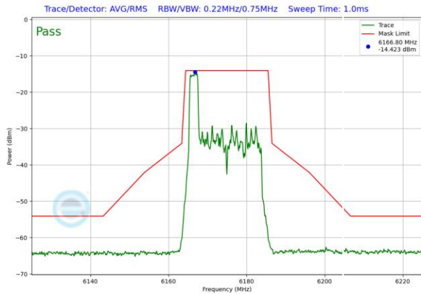
Plot 7-1629. LPI In-Band Emission Plot SDM Diversity Antenna 1b (20MHz 802.11ax RU26 (UNII Band 5) – Ch. 45)
