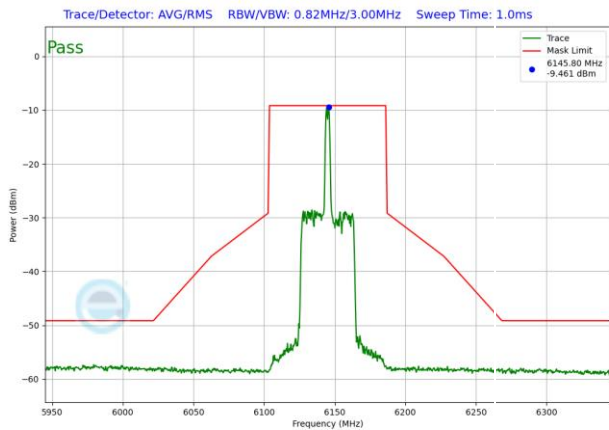
Plot 7-1520. LPI In-Band Emission Plot SDM Antenna 3b (80MHz 802.11ax RU26 (UNII Band 5) – Ch. 39)
