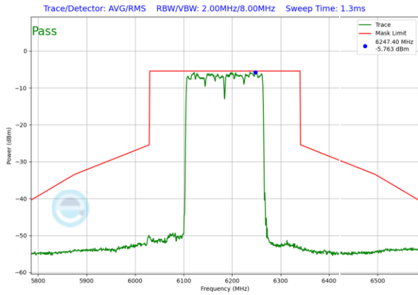
Plot 7-1531. LPI In-Band Emission Plot SDM Antenna WF5T (160MHz 802.11ax RU996x2 (UNII Band 5) – Ch. 47)
