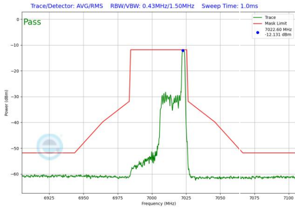
Plot 7-1609. LPI In-Band Emission Plot SDM Antenna WF5T (40MHz 802.11ax RU26 (UNII Band 8) – Ch. 211)
