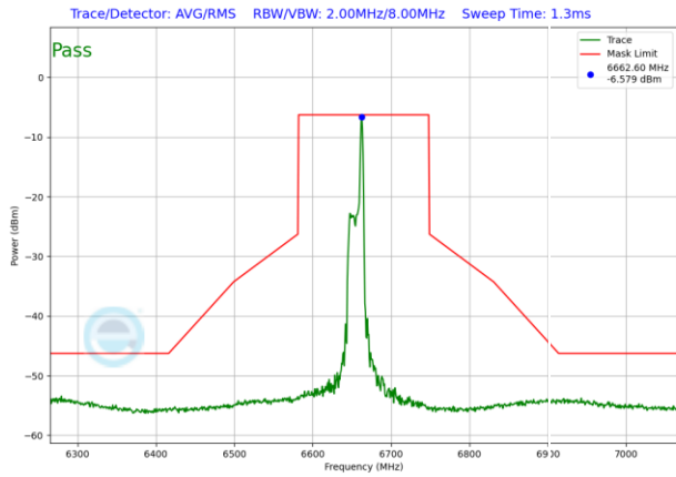
Plot 7-1591. LPI In-Band Emission Plot SDM Antenna WF5T (160MHz 802.11ax RU26 (UNII Band 7) – Ch. 143)
