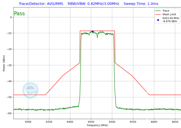
Plot 7-1555. LPI In-Band Emission Plot SDM Antenna WF5T (80MHz 802.11ax RU996 (UNII Band 6) – Ch. 103)
