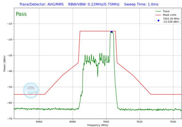
Plot 7-1601. LPI In-Band Emission Plot SDM Antenna WF5T (20MHz 802.11ax RU26 (UNII Band 8) – Ch. 209)
