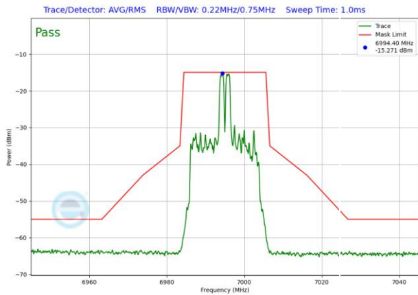
Plot 7-1599. LPI In-Band Emission Plot SDM Antenna WF5T (20MHz 802.11ax RU26 (UNII Band 8) – Ch. 209)
