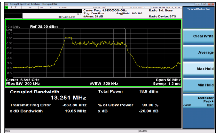
Plot 7-49. 26dB & 99% Bandwidth Plot Antenna 3b SP (20MHz 802.11ax RU26 (UNII Band 7) – Ch. 149)
