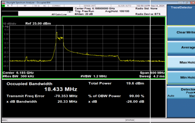
Plot 7-45. 26dB & 99% Bandwidth Plot Antenna 3b SP (160MHz 802.11ax RU26 (UNII Band 5) – Ch. 47)
