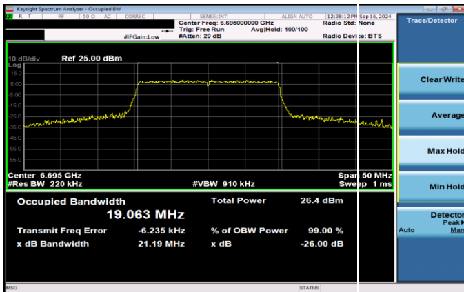
Plot 7-20. 26dB & 99% Bandwidth Plot Antenna 5T SP (20MHz 802.11ax RU242 (UNII Band 7) – Ch. 149)
