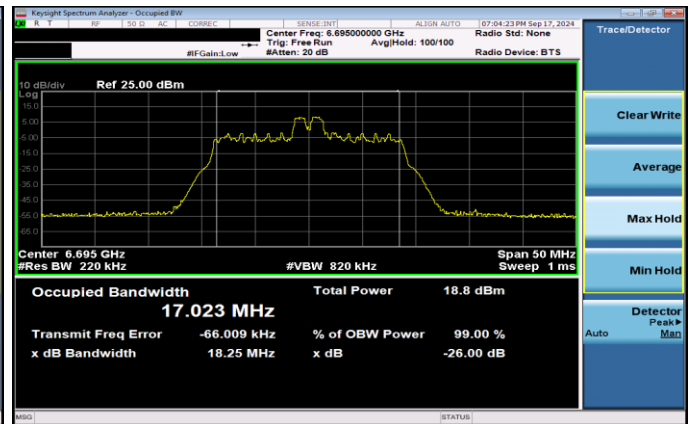
Plot 7-18. 26dB & 99% Bandwidth Plot Antenna 5T SP (20MHz 802.11ax RU26 (UNII Band 7) – Ch. 149)
