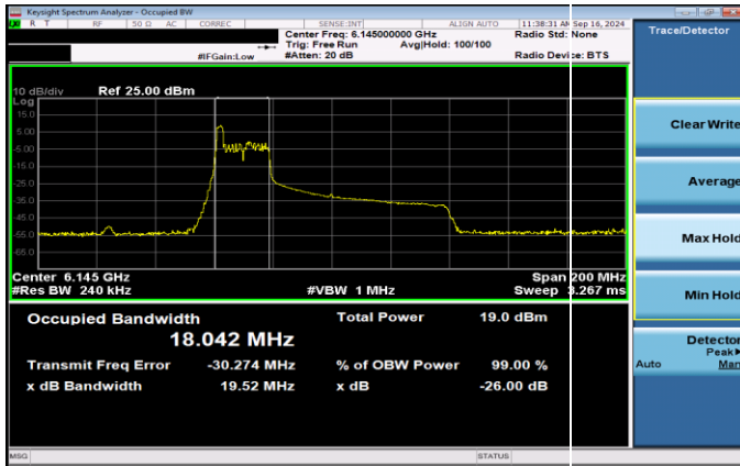
Plot 7-9. 26dB & 99% Bandwidth Plot Antenna 5T SP (80MHz 802.11ax RU26 (UNII Band 5) – Ch. 39)
