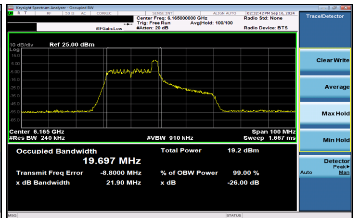
Plot 7-38. 26dB & 99% Bandwidth Plot Antenna 3b SP (40MHz 802.11ax RU26 (UNII Band 5) – Ch. 43)
