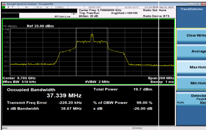
Plot 7-26. 26dB & 99% Bandwidth Plot Antenna 5T SP (80MHz 802.11ax RU26 (UNII Band 7) – Ch. 151)
