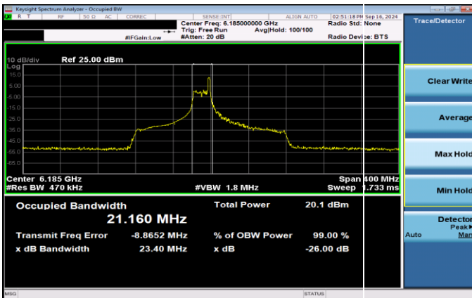
Plot 7-46. 26dB & 99% Bandwidth Plot Antenna 3b SP (160MHz 802.11ax RU26 (UNII Band 5) – Ch. 47)
