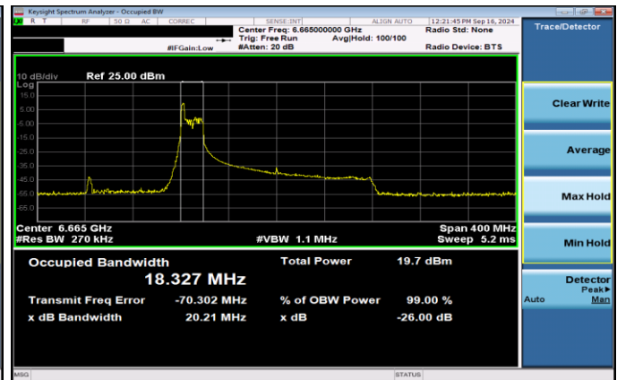
Plot 7-29. 26dB & 99% Bandwidth Plot Antenna 5T SP (160MHz 802.11ax RU26 (UNII Band 7) – Ch. 143)
