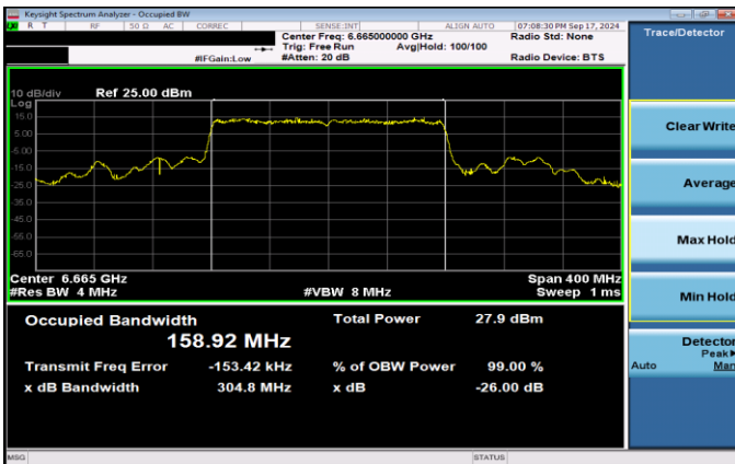
Plot 7-32. 26dB & 99% Bandwidth Plot Antenna 5T SP (160MHz 802.11ax RU996x2 (UNII Band 7) – Ch. 143)
