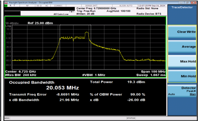
Plot 7-22. 26dB & 99% Bandwidth Plot Antenna 5T SP (40MHz 802.11ax RU26 (UNII Band 7) – Ch. 155)
