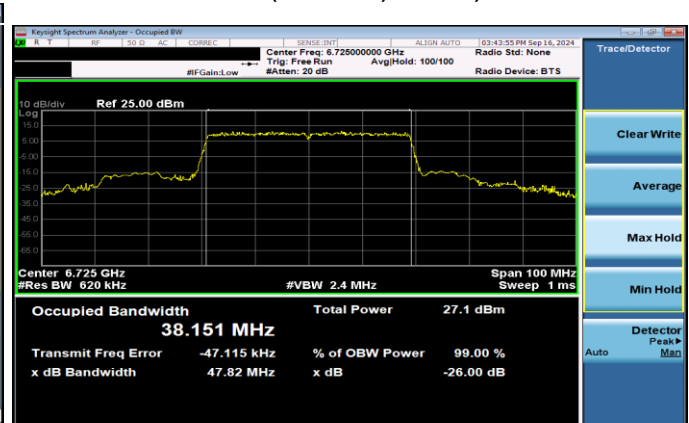
Plot 7-56. 26dB & 99% Bandwidth Plot Antenna 3b SP (40MHz 802.11ax RU484 (UNII Band 7) – Ch. 155)
