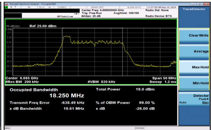
Plot 7-17. 26dB & 99% Bandwidth Plot Antenna 5T SP (20MHz 802.11ax RU26 (UNII Band 7) – Ch. 149)
