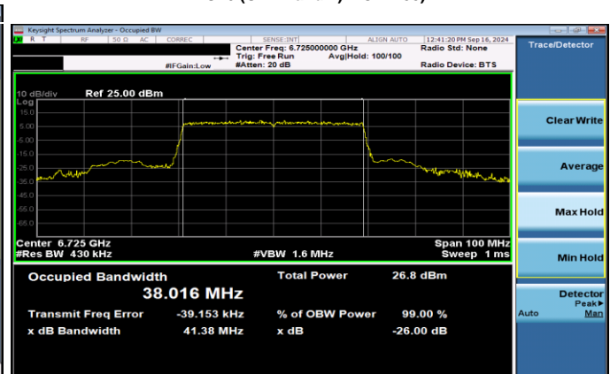
Plot 7-24. 26dB & 99% Bandwidth Plot Antenna 5T SP (40MHz 802.11ax RU484 (UNII Band 7) – Ch. 155)
