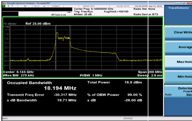
Plot 7-41. 26dB & 99% Bandwidth Plot Antenna 3b SP (80MHz 802.11ax RU26 (UNII Band 5) – Ch. 39)
