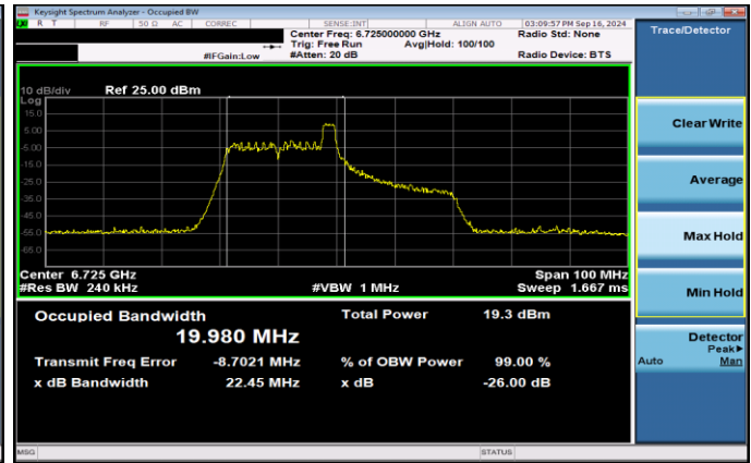
Plot 7-54. 26dB & 99% Bandwidth Plot Antenna 3b SP (40MHz 802.11ax RU26 (UNII Band 7) – Ch. 155)
