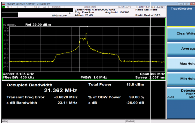
Plot 7-14. 26dB & 99% Bandwidth Plot Antenna 5T SP (160MHz 802.11ax RU26 (UNII Band 5) – Ch. 47)
