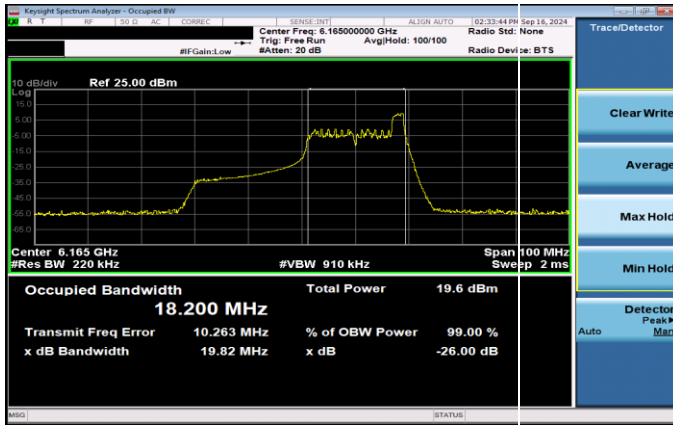
Plot 7-39. 26dB & 99% Bandwidth Plot Antenna 3b SP (40MHz 802.11ax RU26 (UNII Band 5) – Ch. 43)
