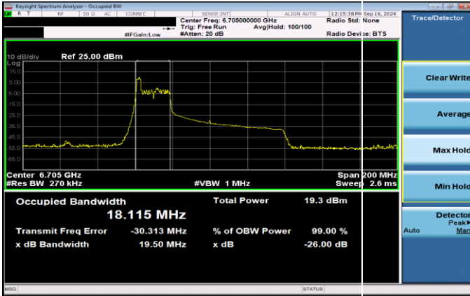
Plot 7-25. 26dB & 99% Bandwidth Plot Antenna 5T SP (80MHz 802.11ax RU26 (UNII Band 7) – Ch. 151)
