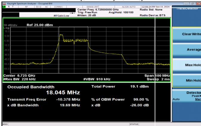
Plot 7-21. 26dB & 99% Bandwidth Plot Antenna 5T SP (40MHz 802.11ax RU26 (UNII Band 7) – Ch. 155)
