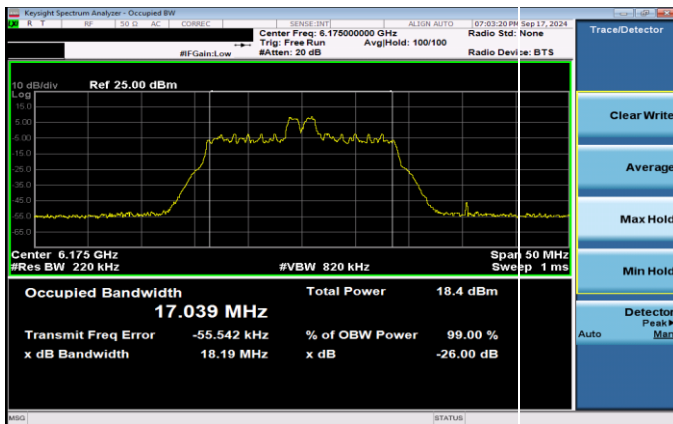
Plot 7-2. 26dB & 99% Bandwidth Plot Antenna 5T SP (20MHz 802.11ax RU26 (UNII Band 5) – Ch. 45)
