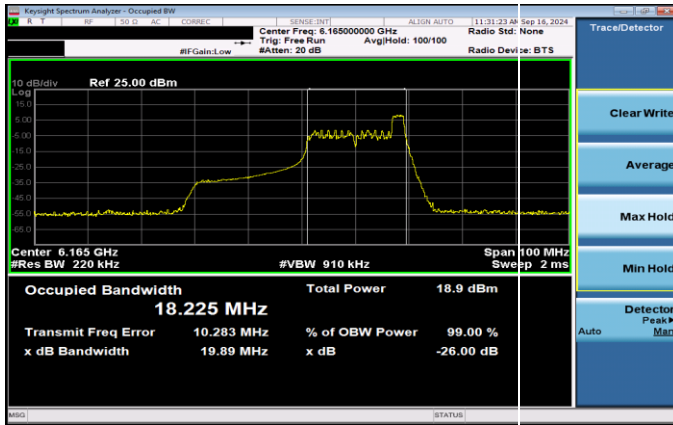
Plot 7-7. 26dB & 99% Bandwidth Plot Antenna 5T SP (40MHz 802.11ax RU26 (UNII Band 5) – Ch. 43)
