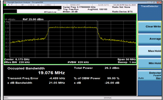
Plot 7-36. 26dB & 99% Bandwidth Plot Antenna 3b SP (20MHz 802.11ax RU242 (UNII Band 5) – Ch. 45)
