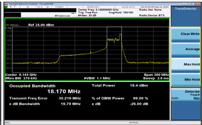
Plot 7-43. 26dB & 99% Bandwidth Plot Antenna 3b SP (80MHz 802.11ax RU26 (UNII Band 5) – Ch. 39)
