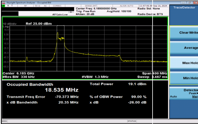
Plot 7-13. 26dB & 99% Bandwidth Plot Antenna 5T SP (160MHz 802.11ax RU26 (UNII Band 5) – Ch. 47)
