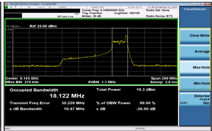
Plot 7-11. 26dB & 99% Bandwidth Plot Antenna 5T SP (80MHz 802.11ax RU26 (UNII Band 5) – Ch. 39)
