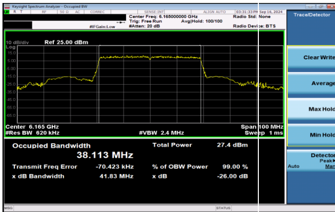
Plot 7-40. 26dB & 99% Bandwidth Plot Antenna 3b SP (40MHz 802.11ax RU484 (UNII Band 5) – Ch. 43)
