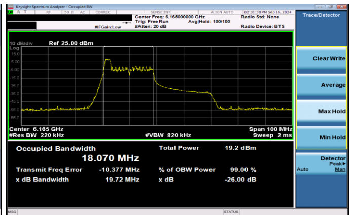
Plot 7-37. 26dB & 99% Bandwidth Plot Antenna 3b SP (40MHz 802.11ax RU26 (UNII Band 5) – Ch. 43)
