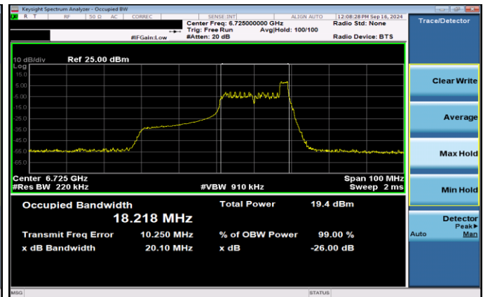
Plot 7-23. 26dB & 99% Bandwidth Plot Antenna 5T SP (40MHz 802.11ax RU26 (UNII Band 7) – Ch. 155)
