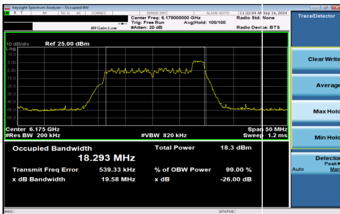
Plot 7-3. 26dB & 99% Bandwidth Plot Antenna 5T SP (20MHz 802.11ax RU26 (UNII Band 5) – Ch. 45)
