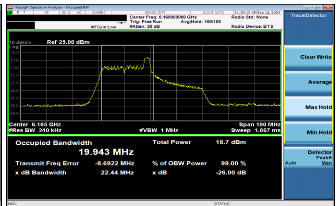
Plot 7-6. 26dB & 99% Bandwidth Plot Antenna 5T SP (40MHz 802.11ax RU26 (UNII Band 5) – Ch. 43)
