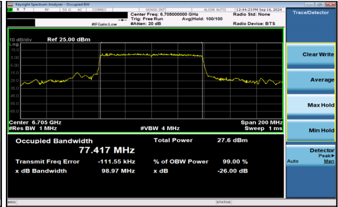
Plot 7-28. 26dB & 99% Bandwidth Plot Antenna 5T SP (80MHz 802.11ax RU996 (UNII Band 7) – Ch. 151)
