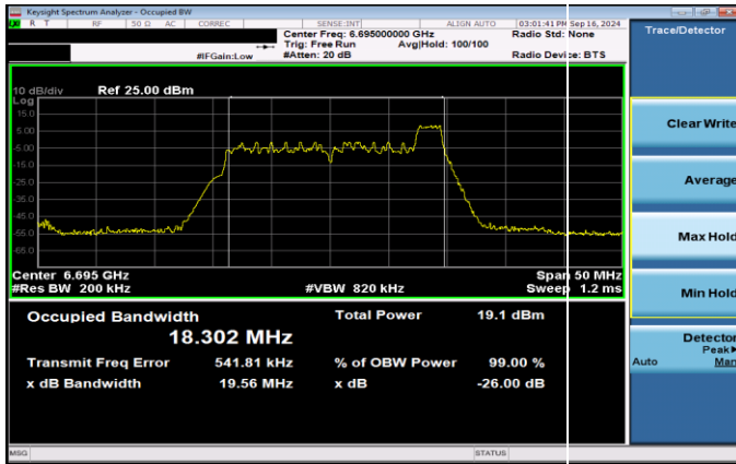
Plot 7-51. 26dB & 99% Bandwidth Plot Antenna 3b SP (20MHz 802.11ax RU26 (UNII Band 7) – Ch. 149)
