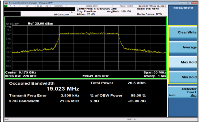
Plot 7-4. 26dB & 99% Bandwidth Plot Antenna 5T SP (20MHz 802.11ax RU242 (UNII Band 5) – Ch. 45)
