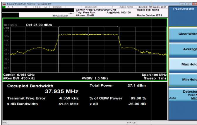
Plot 7-8. 26dB & 99% Bandwidth Plot Antenna 5T SP (40MHz 802.11ax RU484 (UNII Band 5) – Ch. 43)
