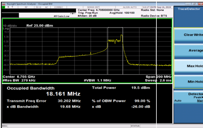
Plot 7-27. 26dB & 99% Bandwidth Plot Antenna 5T SP (80MHz 802.11ax RU26 (UNII Band 7) – Ch. 151)
