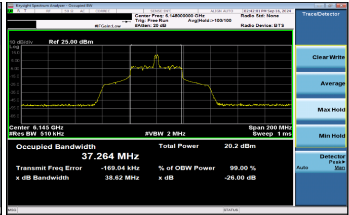
Plot 7-42. 26dB & 99% Bandwidth Plot Antenna 3b SP (80MHz 802.11ax RU26 (UNII Band 5) – Ch. 39)
