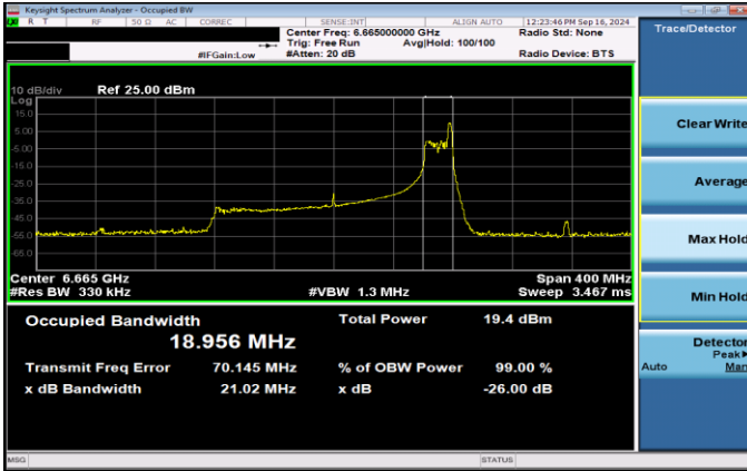
Plot 7-31. 26dB & 99% Bandwidth Plot Antenna 5T SP (160MHz 802.11ax RU26 (UNII Band 7) – Ch. 143)
