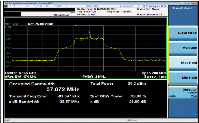
Plot 7-10. 26dB & 99% Bandwidth Plot Antenna 5T SP (80MHz 802.11ax RU26 (UNII Band 5) – Ch. 39)
