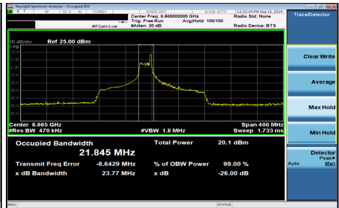
Plot 7-30. 26dB & 99% Bandwidth Plot Antenna 5T SP (160MHz 802.11ax RU26 (UNII Band 7) – Ch. 143)
