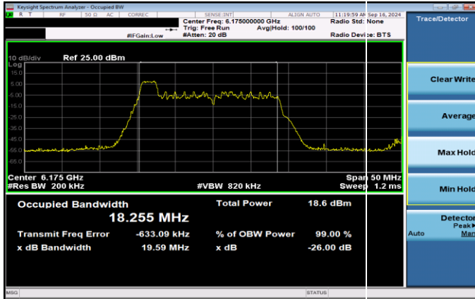
Plot 7-1. 26dB & 99% Bandwidth Plot Antenna 5T SP (20MHz 802.11ax RU26 (UNII Band 5) – Ch. 45)
