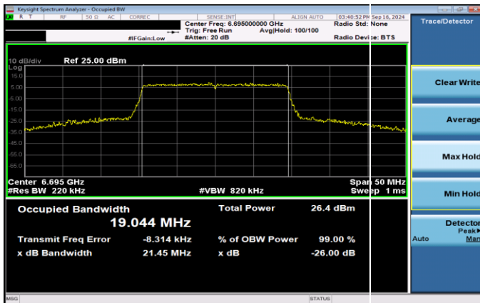
Plot 7-52. 26dB & 99% Bandwidth Plot Antenna 3b SP (20MHz 802.11ax RU242 (UNII Band 7) – Ch. 149)
