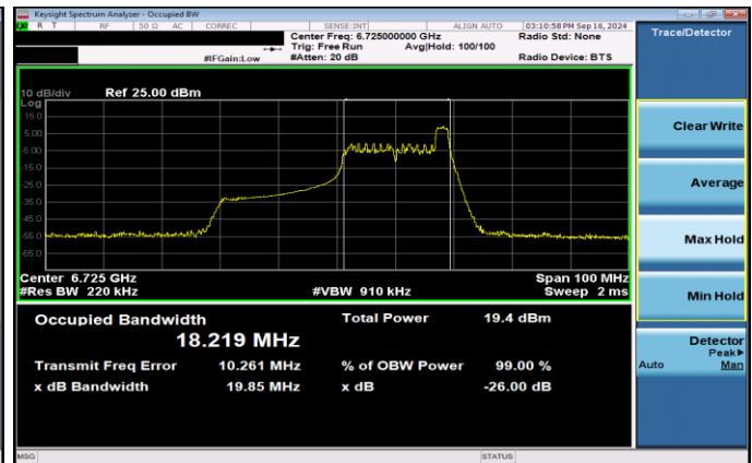
Plot 7-55. 26dB & 99% Bandwidth Plot Antenna 3b SP (40MHz 802.11ax RU26 (UNII Band 7) – Ch. 155)
