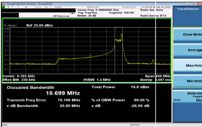
Plot 7-15. 26dB & 99% Bandwidth Plot Antenna 5T SP (160MHz 802.11ax RU26 (UNII Band 5) – Ch. 47)
