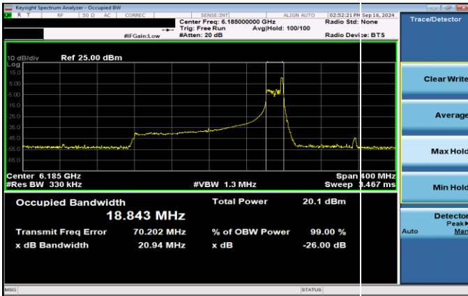
Plot 7-47. 26dB & 99% Bandwidth Plot Antenna 3b SP (160MHz 802.11ax RU26 (UNII Band 5) – Ch. 47)
