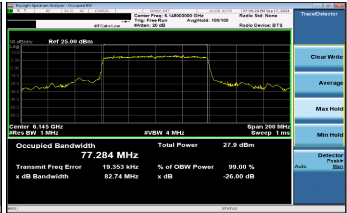
Plot 7-12. 26dB & 99% Bandwidth Plot Antenna 5T SP (80MHz 802.11ax RU996 (UNII Band 5) – Ch. 39)
