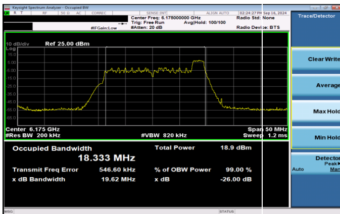
Plot 7-35. 26dB & 99% Bandwidth Plot Antenna 3b SP (20MHz 802.11ax RU26 (UNII Band 5) – Ch. 45)
