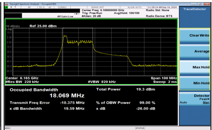
Plot 7-5. 26dB & 99% Bandwidth Plot Antenna 5T SP (40MHz 802.11ax RU26 (UNII Band 5) – Ch. 43)
