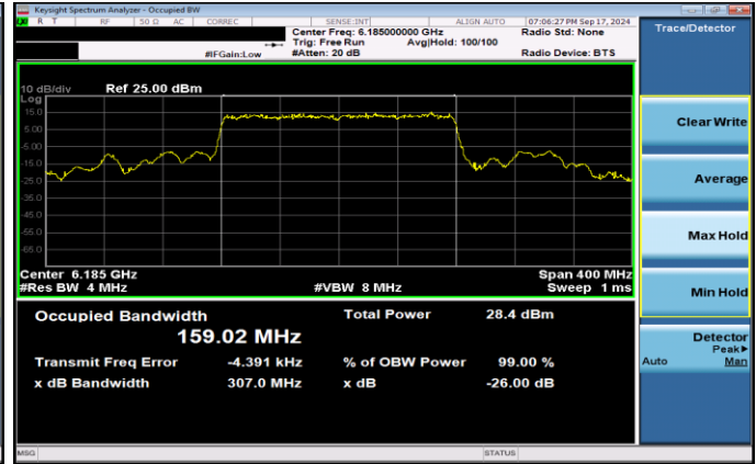
Plot 7-16. 26dB & 99% Bandwidth Plot Antenna 5T SP (160MHz 802.11ax RU996x2 (UNII Band 5) – Ch. 47)
