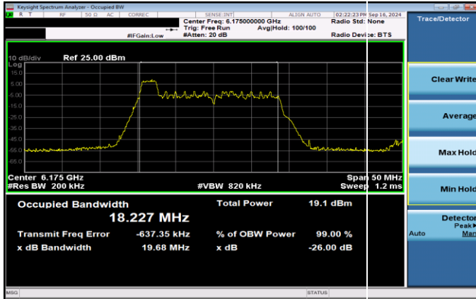
Plot 7-33. 26dB & 99% Bandwidth Plot Antenna 3b SP (20MHz 802.11ax RU26 (UNII Band 5) – Ch. 45)
