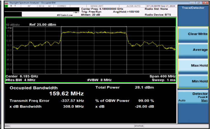
Plot 7-48. 26dB & 99% Bandwidth Plot Antenna 3b SP (160MHz 802.11ax RU996x2 (UNII Band 5) – Ch. 47)
