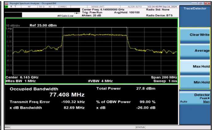
Plot 7-44. 26dB & 99% Bandwidth Plot Antenna 3b SP (80MHz 802.11ax RU996 (UNII Band 5) – Ch. 39)
