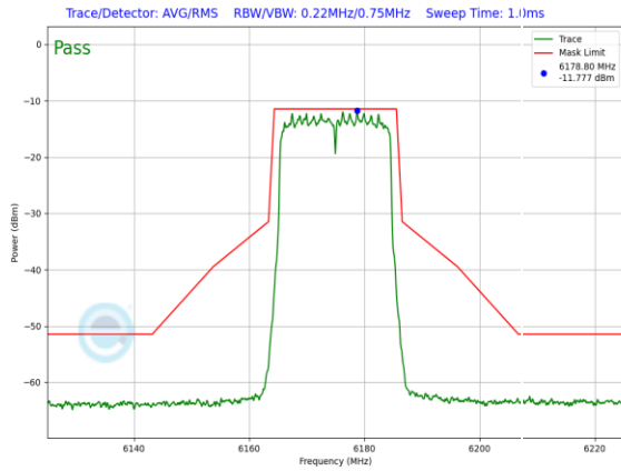
Plot 7-338. LPI In-Band Emission Plot Antenna 5T LPI (20MHz 802.11ax (UNII Band 5) – Ch. 45, MCS11)
