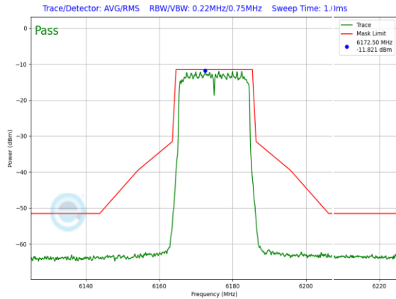
Plot 7-378. In-Band Emission Plot Antenna 3b LPI (20MHz) 802.11ax (UNII Band 5) – Ch. 45, MCS11)
