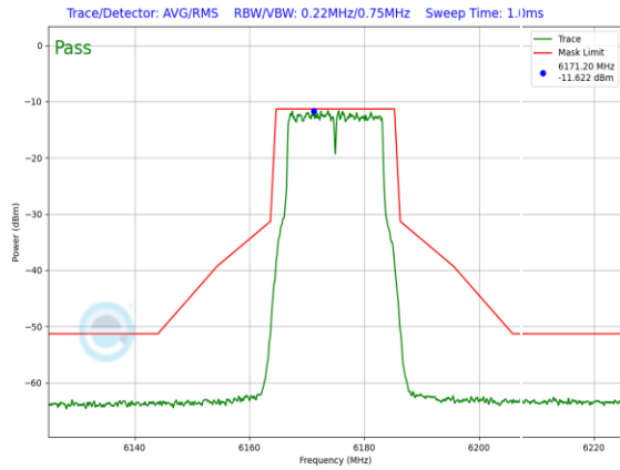
Plot 7-377. In-Band Emission Plot Antenna 3b LPI (20MHz) 802.11a (UNII Band 5) – Ch. 45, 54Mbps)
