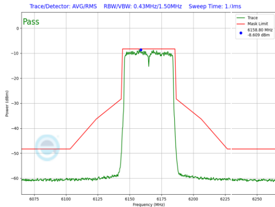
Plot 7-379. In-Band Emission Plot Antenna 3b LPI (40MHz) 802.11ax (UNII Band 5) – Ch. 43, MCS11)
