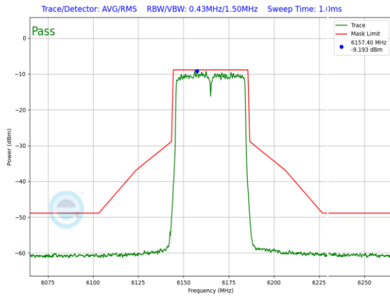
Plot 7-339. LPI In-Band Emission Plot Antenna 5T LPI (40MHz 802.11ax (UNII Band 5) – Ch. 43, MCS11)
