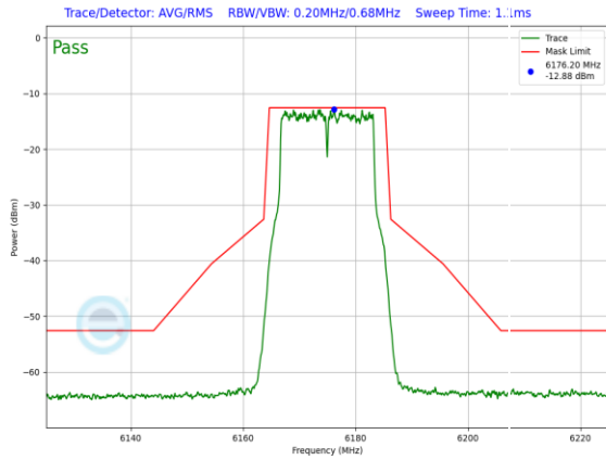
Plot 7-337. LPI In-Band Emission Plot Antenna 5T LPI (20MHz 802.11a (UNII Band 5) – Ch. 45, 54Mbps)
