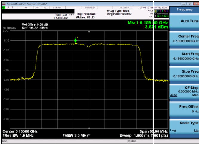
Plot 7-322. Power Spectral Density Plot CDD Antenna 1b SP (40MHz) 802.11ax (UNII Band 5) – Ch. 43, MCS11)
