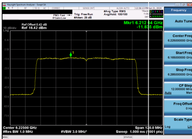
Plot 7-331. Power Spectral Density Plot CDD Antenna 1b VLP (80MHz 802.11ax (UNII Band 5) – Ch. 55, MCS11)
