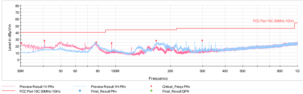
Plot 7-3. Radiated Spurious Emissions 30MHz – 1GHz (Charging Rate 2.6C, with AC/DC Adapter)
