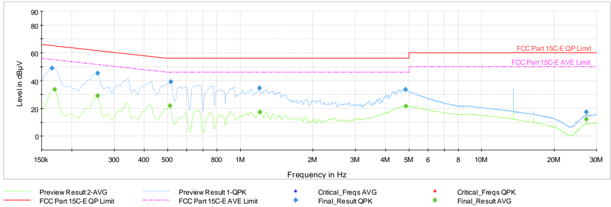
Plot 7-4. AC Line-Conducted Plot (L1, Charging Rate 2.6C, with AC/DC Adapter)
