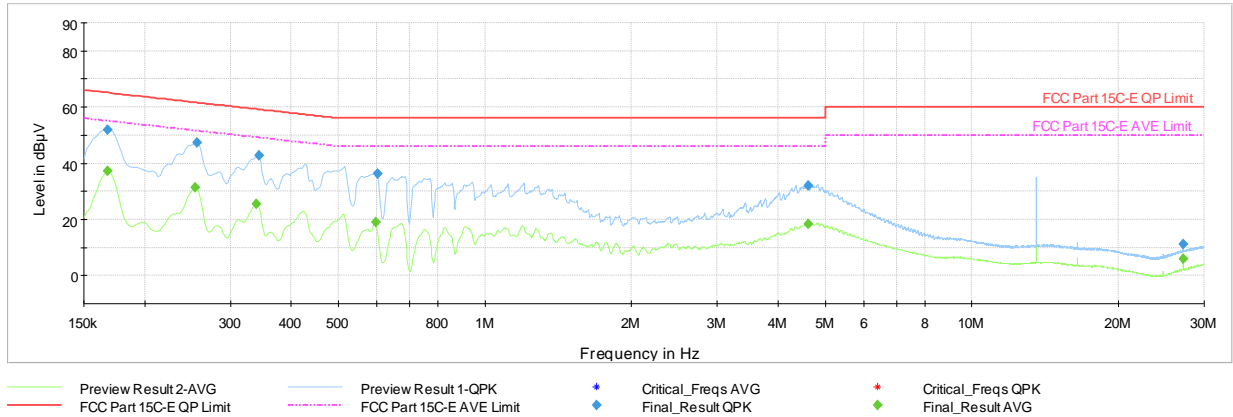
Plot 7-5. AC Line-Conducted Plot (N, Charging Rate 2.6C, with AC/DC Adapter)
