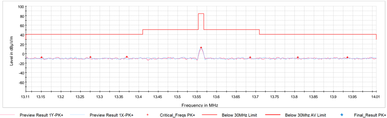
Plot 7-1. In Band Radiated Spurious Emissions (Charging Rate 2.6C, with AC/DC Adapter)
