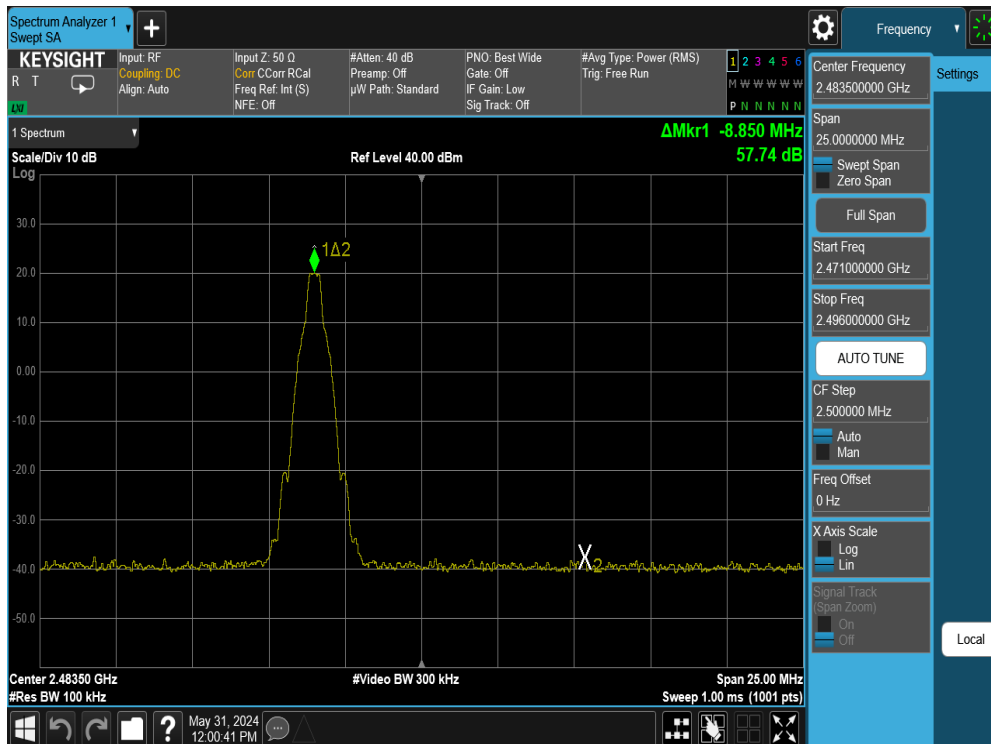
Plot 7-28. Band Edge Plot Antenna 1a (Bluetooth with Hopping Disabled, GFSK, ePA – Ch. 78)
