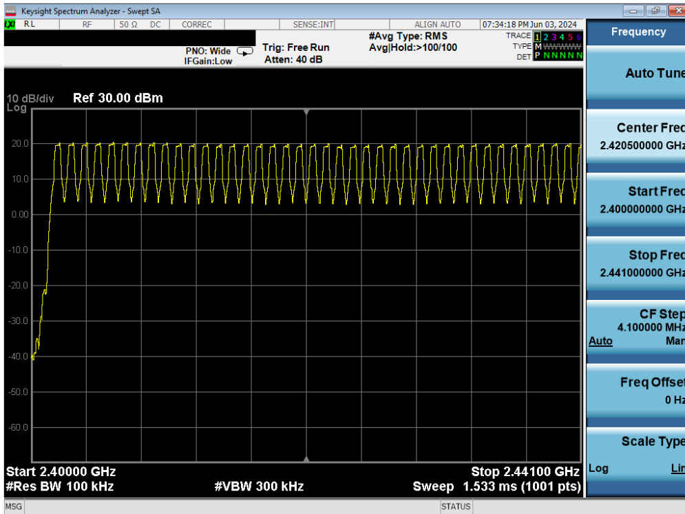
Plot 7-55. Low End Spectrum Channel Hopping Plot Antenna 3a (Bluetooth, GFSK, ePA)
