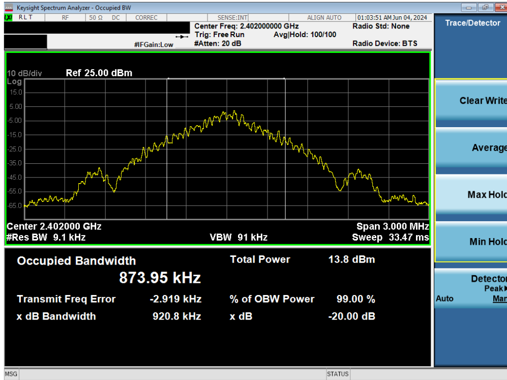
Plot 7-13. 20dB BW and 99% OBW Plot Antenna 4 (Bluetooth, GFSK, iPA – Ch. 0)
