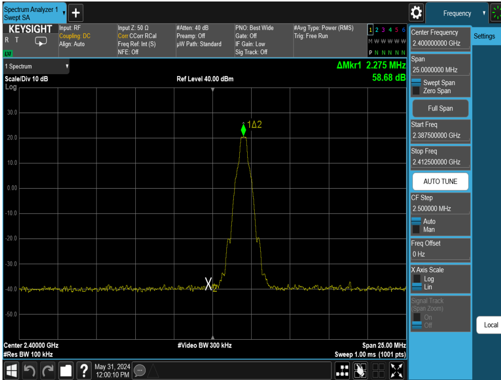
Plot 7-27. Band Edge Plot Antenna 1a (Bluetooth with Hopping Disabled, GFSK, ePA – Ch. 0)
