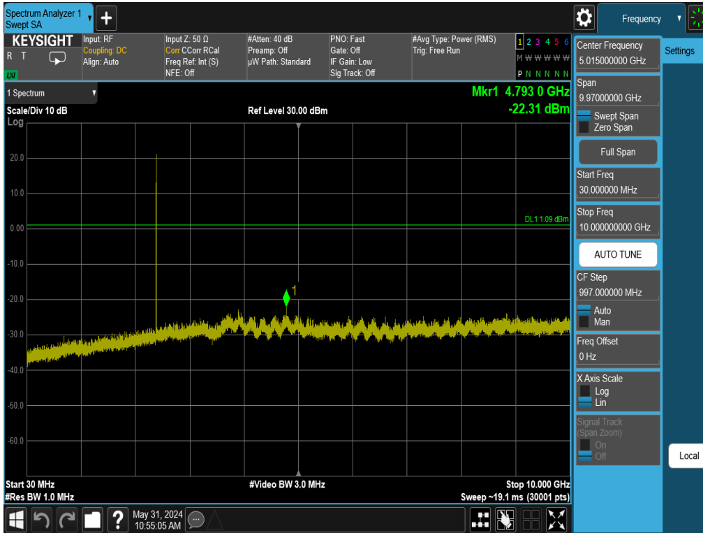
Plot 7-67. Conducted Spurious Plot Antenna 3a (Bluetooth, GFSK, ePA – Ch. 0)
