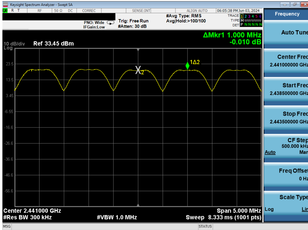
Plot 7-43. Channel Spacing Plot Antenna 3a (Bluetooth, GFSK, ePA)
