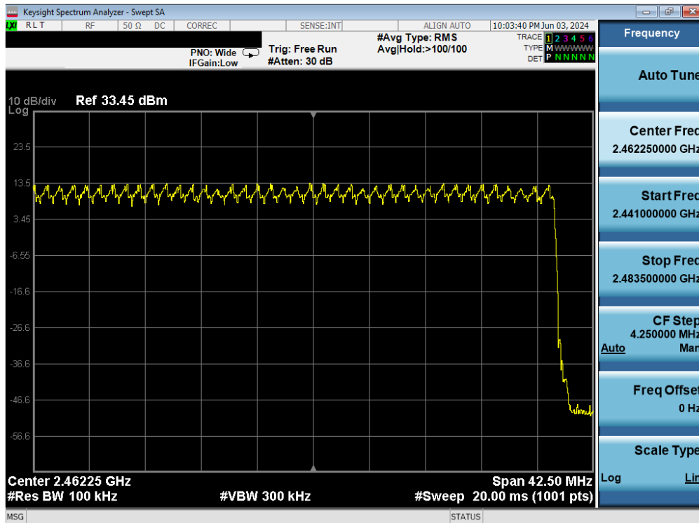
Plot 7-62. High End Spectrum Channel Hopping Plot Antenna 1a (Bluetooth, 8DPSK, ePA)
