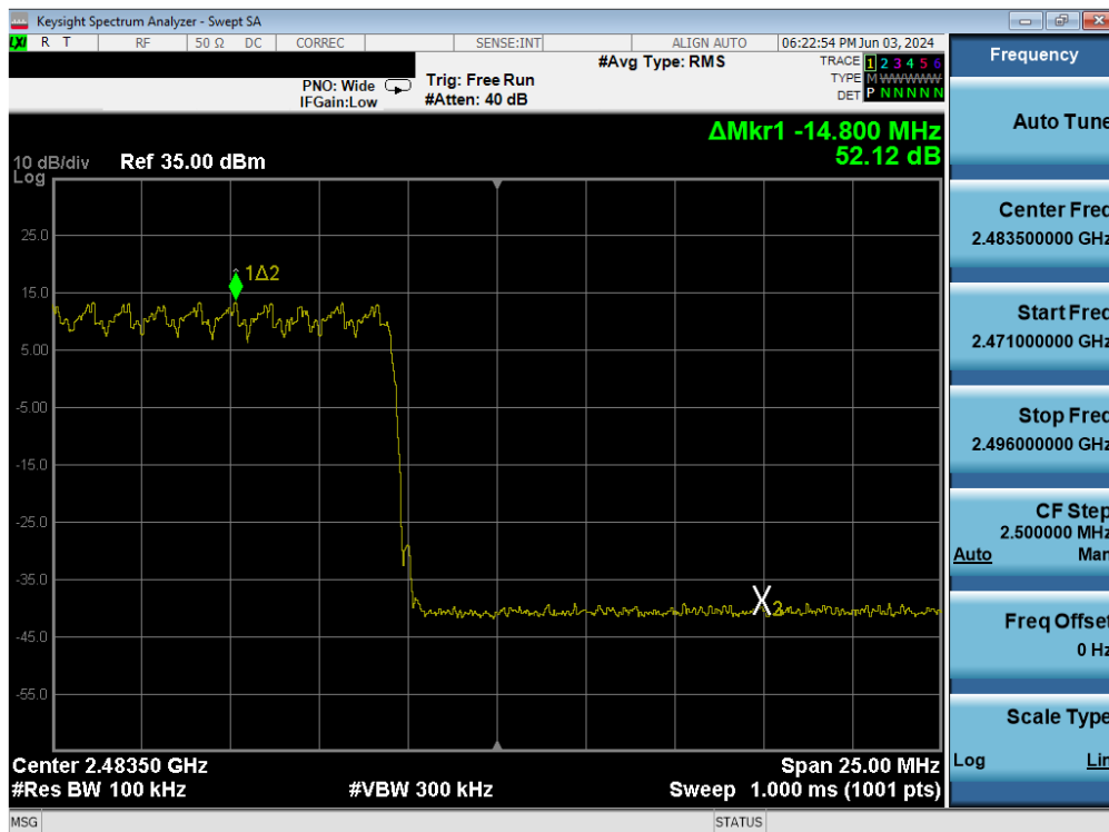
Plot 7-26. Band Edge Plot Antenna 3a (Bluetooth with Hopping Enabled, 8DPSK, ePA)
