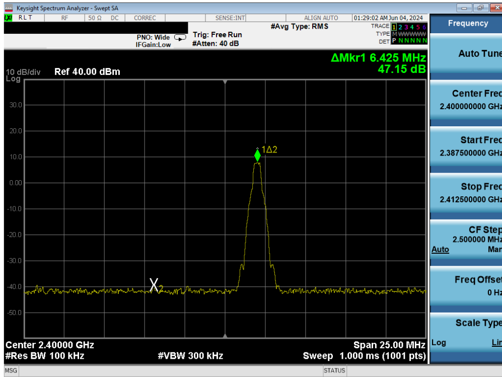
Plot 7-35. Band Edge Plot Antenna 4 (Bluetooth with Hopping Disabled, GFSK, iPA – Ch. 0)
