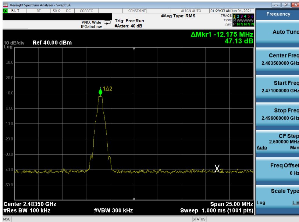
Plot 7-36. Band Edge Plot Antenna 4 (Bluetooth with Hopping Disabled, GFSK, iPA - Ch. 78)
