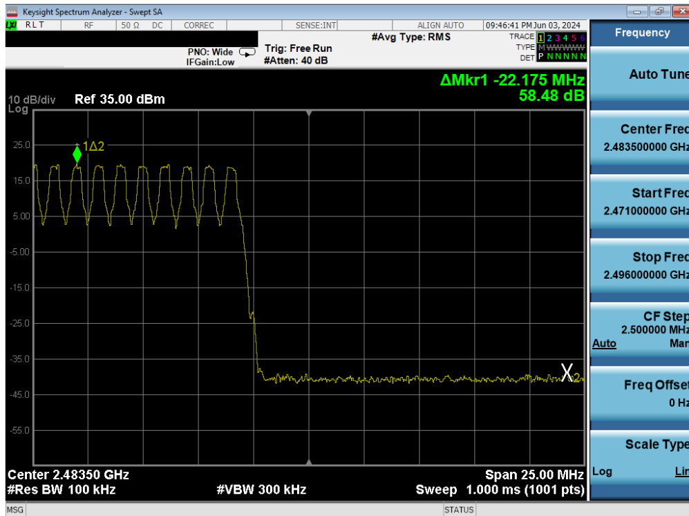
Plot 7-30. Band Edge Plot Antenna 1a (Bluetooth with Hopping Enabled, GFSK, ePA)
