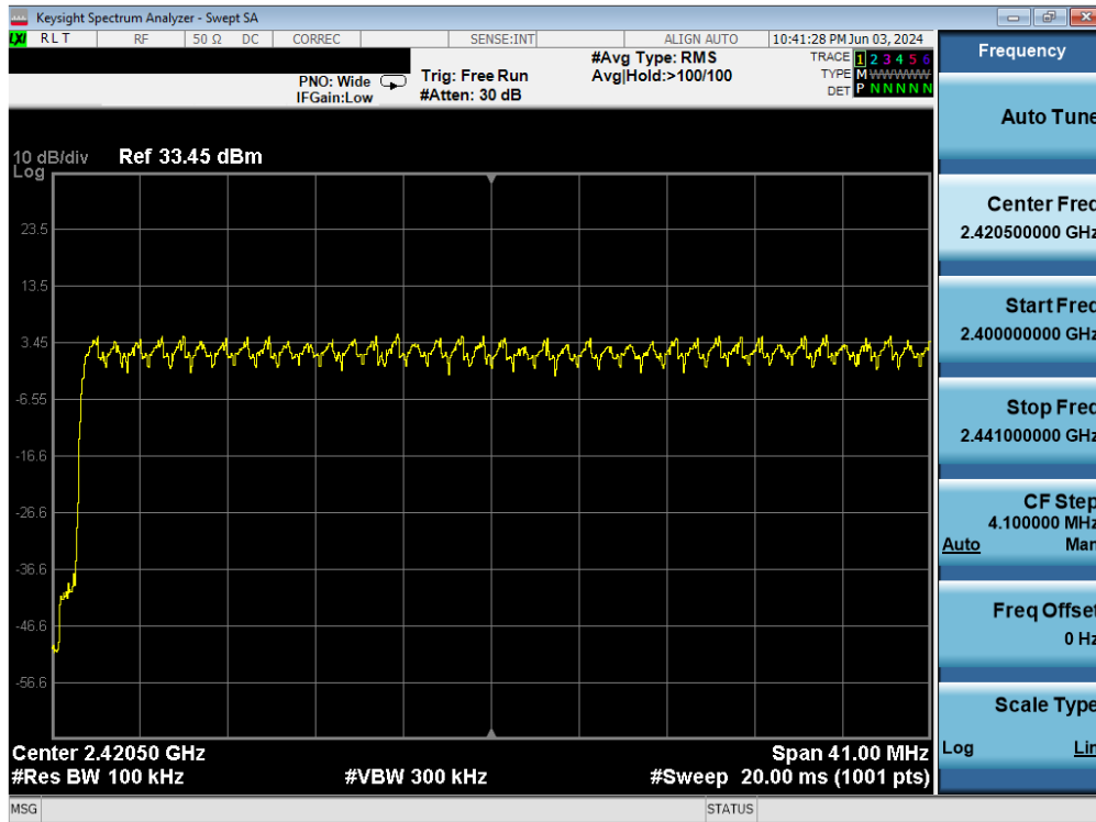
Plot 7-65. Low End Spectrum Channel Hopping Plot Antenna 4 (Bluetooth, 8DPSK, iPA)
