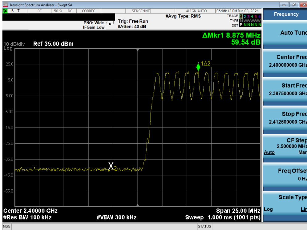
Plot 7-21. Band Edge Plot Antenna 3a (Bluetooth with Hopping Enabled, GFSK, ePA)
