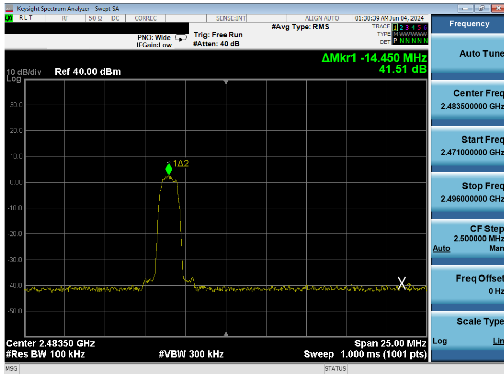
Plot 7-40. Band Edge Plot Antenna 4 (Bluetooth with Hopping Disabled, 8DPSK, iPA – Ch. 78)
