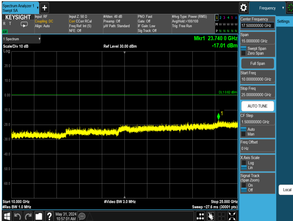
Plot 7-70. Conducted Spurious Plot Antenna 3a (Bluetooth, GFSK, ePA Ch. 39)
