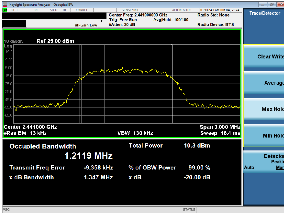
Plot 7-17. 20dB BW and 99% OBW Plot Antenna 4 (Bluetooth, 8DPSK, iPA – Ch. 39)
