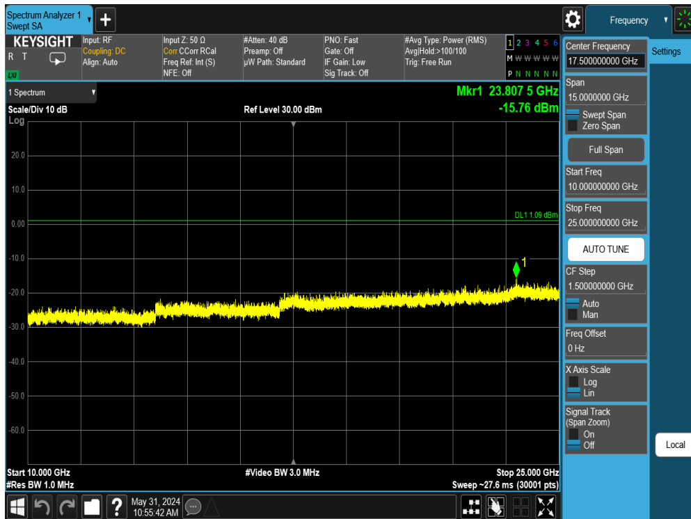
Plot 7-68. Conducted Spurious Plot Antenna 3a (Bluetooth, GFSK, ePA – Ch. 0)
