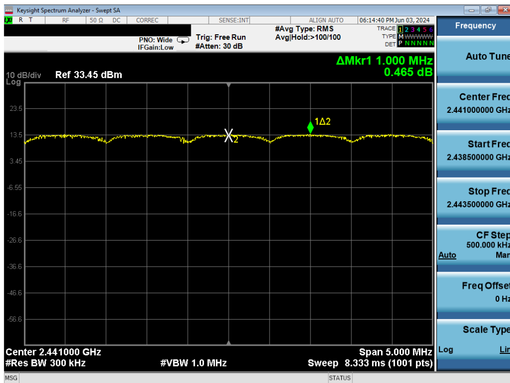
Plot 7-44. Channel Spacing Plot Antenna 3a (Bluetooth, 8DPSK, ePA)
