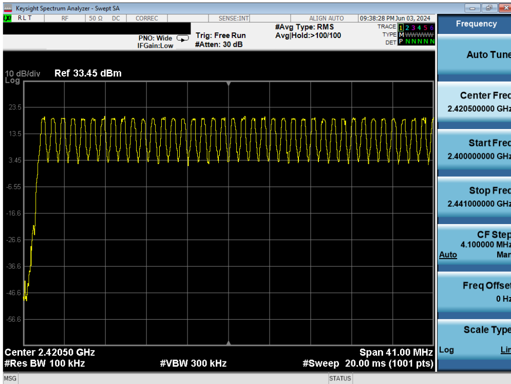
Plot 7-59. Low End Spectrum Channel Hopping Plot Antenna 1a (Bluetooth, GFSK, ePA)
