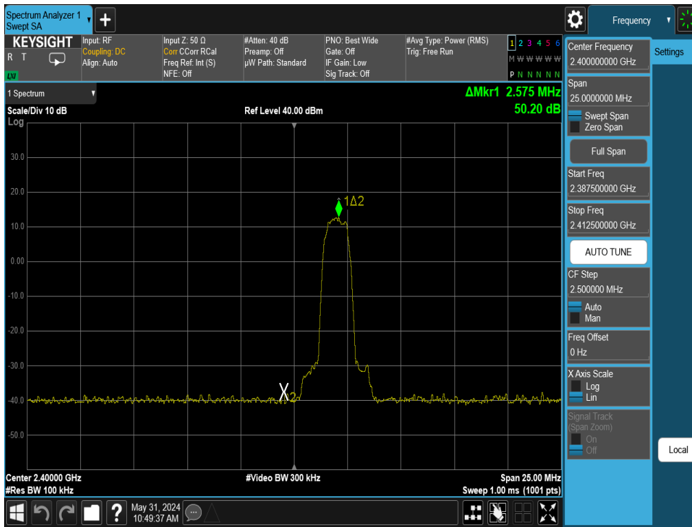
Plot 7-23. Band Edge Plot Antenna 3a (Bluetooth with Hopping Disabled, 8DPSK, ePA – Ch. 0)
