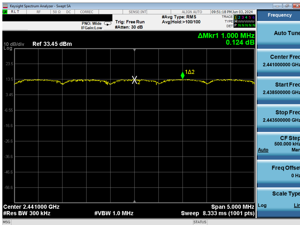
Plot 7-46. Channel Spacing Plot Antenna 1a (Bluetooth, 8DPSK, ePA)
