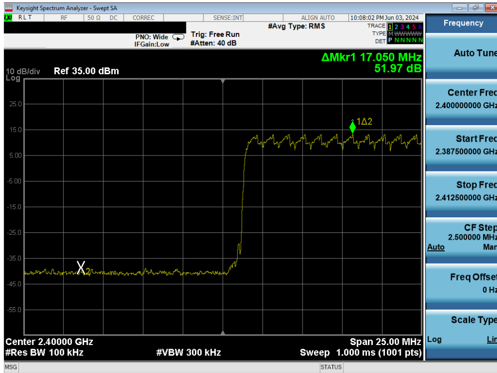
Plot 7-33. Band Edge Plot Antenna 1a (Bluetooth with Hopping Enabled, 8DPSK, ePA)
