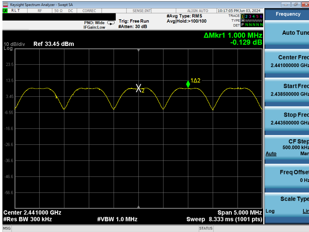
Plot 7-47. Channel Spacing Plot Antenna 4 (Bluetooth, GFSK, iPA)
