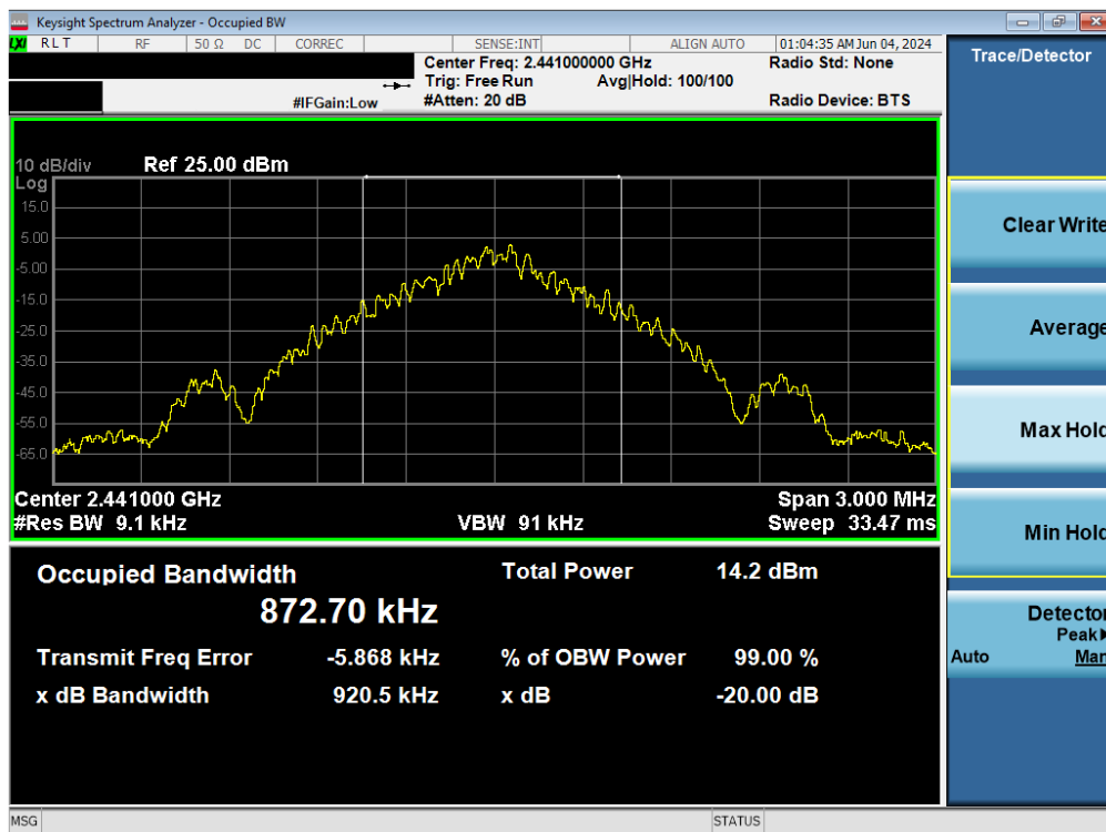
Plot 7-14. 20dB BW and 99% OBW Plot Antenna 4 (Bluetooth, GFSK, iPA – Ch. 39)
