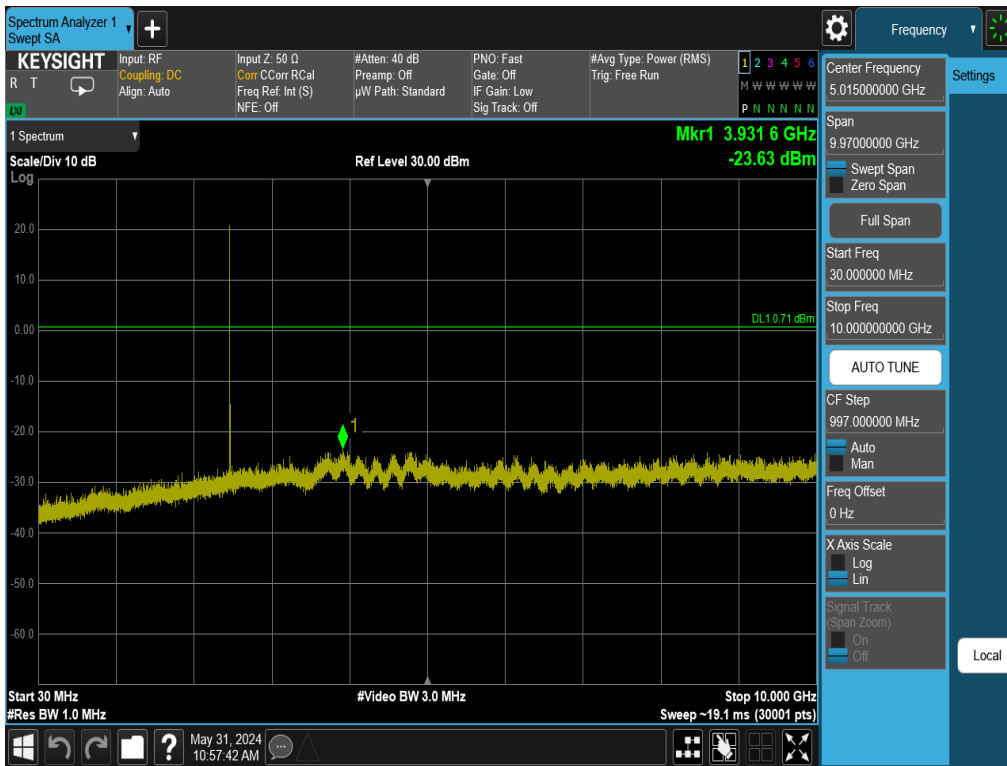
Plot 7-71. Conducted Spurious Plot Antenna 3a (Bluetooth, GFSK, ePA – Ch. 78)
