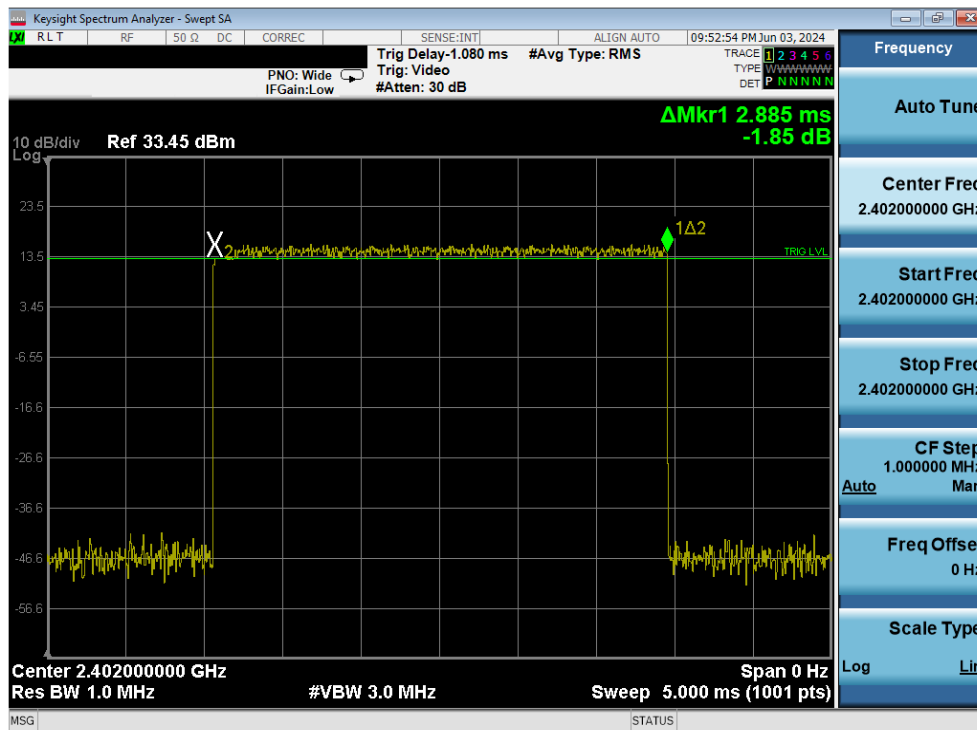
Plot 7-52. Time of Occupancy Plot Antenna 1a (Bluetooth, 8DPSK, ePA)
