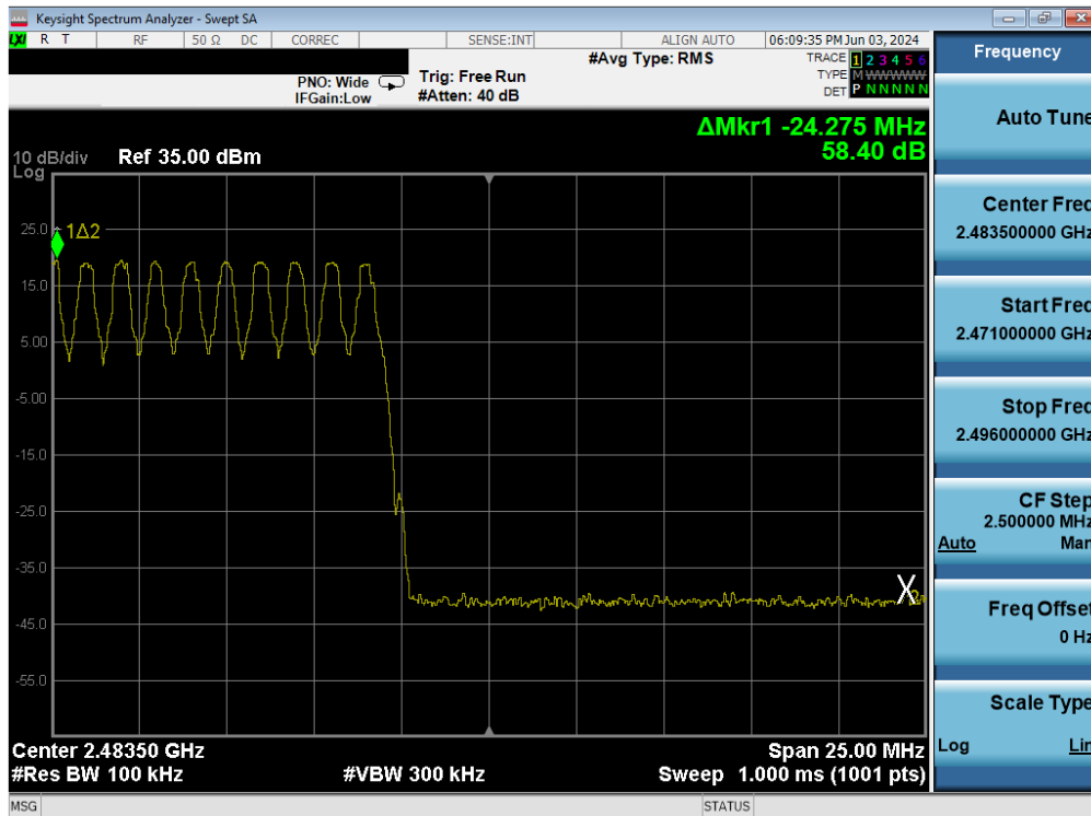
Plot 7-22. Band Edge Plot Antenna 3a (Bluetooth with Hopping Enabled, GFSK, ePA)
