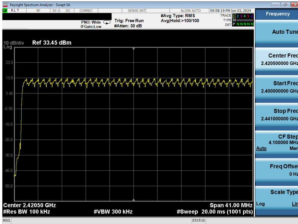
Plot 7-61. Low End Spectrum Channel Hopping Plot Antenna 1a (Bluetooth, 8DPSK, ePA)
