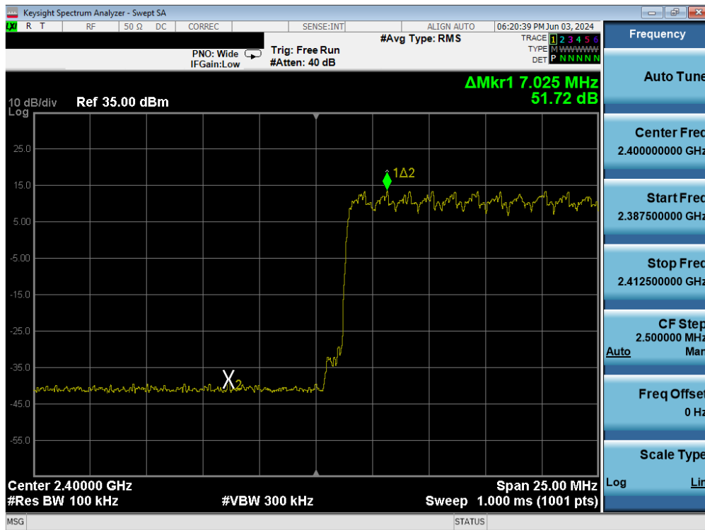
Plot 7-25. Band Edge Plot Antenna 3a (Bluetooth with Hopping Enabled, 8DPSK, ePA)
