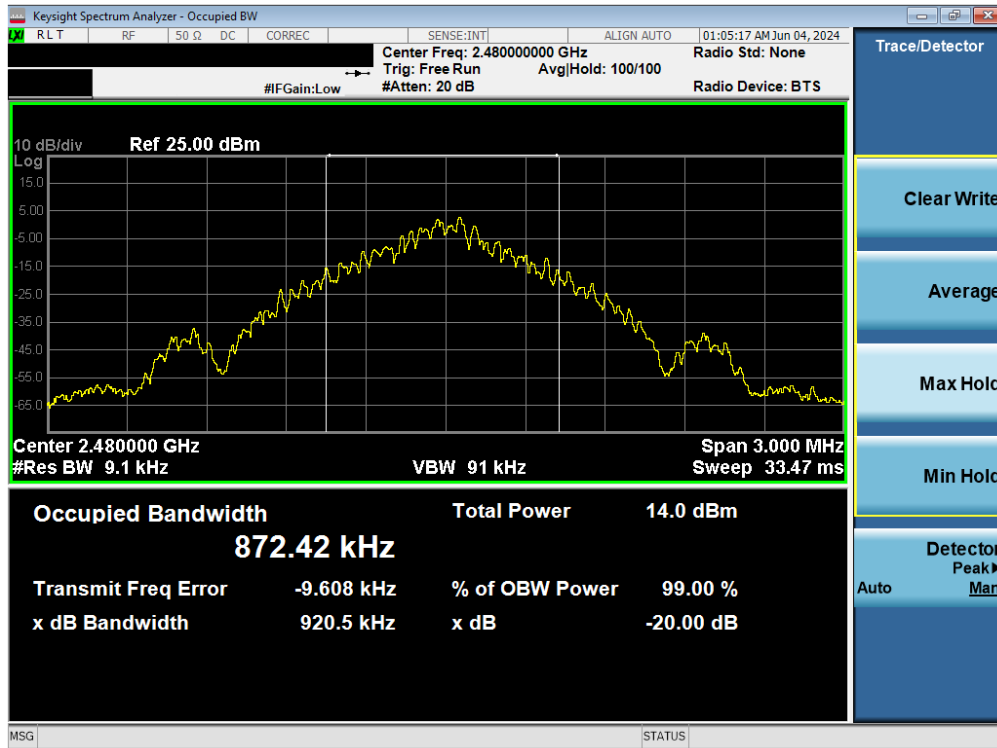
Plot 7-15. 20dB BW and 99% OBW Plot Antenna 4 (Bluetooth, GFSK, iPA – Ch. 78)
