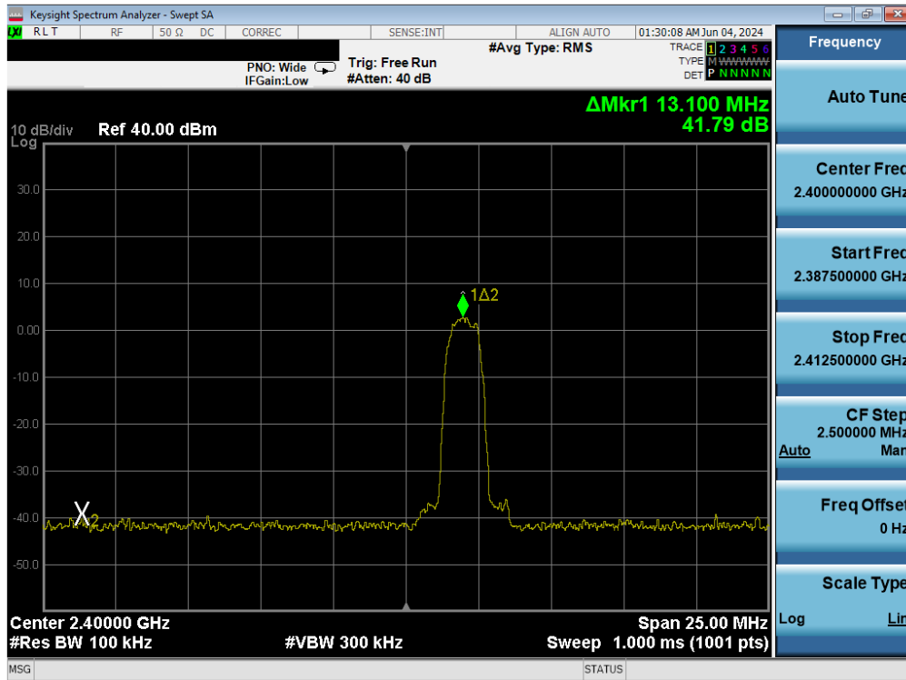
Plot 7-39. Band Edge Plot Antenna 4 (Bluetooth with Hopping Disabled, 8DPSK, iPA – Ch. 0)
