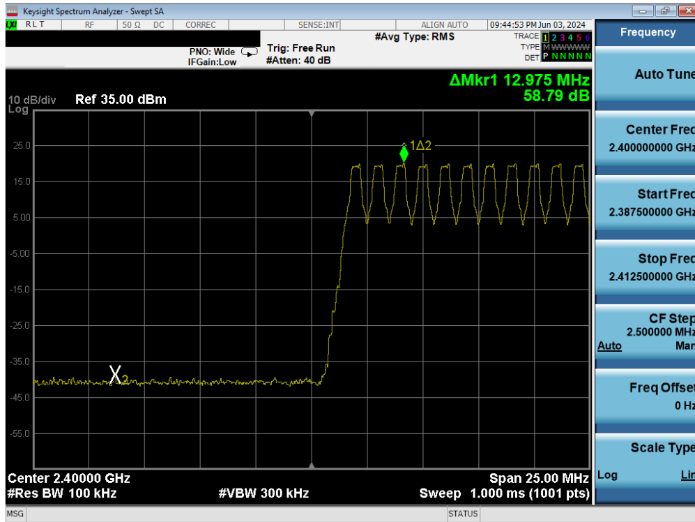
Plot 7-29. Band Edge Plot Antenna 1a (Bluetooth with Hopping Enabled, GFSK, ePA)
