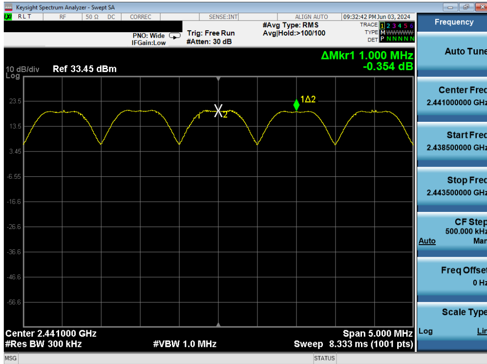
Plot 7-45. Channel Spacing Plot Antenna 1a (Bluetooth, GFSK, ePA)
