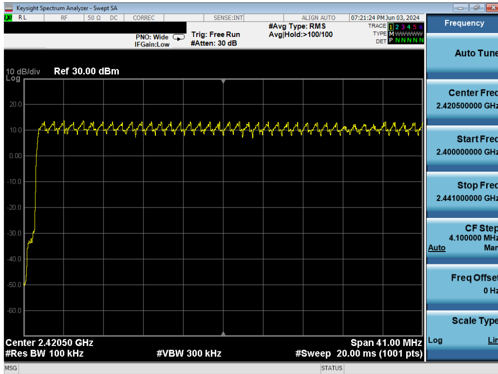
Plot 7-57. Low End Spectrum Channel Hopping Plot Antenna 3a (Bluetooth, 8DPSK, ePA)
