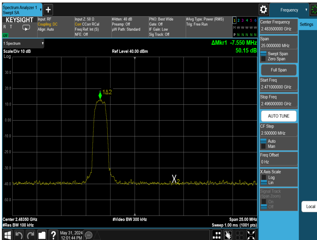
Plot 7-32. Band Edge Plot Antenna 1a (Bluetooth with Hopping Disabled, 8DPSK, ePA – Ch. 78)
