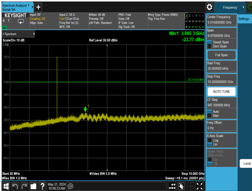
Plot 7-69. Conducted Spurious Plot Antenna 3a (Bluetooth, GFSK, ePA – Ch. 39)
