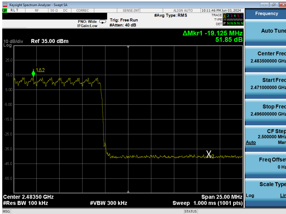
Plot 7-34. Band Edge Plot Antenna 1a (Bluetooth with Hopping Enabled, 8DPSK, ePA)
