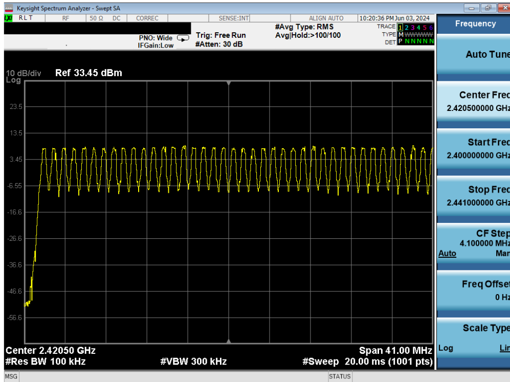
Plot 7-63. Low End Spectrum Channel Hopping Plot Antenna 4 (Bluetooth, GFSK, iPA)
