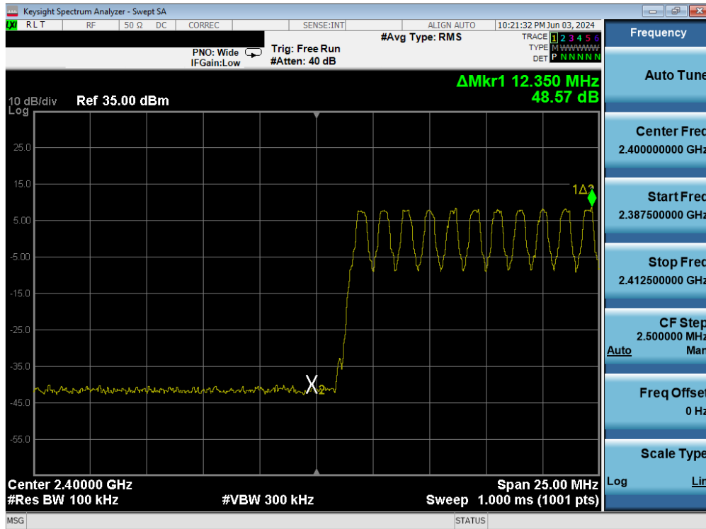
Plot 7-37. Band Edge Plot Antenna 4 (Bluetooth with Hopping Enabled, GFSK, iPA)
