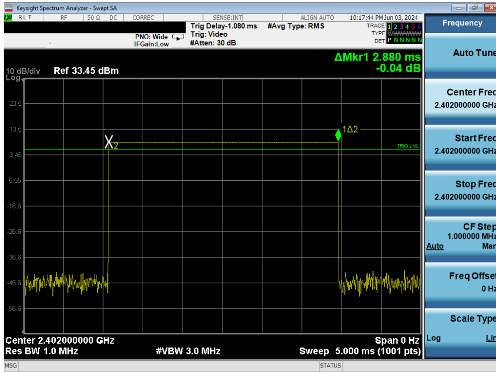
Plot 7-53. Time of Occupancy Plot Antenna 4 (Bluetooth, GFSK, iPA)
