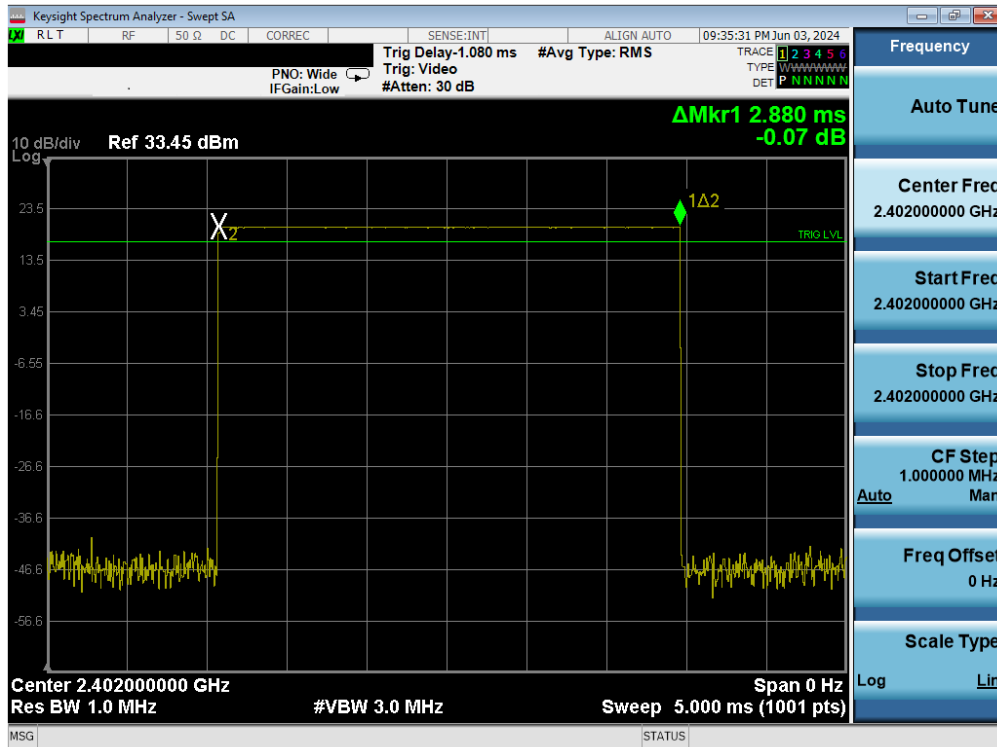
Plot 7-51. Time of Occupancy Plot Antenna 1a (Bluetooth, GFSK, ePA)
