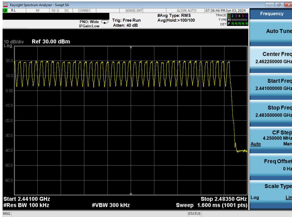
Plot 7-56. High End Spectrum Channel Hopping Plot Antenna 3a (Bluetooth, GFSK, ePA)
