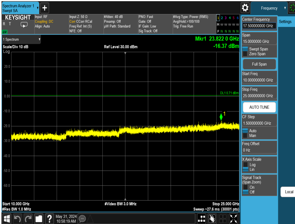
Plot 7-72. Conducted Spurious Plot Antenna 3a (Bluetooth, GFSK, ePA – Ch. 78)
