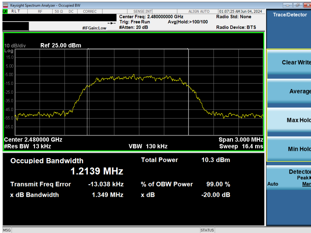
Plot 7-18. 20dB BW and 99% OBW Plot Antenna 4 (Bluetooth, 8DPSK, iPA – Ch. 78)
