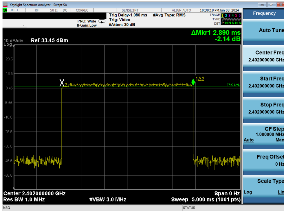
Plot 7-54. Time of Occupancy Plot Antenna 4 (Bluetooth, 8DPSK, iPA)
