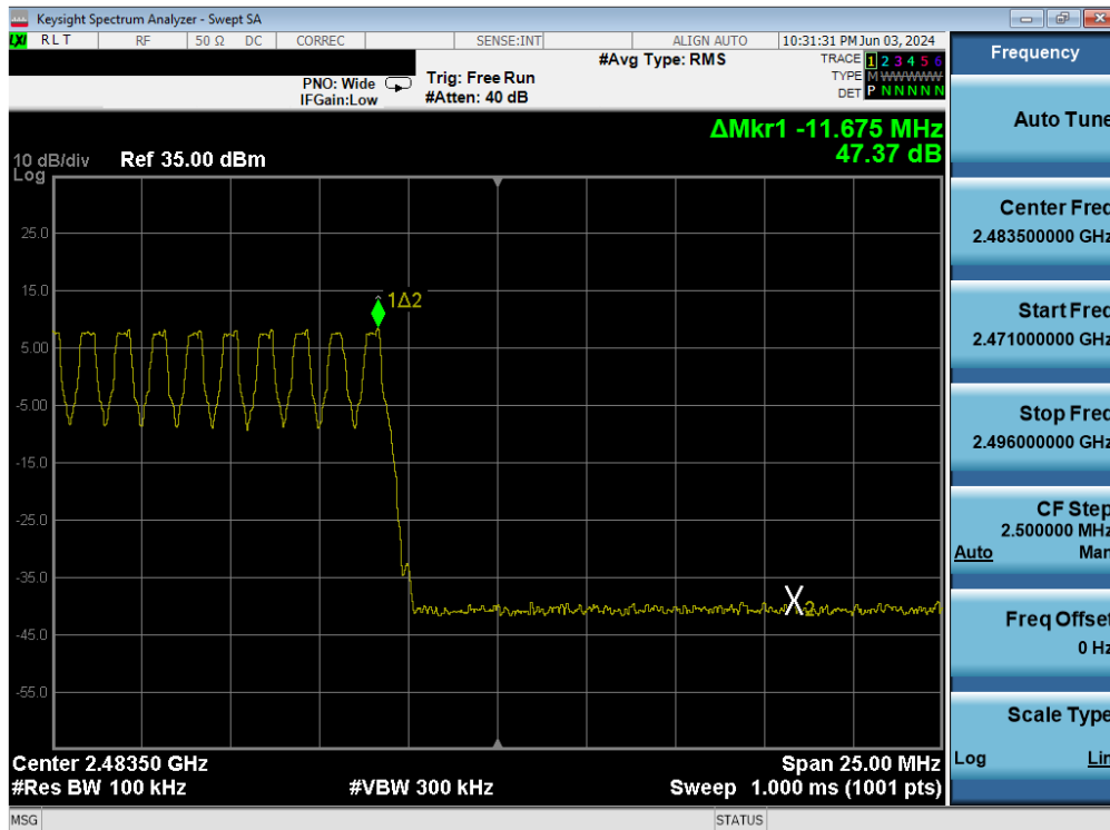
Plot 7-38. Band Edge Plot Antenna 4 (Bluetooth with Hopping Enabled, GFSK, iPA)
