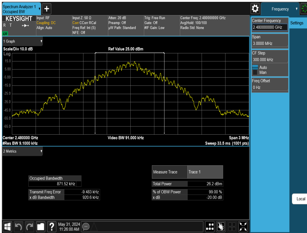
Plot 7-9. 20dB BW and 99% OBW Plot Antenna 1a (Bluetooth, GFSK, ePA – Ch. 78)
