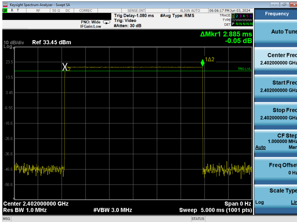
Plot 7-49. Time of Occupancy Plot Antenna 3a (Bluetooth, GFSK, ePA)
