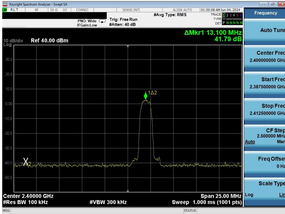
Plot 7-41. Band Edge Plot Antenna 4 (Bluetooth with Hopping Enabled, 8DPSK, iPA)
