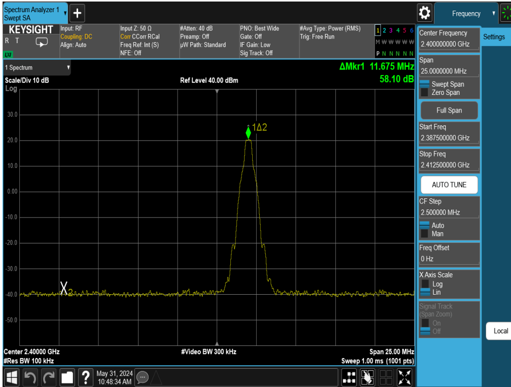
Plot 7-19. Band Edge Plot Antenna 3a (Bluetooth with Hopping Disabled, GFSK, ePA – Ch. 0)
