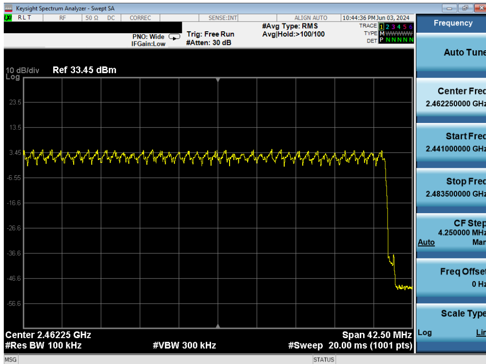
Plot 7-66. High End Spectrum Channel Hopping Plot Antenna 4 (Bluetooth, 8DPSK, iPA)
