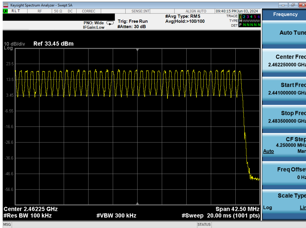
Plot 7-60. High End Spectrum Channel Hopping Plot Antenna 1a (Bluetooth, GFSK, ePA)
