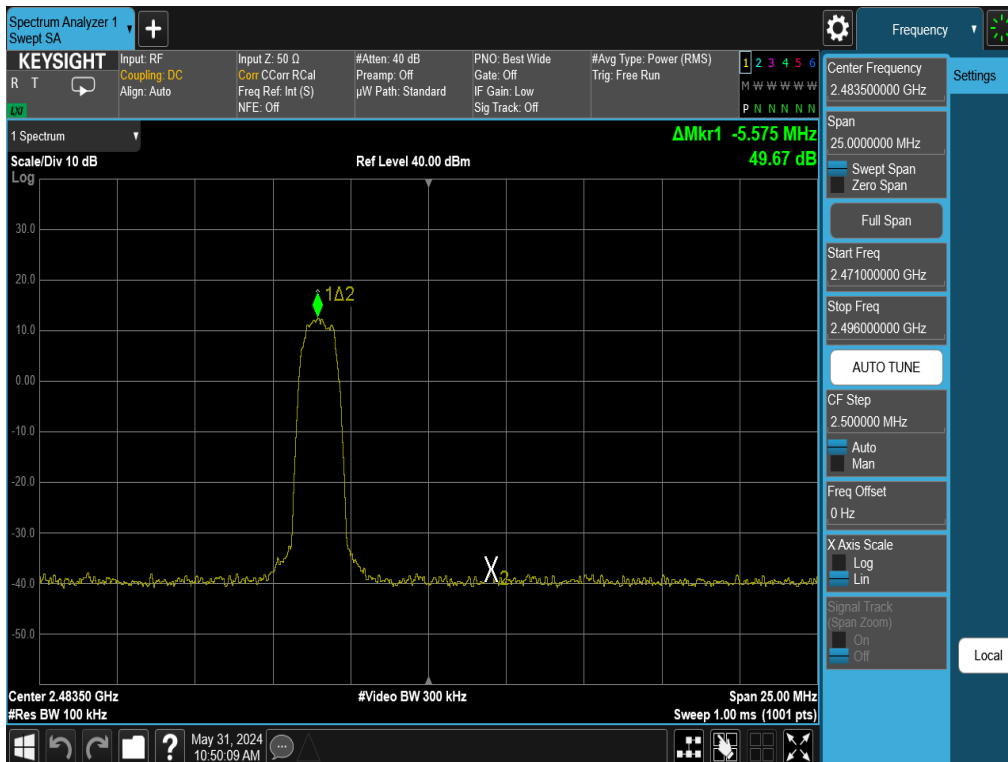
Plot 7-24. Band Edge Plot Antenna 3a (Bluetooth with Hopping Disabled, 8DPSK, ePA – Ch. 78)
