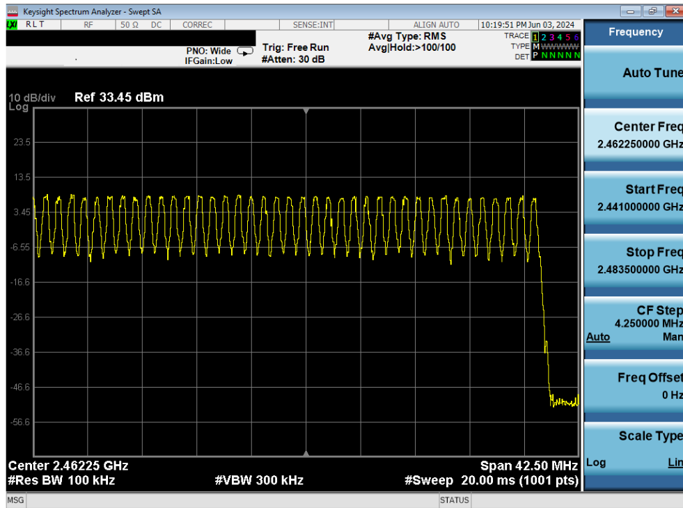
Plot 7-64. High End Spectrum Channel Hopping Plot Antenna 4 (Bluetooth, GFSK, iPA)
