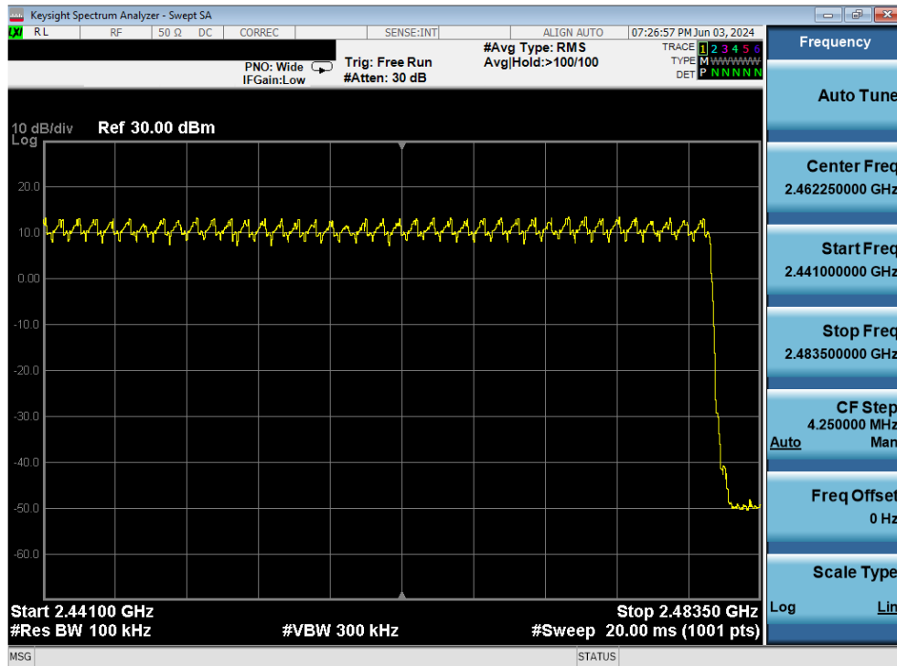
Plot 7-58. High End Spectrum Channel Hopping Plot Antenna 3a (Bluetooth, 8DPSK, ePA)
