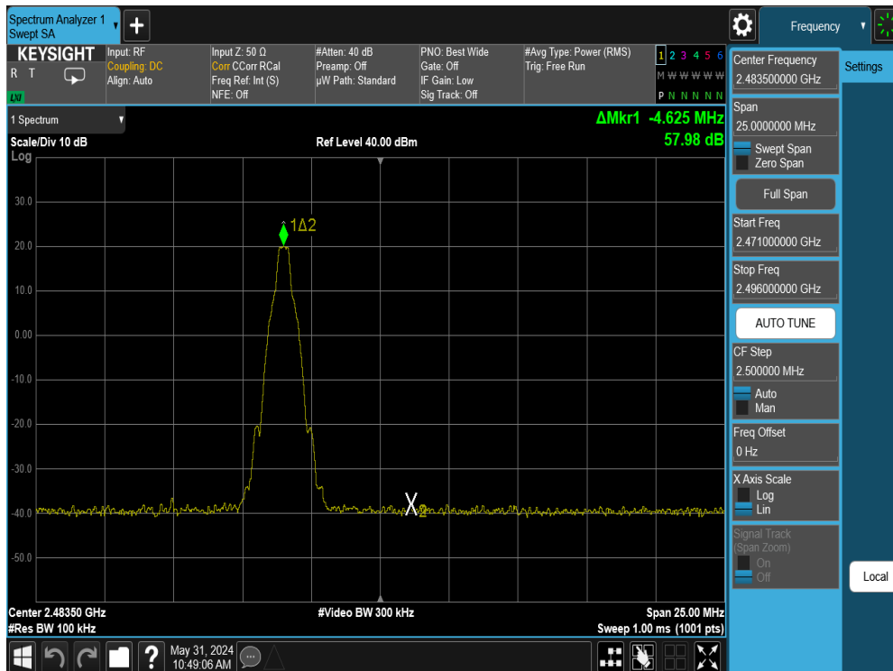
Plot 7-20. Band Edge Plot Antenna 3a (Bluetooth with Hopping Disabled, GFSK, ePA – Ch. 78)
