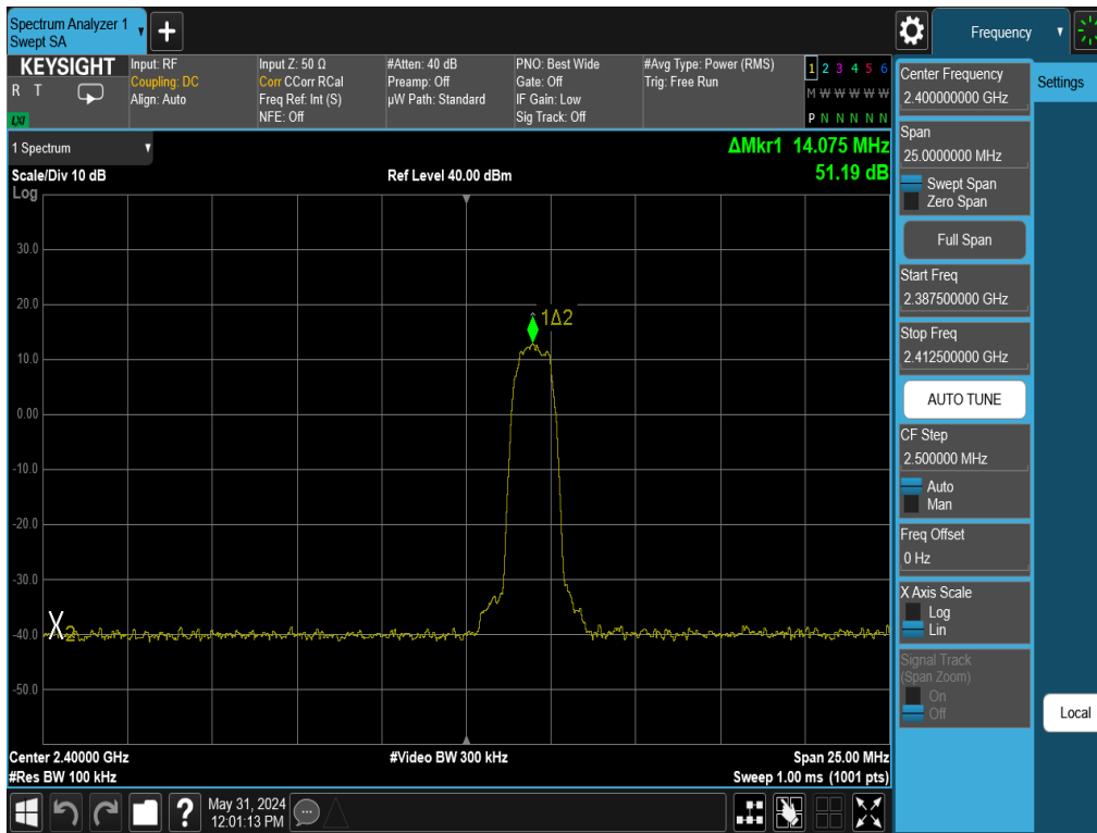
Plot 7-31. Band Edge Plot Antenna 1a (Bluetooth with Hopping Disabled, 8DPSK, ePA – Ch. 0)
