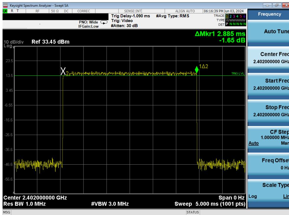
Plot 7-50. Time of Occupancy Plot Antenna 3a (Bluetooth, 8DPSK, ePA)
