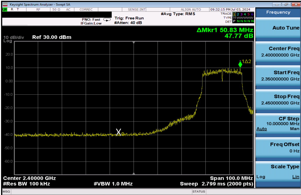
Plot 7-348. Band Edge Plot Antenna 1a (802.11g – Ch. 6 Low) – 24Mbps
