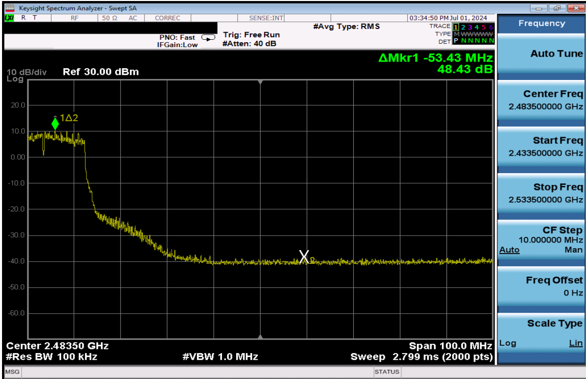
Plot 7-363. Band Edge Plot Antenna 1a (802.11n (2.4GHz) - Ch. 6 High) - MCS4
