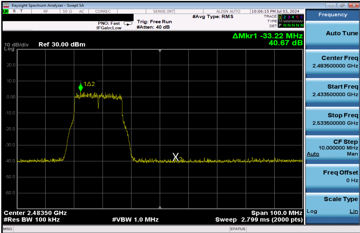
Plot 7-399. Band Edge Plot Antenna 1a (802.11g – Ch. 11) – 54Mbps
