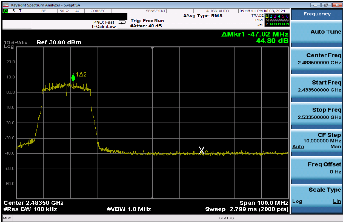
Plot 7-366. Band Edge Plot Antenna 1a (802.11n (2.4GHz) – Ch. 9) – MCS4
