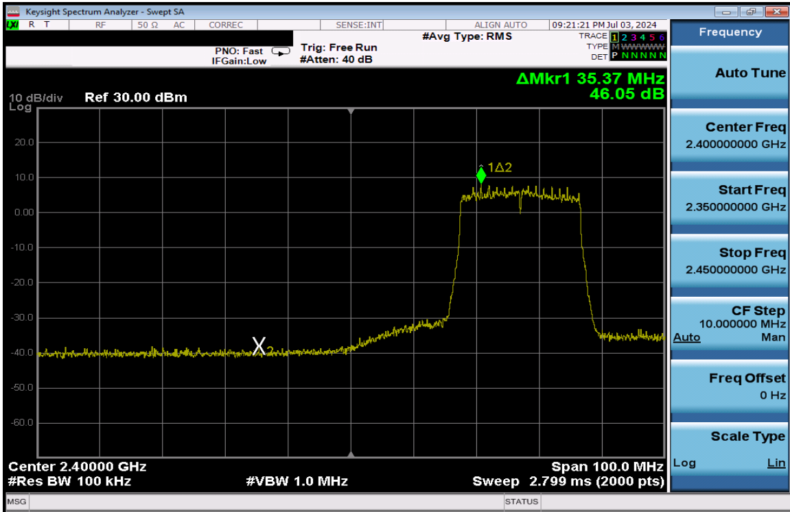
Plot 7-333. Band Edge Plot Antenna 1a (802.11ax (SU - 2.4GHz) – Ch. 4) – MCS2
