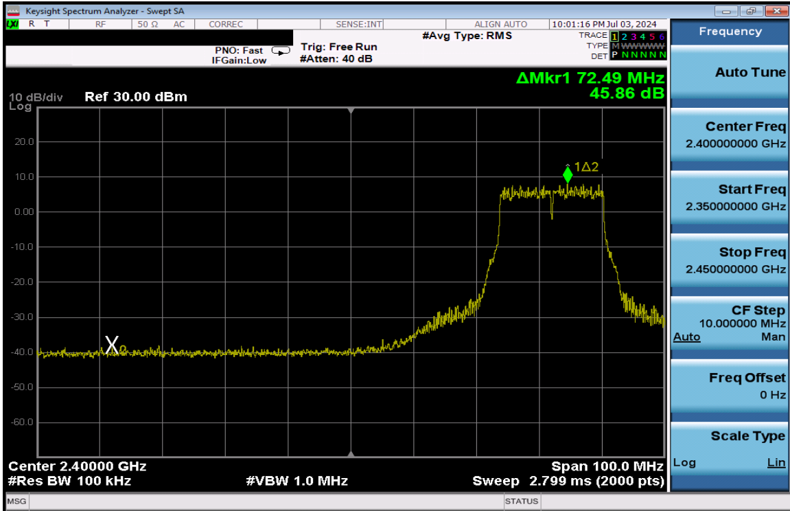
Plot 7-392. Band Edge Plot Antenna 1a (802.11g – Ch. 5) – 54Mbps
