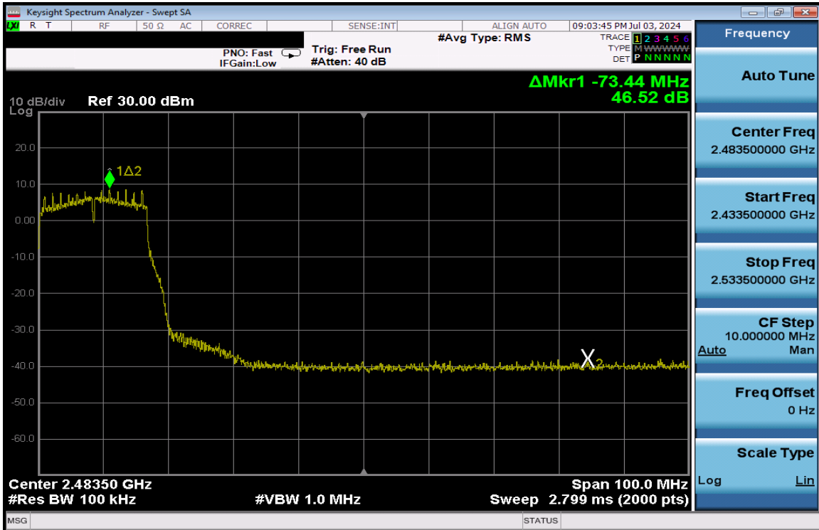
Plot 7-309. Band Edge Plot Antenna 1a (802.11g – Ch. 7) – 12Mbps
