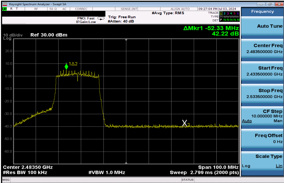
Plot 7-341. Band Edge Plot Antenna 1a (802.11ax (SU - 2.4GHz) – Ch. 11) – MCS2
