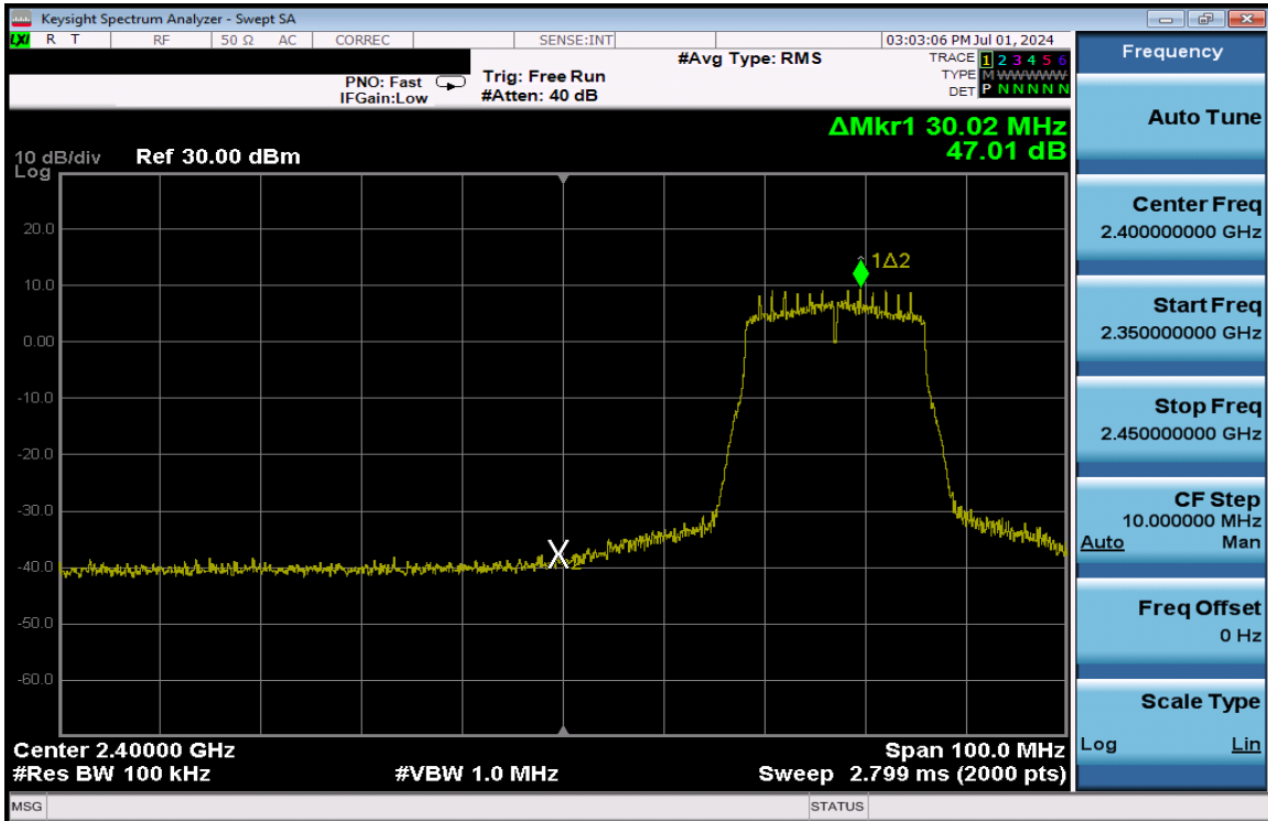
Plot 7-319. Band Edge Plot Antenna 1a (802.11n (2.4GHz) – Ch. 4) – MCS2
