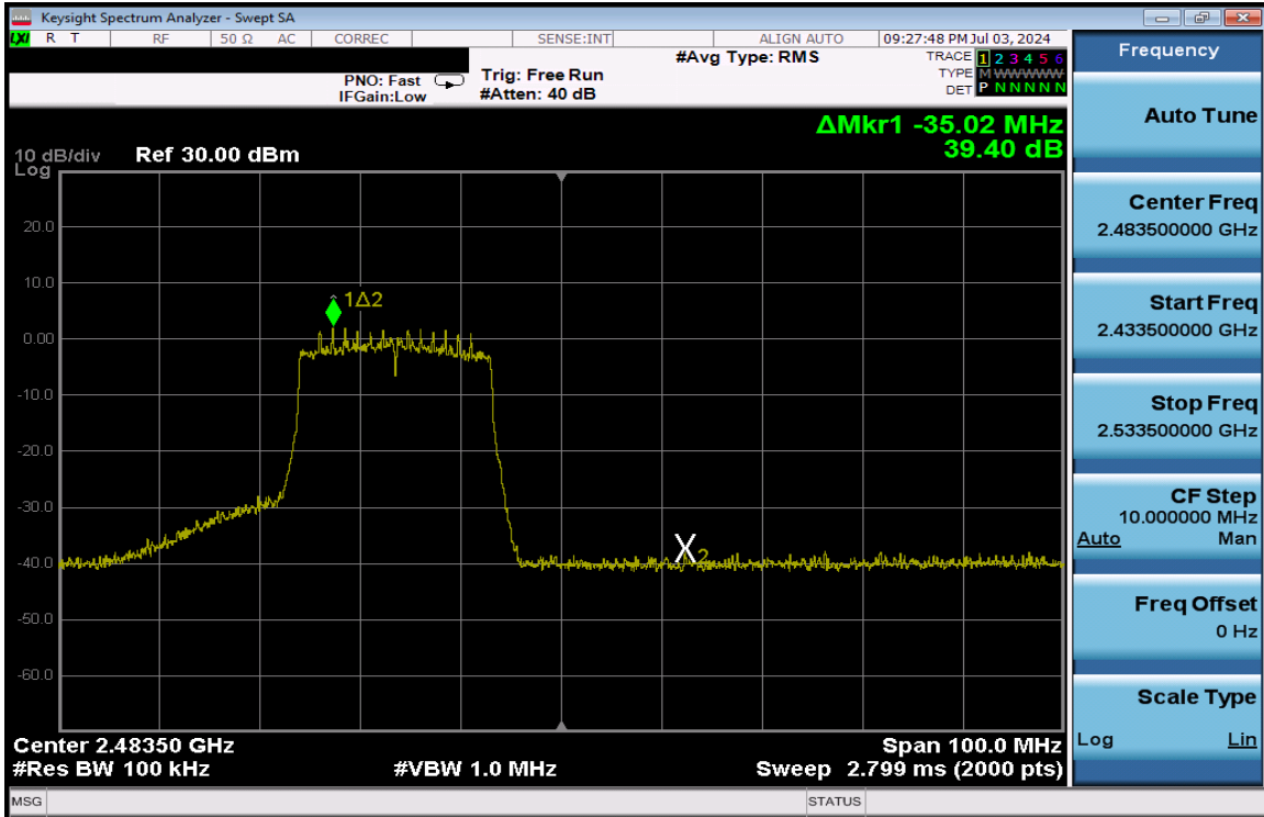
Plot 7-342. Band Edge Plot Antenna 1a (802.11ax (SU - 2.4GHz) – Ch. 12) – MCS2
