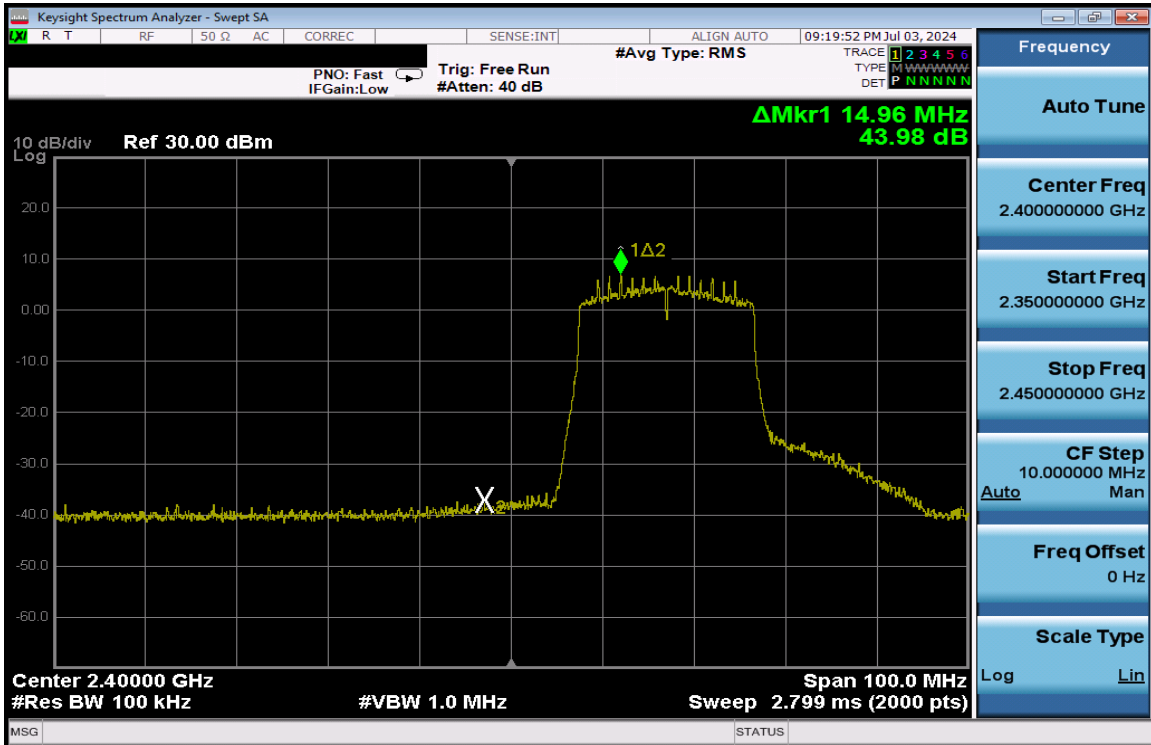
Plot 7-331. Band Edge Plot Antenna 1a (802.11ax (SU - 2.4GHz) – Ch. 2) – MCS2
