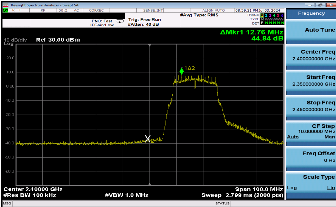
Plot 7-303. Band Edge Plot Antenna 1a (802.11g – Ch. 2) – 12Mbps
