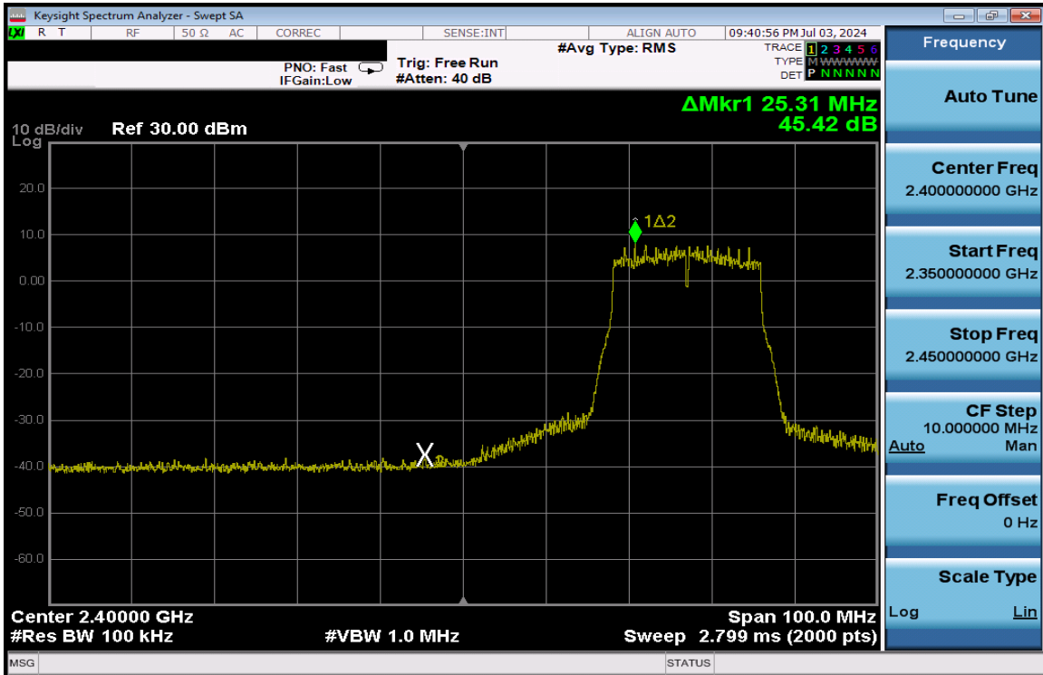
Plot 7-360. Band Edge Plot Antenna 1a (802.11n (2.4GHz) – Ch. 4) – MCS4
