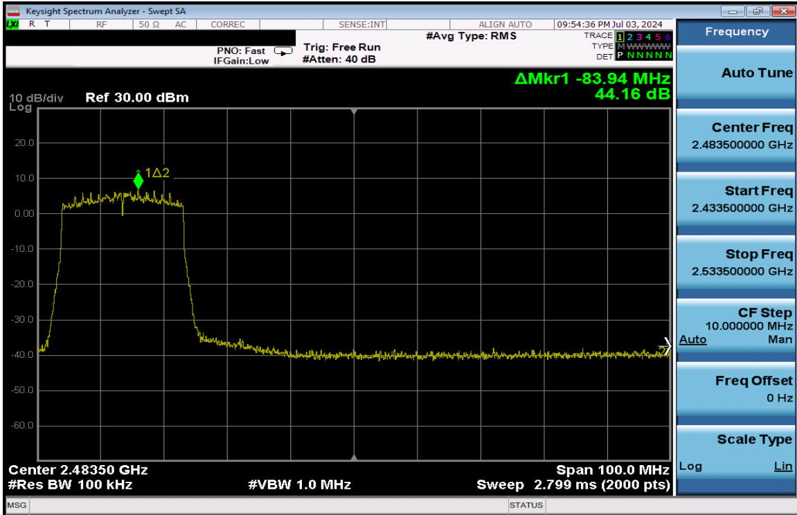
Plot 7-379. Band Edge Plot Antenna 1a (802.11ax (SU - 2.4GHz) – Ch. 8) – MCS4
