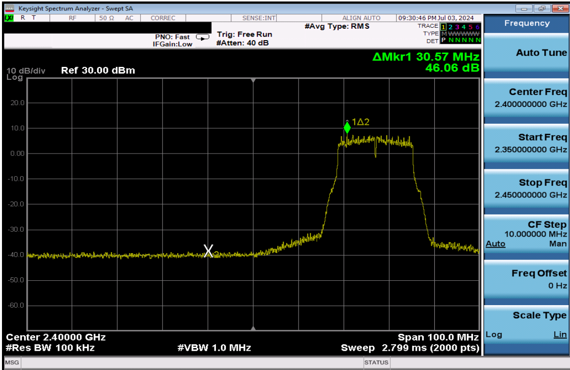
Plot 7-346. Band Edge Plot Antenna 1a (802.11g – Ch. 4) – 24Mbps
