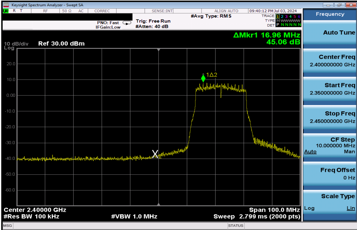
Plot 7-359. Band Edge Plot Antenna 1a (802.11n (2.4GHz) – Ch. 3) – MCS4
