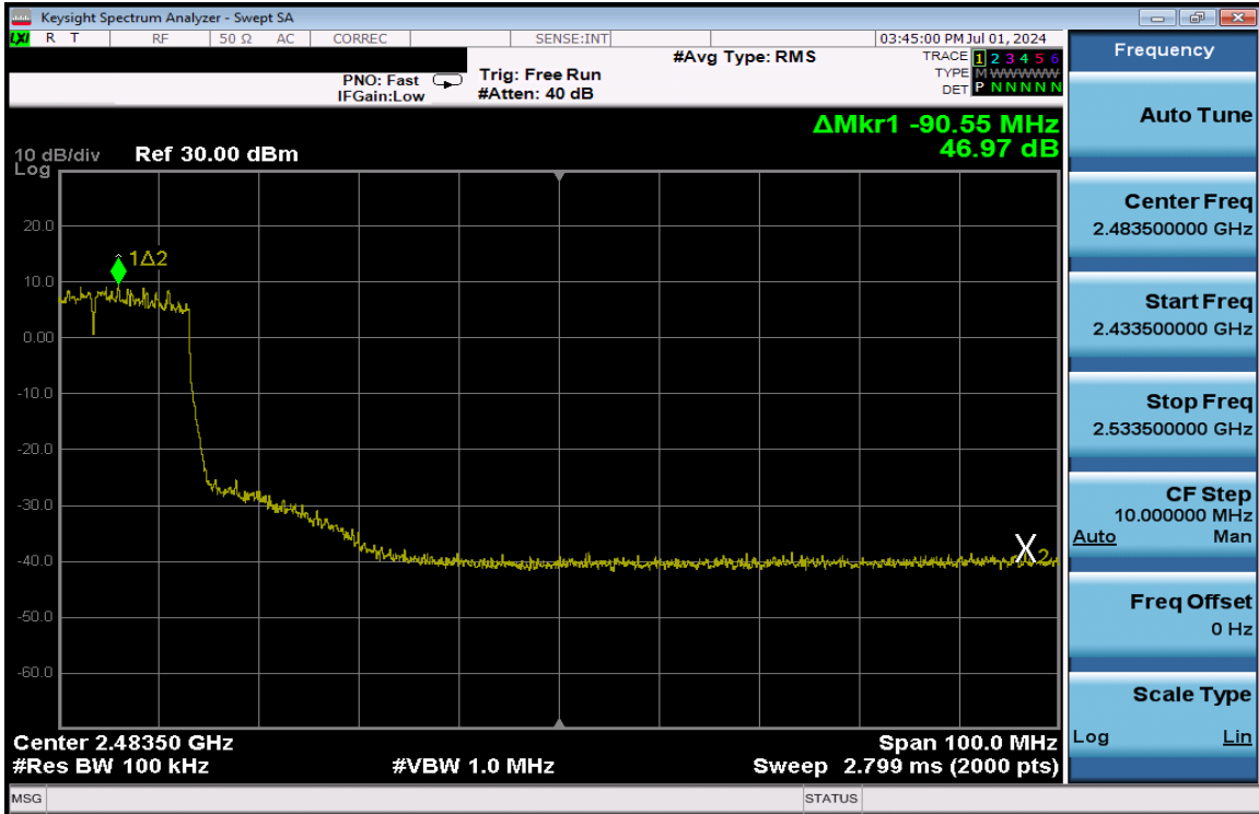
Plot 7-377. Band Edge Plot Antenna 1a (802.11ax (SU - 2.4GHz) – Ch. 6 High) – MCS4
