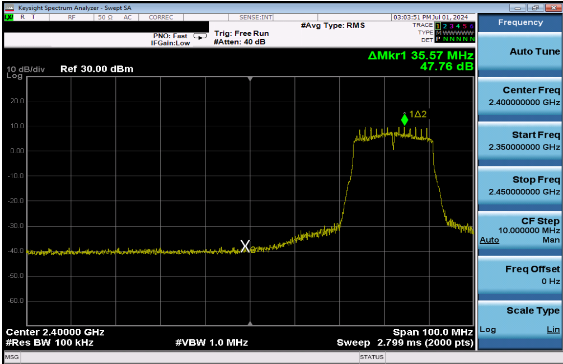
Plot 7-320. Band Edge Plot Antenna 1a (802.11n (2.4GHz) – Ch. 5) – MCS2
