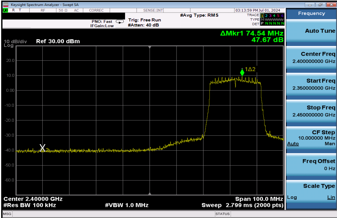
Plot 7-334. Band Edge Plot Antenna 1a (802.11ax (SU - 2.4GHz) – Ch. 5) – MCS2
