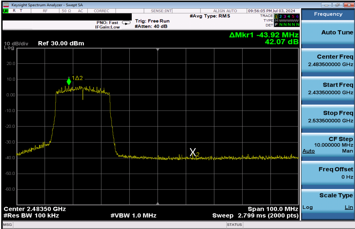
Plot 7-381. Band Edge Plot Antenna 1a (802.11ax (SU - 2.4GHz) – Ch. 10) – MCS4
