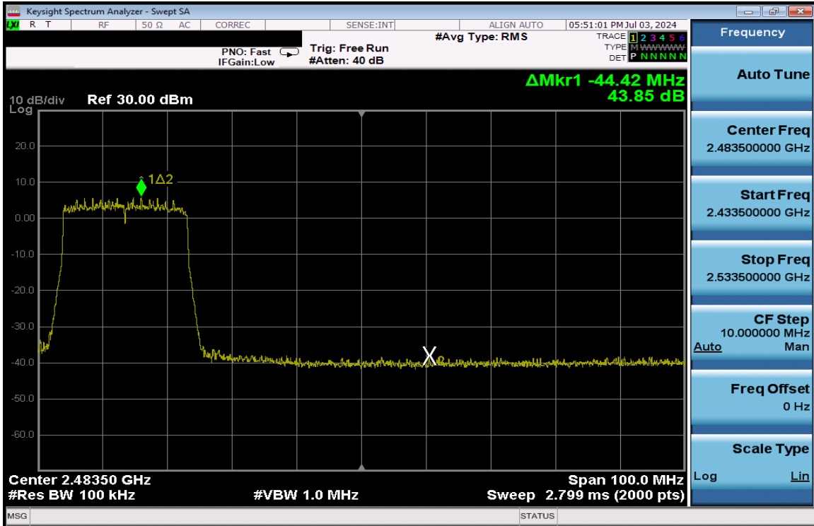
Plot 7-297. Band Edge Plot Antenna 3a (802.11ax (SU - 2.4GHz) – Ch. 8) – MCS9
