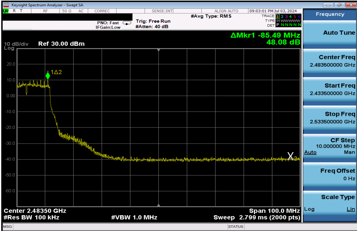
Plot 7-308. Band Edge Plot Antenna 1a (802.11g – Ch. 6 High) – 12Mbps
