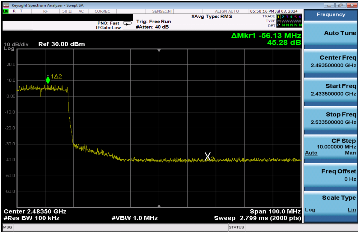
Plot 7-296. Band Edge Plot Antenna 3a (802.11ax (SU - 2.4GHz) – Ch. 7) – MCS9
