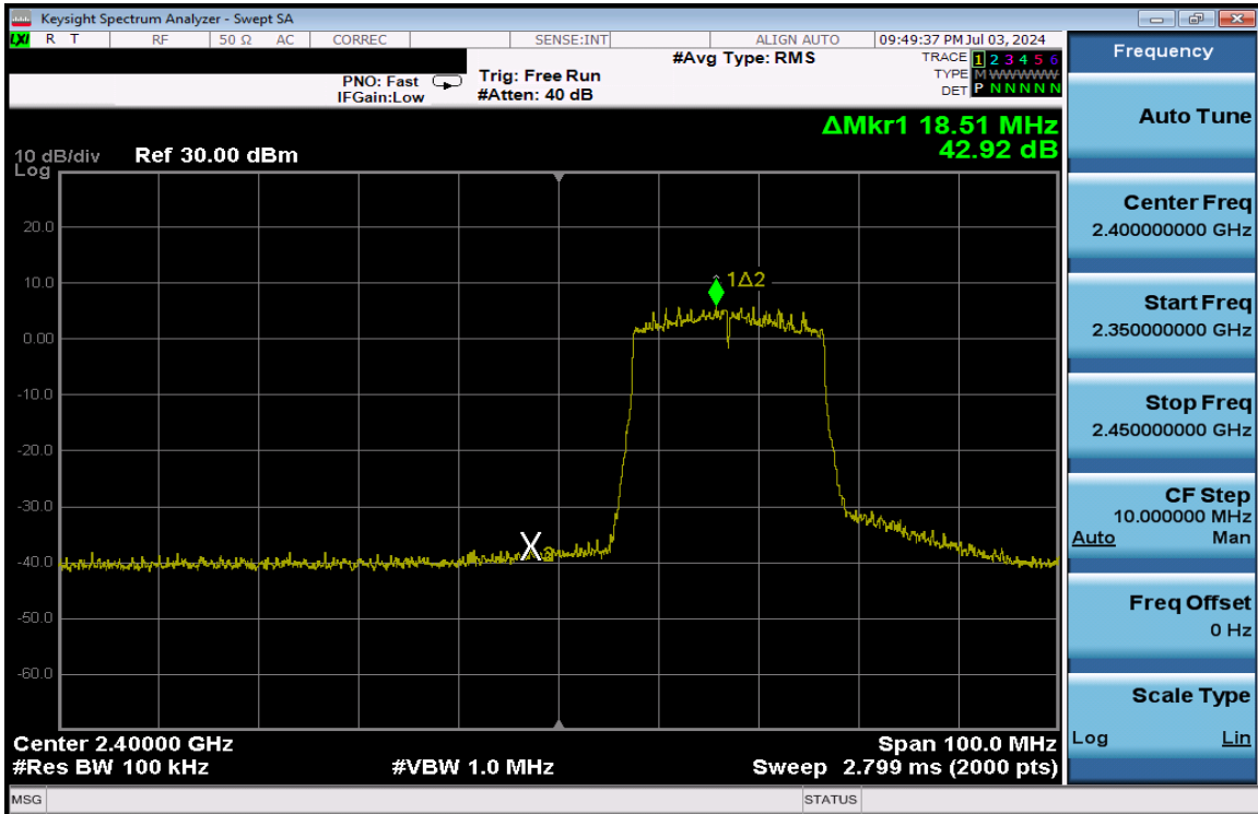
Plot 7-372. Band Edge Plot Antenna 1a (802.11ax (SU - 2.4GHz) – Ch. 2) – MCS4
