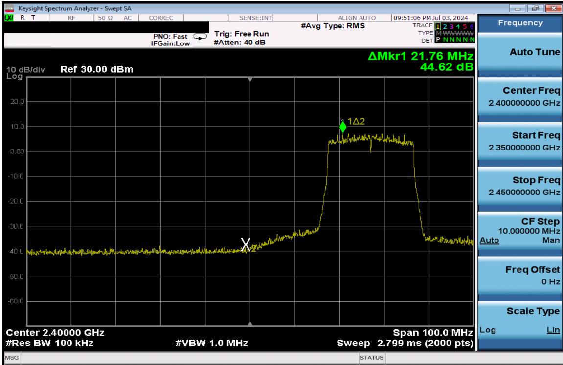
Plot 7-374. Band Edge Plot Antenna 1a (802.11ax (SU - 2.4GHz) – Ch. 4) – MCS4
