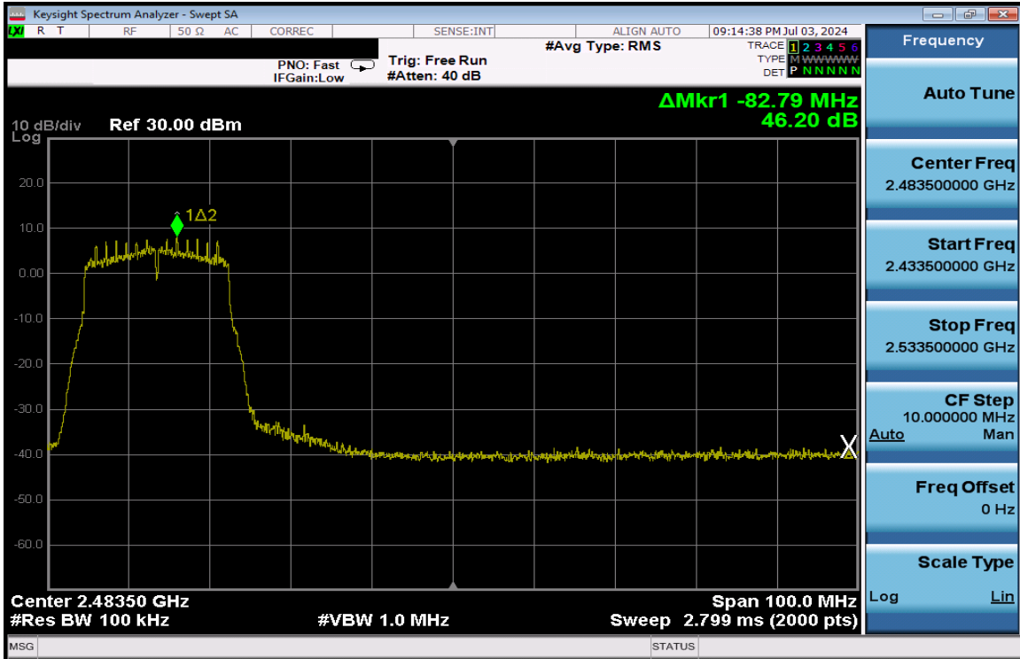
Plot 7-324. Band Edge Plot Antenna 1a (802.11n (2.4GHz) - Ch. 8) - MCS2
