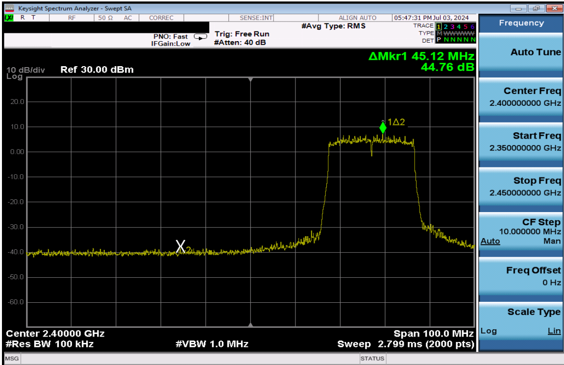
Plot 7-292. Band Edge Plot Antenna 3a (802.11ax (SU - 2.4GHz) – Ch. 4) – MCS9
