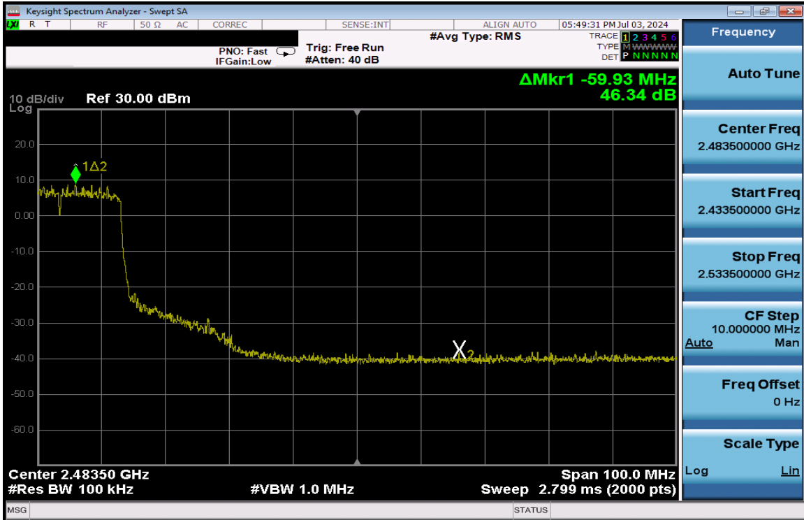
Plot 7-295. Band Edge Plot Antenna 3a (802.11ax (SU - 2.4GHz) – Ch. 6 High) – MCS9
