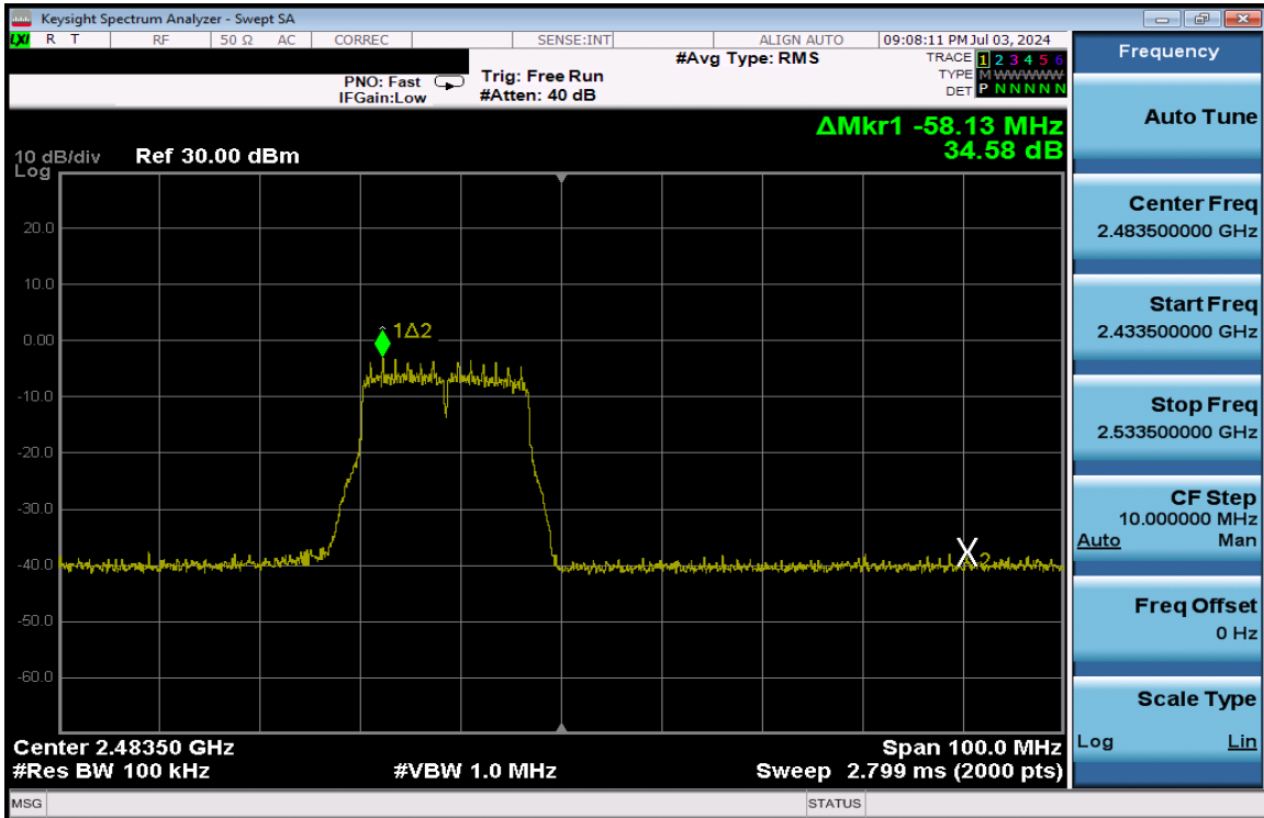
Plot 7-315. Band Edge Plot Antenna 1a (802.11g – Ch. 13) – 12Mbps
