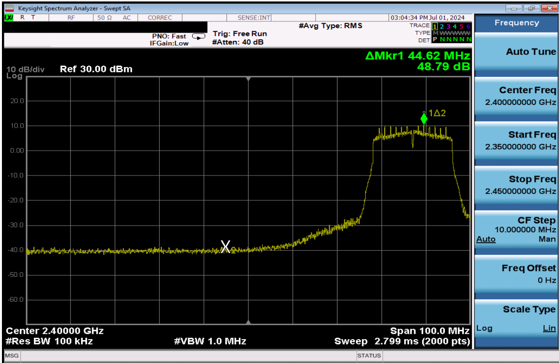
Plot 7-321. Band Edge Plot Antenna 1a (802.11n (2.4GHz) – Ch. 6 Low) – MCS2
