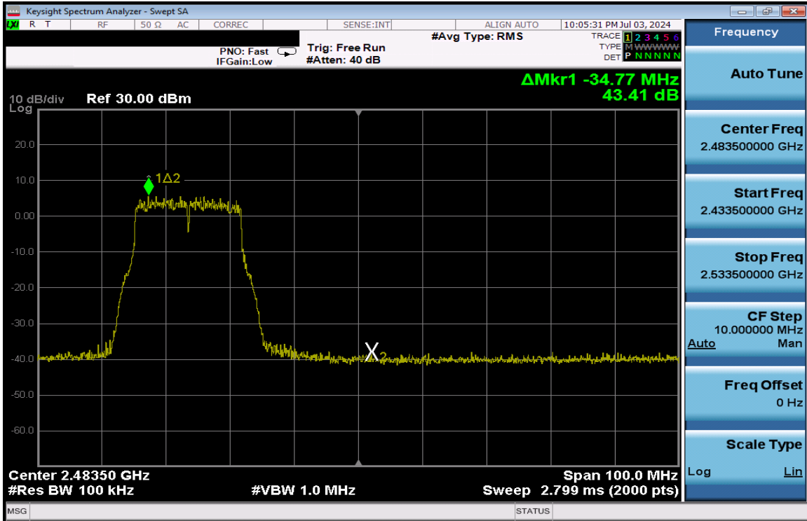
Plot 7-398. Band Edge Plot Antenna 1a (802.11g – Ch. 10) – 54Mbps
