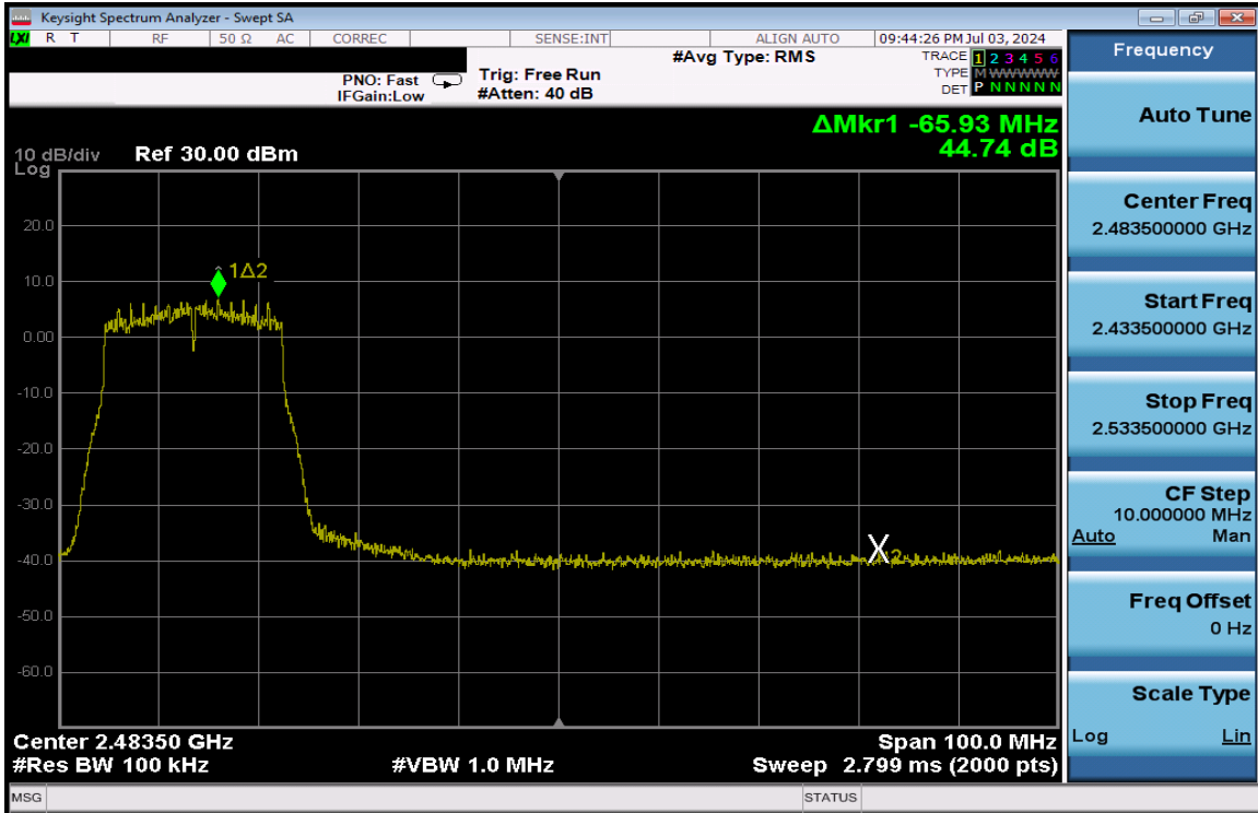
Plot 7-365. Band Edge Plot Antenna 1a (802.11n (2.4GHz) – Ch. 8) – MCS4
