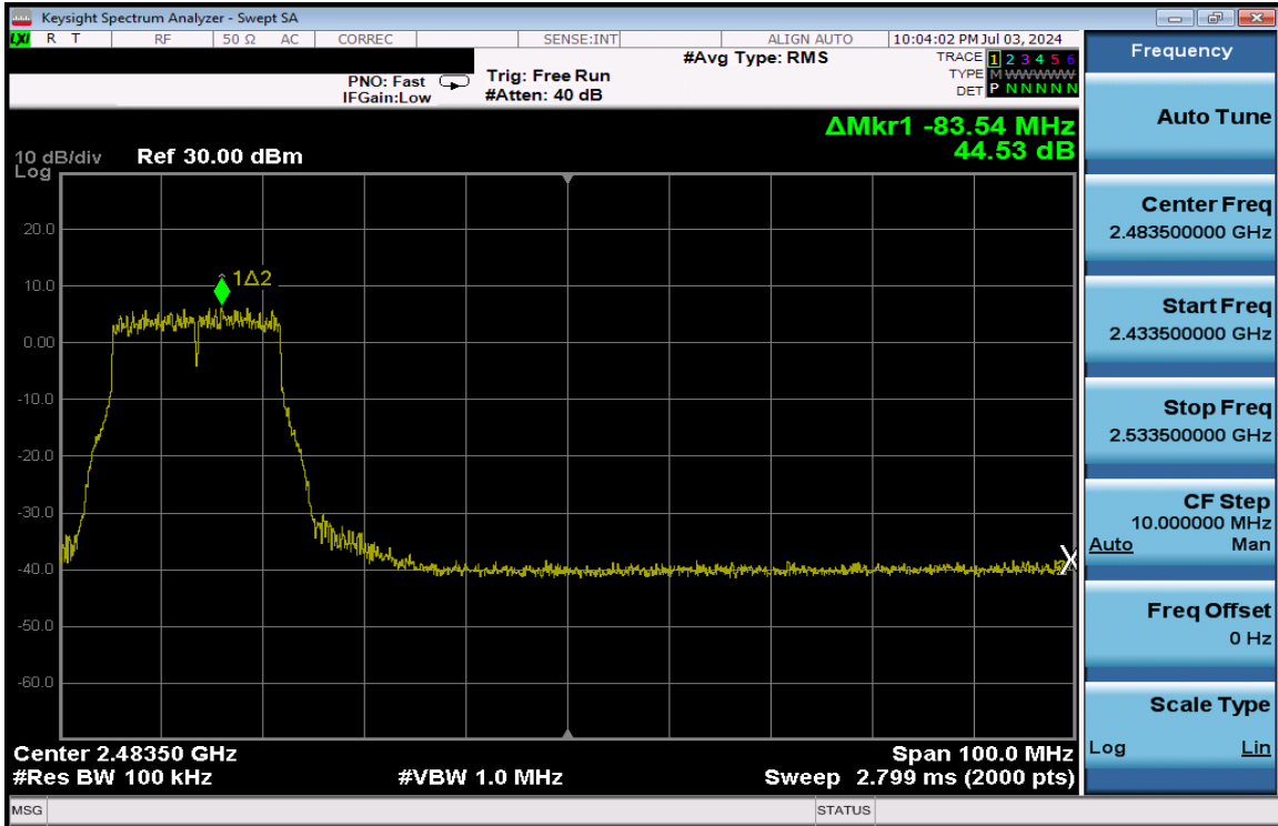
Plot 7-396. Band Edge Plot Antenna 1a (802.11g – Ch. 8) – 54Mbps
