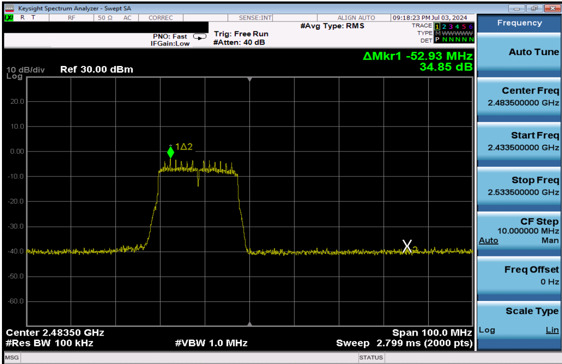
Plot 7-329. Band Edge Plot Antenna 1a (802.11n (2.4GHz) – Ch. 13) – MCS2
