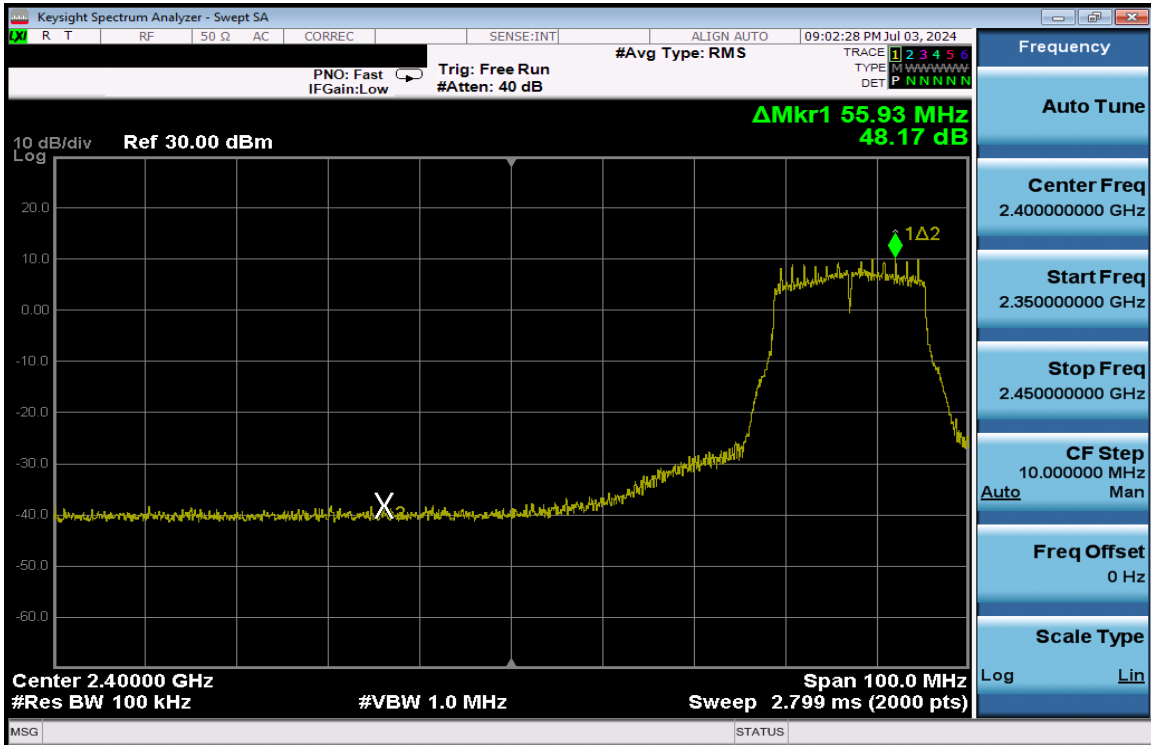
Plot 7-307. Band Edge Plot Antenna 1a (802.11g – Ch. 6 Low) – 12Mbps
