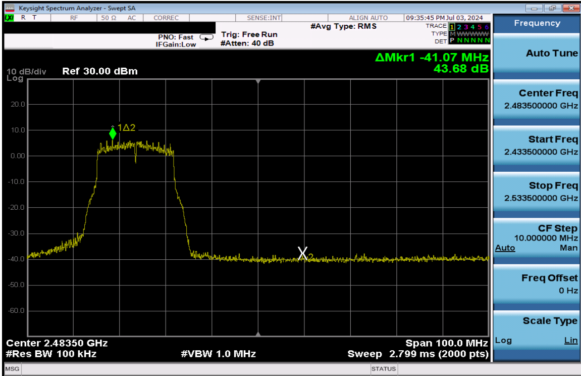
Plot 7-353. Band Edge Plot Antenna 1a (802.11g – Ch. 10) – 24Mbps
