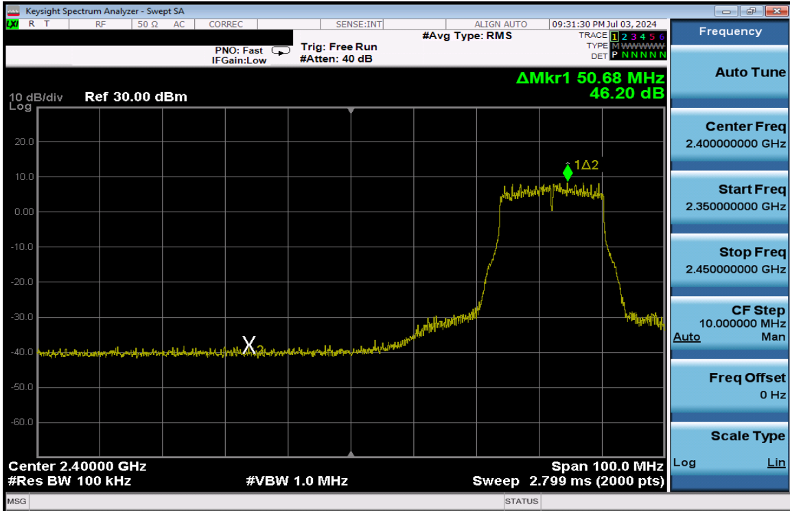
Plot 7-347. Band Edge Plot Antenna 1a (802.11g – Ch. 5) – 24Mbps
