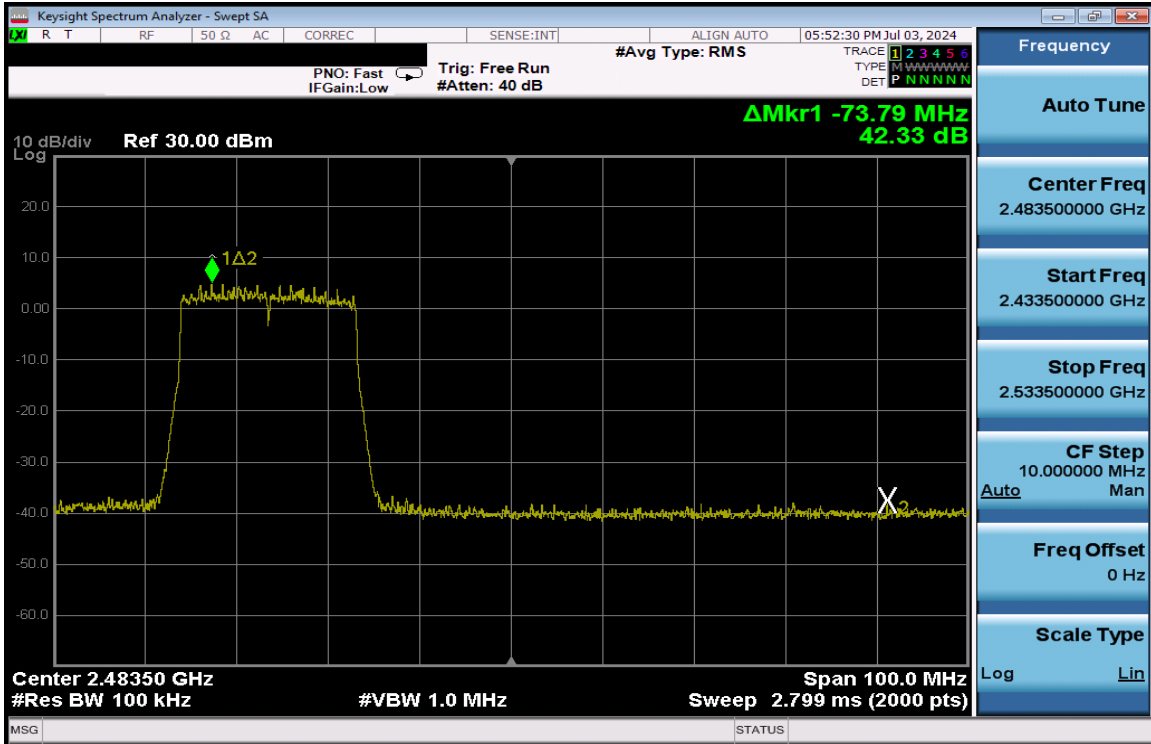
Plot 7-299. Band Edge Plot Antenna 3a (802.11ax (SU - 2.4GHz) – Ch. 10) – MCS9
