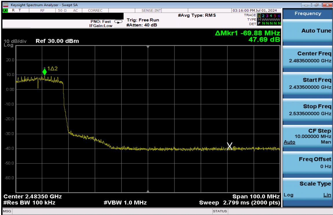
Plot 7-337. Band Edge Plot Antenna 1a (802.11ax (SU - 2.4GHz) – Ch. 7) – MCS2
