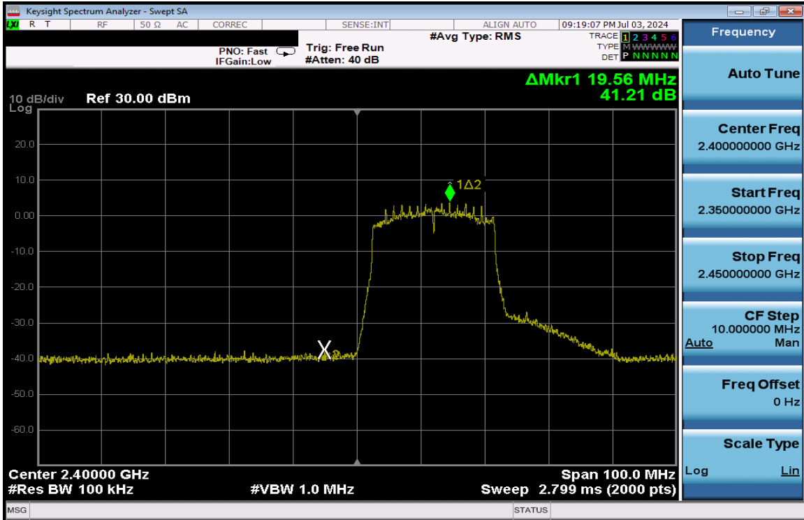
Plot 7-330. Band Edge Plot Antenna 1a (802.11ax (SU - 2.4GHz) – Ch. 1) – MCS2
