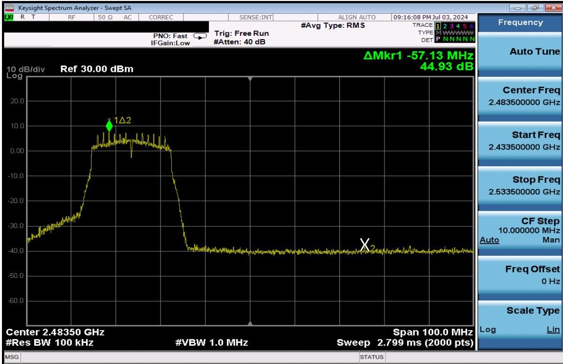
Plot 7-326. Band Edge Plot Antenna 1a (802.11n (2.4GHz) – Ch. 10) – MCS2
