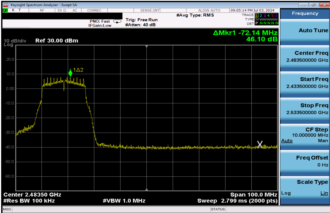
Plot 7-311. Band Edge Plot Antenna 1a (802.11g – Ch. 9) – 12Mbps
