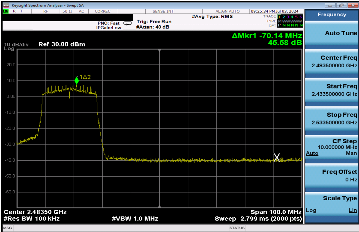
Plot 7-339. Band Edge Plot Antenna 1a (802.11ax (SU - 2.4GHz) – Ch. 9) – MCS2
