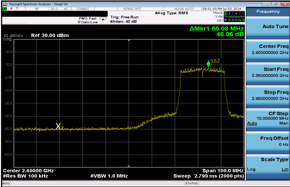
Plot 7-375. Band Edge Plot Antenna 1a (802.11ax (SU - 2.4GHz) – Ch. 5) – MCS4
