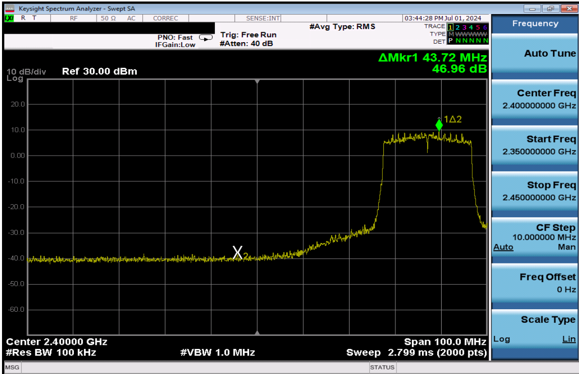
Plot 7-376. Band Edge Plot Antenna 1a (802.11ax (SU - 2.4GHz) – Ch. 6 Low) – MCS4
