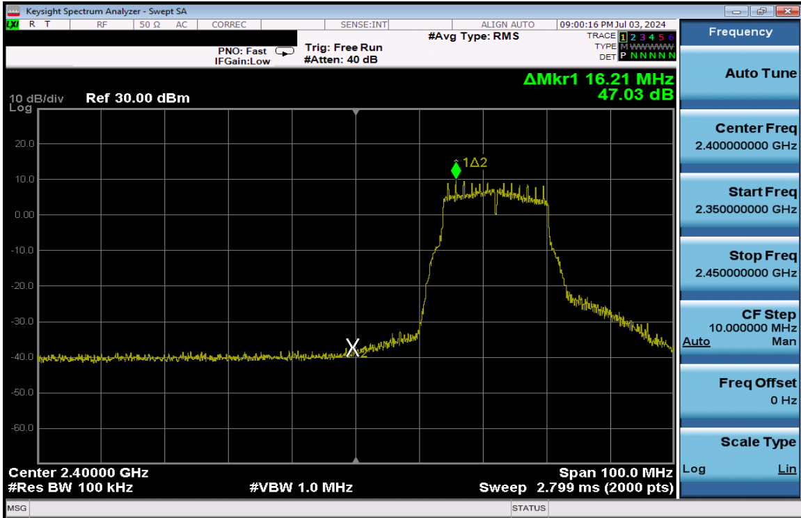
Plot 7-304. Band Edge Plot Antenna 1a (802.11g – Ch. 3) – 12Mbps
