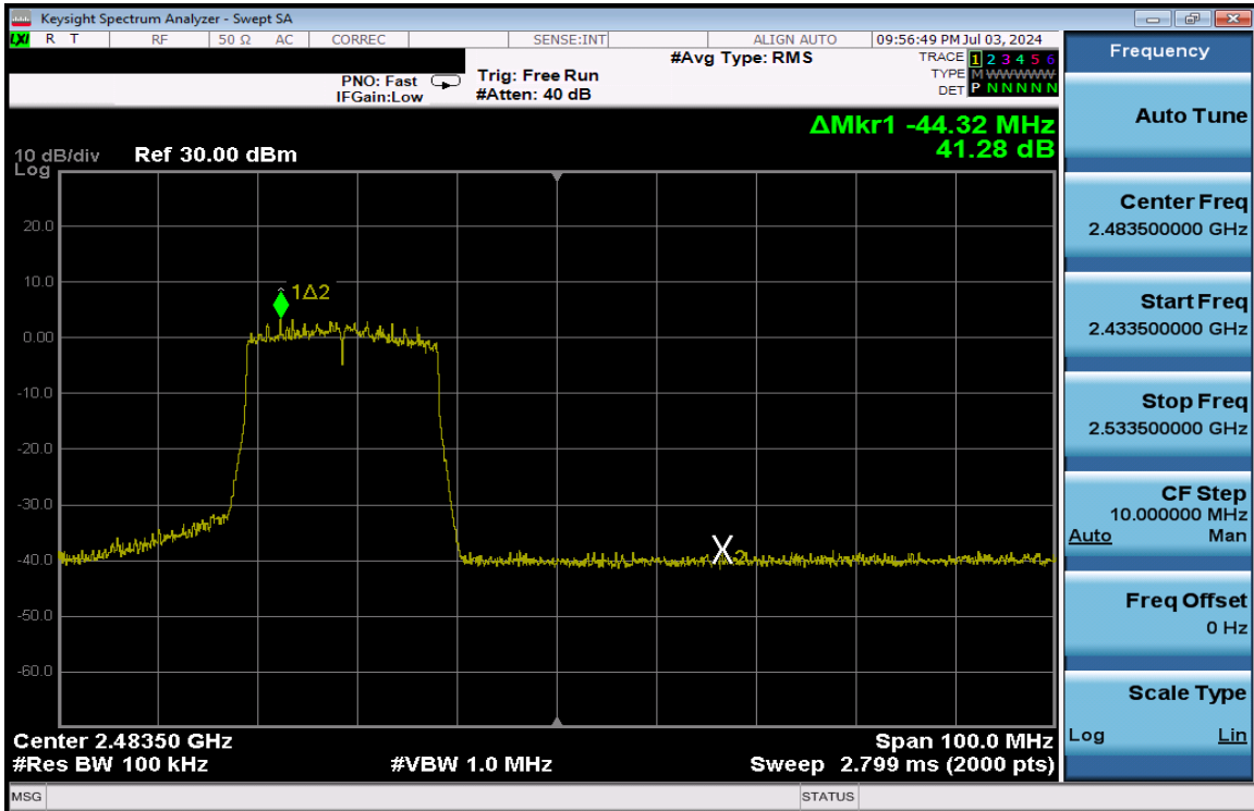
Plot 7-382. Band Edge Plot Antenna 1a (802.11ax (SU - 2.4GHz) – Ch. 11) – MCS4
