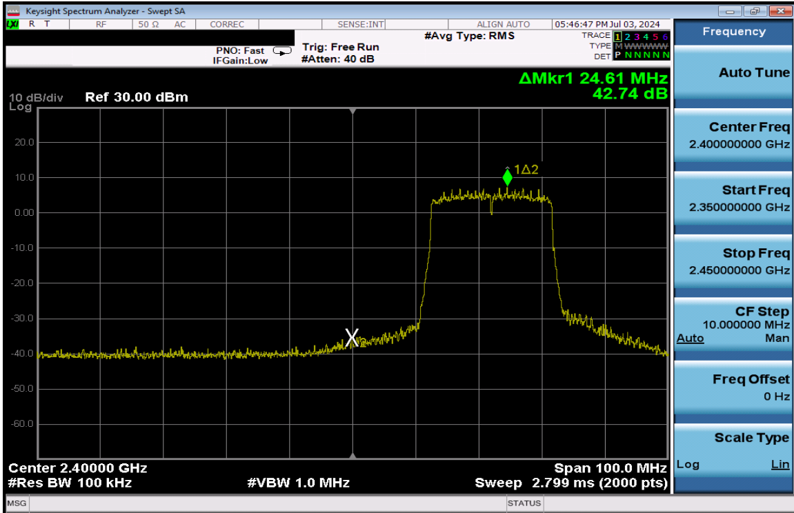
Plot 7-291. Band Edge Plot Antenna 3a (802.11ax (SU - 2.4GHz) – Ch. 3) – MCS9
