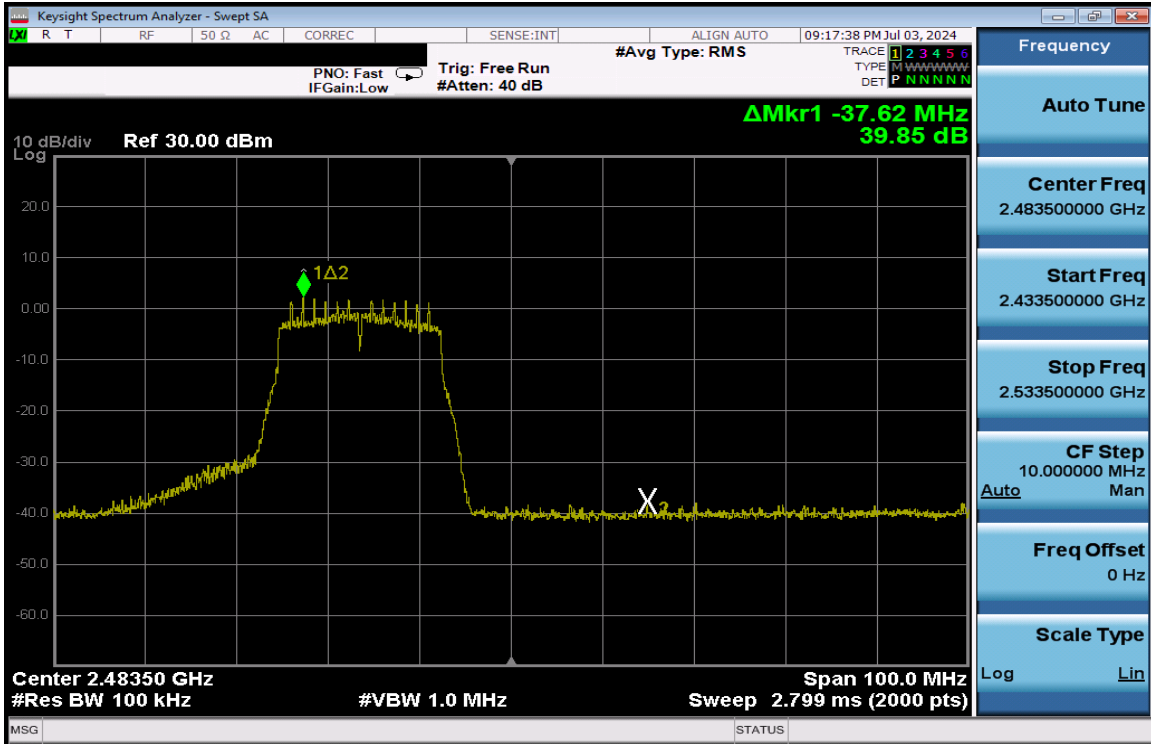
Plot 7-328. Band Edge Plot Antenna 1a (802.11n (2.4GHz) – Ch. 12) – MCS2
