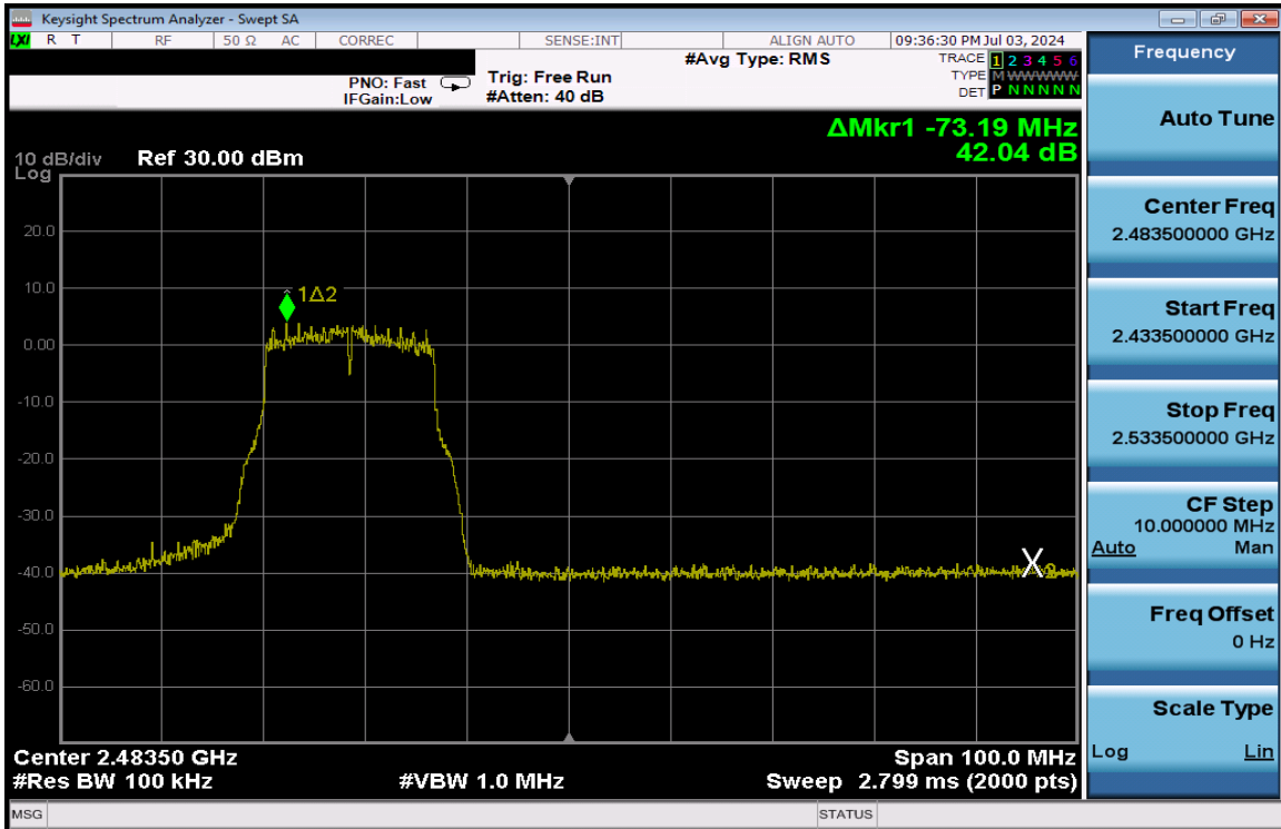
Plot 7-354. Band Edge Plot Antenna 1a (802.11g – Ch. 11) – 24Mbps
