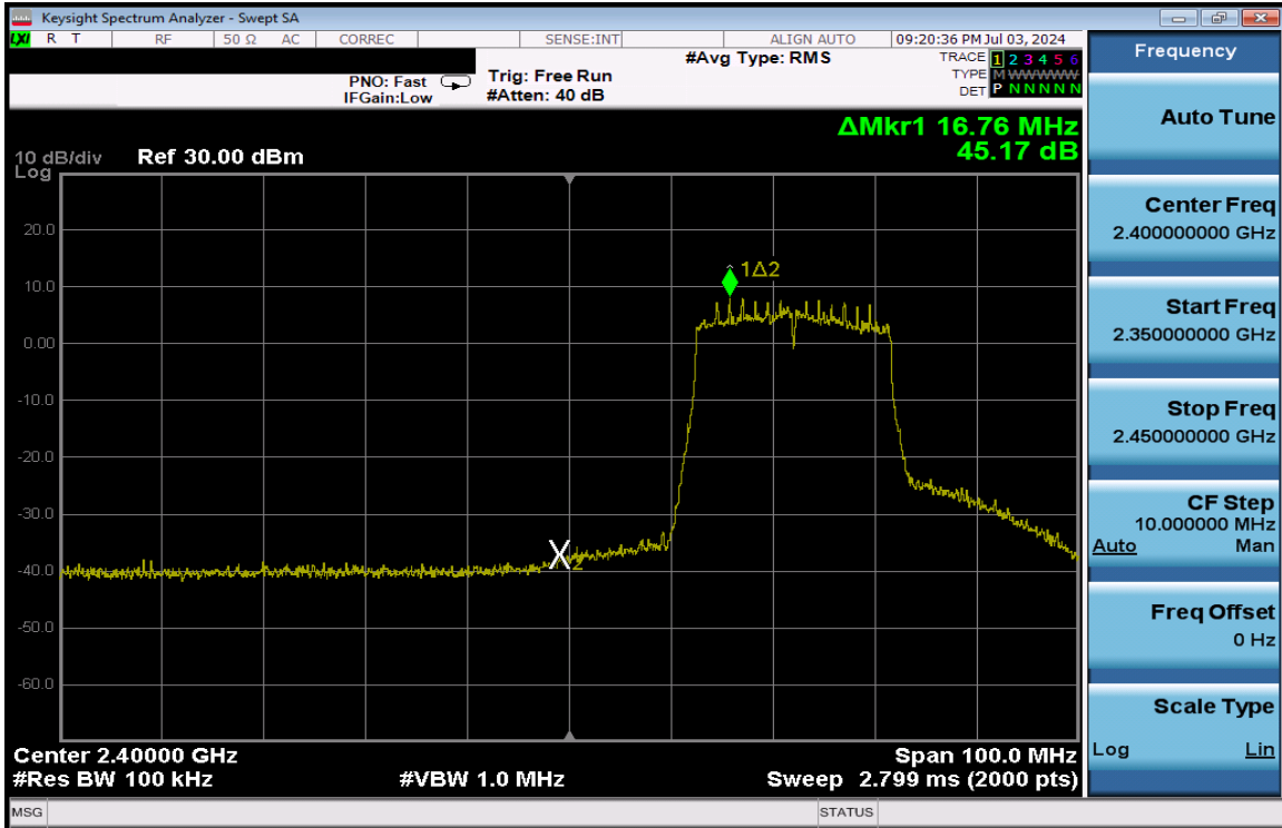
Plot 7-332. Band Edge Plot Antenna 1a (802.11ax (SU - 2.4GHz) – Ch. 3) – MCS2
