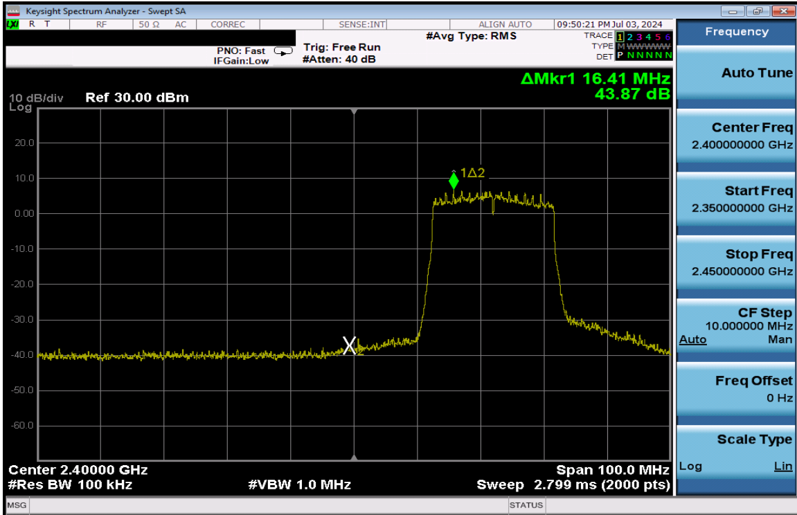
Plot 7-373. Band Edge Plot Antenna 1a (802.11ax (SU - 2.4GHz) – Ch. 3) – MCS4
