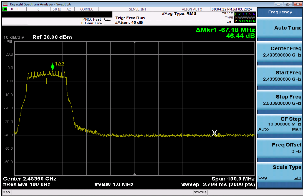
Plot 7-310. Band Edge Plot Antenna 1a (802.11g – Ch. 8) – 12Mbps
