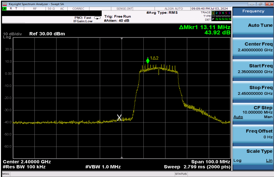
Plot 7-317. Band Edge Plot Antenna 1a (802.11n (2.4GHz) – Ch. 2) – MCS2
