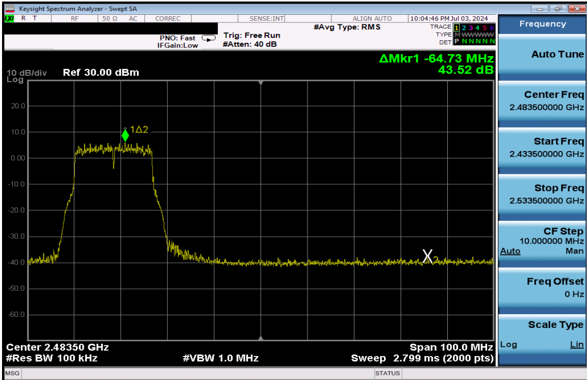
Plot 7-397. Band Edge Plot Antenna 1a (802.11g – Ch. 9) – 54Mbps
