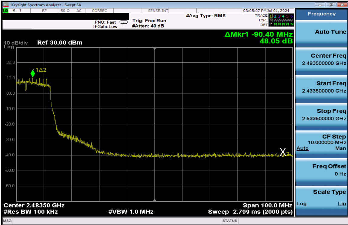
Plot 7-322. Band Edge Plot Antenna 1a (802.11n (2.4GHz) - Ch. 6 High) - MCS2
