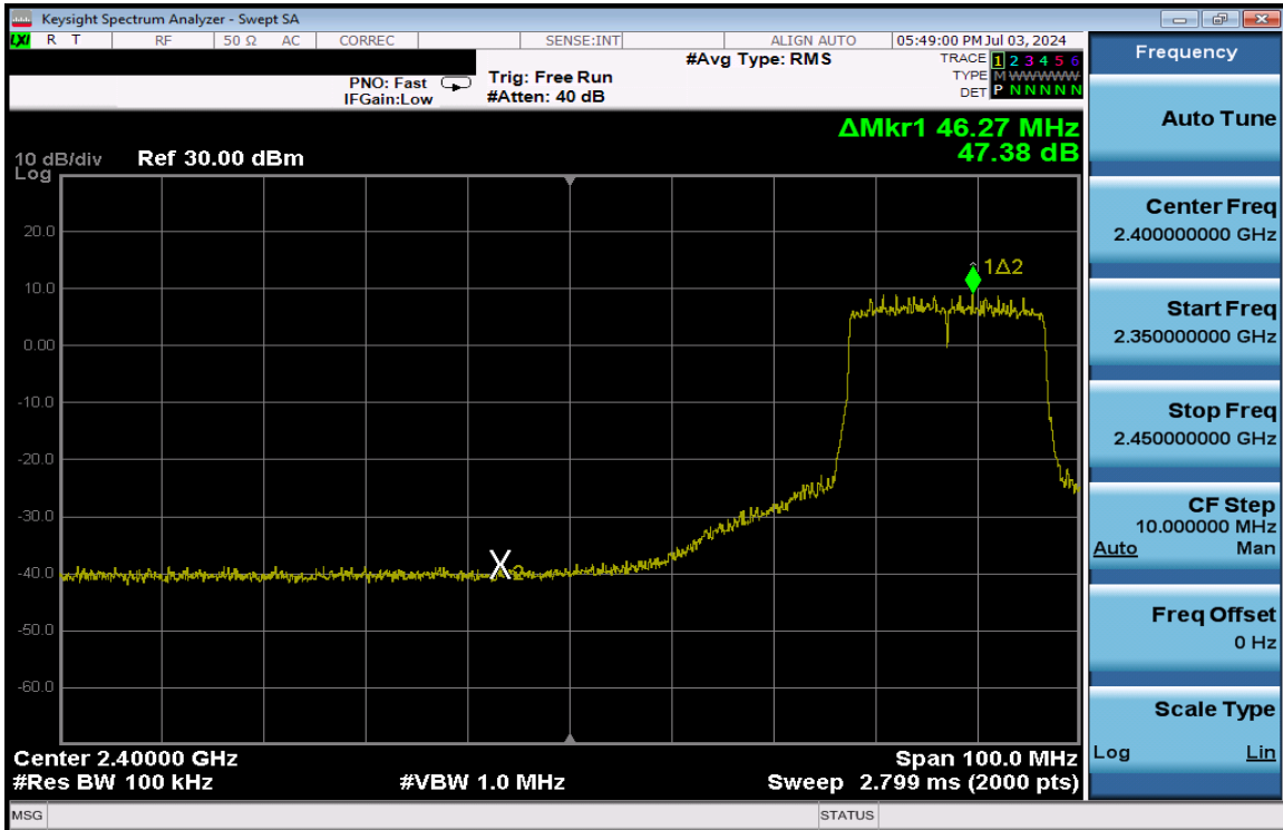
Plot 7-294. Band Edge Plot Antenna 3a (802.11ax (SU - 2.4GHz) – Ch. 6 Low) – MCS9
