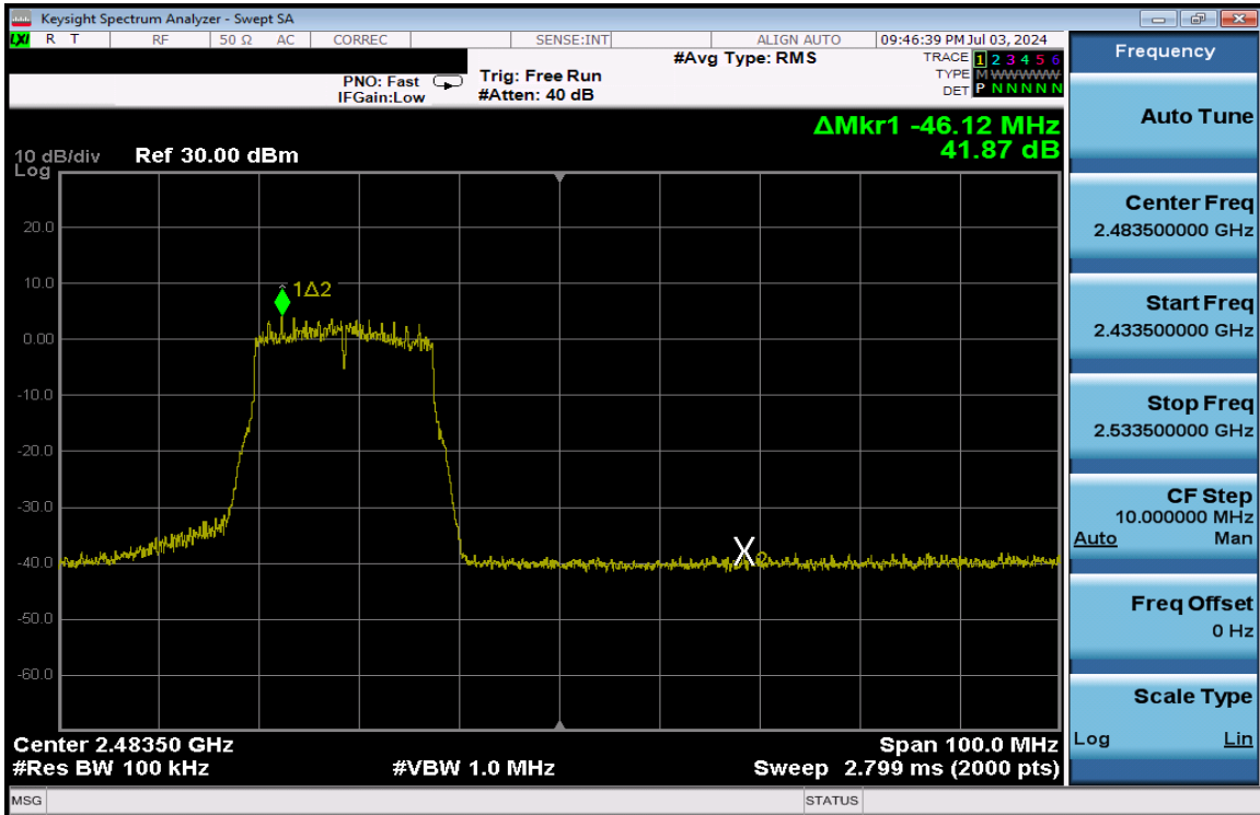
Plot 7-368. Band Edge Plot Antenna 1a (802.11n (2.4GHz) – Ch. 11) – MCS4
