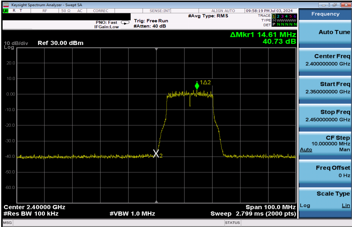
Plot 7-388. Band Edge Plot Antenna 1a (802.11g – Ch. 1) – 54Mbps
