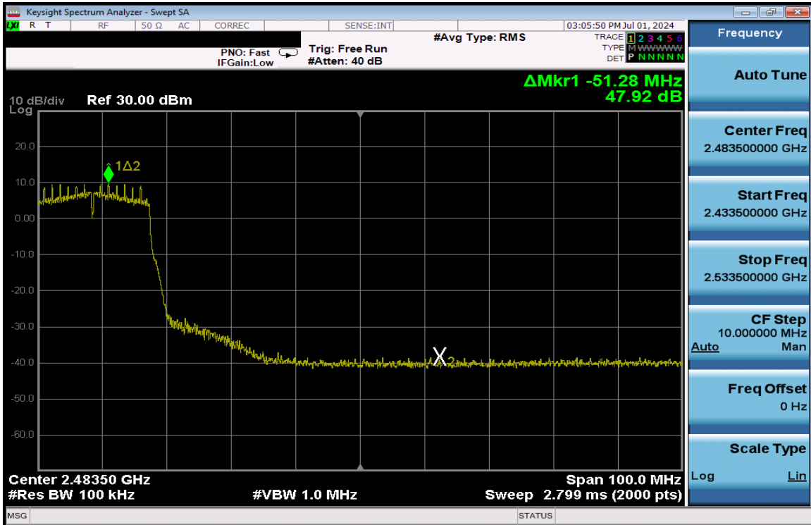
Plot 7-323. Band Edge Plot Antenna 1a (802.11n (2.4GHz) - Ch. 7) - MCS2
