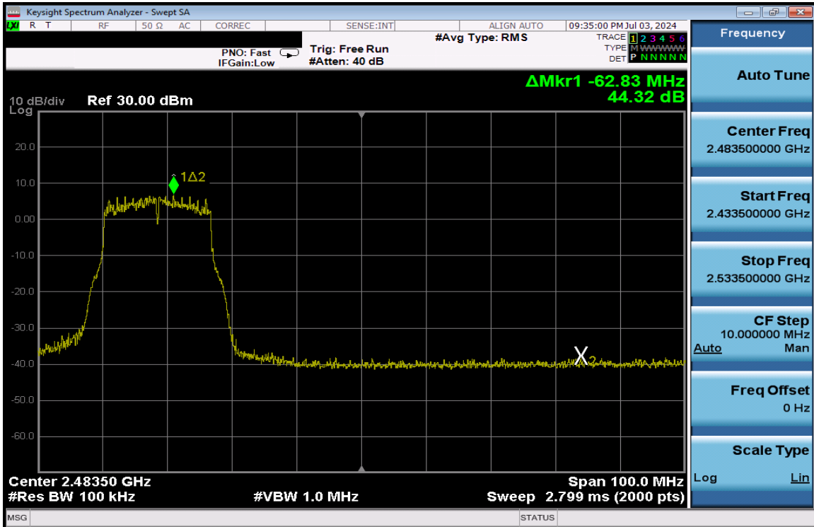
Plot 7-352. Band Edge Plot Antenna 1a (802.11g – Ch. 9) – 24Mbps
