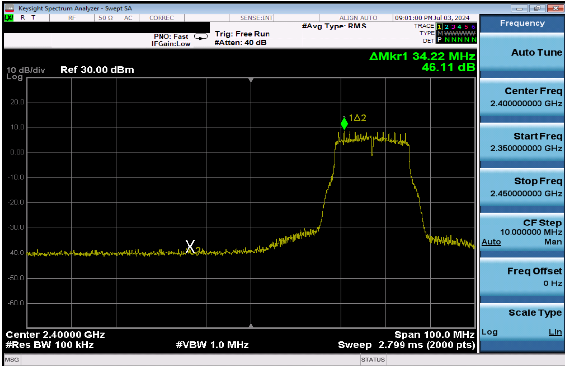
Plot 7-305. Band Edge Plot Antenna 1a (802.11g – Ch. 4) – 12Mbps
