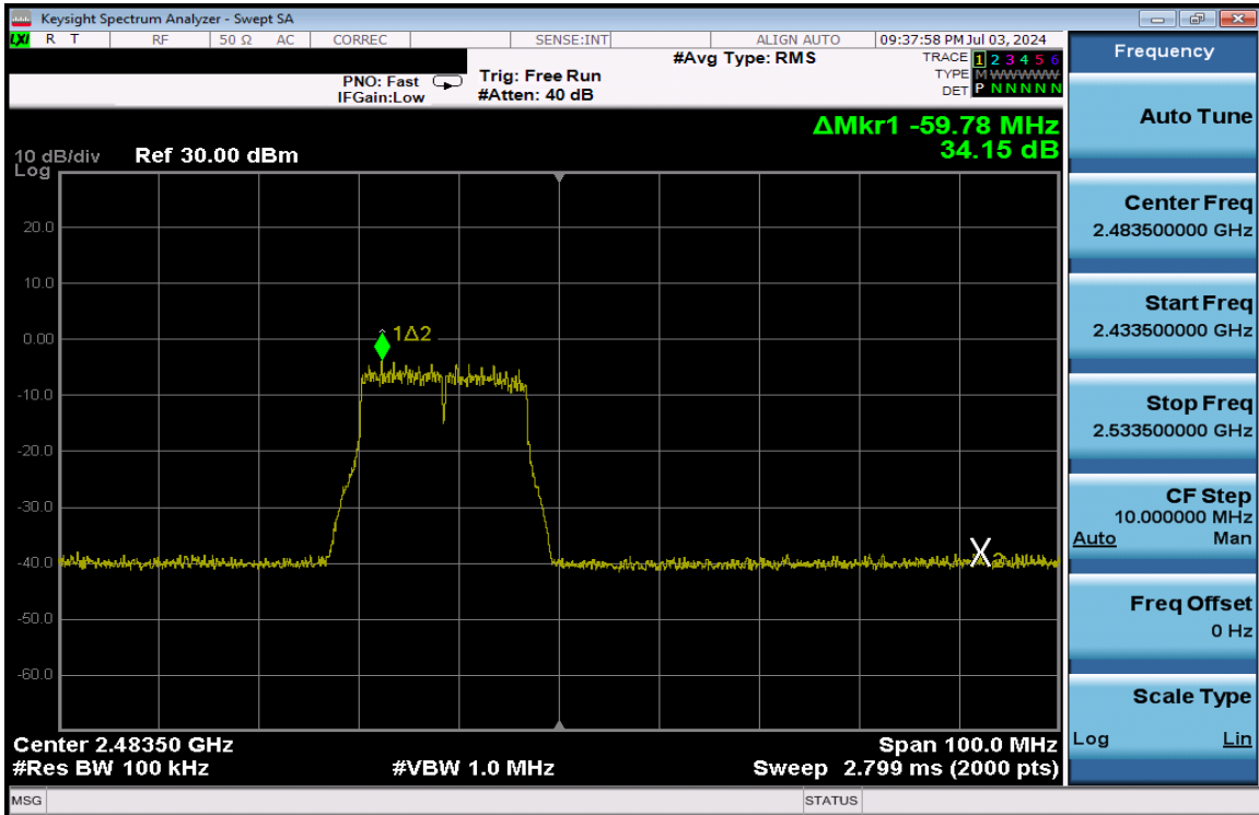
Plot 7-356. Band Edge Plot Antenna 1a (802.11g – Ch. 13) – 24Mbps
