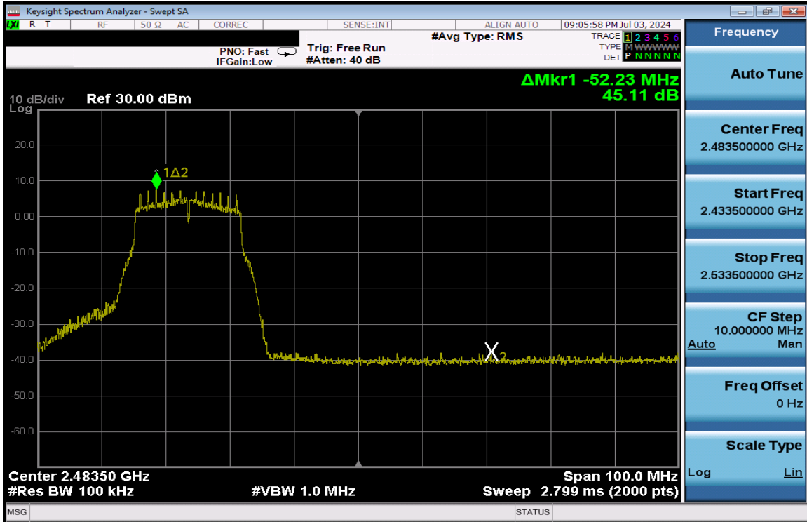
Plot 7-312. Band Edge Plot Antenna 1a (802.11g – Ch. 10) – 12Mbps
