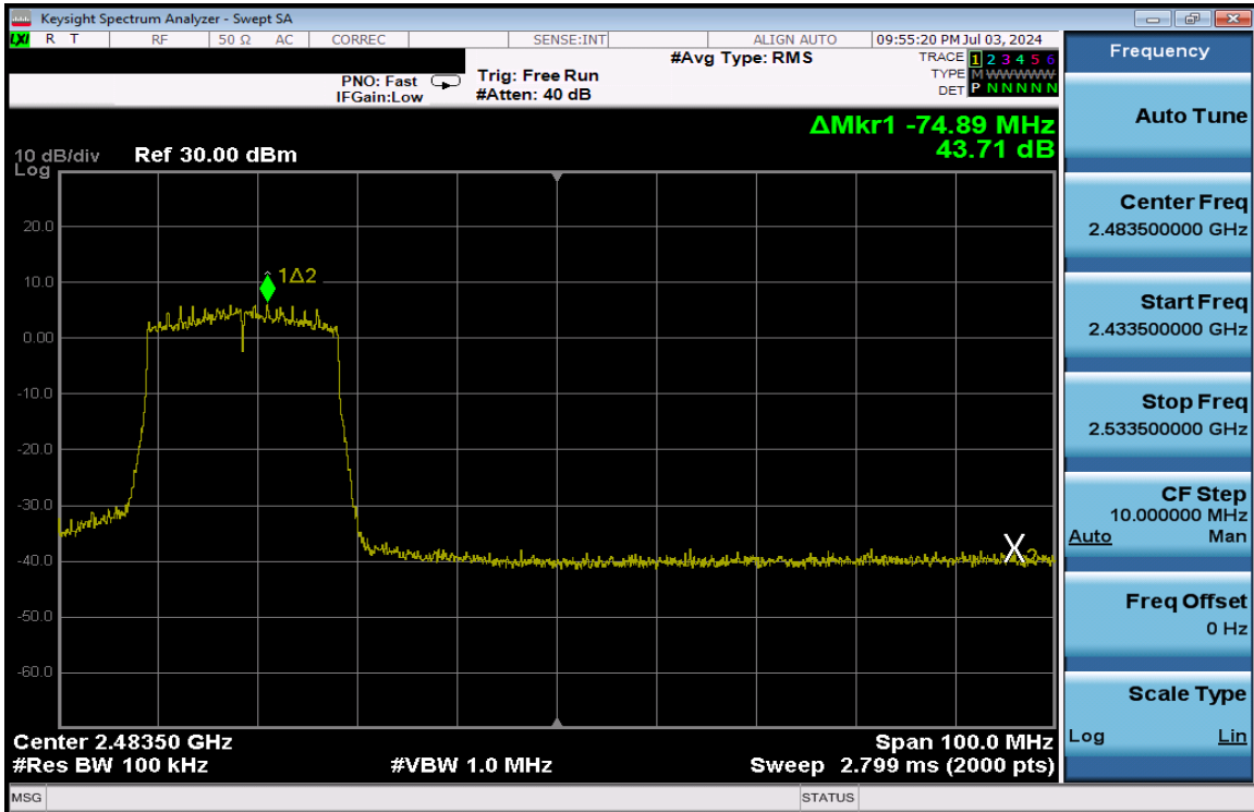
Plot 7-380. Band Edge Plot Antenna 1a (802.11ax (SU - 2.4GHz) – Ch. 9) – MCS4
