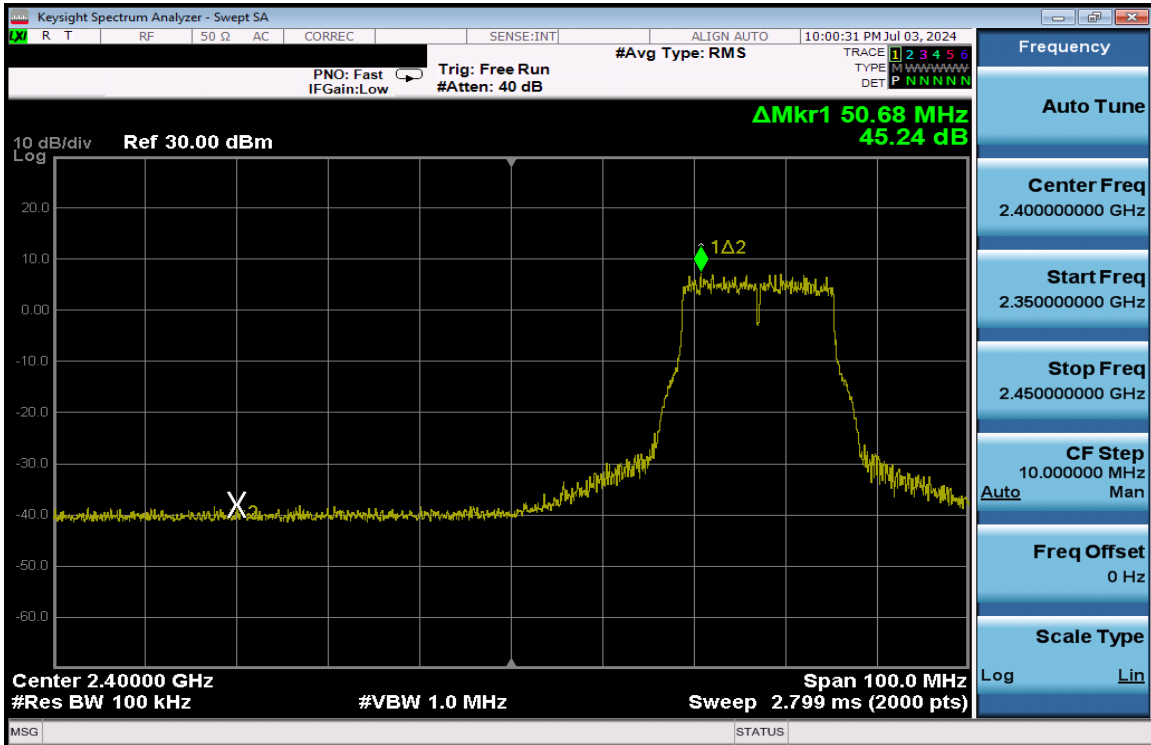
Plot 7-391. Band Edge Plot Antenna 1a (802.11g – Ch. 4) – 54Mbps
