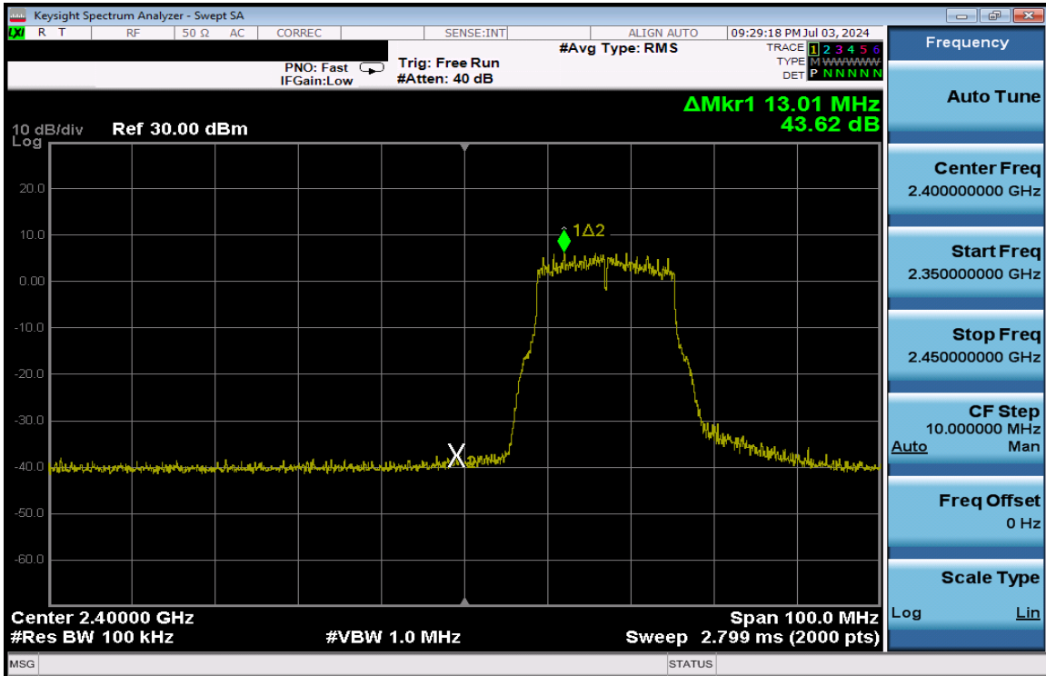
Plot 7-344. Band Edge Plot Antenna 1a (802.11g – Ch. 2) – 24Mbps
