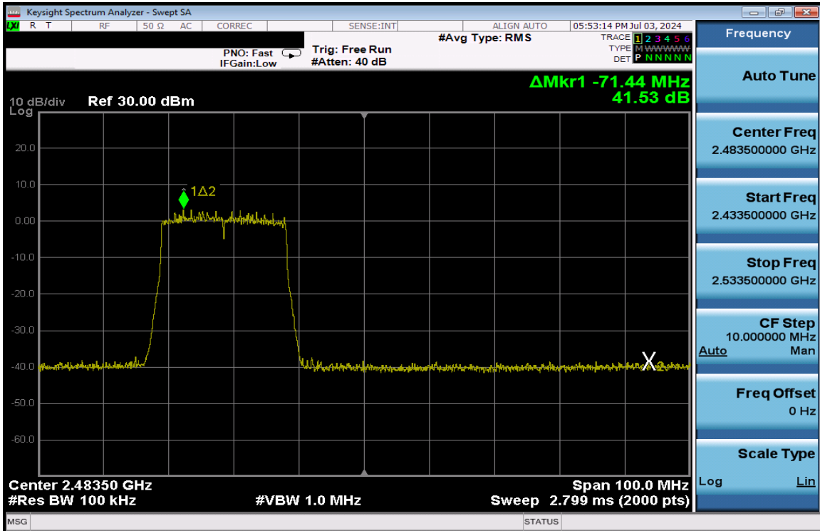
Plot 7-300. Band Edge Plot Antenna 3a (802.11ax (SU - 2.4GHz) – Ch. 11) – MCS9
