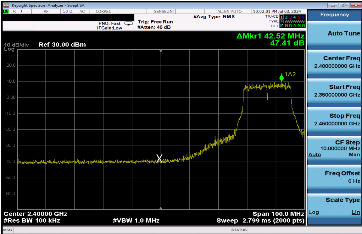
Plot 7-393. Band Edge Plot Antenna 1a (802.11g – Ch. 6 Low) – 54Mbps
