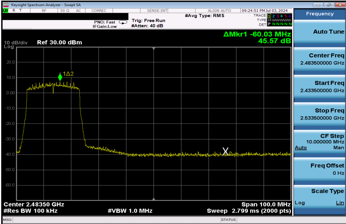
Plot 7-338. Band Edge Plot Antenna 1a (802.11ax (SU - 2.4GHz) – Ch. 8) – MCS2
