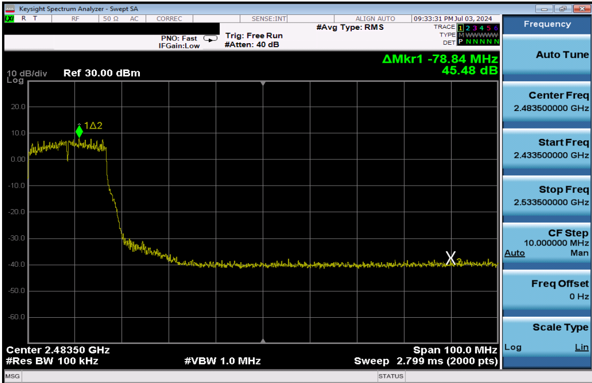
Plot 7-350. Band Edge Plot Antenna 1a (802.11g – Ch. 7) – 24Mbps
