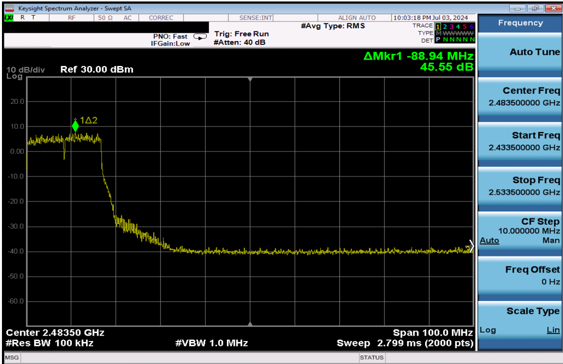
Plot 7-395. Band Edge Plot Antenna 1a (802.11g – Ch. 7) – 54Mbps
