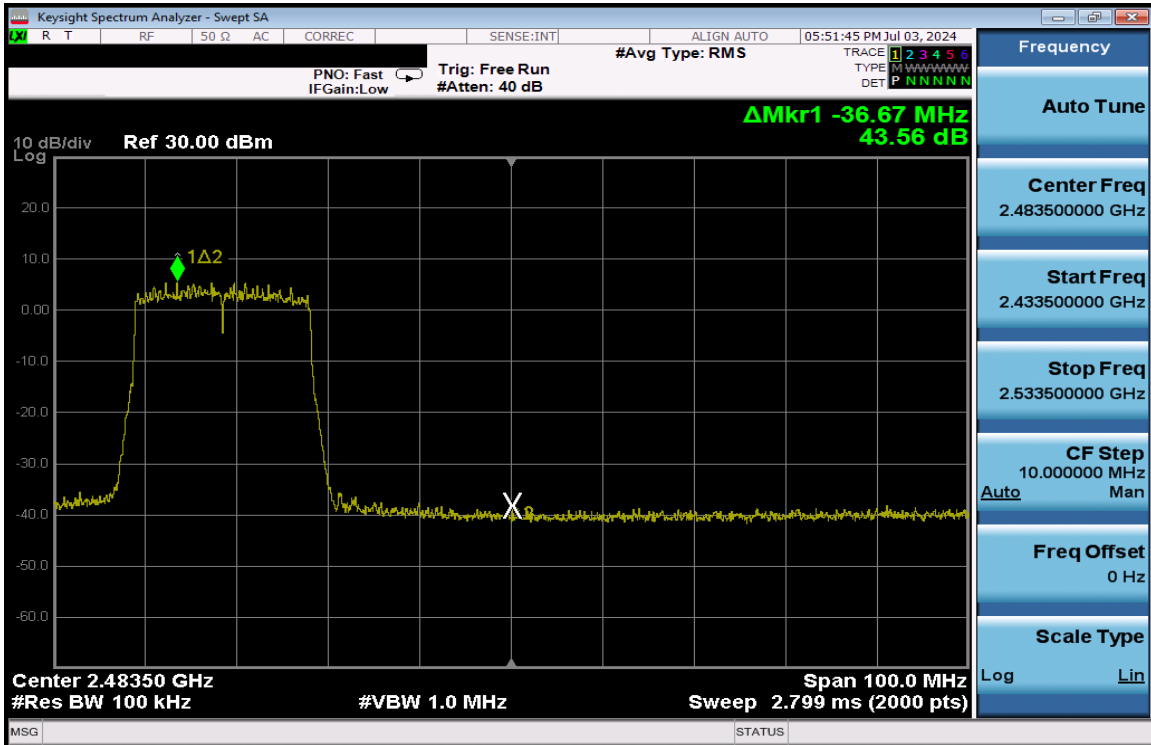
Plot 7-298. Band Edge Plot Antenna 3a (802.11ax (SU - 2.4GHz) – Ch. 9) – MCS9
