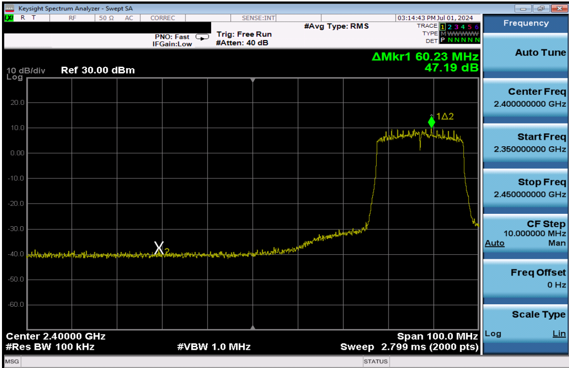
Plot 7-335. Band Edge Plot Antenna 1a (802.11ax (SU - 2.4GHz) – Ch. 6 Low) – MCS2
