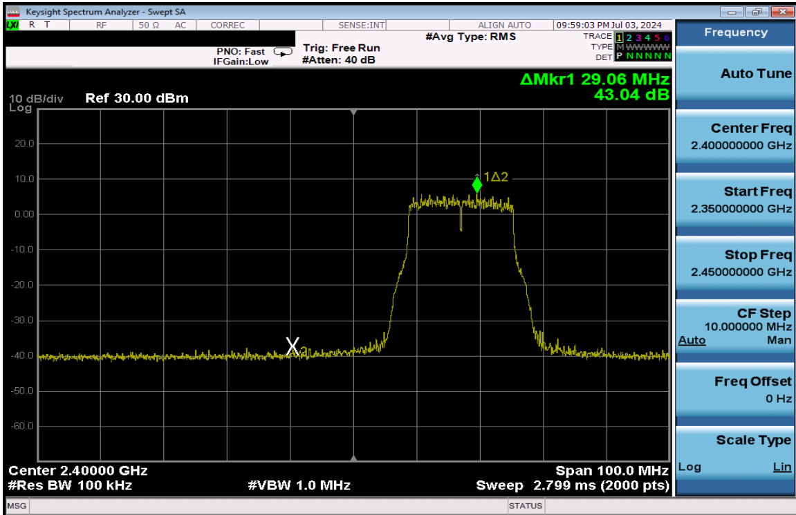
Plot 7-389. Band Edge Plot Antenna 1a (802.11g – Ch. 2) – 54Mbps
