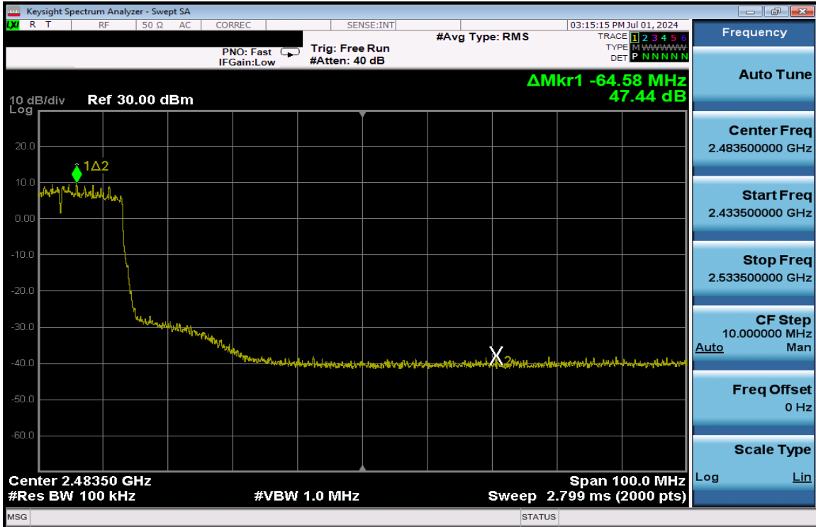
Plot 7-336. Band Edge Plot Antenna 1a (802.11ax (SU - 2.4GHz) – Ch. 6 High) – MCS2
