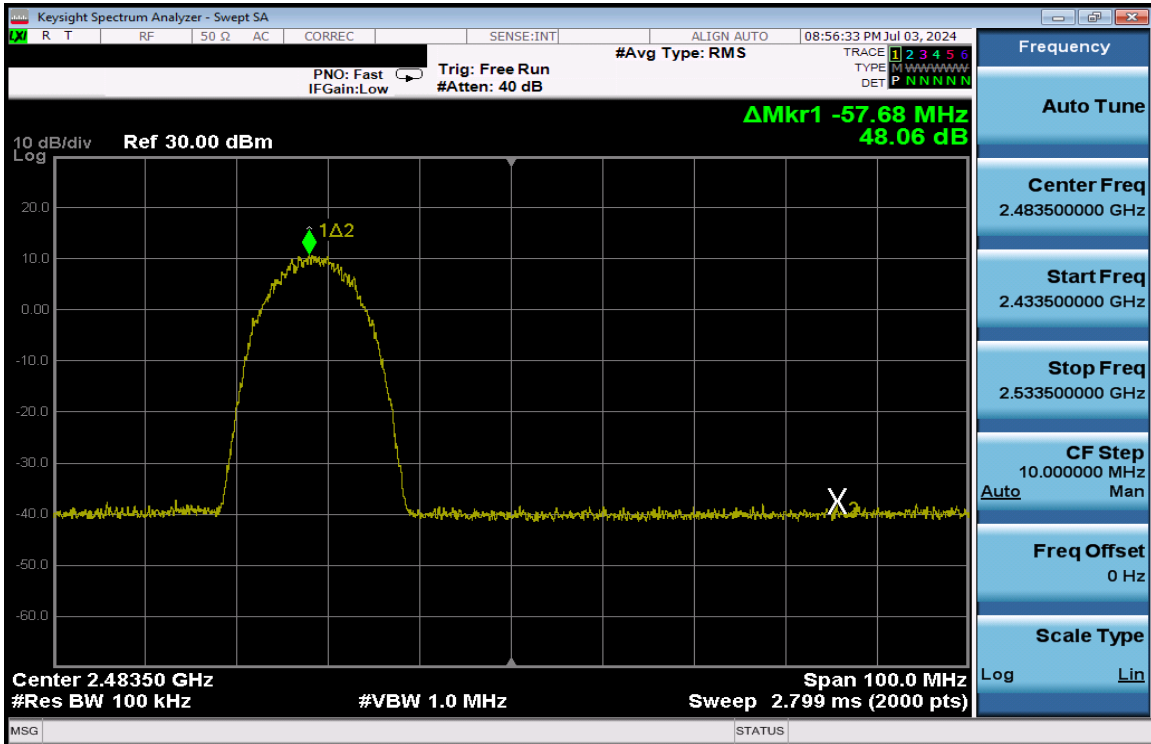
Plot 7-385. Band Edge Plot Antenna 1a (802.11b – Ch. 11) – 11Mbps
