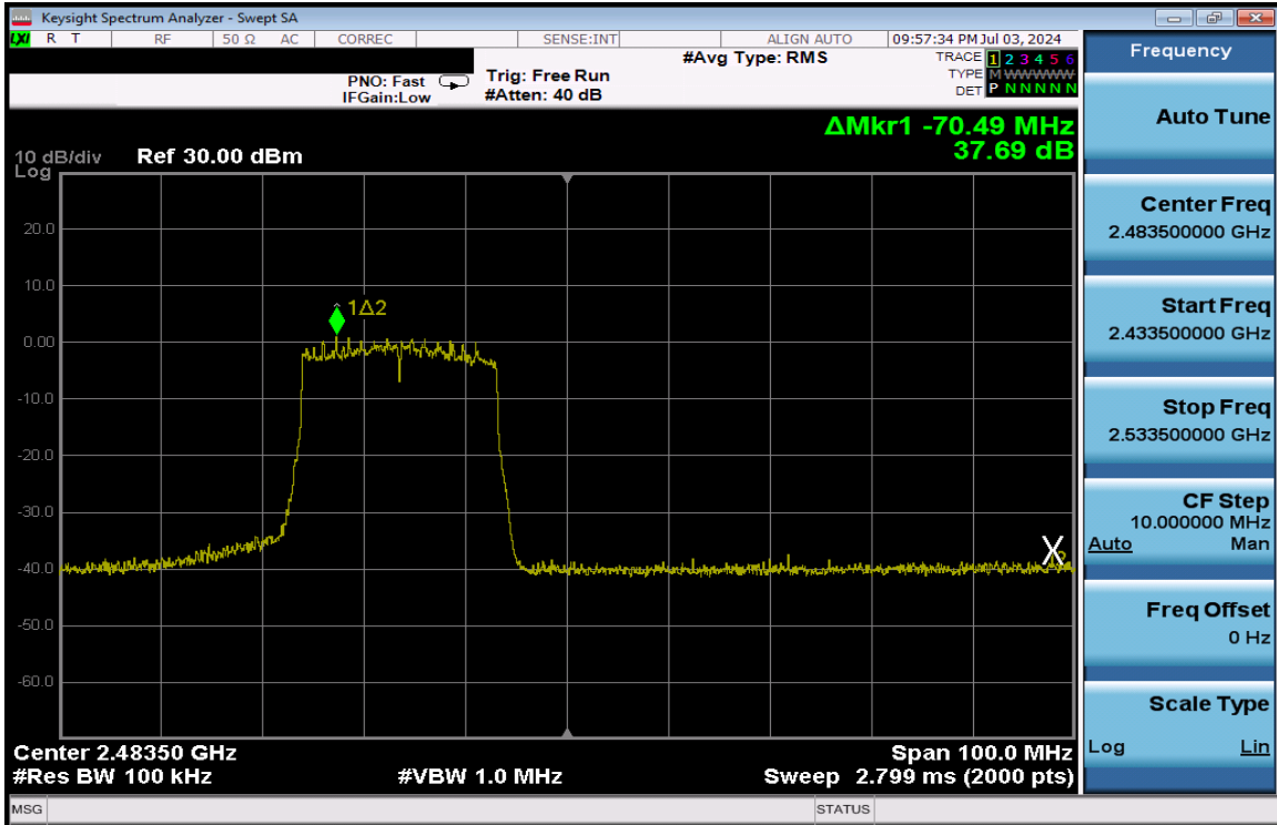
Plot 7-383. Band Edge Plot Antenna 1a (802.11ax (SU - 2.4GHz) – Ch. 12) – MCS4
