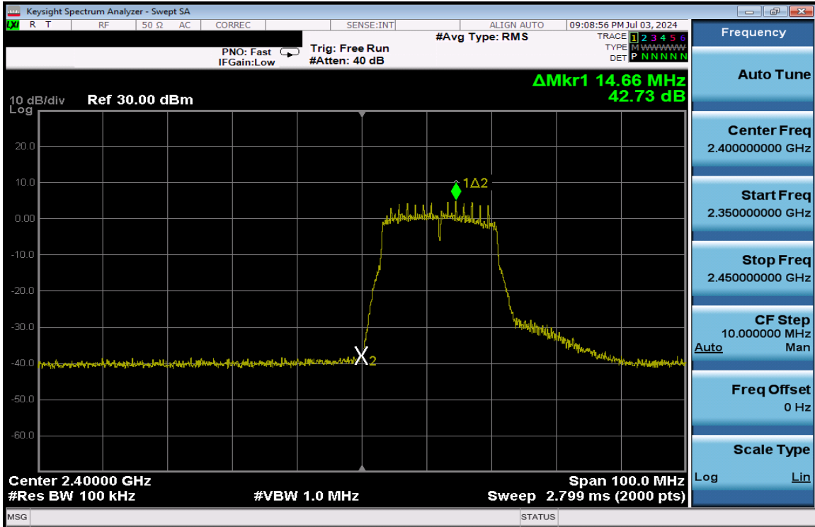
Plot 7-316. Band Edge Plot Antenna 1a (802.11n (2.4GHz) – Ch. 1) – MCS2
