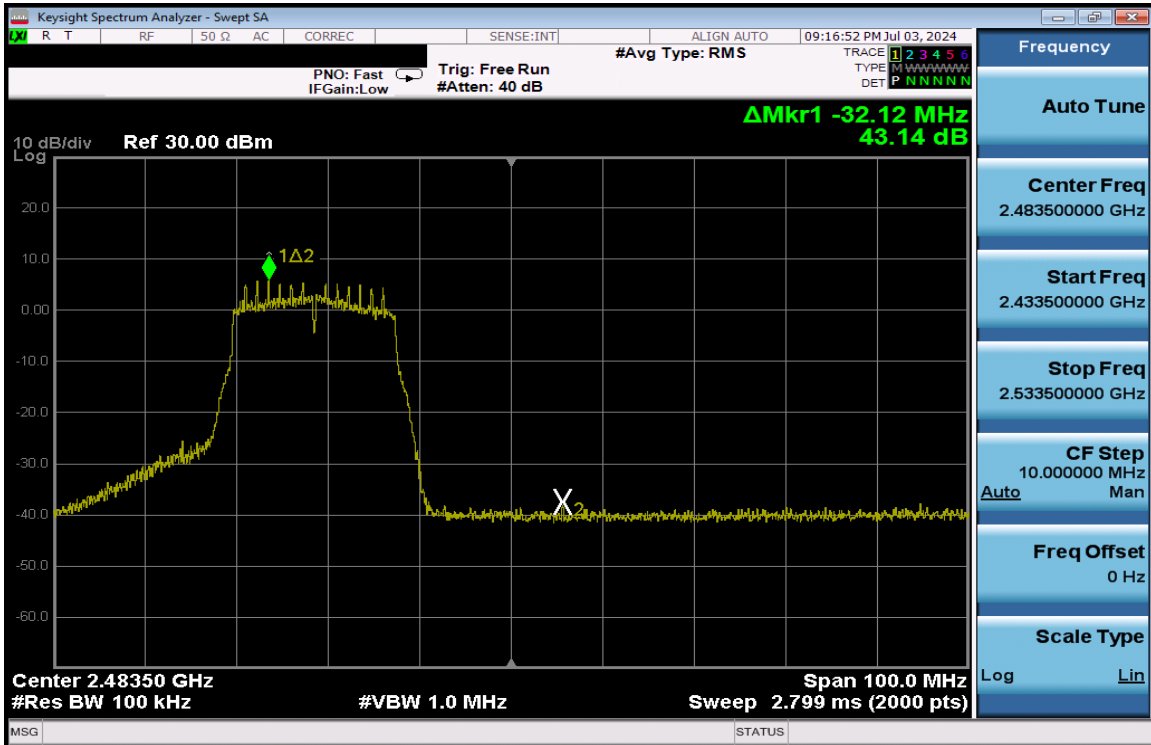
Plot 7-327. Band Edge Plot Antenna 1a (802.11n (2.4GHz) – Ch. 11) – MCS2
