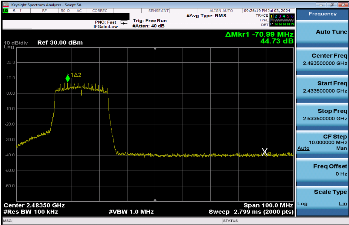
Plot 7-340. Band Edge Plot Antenna 1a (802.11ax (SU - 2.4GHz) – Ch. 10) – MCS2
