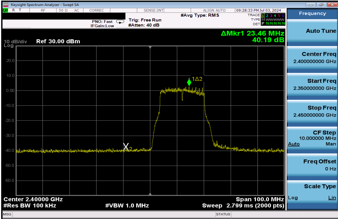
Plot 7-343. Band Edge Plot Antenna 1a (802.11g – Ch. 1) – 24Mbps
