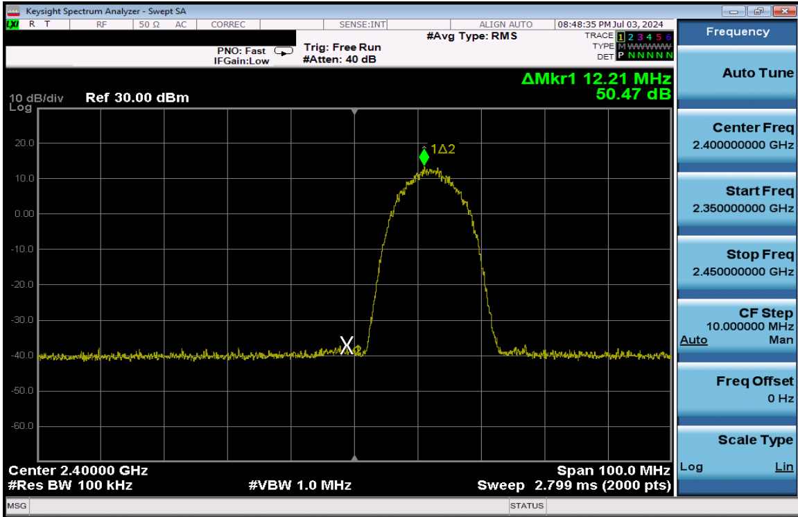
Plot 7-384. Band Edge Plot Antenna 1a (802.11b – Ch. 1) – 11Mbps
