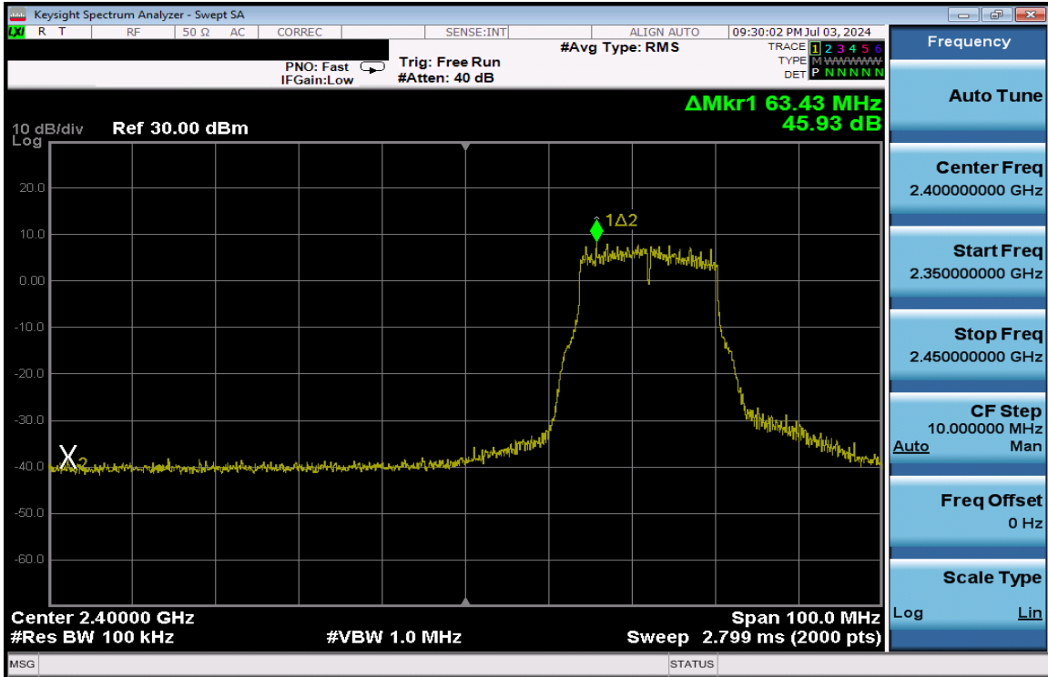
Plot 7-345. Band Edge Plot Antenna 1a (802.11g – Ch. 3) – 24Mbps
