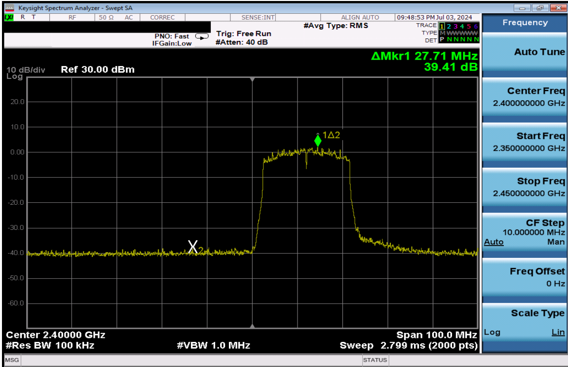
Plot 7-371. Band Edge Plot Antenna 1a (802.11ax (SU - 2.4GHz) – Ch. 1) – MCS4
