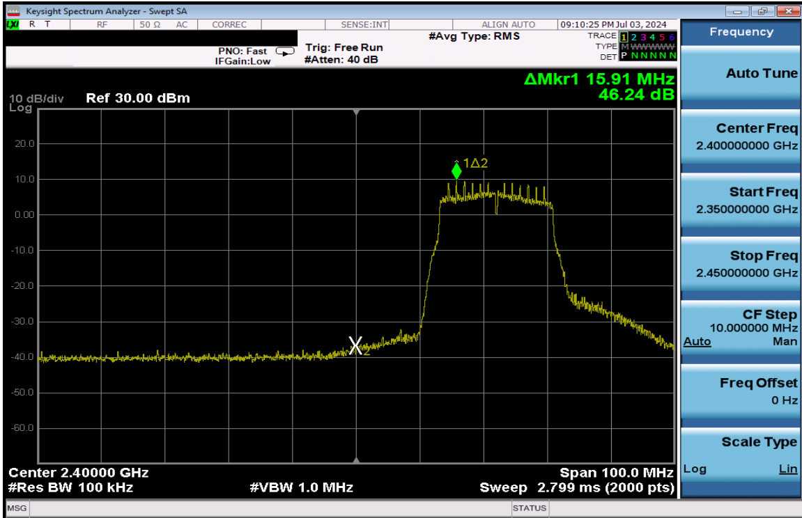
Plot 7-318. Band Edge Plot Antenna 1a (802.11n (2.4GHz) – Ch. 3) – MCS2
