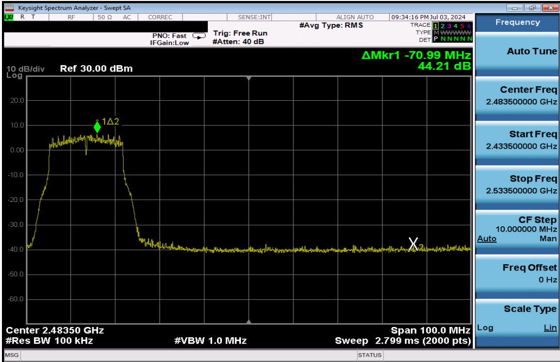
Plot 7-351. Band Edge Plot Antenna 1a (802.11g – Ch. 8) – 24Mbps
