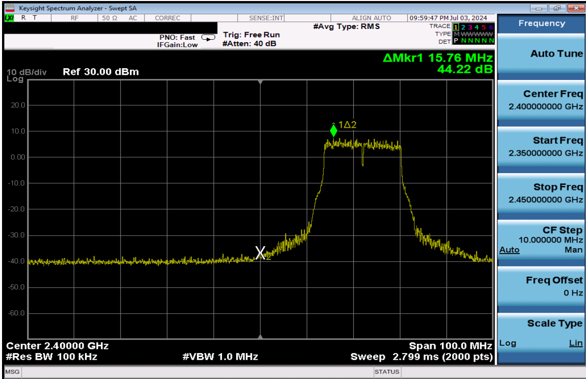
Plot 7-390. Band Edge Plot Antenna 1a (802.11g – Ch. 3) – 54Mbps
