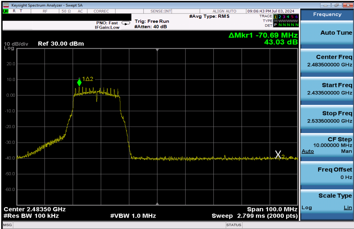
Plot 7-313. Band Edge Plot Antenna 1a (802.11g – Ch. 11) – 12Mbps
