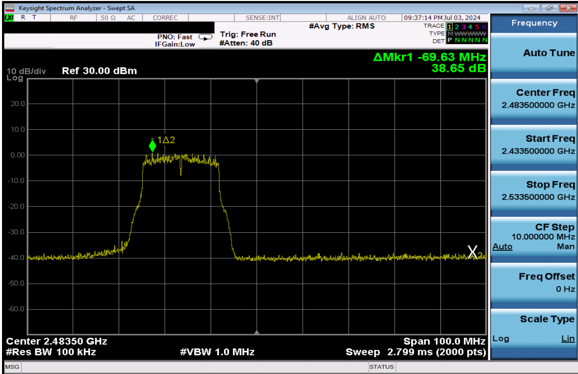
Plot 7-355. Band Edge Plot Antenna 1a (802.11g – Ch. 12) – 24Mbps
