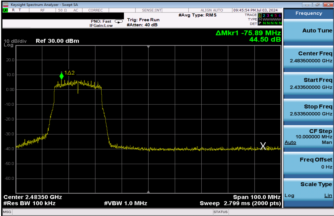
Plot 7-367. Band Edge Plot Antenna 1a (802.11n (2.4GHz) – Ch. 10) – MCS4
