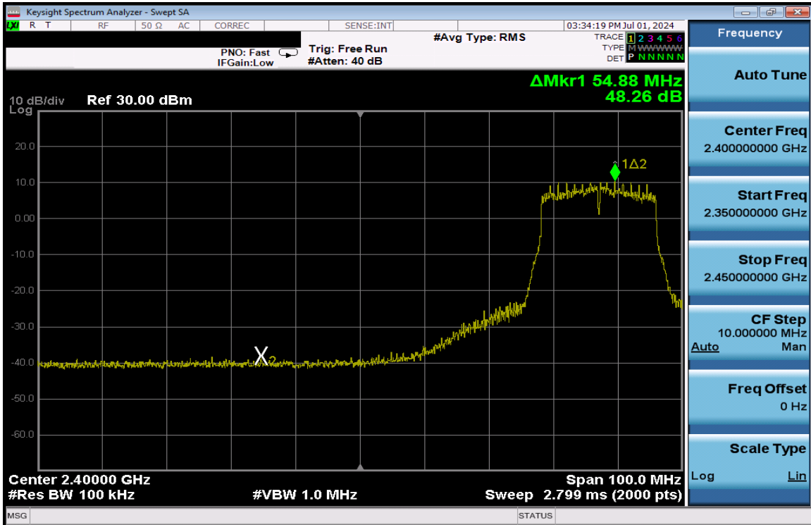
Plot 7-362. Band Edge Plot Antenna 1a (802.11n (2.4GHz) – Ch. 6 Low) – MCS4
