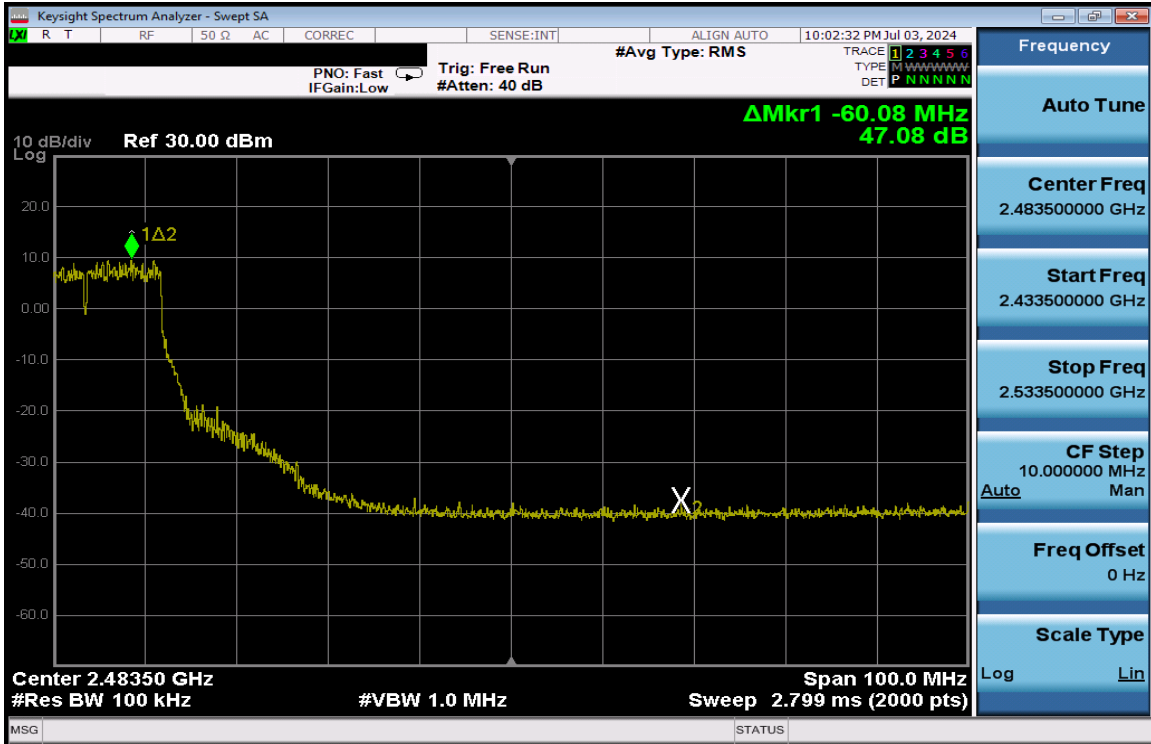
Plot 7-394. Band Edge Plot Antenna 1a (802.11g – Ch. 6 High) – 54Mbps
