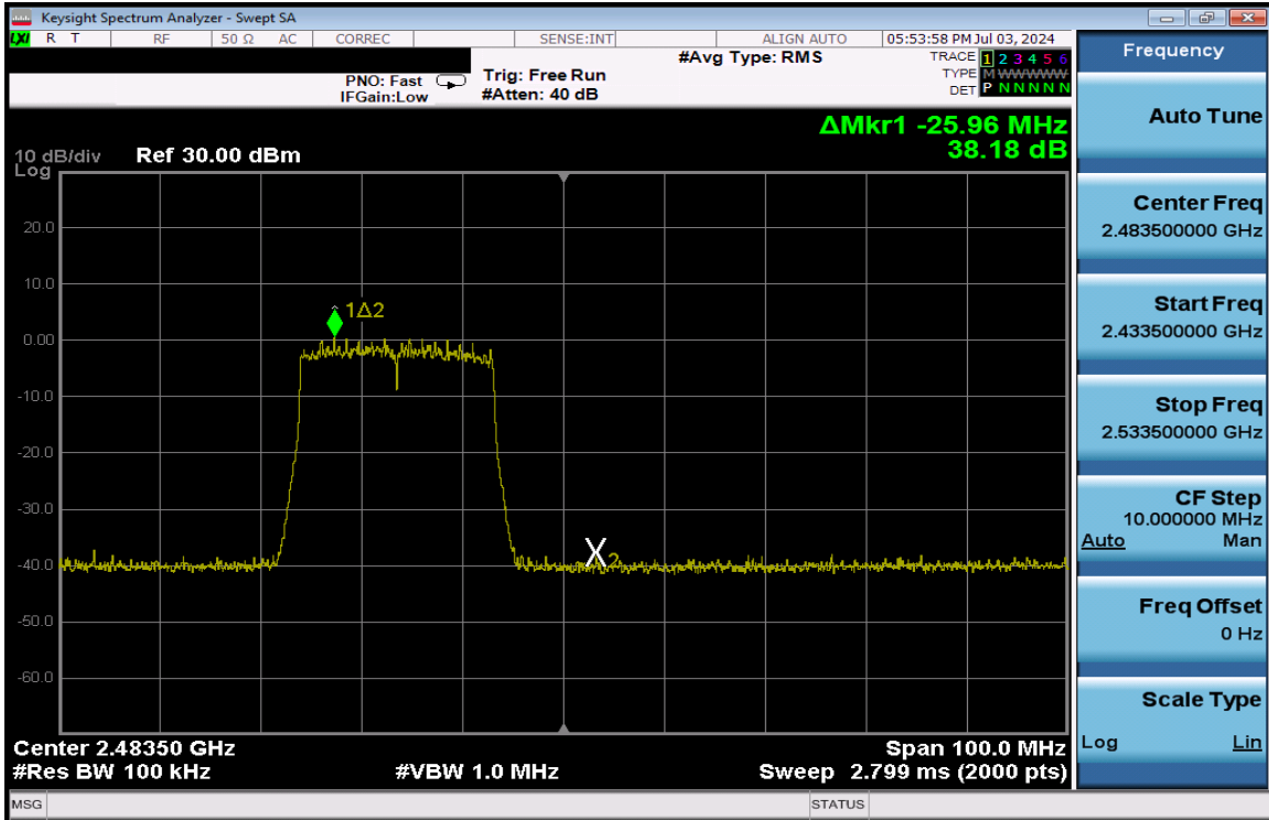
Plot 7-301. Band Edge Plot Antenna 3a (802.11ax (SU - 2.4GHz) – Ch. 12) – MCS9
