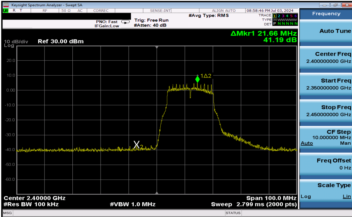
Plot 7-302. Band Edge Plot Antenna 1a (802.11g – Ch. 1) – 12Mbps
