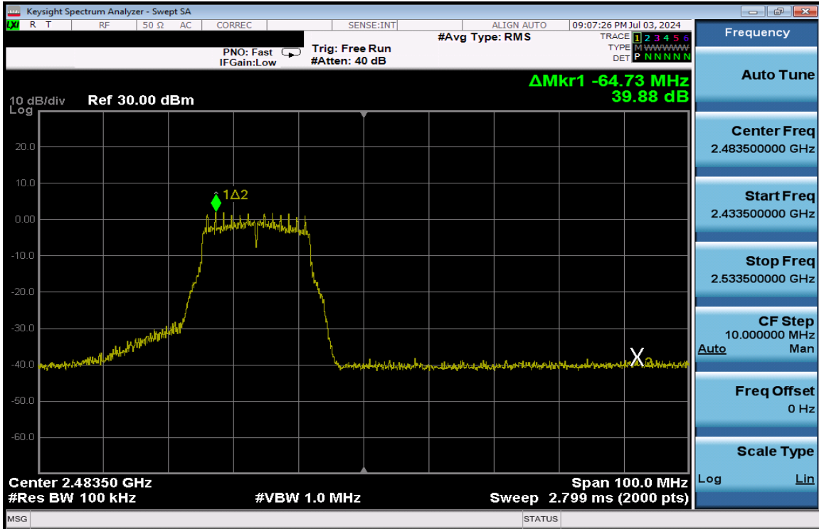
Plot 7-314. Band Edge Plot Antenna 1a (802.11g – Ch. 12) – 12Mbps
