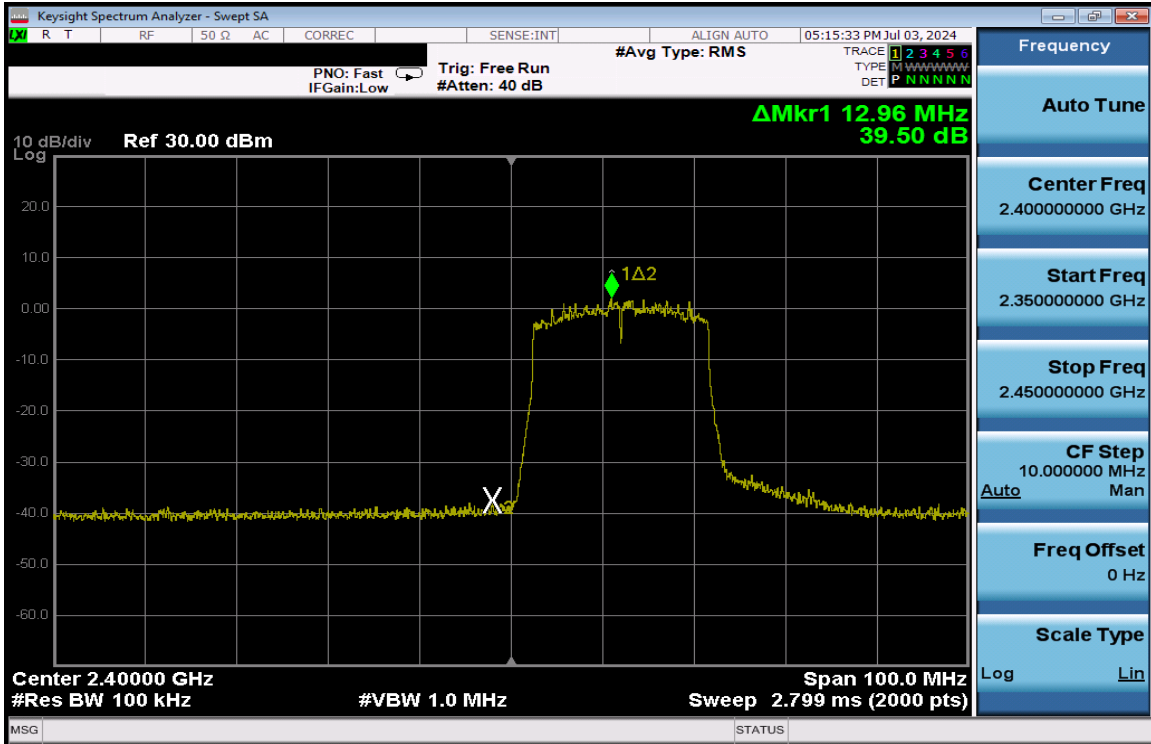
Plot 7-244. Band Edge Plot Antenna 3a (802.11ax (SU - 2.4GHz) – Ch. 1) – MCS4
