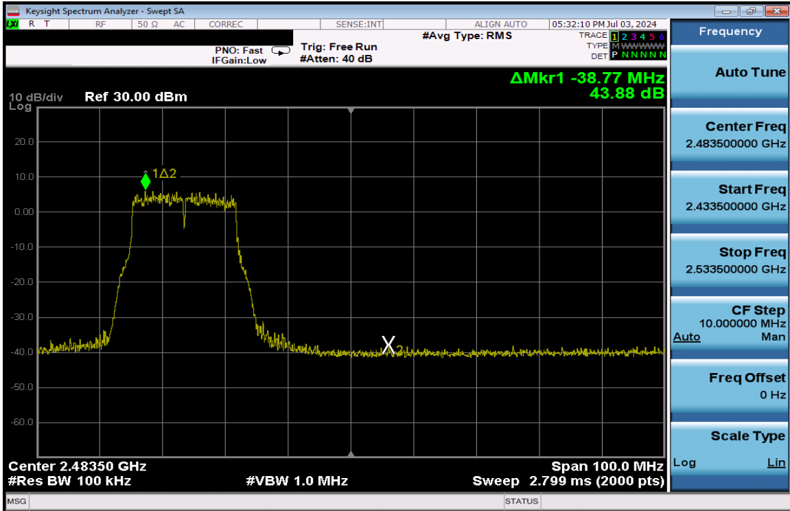
Plot 7-271. Band Edge Plot Antenna 3a (802.11g – Ch. 10) – 54Mbps
