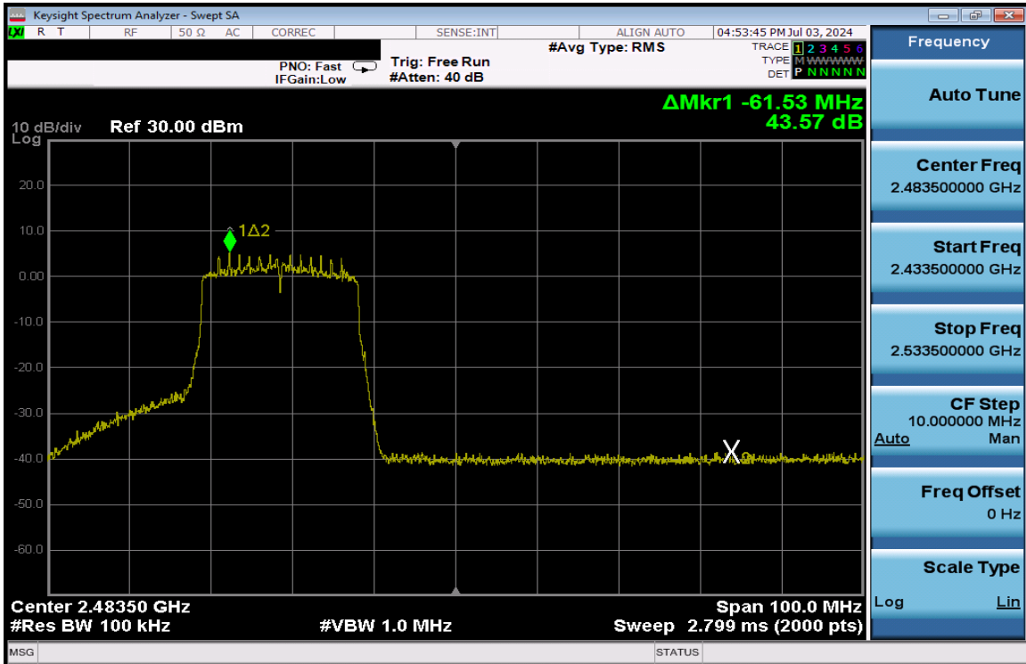
Plot 7-214. Band Edge Plot Antenna 3a (802.11ax (SU - 2.4GHz) – Ch. 11) – MCS2
