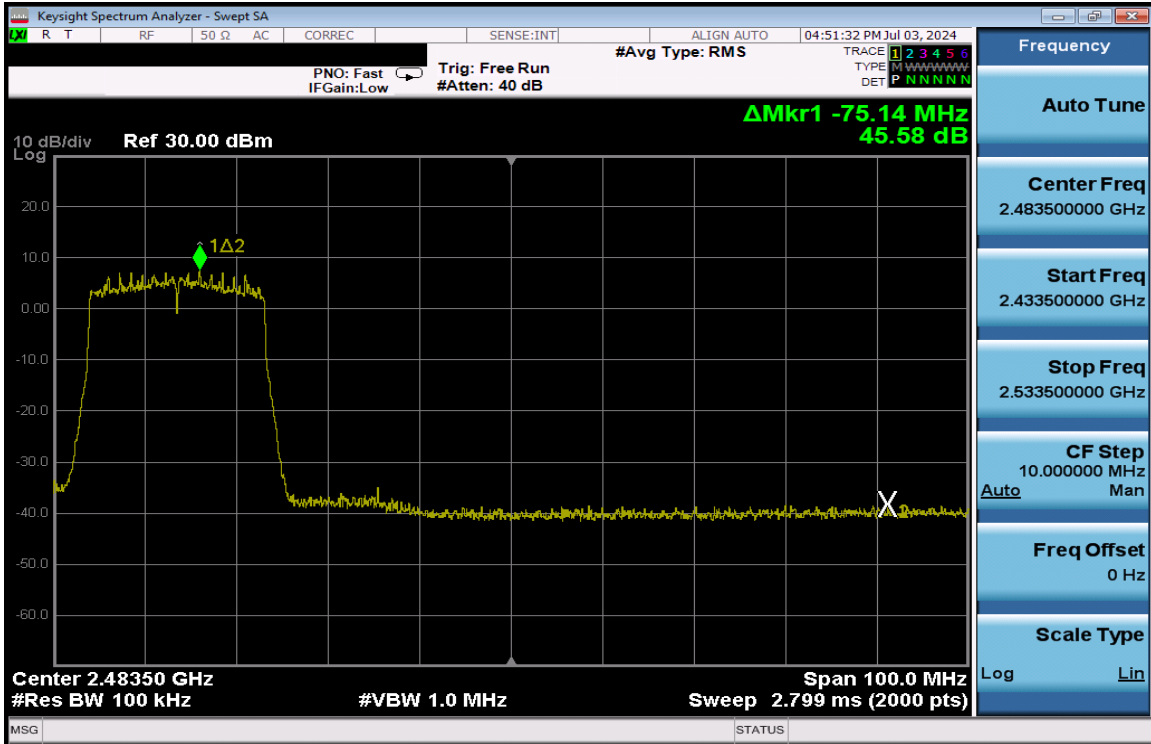
Plot 7-211. Band Edge Plot Antenna 3a (802.11ax (SU - 2.4GHz) – Ch. 8) – MCS2
