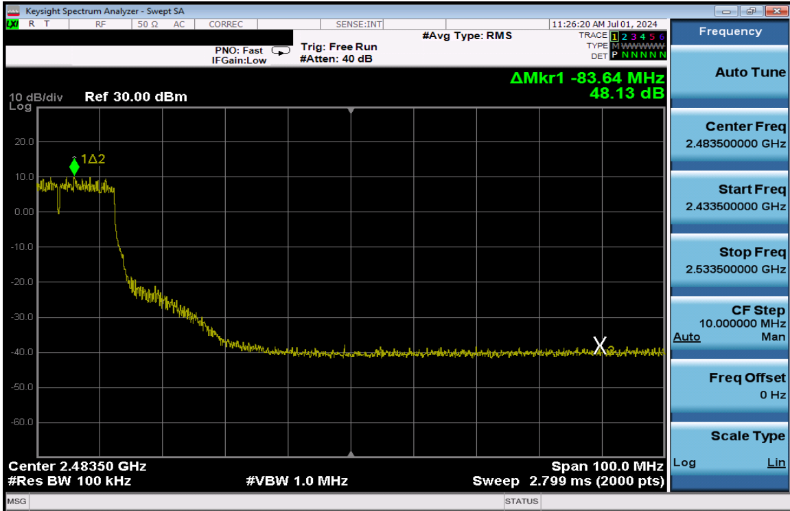
Plot 7-281. Band Edge Plot Antenna 3a (802.11n (2.4GHz) – Ch. 6 High) – MCS7
