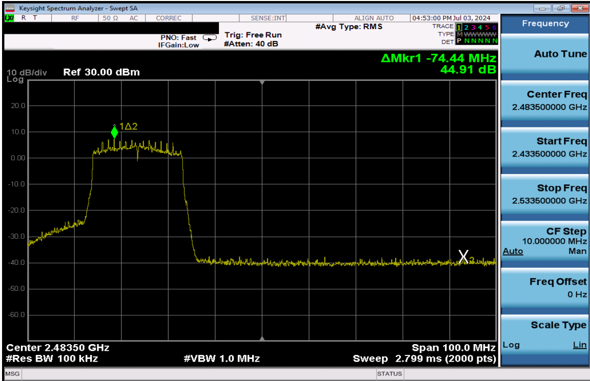
Plot 7-213. Band Edge Plot Antenna 3a (802.11ax (SU - 2.4GHz) – Ch. 10) – MCS2
