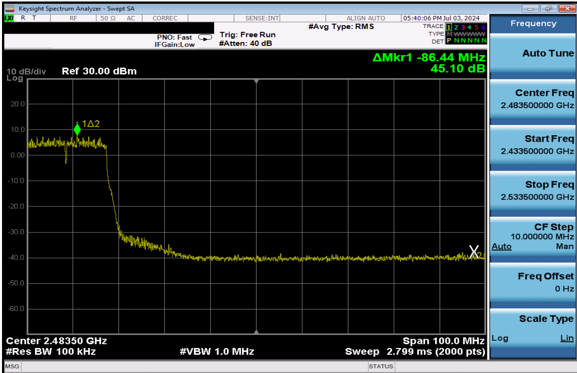
Plot 7-282. Band Edge Plot Antenna 3a (802.11n (2.4GHz) – Ch. 7) – MCS7
