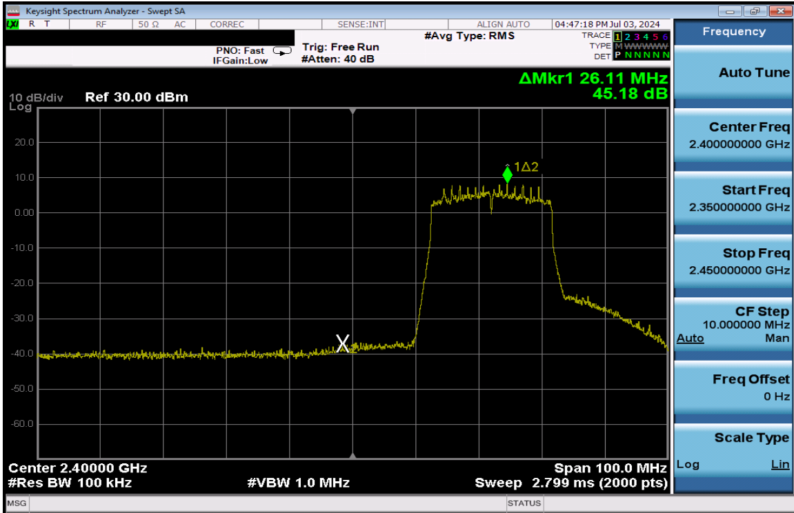
Plot 7-205. Band Edge Plot Antenna 3a (802.11ax (SU - 2.4GHz) – Ch. 3) – MCS2
