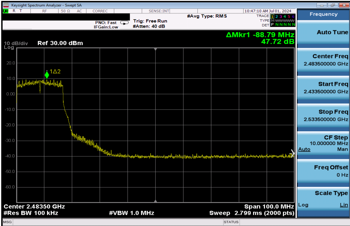
Plot 7-223. Band Edge Plot Antenna 3a (802.11g – Ch. 7) – 24Mbps
