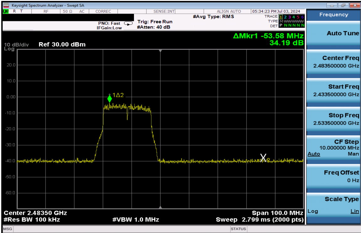
Plot 7-274. Band Edge Plot Antenna 3a (802.11g – Ch. 13) – 54Mbps
