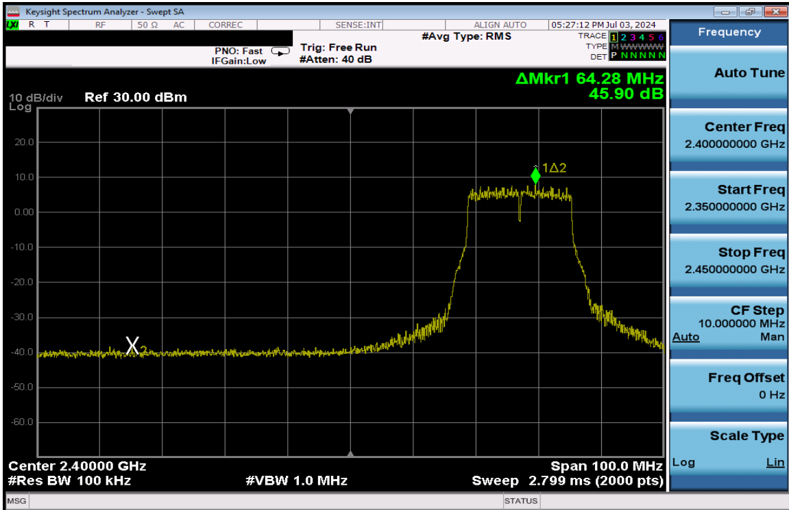
Plot 7-264. Band Edge Plot Antenna 3a (802.11g – Ch. 4) – 54Mbps
