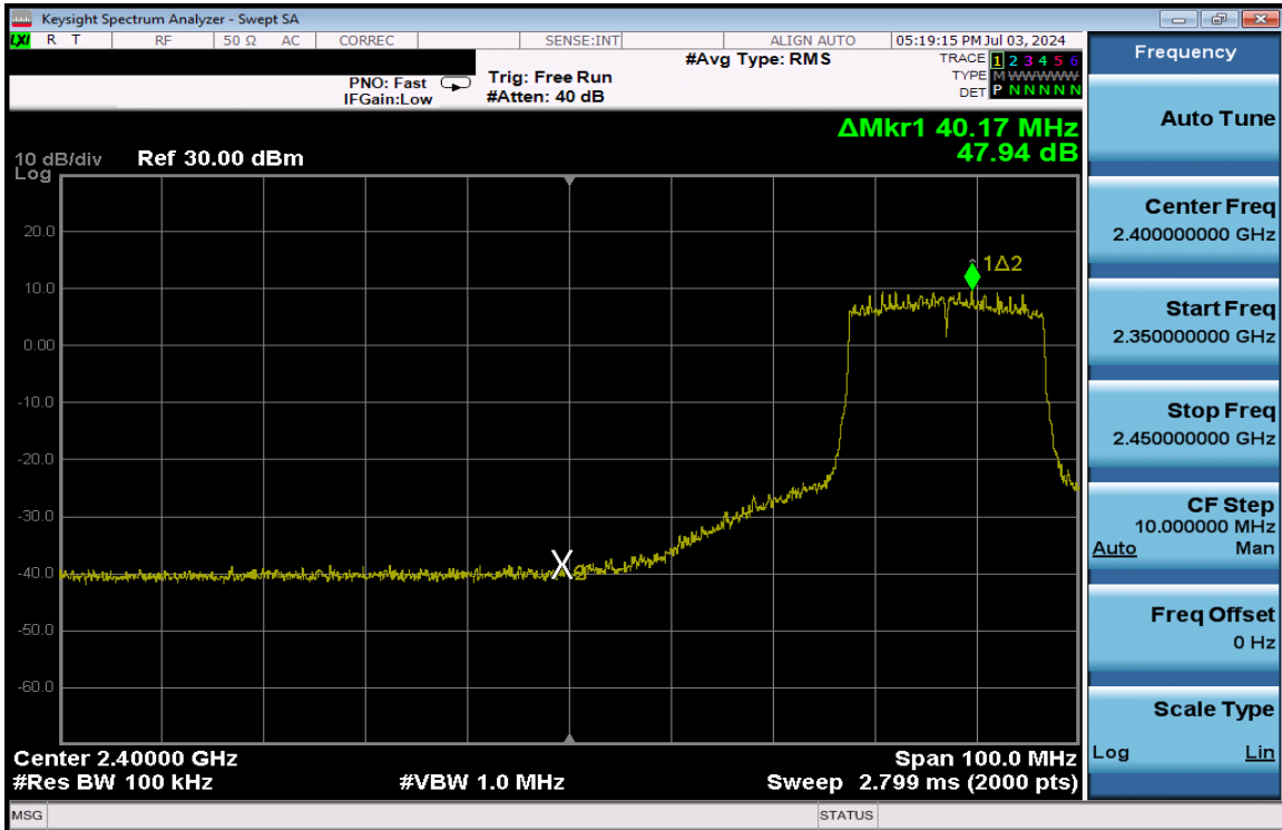
Plot 7-249. Band Edge Plot Antenna 3a (802.11ax (SU - 2.4GHz) – Ch. 6 Low) – MCS4
