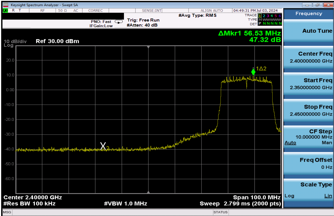
Plot 7-208. Band Edge Plot Antenna 3a (802.11ax (SU - 2.4GHz) – Ch. 6 Low) – MCS2
