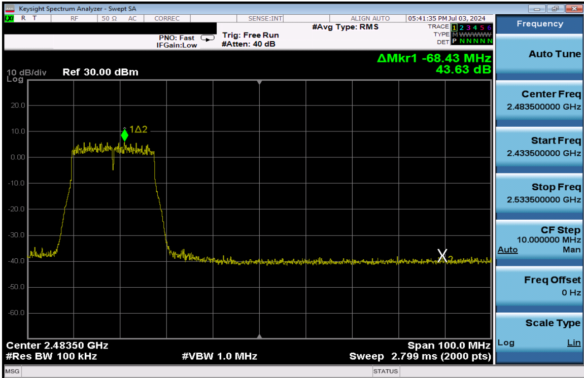
Plot 7-284. Band Edge Plot Antenna 3a (802.11n (2.4GHz) – Ch. 9) – MCS7
