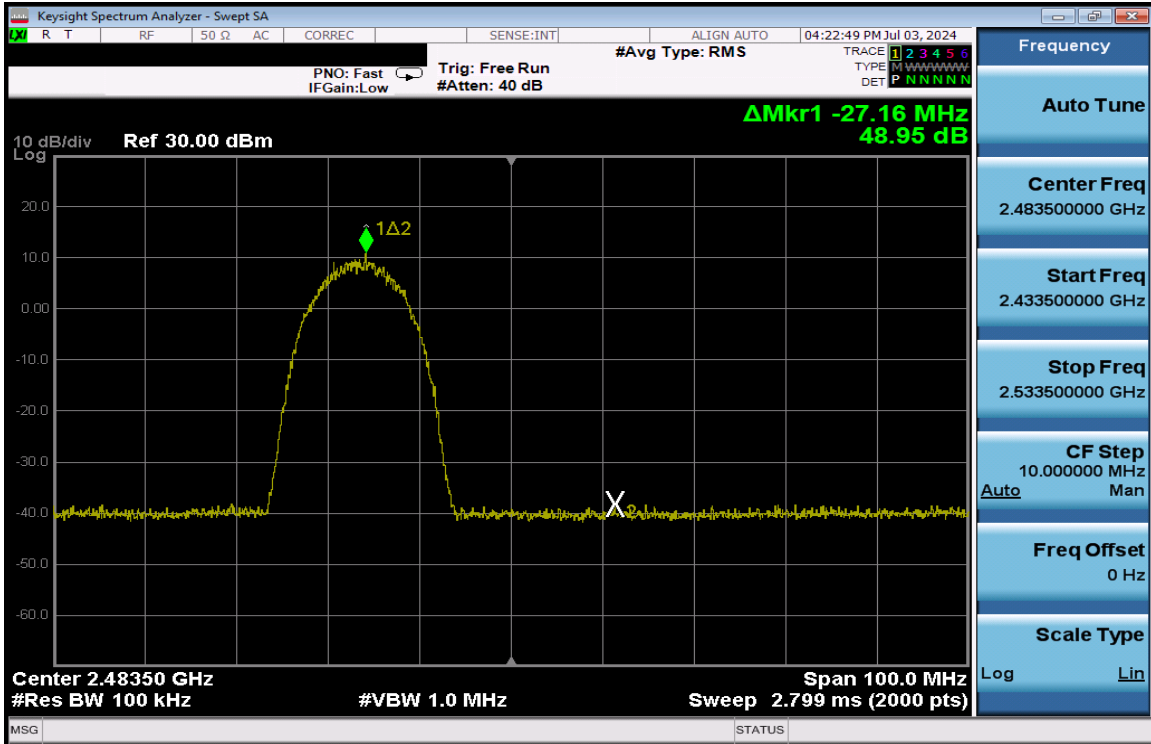
Plot 7-259. Band Edge Plot Antenna 3a (802.11b – Ch. 12) – 11Mbps
