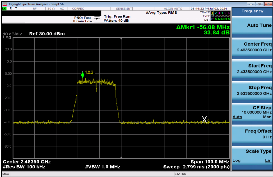
Plot 7-288. Band Edge Plot Antenna 3a (802.11n (2.4GHz) – Ch. 13) – MCS7
