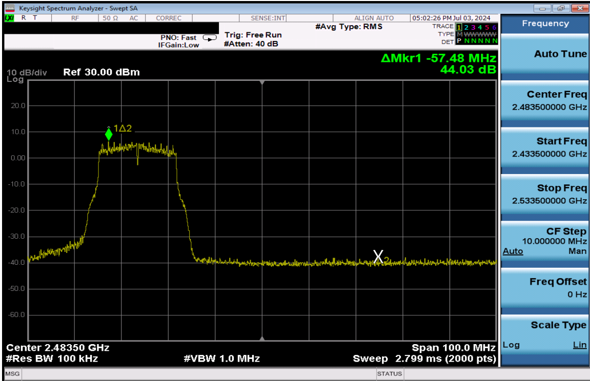
Plot 7-226. Band Edge Plot Antenna 3a (802.11g – Ch. 10) – 24Mbps
