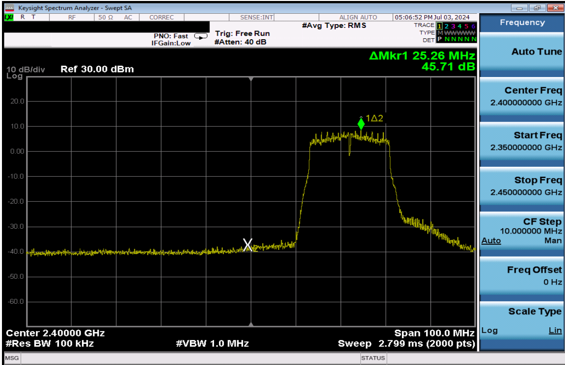
Plot 7-232. Band Edge Plot Antenna 3a (802.11n (2.4GHz) – Ch. 3) – MCS4
