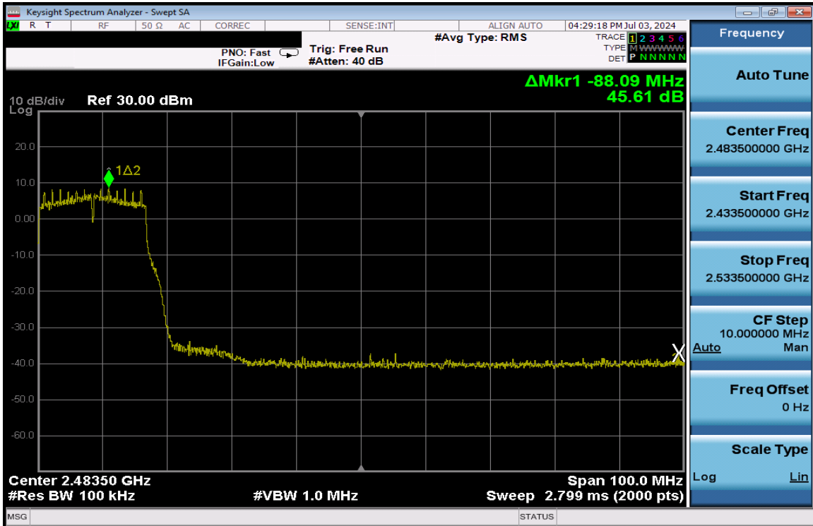
Plot 7-182. Band Edge Plot Antenna 3a (802.11g – Ch. 7) – 12Mbps
