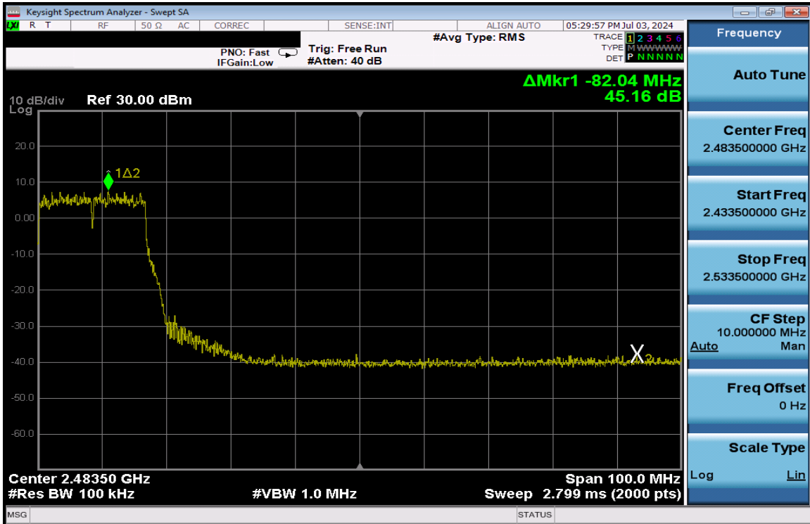
Plot 7-268. Band Edge Plot Antenna 3a (802.11g – Ch. 7) – 54Mbps
