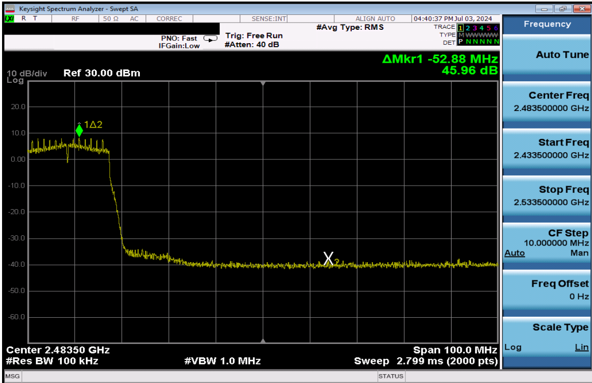
Plot 7-196. Band Edge Plot Antenna 3a (802.11n (2.4GHz) – Ch. 7) – MCS2
