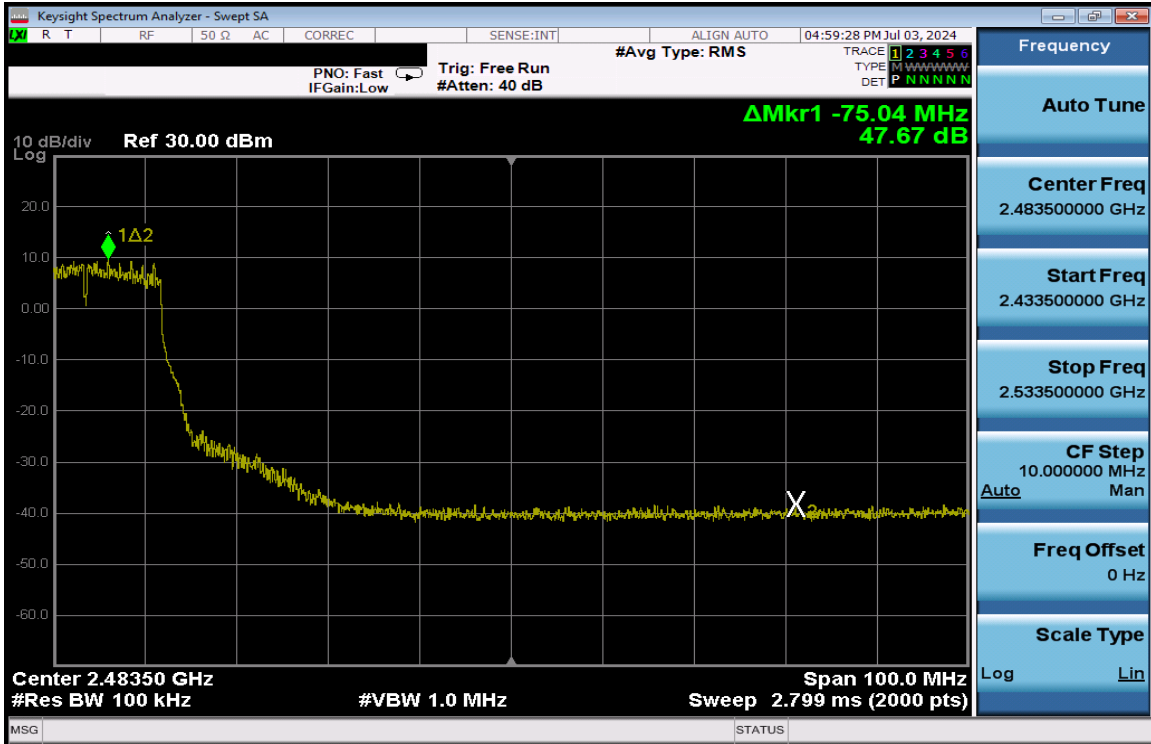
Plot 7-222. Band Edge Plot Antenna 3a (802.11g – Ch. 6 High) – 24Mbps
