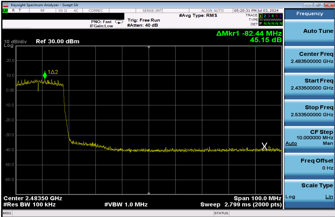
Plot 7-251. Band Edge Plot Antenna 3a (802.11ax (SU - 2.4GHz) – Ch. 7) – MCS4
