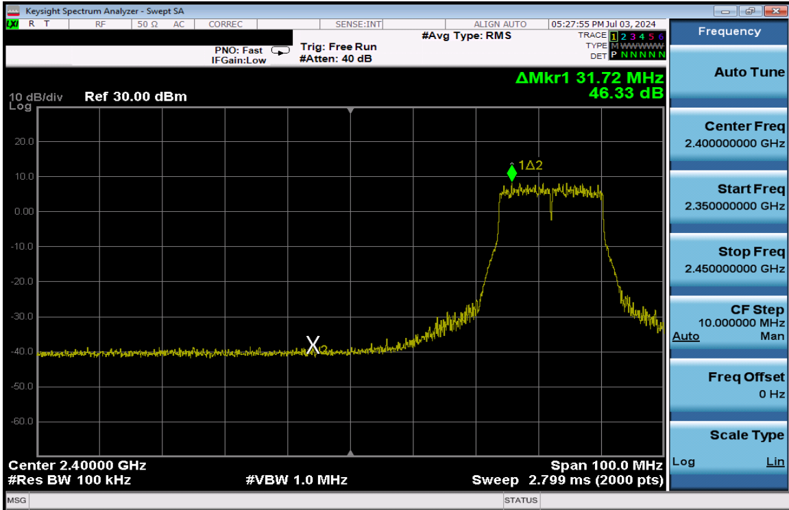
Plot 7-265. Band Edge Plot Antenna 3a (802.11g – Ch. 5) – 54Mbps
