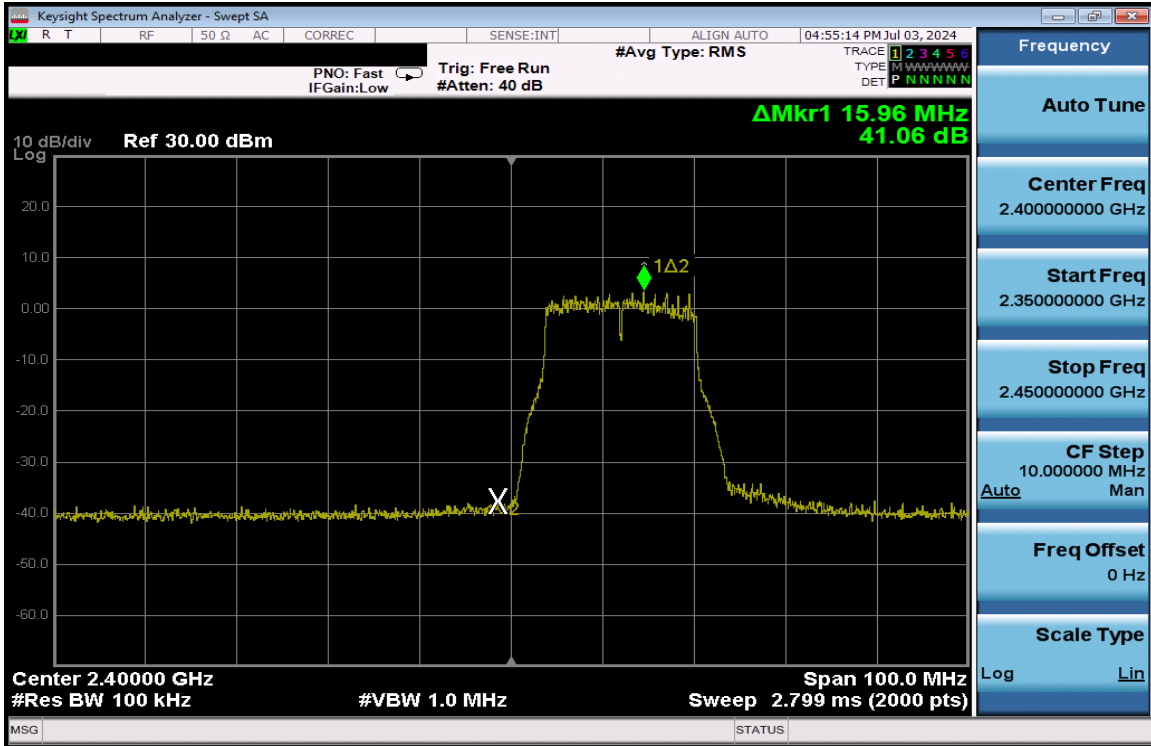
Plot 7-216. Band Edge Plot Antenna 3a (802.11g – Ch. 1) – 24Mbps
