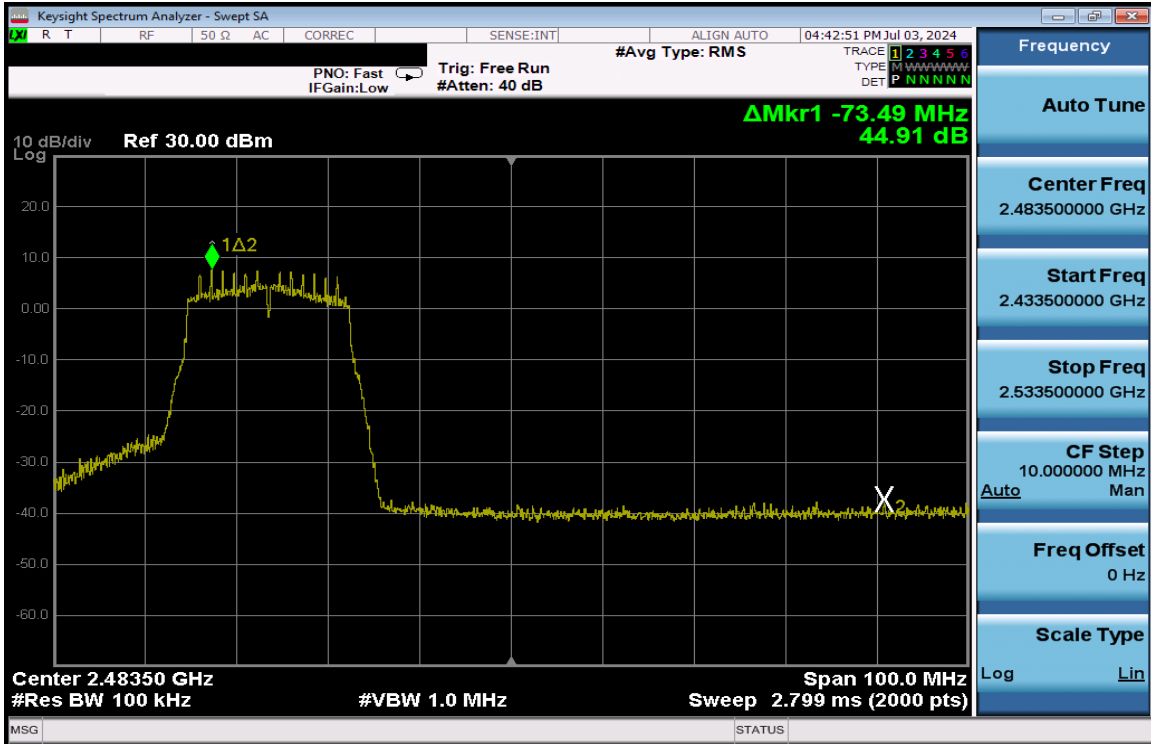
Plot 7-199. Band Edge Plot Antenna 3a (802.11n (2.4GHz) – Ch. 10) – MCS2
