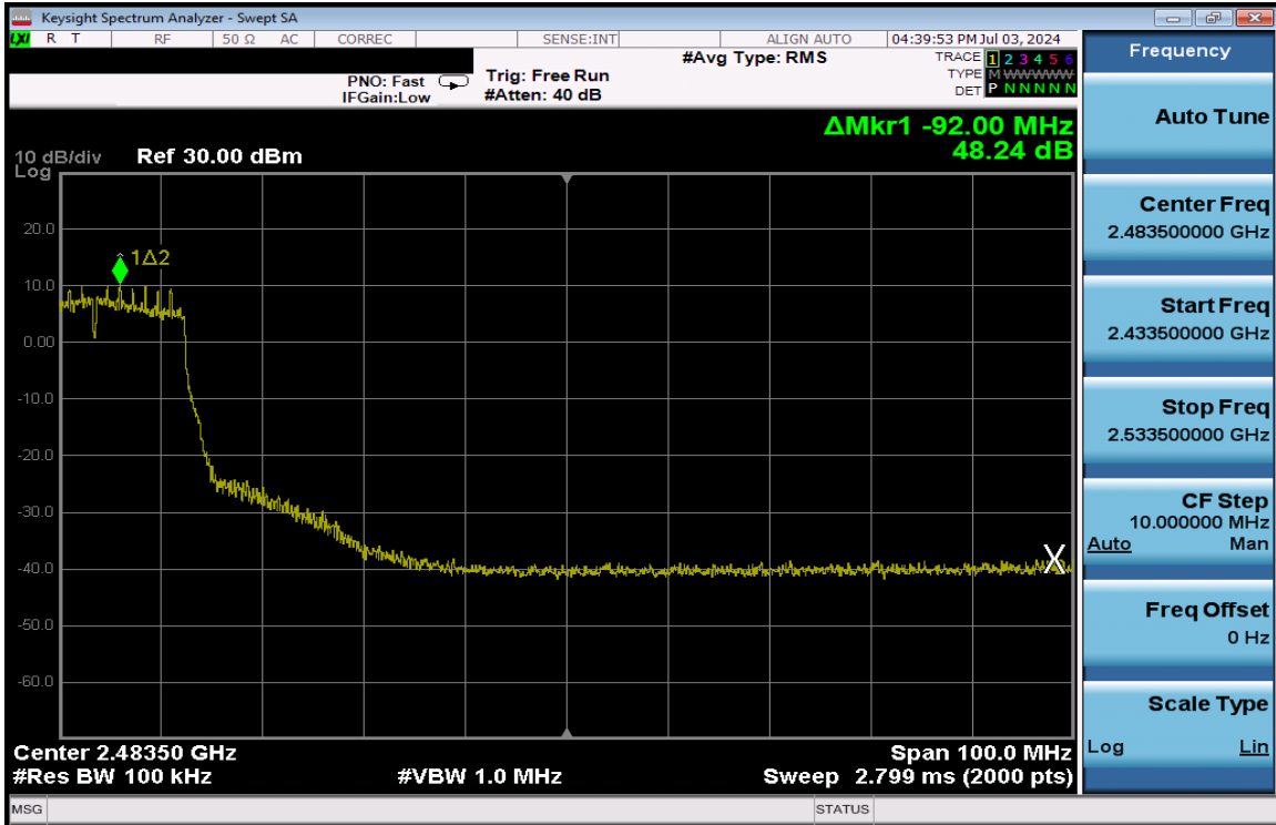
Plot 7-195. Band Edge Plot Antenna 3a (802.11n (2.4GHz) – Ch. 6 High) – MCS2
