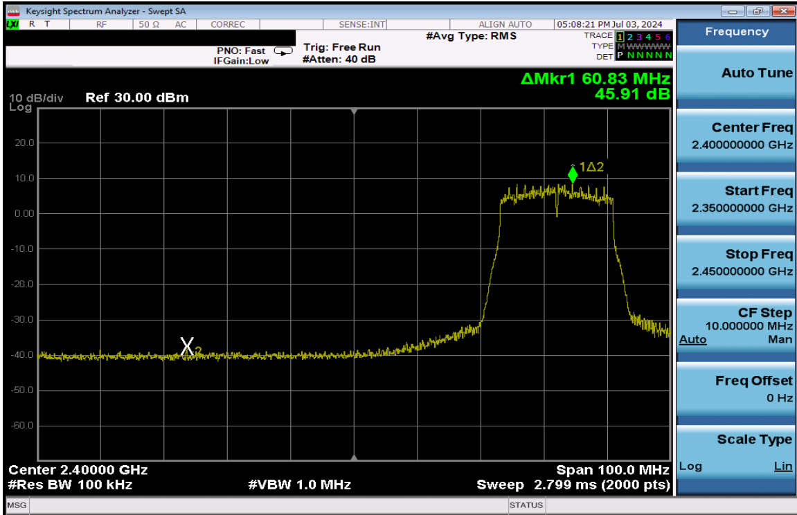
Plot 7-234. Band Edge Plot Antenna 3a (802.11n (2.4GHz) – Ch. 5) – MCS4
