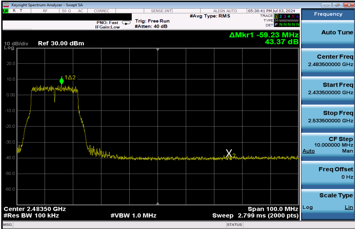
Plot 7-269. Band Edge Plot Antenna 3a (802.11g – Ch. 8) – 54Mbps
