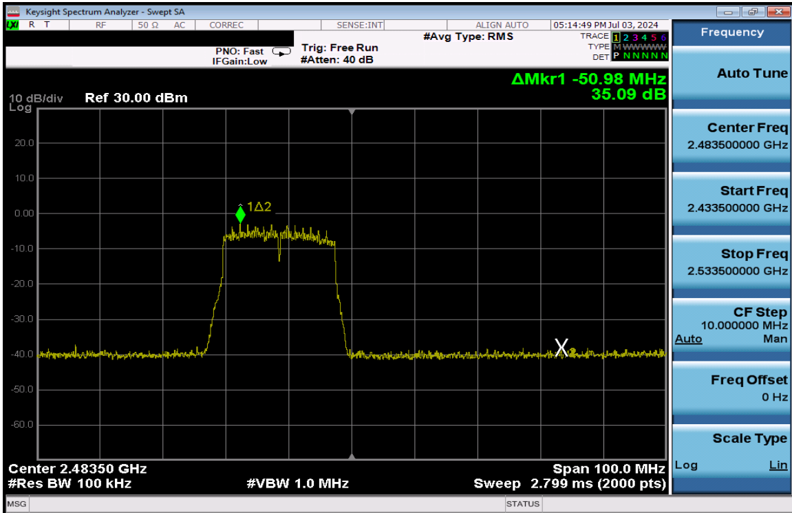
Plot 7-243. Band Edge Plot Antenna 3a (802.11n (2.4GHz) – Ch. 13) – MCS4
