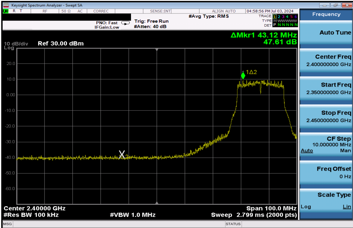
Plot 7-221. Band Edge Plot Antenna 3a (802.11g – Ch. 6 Low) – 24Mbps
