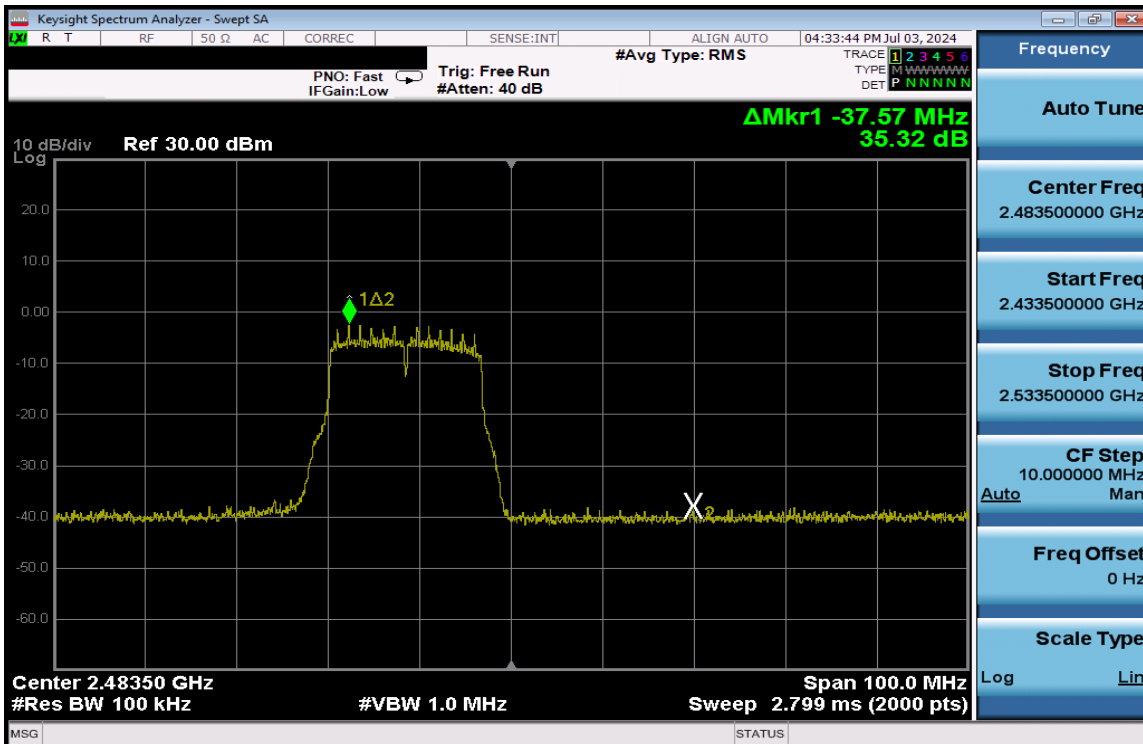
Plot 7-188. Band Edge Plot Antenna 3a (802.11g – Ch. 13) – 12Mbps
