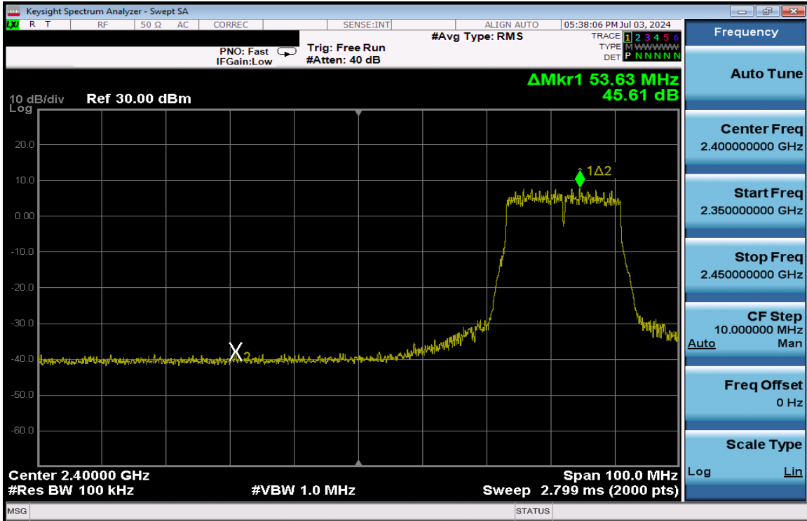
Plot 7-279. Band Edge Plot Antenna 3a (802.11n (2.4GHz) – Ch. 5) – MCS7
