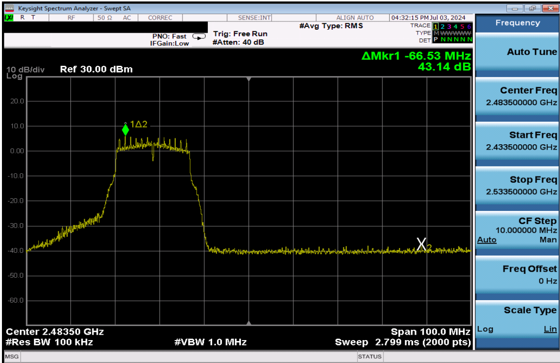
Plot 7-186. Band Edge Plot Antenna 3a (802.11g - Ch. 11) - 12Mbps
