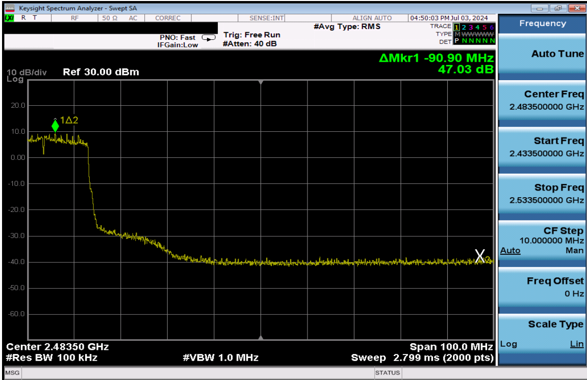
Plot 7-209. Band Edge Plot Antenna 3a (802.11ax (SU - 2.4GHz) – Ch. 6 High) – MCS2
