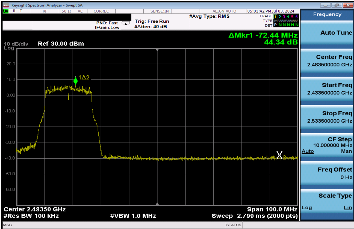
Plot 7-225. Band Edge Plot Antenna 3a (802.11g – Ch. 9) – 24Mbps
