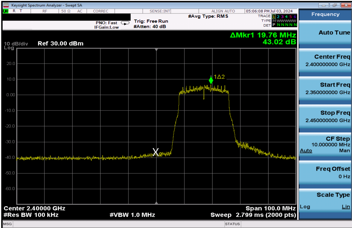
Plot 7-231. Band Edge Plot Antenna 3a (802.11n (2.4GHz) – Ch. 2) – MCS4
