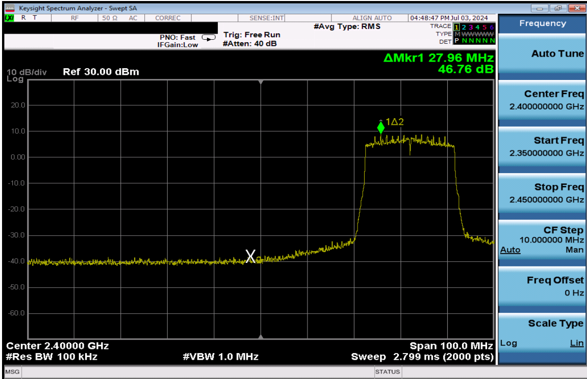
Plot 7-207. Band Edge Plot Antenna 3a (802.11ax (SU - 2.4GHz) – Ch. 5) – MCS2
