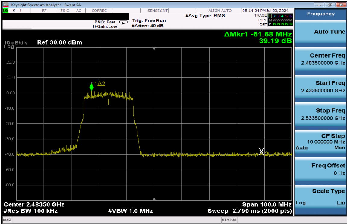
Plot 7-242. Band Edge Plot Antenna 3a (802.11n (2.4GHz) – Ch. 12) – MCS4
