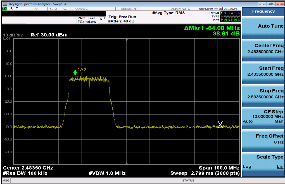
Plot 7-287. Band Edge Plot Antenna 3a (802.11n (2.4GHz) – Ch. 12) – MCS7
