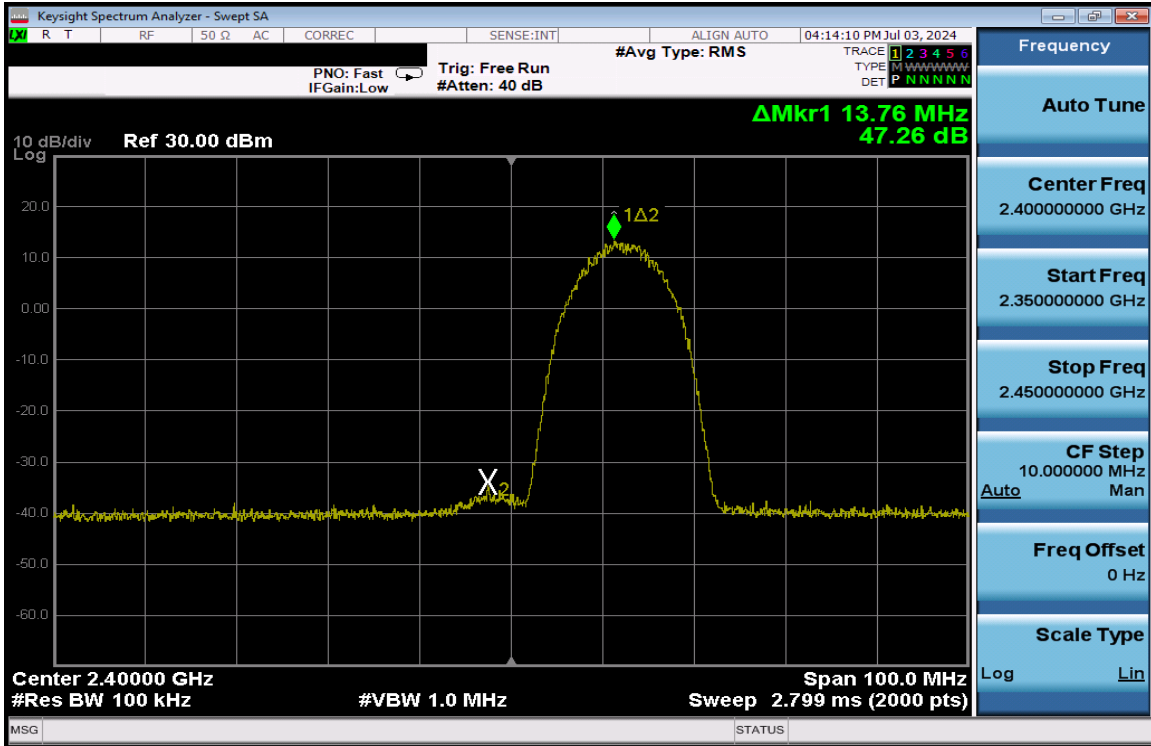
Plot 7-257. Band Edge Plot Antenna 3a (802.11b – Ch. 1) – 11Mbps
