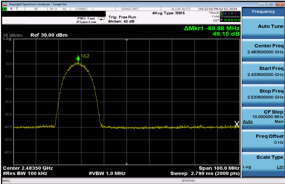
Plot 7-258. Band Edge Plot Antenna 3a (802.11b – Ch. 11) – 11Mbps
