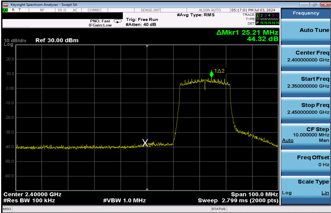
Plot 7-246. Band Edge Plot Antenna 3a (802.11ax (SU - 2.4GHz) – Ch. 3) – MCS4
