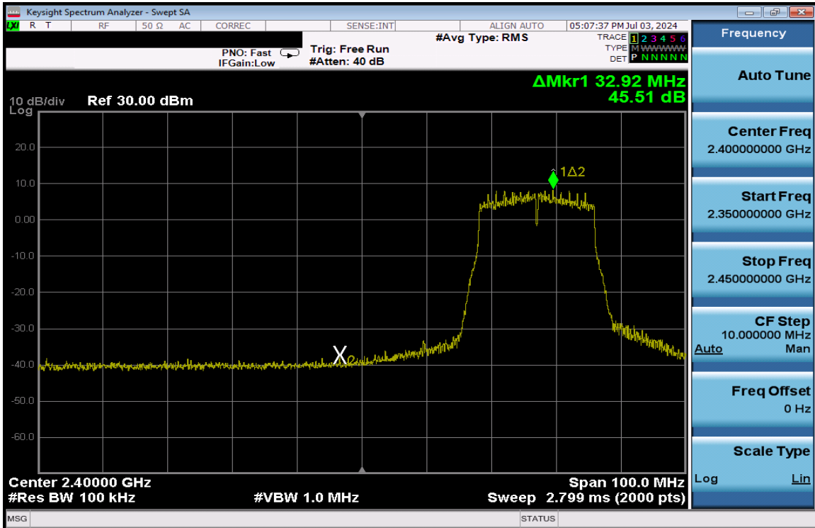
Plot 7-233. Band Edge Plot Antenna 3a (802.11n (2.4GHz) – Ch. 4) – MCS4
