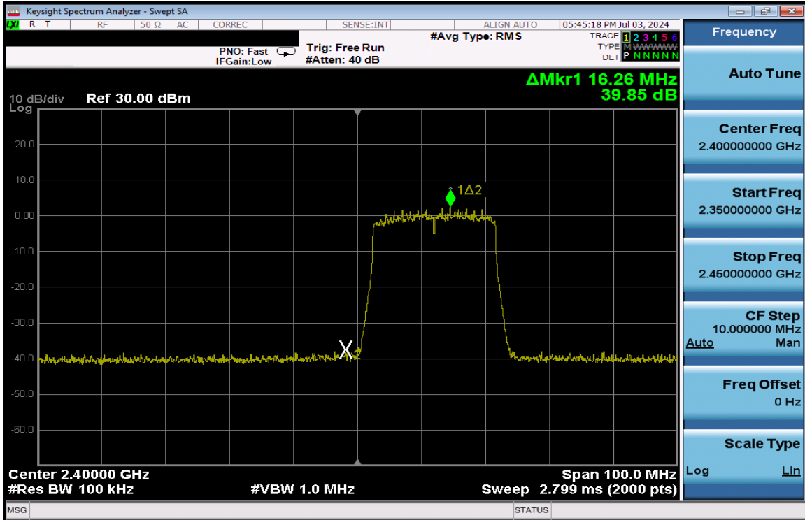
Plot 7-289. Band Edge Plot Antenna 3a (802.11ax (SU - 2.4GHz) - Ch. 1) - MCS9
