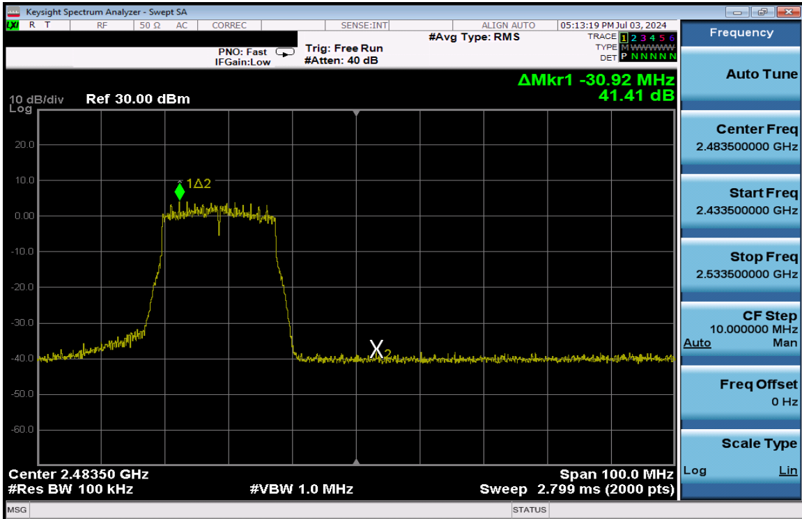
Plot 7-241. Band Edge Plot Antenna 3a (802.11n (2.4GHz) – Ch. 11) – MCS4
