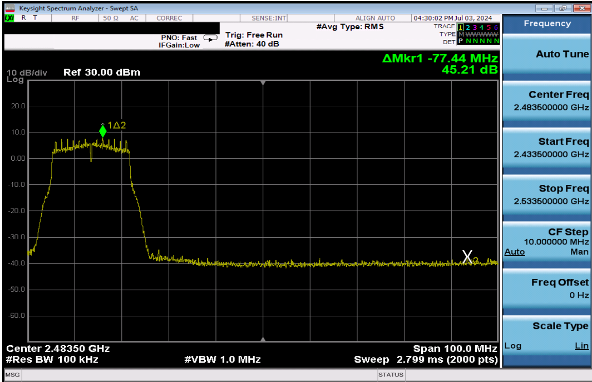
Plot 7-183. Band Edge Plot Antenna 3a (802.11g – Ch. 8) – 12Mbps
