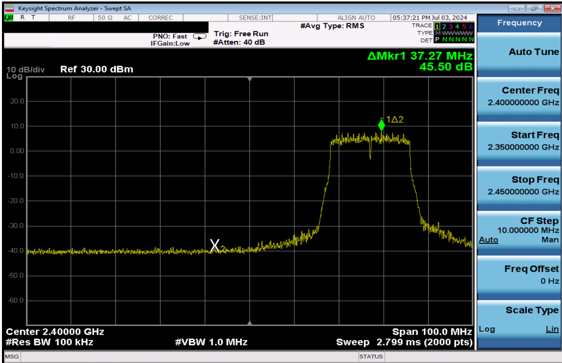
Plot 7-278. Band Edge Plot Antenna 3a (802.11n (2.4GHz) – Ch. 4) – MCS7
