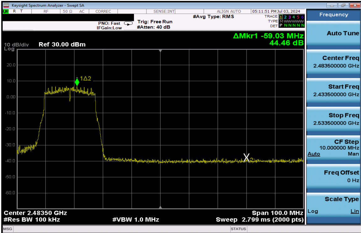
Plot 7-239. Band Edge Plot Antenna 3a (802.11n (2.4GHz) – Ch. 9) – MCS4
