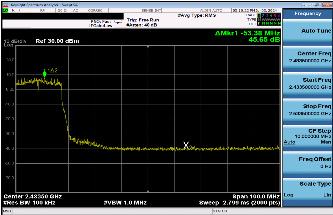
Plot 7-237. Band Edge Plot Antenna 3a (802.11n (2.4GHz) – Ch. 7) – MCS4
