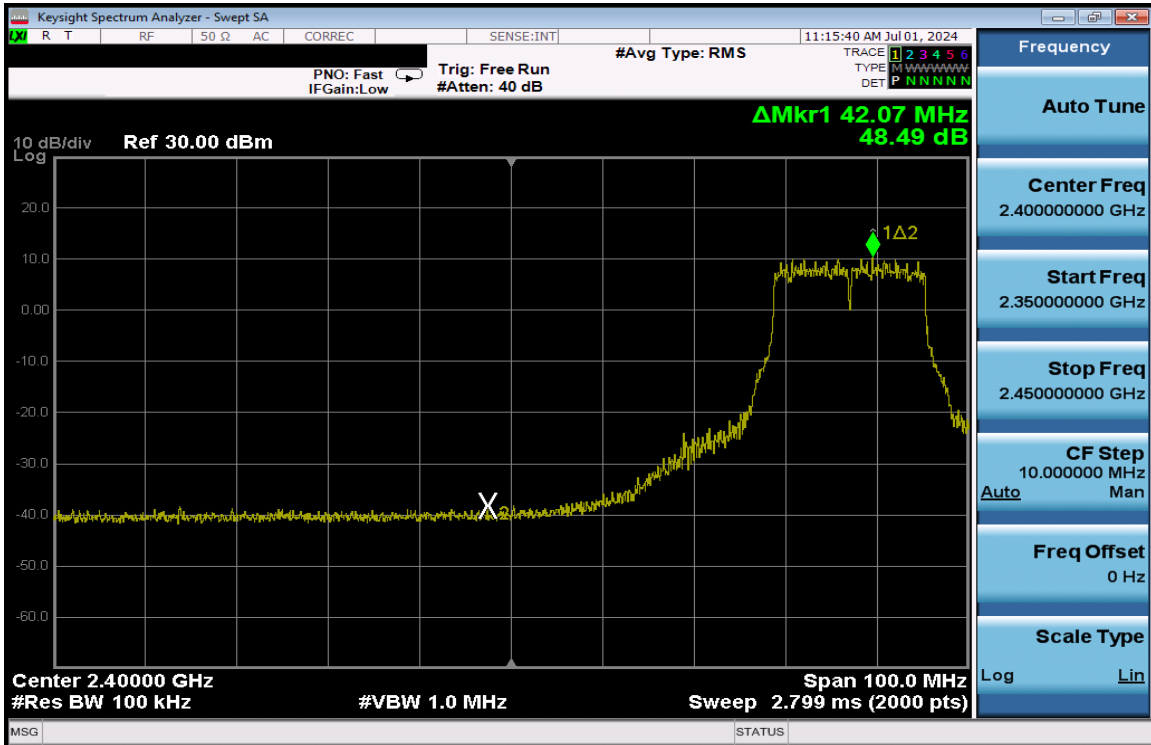
Plot 7-266. Band Edge Plot Antenna 3a (802.11g – Ch. 6 Low) – 54Mbps
