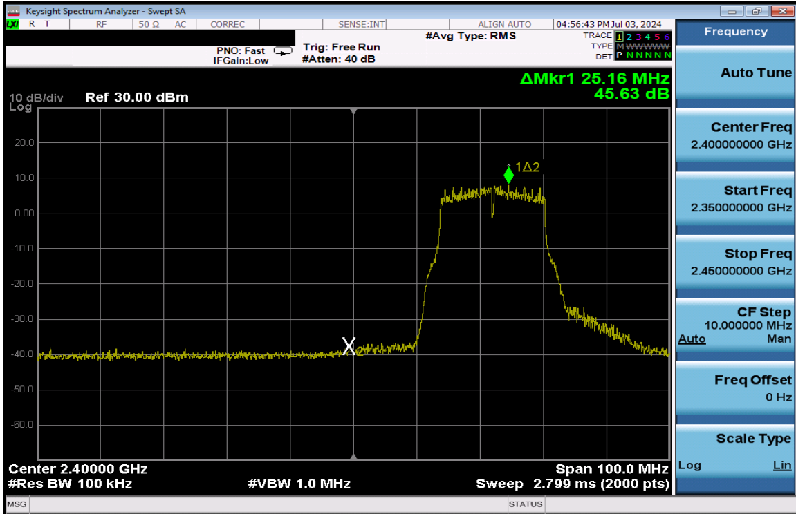
Plot 7-218. Band Edge Plot Antenna 3a (802.11g – Ch. 3) – 24Mbps
