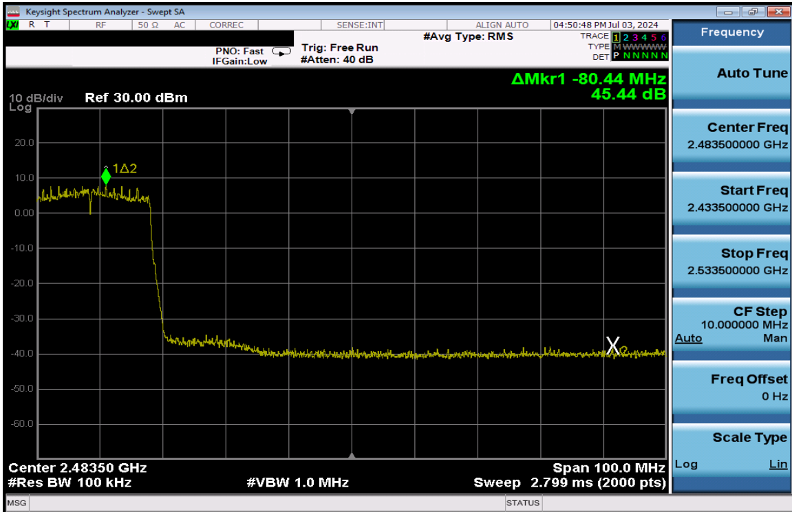
Plot 7-210. Band Edge Plot Antenna 3a (802.11ax (SU - 2.4GHz) – Ch. 7) – MCS2
