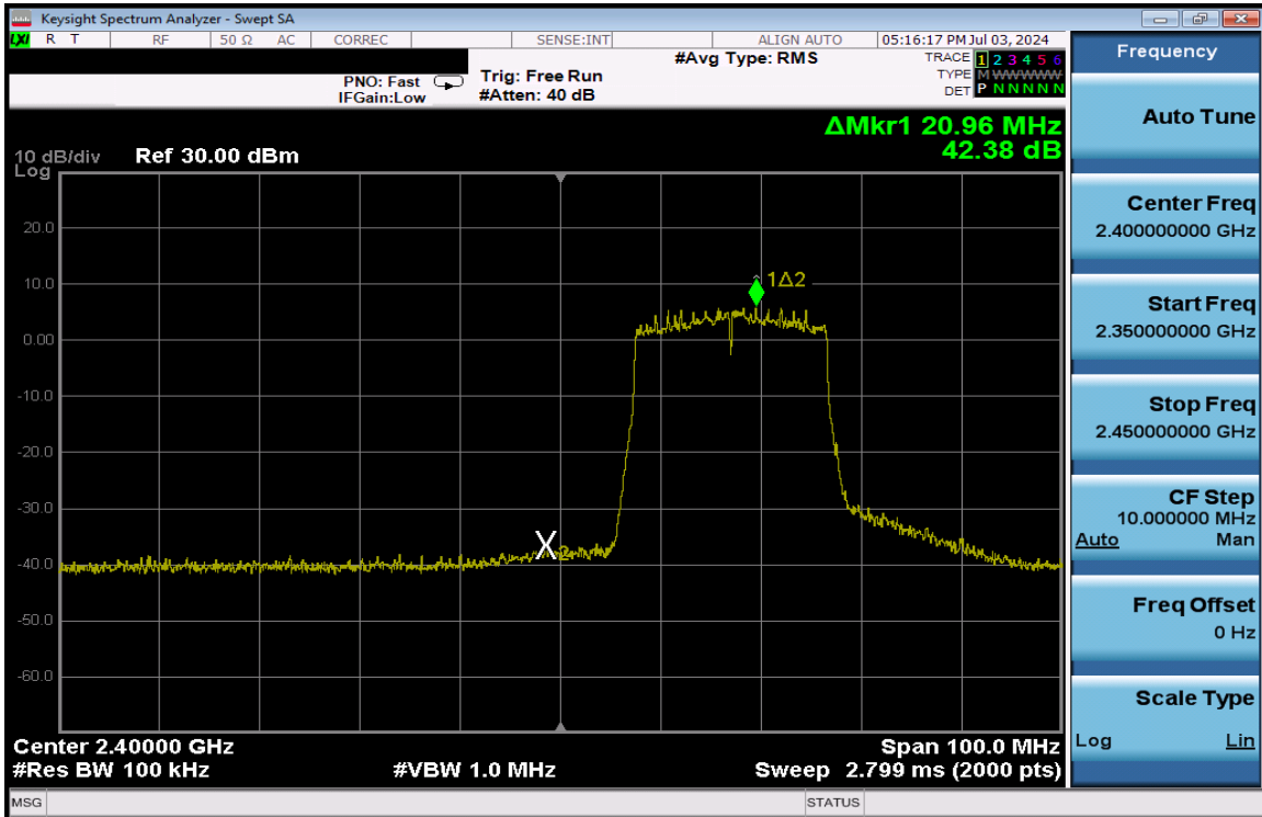
Plot 7-245. Band Edge Plot Antenna 3a (802.11ax (SU - 2.4GHz) – Ch. 2) – MCS4
