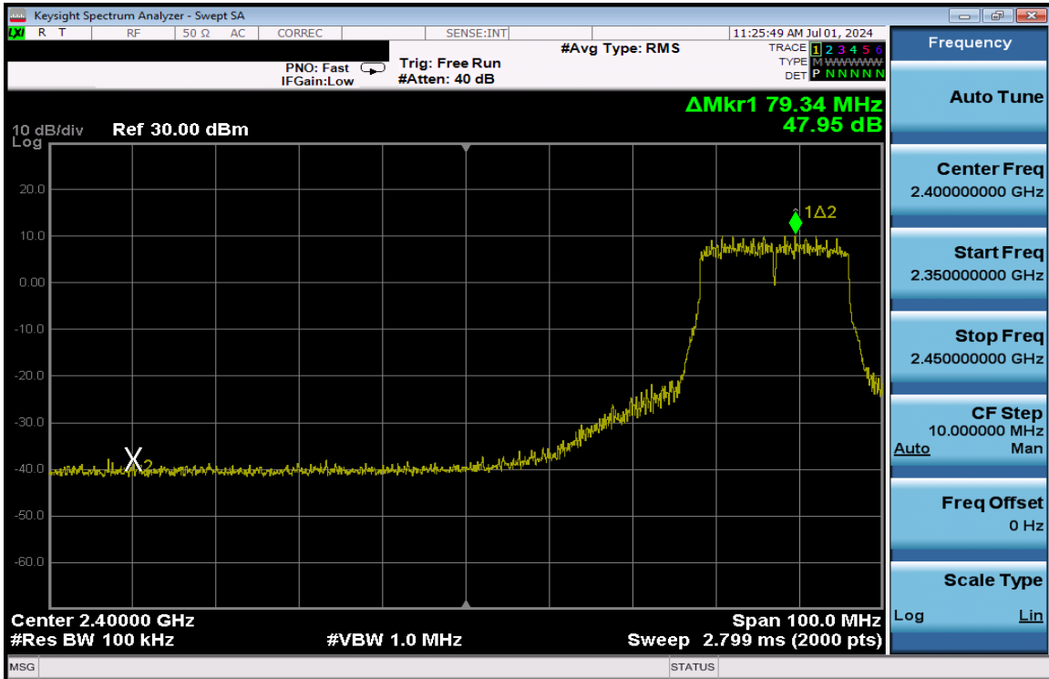
Plot 7-280. Band Edge Plot Antenna 3a (802.11n (2.4GHz) – Ch. 6 Low) – MCS7
