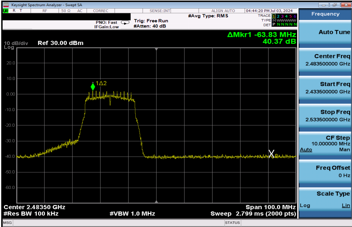
Plot 7-201. Band Edge Plot Antenna 3a (802.11n (2.4GHz) – Ch. 12) – MCS2
