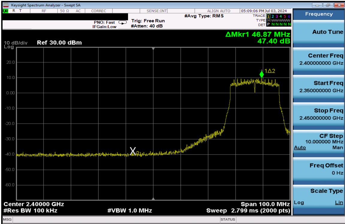
Plot 7-235. Band Edge Plot Antenna 3a (802.11n (2.4GHz) – Ch. 6 Low) – MCS4
