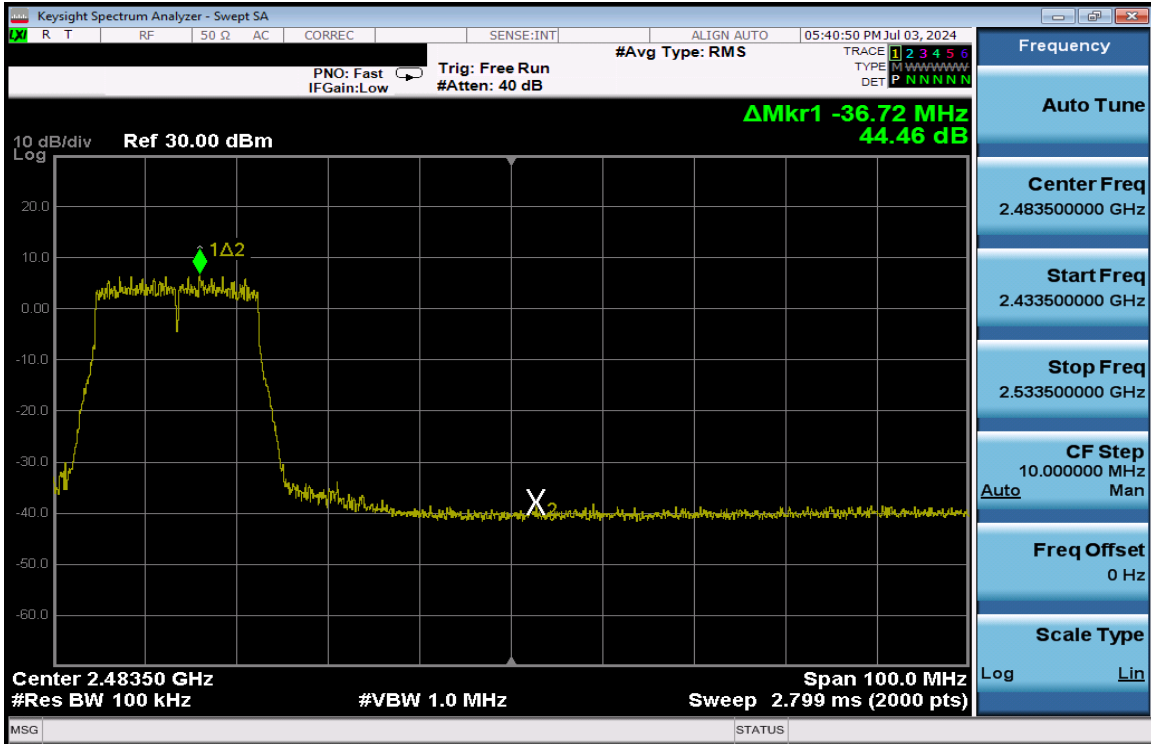
Plot 7-283. Band Edge Plot Antenna 3a (802.11n (2.4GHz) – Ch. 8) – MCS7
