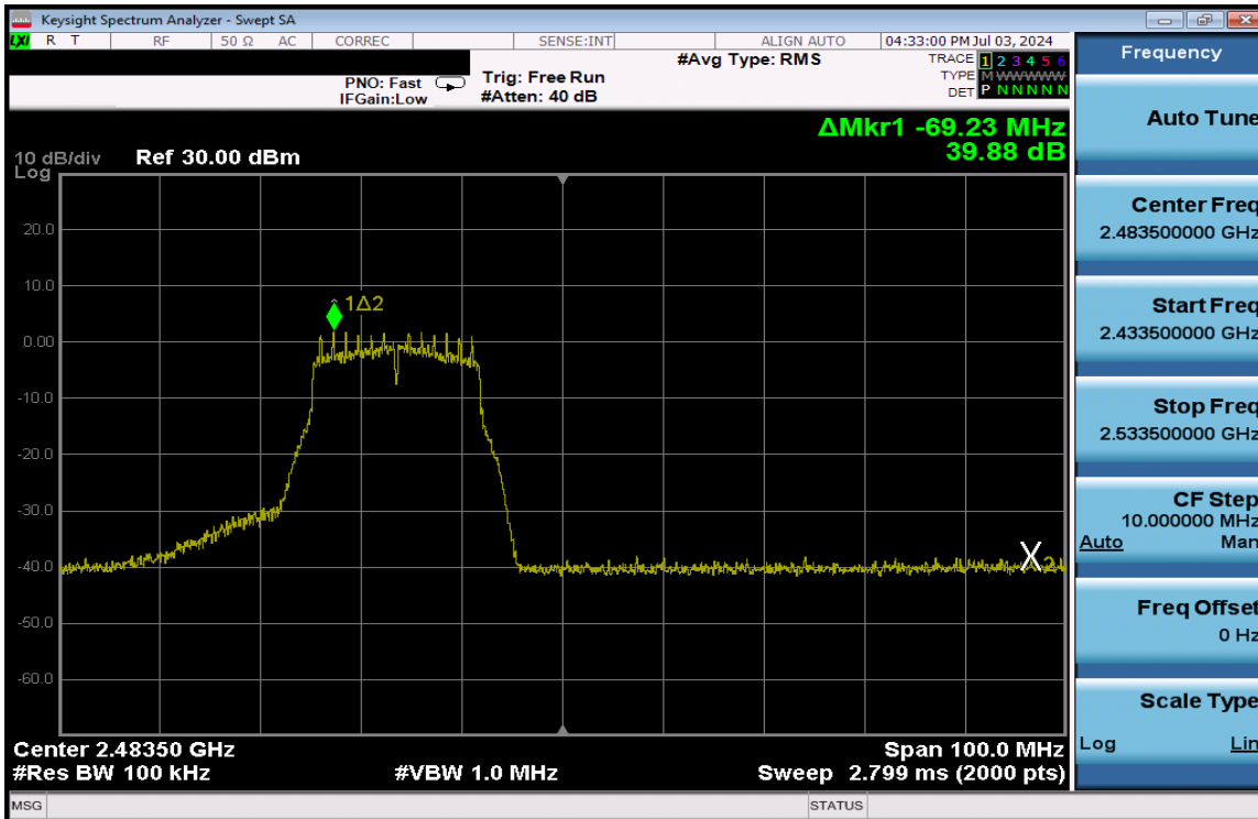
Plot 7-187. Band Edge Plot Antenna 3a (802.11g – Ch. 12) – 12Mbps
