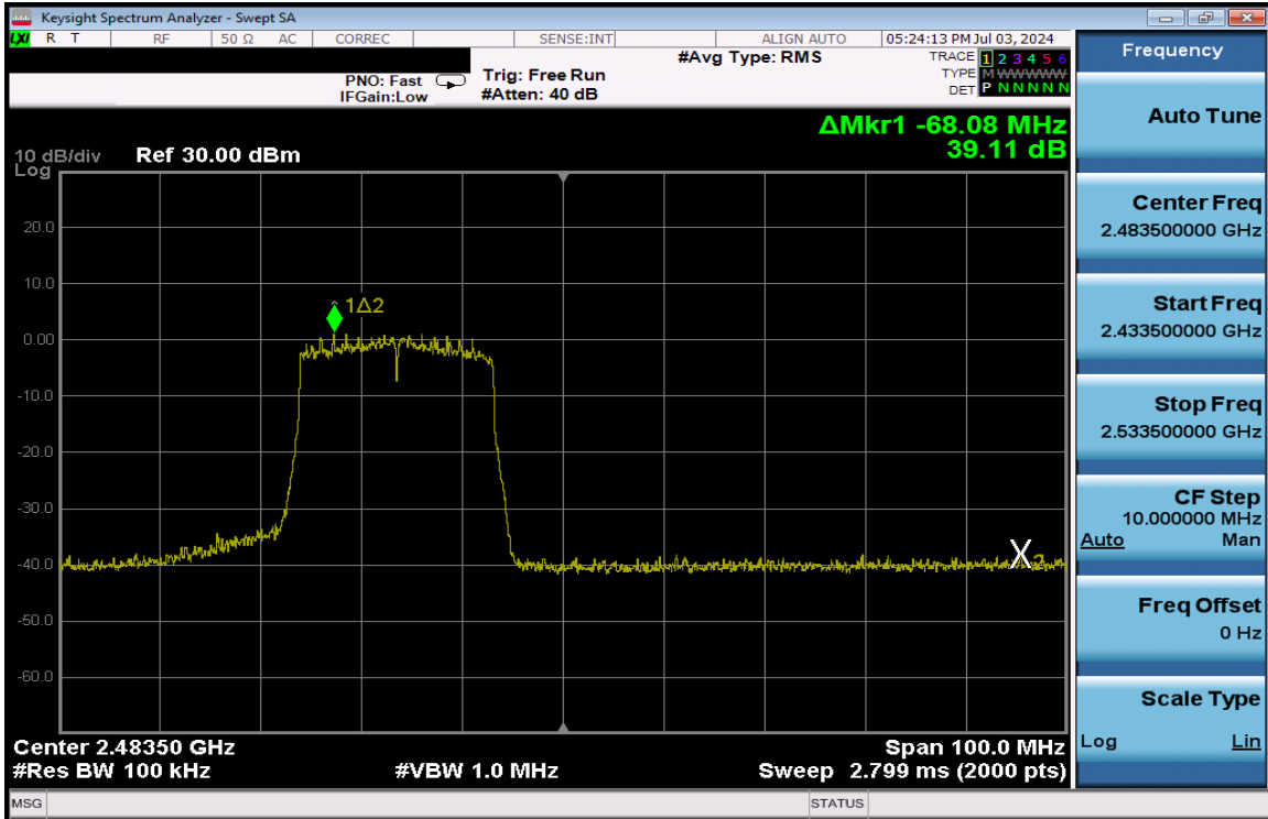
Plot 7-256. Band Edge Plot Antenna 3a (802.11ax (SU - 2.4GHz) – Ch. 12) – MCS4
