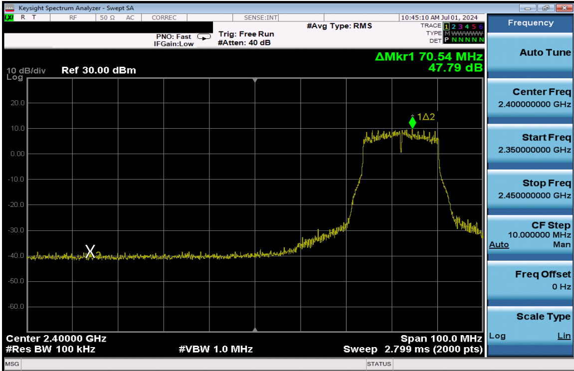
Plot 7-220. Band Edge Plot Antenna 3a (802.11g – Ch. 5) – 24Mbps
