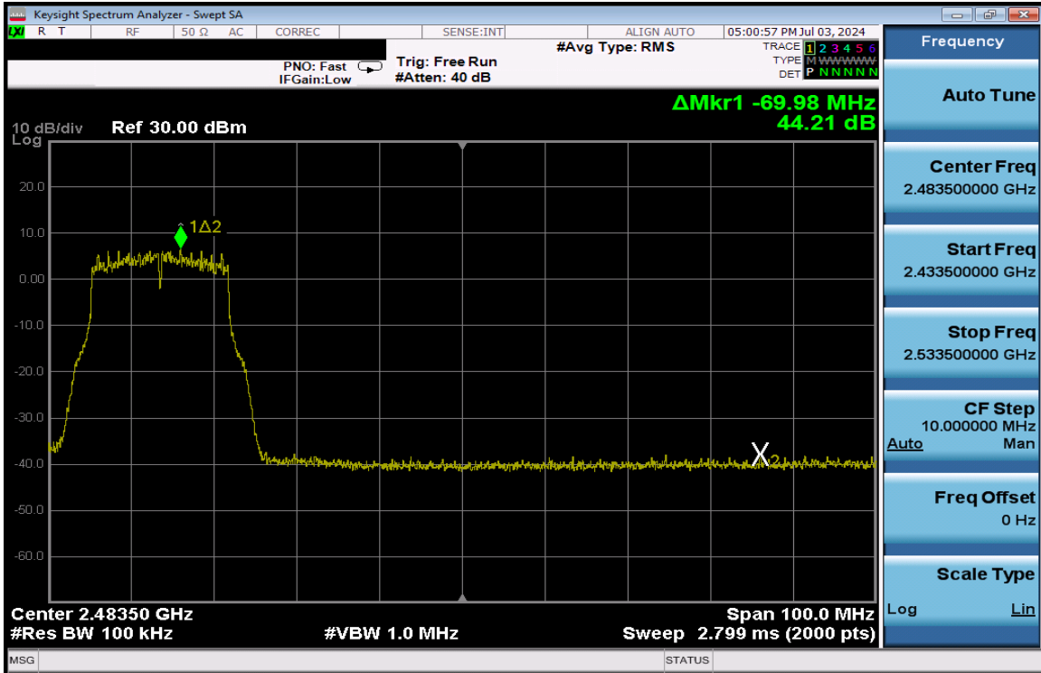
Plot 7-224. Band Edge Plot Antenna 3a (802.11g – Ch. 8) – 24Mbps
