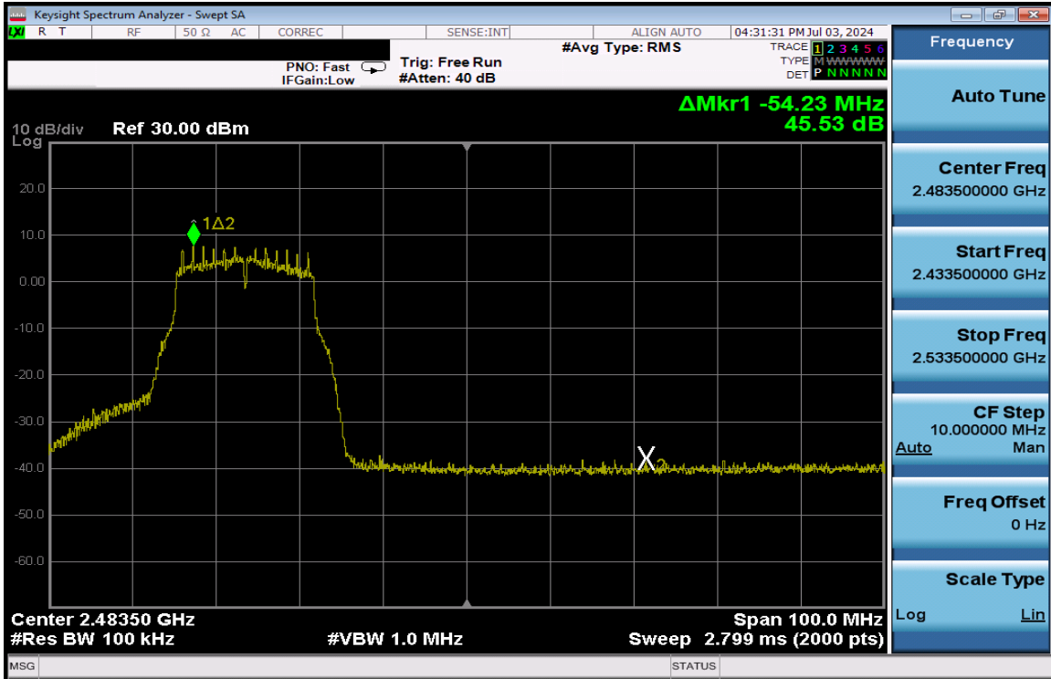
Plot 7-185. Band Edge Plot Antenna 3a (802.11g - Ch. 10) - 12Mbps
