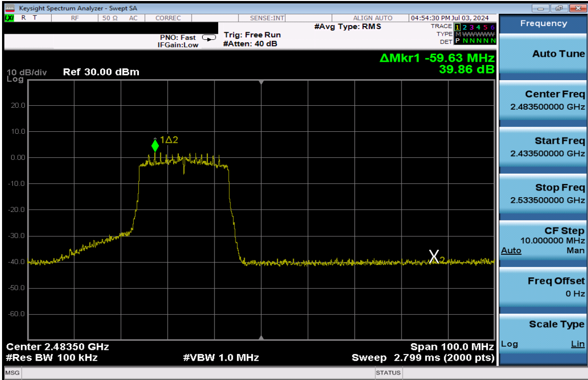
Plot 7-215. Band Edge Plot Antenna 3a (802.11ax (SU - 2.4GHz) – Ch. 12) – MCS2
