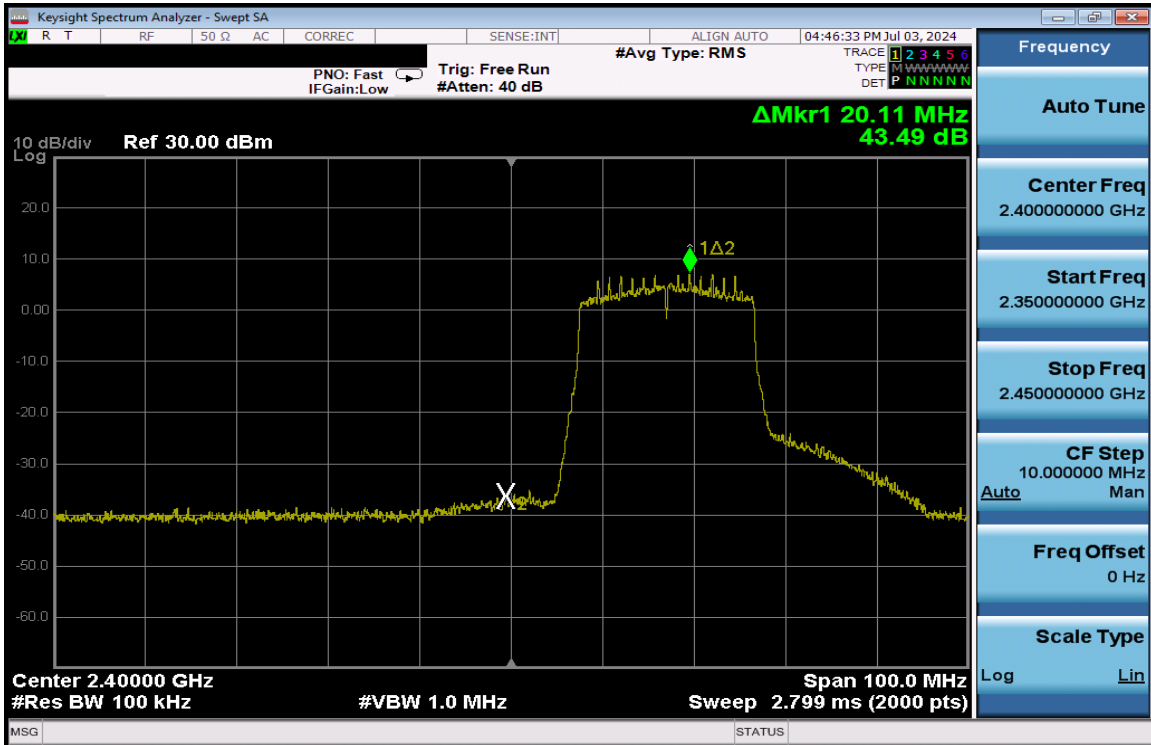
Plot 7-204. Band Edge Plot Antenna 3a (802.11ax (SU - 2.4GHz) – Ch. 2) – MCS2
