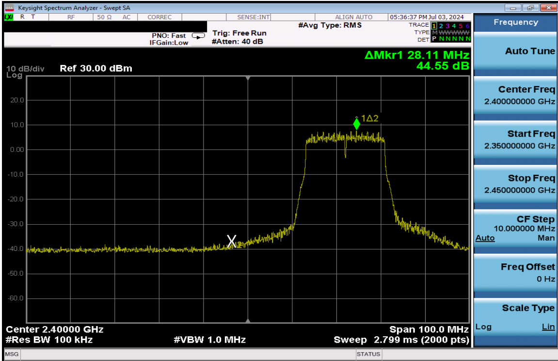
Plot 7-277. Band Edge Plot Antenna 3a (802.11n (2.4GHz) – Ch. 3) – MCS7
