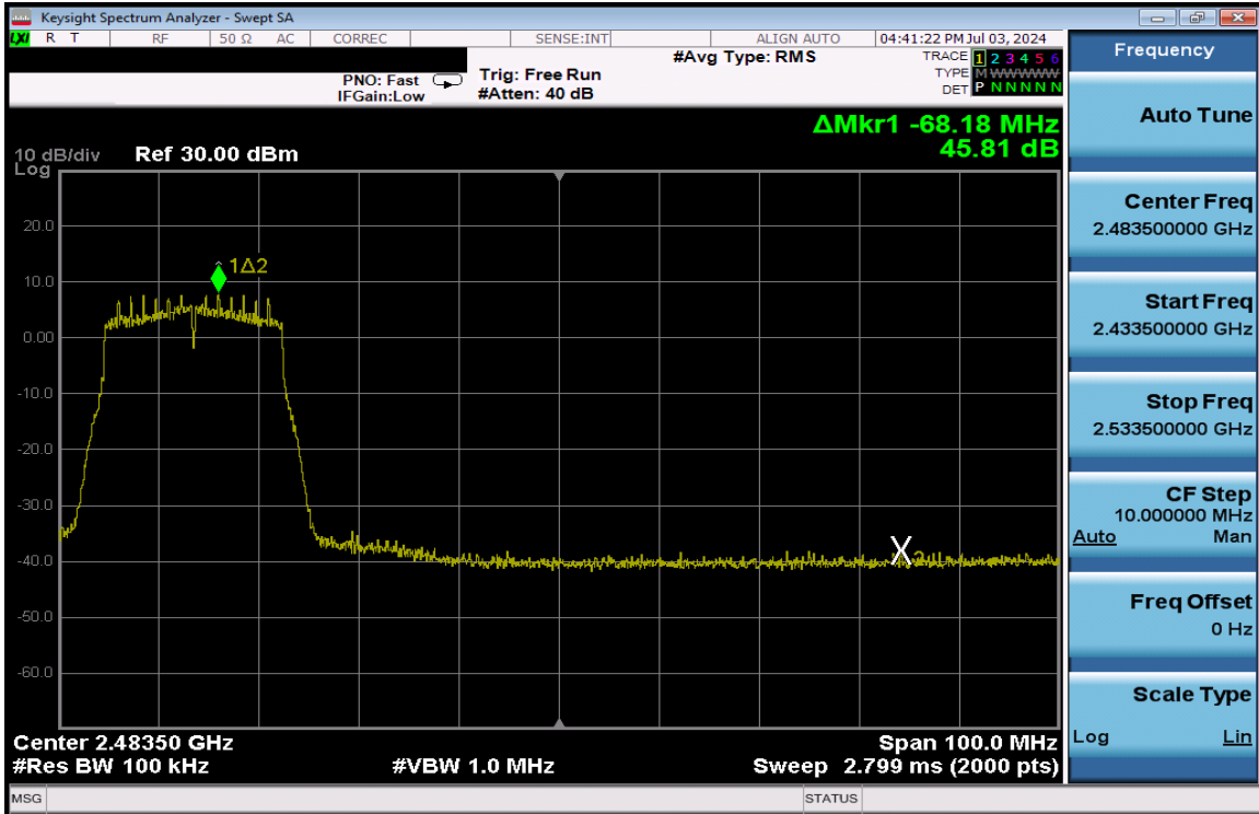
Plot 7-197. Band Edge Plot Antenna 3a (802.11n (2.4GHz) – Ch. 8) – MCS2
