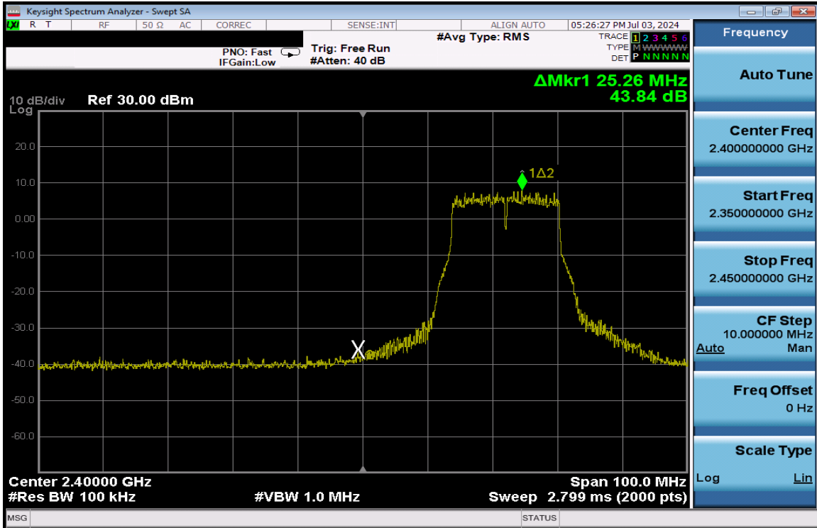
Plot 7-263. Band Edge Plot Antenna 3a (802.11g – Ch. 3) – 54Mbps
