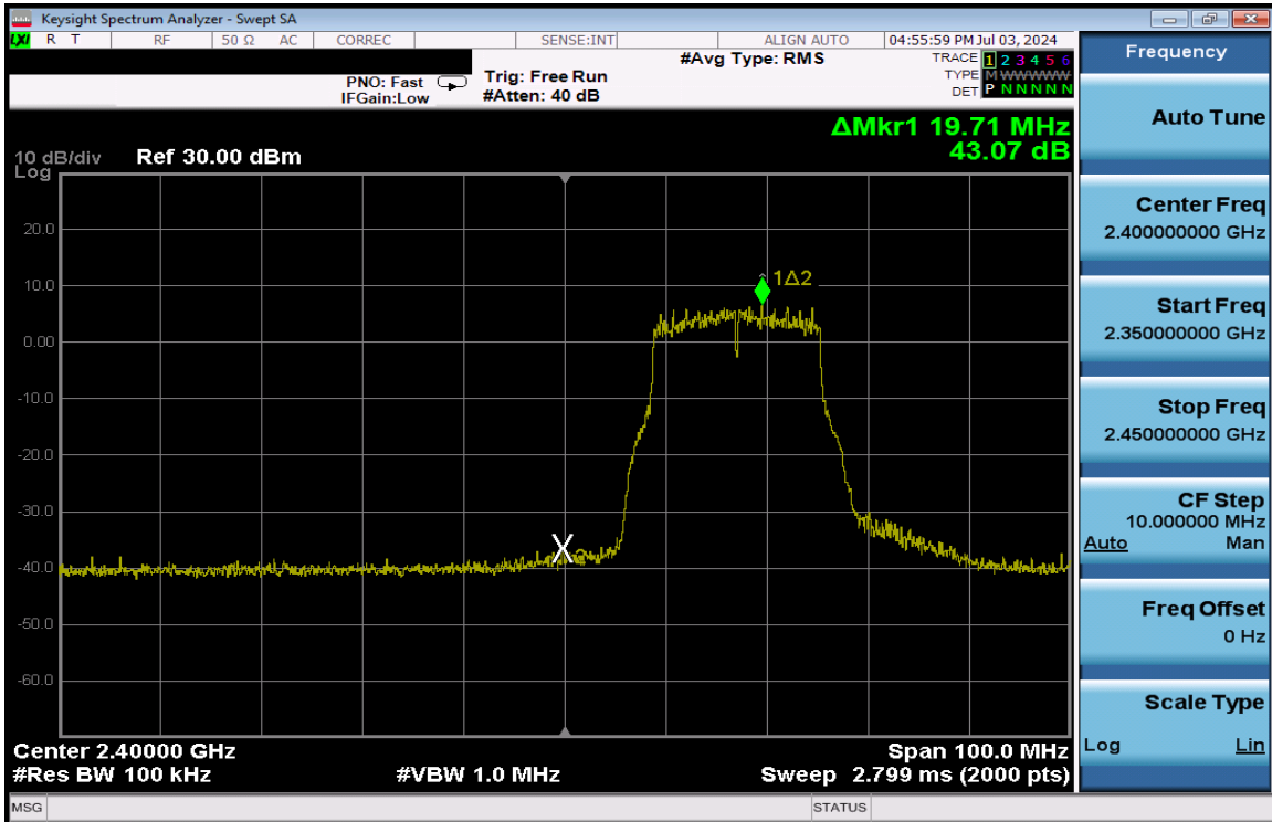
Plot 7-217. Band Edge Plot Antenna 3a (802.11g – Ch. 2) – 24Mbps
