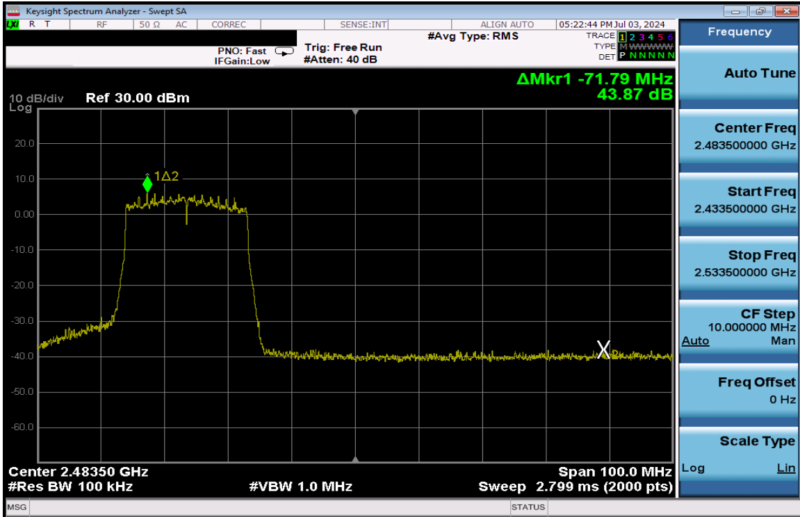
Plot 7-254. Band Edge Plot Antenna 3a (802.11ax (SU - 2.4GHz) – Ch. 10) – MCS4
