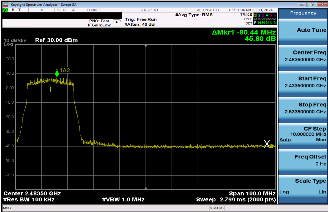
Plot 7-238. Band Edge Plot Antenna 3a (802.11n (2.4GHz) – Ch. 8) – MCS4
