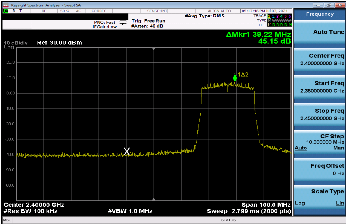
Plot 7-247. Band Edge Plot Antenna 3a (802.11ax (SU - 2.4GHz) – Ch. 4) – MCS4
