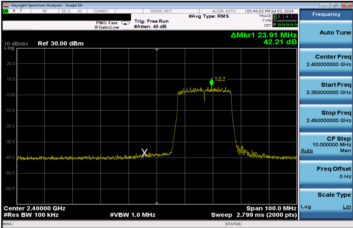
Plot 7-290. Band Edge Plot Antenna 3a (802.11ax (SU - 2.4GHz) - Ch. 2) - MCS9
