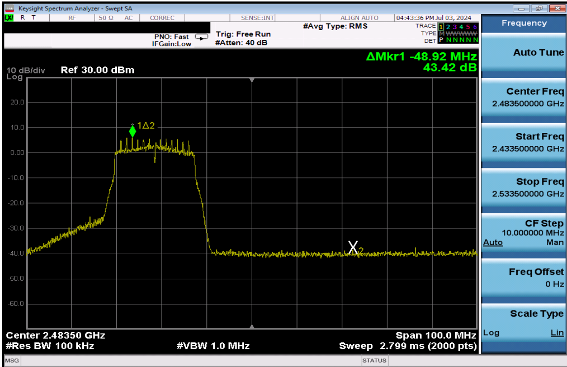
Plot 7-200. Band Edge Plot Antenna 3a (802.11n (2.4GHz) – Ch. 11) – MCS2
