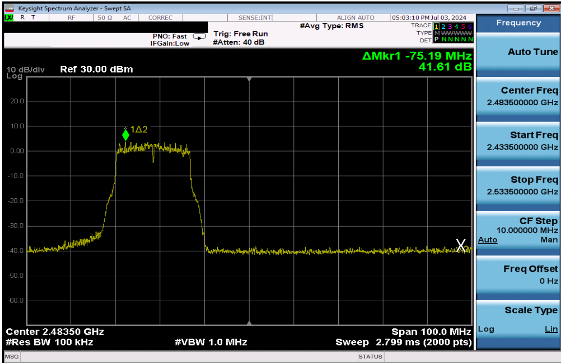
Plot 7-227. Band Edge Plot Antenna 3a (802.11g – Ch. 11) – 24Mbps
