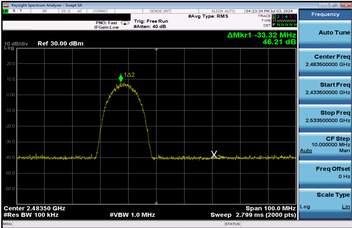
Plot 7-260. Band Edge Plot Antenna 3a (802.11b – Ch. 13) – 11Mbps
