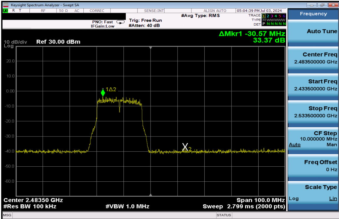
Plot 7-229. Band Edge Plot Antenna 3a (802.11g – Ch. 13) – 24Mbps
