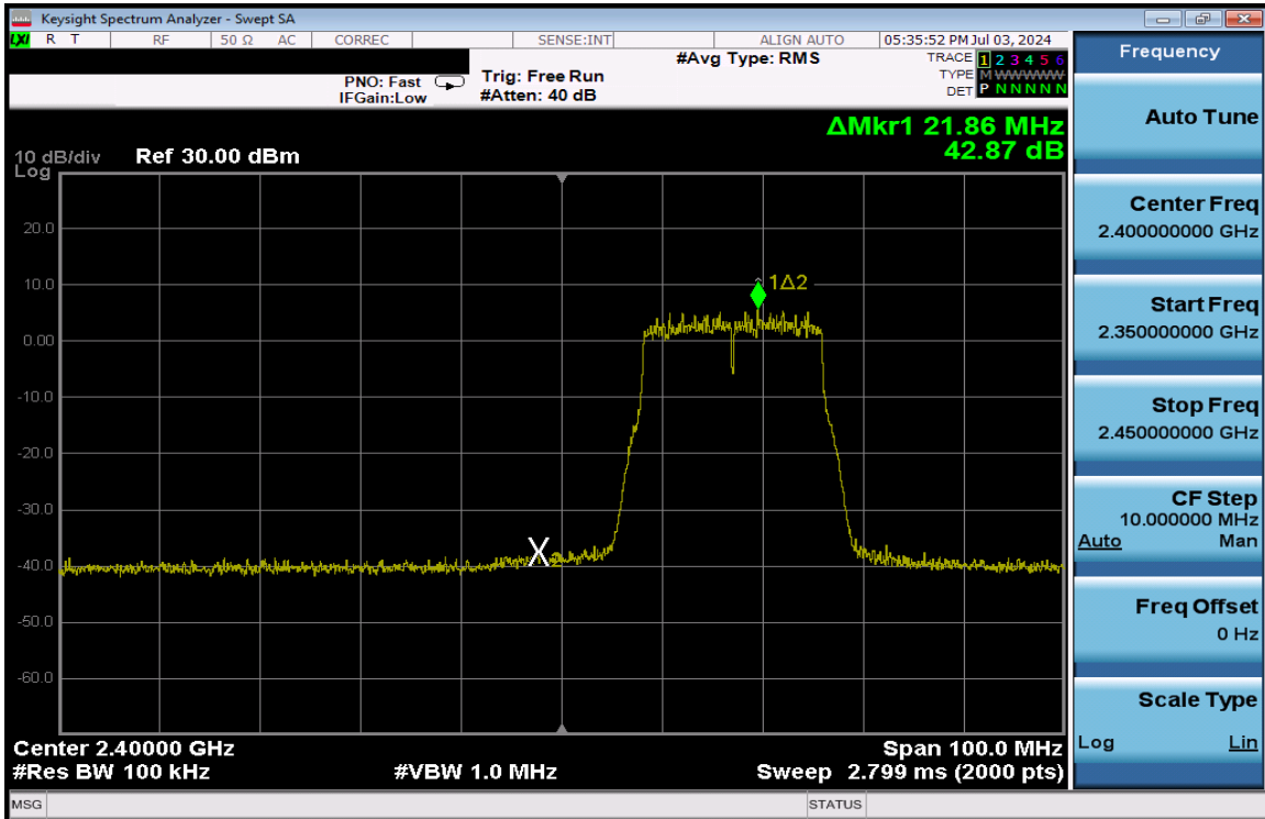
Plot 7-276. Band Edge Plot Antenna 3a (802.11n (2.4GHz) – Ch. 2) – MCS7
