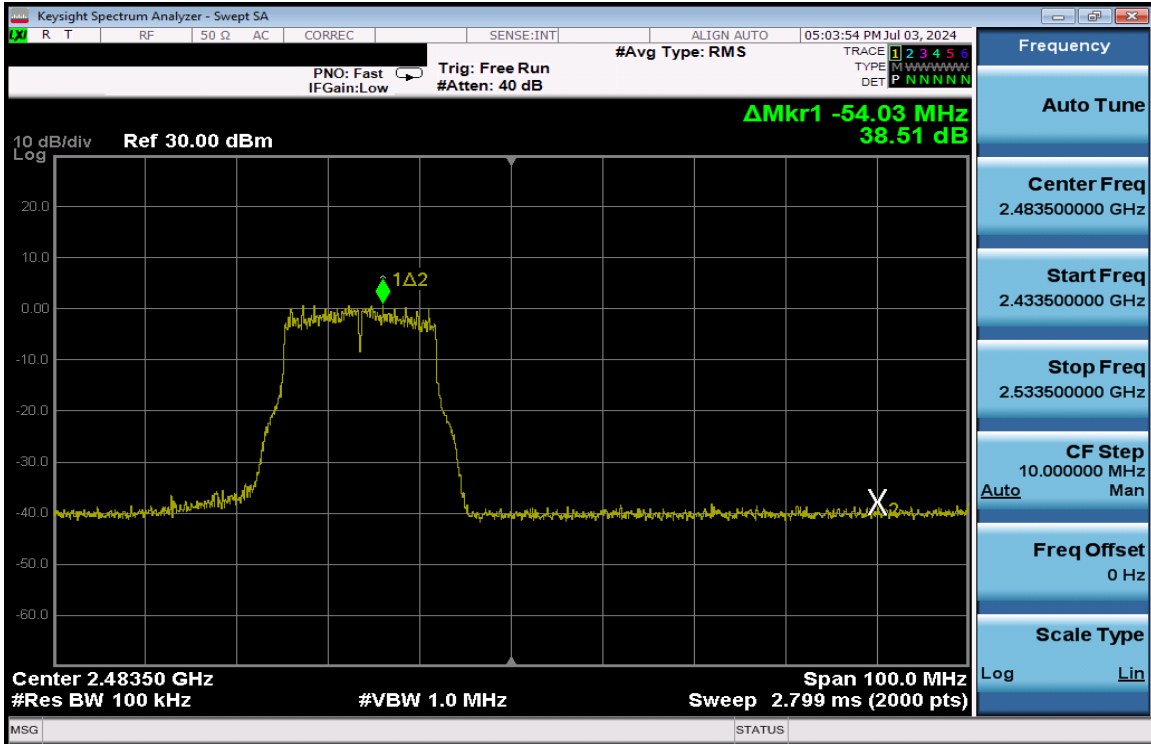
Plot 7-228. Band Edge Plot Antenna 3a (802.11g – Ch. 12) – 24Mbps
