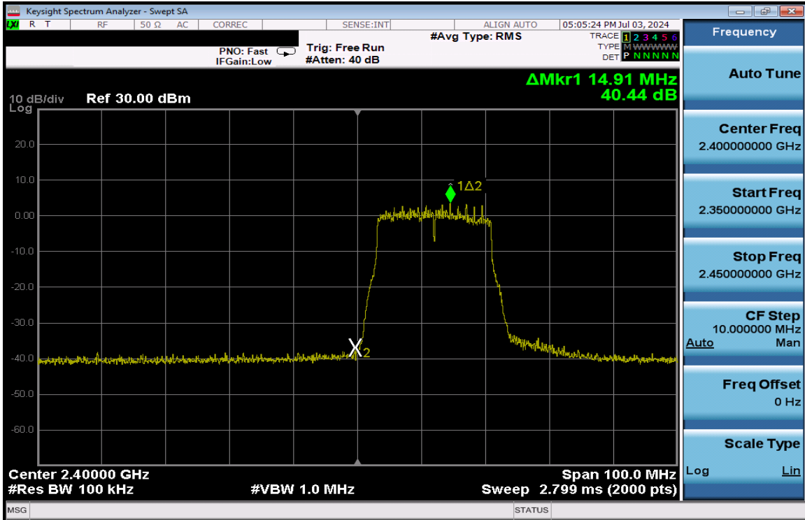
Plot 7-230. Band Edge Plot Antenna 3a (802.11n (2.4GHz) – Ch. 1) – MCS4
