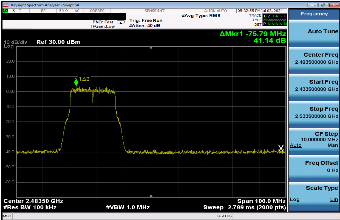
Plot 7-272. Band Edge Plot Antenna 3a (802.11g – Ch. 11) – 54Mbps
