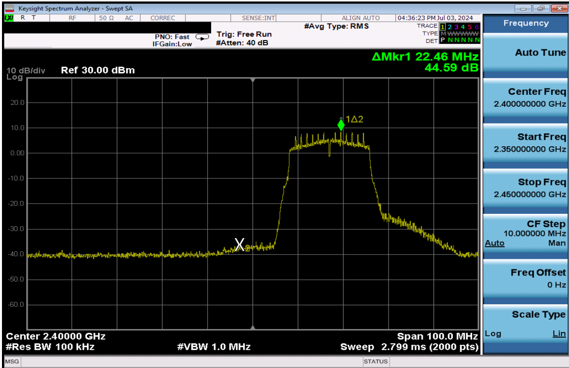
Plot 7-190. Band Edge Plot Antenna 3a (802.11n (2.4GHz) – Ch. 2) – MCS2
