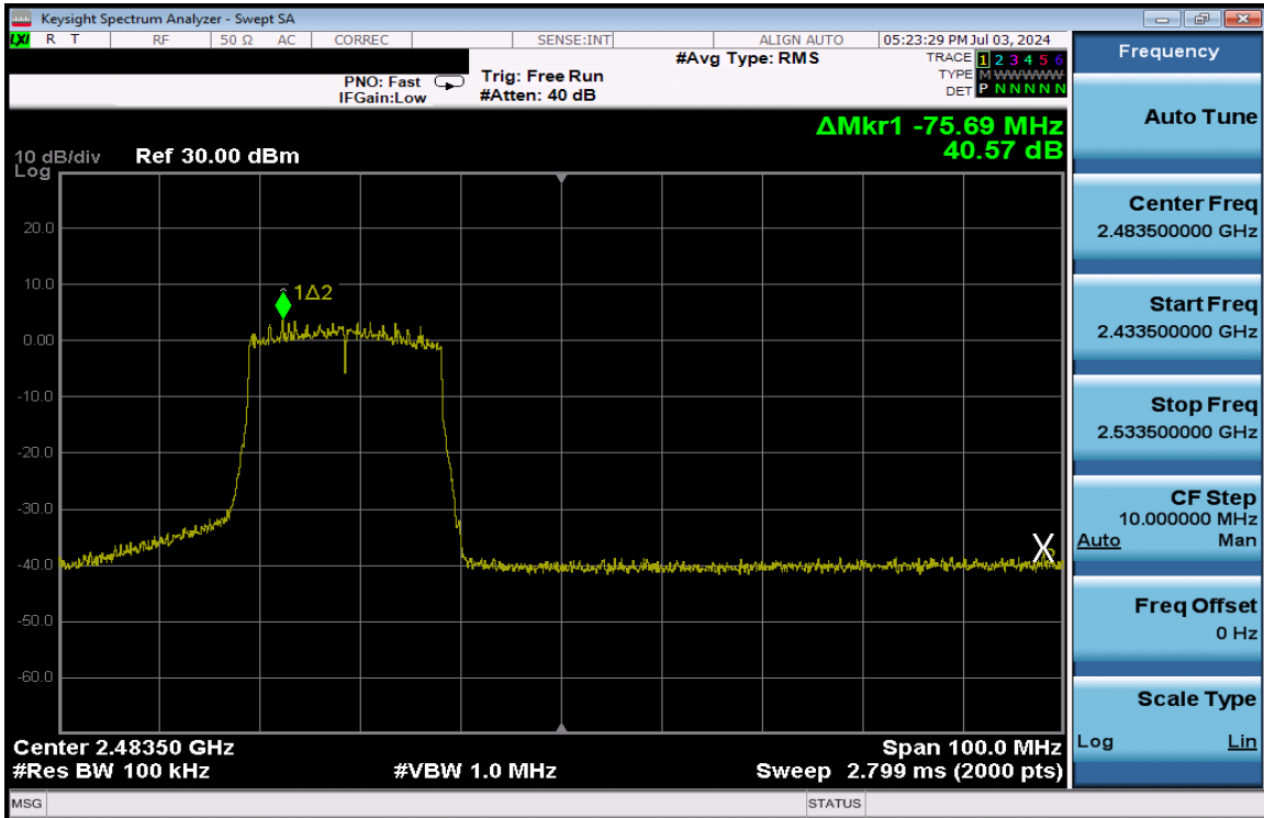
Plot 7-255. Band Edge Plot Antenna 3a (802.11ax (SU - 2.4GHz) – Ch. 11) – MCS4
