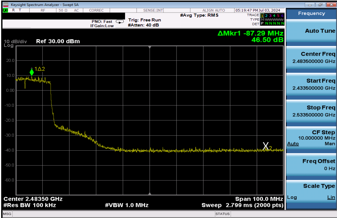
Plot 7-250. Band Edge Plot Antenna 3a (802.11ax (SU - 2.4GHz) – Ch. 6 High) – MCS4
