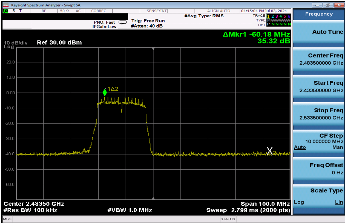
Plot 7-202. Band Edge Plot Antenna 3a (802.11n (2.4GHz) – Ch. 13) – MCS2
