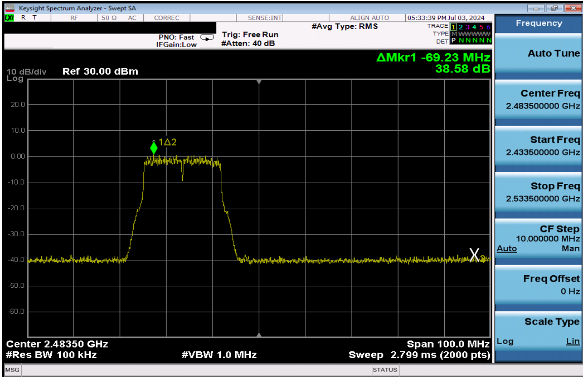
Plot 7-273. Band Edge Plot Antenna 3a (802.11g – Ch. 12) – 54Mbps
