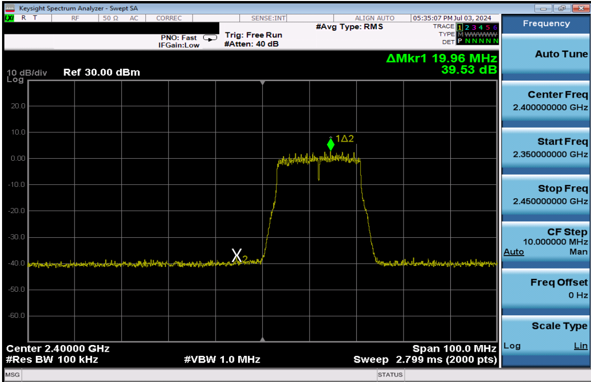
Plot 7-275. Band Edge Plot Antenna 3a (802.11n (2.4GHz) – Ch. 1) – MCS7
