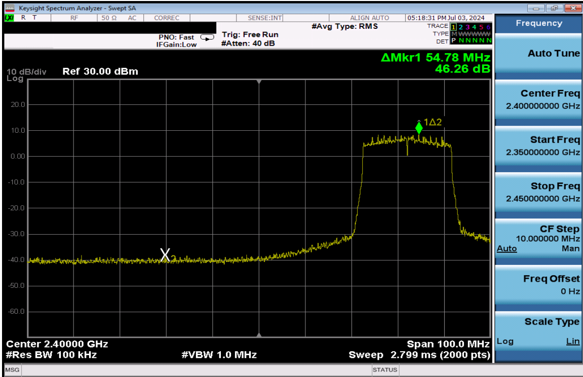
Plot 7-248. Band Edge Plot Antenna 3a (802.11ax (SU - 2.4GHz) – Ch. 5) – MCS4
