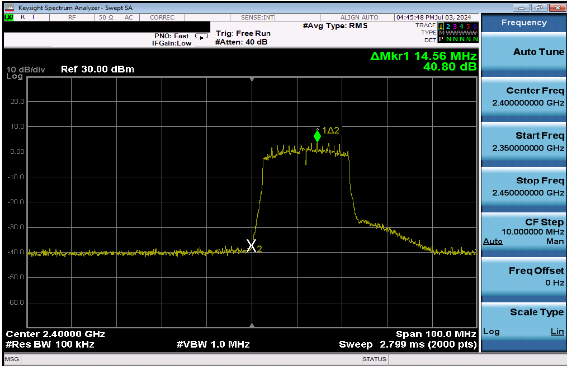
Plot 7-203. Band Edge Plot Antenna 3a (802.11ax (SU - 2.4GHz) – Ch. 1) – MCS2
