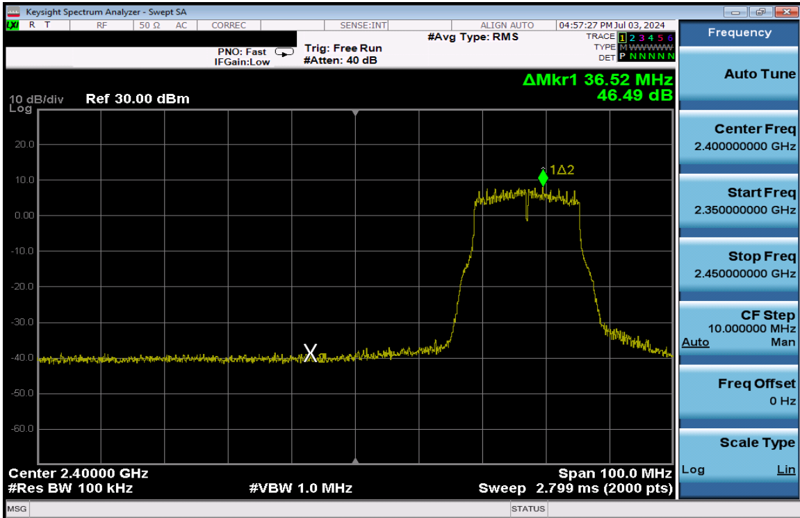
Plot 7-219. Band Edge Plot Antenna 3a (802.11g – Ch. 4) – 24Mbps
