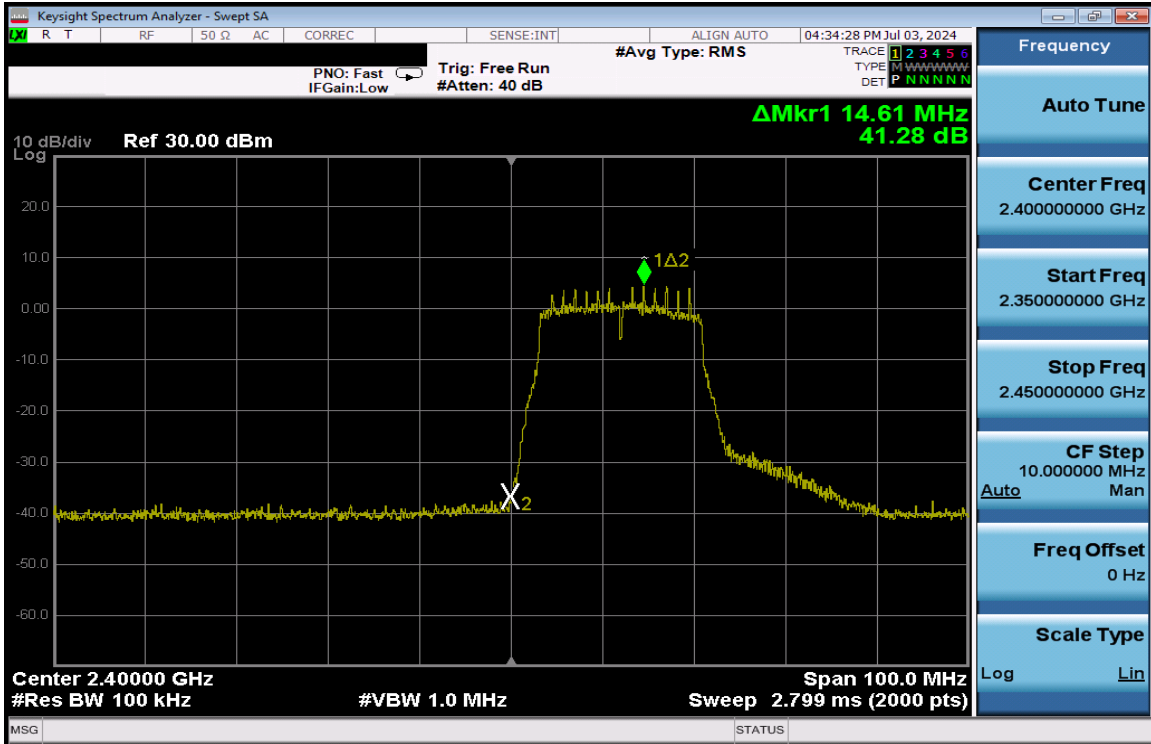
Plot 7-189. Band Edge Plot Antenna 3a (802.11n (2.4GHz) – Ch. 1) – MCS2
