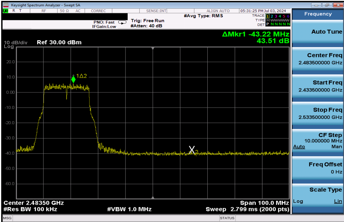
Plot 7-270. Band Edge Plot Antenna 3a (802.11g – Ch. 9) – 54Mbps
