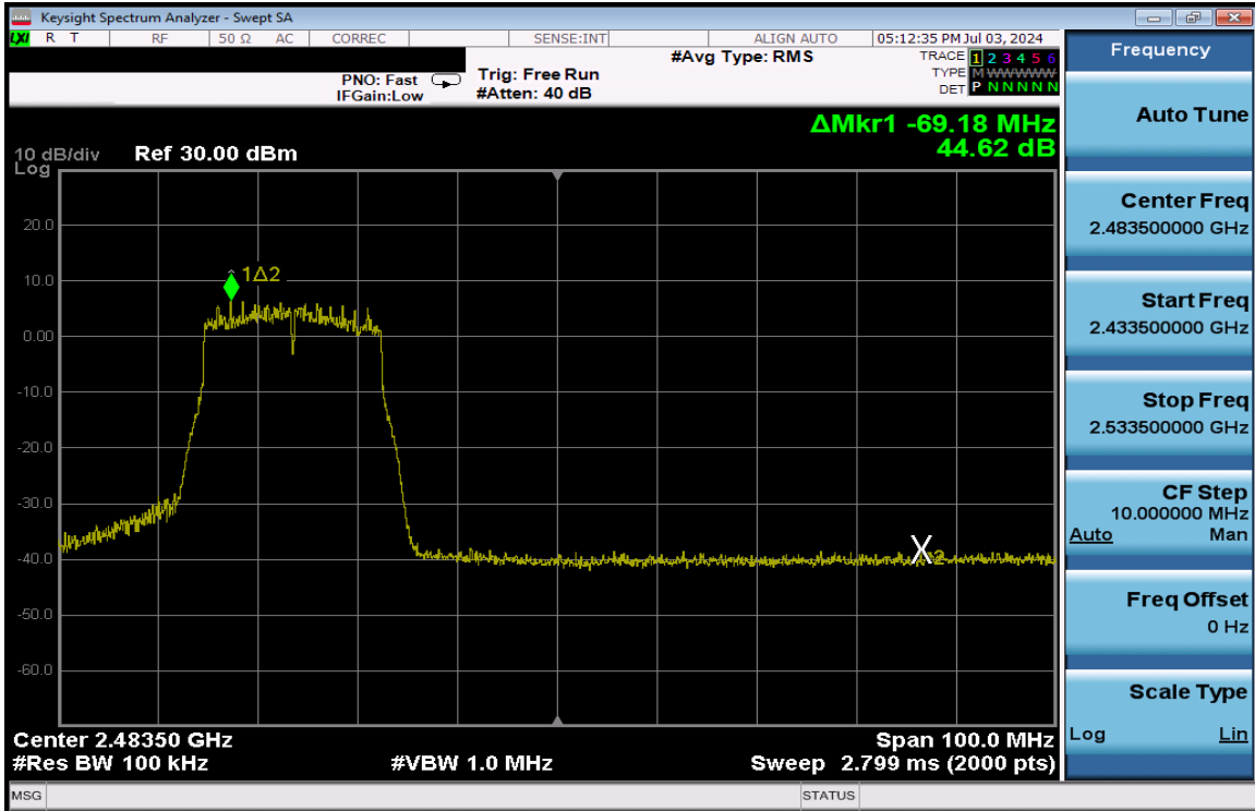
Plot 7-240. Band Edge Plot Antenna 3a (802.11n (2.4GHz) – Ch. 10) – MCS4
