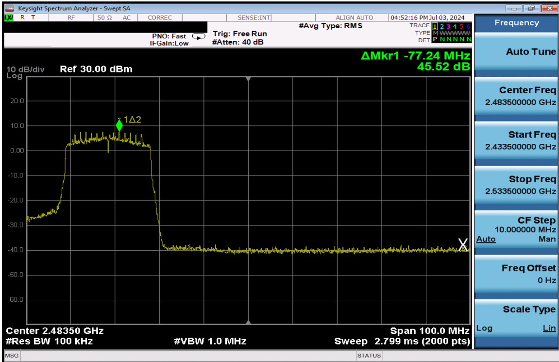
Plot 7-212. Band Edge Plot Antenna 3a (802.11ax (SU - 2.4GHz) – Ch. 9) – MCS2
