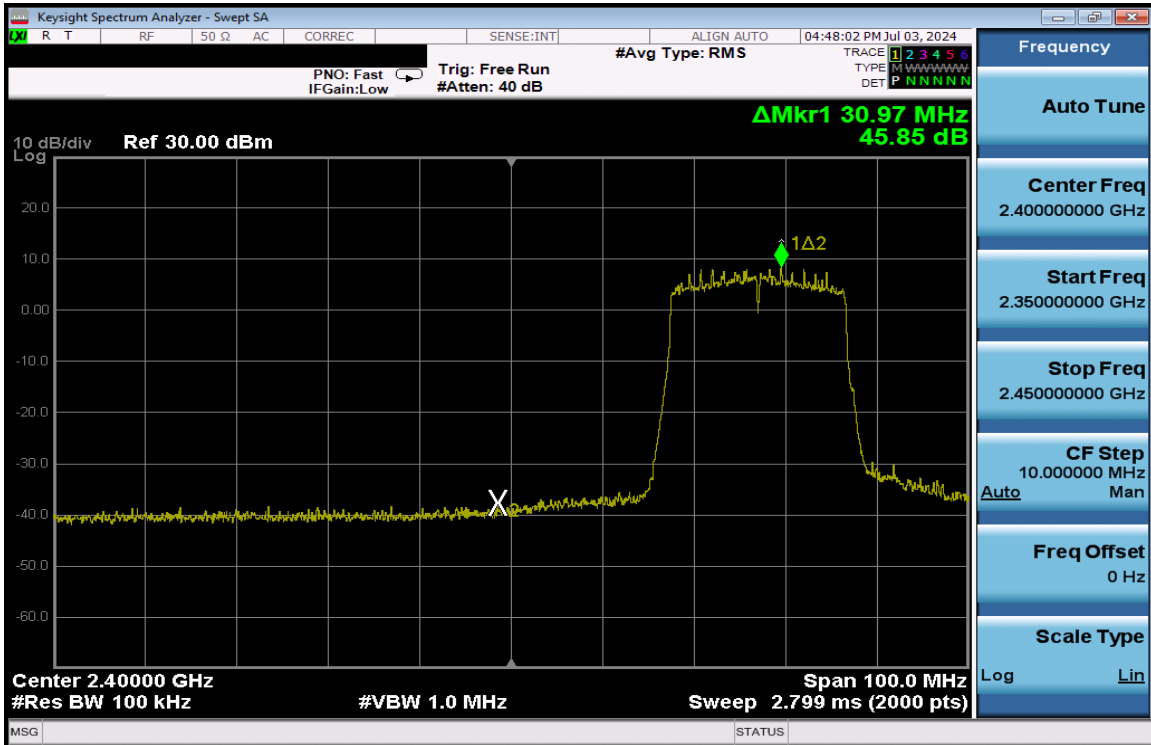
Plot 7-206. Band Edge Plot Antenna 3a (802.11ax (SU - 2.4GHz) – Ch. 4) – MCS2
