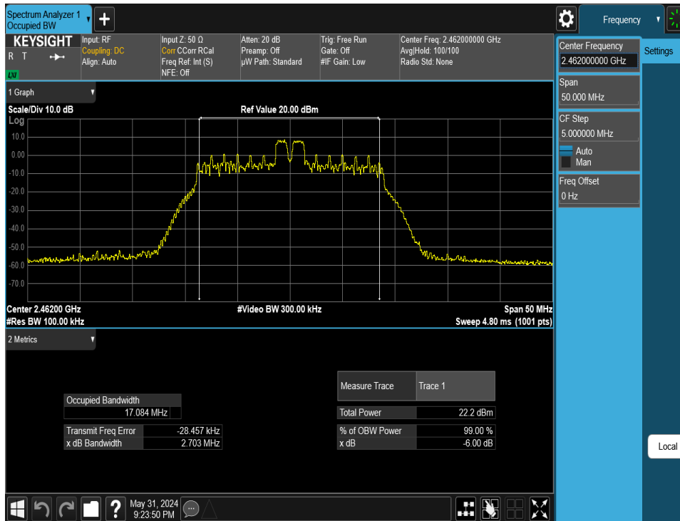
Plot 7-8. 6dB BW & 99% OBW Antenna 3a (802.11ax OFDMA – RU26 Index 4 – Ch. 11)
