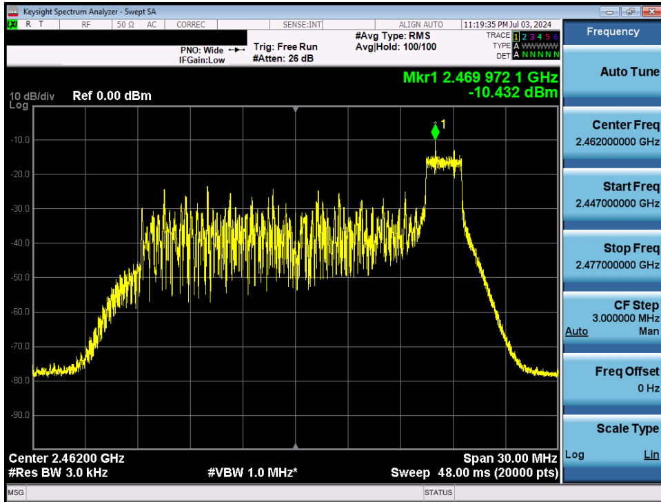
Plot 7-66. Power Spectral Density Plot Antenna 1a (802.11ax OFDMA – RU26 Index 8 – Ch. 11)
