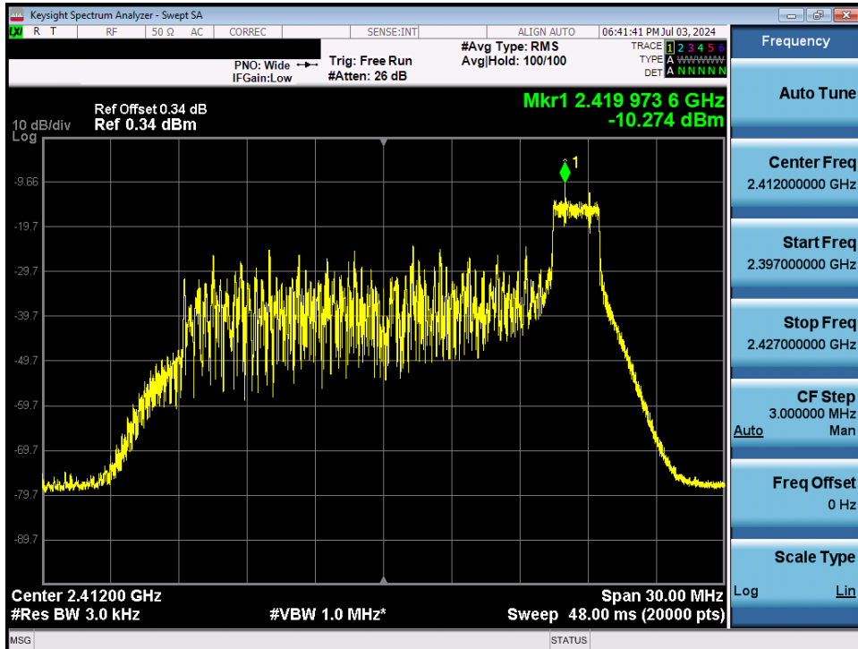
Plot 7-53. Power Spectral Density Plot Antenna 3a (802.11ax OFDMA – RU26 Index 8 – Ch. 1)
