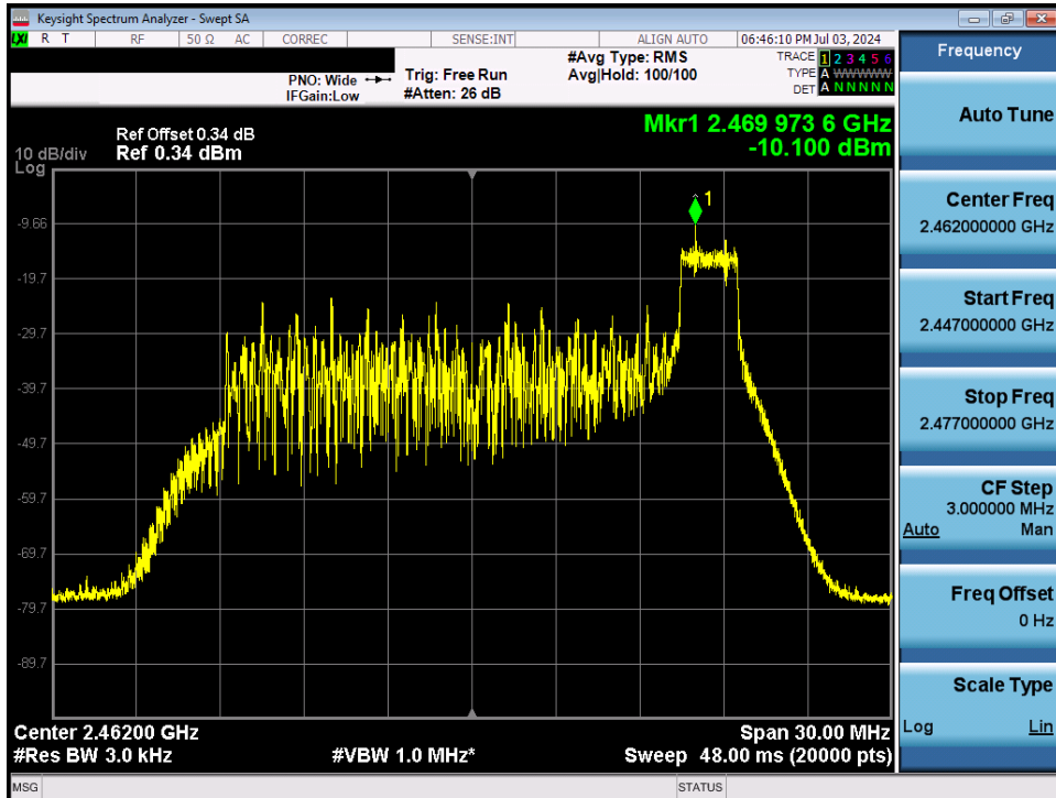
Plot 7-65. Power Spectral Density Plot Antenna 3a (802.11ax OFDMA – RU26 Index 8 – Ch. 11)
