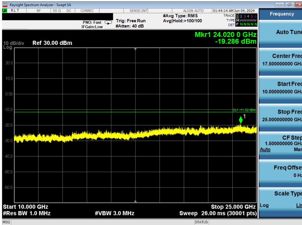
Plot 7-98. Conducted Spurious Plot Antenna 4 (Bluetooth (LE), 1Mbps, iPA – Ch. 0)
