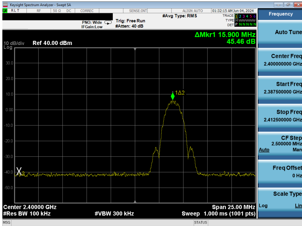
Plot 7-83. Band Edge Plot Antenna 4 (Bluetooth (LE), 2Mbps, iPA – Ch. 1)
