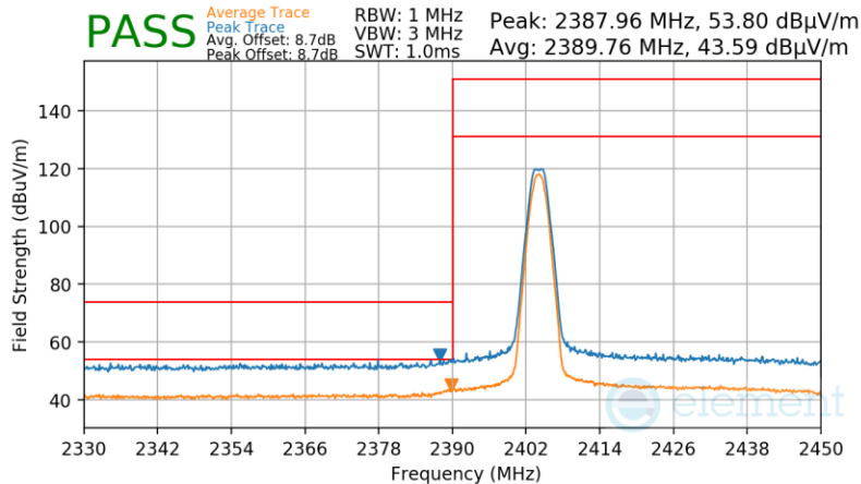
Plot 7-118. Radiated Restricted Lower Band Edge Measurement Antenna 3a (Average & Peak)
