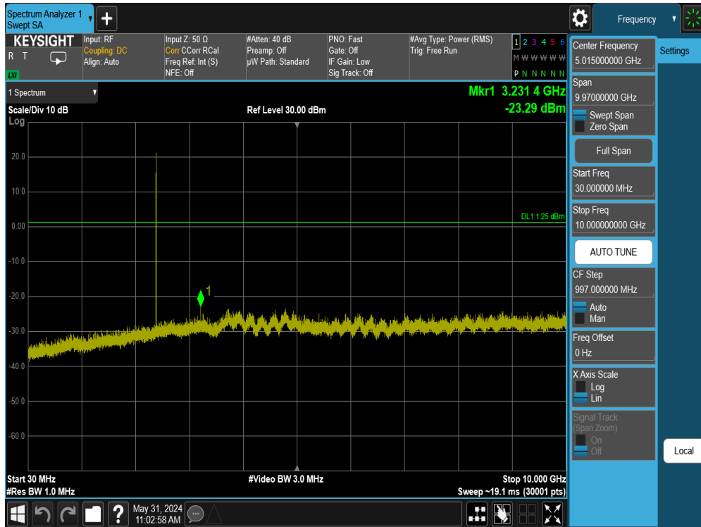
Plot 7-85. Conducted Spurious Plot Antenna 3a (Bluetooth (LE), 1Mbps, ePA – Ch. 0)
