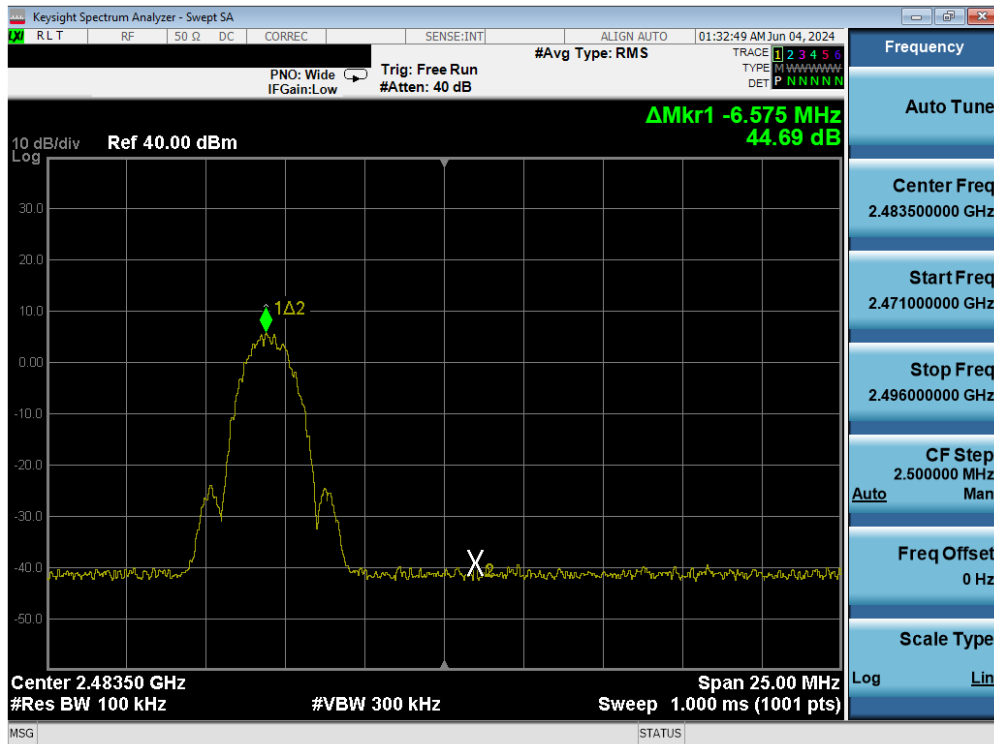
Plot 7-84. Band Edge Plot Antenna 4 (Bluetooth (LE), 2Mbps, iPA – Ch. 38)
