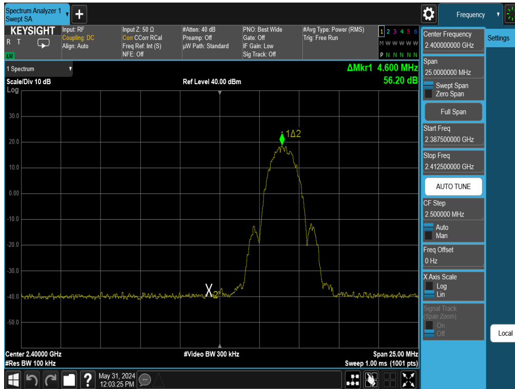
Plot 7-79. Band Edge Plot Antenna 1a (Bluetooth (LE), 2Mbps, ePA – Ch. 1)
