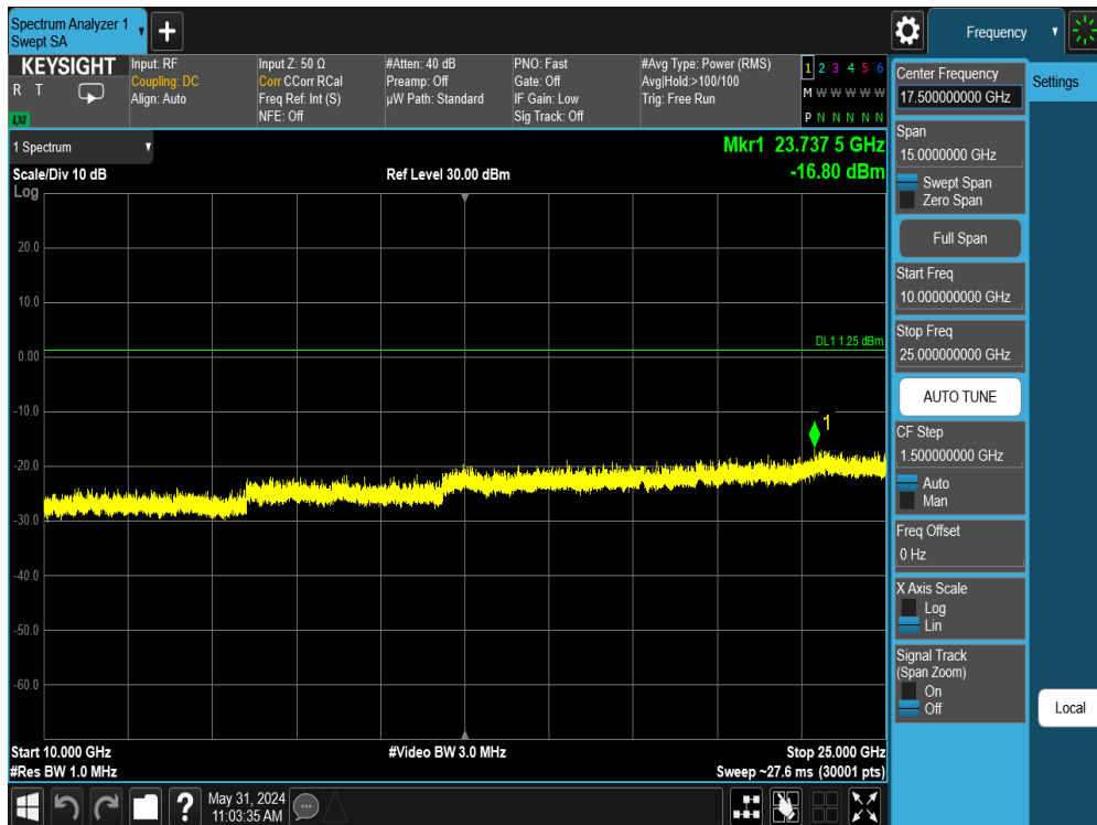
Plot 7-86. Conducted Spurious Plot Antenna 3a (Bluetooth (LE), 1Mbps, ePA – Ch. 0)
