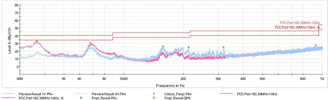
Plot 7-132. Radiated Spurious Emissions Below 1GHz TxBF (1Mbps, ePA – Ch.39, Pol. H & V, with AC/DC Adapter and USB-C Cable)
