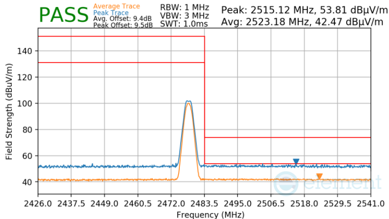
Plot 7-127. Radiated Restricted Upper Band Edge Measurement Antenna 4 (Average & Peak)
