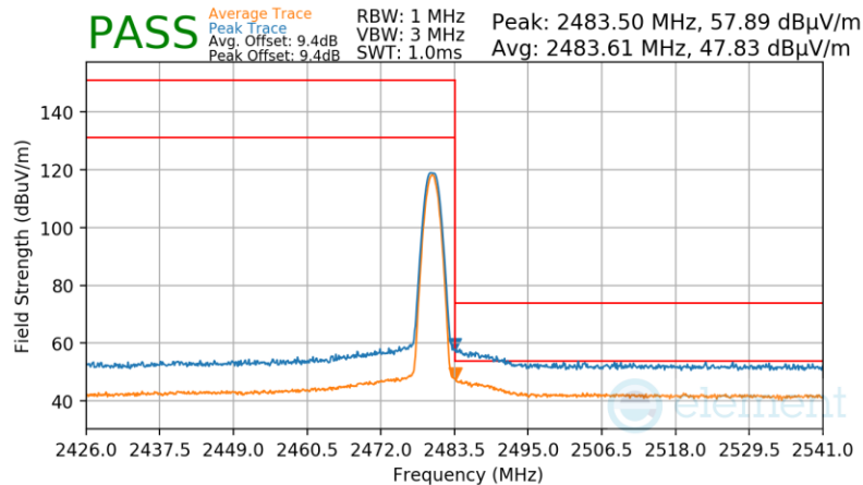
Plot 7-117. Radiated Restricted Upper Band Edge Measurement Antenna 3a (Average & Peak)
