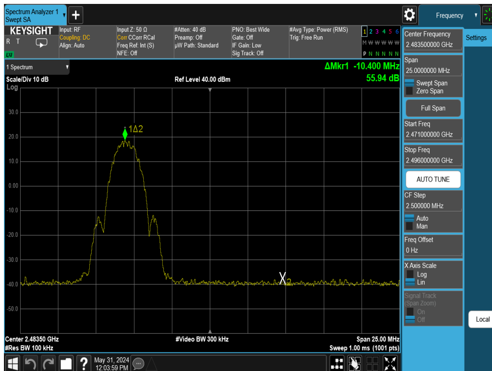
Plot 7-80. Band Edge Plot Antenna 1a (Bluetooth (LE), 2Mbps, ePA – Ch. 38)
