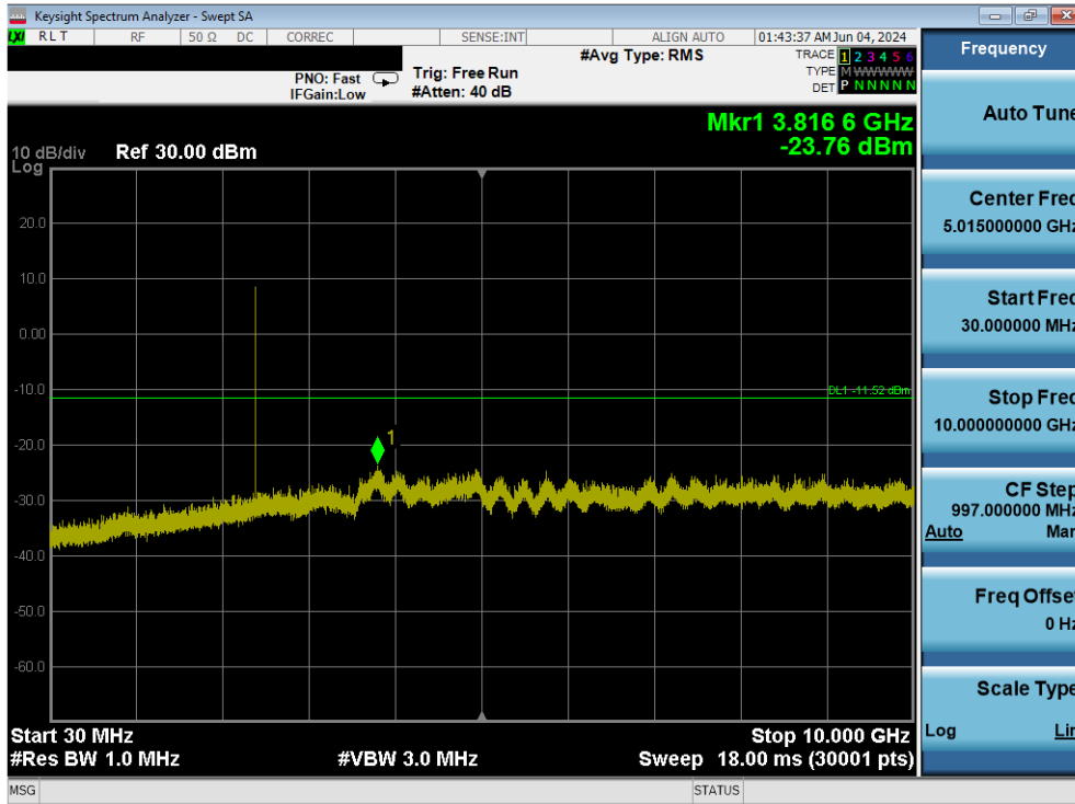
Plot 7-97. Conducted Spurious Plot Antenna 4 (Bluetooth (LE), 1Mbps, iPA – Ch. 0)
