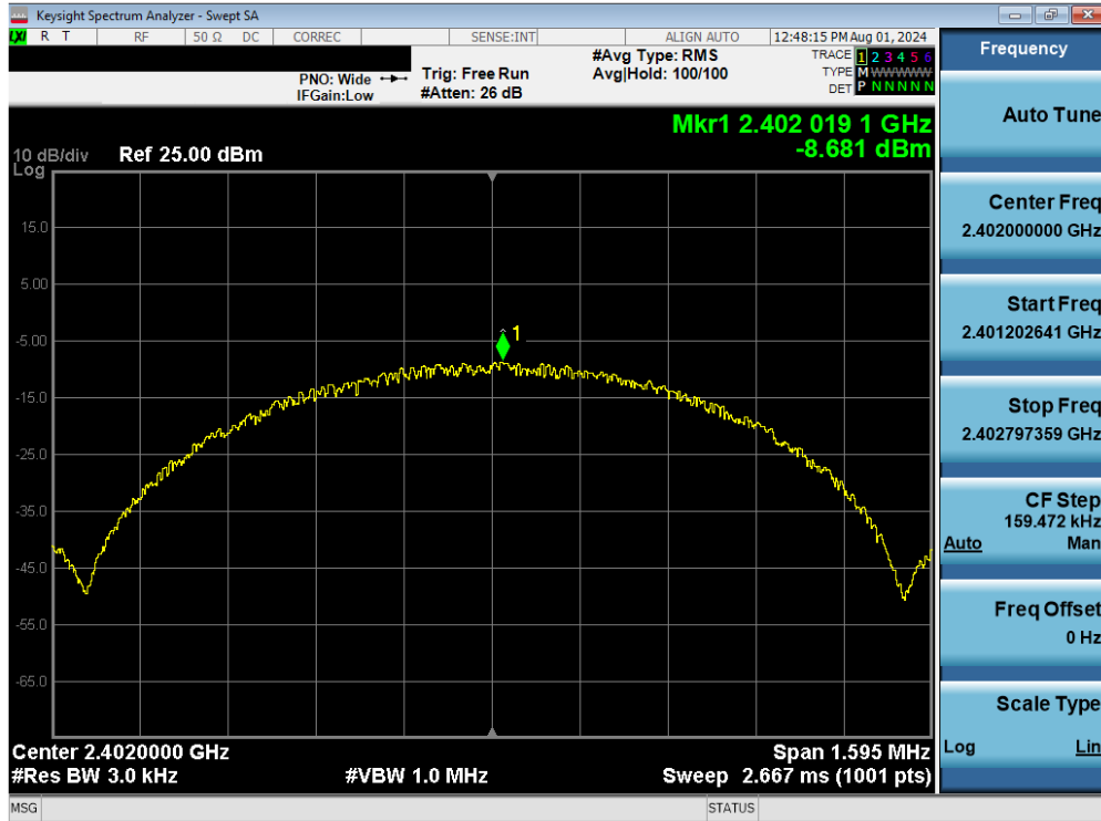
Plot 7-43. Power Spectral Density Plot Antenna 4 (Bluetooth (LE), 1Mbps, iPA – Ch. 0)
