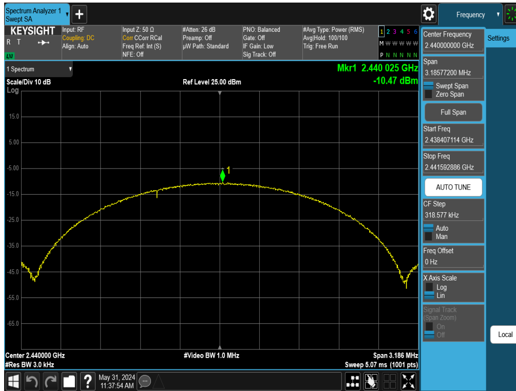
Plot 7-41. Power Spectral Density Plot Antenna 1a (Bluetooth (LE), 2Mbps, iPA – Ch. 19)
