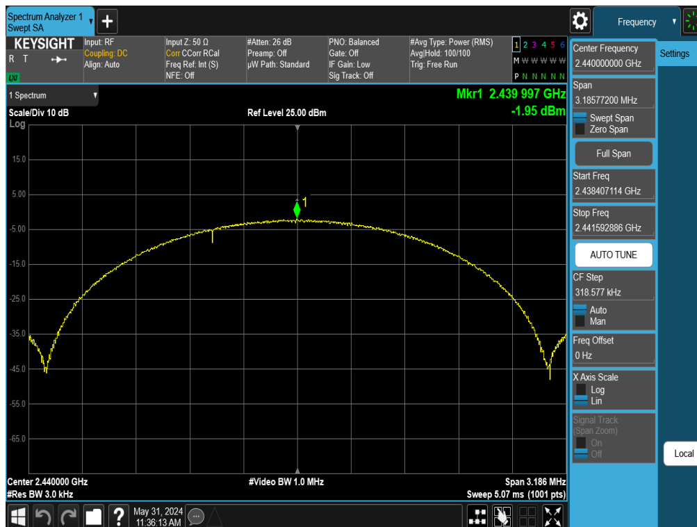
Plot 7-38. Power Spectral Density Plot Antenna 1a (Bluetooth (LE), 2Mbps, ePA – Ch. 19)
