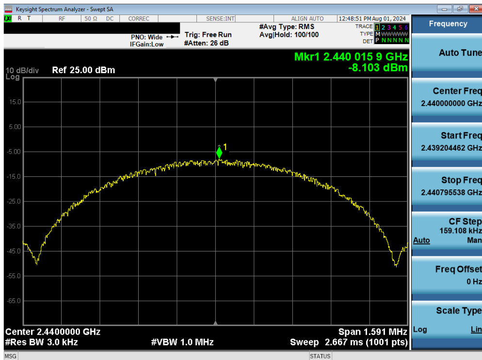
Plot 7-44. Power Spectral Density Plot Antenna 4 (Bluetooth (LE), 1Mbps, iPA – Ch. 19)
