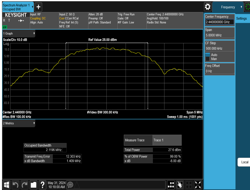
Plot 7-5. 6dB BW & 99% OBW Plot Antenna 3a (Bluetooth (LE), 2Mbps, ePA – Ch. 19)
