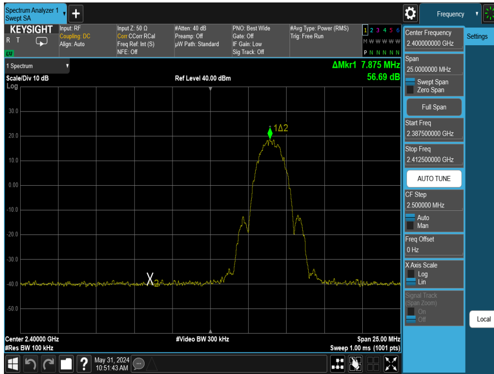
Plot 7-75. Band Edge Plot Antenna 3a (Bluetooth (LE), 2Mbps, ePA – Ch. 1)
