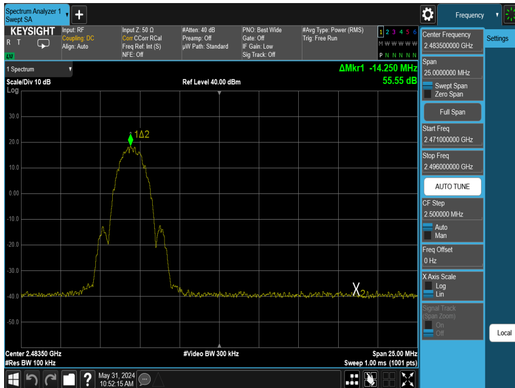
Plot 7-76. Band Edge Plot Antenna 3a (Bluetooth (LE), 2Mbps, ePA – Ch. 38)
