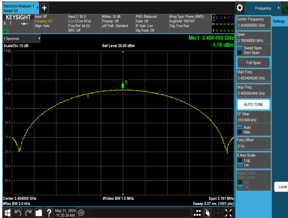
Plot 7-37. Power Spectral Density Plot Antenna 1a (Bluetooth (LE), 2Mbps, ePA – Ch. 1)
