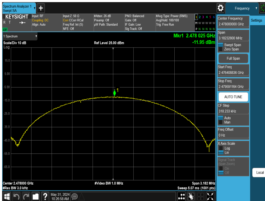
Plot 7-30. Power Spectral Density Plot Antenna 3a (Bluetooth (LE), 2Mbps, iPA – Ch. 38)
