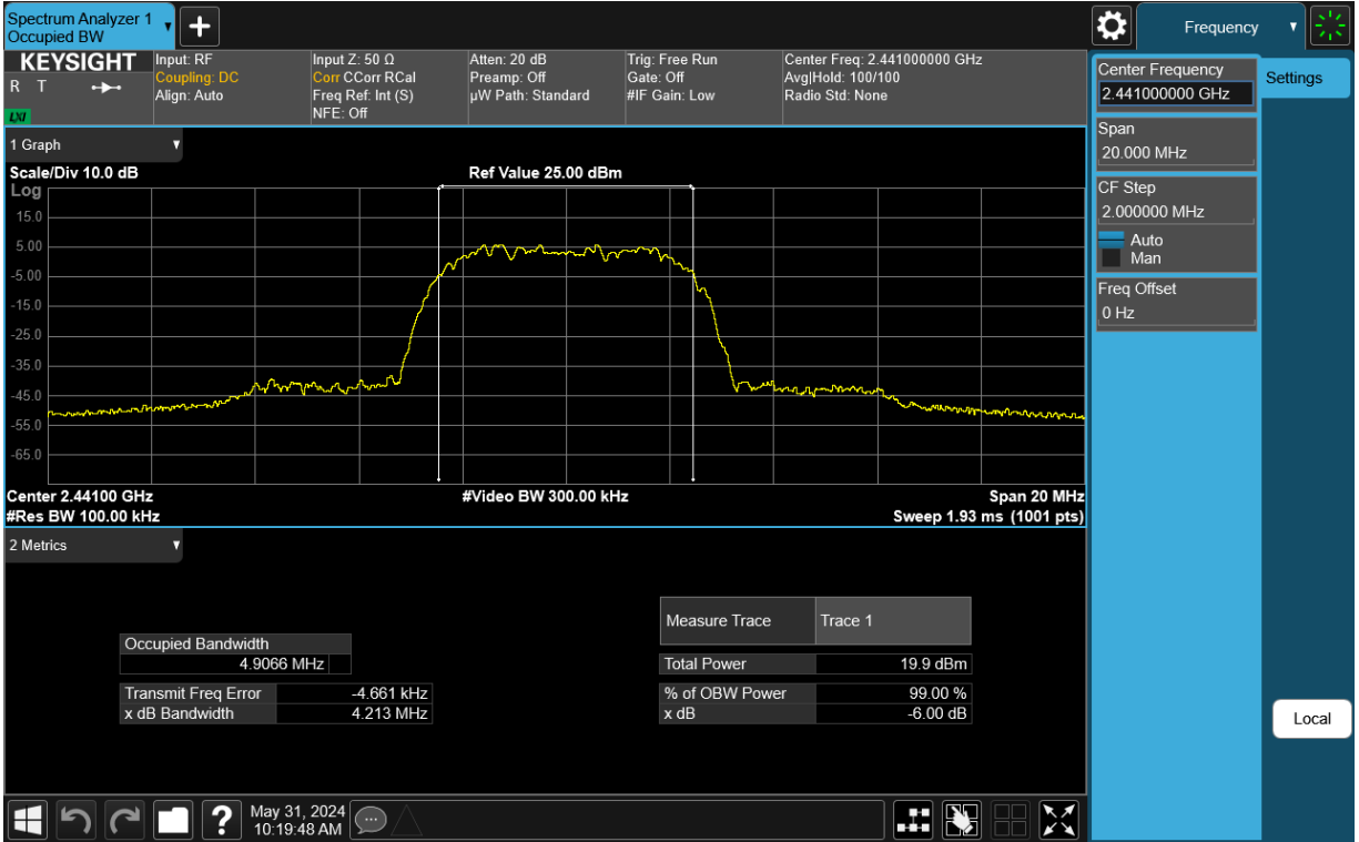
Plot 7-5. 6dB BW & 99% OBW Plot Antenna 3a (Bluetooth (HDR8), 8Mbps, ePA – Ch. 38)
