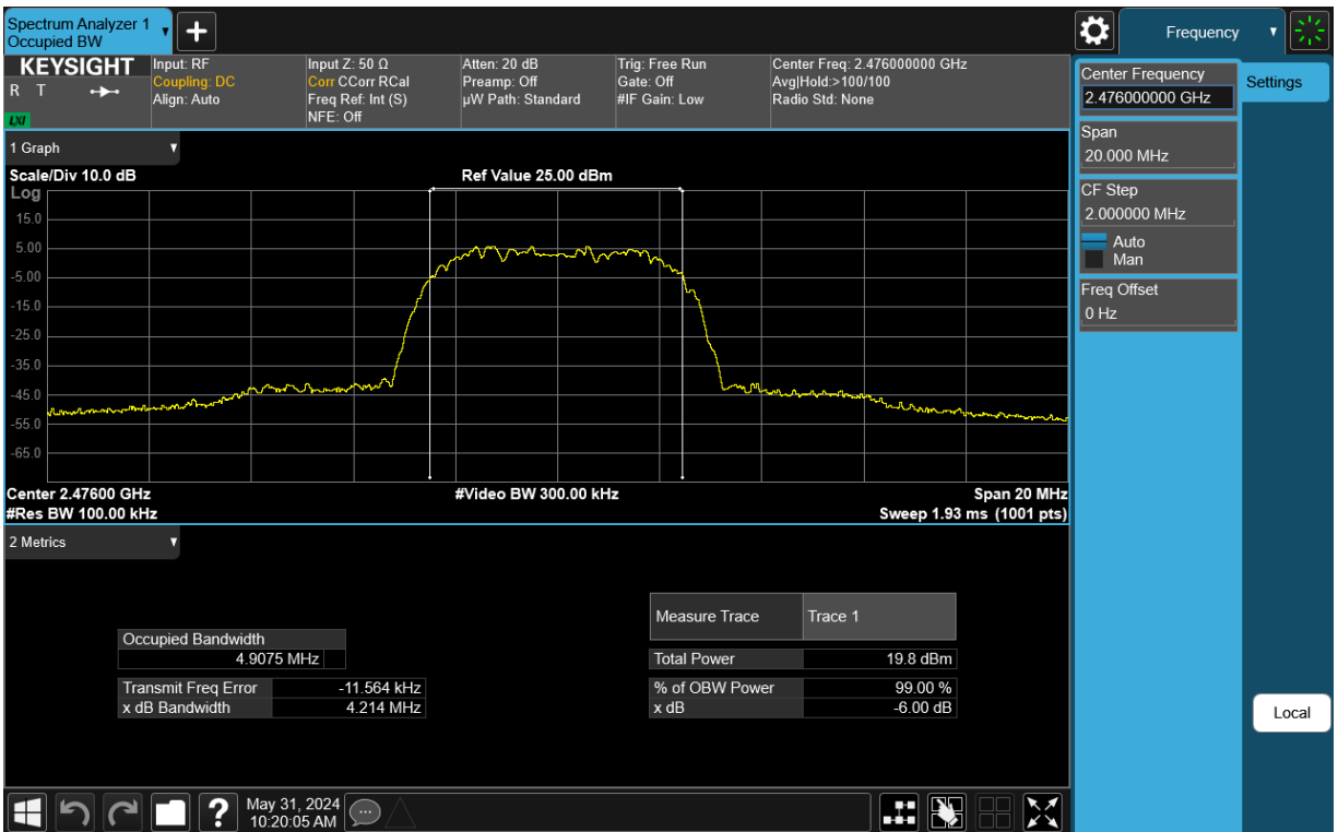
Plot 7-6. 6dB BW & 99% OBW Plot Antenna 3a (Bluetooth (HDR8), 8Mbps, ePA – Ch. 73)
