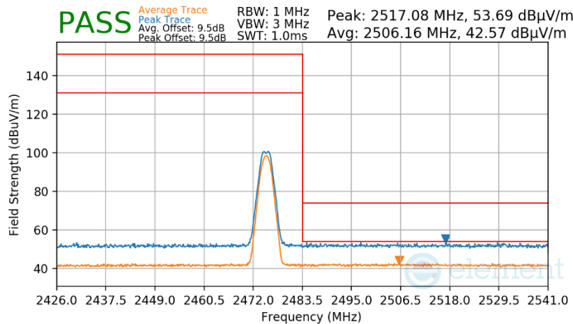
Plot 7-64. Radiated Restricted Upper Band Edge Measurement Antenna 4
