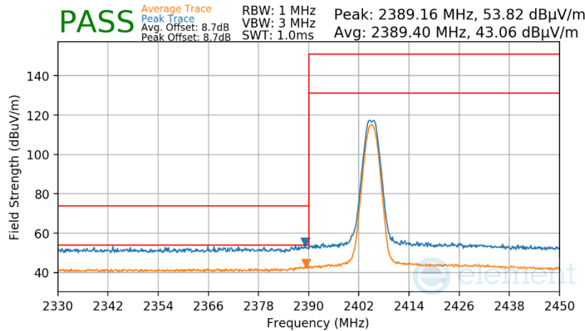
Plot 7-61. Radiated Restricted Lower Band Edge Measurement Antenna 1a
