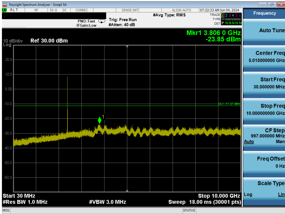
Plot 7-43. Conducted Spurious Antenna 4 (802.15.4, iPA – Ch. 11)
