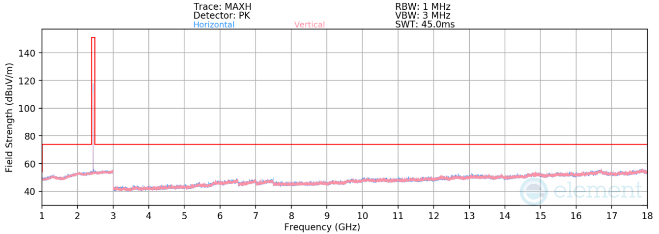
Plot 7-51. Radiated Spurious Emissions 1-18GHz Antenna 3a (802.15.4 ePA – Ch. 18)
