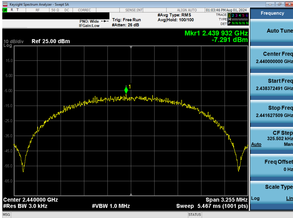
Plot 7-23. Power Spectral Density Antenna 4 (802.15.4, iPA – Ch. 18)
