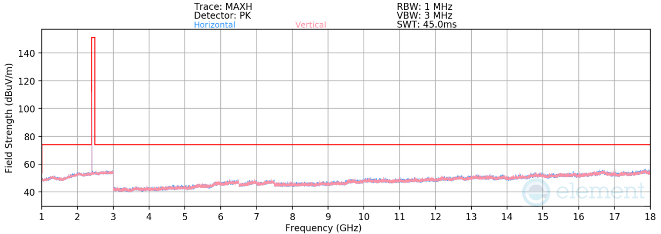
Plot 7-49. Radiated Spurious Emissions 1-18GHz Antenna 3a (802.15.4 ePA – Ch. 11)
