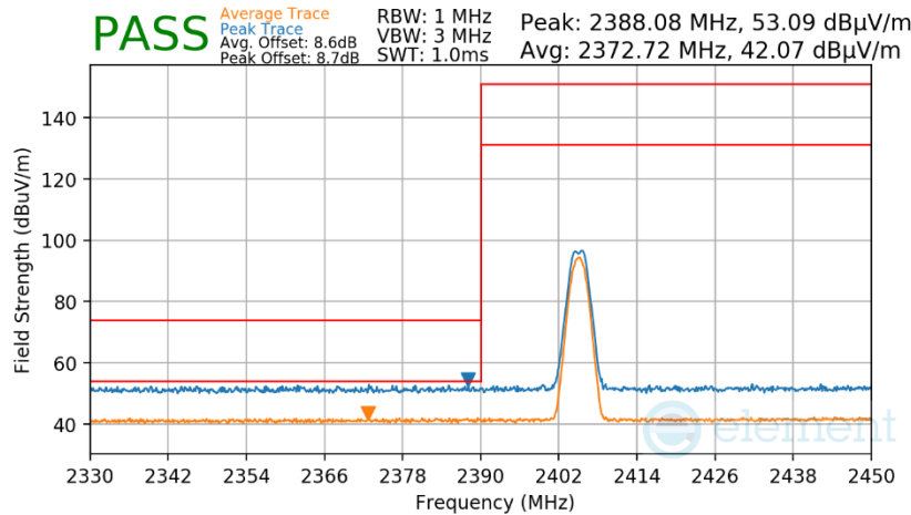
Plot 7-63. Radiated Restricted Lower Band Edge Measurement Antenna 4
