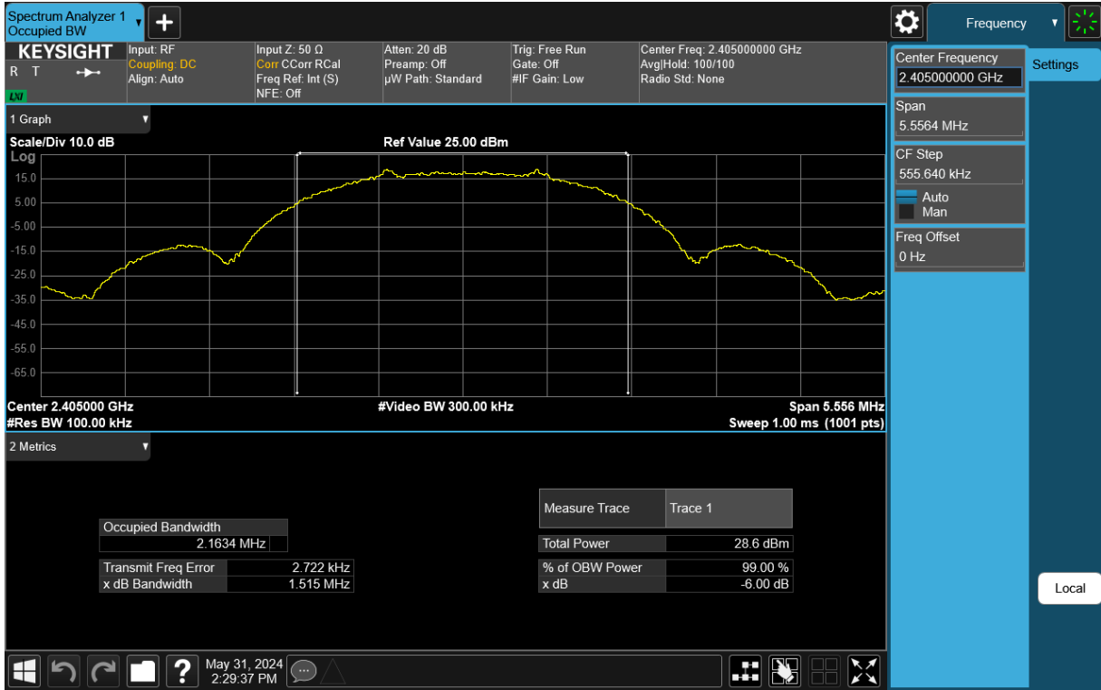
Plot 7-1. 6dB BW & 99% OBW Antenna 3a (802.15.4, Ch. 11)
