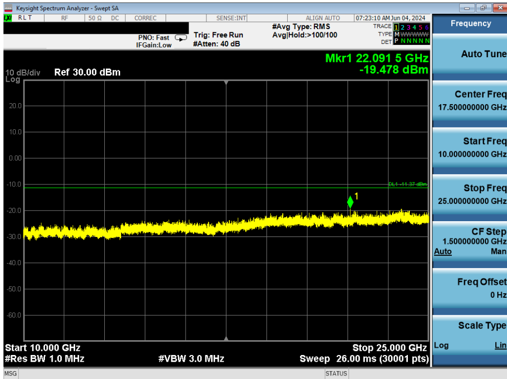
Plot 7-44. Conducted Spurious Antenna 4 (802.15.4, iPA – Ch. 11)
