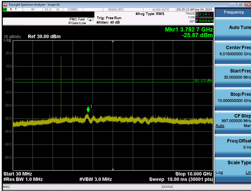
Plot 7-39. Conducted Spurious Antenna 1a (802.15.4, ePA – Ch. 18)
