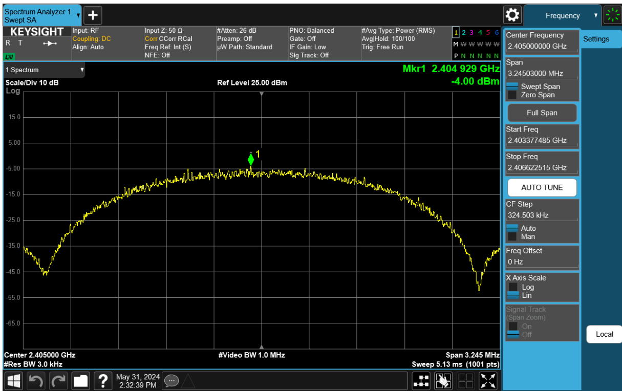
Plot 7-13. Power Spectral Density Antenna 3a (802.15.4, iPA – Ch. 11)
