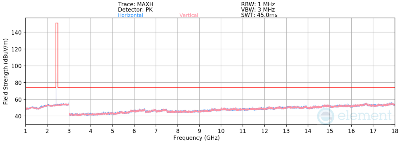
Plot 7-56. Radiated Spurious Emissions 1-18GHz Antenna 4 (802.15.4 iPA – Ch. 11)
