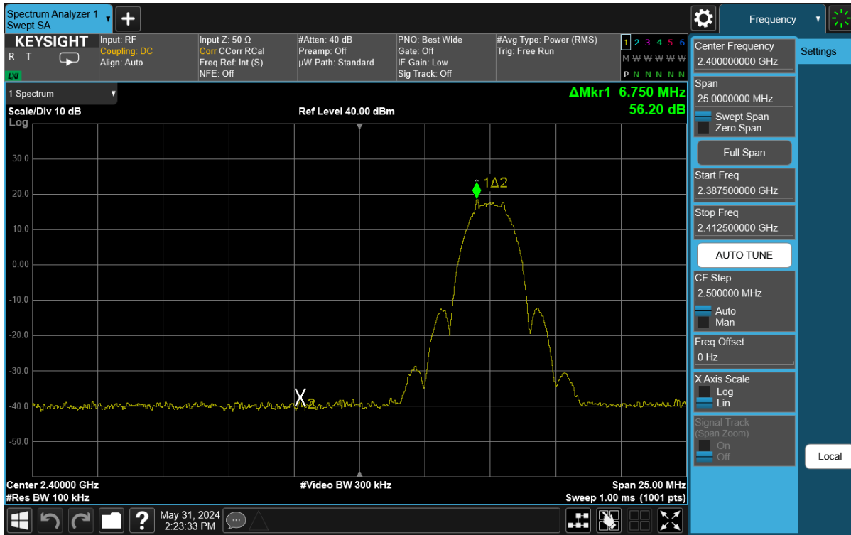
Plot 7-27. Band Edge Antenna 1a (802.15.4, ePA – Ch. 11)
