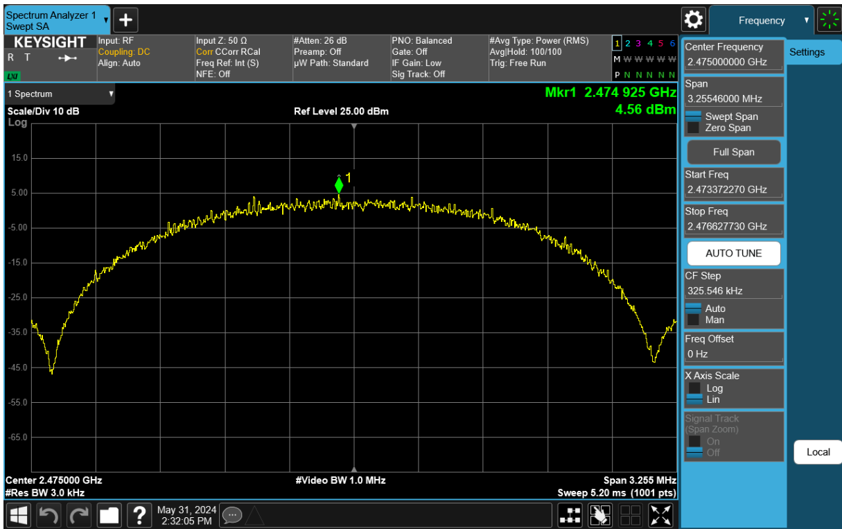
Plot 7-12. Power Spectral Density Antenna 3a (802.15.4, ePA – Ch. 25)
