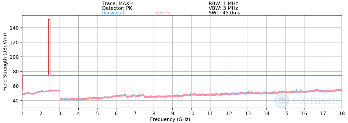
Plot 7-58. Radiated Spurious Emissions 1-18GHz Antenna 4 (802.15.4 iPA – Ch. 25)
