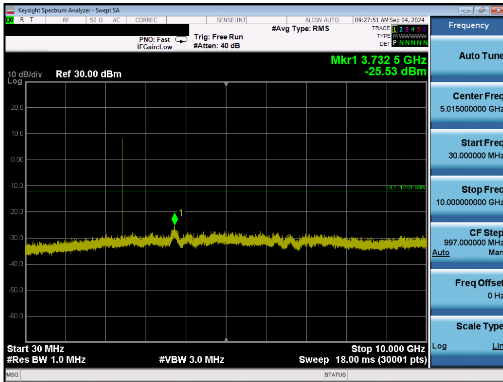
Plot 7-45. Conducted Spurious Antenna 4 (802.15.4, iPA – Ch. 18)
