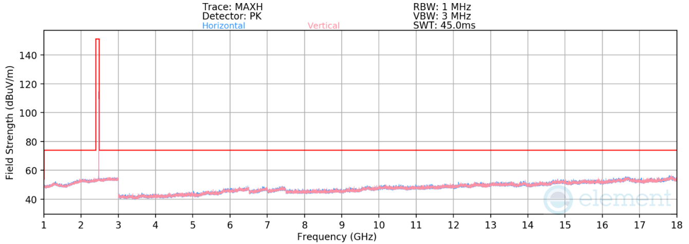
Plot 7-55. Radiated Spurious Emissions 1-18GHz Antenna 1a (802.15.4 ePA – Ch. 25)
