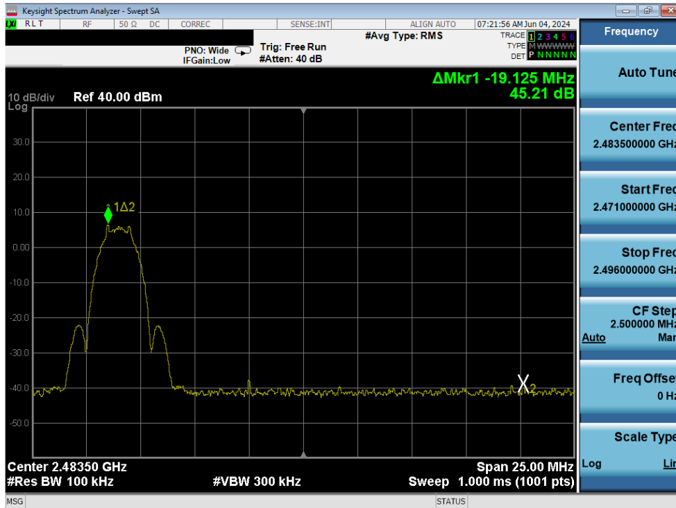
Plot 7-30. Band Edge Antenna 4 (802.15.4, iPA – Ch. 25)
