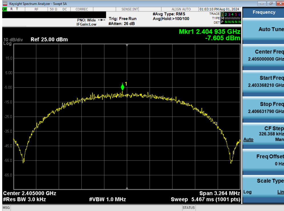
Plot 7-22. Power Spectral Density Antenna 4 (802.15.4, iPA – Ch. 11)
