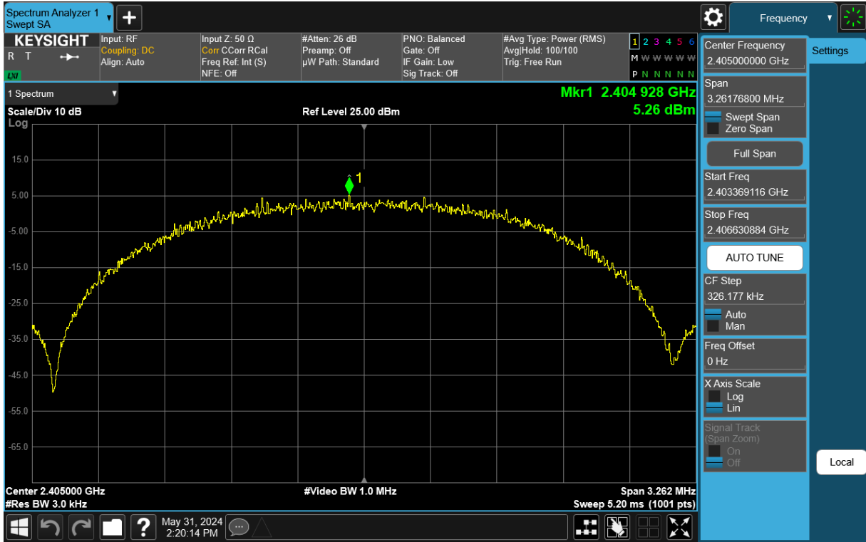
Plot 7-16. Power Spectral Density Antenna 1a (802.15.4, ePA – Ch. 11)
