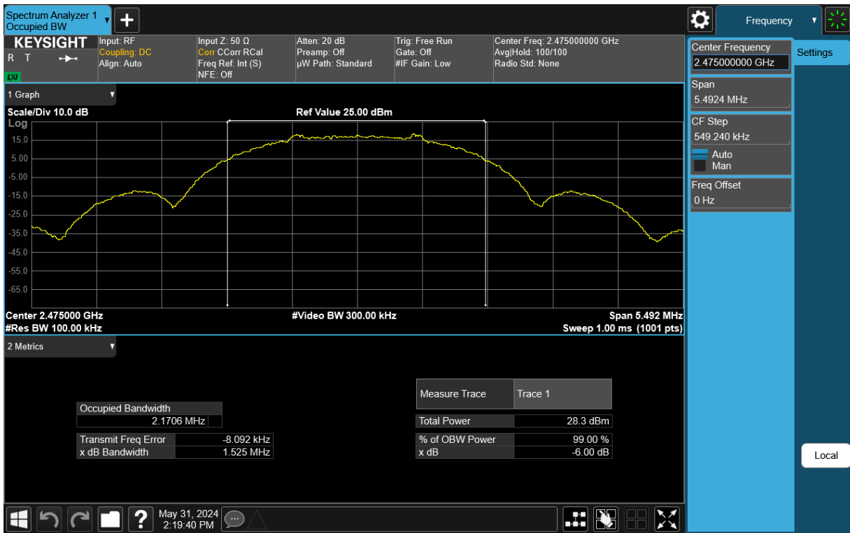
Plot 7-6. 6dB BW & 99% OBW Antenna 1a (802.15.4, Ch. 25)
