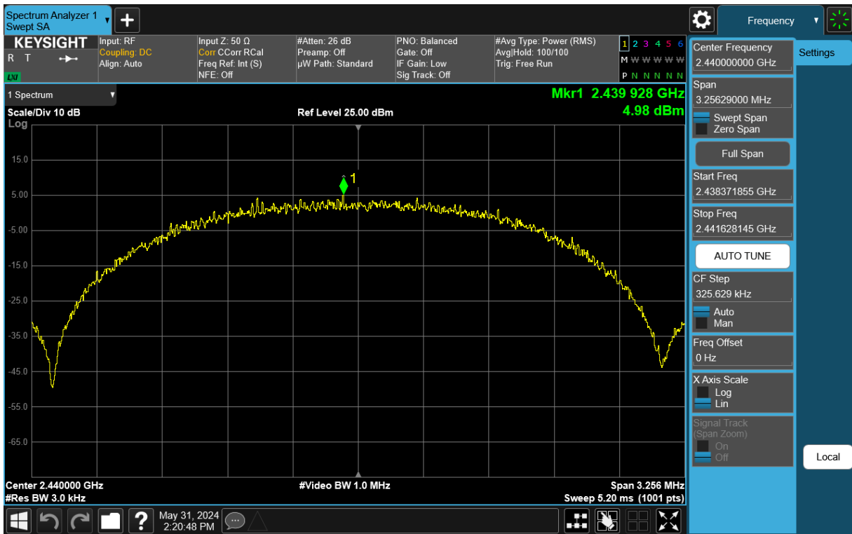
Plot 7-17. Power Spectral Density Antenna 1a (802.15.4, ePA – Ch. 18)
