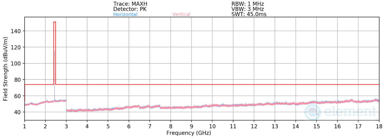
Plot 7-54. Radiated Spurious Emissions 1-18GHz Antenna 1a (802.15.4 ePA – Ch. 18)
