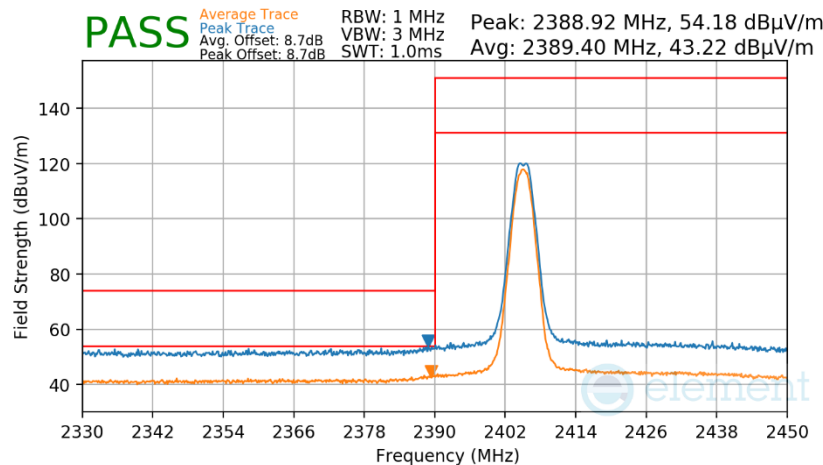
Plot 7-59. Radiated Restricted Lower Band Edge Measurement Antenna 3a
