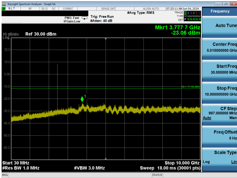
Plot 7-47. Conducted Spurious Antenna 4 (802.15.4, iPA – Ch. 25)
