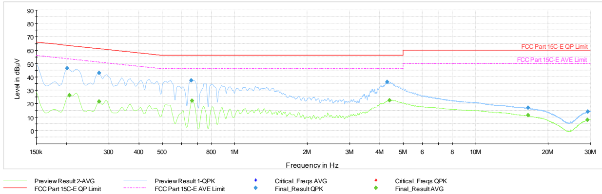
Plot 7-67. AC Line Conducted Emission with 802.15.4 Antenna 3a (N, 250 kbps, ePA - Ch.11, with AC/DC Adapter via USB-C cable with wire charger)
