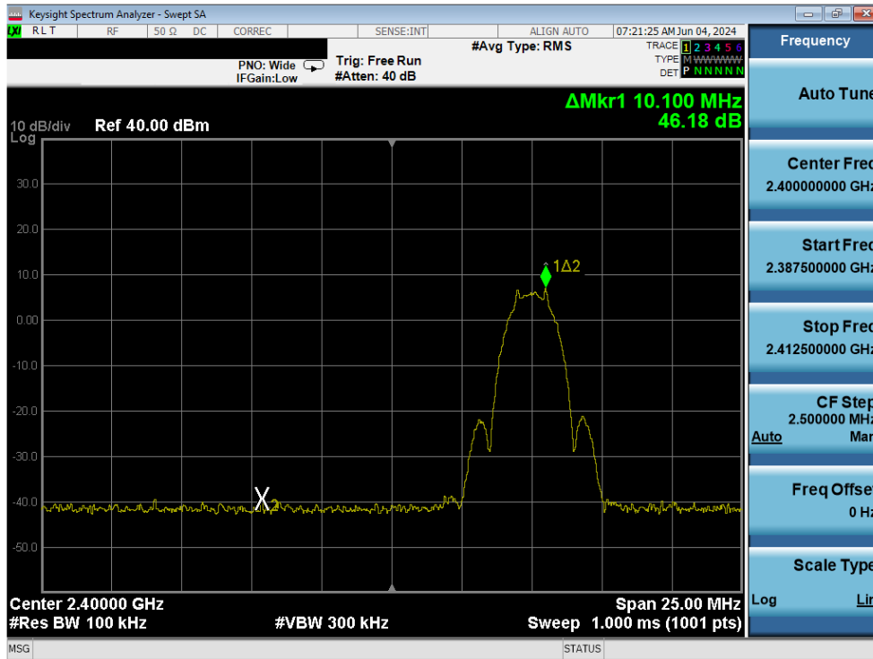
Plot 7-29. Band Edge Antenna 4 (802.15.4, iPA – Ch. 11)
