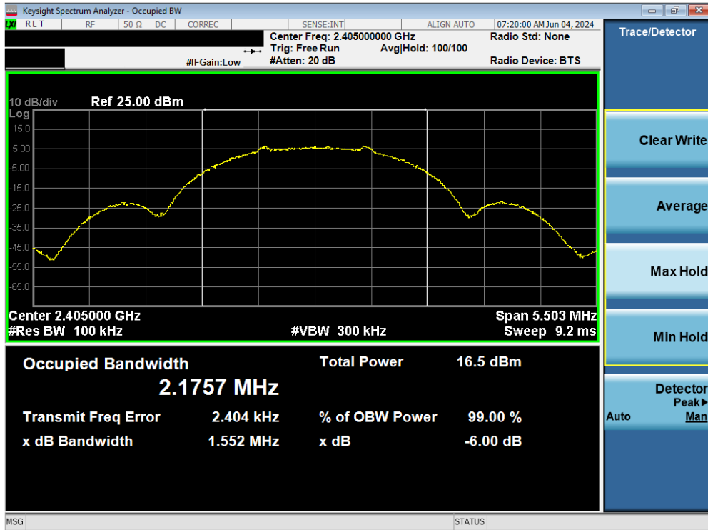
Plot 7-7. 6dB BW & 99% OBW Antenna 4 (802.15.4, Ch. 11)
