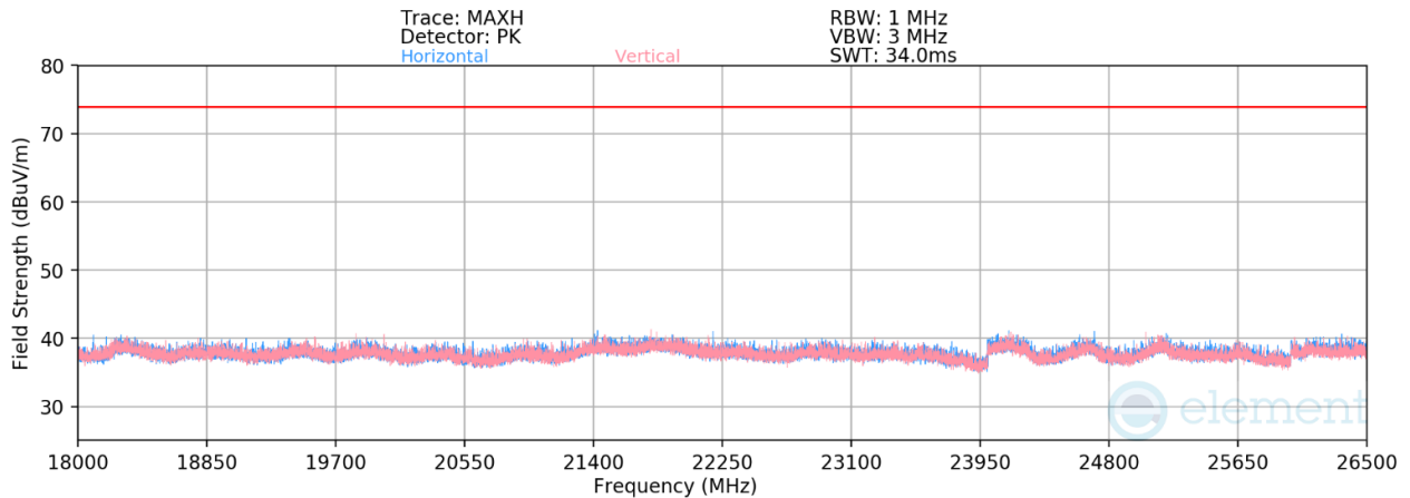
Plot 7-50. Radiated Spurious Emissions Above 18GHz Antenna 3a (802.15.4 ePA – Ch. 11)
