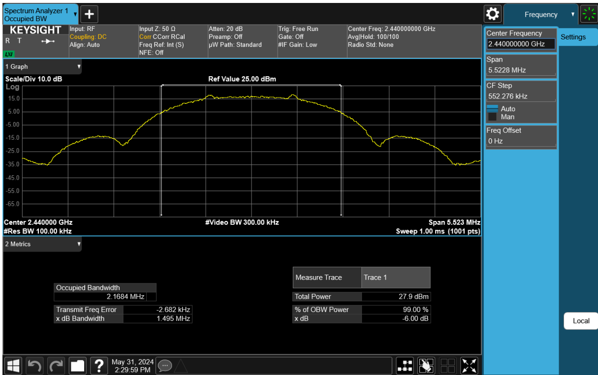
Plot 7-2. 6dB BW & 99% OBW Antenna 3a (802.15.4, Ch. 18)
