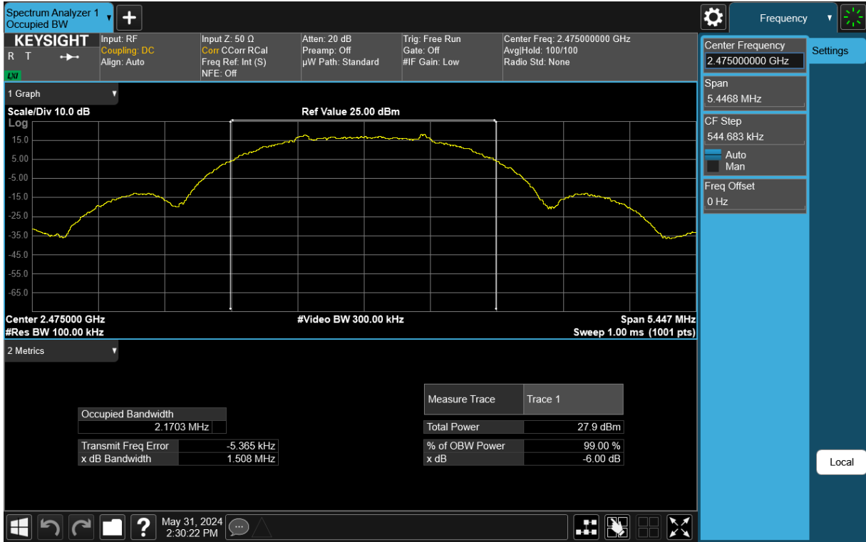
Plot 7-3. 6dB BW & 99% OBW Antenna 3a (802.15.4, Ch. 25)
