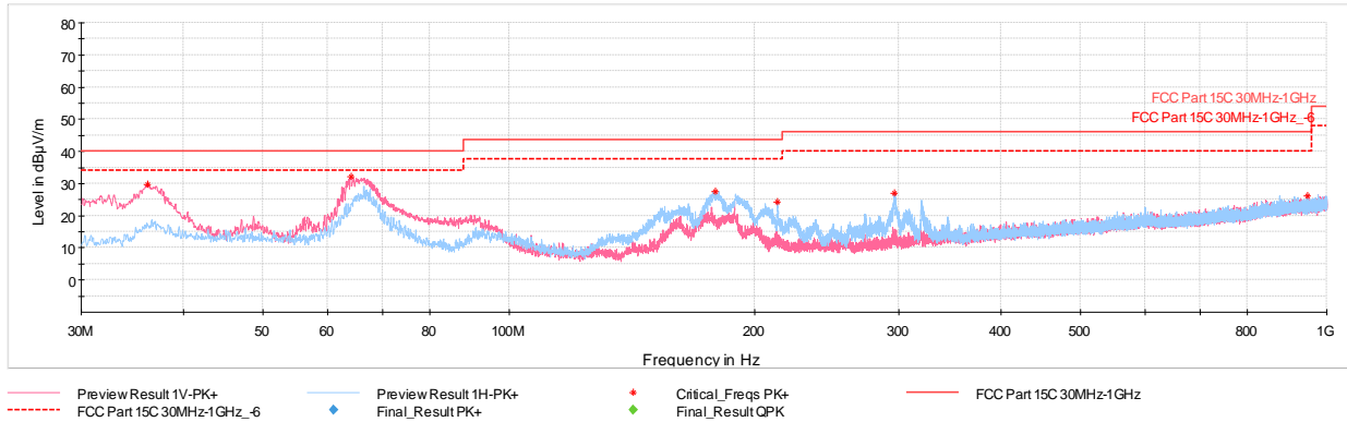
Plot 7-65. Radiated Spurious Emissions 30MHz-1GHz Antenna 3a (250kbps, ePA - Ch.11, with AC/DC Adapter via USB-C cable with wire charger)
