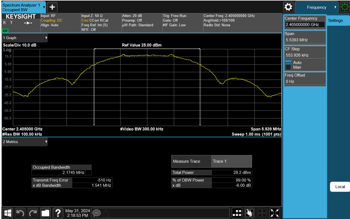
Plot 7-4. 6dB BW & 99% OBW Antenna 1a (802.15.4, Ch. 11)
