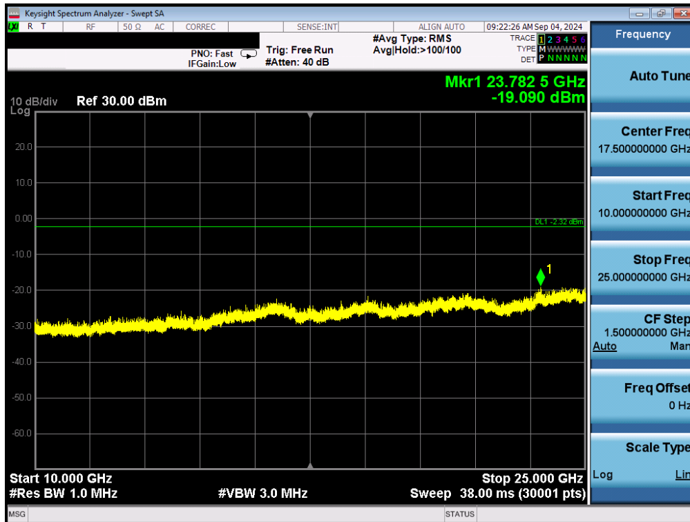
Plot 7-34. Conducted Spurious Antenna 3a (802.15.4, ePA – Ch. 18)
