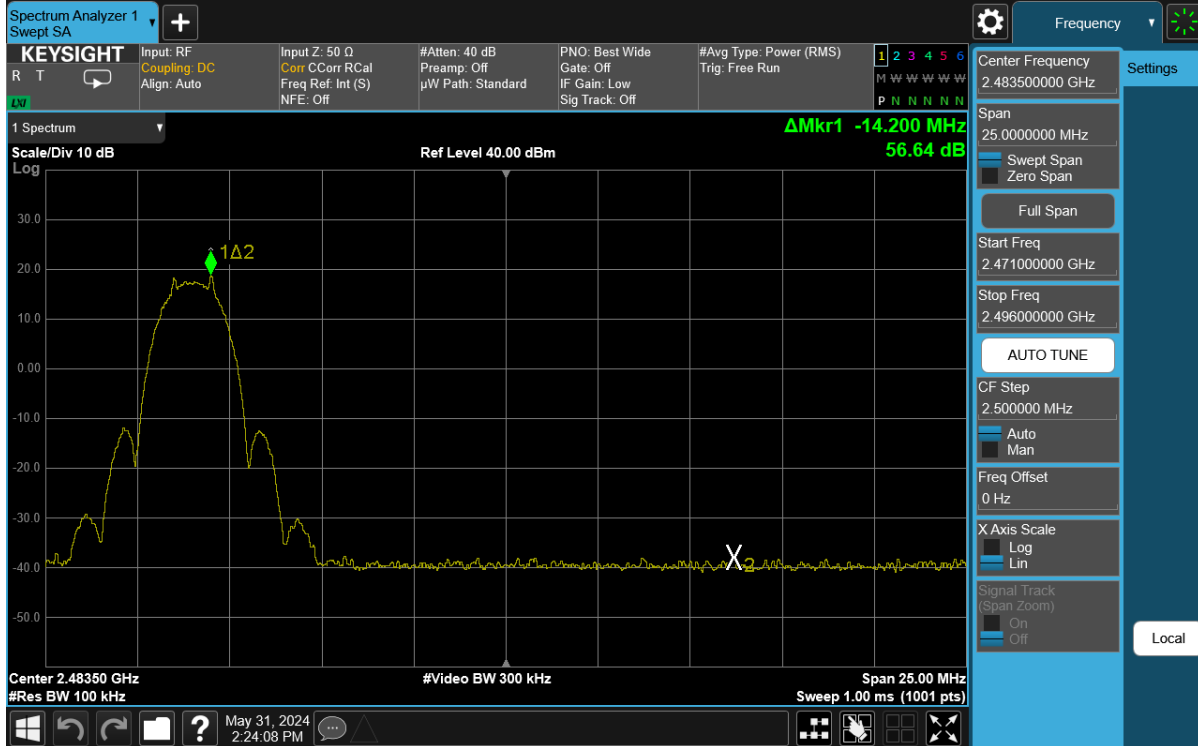
Plot 7-28. Band Edge Antenna 1a (802.15.4, ePA – Ch. 25)
