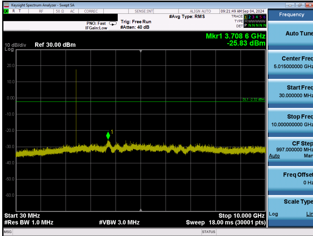
Plot 7-33. Conducted Spurious Antenna 3a (802.15.4, ePA – Ch. 18)
