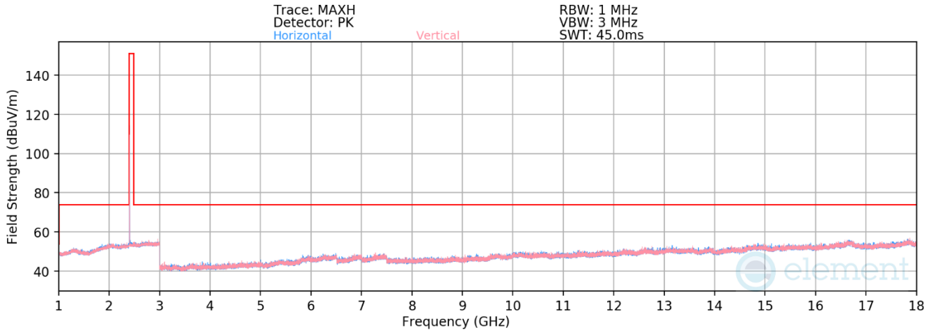
Plot 7-53. Radiated Spurious Emissions 1-18GHz Antenna 1a (802.15.4 ePA – Ch. 11)
