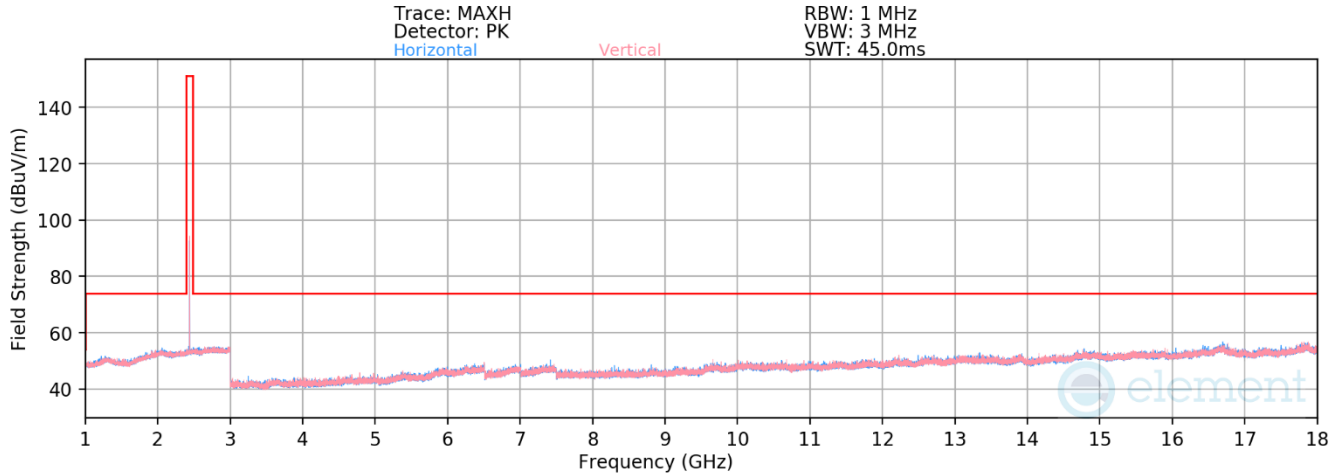
Plot 7-57. Radiated Spurious Emissions 1-18GHz Antenna 4 (802.15.4 iPA – Ch. 18)
