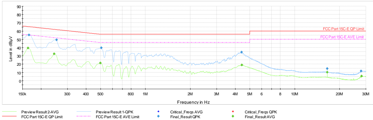
Plot 7-66. AC Line Conducted Emission with 802.15.4 Antenna 3a (L1, 250 kbps, ePA - Ch.11, with AC/DC Adapter via USB-C cable with wire charger)
