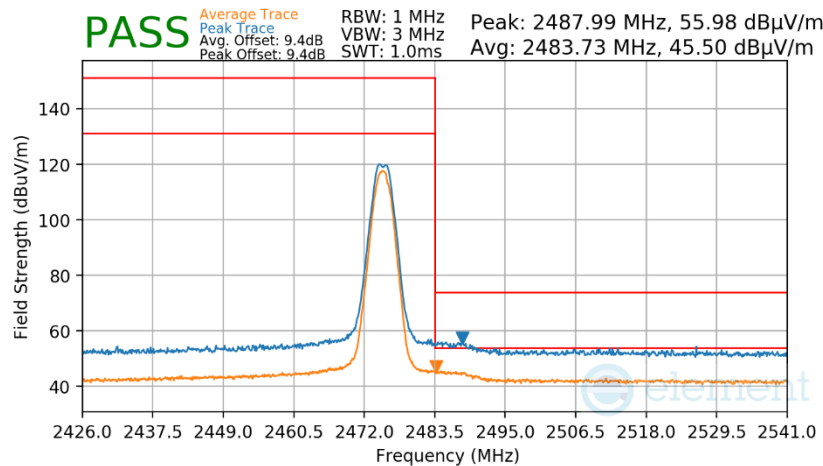
Plot 7-60. Radiated Restricted Upper Band Edge Measurement Antenna 3a
