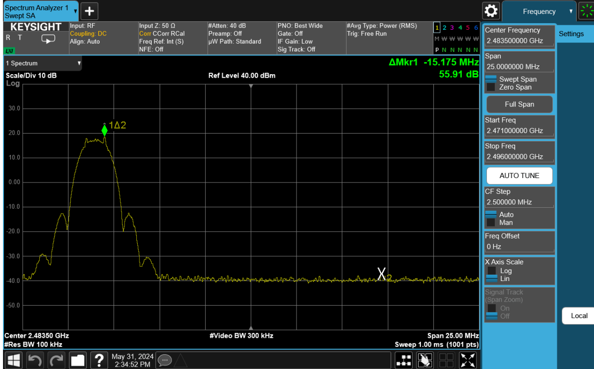
Plot 7-26. Band Edge Antenna 3a (802.15.4, ePA – Ch. 25)
