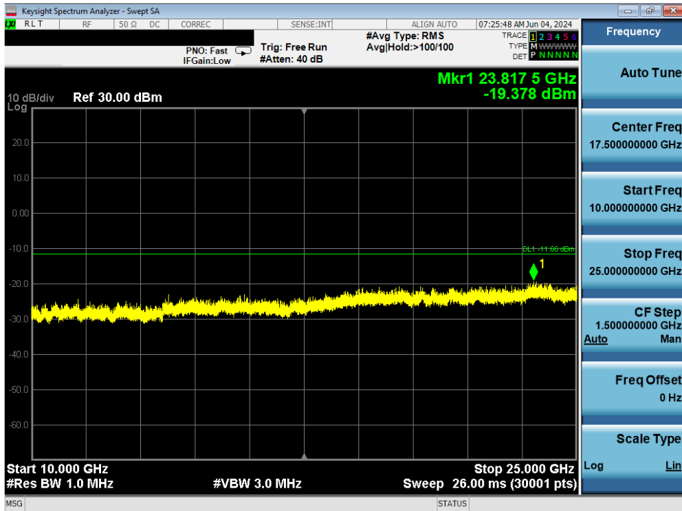
Plot 7-48. Conducted Spurious Antenna 4 (802.15.4, iPA – Ch. 25)
