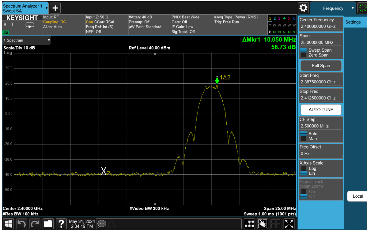
Plot 7-25. Band Edge Antenna 3a (802.15.4, ePA – Ch. 11)
