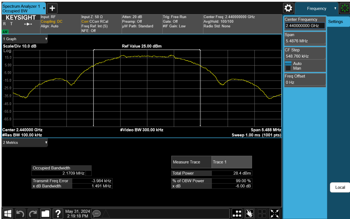
Plot 7-5. 6dB BW & 99% OBW Antenna 1a (802.15.4, Ch. 18)
