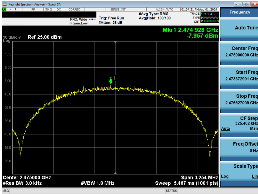
Plot 7-24. Power Spectral Density Antenna 4 (802.15.4, iPA – Ch. 25)
