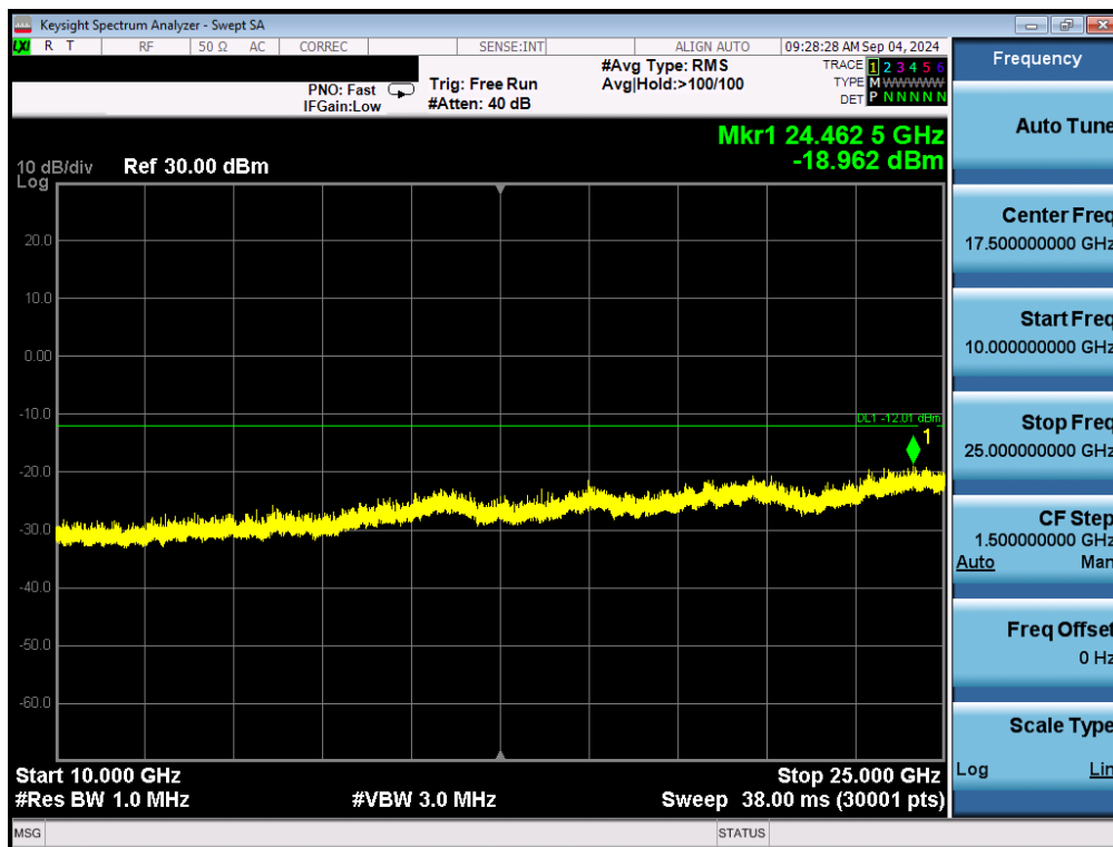
Plot 7-46. Conducted Spurious Antenna 4 (802.15.4, iPA – Ch. 18)
