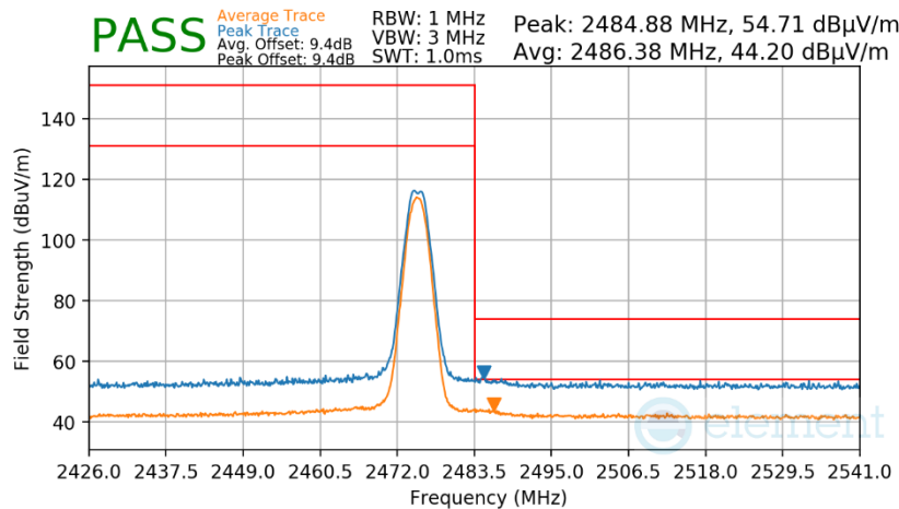
Plot 7-62. Radiated Restricted Upper Band Edge Measurement Antenna 1a
