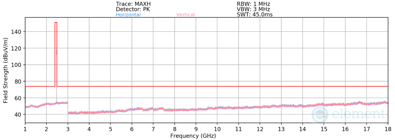
Plot 7-52. Radiated Spurious Emissions 1-18GHz Antenna 3a (802.15.4 ePA – Ch. 25)
