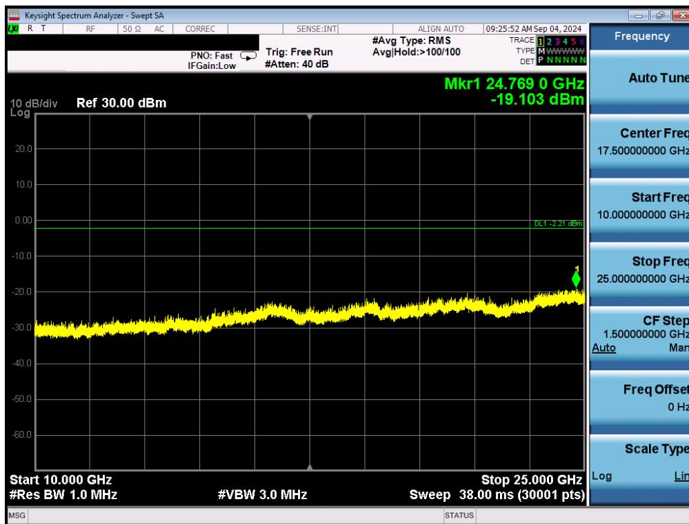
Plot 7-40. Conducted Spurious Antenna 1a (802.15.4, ePA – Ch. 18)
