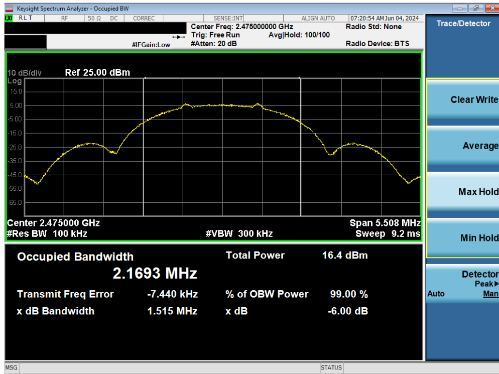
Plot 7-9. 6dB BW & 99% OBW Antenna 4 (802.15.4, Ch. 25)
