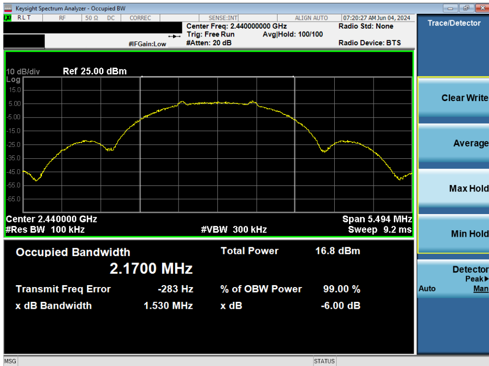
Plot 7-8. 6dB BW & 99% OBW Antenna 4 (802.15.4, Ch. 18)
