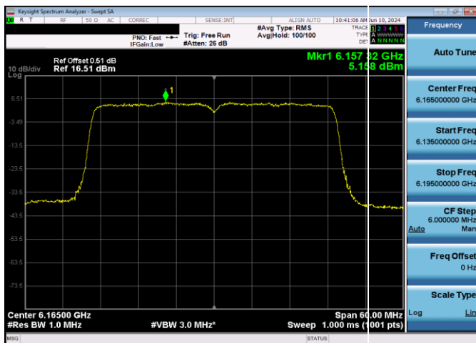
Plot 7-195. Power Spectral Density Plot CDD Antenna WF5T SP (40MHz 802.11ax (UNII Band 5) – Ch. 43, MCS11)
