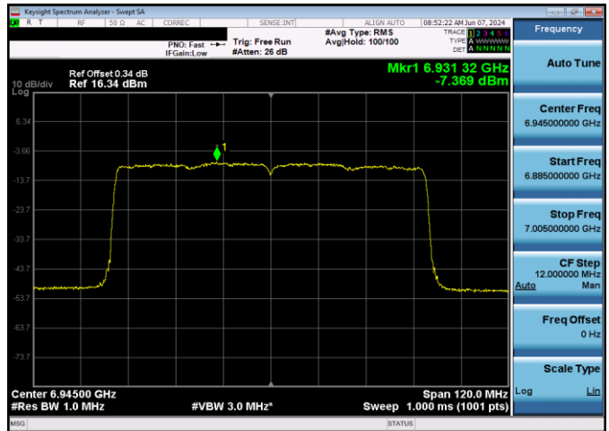
Plot 7-189. Power Spectral Density Plot SDM Antenna WF5T LPI (80MHz 802.11ax (UNII Band 8) – Ch. 199, MCS11)
