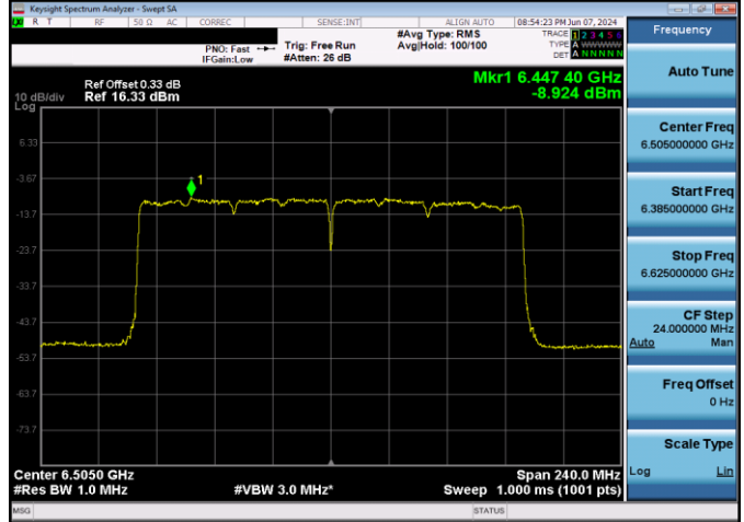
Plot 7-176. Power Spectral Density Plot SDM Antenna WF2 LPI (160MHz 802.11ax (UNII Band 6) – Ch. 111, MCS11)
