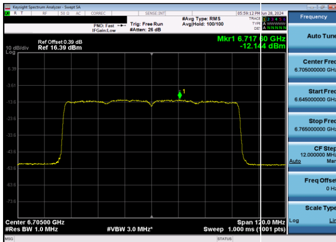
Plot 7-222. Power Spectral Density Plot CDD Antenna WF2 VLP (80MHz 802.11ax (UNII Band 7) – Ch. 151, MCS11)
