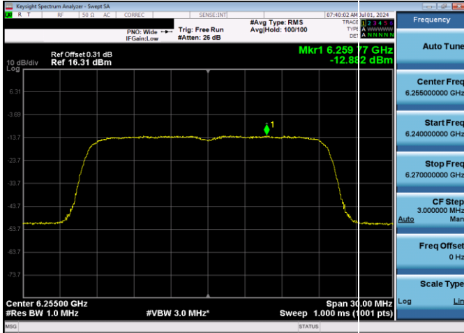
Plot 7-209. Power Spectral Density Plot SDM Antenna WF5T VLP (20MHz 802.11ax (UNII Band 5) – Ch. 61, MCS11)
