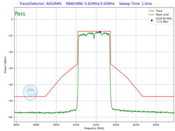
Plot 7-228. LPI In-Band Emission Plot Antenna WF5T LPI (80MHz 802.11ax (UNII Band 5) – Ch. 39, MCS11)
