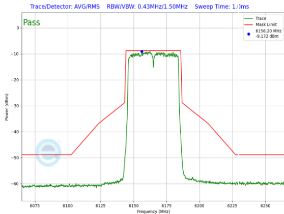
Plot 7-227. LPI In-Band Emission Plot Antenna WF5T LPI (40MHz 802.11ax (UNII Band 5) – Ch. 43, MCS11)
