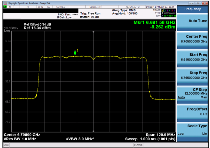
Plot 7-182. Power Spectral Density Plot SDM Antenna WF2 LPI (80MHz 802.11ax (UNII Band 7) – Ch. 151, MCS11)
