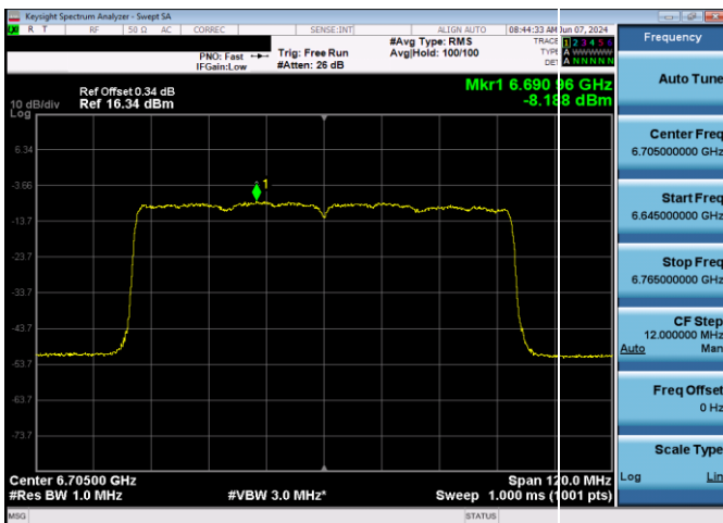
Plot 7-181. Power Spectral Density Plot SDM Antenna WF5T LPI (80MHz 802.11ax (UNII Band 7) – Ch. 151, MCS11)
