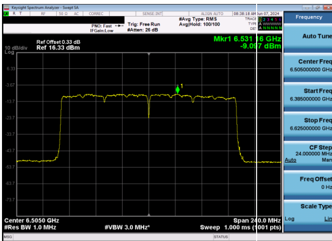
Plot 7-175. Power Spectral Density Plot SDM Antenna WF5T LPI (160MHz 802.11ax (UNII Band 6) – Ch. 111, MCS11)
