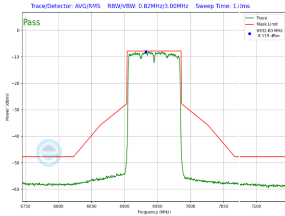
Plot 7-243. LPI In-Band Emission Plot Antenna WF5T LPI (80MHz 802.11ax (UNII Band 8) – Ch. 199, MCS11)
