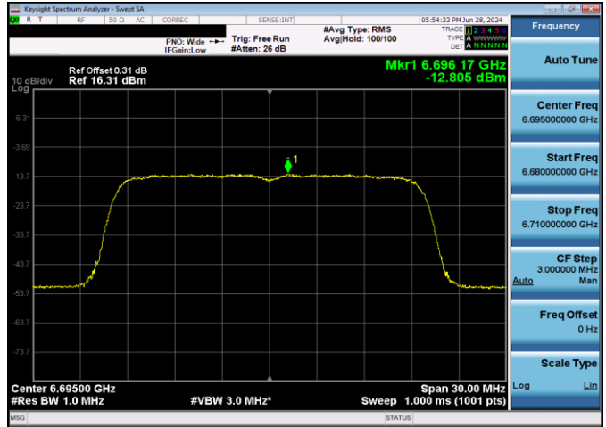
Plot 7-218. Power Spectral Density Plot SDM Antenna WF2 VLP (20MHz 802.11ax (UNII Band 7) – Ch. 149, MCS11)
