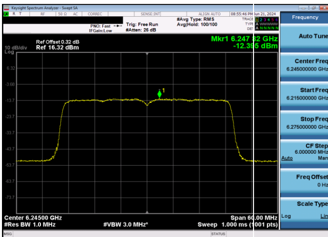
Plot 7-211. Power Spectral Density Plot CDD Antenna WF5T VLP (40MHz 802.11ax (UNII Band 5) – Ch. 59, MCS11)
