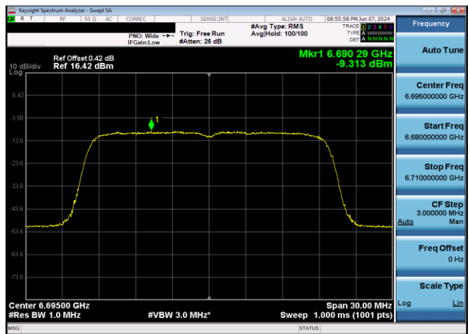
Plot 7-178. Power Spectral Density Plot SDM Antenna WF2 LPI (20MHz 802.11ax (UNII Band 7) – Ch. 149, MCS11)
