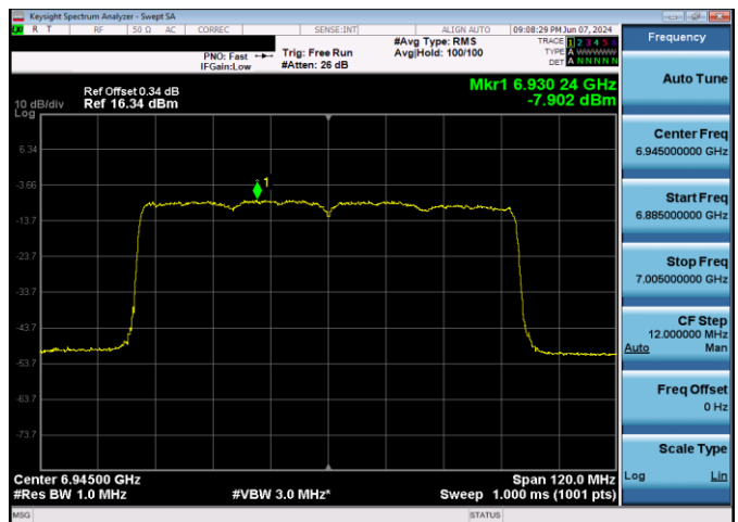
Plot 7-190. Power Spectral Density Plot SDM Antenna WF2 LPI (80MHz 802.11ax (UNII Band 8) – Ch. 199, MCS11)
