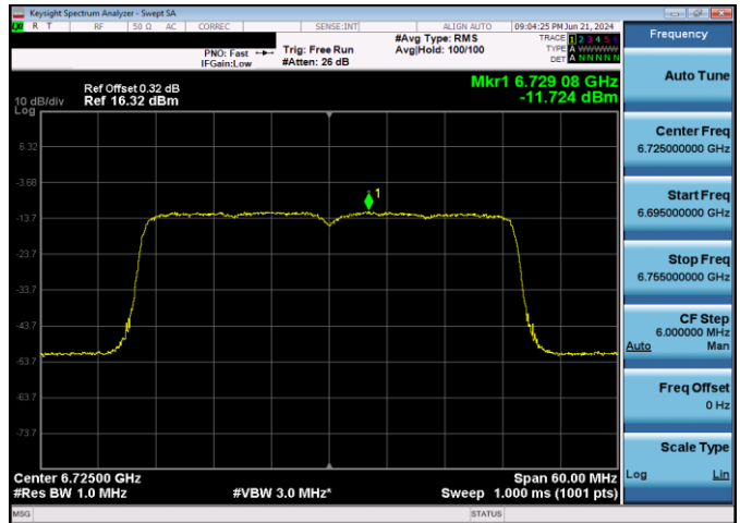
Plot 7-219. Power Spectral Density Plot CDD Antenna WF5T VLP (40MHz 802.11ax (UNII Band 7) – Ch. 155, MCS11)
