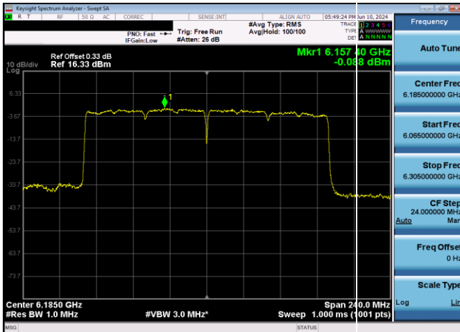
Plot 7-200. Power Spectral Density Plot CDD Antenna WF2 SP (160MHz 802.11ax (UNII Band 5) - Ch. 47, MCS11)
