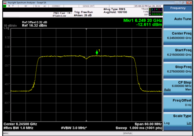
Plot 7-212. Power Spectral Density Plot CDD Antenna WF2 VLP (40MHz 802.11ax (UNII Band 5) – Ch. 59, MCS11)
