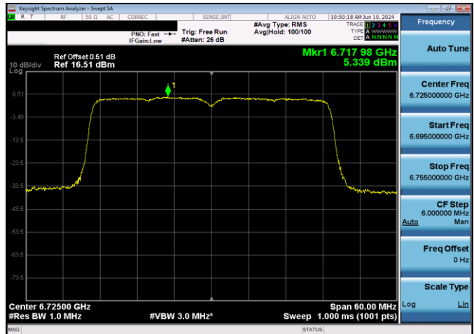
Plot 7-203. Power Spectral Density Plot CDD Antenna WF5T SP (40MHz 802.11ax (UNII Band 7) - Ch. 155, MCS11)
