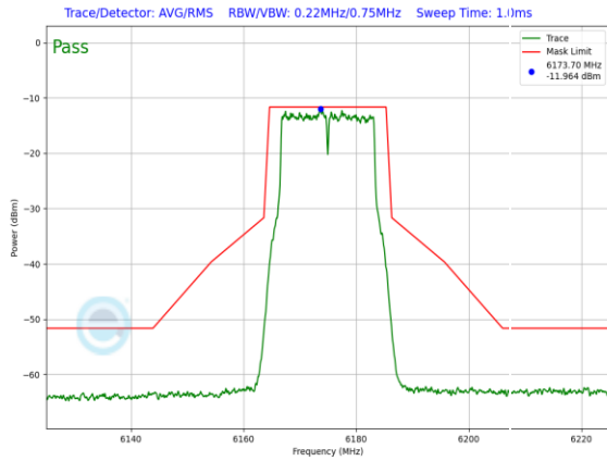
Plot 7-225. LPI In-Band Emission Plot Antenna WF5T LPI (20MHz 802.11a (UNII Band 5) – Ch. 45, 54Mbps)
