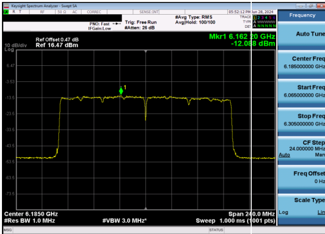
Plot 7-216. Power Spectral Density Plot CDD Antenna WF2 VLP (160MHz 802.11ax (UNII Band 5) – Ch. 47, MCS11)
