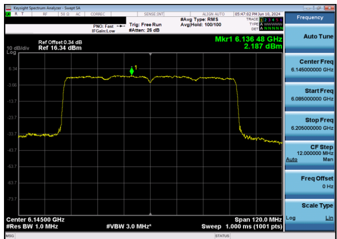
Plot 7-198. Power Spectral Density Plot CDD Antenna WF2 SP (80MHz 802.11ax (UNII Band 5) – Ch. 39, MCS11)
