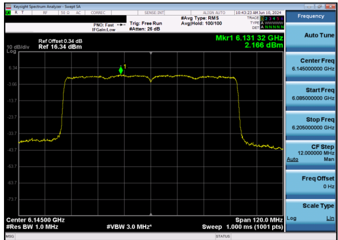
Plot 7-197. Power Spectral Density Plot CDD Antenna WF5T SP (80MHz 802.11ax (UNII Band 5) – Ch. 39, MCS11)
