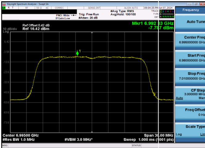
Plot 7-186. Power Spectral Density Plot SDM Antenna WF2 LPI (20MHz 802.11ax (UNII Band 8) – Ch. 209, MCS11)
