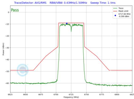
Plot 7-237. LPI In-Band Emission Plot Antenna WF5T LPI (40MHz 802.11ax (UNII Band 7) – Ch. 155, MCS11)
