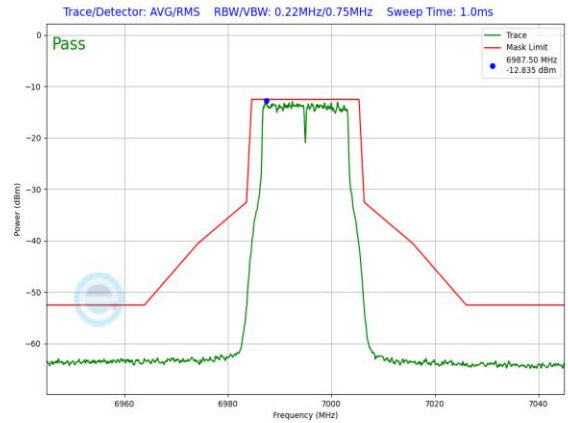
Plot 7-240. LPI In-Band Emission Plot Antenna WF5T LPI (20MHz 802.11a (UNII Band 8) – Ch. 209, 54Mbps)
