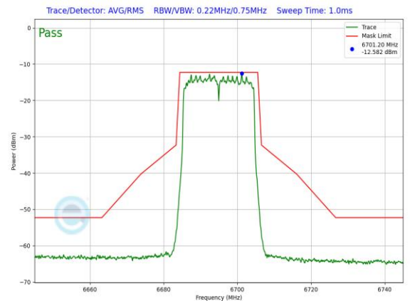
Plot 7-236. LPI In-Band Emission Plot Antenna WF5T LPI (20MHz 802.11ax (UNII Band 7) – Ch. 149, MCS11)
