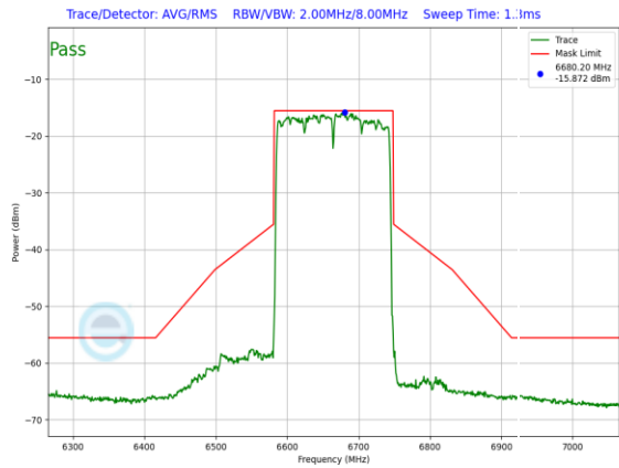
Plot 7-239. LPI In-Band Emission Plot Antenna WF5T LPI (160MHz 802.11ax (UNII Band 7) – Ch. 143, MCS11)
