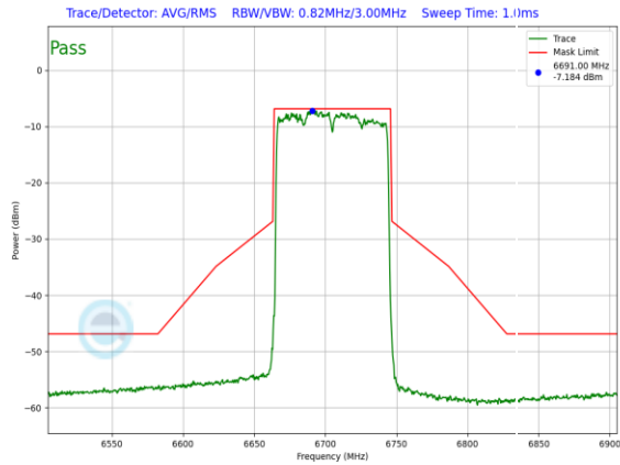
Plot 7-238. LPI In-Band Emission Plot Antenna WF5T LPI (80MHz 802.11ax (UNII Band 7) – Ch. 151, MCS11)
