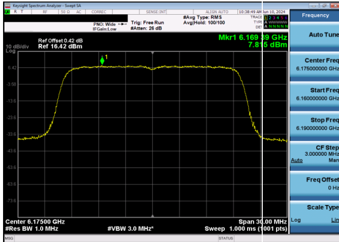
Plot 7-193. Power Spectral Density Plot SDM Antenna WF5T SP (20MHz 802.11ax (UNII Band 5) – Ch. 45, MCS11)
