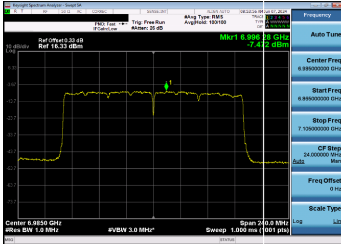
Plot 7-191. Power Spectral Density Plot SDM Antenna WF5T LPI (160MHz 802.11ax (UNII Band 8) – Ch. 207, MCS11)
