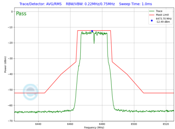
Plot 7-230. LPI In-Band Emission Plot Antenna WF5T LPI (20MHz 802.11a (UNII Band 6) – Ch. 105, 54Mbps)
