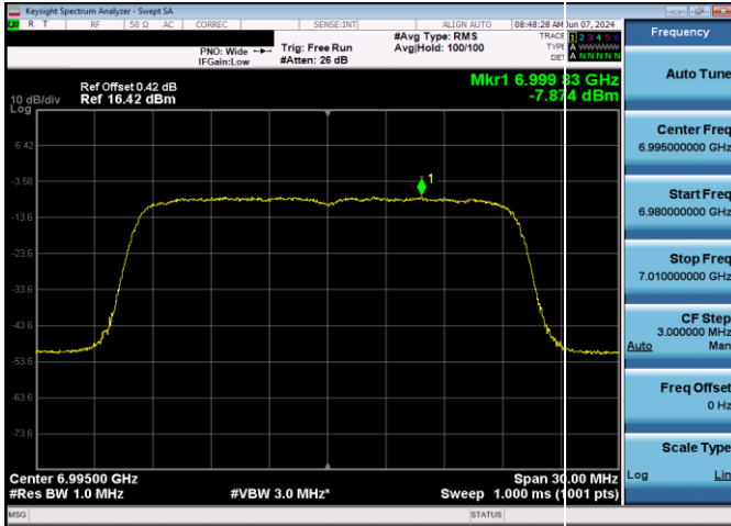
Plot 7-185. Power Spectral Density Plot SDM Antenna WF5T LPI (20MHz 802.11ax (UNII Band 8) – Ch. 209, MCS11)
