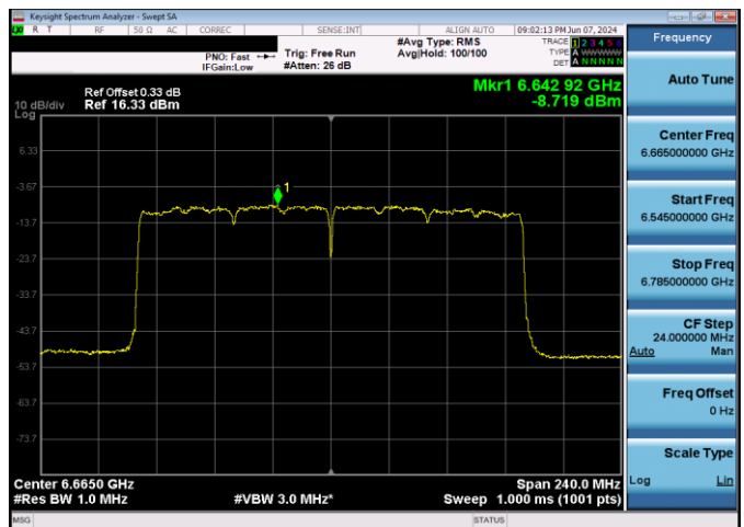
Plot 7-184. Power Spectral Density Plot SDM Antenna WF2 LPI (160MHz 802.11ax (UNII Band 7) – Ch. 143, MCS11)
