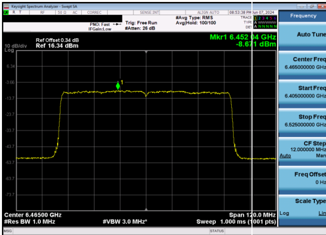
Plot 7-174. Power Spectral Density Plot SDM Antenna WF2 LPI (80MHz 802.11ax (UNII Band 6) – Ch. 103, MCS11)
