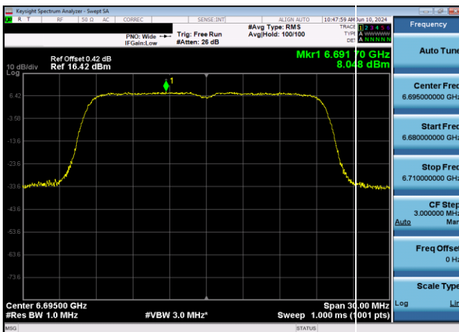
Plot 7-201. Power Spectral Density Plot SDM Antenna WF5T SP (20MHz 802.11ax (UNII Band 7) - Ch. 149, MCS11)
