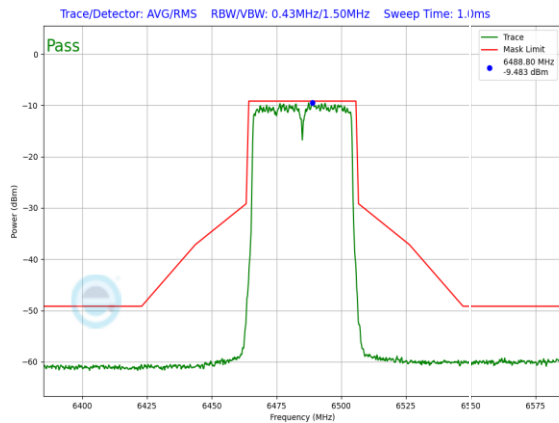
Plot 7-232. LPI In-Band Emission Plot Antenna WF5T LPI (40MHz 802.11ax (UNII Band 6) – Ch. 107, MCS11)
