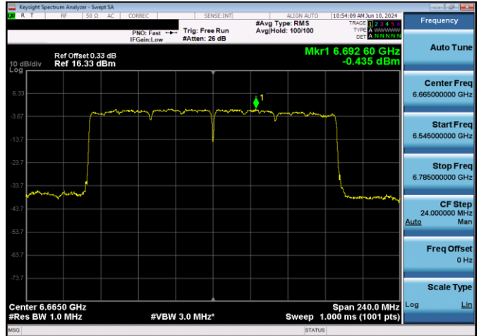
Plot 7-207. Power Spectral Density Plot CDD Antenna WF5T SP (160MHz 802.11ax (UNII Band 7) – Ch. 143, MCS11)
