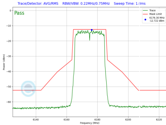
Plot 7-226. LPI In-Band Emission Plot Antenna WF5T LPI (20MHz 802.11ax (UNII Band 5) – Ch. 45, MCS11)
