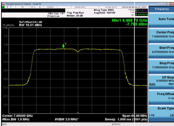
Plot 7-187. Power Spectral Density Plot SDM Antenna WF5T LPI (40MHz 802.11ax (UNII Band 8) – Ch. 211, MCS11)
