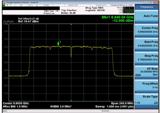
Plot 7-223. Power Spectral Density Plot CDD Antenna WF5T VLP (160MHz 802.11ax (UNII Band 7) – Ch. 143, MCS11)
