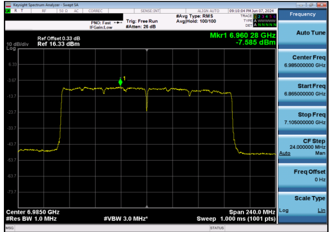
Plot 7-192. Power Spectral Density Plot SDM Antenna WF2 LPI (160MHz 802.11ax (UNII Band 8) – Ch. 207, MCS11)
