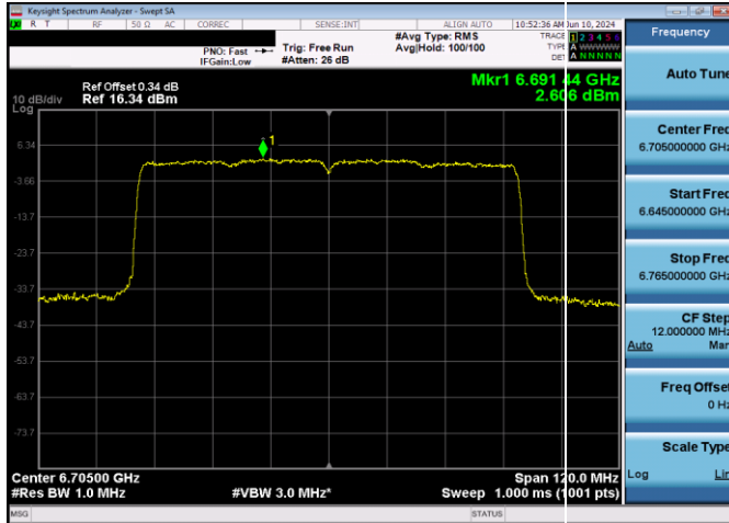
Plot 7-205. Power Spectral Density Plot CDD Antenna WF5T SP (80MHz 802.11ax (UNII Band 7) – Ch. 151, MCS11)
