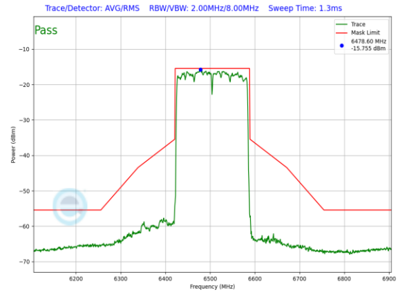
Plot 7-234. LPI In-Band Emission Plot Antenna WF5T LPI (160MHz 802.11ax (UNII Band 6) – Ch. 111, MCS11)
