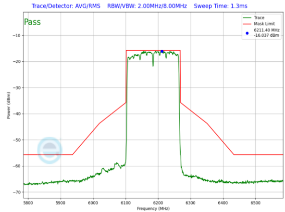
Plot 7-229. LPI In-Band Emission Plot Antenna WF5T LPI (160MHz 802.11ax (UNII Band 5) – Ch. 47, MCS11)
