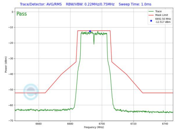
Plot 7-235. LPI In-Band Emission Plot Antenna WF5T LPI (20MHz 802.11a (UNII Band 7) – Ch. 149, 54Mbps)
