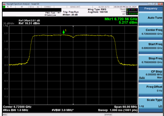
Plot 7-204. Power Spectral Density Plot CDD Antenna WF2 SP (40MHz 802.11ax (UNII Band 7) - Ch. 155, MCS11)
