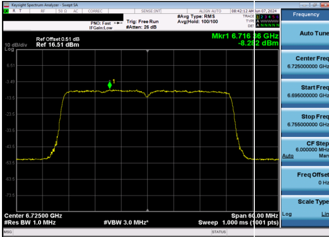
Plot 7-179. Power Spectral Density Plot SDM Antenna WF5T LPI (40MHz 802.11ax (UNII Band 7) – Ch. 155, MCS11)
