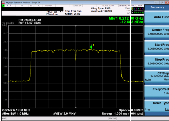
Plot 7-215. Power Spectral Density Plot CDD Antenna WF5T VLP (160MHz 802.11ax (UNII Band 5) – Ch. 47, MCS11)
