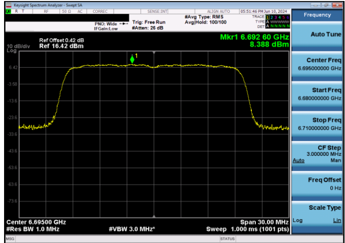
Plot 7-202. Power Spectral Density Plot SDM Antenna WF2 SP (20MHz 802.11ax (UNII Band 7) - Ch. 149, MCS11)
