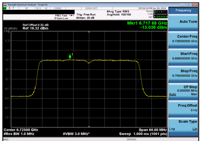
Plot 7-220. Power Spectral Density Plot CDD Antenna WF2 VLP (40MHz 802.11ax (UNII Band 7) – Ch. 155, MCS11)
