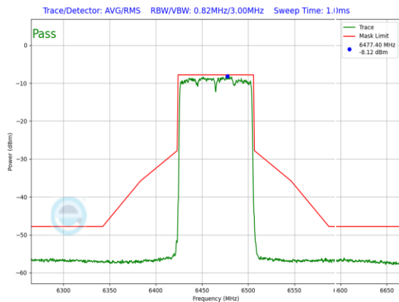
Plot 7-233. LPI In-Band Emission Plot Antenna WF5T LPI (80MHz 802.11ax (UNII Band 6) – Ch. 103, MCS11)
