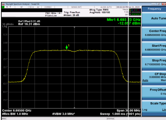
Plot 7-217. Power Spectral Density Plot SDM Antenna WF5T VLP (20MHz 802.11ax (UNII Band 7) – Ch. 149, MCS11)
