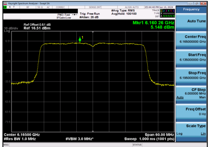
Plot 7-196. Power Spectral Density Plot CDD Antenna WF2 SP (40MHz 802.11ax (UNII Band 5) – Ch. 43, MCS11)
