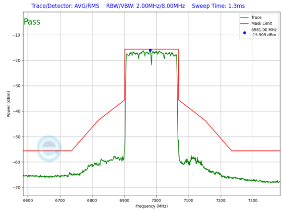
Plot 7-244. LPI In-Band Emission Plot Antenna WF5T LPI (160MHz 802.11ax (UNII Band 8) – Ch. 207, MCS11)
