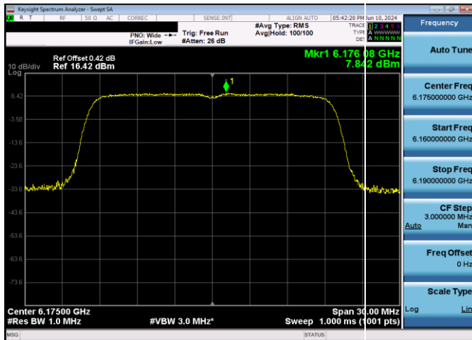
Plot 7-194. Power Spectral Density Plot SDM Antenna WF2 SP (20MHz 802.11ax (UNII Band 5) – Ch. 45, MCS11)
