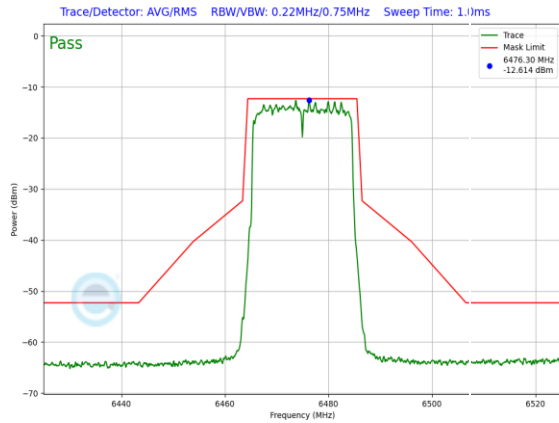
Plot 7-231. LPI In-Band Emission Plot Antenna WF5T LPI (20MHz 802.11ax (UNII Band 6) – Ch. 105, MCS11)
