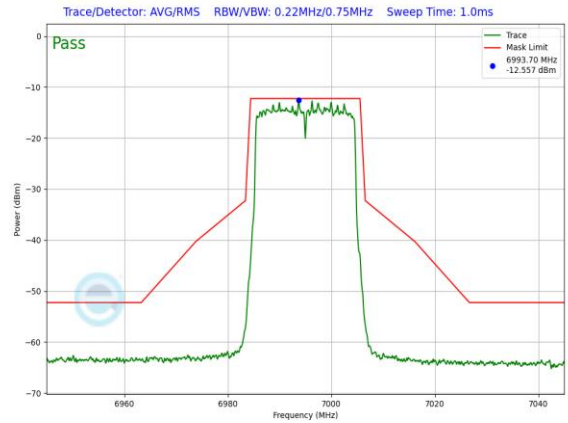
Plot 7-241. LPI In-Band Emission Plot Antenna WF5T LPI (20MHz 802.11ax (UNII Band 8) – Ch. 209, MCS11)
