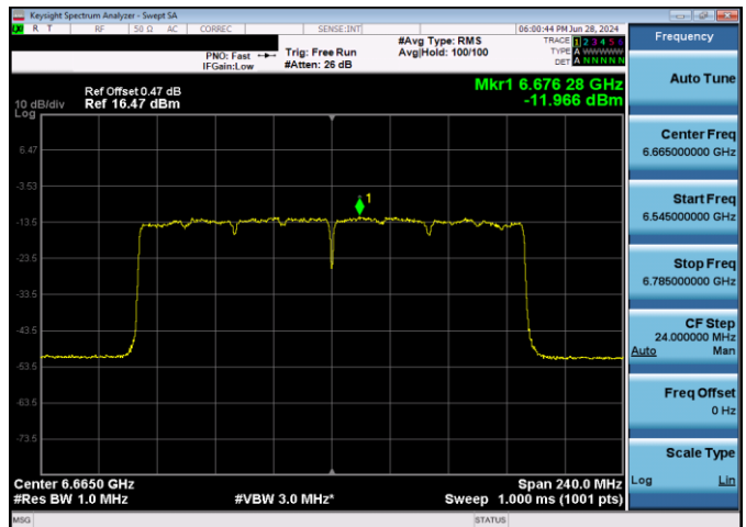
Plot 7-224. Power Spectral Density Plot CDD Antenna WF2 VLP (160MHz 802.11ax (UNII Band 7) – Ch. 143, MCS11)
