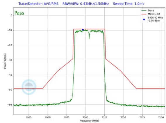
Plot 7-242. LPI In-Band Emission Plot Antenna WF5T LPI (40MHz 802.11ax (UNII Band 8) – Ch. 211, MCS11)
