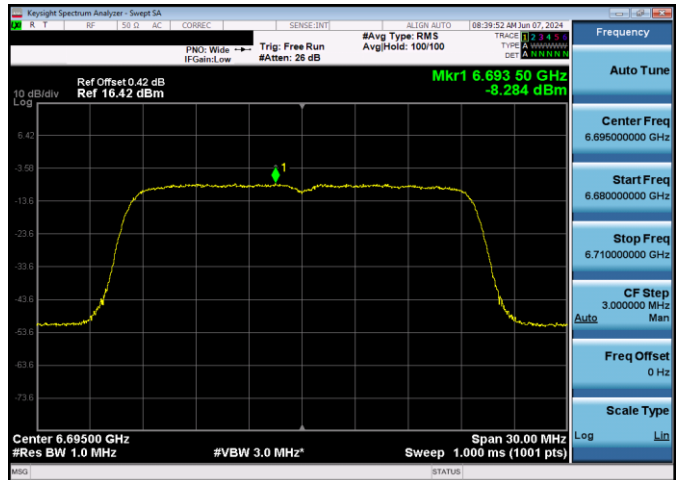
Plot 7-177. Power Spectral Density Plot SDM Antenna WF5T LPI (20MHz 802.11ax (UNII Band 7) – Ch. 149, MCS11)
