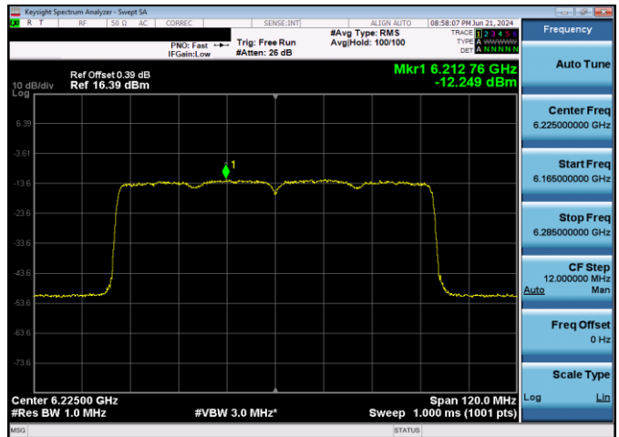
Plot 7-213. Power Spectral Density Plot CDD Antenna WF5T VLP (80MHz 802.11ax (UNII Band 5) – Ch. 55, MCS11)
