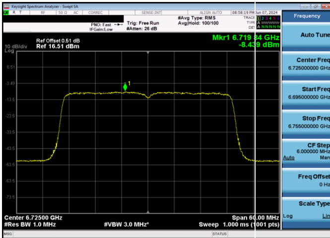
Plot 7-180. Power Spectral Density Plot SDM Antenna WF2 LPI (40MHz 802.11ax (UNII Band 7) – Ch. 155, MCS11)
