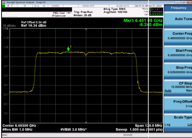
Plot 7-173. Power Spectral Density Plot SDM Antenna WF5T LPI (80MHz 802.11ax (UNII Band 6) – Ch. 103, MCS11)
