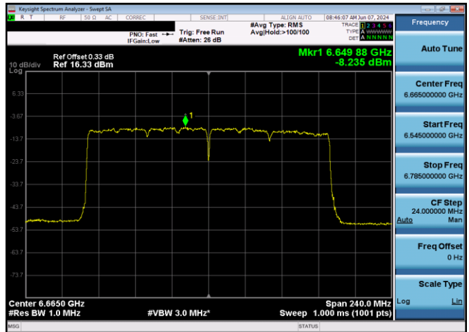
Plot 7-183. Power Spectral Density Plot SDM Antenna WF5T LPI (160MHz 802.11ax (UNII Band 7) – Ch. 143, MCS11)
