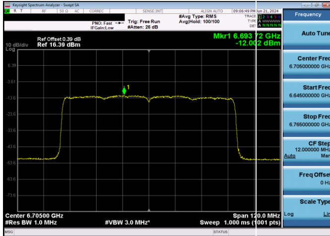
Plot 7-221. Power Spectral Density Plot CDD Antenna WF5T VLP (80MHz 802.11ax (UNII Band 7) – Ch. 151, MCS11)
