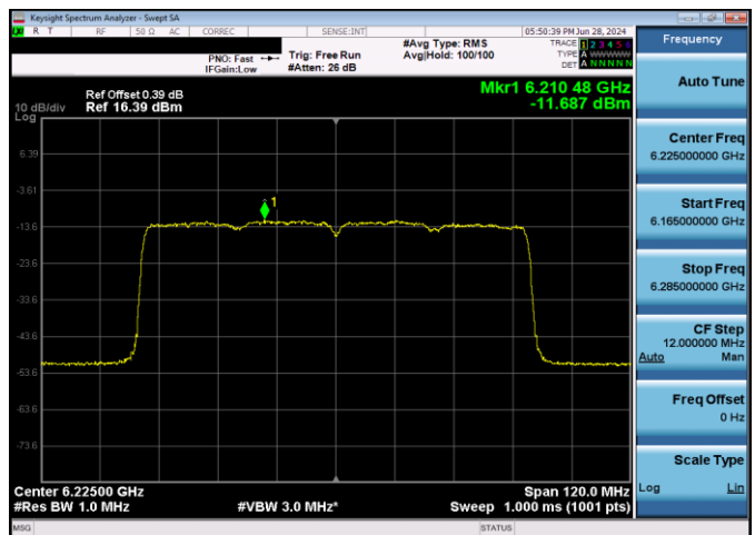
Plot 7-214. Power Spectral Density Plot CDD Antenna WF2 VLP (80MHz 802.11ax (UNII Band 5) – Ch. 55, MCS11)
