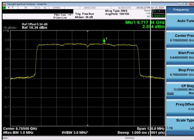
Plot 7-206. Power Spectral Density Plot CDD Antenna WF2 SP (80MHz 802.11ax (UNII Band 7) – Ch. 151, MCS11)
