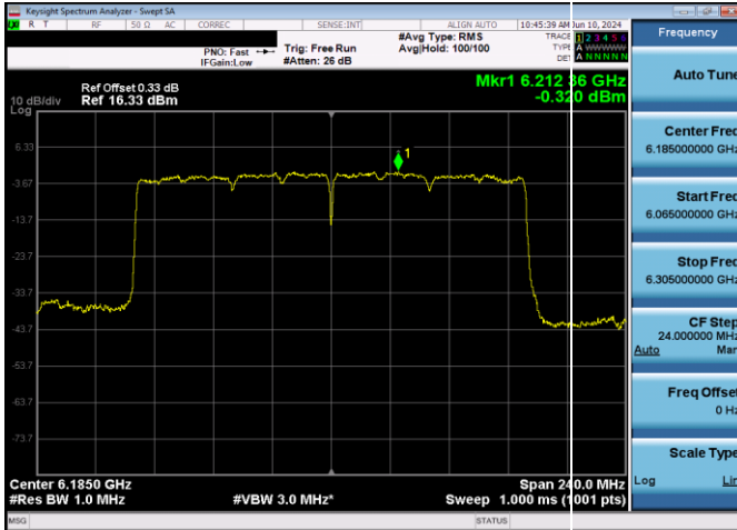
Plot 7-199. Power Spectral Density Plot CDD Antenna WF5T SP (160MHz 802.11ax (UNII Band 5) - Ch. 47, MCS11)
