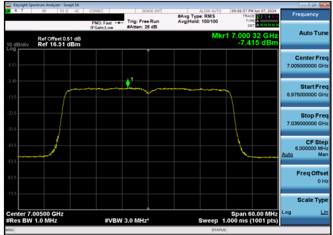
Plot 7-188. Power Spectral Density Plot SDM Antenna WF2 LPI (40MHz 802.11ax (UNII Band 8) – Ch. 211, MCS11)
