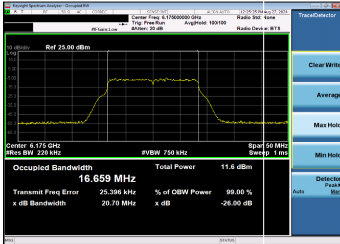
Plot 7-11. 26dB & 99% Bandwidth Plot Antenna WF5T LPI (20MHz 802.11a (UNII Band 5) – Ch. 45, 54Mbps)
