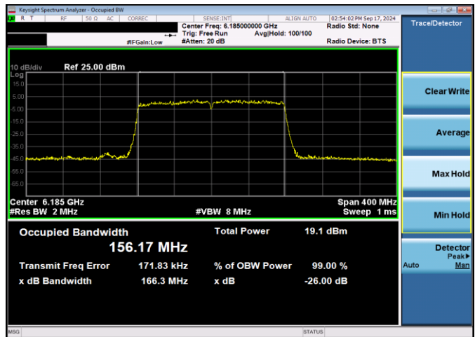
Plot 7-35. 26dB & 99% Bandwidth Plot Antenna WF5T VLP (160MHz 802.11ax (UNII Band 5) – Ch. 47, MCS11)
