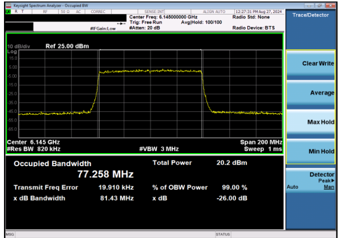
Plot 7-14. 26dB & 99% Bandwidth Plot Antenna WF5T LPI (80MHz 802.11ax (UNII Band 5) – Ch. 39, MCS11)
