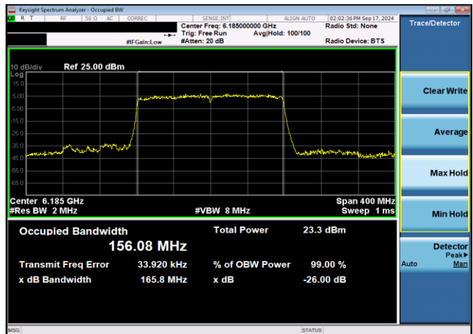
Plot 7-15. 26dB & 99% Bandwidth Plot Antenna WF5T LPI (160MHz 802.11ax (UNII Band 5) – Ch. 47, MCS11)
