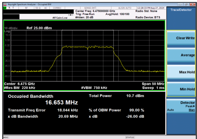
Plot 7-16. 26dB & 99% Bandwidth Plot Antenna WF5T LPI (20MHz 802.11a (UNII Band 6) – Ch. 105, 54Mbps)
