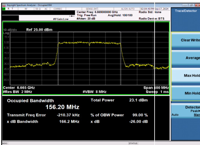
Plot 7-25. 26dB & 99% Bandwidth Plot Antenna WF5T LPI (160MHz 802.11ax (UNII Band 7) – Ch. 143, MCS11)
