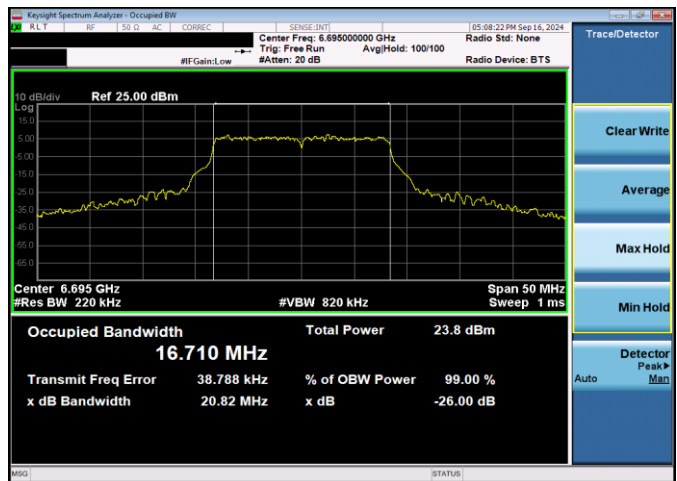
Plot 7-46. 26dB & 99% Bandwidth Plot Antenna WF2 SP (20MHz 802.11a (UNII Band 7) – Ch. 149, 54Mbps)
