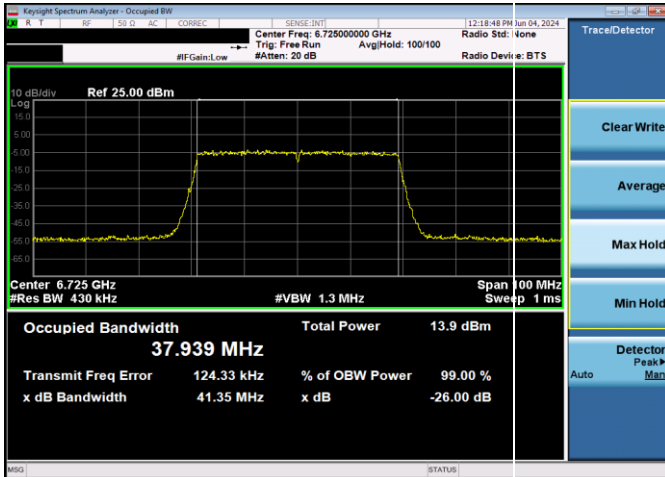
Plot 7-23. 26dB & 99% Bandwidth Plot Antenna WF5T LPI (40MHz 802.11ax (UNII Band 7) – Ch. 155, MCS11)
