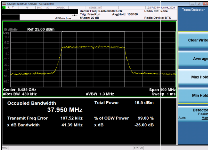
Plot 7-18. 26dB & 99% Bandwidth Plot Antenna WF5T LPI (40MHz 802.11ax (UNII Band 6) – Ch. 107, MCS11)
