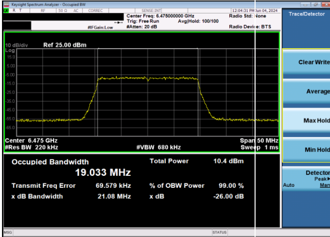
Plot 7-17. 26dB & 99% Bandwidth Plot Antenna WF5T LPI (20MHz 802.11ax (UNII Band 6) – Ch. 105, MCS11)
