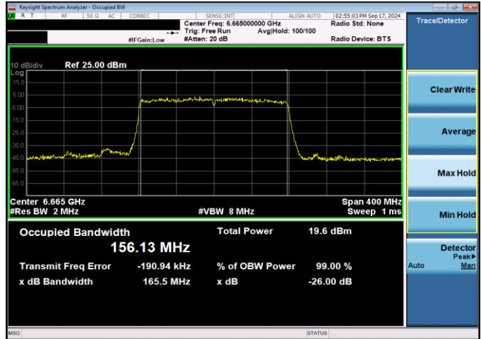
Plot 7-40. 26dB & 99% Bandwidth Plot Antenna WF5T VLP (160MHz 802.11ax (UNII Band 7) – Ch. 143, MCS11)
