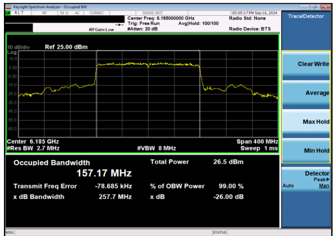
Plot 7-45. 26dB & 99% Bandwidth Plot Antenna WF2 SP (160MHz 802.11ax (UNII Band 5) – Ch. 47, MCS11)
