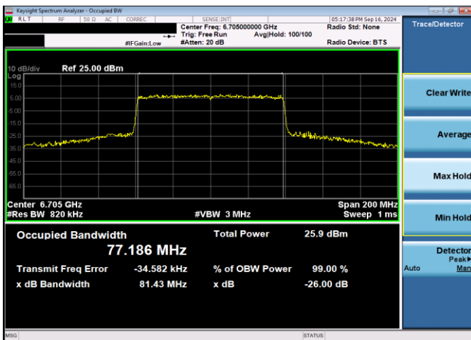
Plot 7-49. 26dB & 99% Bandwidth Plot Antenna WF2 SP (80MHz 802.11ax (UNII Band 7) – Ch. 151, MCS11)
