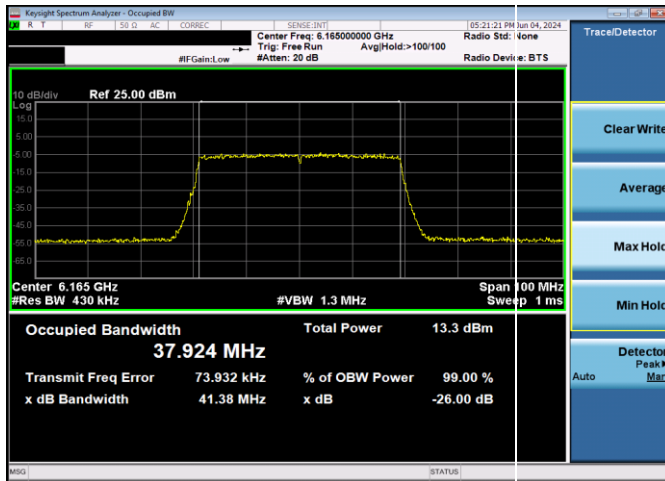
Plot 7-53. 26dB & 99% Bandwidth Plot Antenna WF2 LPI (40MHz 802.11ax (UNII Band 5) – Ch. 43, MCS11)
