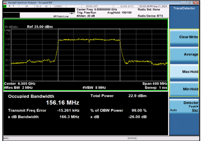
Plot 7-20. 26dB & 99% Bandwidth Plot Antenna WF5T LPI (160MHz 802.11ax (UNII Band 6) – Ch. 111, MCS11)
