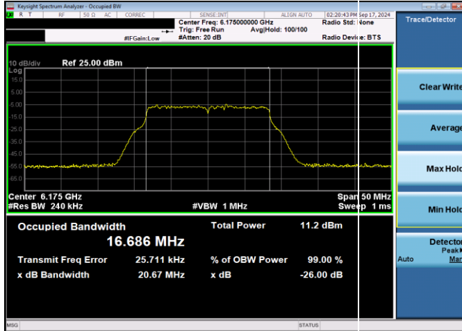
Plot 7-51. 26dB & 99% Bandwidth Plot Antenna WF2 LPI (20MHz 802.11a (UNII Band 5) – Ch. 45, 54Mbps)
