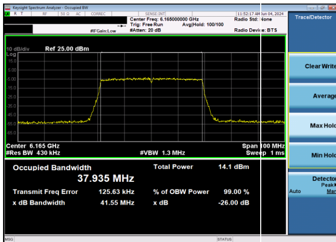
Plot 7-13. 26dB & 99% Bandwidth Plot Antenna WF5T LPI (40MHz 802.11ax (UNII Band 5) – Ch. 43, MCS11)
