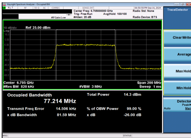
Plot 7-39. 26dB & 99% Bandwidth Plot Antenna WF5T VLP (80MHz 802.11ax (UNII Band 7) – Ch. 151, MCS11)
