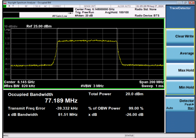
Plot 7-54. 26dB & 99% Bandwidth Plot Antenna WF2 LPI (80MHz 802.11ax (UNII Band 5) – Ch. 39, MCS11)
