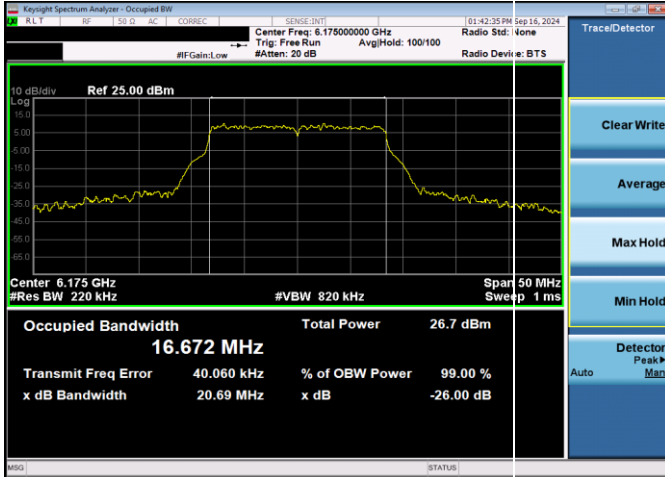
Plot 7-1. 26dB & 99% Bandwidth Plot Antenna WF5T SP (20MHz 802.11a (UNII Band 5) – Ch. 45, 54Mbps)
