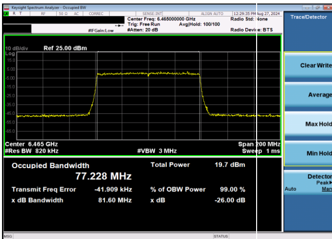
Plot 7-19. 26dB & 99% Bandwidth Plot Antenna WF5T LPI (80MHz 802.11ax (UNII Band 6) – Ch. 103, MCS11)
