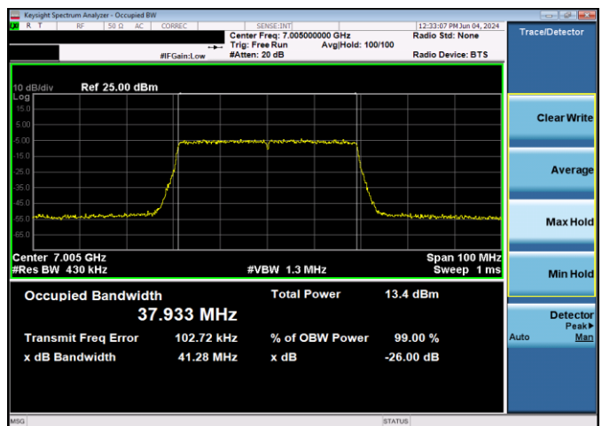
Plot 7-28. 26dB & 99% Bandwidth Plot Antenna WF5T LPI (40MHz 802.11ax (UNII Band 8) – Ch. 211, MCS11)
