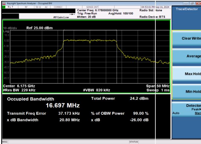
Plot 7-41. 26dB & 99% Bandwidth Plot Antenna WF2 SP (20MHz 802.11a (UNII Band 5) – Ch. 45, 54Mbps)
