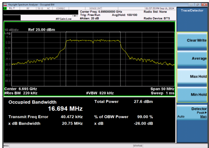
Plot 7-6. 26dB & 99% Bandwidth Plot Antenna WF5T SP (20MHz 802.11a (UNII Band 7) – Ch. 149, 54Mbps)
