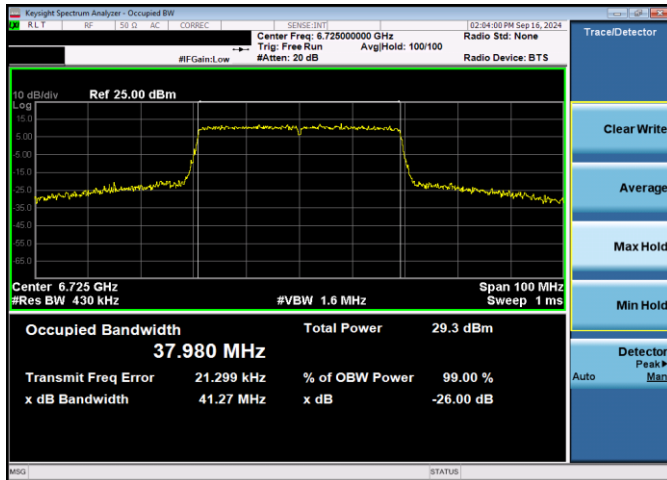
Plot 7-8. 26dB & 99% Bandwidth Plot Antenna WF5T SP (40MHz 802.11ax (UNII Band 7) – Ch. 155, MCS11)
