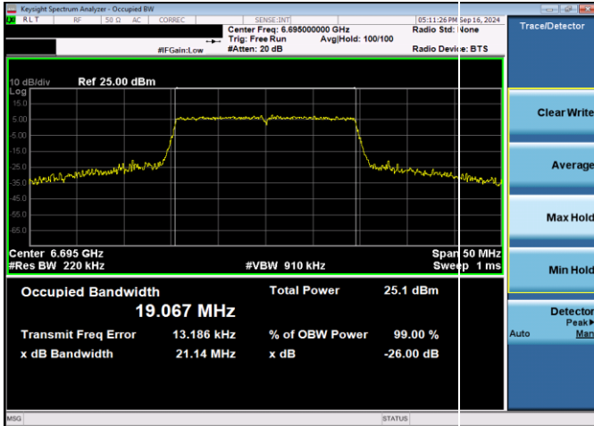
Plot 7-47. 26dB & 99% Bandwidth Plot Antenna WF2 SP (20MHz 802.11ax (UNII Band 7) – Ch. 149, MCS11
