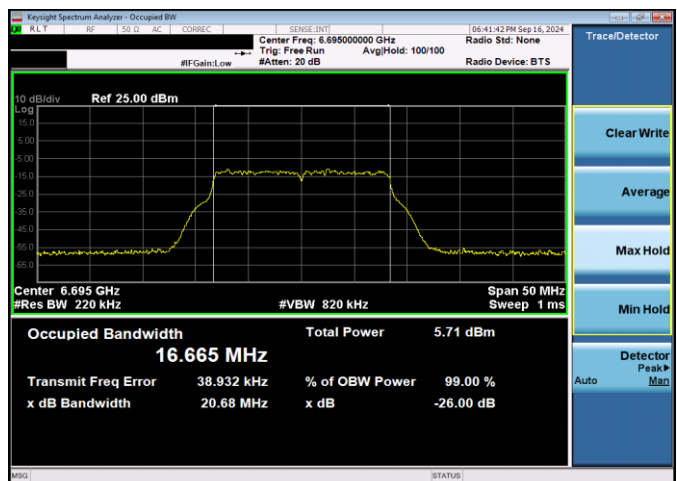
Plot 7-36. 26dB & 99% Bandwidth Plot Antenna WF5T VLP (20MHz 802.11a (UNII Band 7) – Ch. 149, 54Mbps)
