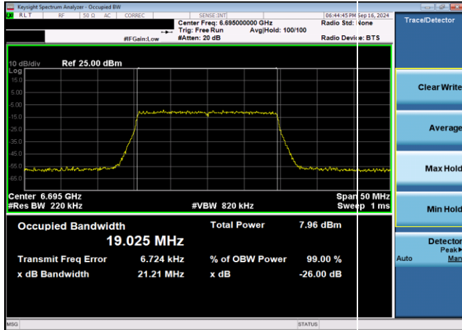
Plot 7-37. 26dB & 99% Bandwidth Plot Antenna WF5T VLP (20MHz 802.11ax (UNII Band 7) – Ch. 149, MCS11)
