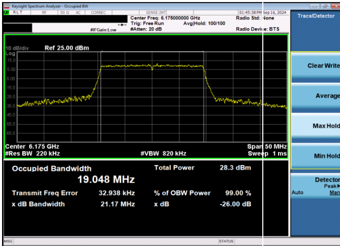
Plot 7-2. 26dB & 99% Bandwidth Plot Antenna WF5T SP (20MHz 802.11ax (UNII Band 5) – Ch. 45, MCS11)
