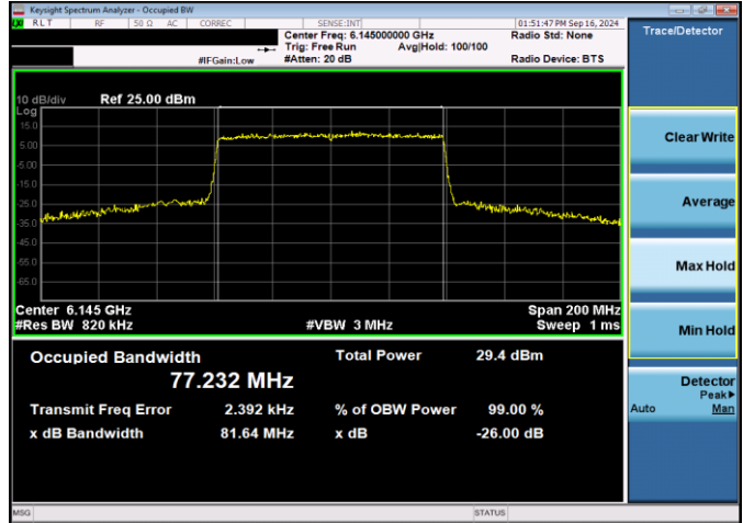
Plot 7-4. 26dB & 99% Bandwidth Plot Antenna WF5T SP (80MHz 802.11ax (UNII Band 5) – Ch. 39, MCS11)
