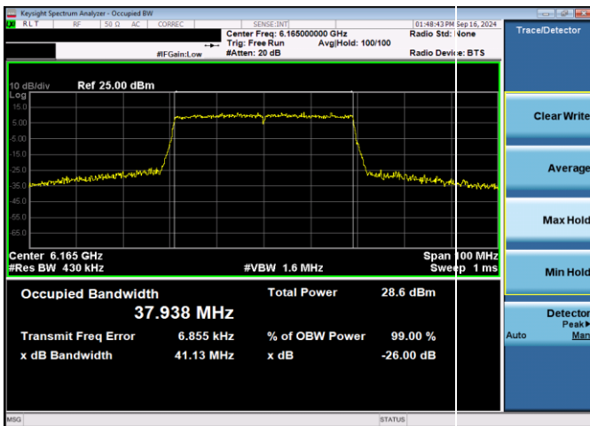
Plot 7-3. 26dB & 99% Bandwidth Plot Antenna WF5T SP (40MHz 802.11ax (UNII Band 5) – Ch. 43, MCS11)
