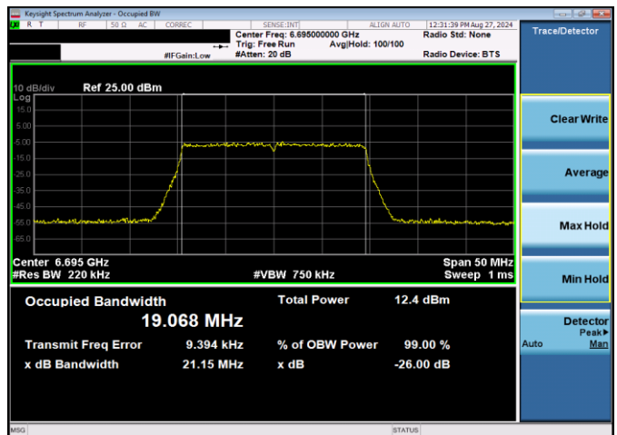
Plot 7-22. 26dB & 99% Bandwidth Plot Antenna WF5T LPI (20MHz 802.11ax (UNII Band 7) – Ch. 149, MCS11)
