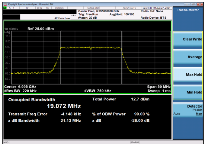
Plot 7-27. 26dB & 99% Bandwidth Plot Antenna WF5T LPI (20MHz 802.11ax (UNII Band 8) – Ch. 209, MCS11)
