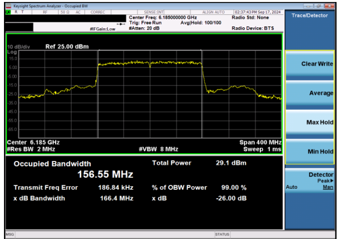
Plot 7-5. 26dB & 99% Bandwidth Plot Antenna WF5T SP (160MHz 802.11ax (UNII Band 5) – Ch. 47, MCS11)
