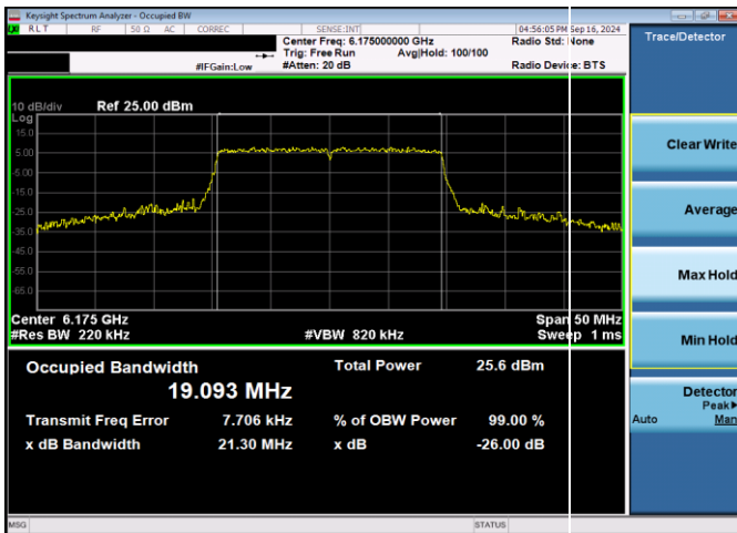
Plot 7-42. 26dB & 99% Bandwidth Plot Antenna WF2 SP (20MHz 802.11ax (UNII Band 5) – Ch. 45, MCS11)
