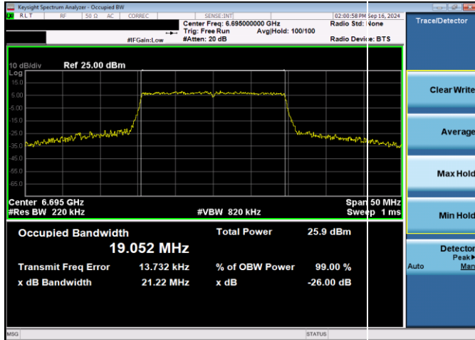
Plot 7-7. 26dB & 99% Bandwidth Plot Antenna WF5T SP (20MHz 802.11ax (UNII Band 7) – Ch. 149, MCS11)
