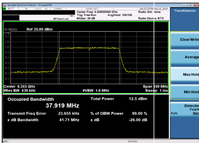
Plot 7-33. 26dB & 99% Bandwidth Plot Antenna WF5T VLP (40MHz 802.11ax (UNII Band 5) – Ch. 59, MCS11)
