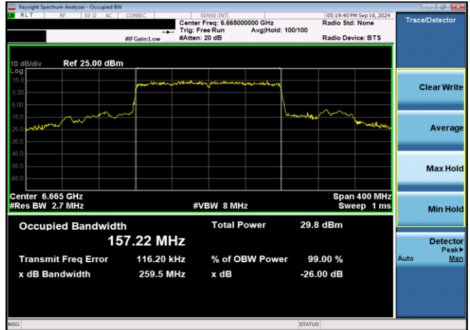
Plot 7-50. 26dB & 99% Bandwidth Plot Antenna WF2 SP (160MHz 802.11ax (UNII Band 7) – Ch. 143, MCS11)
