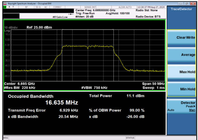
Plot 7-21. 26dB & 99% Bandwidth Plot Antenna WF5T LPI (20MHz 802.11a (UNII Band 7) – Ch. 149, 54Mbps)
