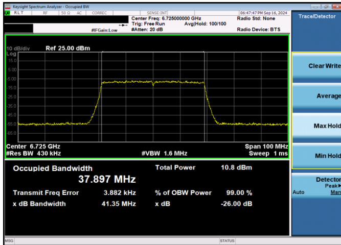
Plot 7-38. 26dB & 99% Bandwidth Plot Antenna WF5T VLP (40MHz 802.11ax (UNII Band 7) – Ch. 155, MCS11)
