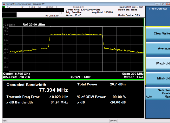
Plot 7-9. 26dB & 99% Bandwidth Plot Antenna WF5T SP (80MHz 802.11ax (UNII Band 7) – Ch. 151, MCS11)
