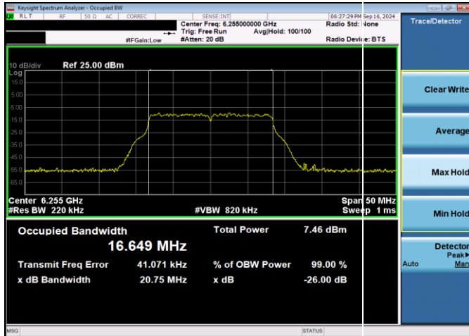
Plot 7-31. 26dB & 99% Bandwidth Plot Antenna WF5T VLP (20MHz 802.11a (UNII Band 5) – Ch. 61, 54Mbps)
