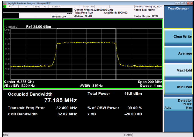
Plot 7-34. 26dB & 99% Bandwidth Plot Antenna WF5T VLP (80MHz 802.11ax (UNII Band 5) – Ch. 55, MCS11)
