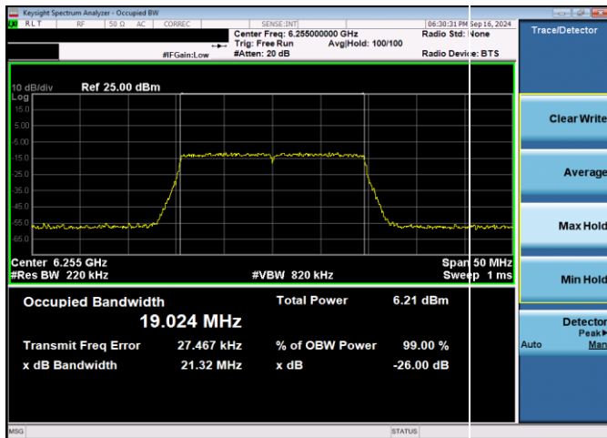
Plot 7-32. 26dB & 99% Bandwidth Plot Antenna WF5T VLP (20MHz 802.11ax (UNII Band 5) – Ch. 61, MCS11)
