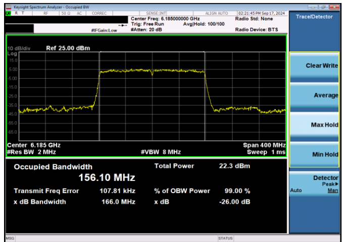
Plot 7-55. 26dB & 99% Bandwidth Plot Antenna WF2 LPI (160MHz 802.11ax (UNII Band 5) – Ch. 47, MCS11)
