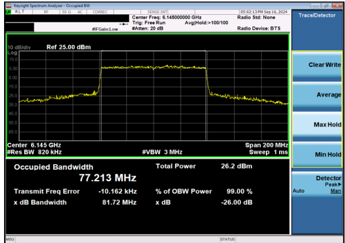
Plot 7-44. 26dB & 99% Bandwidth Plot Antenna WF2 SP (80MHz 802.11ax (UNII Band 5) – Ch. 39, MCS11)
