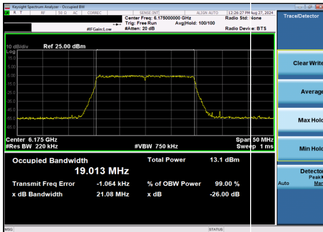
Plot 7-12. 26dB & 99% Bandwidth Plot Antenna WF5T LPI (20MHz 802.11ax (UNII Band 5) – Ch. 45, MCS11)
