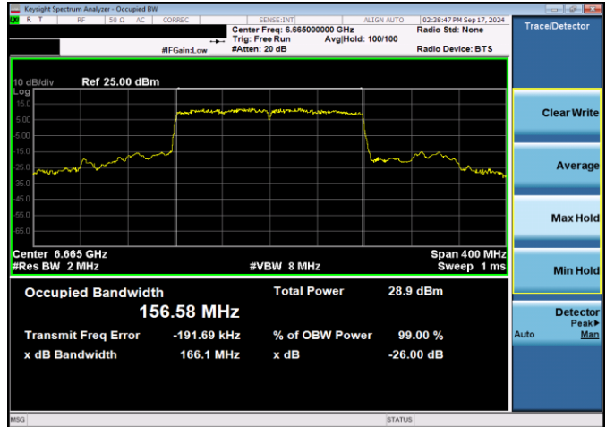
Plot 7-10. 26dB & 99% Bandwidth Plot Antenna WF5T SP (160MHz 802.11ax (UNII Band 7) – Ch. 143, MCS11)
