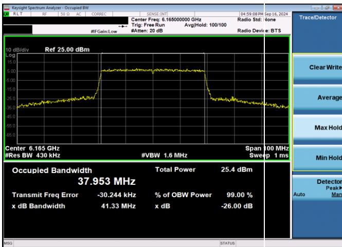
Plot 7-43. 26dB & 99% Bandwidth Plot Antenna WF2 SP (40MHz 802.11ax (UNII Band 5) – Ch. 43, MCS11)
