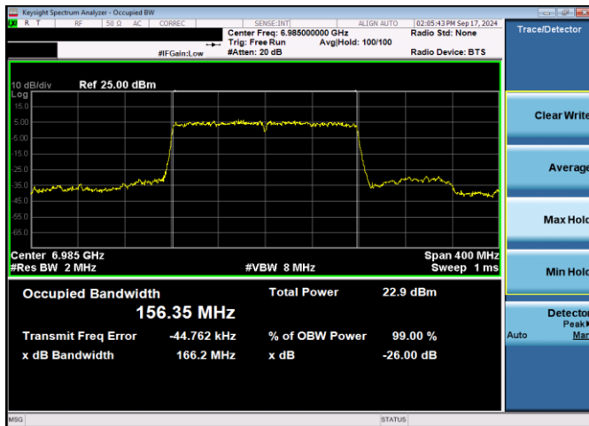
Plot 7-30. 26dB & 99% Bandwidth Plot Antenna WF5T LPI (160MHz 802.11ax (UNII Band 8) – Ch. 207, MCS11)
