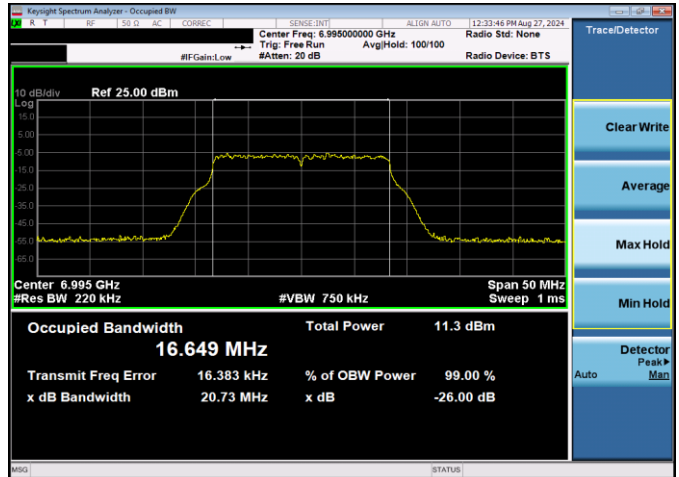
Plot 7-26. 26dB & 99% Bandwidth Plot Antenna WF5T LPI (20MHz 802.11a (UNII Band 8) – Ch. 209, 54Mbps)
