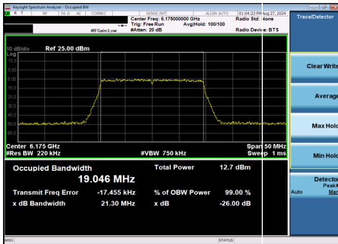
Plot 7-52. 26dB & 99% Bandwidth Plot Antenna WF2 LPI (20MHz 802.11ax (UNII Band 5) – Ch. 45, MCS11)
