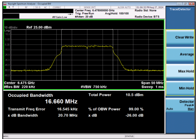
Plot 7-56. 26dB & 99% Bandwidth Plot Antenna WF2 LPI (20MHz 802.11a (UNII Band 6) – Ch. 105, 54Mbps)
