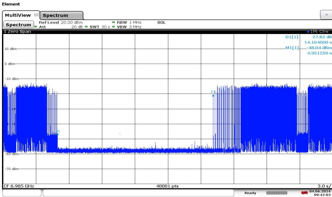
Plot 7-1266. LPI Contention Based Protocol Timing Plot – UNII 8 – 160MHz Channel 207 – Low
