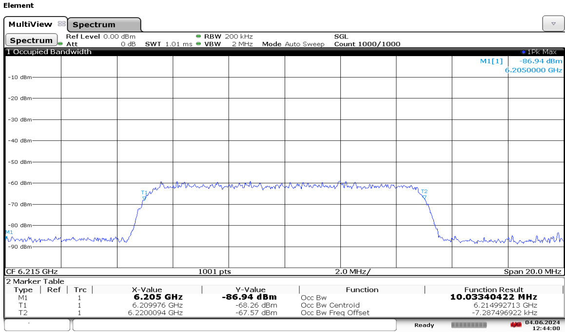
Plot 7-1237. AWGN Signal – UNII 5 – 20MHz
