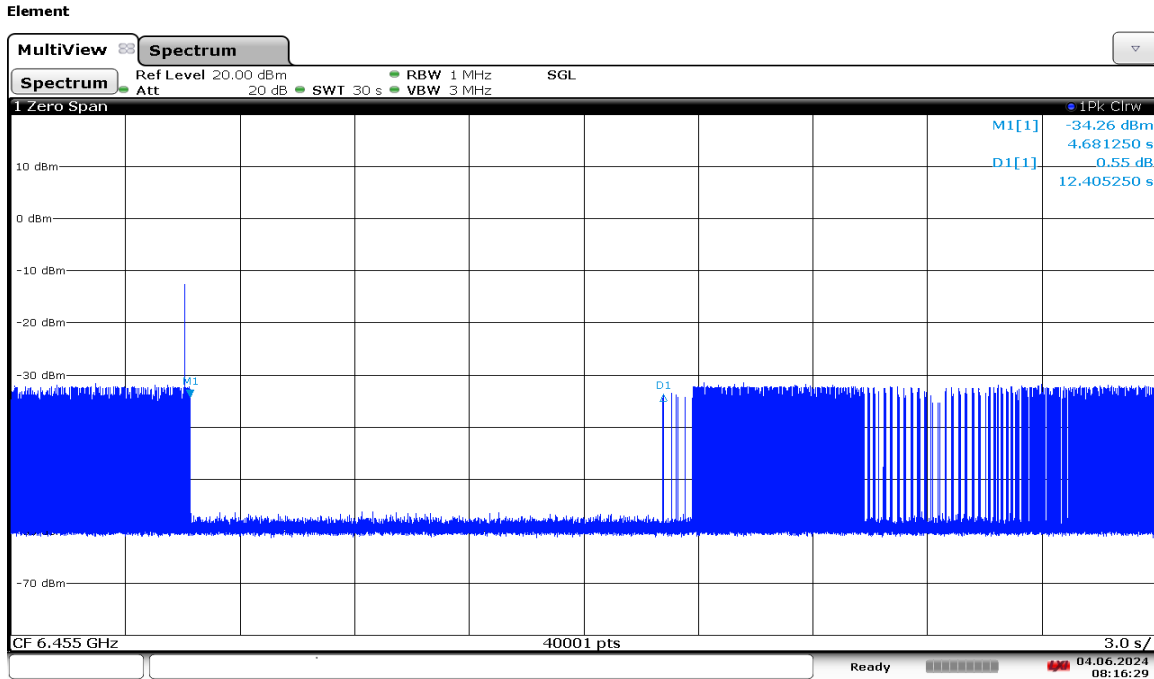
Plot 7-1257. LPI Contention Based Protocol Timing Plot – UNII 6 – 20MHz Channel 101
