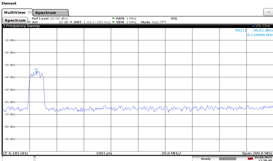
Plot 7-1278. 160MHz Bandwidth – AWGN Signal Injected at Low End – Channel 47
