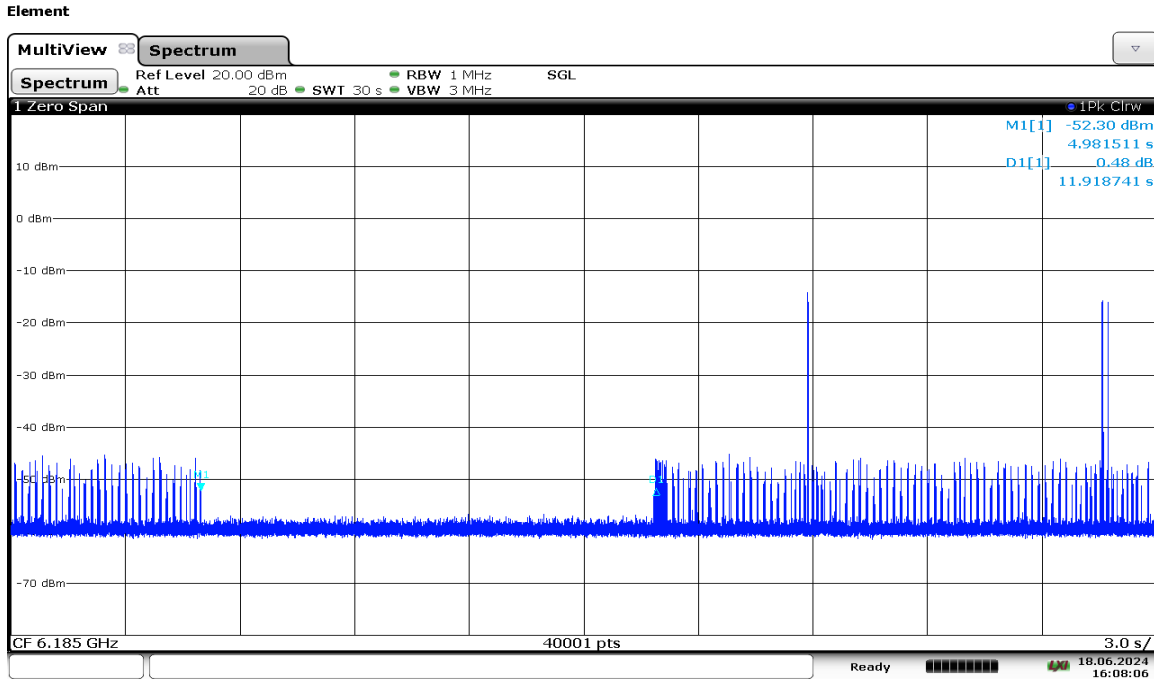
Plot 7-1271. VLP Contention Based Protocol Timing Plot – UNII 5 – 160MHz Channel 47 – Mid
