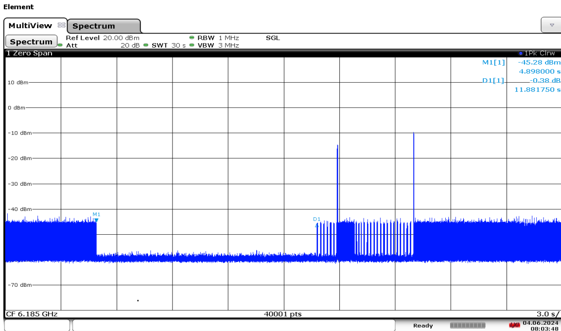
Plot 7-1254. LPI Contention Based Protocol Timing Plot – UNII 5 – 160MHz Channel 47 – Low
