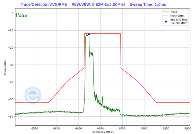
Plot 7-1181. VLP In-Band Emission Plot Antenna WF2 (80MHz 802.11ax RU106 (UNII Band 7) – Ch. 151)
