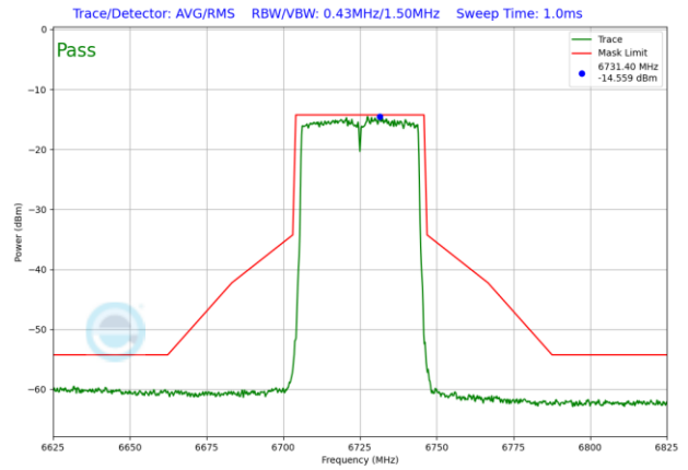
Plot 7-1180. VLP In-Band Emission Plot Antenna WF2 (40MHz 802.11ax RU484 (UNII Band 7) – Ch. 155)
