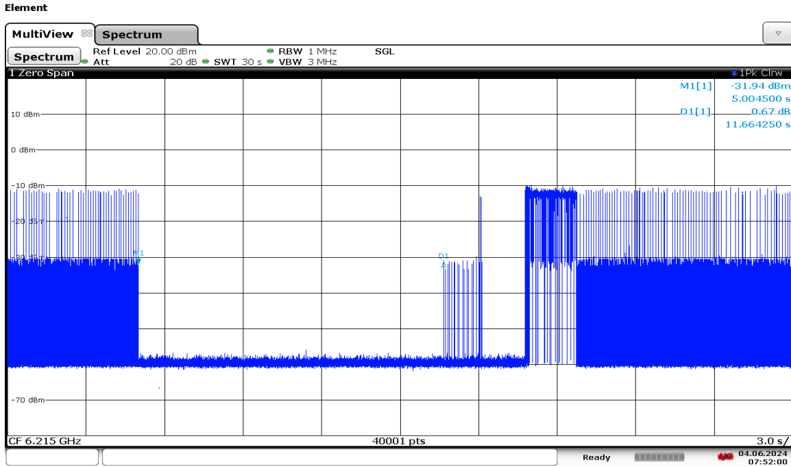
Plot 7-1253. LPI Contention Based Protocol Timing Plot – UNII 5 – 20MHz Channel 53
