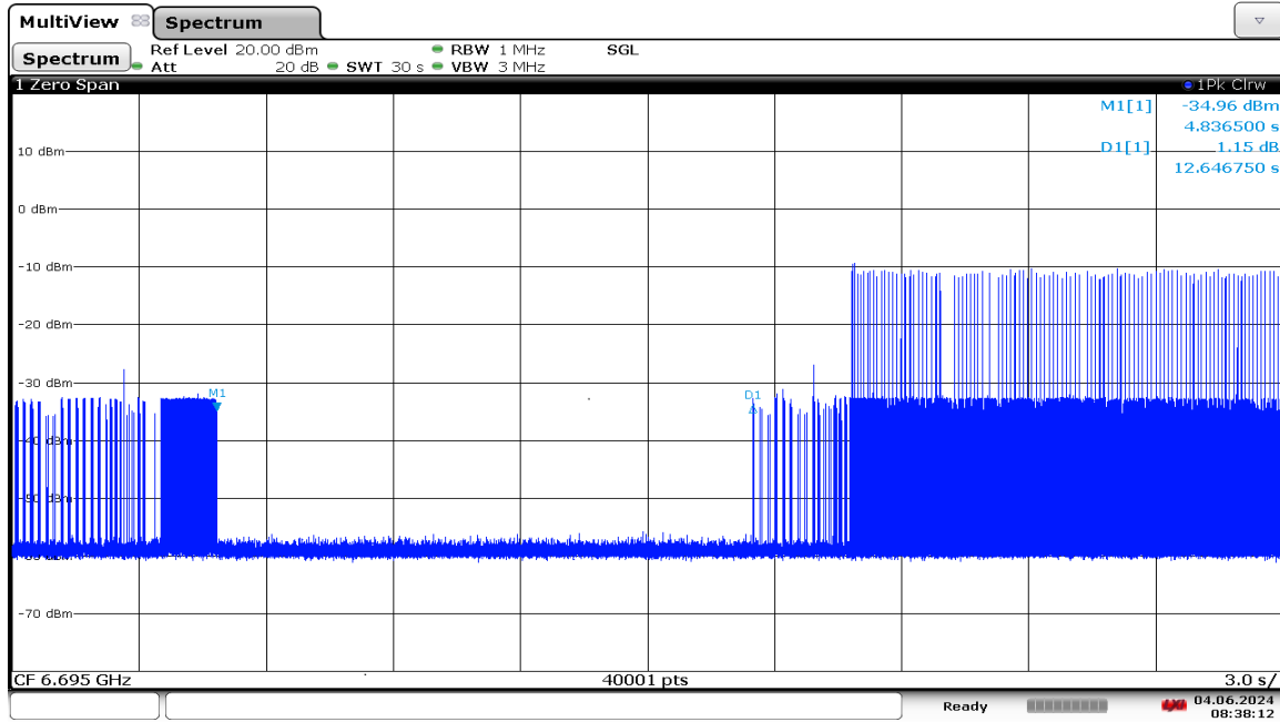
Plot 7-1261. LPI Contention Based Protocol Timing Plot – UNII 7 – 20MHz Channel 149
