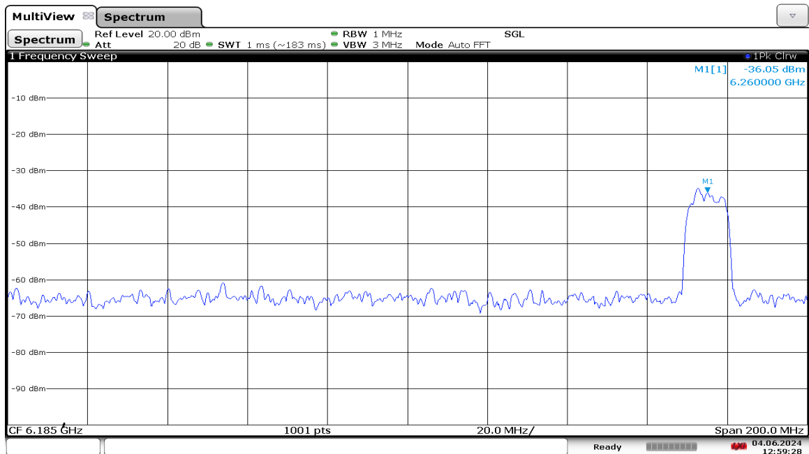
Plot 7-1280. 160MHz Bandwidth – AWGN Signal Injected at High End – Channel 47
