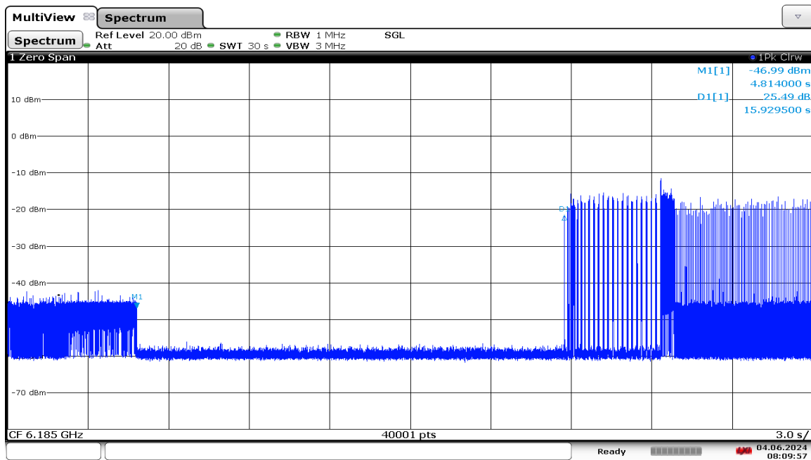
Plot 7-1256. LPI Contention Based Protocol Timing Plot – UNII 5 – 160MHz Channel 47 – High
