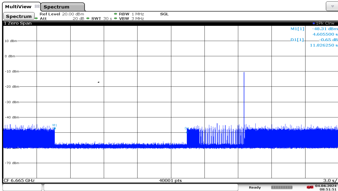
Plot 7-1262. LPI Contention Based Protocol Timing Plot – UNII 7 – 160MHz Channel 143 – Low
