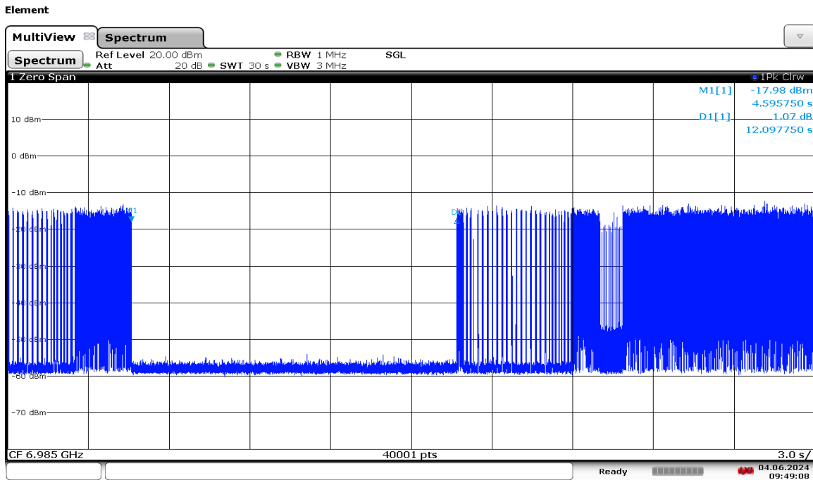
Plot 7-1268. LPI Contention Based Protocol Timing Plot – UNII 8 – 160MHz Channel 207 – High
