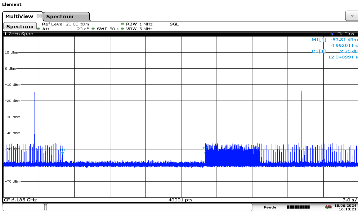
Plot 7-1272. VLP Contention Based Protocol Timing Plot – UNII 5 – 160MHz Channel 47 – High
