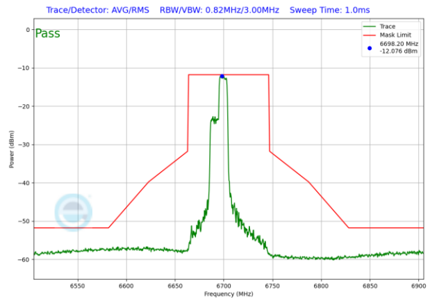
Plot 7-1182. VLP In-Band Emission Plot Antenna WF2 (80MHz 802.11ax RU106 (UNII Band 7) – Ch. 151)
