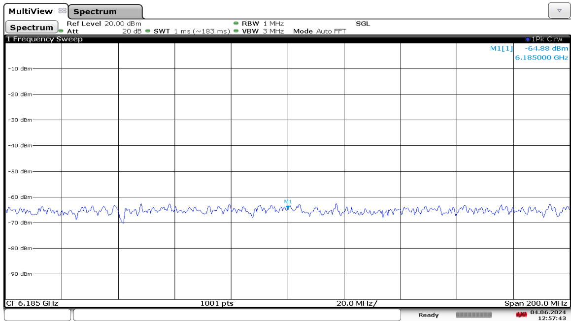
Plot 7-1279. 160MHz Bandwidth – AWGN Signal Injected at Center – Channel 47
