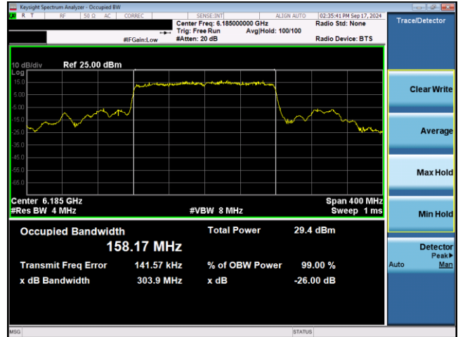
Plot 7-16. 26dB & 99% Bandwidth Plot Antenna WF5T SP (160MHz 802.11ax RU996x2 (UNII Band 5) – Ch. 47)
