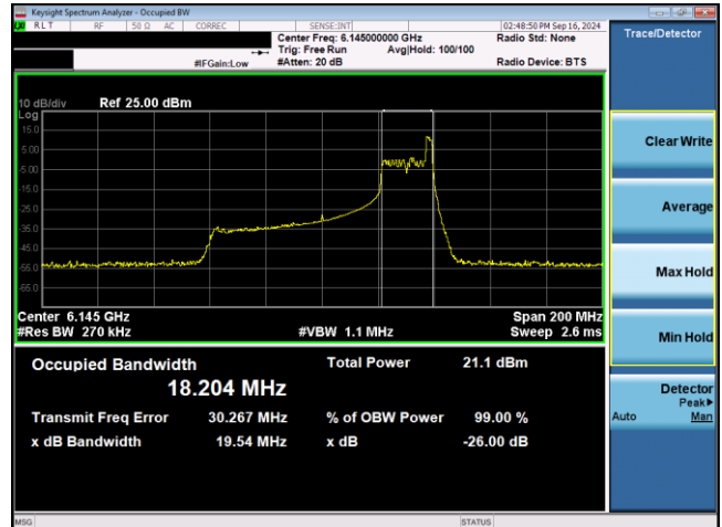
Plot 7-43. 26dB & 99% Bandwidth Plot Antenna WF2 SP (80MHz 802.11ax RU26 (UNII Band 5) – Ch. 39)
