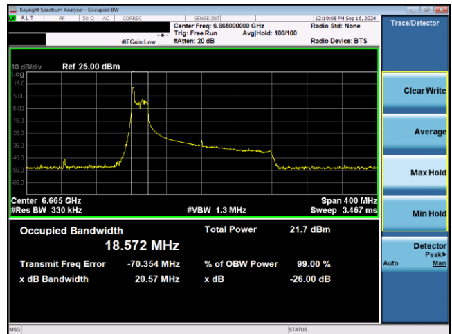
Plot 7-29. 26dB & 99% Bandwidth Plot Antenna WF5T SP (160MHz 802.11ax RU26 (UNII Band 7) – Ch. 143)
