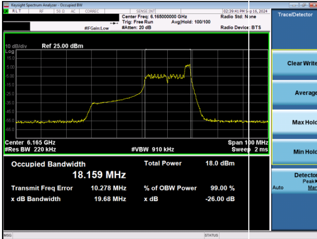
Plot 7-39. 26dB & 99% Bandwidth Plot Antenna WF2 SP (40MHz 802.11ax RU26 (UNII Band 5) – Ch. 43)
