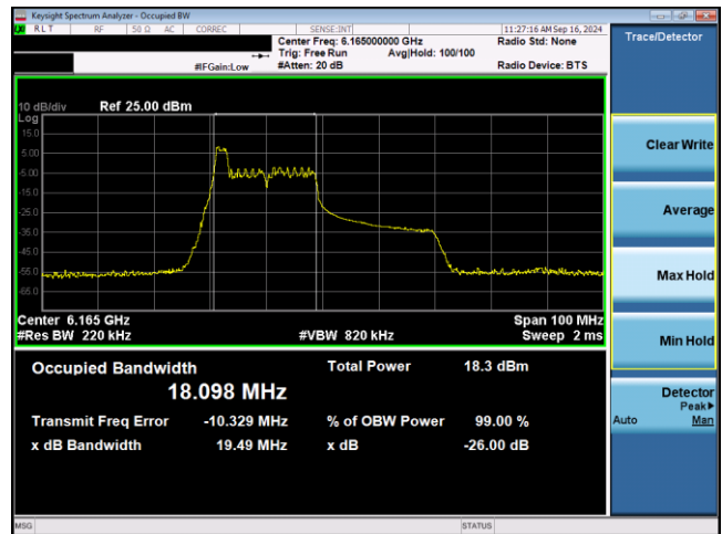
Plot 7-5. 26dB & 99% Bandwidth Plot Antenna WF5T SP (40MHz 802.11ax RU26 (UNII Band 5) – Ch. 43)
