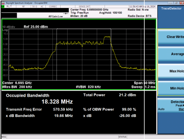
Plot 7-19. 26dB & 99% Bandwidth Plot Antenna WF5T SP (20MHz 802.11ax RU26 (UNII Band 7) – Ch. 149)
