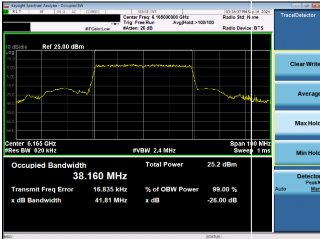
Plot 7-40. 26dB & 99% Bandwidth Plot Antenna WF2 SP (40MHz 802.11ax RU484 (UNII Band 5) – Ch. 43)
