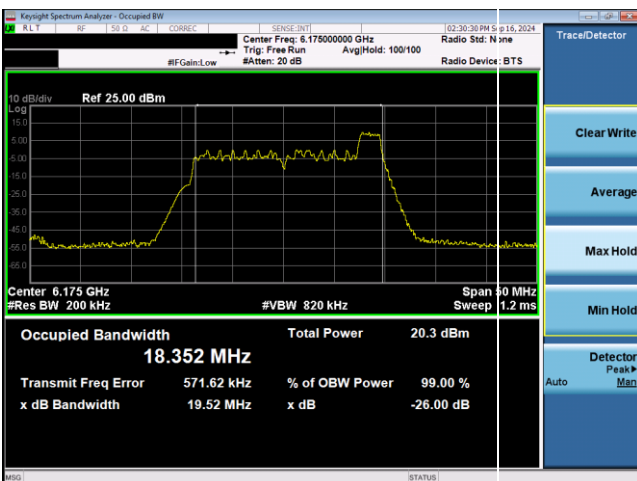
Plot 7-35. 26dB & 99% Bandwidth Plot Antenna WF2 SP (20MHz 802.11ax RU26 (UNII Band 5) – Ch. 45)
