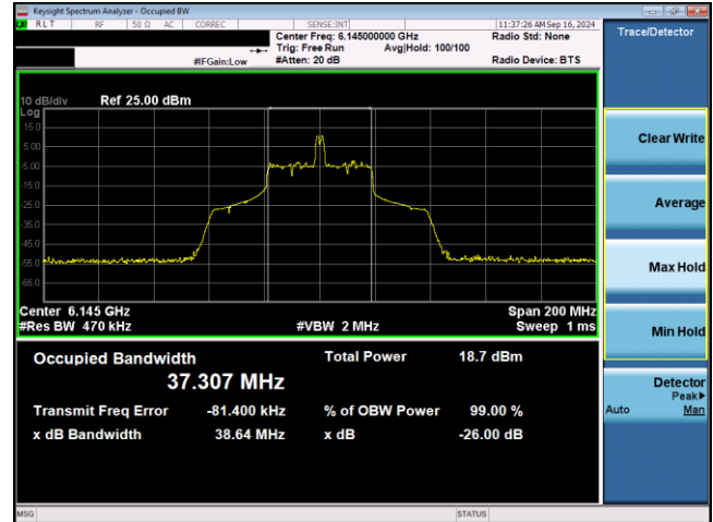
Plot 7-10. 26dB & 99% Bandwidth Plot Antenna WF5T SP (80MHz 802.11ax RU26 (UNII Band 5) – Ch. 39)
