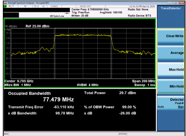
Plot 7-28. 26dB & 99% Bandwidth Plot Antenna WF5T SP (80MHz 802.11ax RU996 (UNII Band 7) – Ch. 151)
