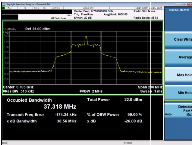
Plot 7-26. 26dB & 99% Bandwidth Plot Antenna WF5T SP (80MHz 802.11ax RU26 (UNII Band 7) – Ch. 151)
