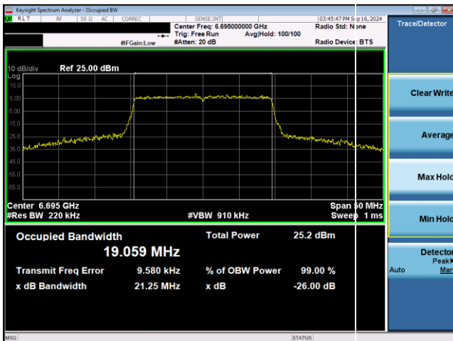
Plot 7-52. 26dB & 99% Bandwidth Plot Antenna WF2 SP (20MHz 802.11ax RU242 (UNII Band 7) – Ch. 149)
