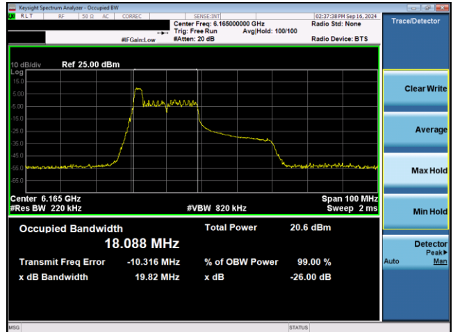
Plot 7-37. 26dB & 99% Bandwidth Plot Antenna WF2 SP (40MHz 802.11ax RU26 (UNII Band 5) – Ch. 43)
