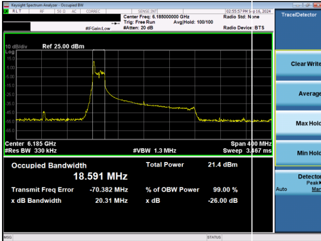
Plot 7-45. 26dB & 99% Bandwidth Plot Antenna WF2 SP (160MHz 802.11ax RU26 (UNII Band 5) – Ch. 47)
