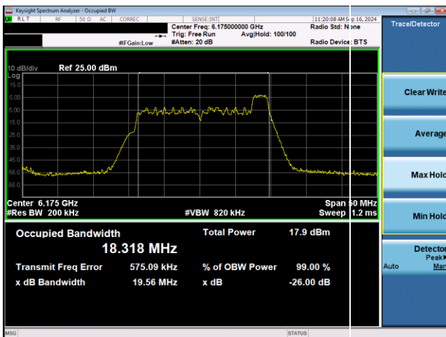
Plot 7-3. 26dB & 99% Bandwidth Plot Antenna WF5T SP (20MHz 802.11ax RU26 (UNII Band 5) – Ch. 45)
