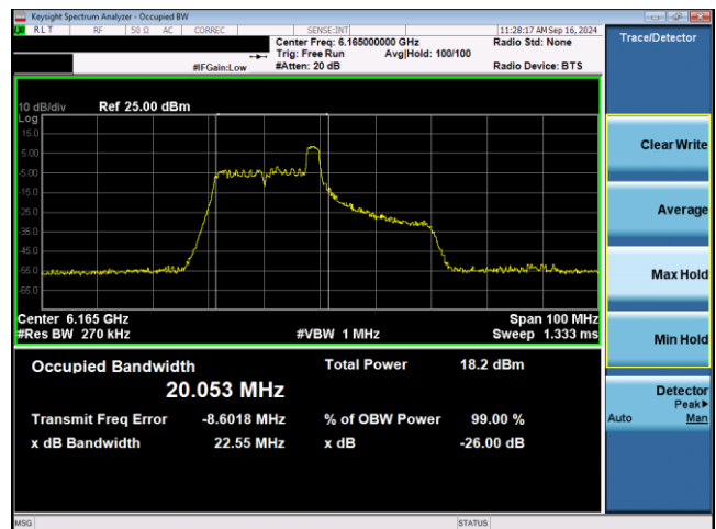
Plot 7-6. 26dB & 99% Bandwidth Plot Antenna WF5T SP (40MHz 802.11ax RU26 (UNII Band 5) – Ch. 43)
