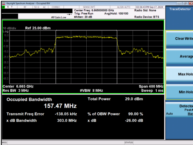
Plot 7-32. 26dB & 99% Bandwidth Plot Antenna WF5T SP (160MHz 802.11ax RU996x2 (UNII Band 7) – Ch. 143)
