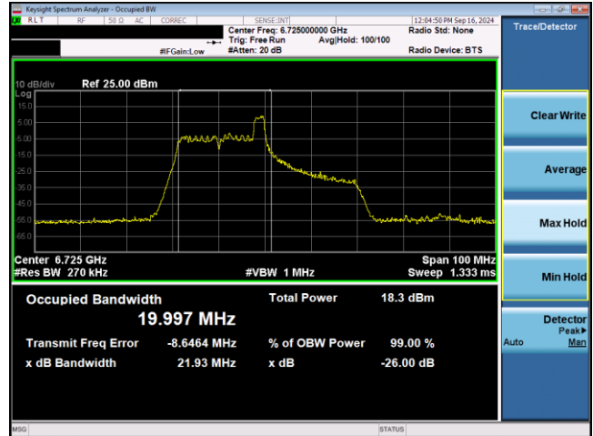
Plot 7-22. 26dB & 99% Bandwidth Plot Antenna WF5T SP (40MHz 802.11ax RU26 (UNII Band 7) – Ch. 155)
