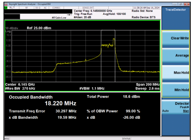
Plot 7-11. 26dB & 99% Bandwidth Plot Antenna WF5T SP (80MHz 802.11ax RU26 (UNII Band 5) – Ch. 39)
