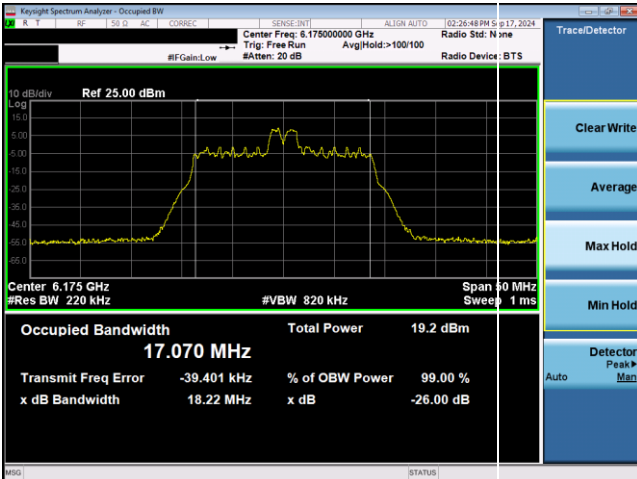
Plot 7-34. 26dB & 99% Bandwidth Plot Antenna WF2 SP (20MHz 802.11ax RU26 (UNII Band 5) – Ch. 45)
