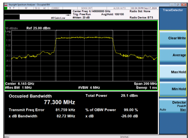
Plot 7-12. 26dB & 99% Bandwidth Plot Antenna WF5T SP (80MHz 802.11ax RU996 (UNII Band 5) – Ch. 39)
