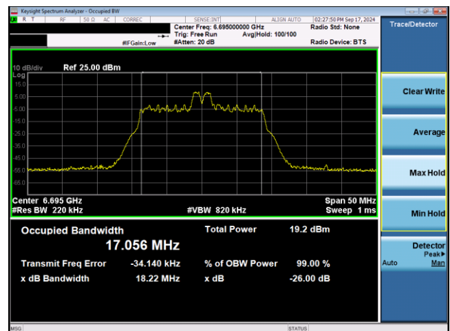
Plot 7-50. 26dB & 99% Bandwidth Plot Antenna WF2 SP (20MHz 802.11ax RU26 (UNII Band 7) – Ch. 149)
