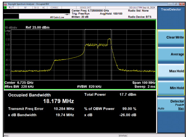
Plot 7-55. 26dB & 99% Bandwidth Plot Antenna WF2 SP (40MHz 802.11ax RU26 (UNII Band 7) – Ch. 155)
