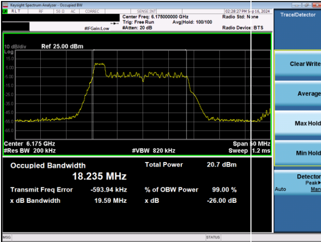
Plot 7-33. 26dB & 99% Bandwidth Plot Antenna WF2 SP (20MHz 802.11ax RU26 (UNII Band 5) – Ch. 45)
