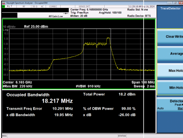
Plot 7-7. 26dB & 99% Bandwidth Plot Antenna WF5T SP (40MHz 802.11ax RU26 (UNII Band 5) – Ch. 43)
