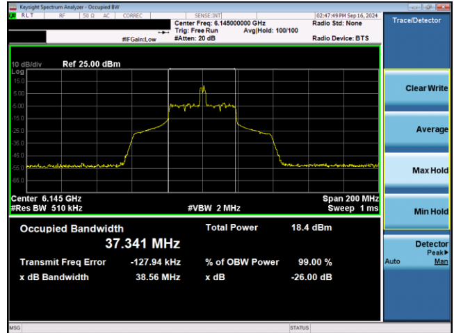
Plot 7-42. 26dB & 99% Bandwidth Plot Antenna WF2 SP (80MHz 802.11ax RU26 (UNII Band 5) – Ch. 39)
