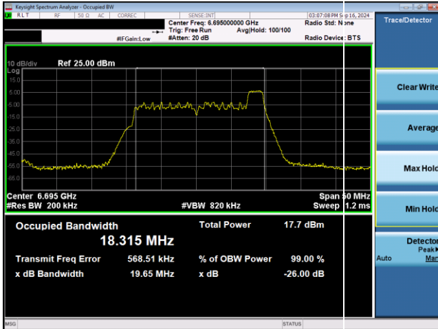
Plot 7-51. 26dB & 99% Bandwidth Plot Antenna WF2 SP (20MHz 802.11ax RU26 (UNII Band 7) – Ch. 149)
