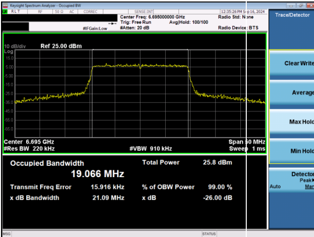
Plot 7-20. 26dB & 99% Bandwidth Plot Antenna WF5T SP (20MHz 802.11ax RU242 (UNII Band 7) – Ch. 149)
