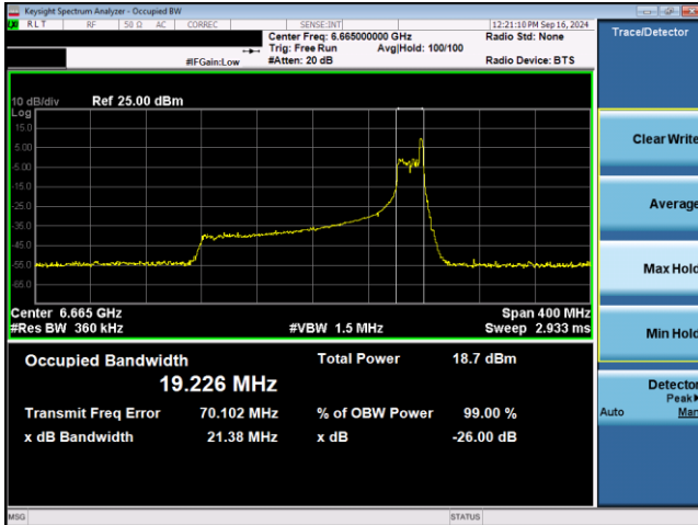
Plot 7-31. 26dB & 99% Bandwidth Plot Antenna WF5T SP (160MHz 802.11ax RU26 (UNII Band 7) – Ch. 143)
