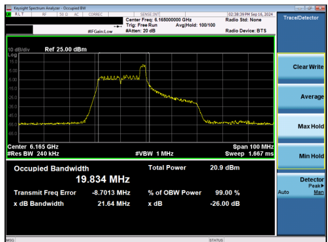
Plot 7-38. 26dB & 99% Bandwidth Plot Antenna WF2 SP (40MHz 802.11ax RU26 (UNII Band 5) – Ch. 43)
