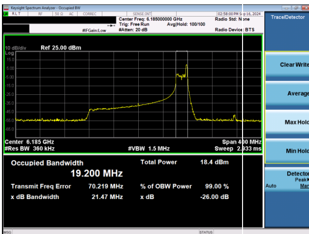
Plot 7-47. 26dB & 99% Bandwidth Plot Antenna WF2 SP (160MHz 802.11ax RU26 (UNII Band 5) – Ch. 47)
