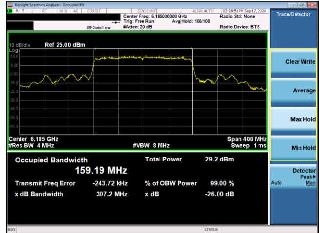
Plot 7-48. 26dB & 99% Bandwidth Plot Antenna WF2 SP (160MHz 802.11ax RU996x2 (UNII Band 5) – Ch. 47)
