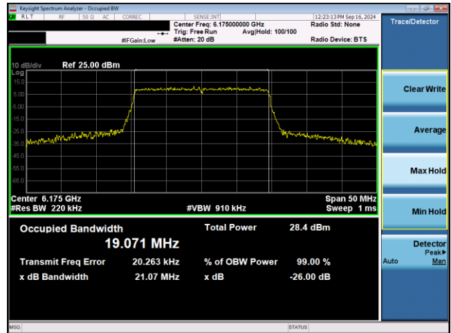
Plot 7-4. 26dB & 99% Bandwidth Plot Antenna WF5T SP (20MHz 802.11ax RU242 (UNII Band 5) – Ch. 45)
