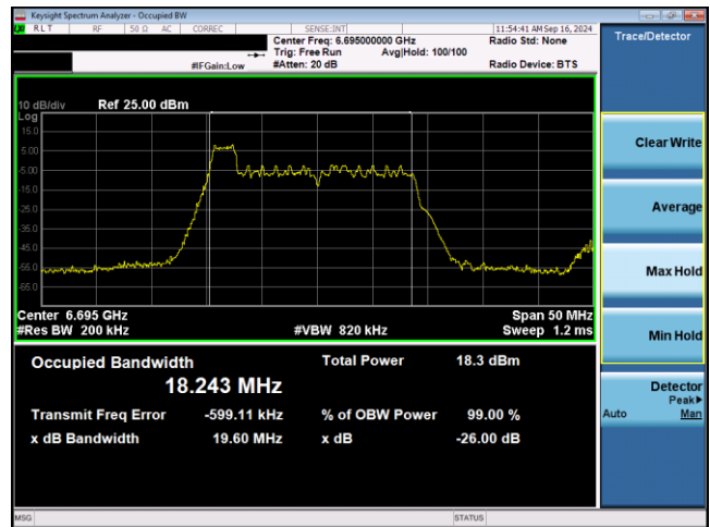
Plot 7-17. 26dB & 99% Bandwidth Plot Antenna WF5T SP (20MHz 802.11ax RU26 (UNII Band 7) – Ch. 149)
