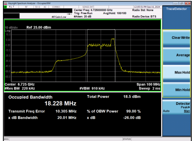
Plot 7-23. 26dB & 99% Bandwidth Plot Antenna WF5T SP (40MHz 802.11ax RU26 (UNII Band 7) – Ch. 155)
