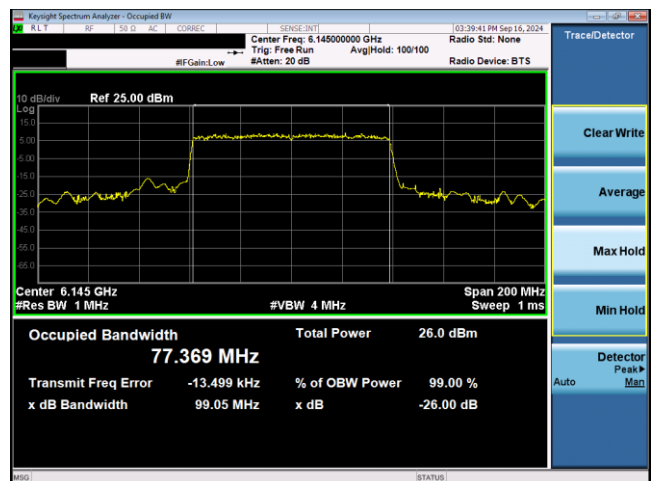
Plot 7-44. 26dB & 99% Bandwidth Plot Antenna WF2 SP (80MHz 802.11ax RU996 (UNII Band 5) – Ch. 39)
