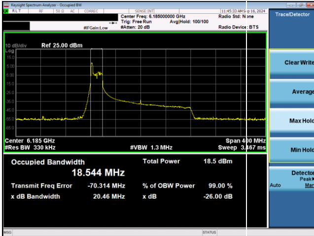
Plot 7-13. 26dB & 99% Bandwidth Plot Antenna WF5T SP (160MHz 802.11ax RU26 (UNII Band 5) – Ch. 47)
