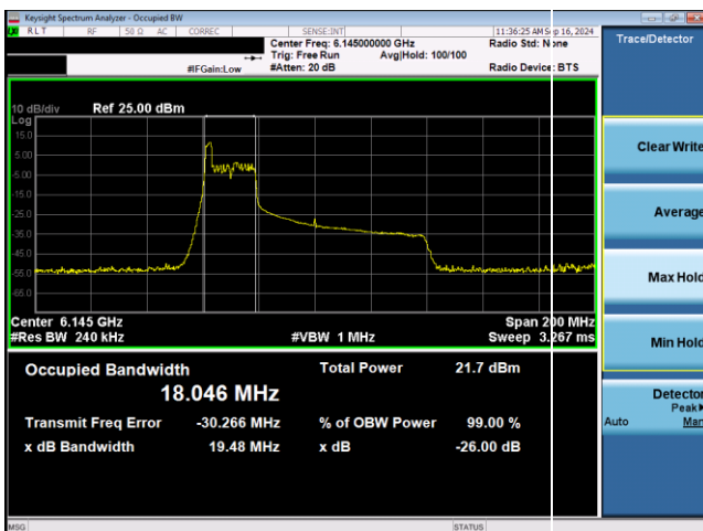
Plot 7-9. 26dB & 99% Bandwidth Plot Antenna WF5T SP (80MHz 802.11ax RU26 (UNII Band 5) – Ch. 39)
