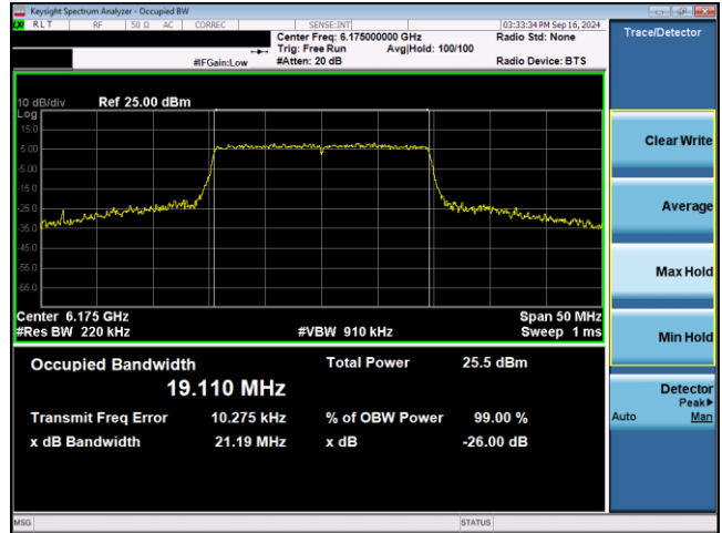
Plot 7-36. 26dB & 99% Bandwidth Plot Antenna WF2 SP (20MHz 802.11ax RU242 (UNII Band 5) – Ch. 45)
