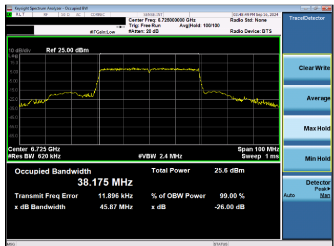
Plot 7-56. 26dB & 99% Bandwidth Plot Antenna WF2 SP (40MHz 802.11ax RU484 (UNII Band 7) – Ch. 155)
