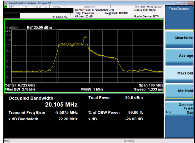
Plot 7-54. 26dB & 99% Bandwidth Plot Antenna WF2 SP (40MHz 802.11ax RU26 (UNII Band 7) – Ch. 155)
