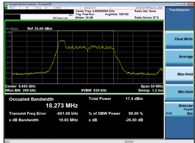
Plot 7-49. 26dB & 99% Bandwidth Plot Antenna WF2 SP (20MHz 802.11ax RU26 (UNII Band 7) – Ch. 149)
