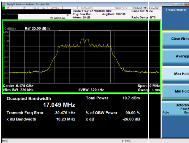
Plot 7-2. 26dB & 99% Bandwidth Plot Antenna WF5T SP (20MHz 802.11ax RU26 (UNII Band 5) – Ch. 45)
