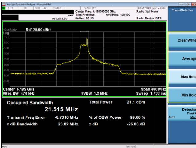
Plot 7-46. 26dB & 99% Bandwidth Plot Antenna WF2 SP (160MHz 802.11ax RU26 (UNII Band 5) – Ch. 47)
