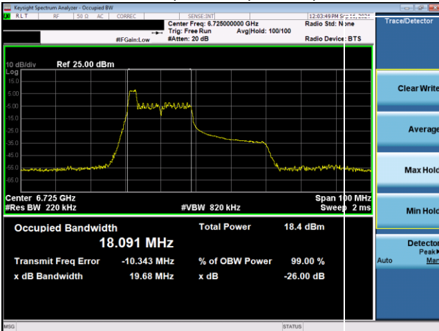
Plot 7-21. 26dB & 99% Bandwidth Plot Antenna WF5T SP (40MHz 802.11ax RU26 (UNII Band 7) – Ch. 155)
