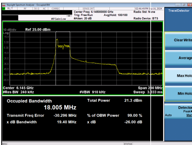
Plot 7-41. 26dB & 99% Bandwidth Plot Antenna WF2 SP (80MHz 802.11ax RU26 (UNII Band 5) – Ch. 39)
