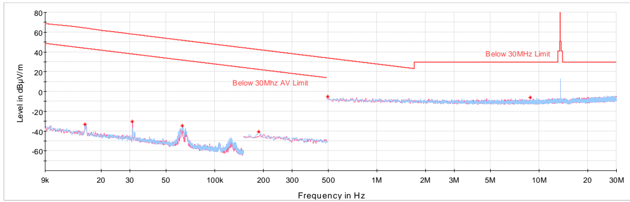
Plot 7-2. Radiated Spurious Plot 9kHz – 30MHz (Charging Rate 2.6C, with AC/DC Adapter)
