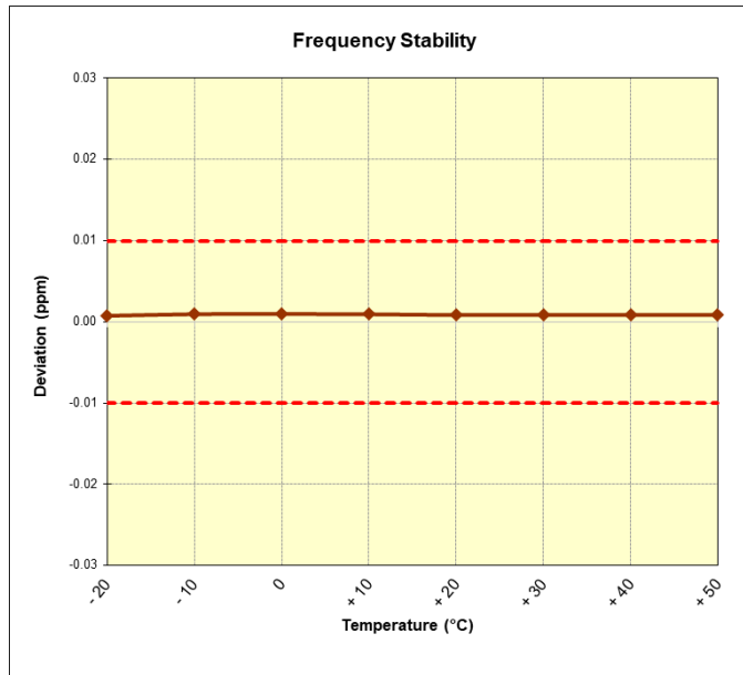
Figure 7-5. Frequency Stability Plot (Charging Rate 2.6C)
