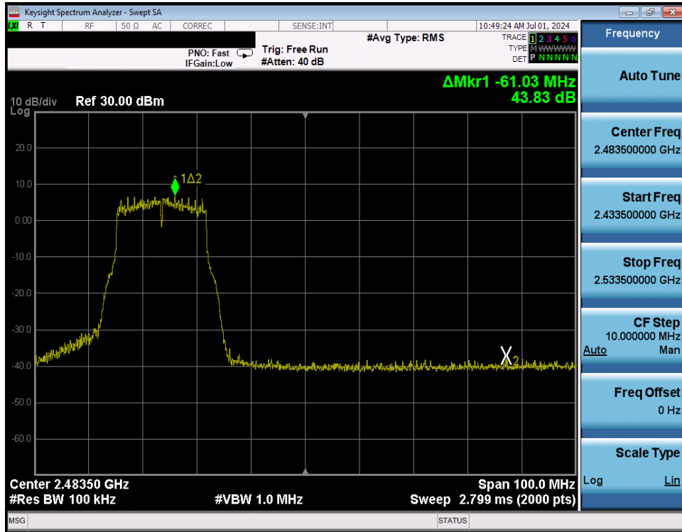
Plot 7-226. Band Edge Plot Antenna WF8 (802.11g – Ch. 10) – 24Mbps
