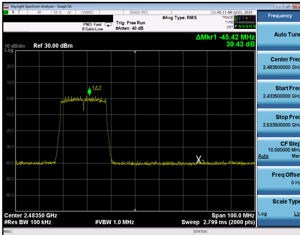
Plot 7-300. Band Edge Plot Antenna WF8 (802.11ax (SU - 2.4GHz) – Ch. 11) – MCS9
