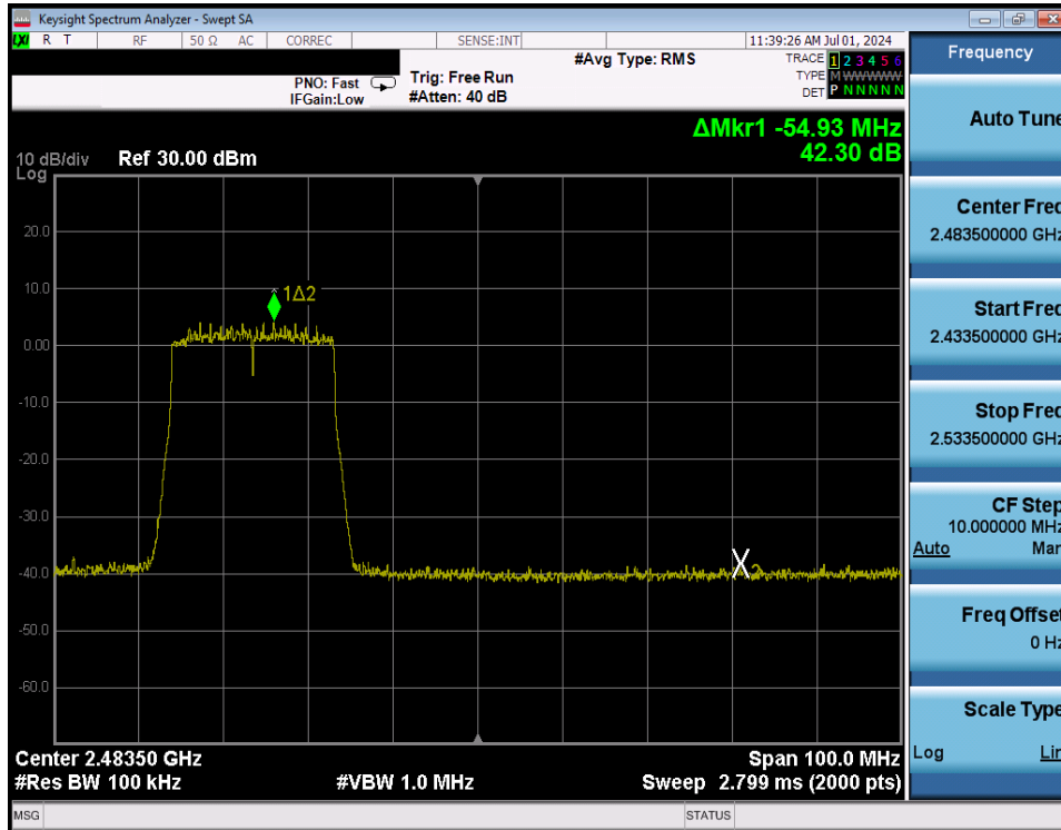
Plot 7-299. Band Edge Plot Antenna WF8 (802.11ax (SU - 2.4GHz) – Ch. 10) – MCS9
