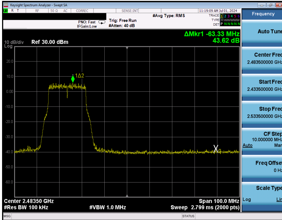
Plot 7-271. Band Edge Plot Antenna WF8 (802.11g – Ch. 10) – 54Mbps
