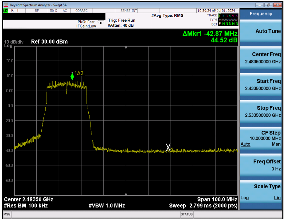
Plot 7-240. Band Edge Plot Antenna WF8 (802.11n (2.4GHz) – Ch. 10) – MCS4
