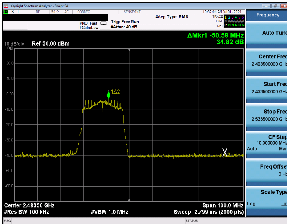
Plot 7-202. Band Edge Plot Antenna WF8 (802.11n (2.4GHz) – Ch. 13) – MCS2
