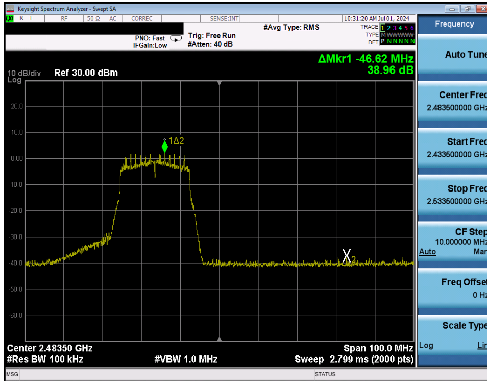
Plot 7-201. Band Edge Plot Antenna WF8 (802.11n (2.4GHz) – Ch. 12) – MCS2
