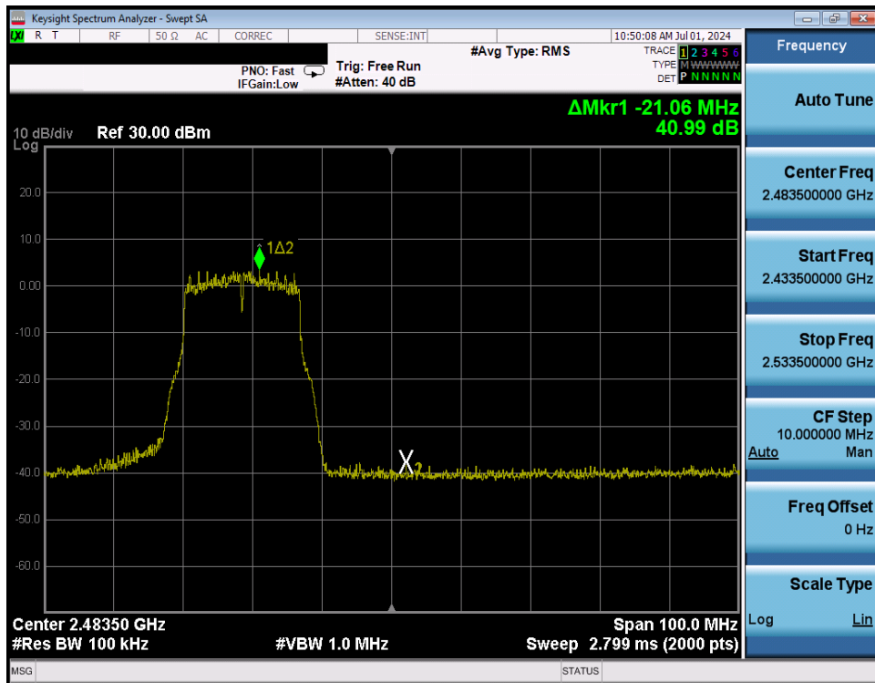
Plot 7-227. Band Edge Plot Antenna WF8 (802.11g – Ch. 11) – 24Mbps
