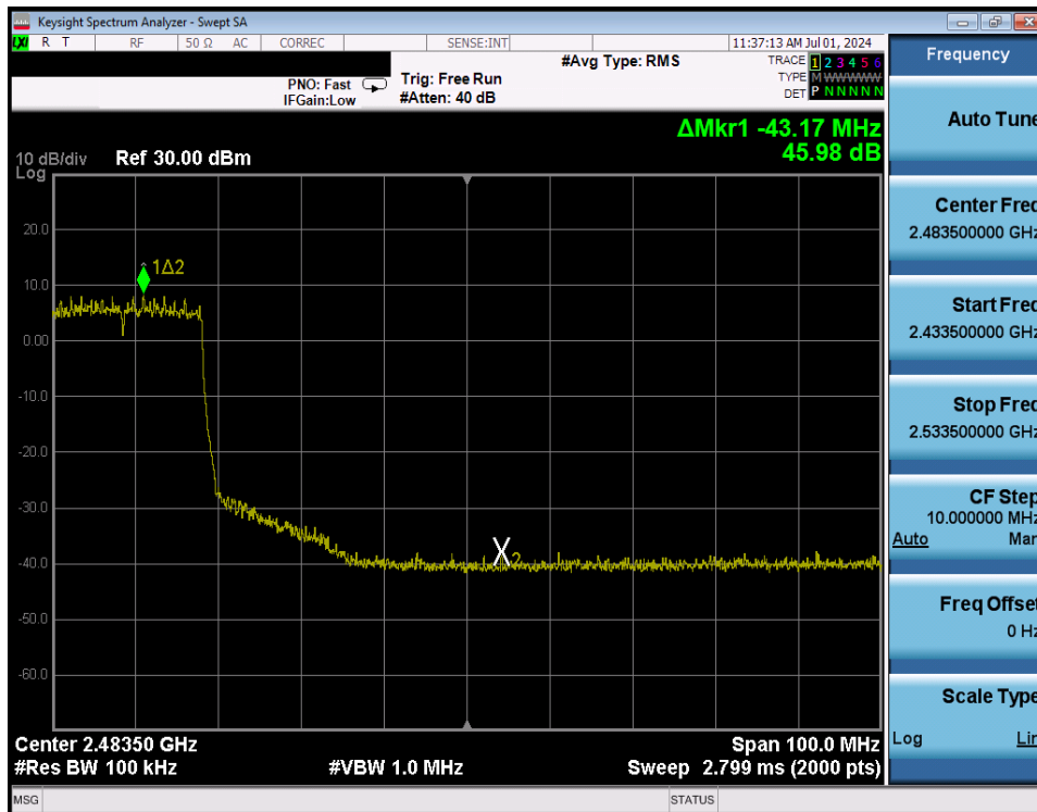
Plot 7-296. Band Edge Plot Antenna WF8 (802.11ax (SU - 2.4GHz) – Ch. 7) – MCS9
