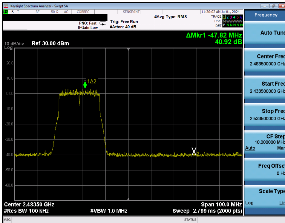
Plot 7-286. Band Edge Plot Antenna WF8 (802.11n (2.4GHz) – Ch. 11) – MCS7
