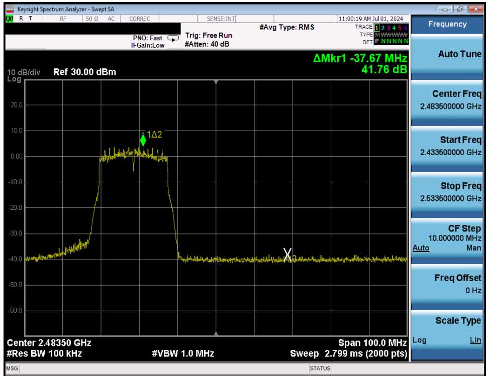
Plot 7-241. Band Edge Plot Antenna WF8 (802.11n (2.4GHz) – Ch. 11) – MCS4
