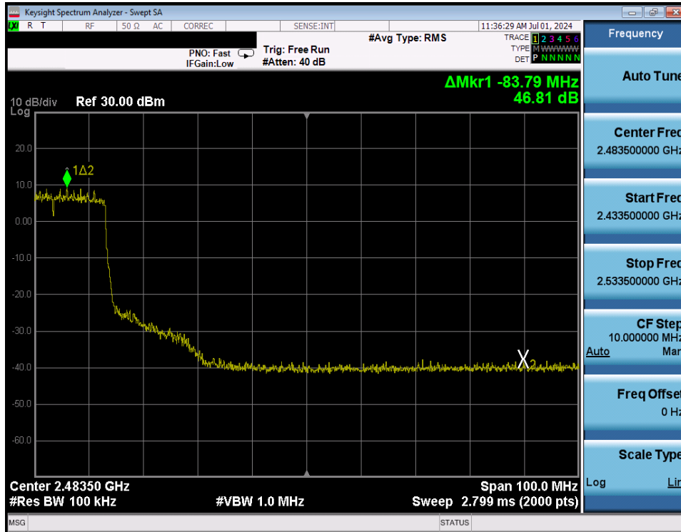
Plot 7-295. Band Edge Plot Antenna WF8 (802.11ax (SU - 2.4GHz) – Ch. 6 High) – MCS9
