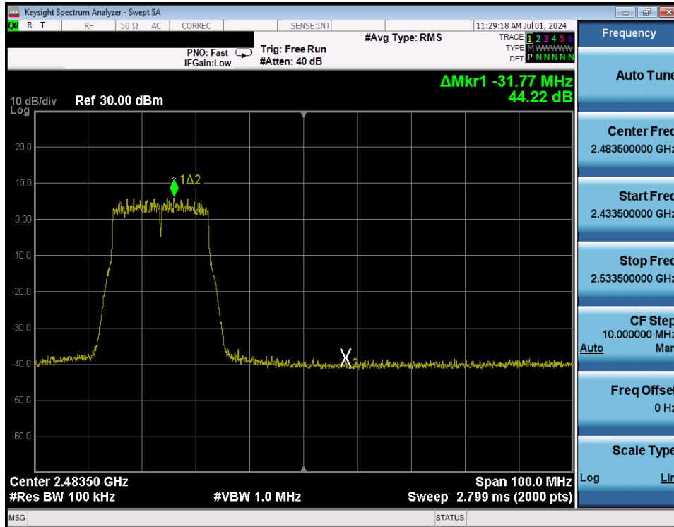
Plot 7-285. Band Edge Plot Antenna WF8 (802.11n (2.4GHz) – Ch. 10) – MCS7
