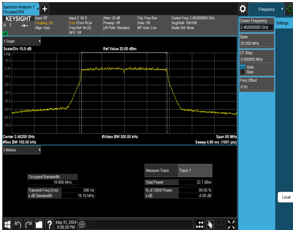
Plot 7-30. 6 dB BW and 99% OBW Plot Antenna WF8 (802.11ax (SU - 2.4GHz) – Ch. 11) – MCS9
