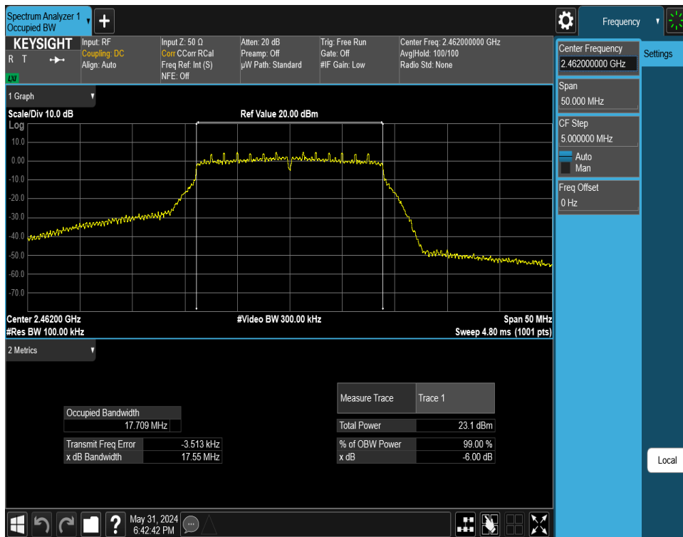
Plot 7-6. 6 dB BW and 99% OBW Plot Antenna WF8 (802.11n (2.4GHz) – Ch. 11) – MCS2
