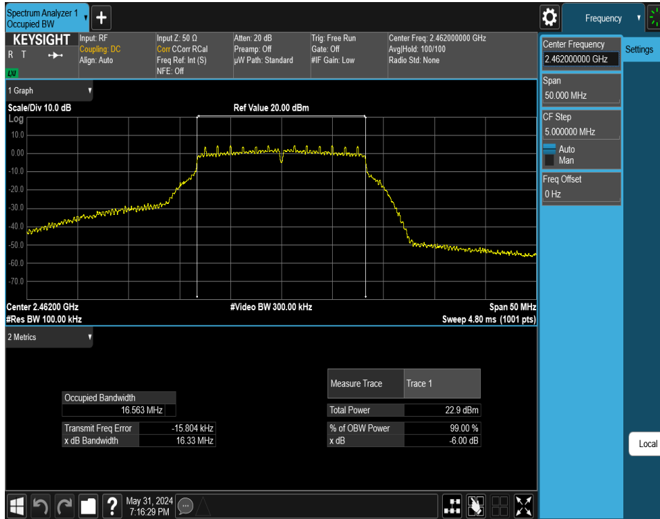
Plot 7-33. 6 dB BW and 99% OBW Plot Antenna WF7 (802.11g – Ch. 11) – 12Mbps
