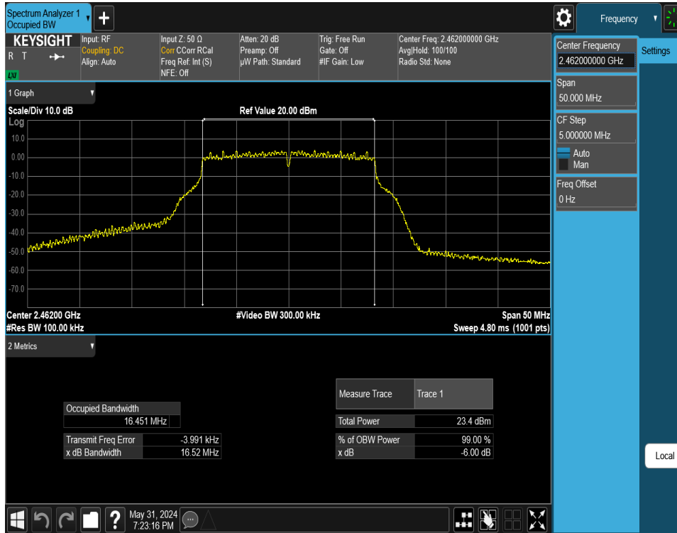
Plot 7-42. 6 dB BW and 99% OBW Plot Antenna WF7 (802.11g – Ch. 11) – 24Mbps
