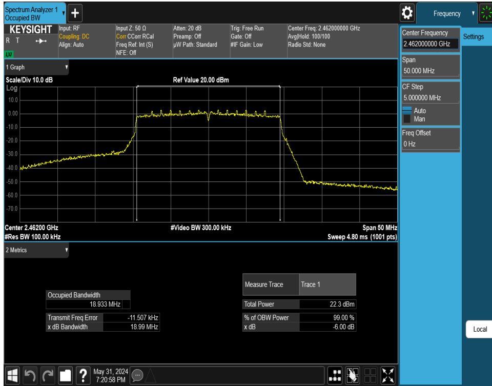
Plot 7-39. 6 dB BW and 99% OBW Plot Antenna WF7 (802.11ax (SU - 2.4GHz) – Ch. 11) – MCS2
