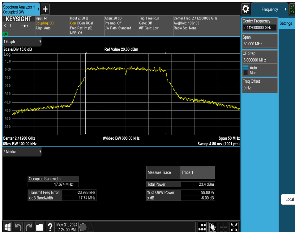
Plot 7-43. 6 dB BW and 99% OBW Plot Antenna WF7 (802.11n (2.4GHz) – Ch. 1) – MCS4
