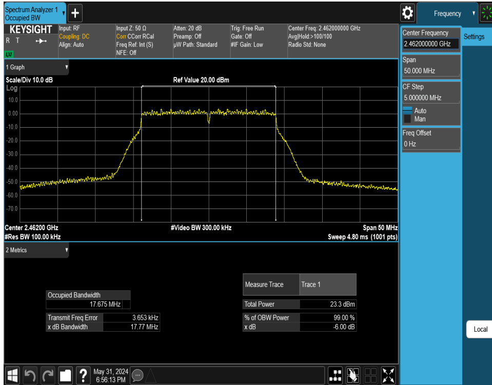
Plot 7-27. 6 dB BW and 99% OBW Plot Antenna WF8 (802.11n (2.4GHz) – Ch. 11) – MCS7
