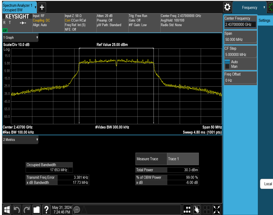
Plot 7-44. 6 dB BW and 99% OBW Plot Antenna WF7 (802.11n (2.4GHz) – Ch. 6) – MCS4
