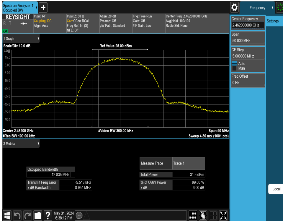
Plot 7-21. 6 dB BW and 99% OBW Plot Antenna WF8 (802.11b – Ch. 11) – 11Mbps
