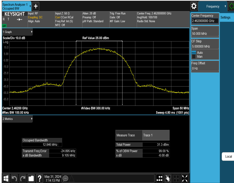
Plot 7-51. 6 dB BW and 99% OBW Plot Antenna WF7 (802.11b – Ch. 11) – 11Mbps
