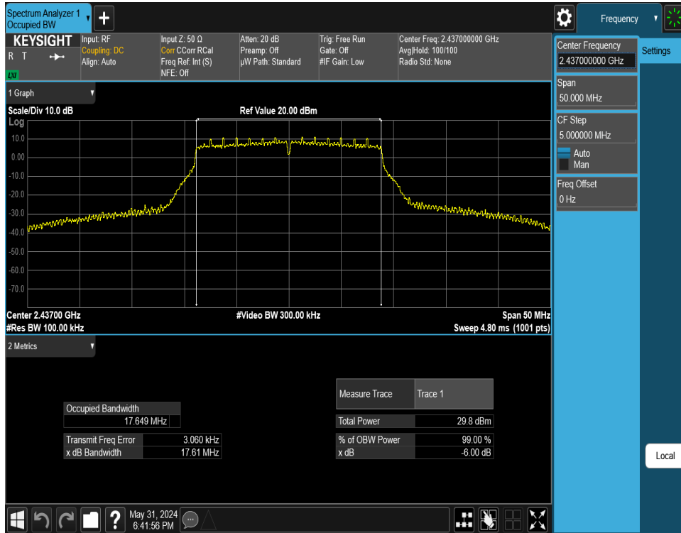
Plot 7-5. 6 dB BW and 99% OBW Plot Antenna WF8 (802.11n (2.4GHz) – Ch. 6) – MCS2
