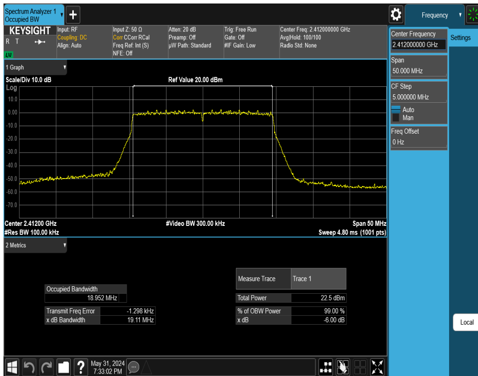
Plot 7-58. 6 dB BW and 99% OBW Plot Antenna WF7 (802.11ax (SU - 2.4GHz) – Ch. 1) – MCS9
