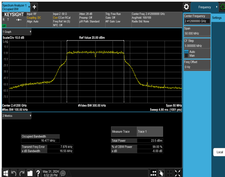
Plot 7-22. 6 dB BW and 99% OBW Plot Antenna WF8 (802.11g – Ch. 1) – 54Mbps
