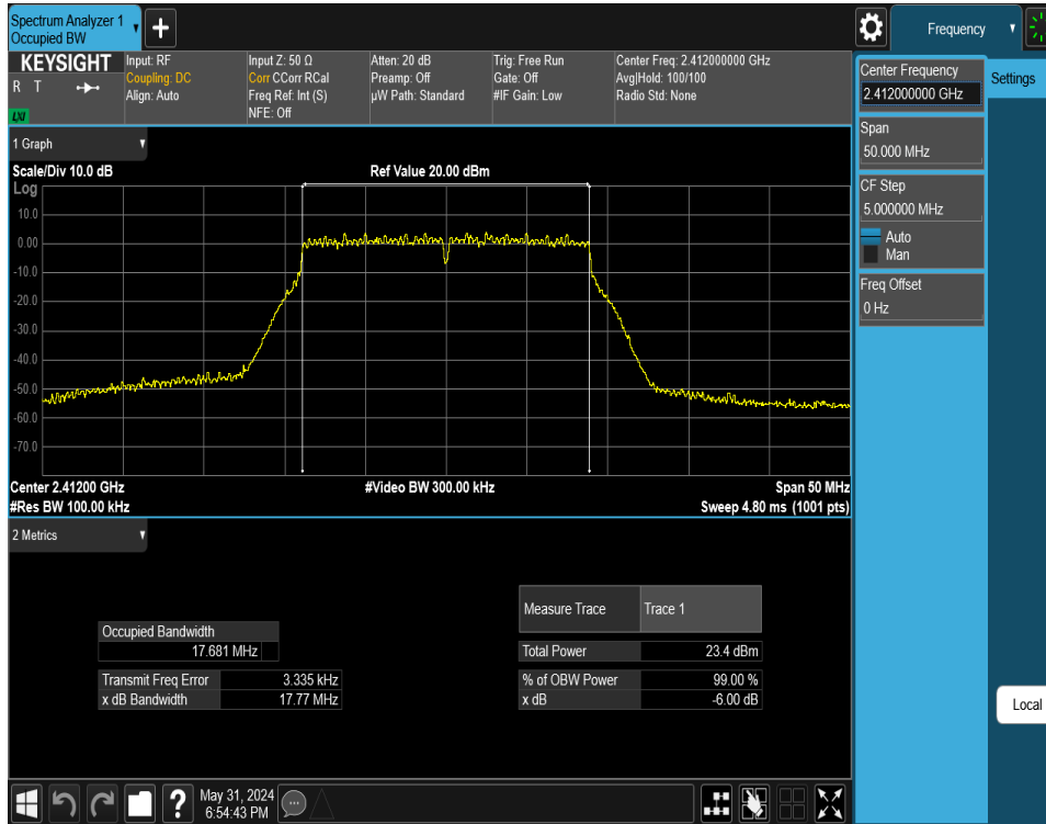
Plot 7-25. 6 dB BW and 99% OBW Plot Antenna WF8 (802.11n (2.4GHz) – Ch. 1) – MCS7
