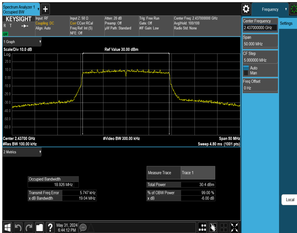
Plot 7-8. 6 dB BW and 99% OBW Plot Antenna WF8 (802.11ax (SU - 2.4GHz) – Ch. 6) – MCS2
