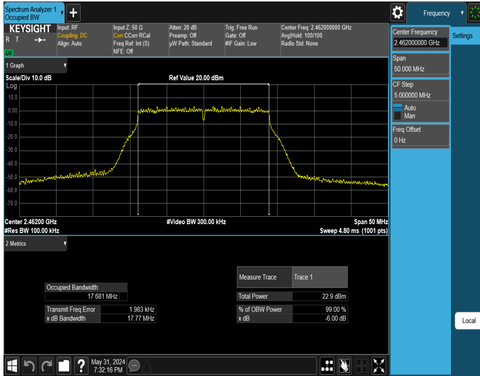
Plot 7-57. 6 dB BW and 99% OBW Plot Antenna WF7 (802.11n (2.4GHz) – Ch. 11) – MCS7
