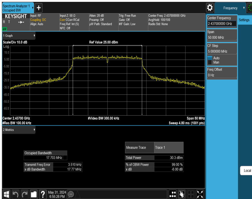
Plot 7-26. 6 dB BW and 99% OBW Plot Antenna WF8 (802.11n (2.4GHz) – Ch. 6) – MCS7
