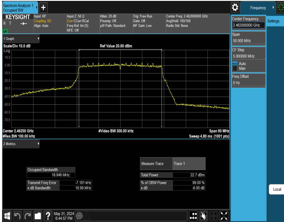
Plot 7-9. 6 dB BW and 99% OBW Plot Antenna WF8 (802.11ax (SU - 2.4GHz) – Ch. 11) – MCS2
