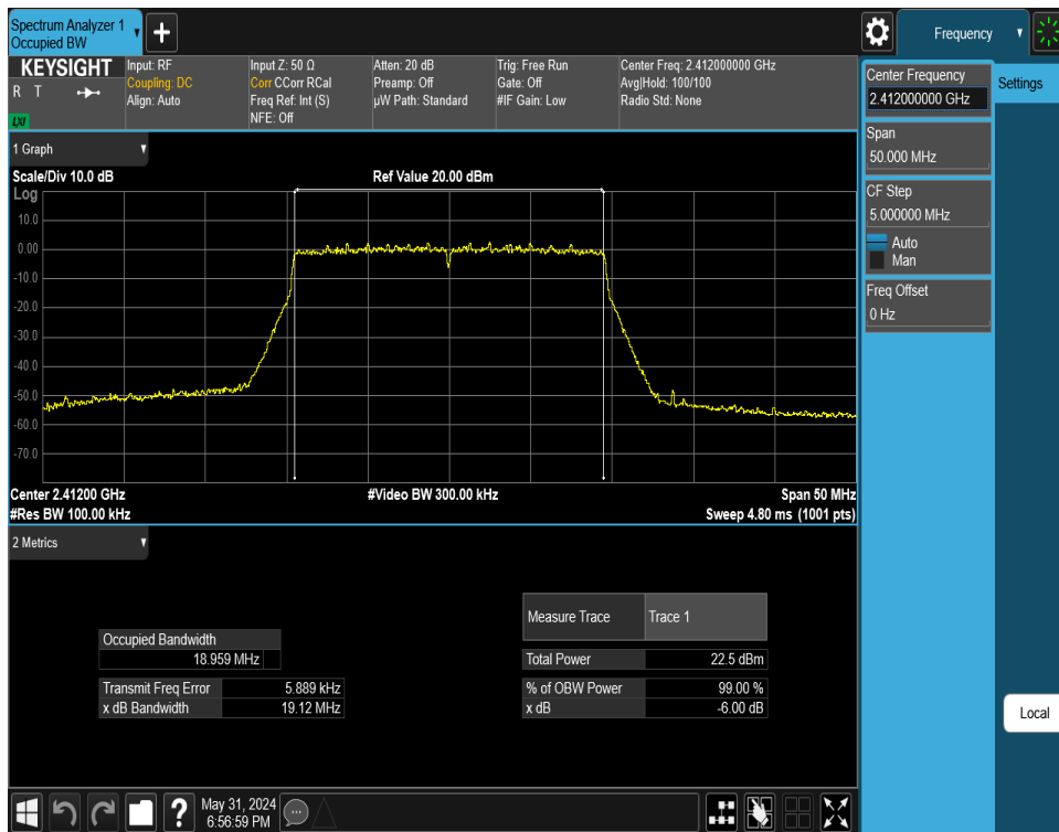
Plot 7-28. 6 dB BW and 99% OBW Plot Antenna WF8 (802.11ax (SU - 2.4GHz) – Ch. 1) – MCS9
