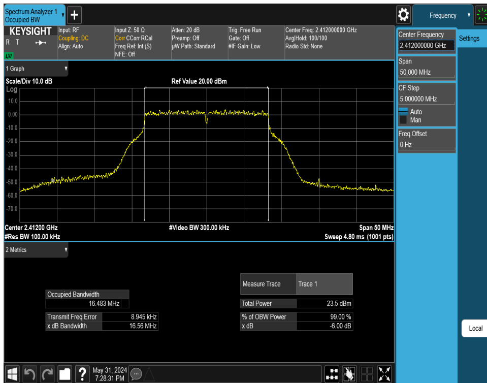
Plot 7-52. 6 dB BW and 99% OBW Plot Antenna WF7 (802.11g – Ch. 1) – 54Mbps
