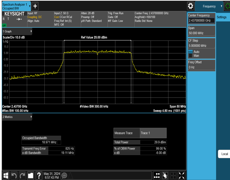
Plot 7-29. 6 dB BW and 99% OBW Plot Antenna WF8 (802.11ax (SU - 2.4GHz) – Ch. 6) – MCS9
