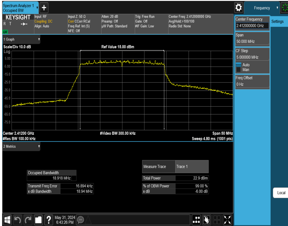
Plot 7-7. 6 dB BW and 99% OBW Plot Antenna WF8 (802.11ax (SU - 2.4GHz) – Ch. 1) – MCS2
