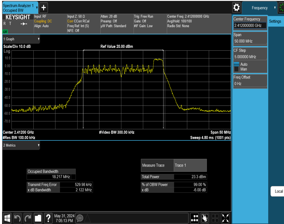
Plot 7-15. 6dB BW & 99% OBW Plot Antenna WF7 (802.11ax OFDMA – RU26 Index 8 – Ch. 1)
