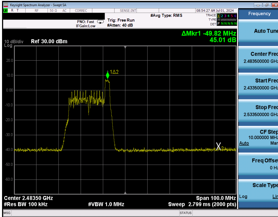
Plot 7-75. Band Edge Antenna WF8 (802.11ax OFDMA – RU26 Index 8 – Ch. 12)
