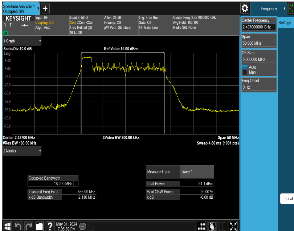
Plot 7-16. 6dB BW & 99% OBW Plot Antenna WF7 (802.11ax OFDMA – RU26 Index 0 – Ch. 6)
