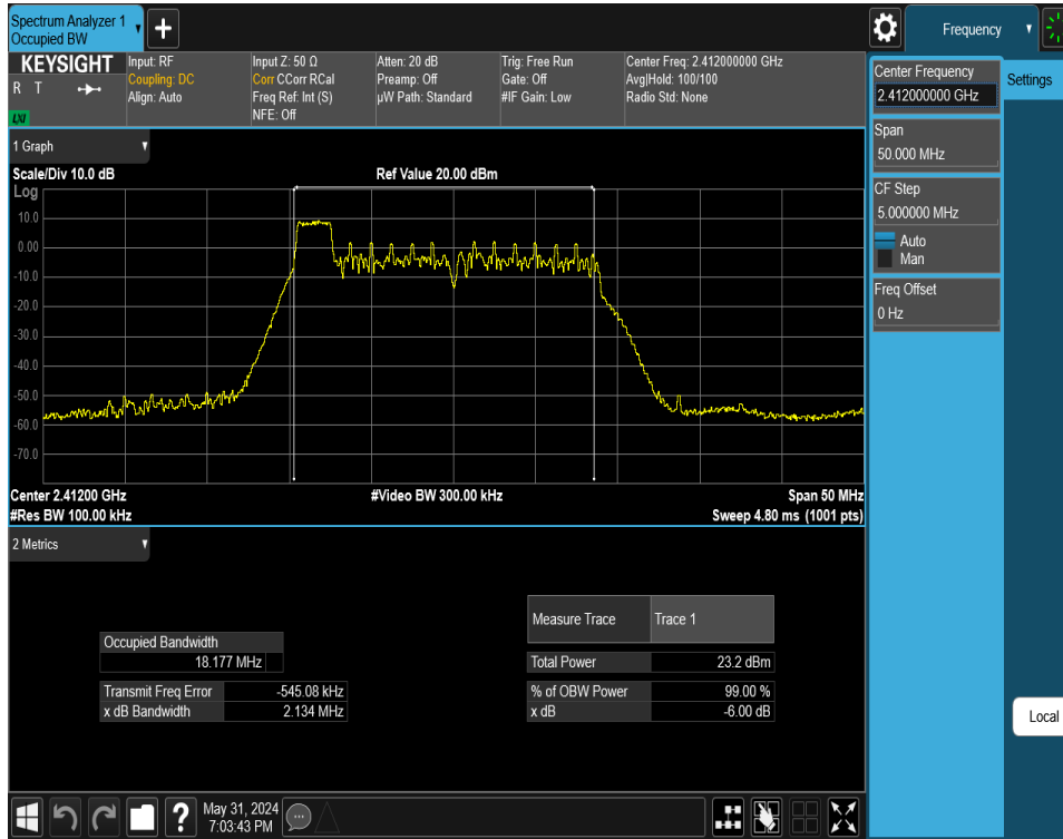
Plot 7-13. 6dB BW & 99% OBW Plot Antenna WF7 (802.11ax OFDMA – RU26 Index 0 – Ch. 1)
