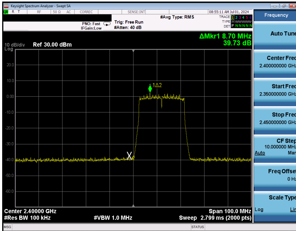
Plot 7-76. Band Edge Antenna WF8 (802.11ax OFDMA – RU242 – Ch. 1)
