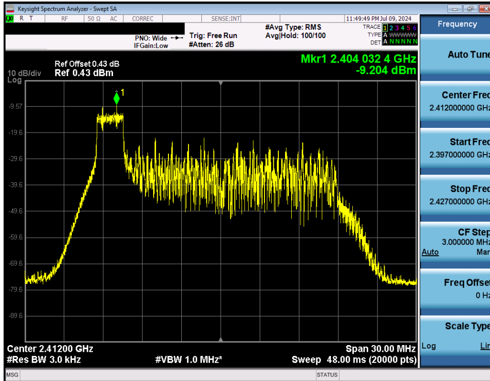
Plot 7-37. Power Spectral Density Plot Antenna WF7 (802.11ax OFDMA – RU26 Index 0 – Ch. 1)
