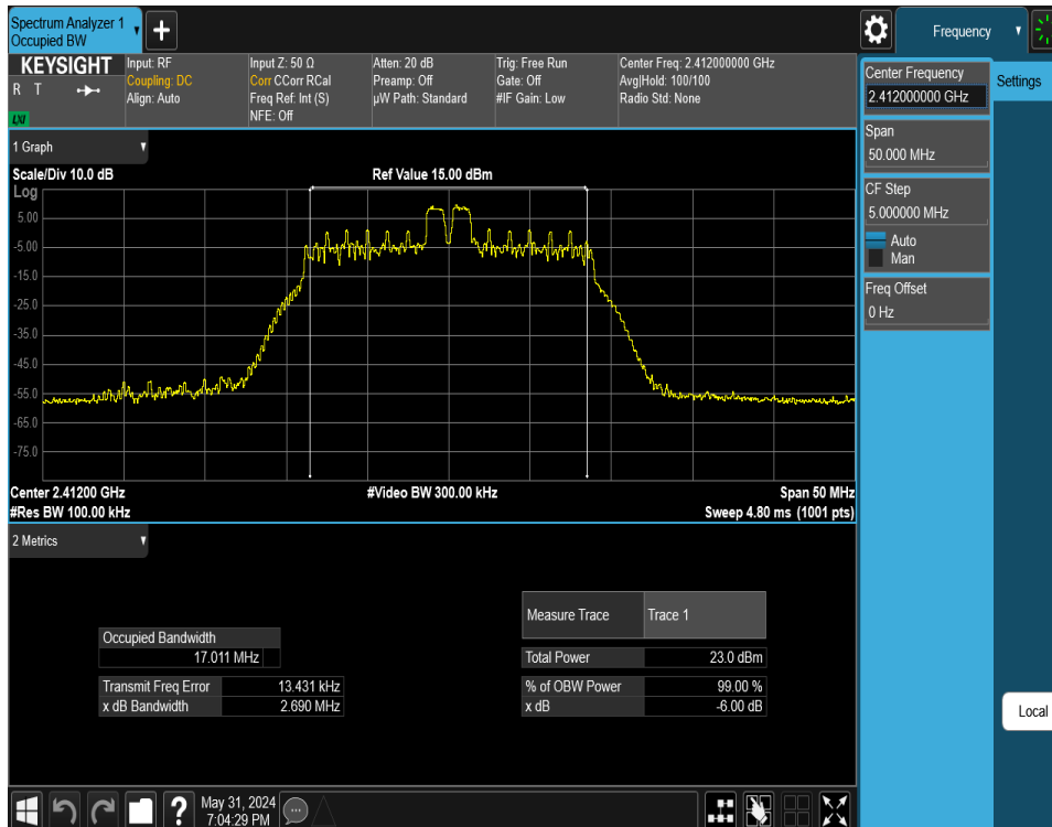
Plot 7-14. 6dB BW & 99% OBW Plot Antenna WF7 (802.11ax OFDMA – RU26 Index 4 – Ch. 1)
