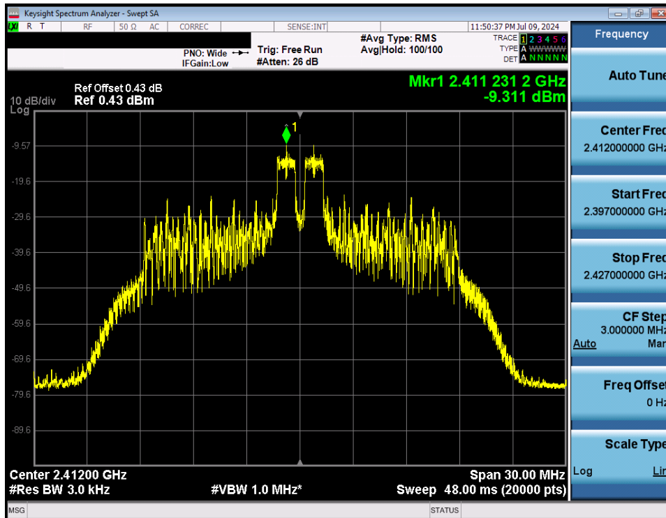
Plot 7-38. Power Spectral Density Plot Antenna WF7 (802.11ax OFDMA – RU26 Index 4 – Ch. 1)
