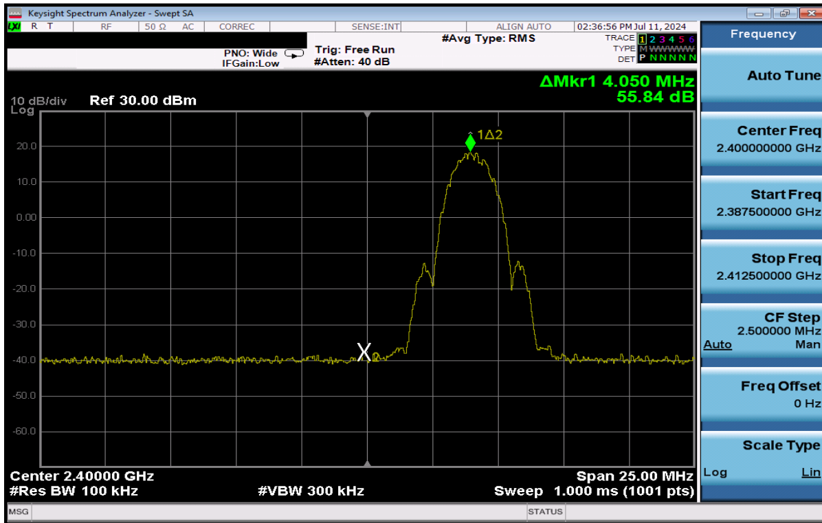
Plot 7-75. Band Edge Plot Antenna WF8 (Bluetooth (LE), 2Mbps, ePA – Ch. 1)
