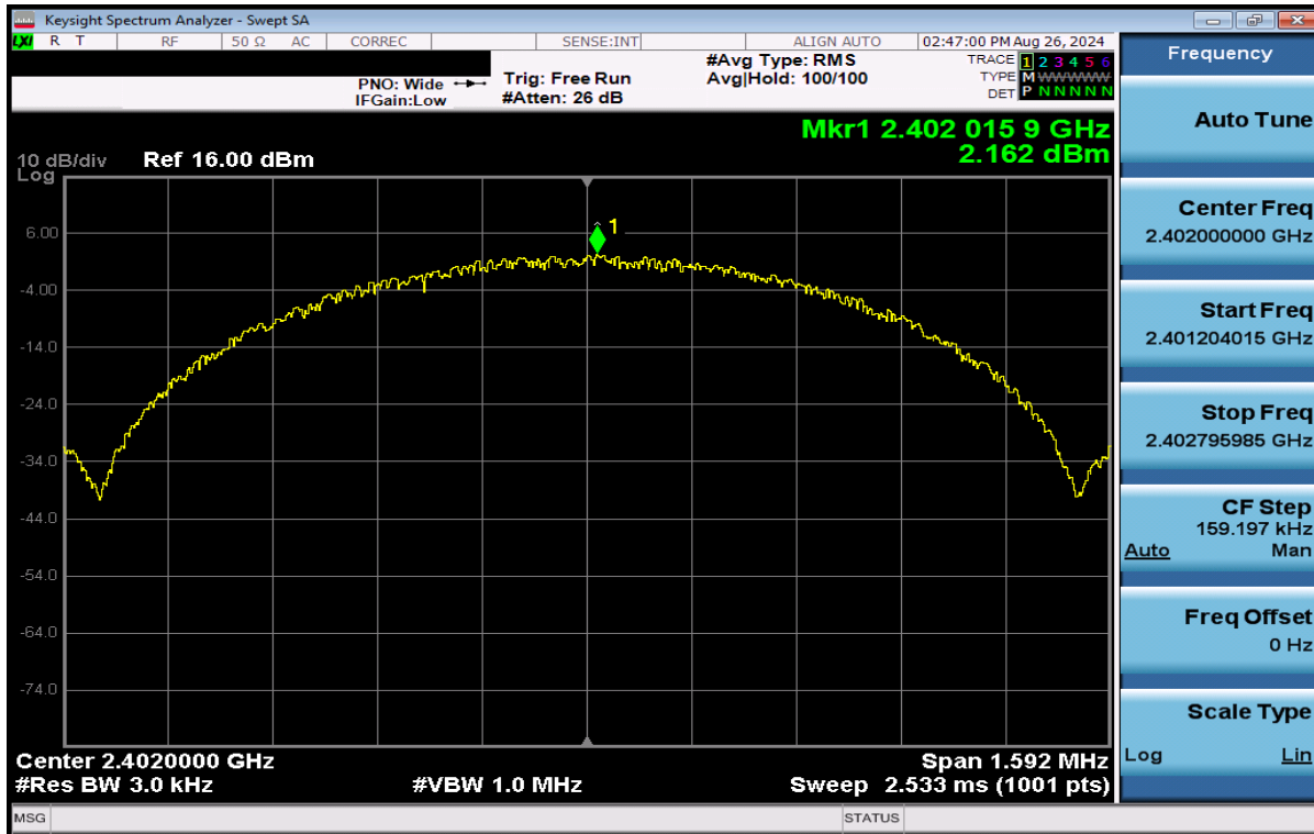
Plot 7-49. Power Spectral Density Plot Antenna WF8 (Bluetooth (LE), 1Mbps, ePA – Ch. 0)
