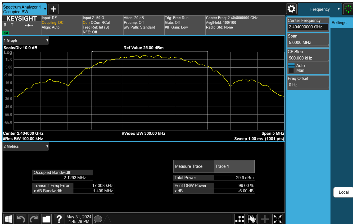
Plot 7-10. 6dB BW & 99% OBW Plot Antenna WF7 (Bluetooth (LE), 2Mbps, ePA – Ch. 1)
