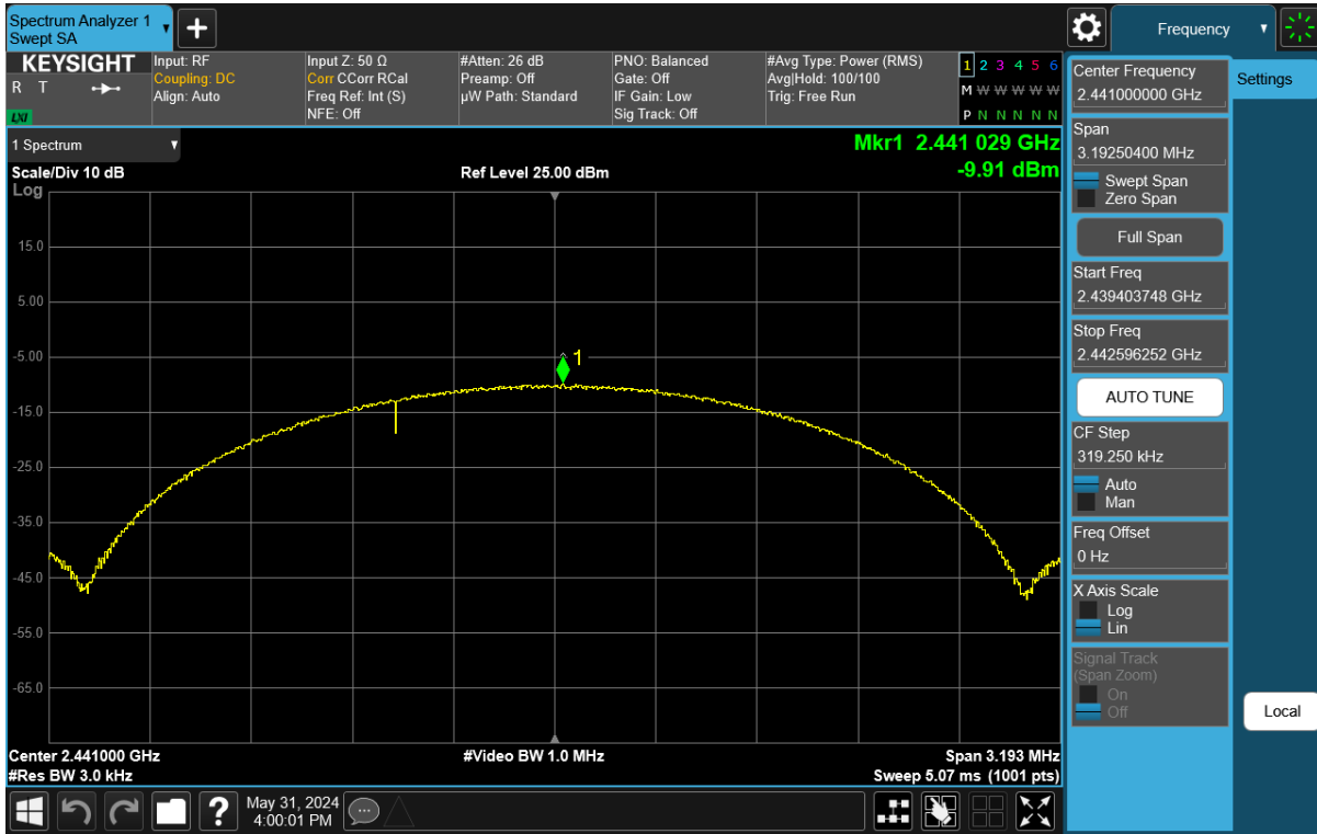
Plot 7-69. Power Spectral Density Plot Antenna WF8 (Bluetooth (LE), 2Mbps, iPA – Ch. 19)
