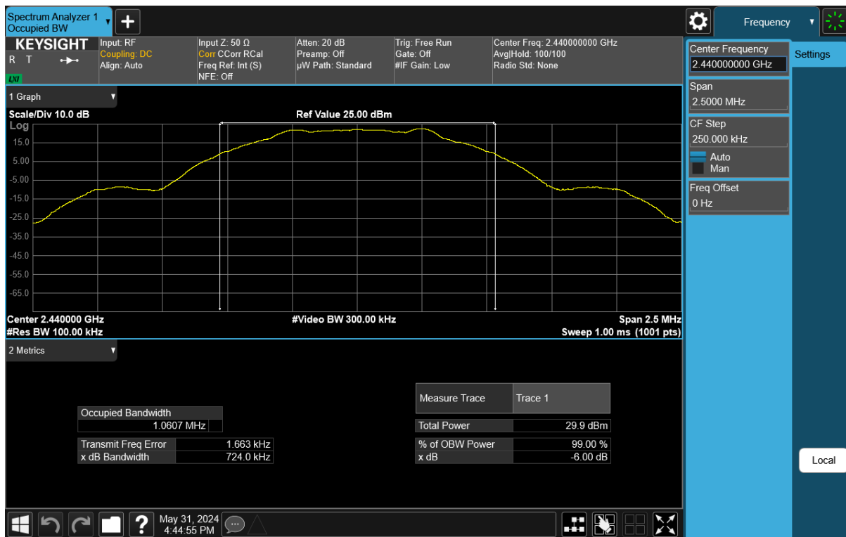
Plot 7-8. 6dB BW & 99% OBW Plot Antenna WF7 (Bluetooth (LE), 1Mbps, ePA – Ch. 19)
