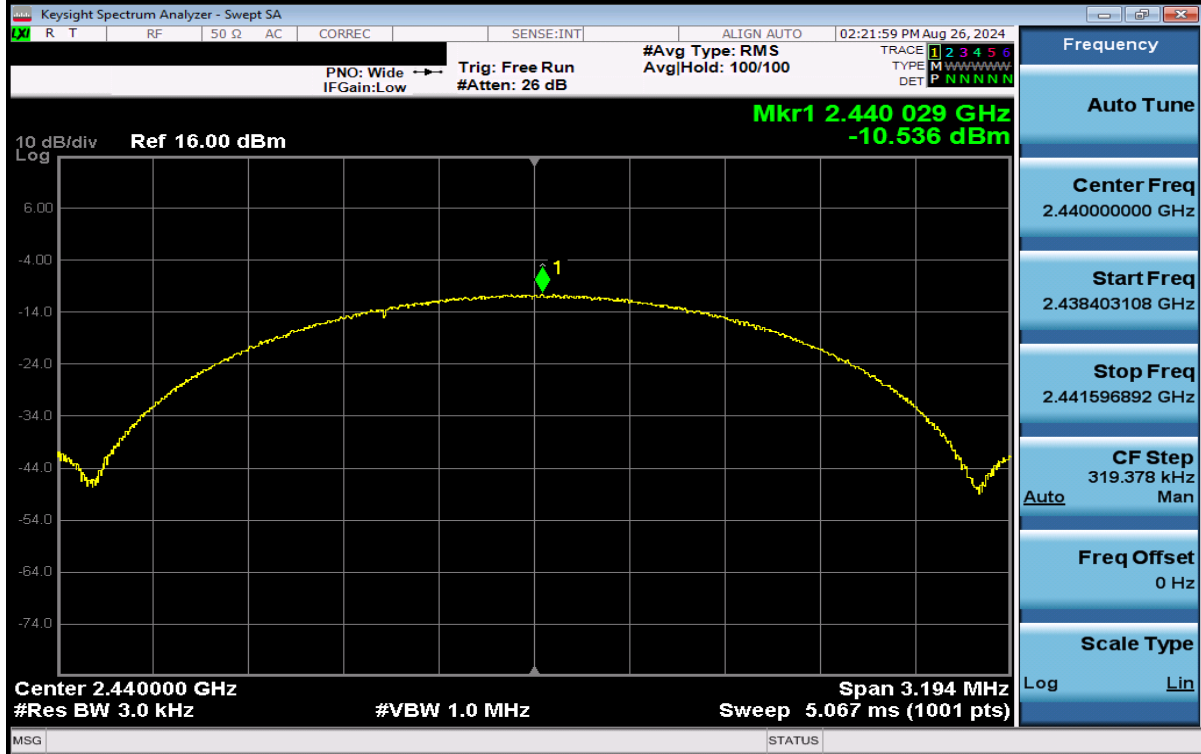
Plot 7-70. Power Spectral Density Plot Antenna WF7 (Bluetooth (LE), 2Mbps, iPA – Ch. 19)
