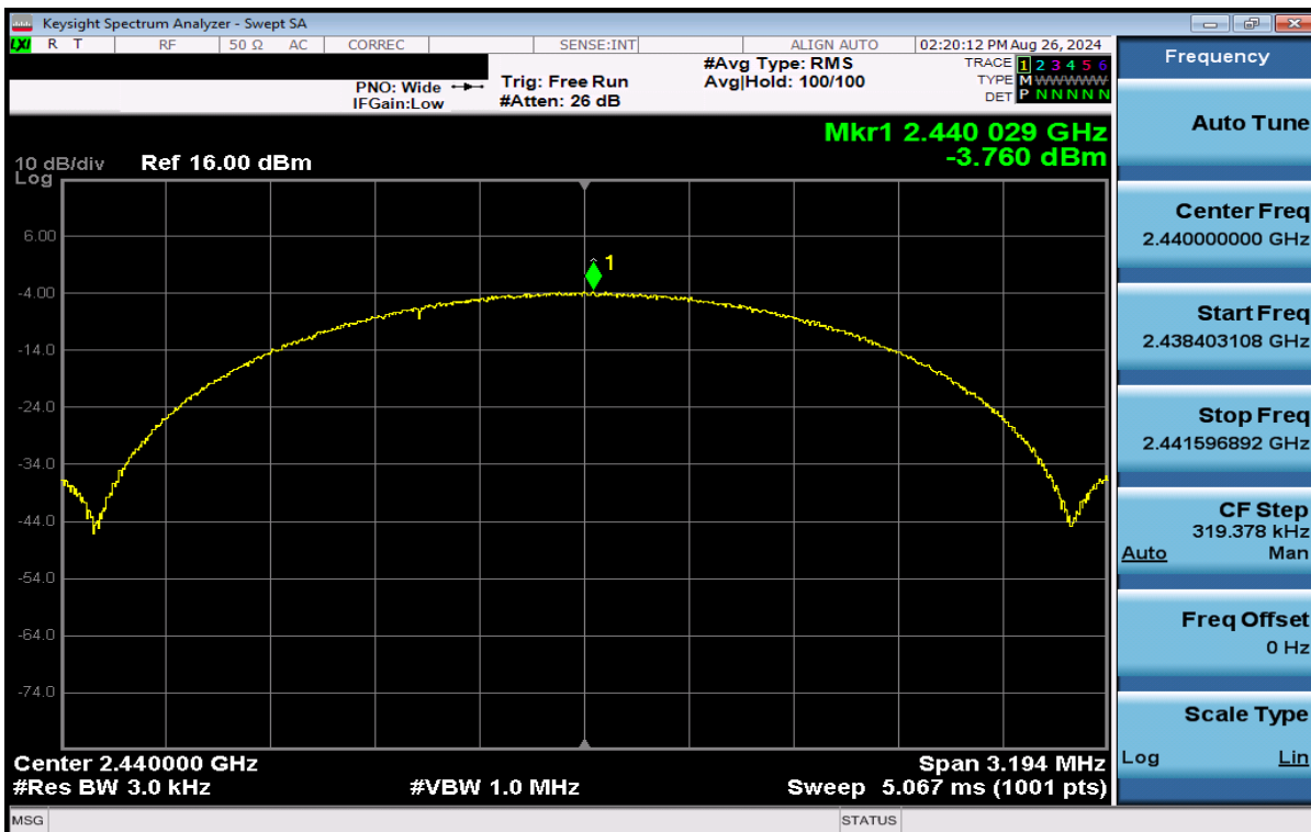
Plot 7-64. Power Spectral Density Plot Antenna WF7 (Bluetooth (LE), 2Mbps, ePA – Ch. 19)
