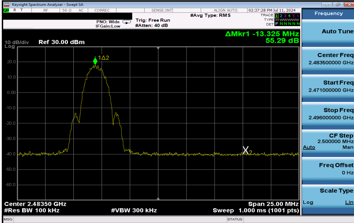
Plot 7-76. Band Edge Plot Antenna WF8 (Bluetooth (LE), 2Mbps, ePA – Ch. 38)
