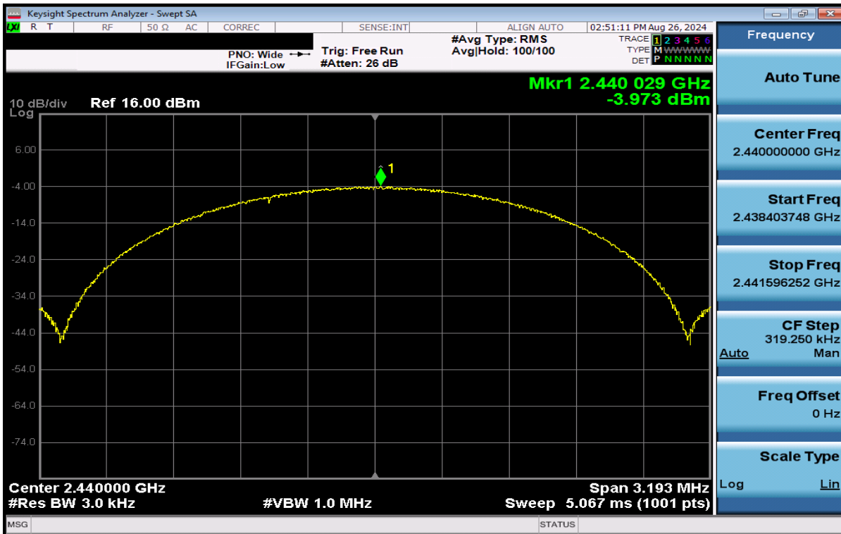
Plot 7-63. Power Spectral Density Plot Antenna WF8 (Bluetooth (LE), 2Mbps, ePA – Ch. 19)
