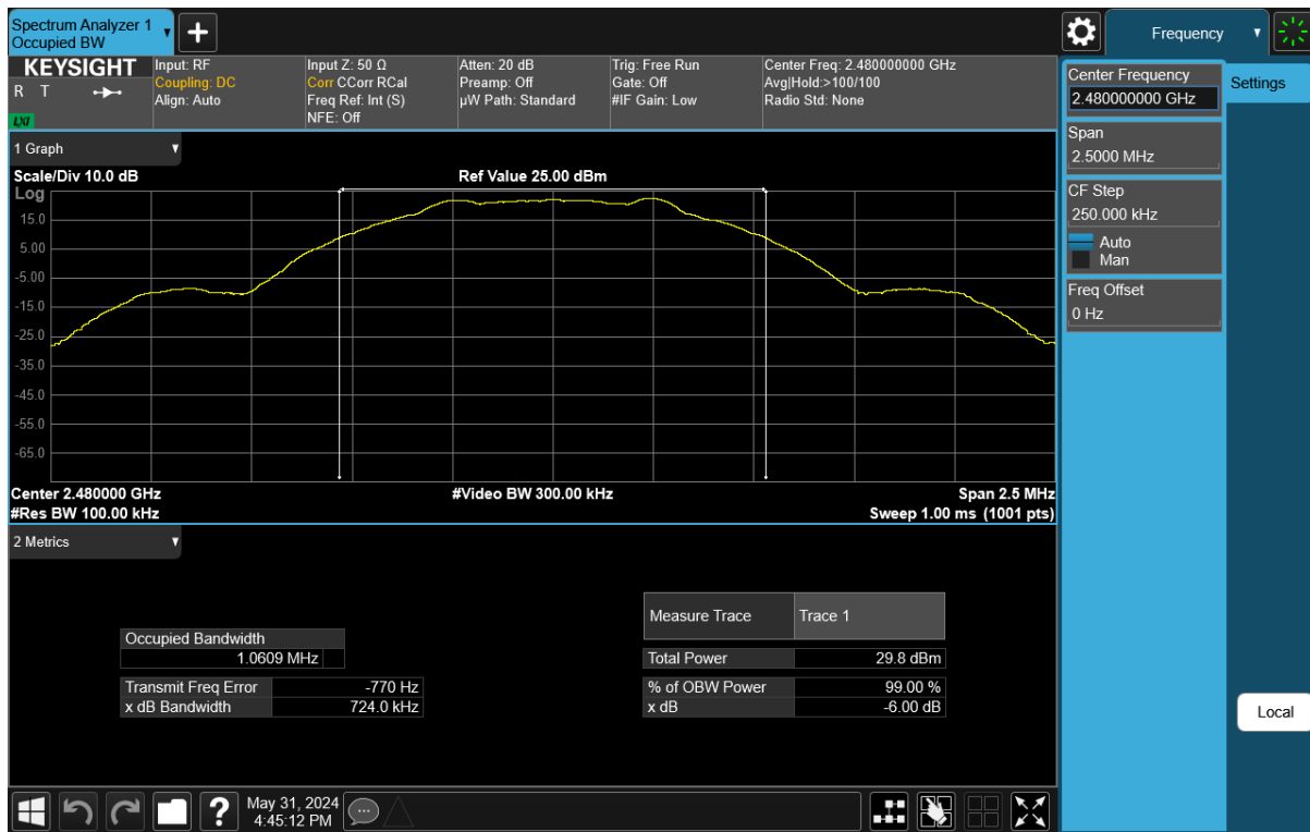
Plot 7-9. 6dB BW & 99% OBW Plot Antenna WF7 (Bluetooth (LE), 1Mbps, ePA – Ch. 39)
