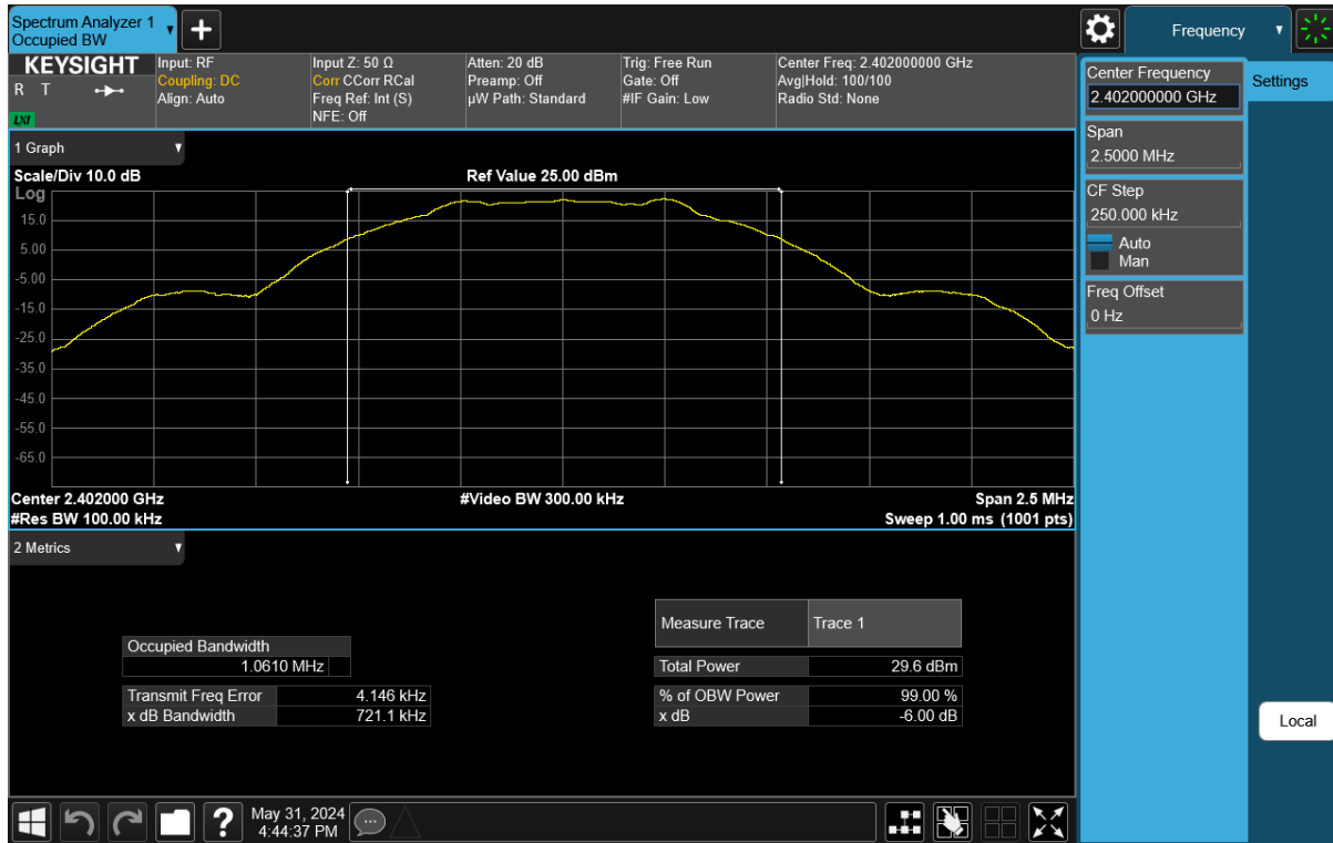
Plot 7-7. 6dB BW & 99% OBW Plot Antenna WF7 (Bluetooth (LE), 1Mbps, ePA – Ch. 0)
