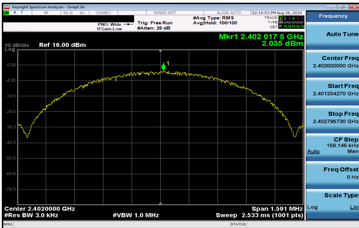
Plot 7-50. Power Spectral Density Plot Antenna WF7 (Bluetooth (LE), 1Mbps, ePA – Ch. 0)
