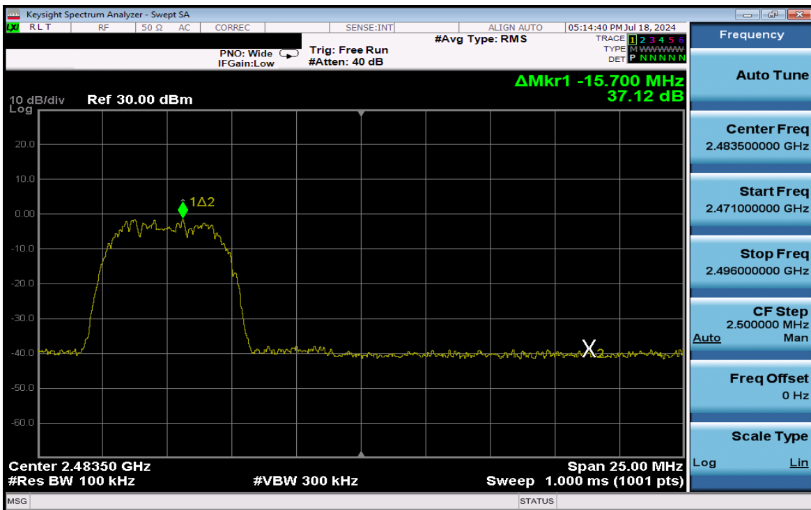
Plot 7-84. Band Edge Plot Antenna WF2 (Bluetooth (HDR8), iPA – Ch. 73)
