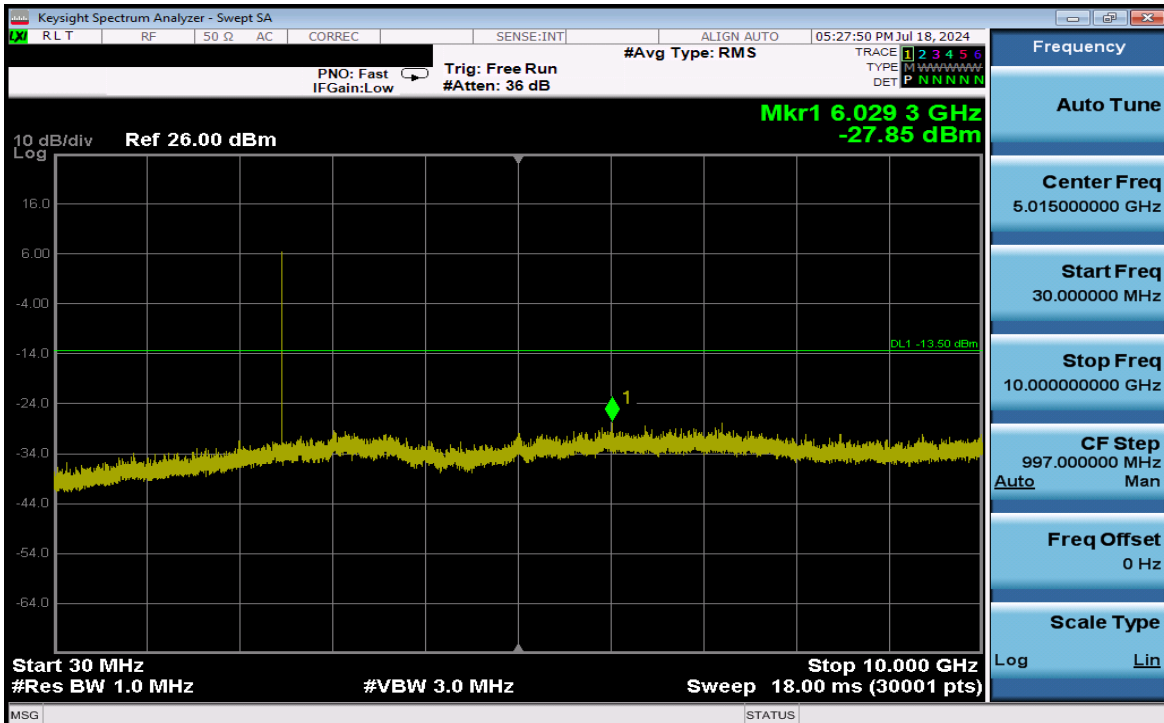
Plot 7-101. Conducted Spurious Plot Antenna WF2 (Bluetooth (HDR4), 4 Mbps, iPA – Ch. 73)
