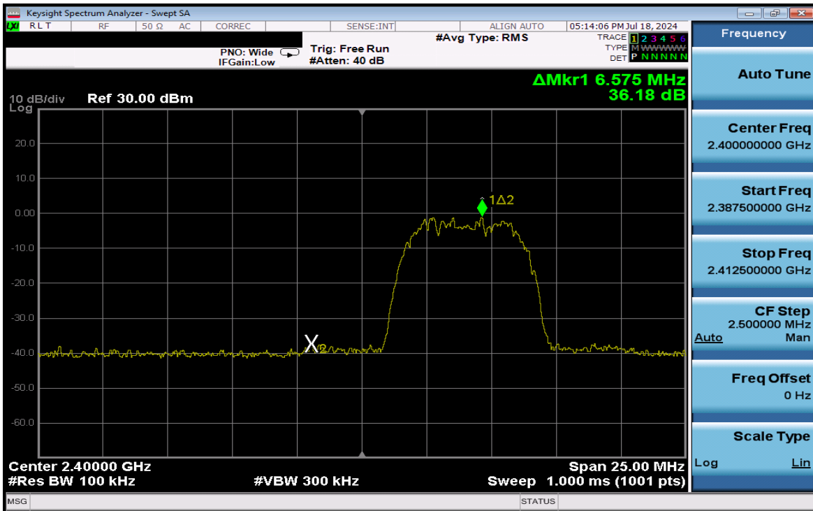
Plot 7-83. Band Edge Plot Antenna WF2 (Bluetooth (HDR8), iPA – Ch. 1)
