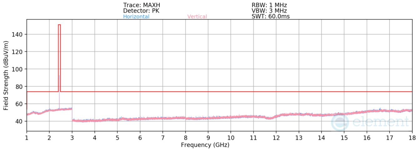
Plot 7-110. Radiated Spurious Emissions 1-18GHz Antenna WF2 (4Mbps, HDR4, iPA – Ch. 38)
