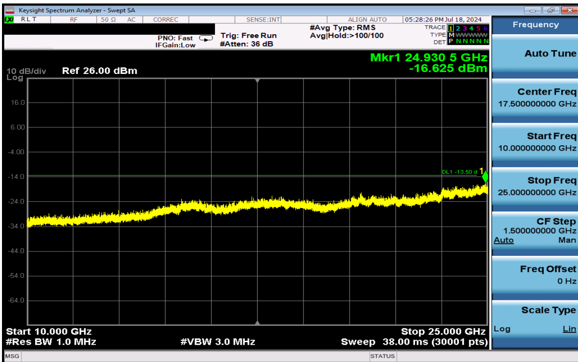
Plot 7-102. Conducted Spurious Plot Antenna WF2 (Bluetooth (HDR4), 4 Mbps, iPA – Ch. 73)
