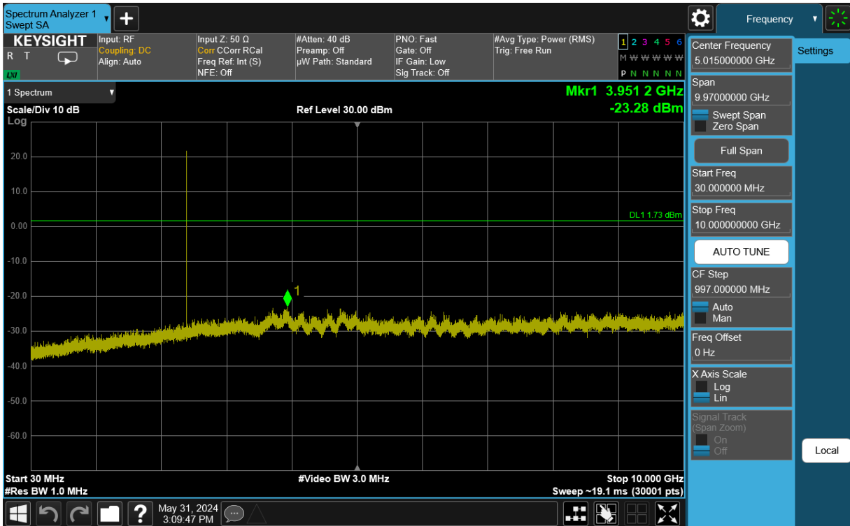
Plot 7-37. Conducted Spurious Antenna WF7 (802.15.4, ePA – Ch. 11)
