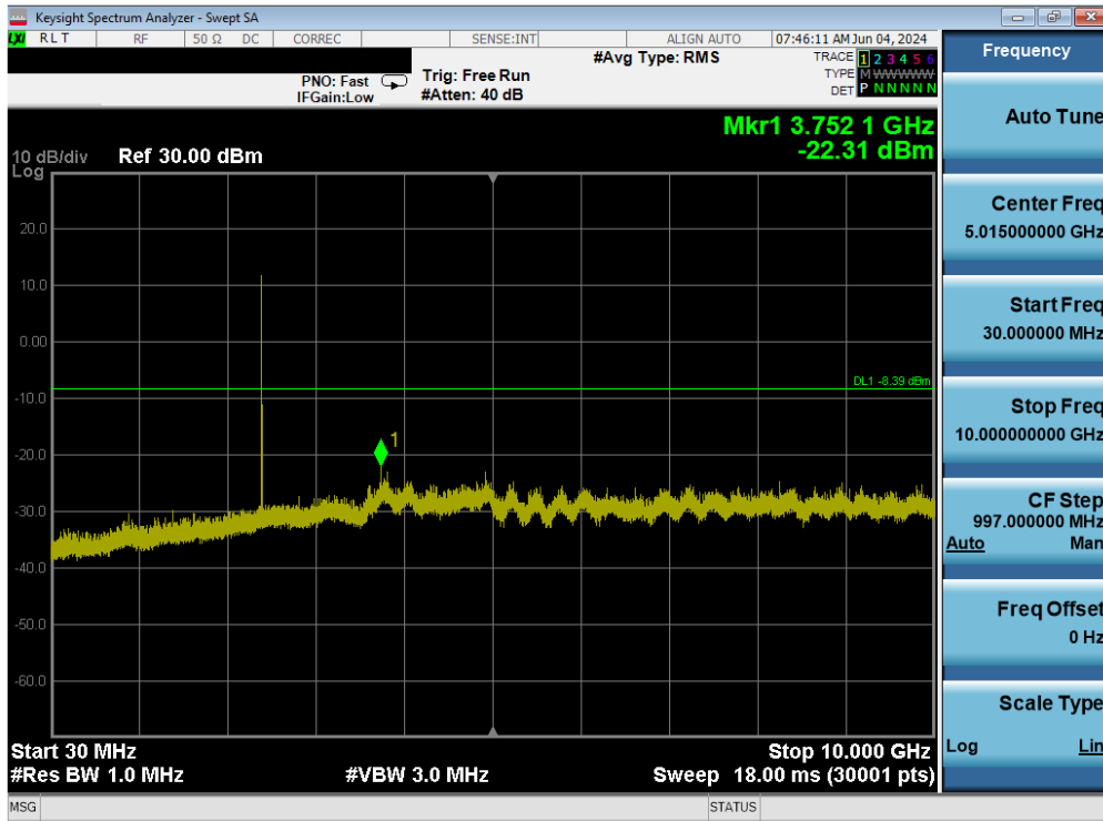
Plot 7-43. Conducted Spurious Antenna WF2 (802.15.4, iPA – Ch. 11)
