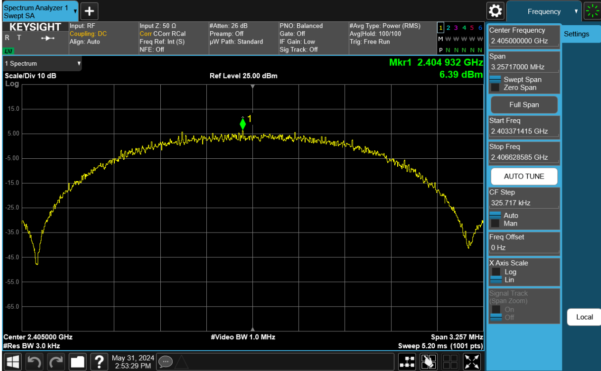
Plot 7-10. Power Spectral Density Antenna WF8 (802.15.4, ePA – Ch. 11)
