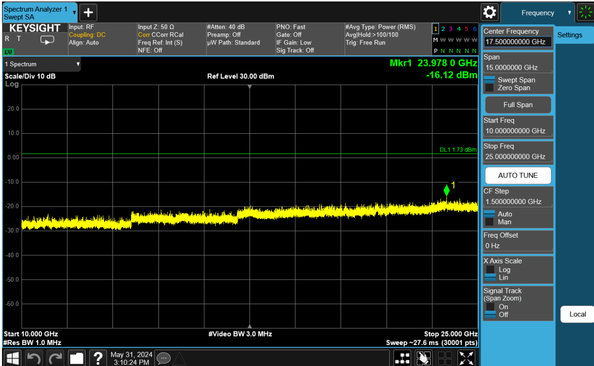
Plot 7-38. Conducted Spurious Antenna WF7 (802.15.4, ePA – Ch. 11)
