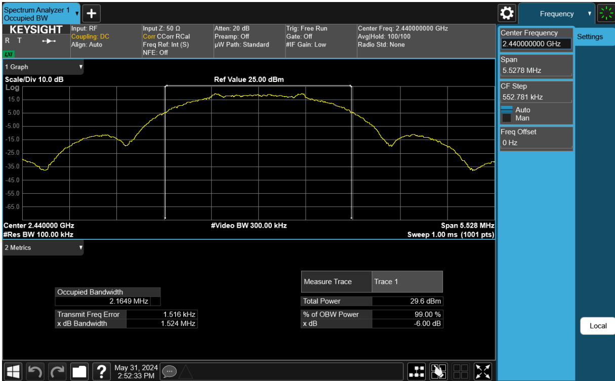
Plot 7-2. 6dB BW & 99% OBW Antenna WF8 (802.15.4, Ch. 18)
