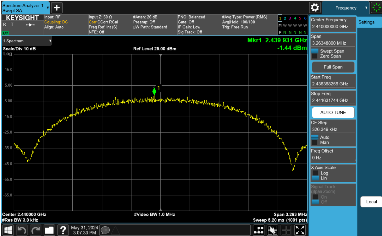
Plot 7-20. Power Spectral Density Antenna WF7 (802.15.4, iPA - Ch. 18)
