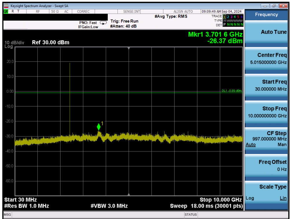
Plot 7-33. Conducted Spurious Antenna WF8 (802.15.4, ePA – Ch. 18)
