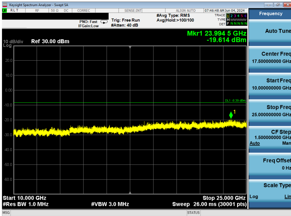
Plot 7-44. Conducted Spurious Antenna WF2 (802.15.4, iPA – Ch. 11)
