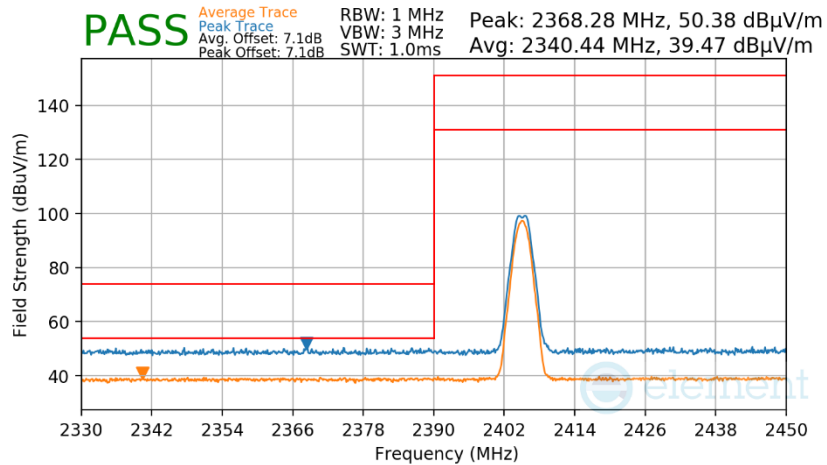
Plot 7-63. Radiated Restricted Lower Band Edge Measurement Antenna WF2
