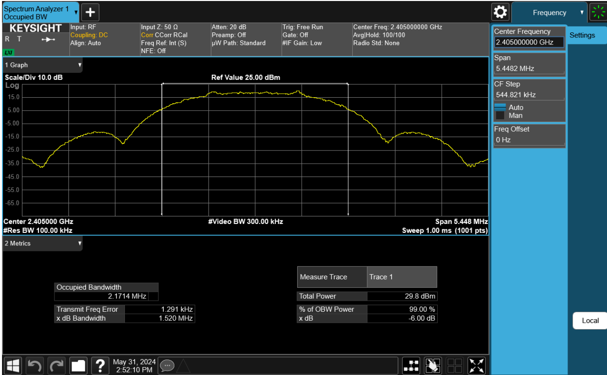
Plot 7-1. 6dB BW & 99% OBW Antenna WF8 (802.15.4, Ch. 11)
