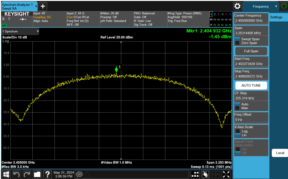
Plot 7-19. Power Spectral Density Antenna WF7 (802.15.4, iPA – Ch. 11)
