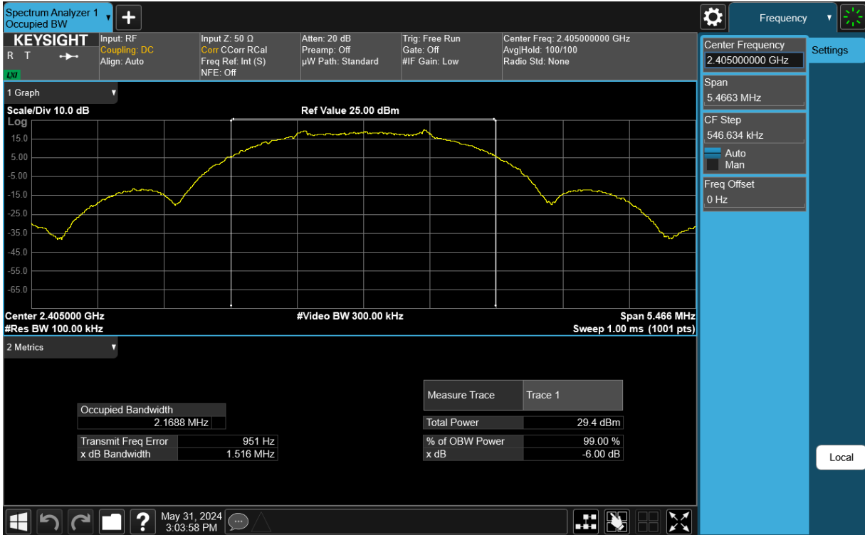
Plot 7-4. 6dB BW & 99% OBW Antenna WF7 (802.15.4, Ch. 11)
