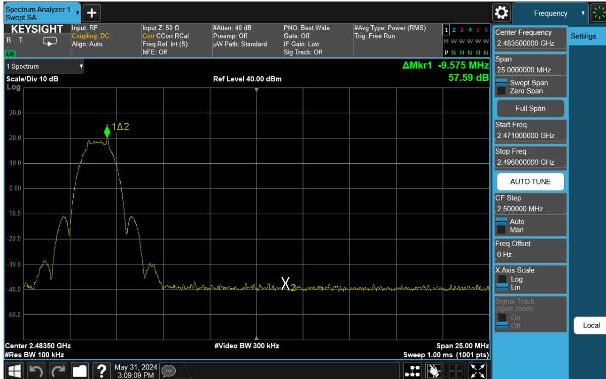
Plot 7-28. Band Edge Antenna WF7 (802.15.4, ePA – Ch. 25)
