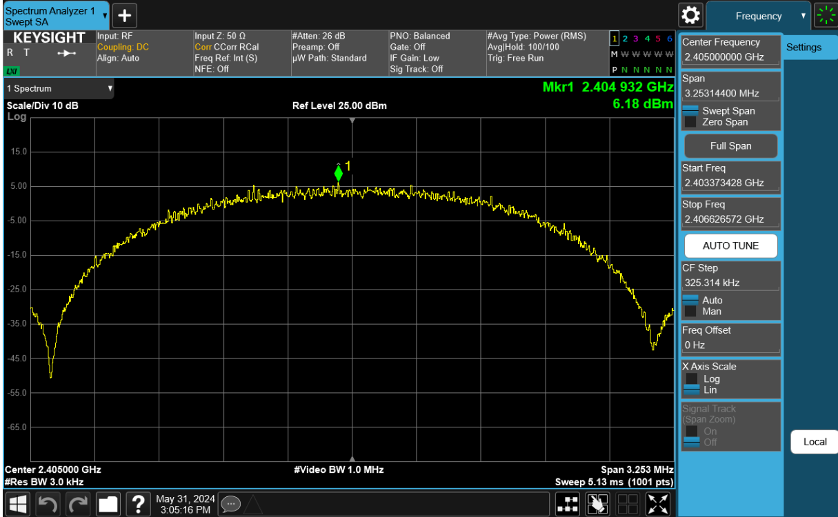
Plot 7-16. Power Spectral Density Antenna WF7 (802.15.4, ePA – Ch. 11)
