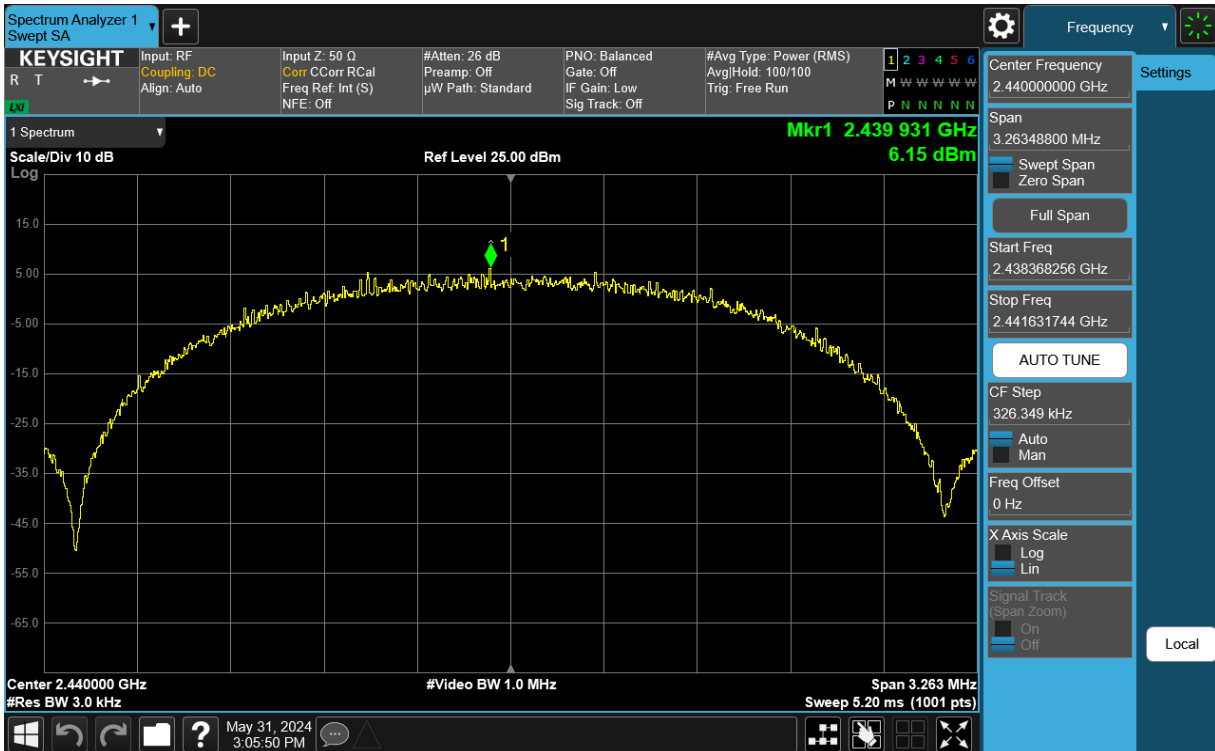
Plot 7-17. Power Spectral Density Antenna WF7 (802.15.4, ePA – Ch. 18)
