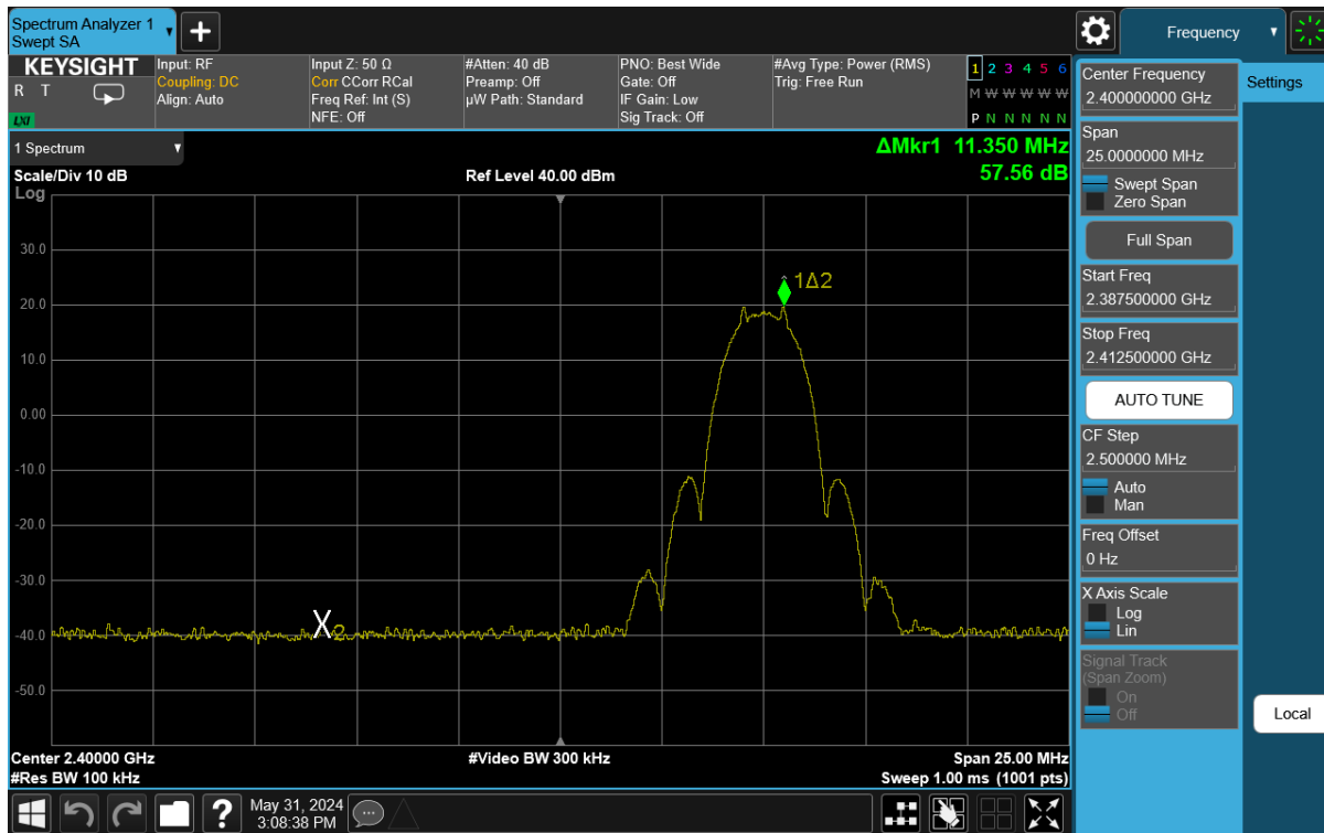
Plot 7-27. Band Edge Antenna WF7 (802.15.4, ePA – Ch. 11)
