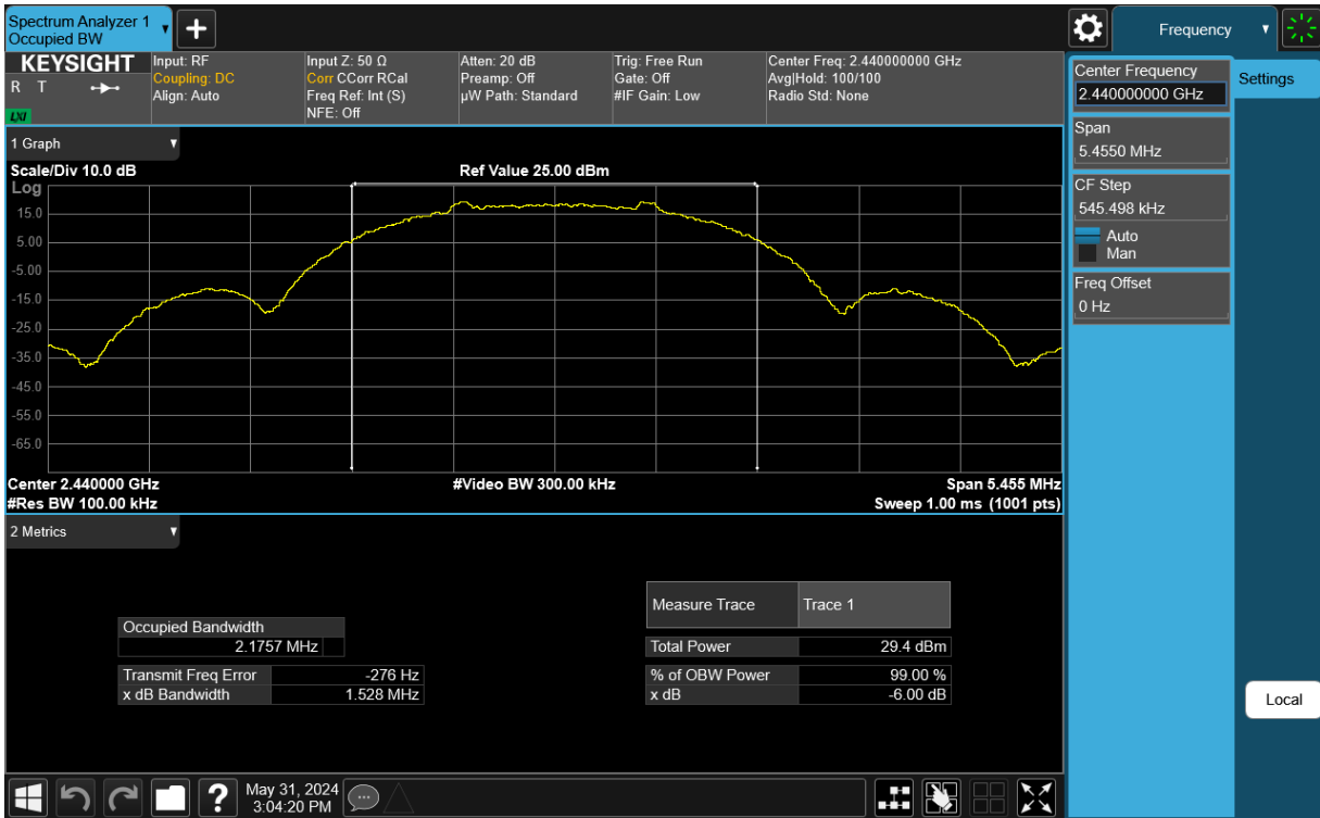
Plot 7-5. 6dB BW & 99% OBW Antenna WF7 (802.15.4, Ch. 18)
