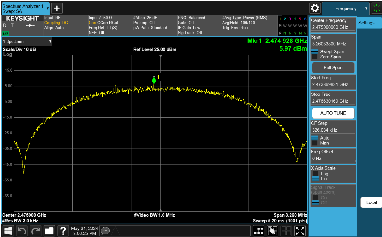
Plot 7-18. Power Spectral Density Antenna WF7 (802.15.4, ePA – Ch. 25)
