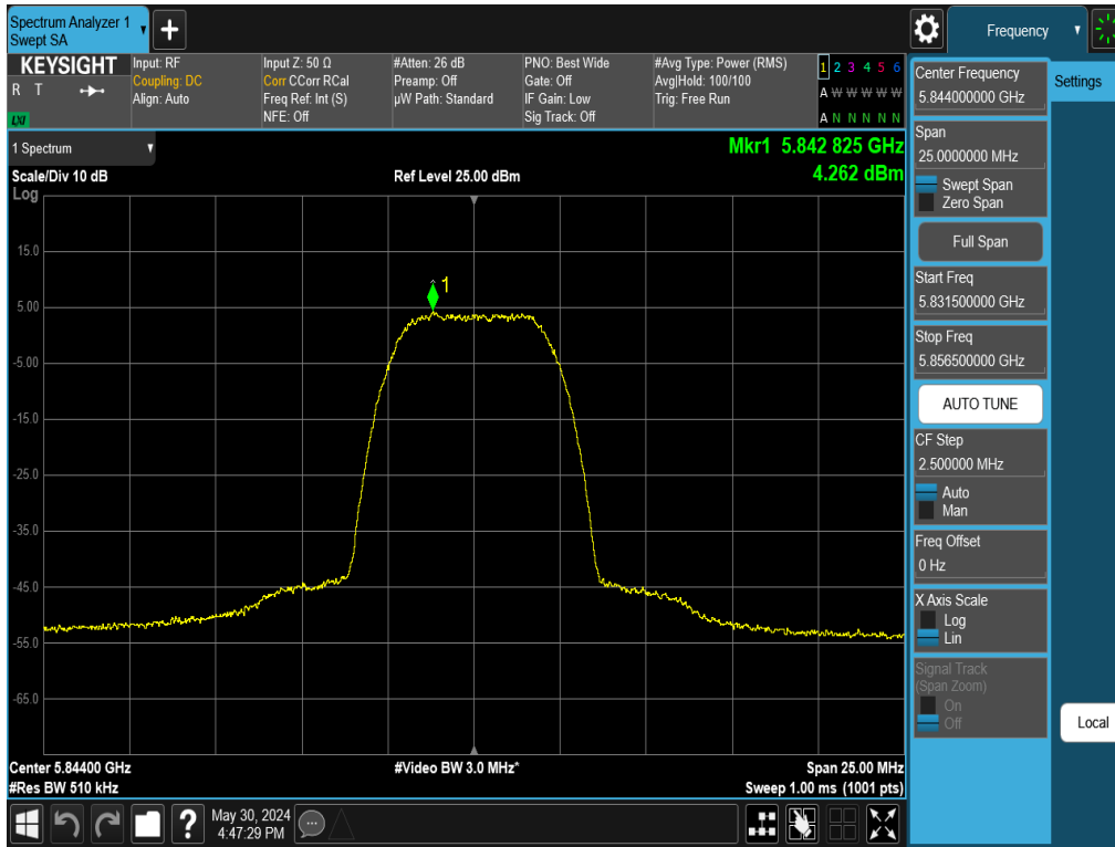
Plot 7-69. PSD Antenna WF5T (NB UNII HDR8, ePA – 5844MHz)
