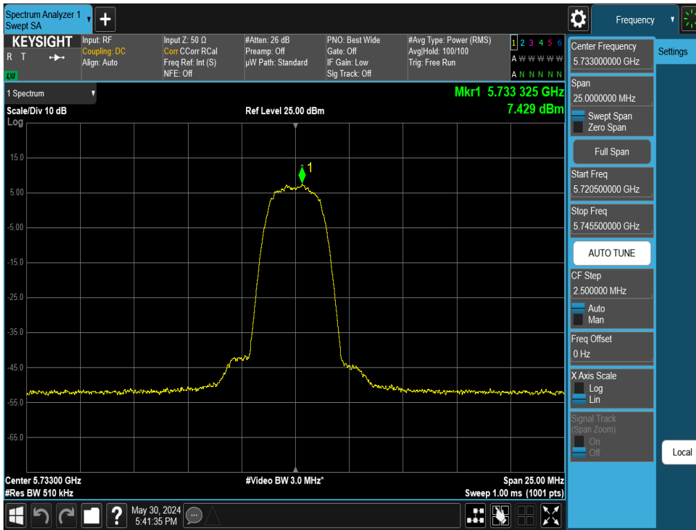
Plot 7-97. PSD Antenna WF2 (NB UNII HDR4, ePA – 5733MHz)
