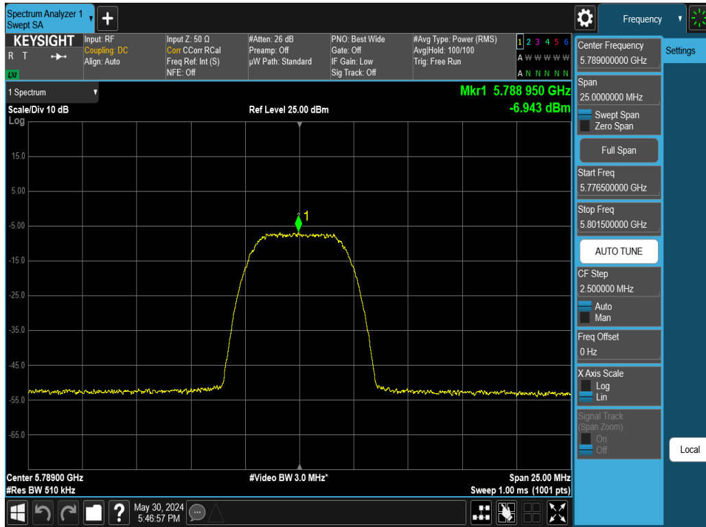
Plot 7-107. PSD Antenna WF2 (NB UNII HDR8, iPA – 5789MHz)
