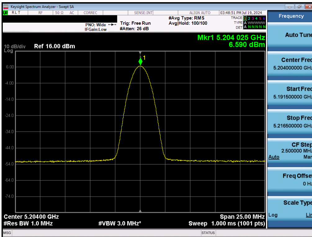
Plot 7-112. PSD TxBF Antenna WF2 (NB UNII BDR, ePA - 5204MHz)
