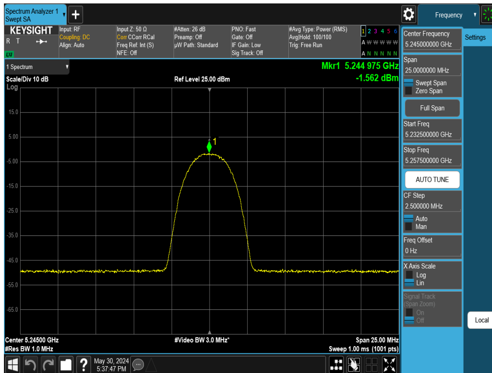
Plot 7-84. PSD Antenna WF2 (NB UNII HDR4, iPA– 5245MHz)
