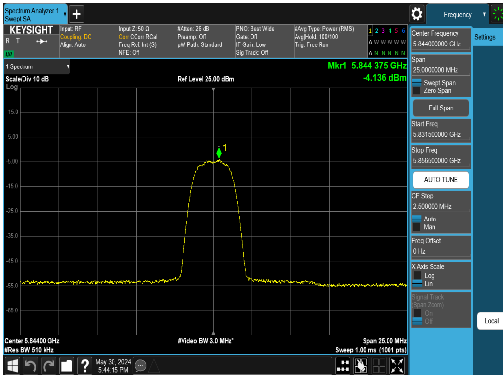
Plot 7-102. PSD Antenna WF2 (NB UNII HDR4, iPA – 5844MHz)
