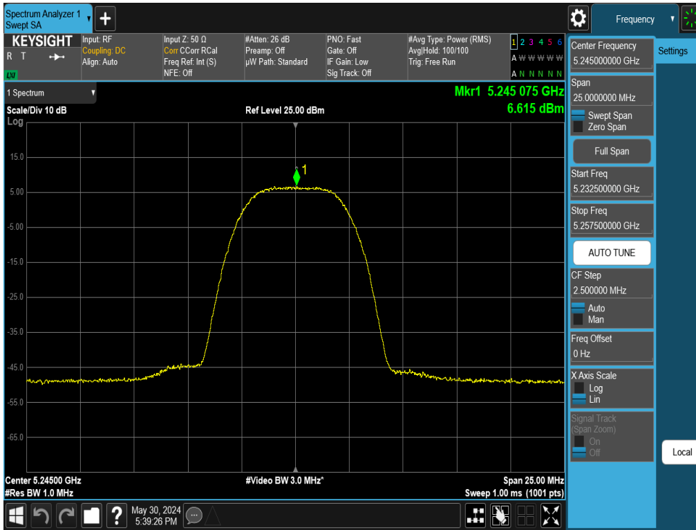
Plot 7-87. PSD Antenna WF2 (NB UNII HDR8, ePA- 5245MHz)
