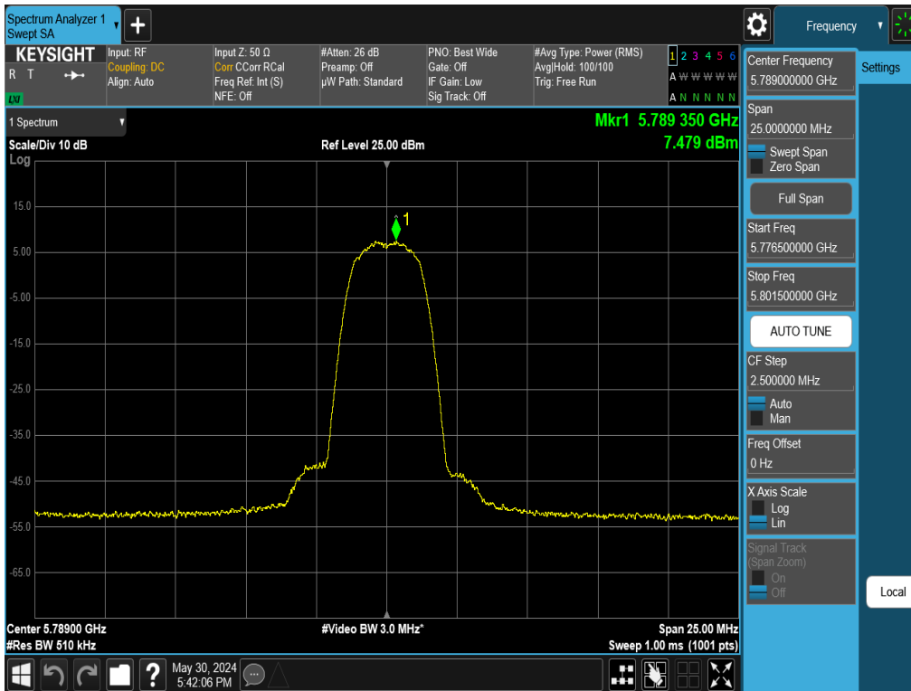
Plot 7-98. PSD Antenna WF2 (NB UNII HDR4, ePA – 5789MHz)
