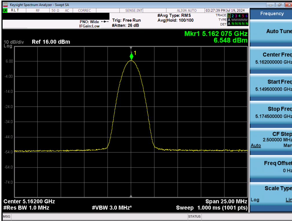
7-109. PSD TxBF Antenna WF5T (NB UNII BDR, ePA – 5162MHz)
