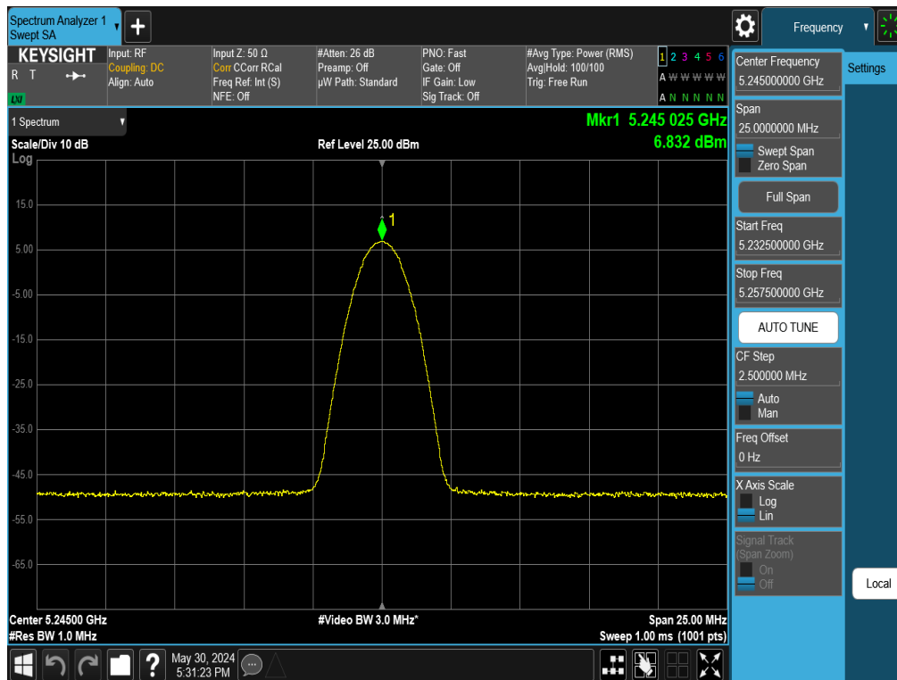
Plot 7-78. PSD Antenna WF2 (NB UNII BDR, iPA– 5245MHz)
