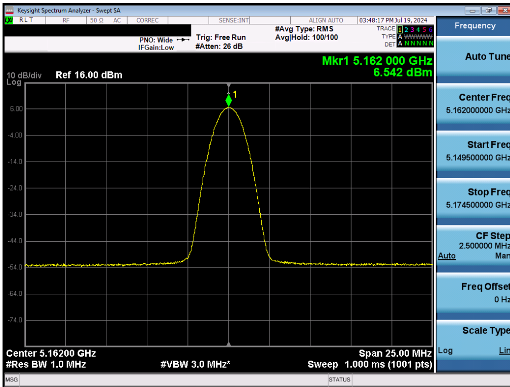
7-110. PSD TxBF Antenna WF2 (NB UNII BDR, ePA – 5162MHz)
