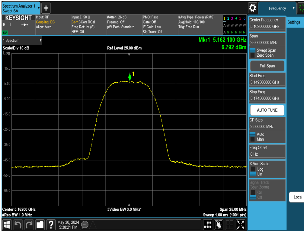
7-85. PSD Antenna WF2 (NB UNII HDR8, ePA – 5162MHz)
