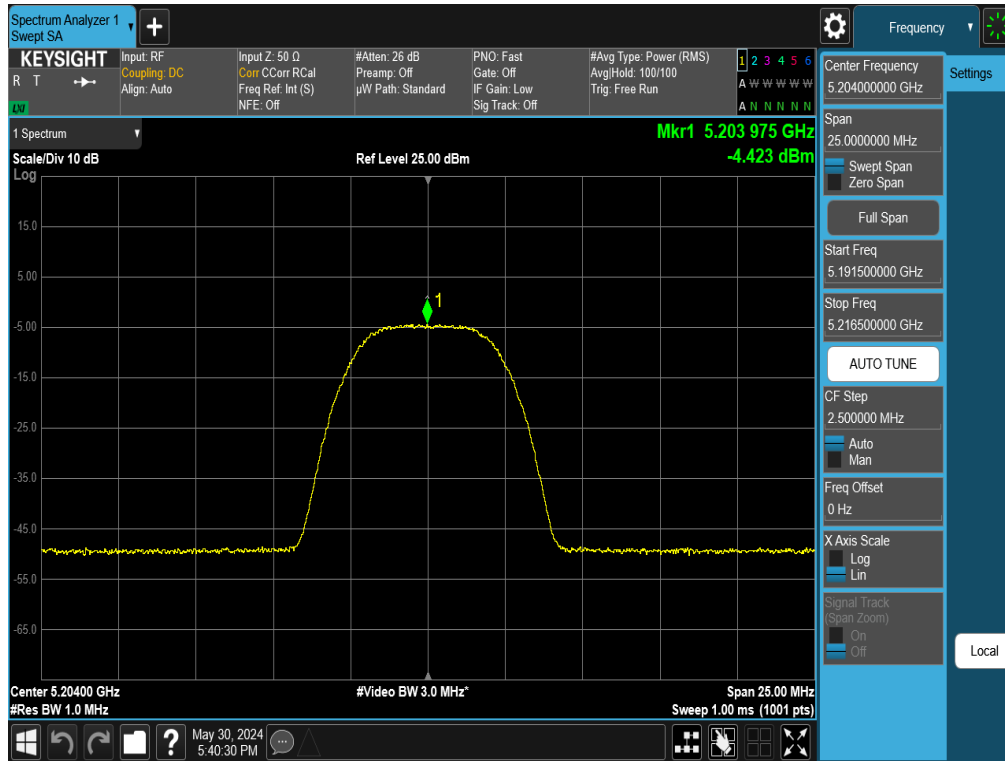
Plot 7-89. PSD Antenna WF2 (NB UNII HDR8, iPA – 5204MHz)
