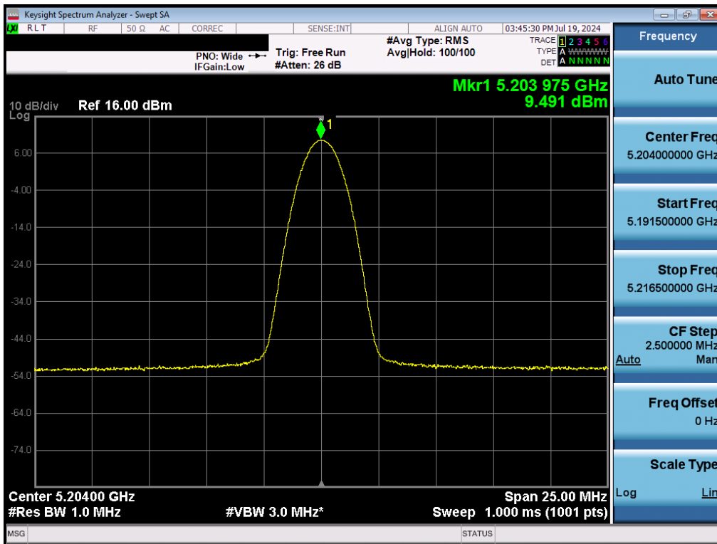
Plot 7-74. PSD Antenna WF2 (NB UNII BDR, ePA – 5204MHz)
