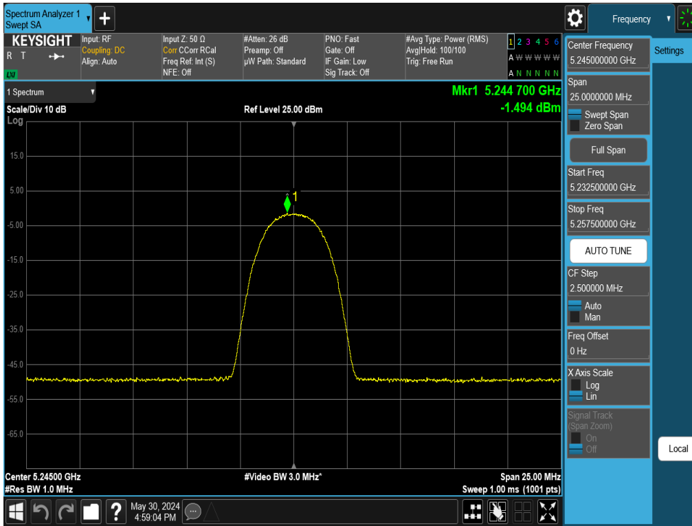
Plot 7-131. PSD TxBF Antenna WF5T (NB UNII HDR4, iPA- 5245MHz)
