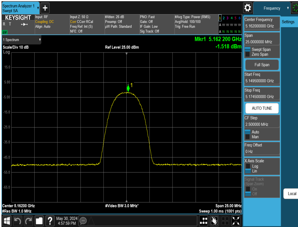
7-127. PSD TxBF Antenna WF5T (NB UNII HDR4, iPA – 5162MHz)
