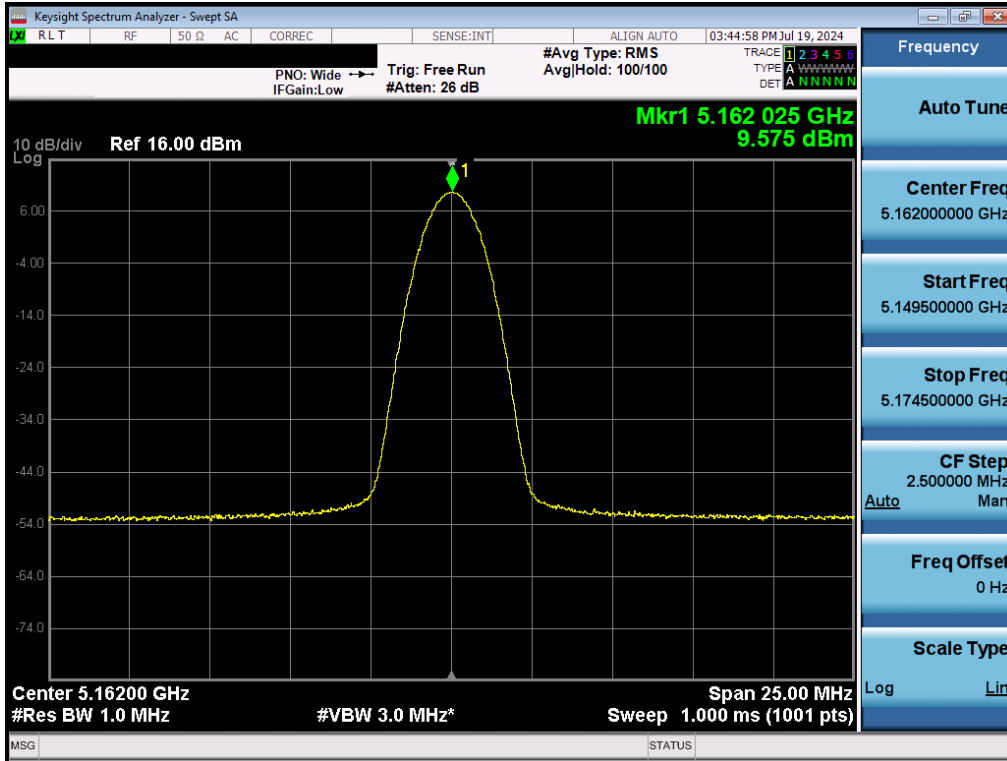
7-73. PSD Antenna WF2 (NB UNII BDR, ePA – 5162MHz)
