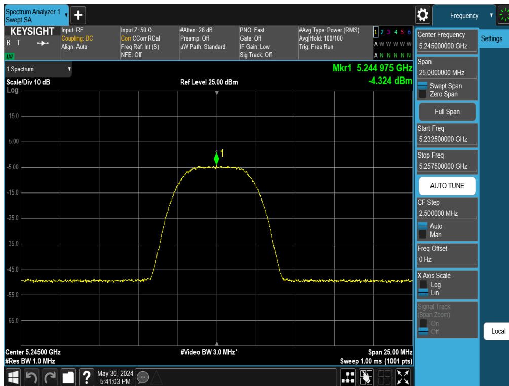
Plot 7-90. PSD Antenna WF2 (NB UNII HDR8, iPA– 5245MHz)
