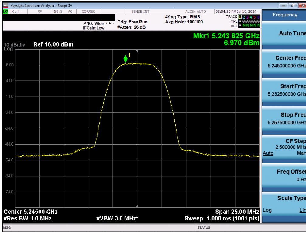
Plot 7-138. PSD TxBF Antenna WF2 (NB UNII HDR8, ePA- 5245MHz)
