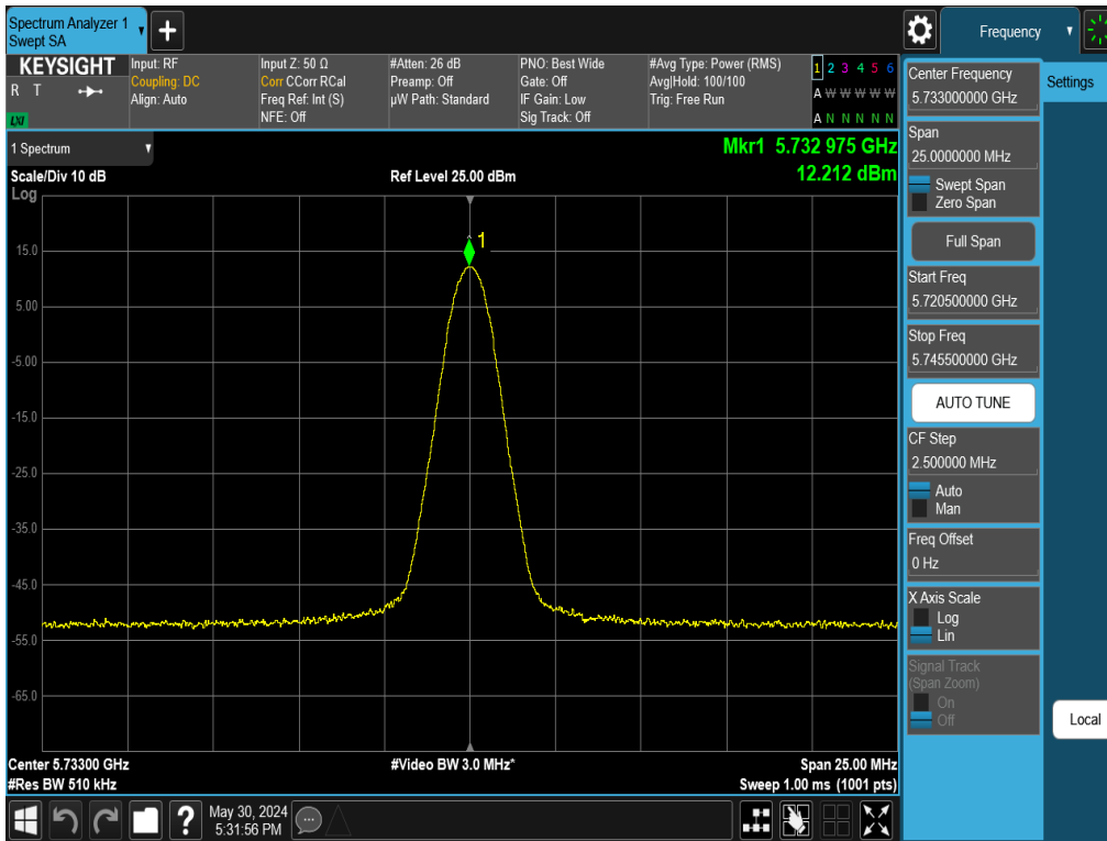
Plot 7-91. PSD Antenna WF2 (NB UNII BDR, ePA – 5733MHz)
