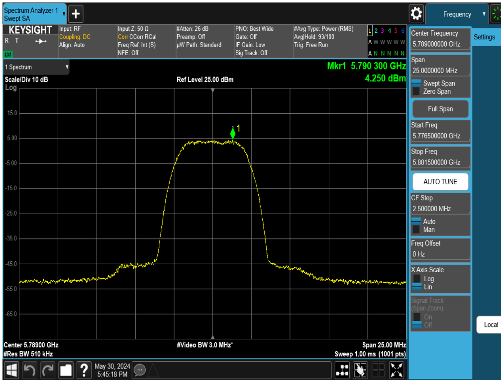
Plot 7-104. PSD Antenna WF2 (NB UNII HDR8, ePA – 5789MHz)
