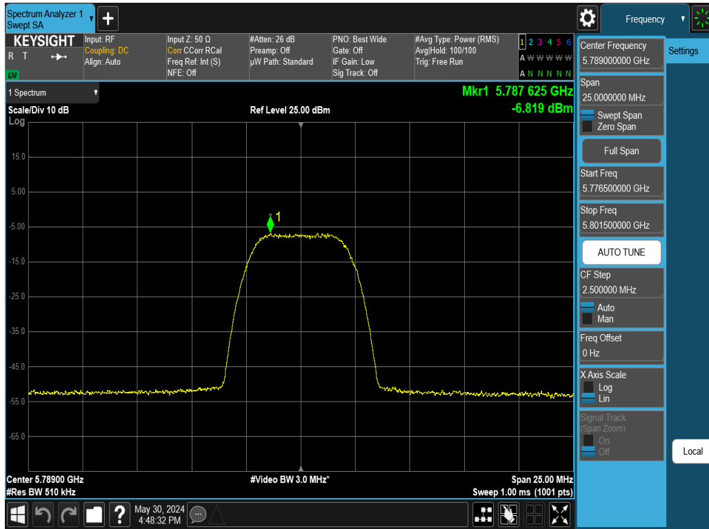
Plot 7-71. PSD Antenna WF5T (NB UNII HDR8, iPA – 5789MHz)
