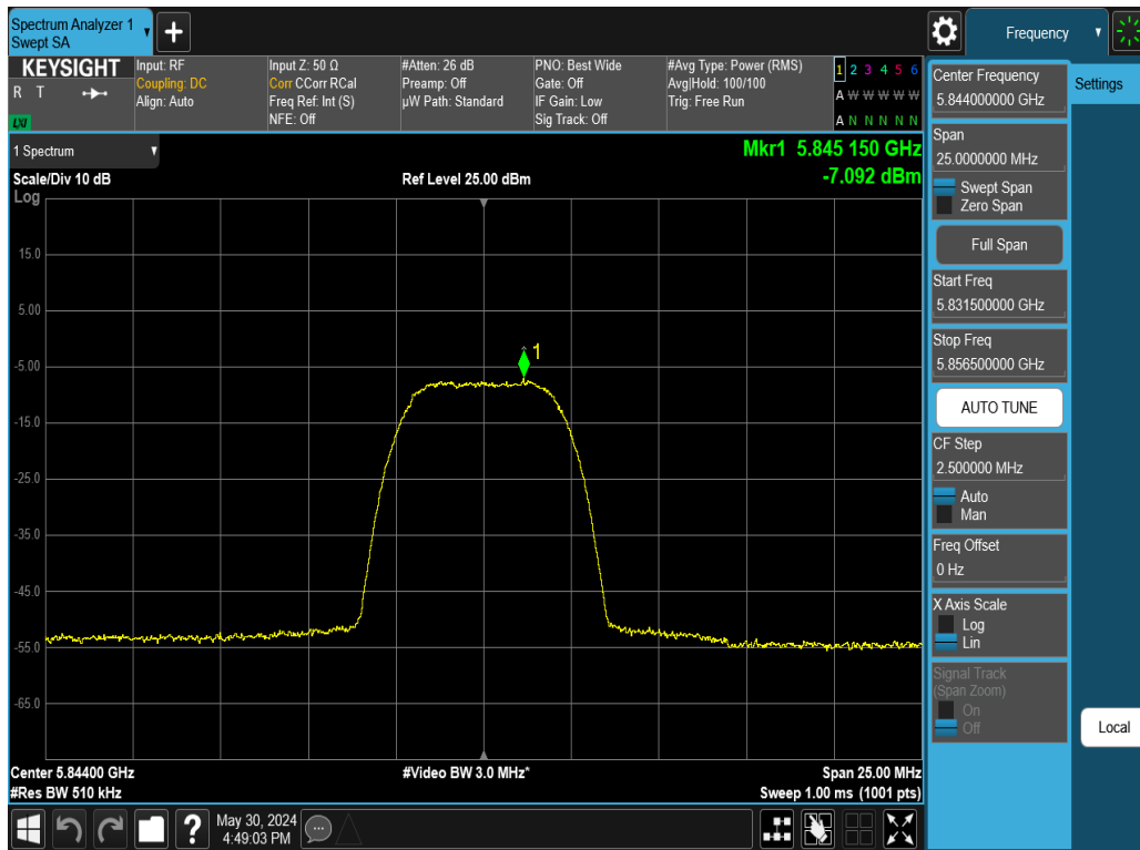
Plot 7-72. PSD Antenna WF5T (NB UNII HDR8, iPA – 5844MHz)
