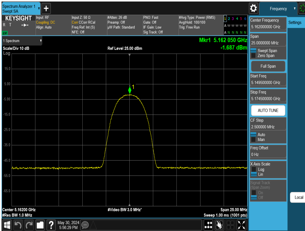
7-128. PSD TxBF Antenna WF2 (NB UNII HDR4, iPA – 5162MHz)
