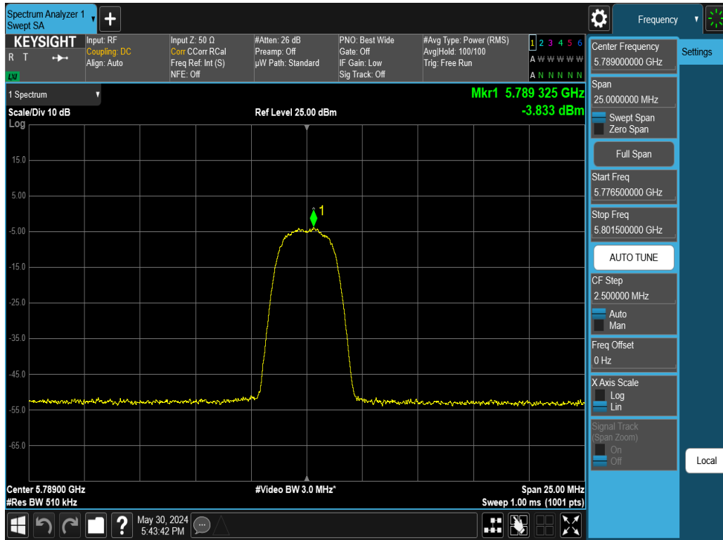
Plot 7-101. PSD Antenna WF2 (NB UNII HDR4, iPA – 5789MHz)
