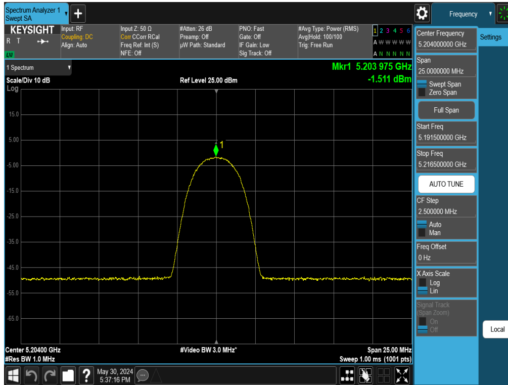
Plot 7-83. PSD Antenna WF2 (NB UNII HDR4, iPA – 5204MHz)
