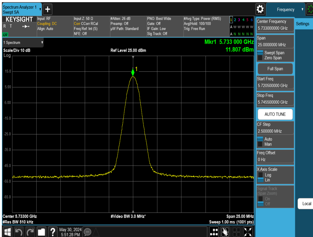
Plot 7-146. PSD TxBF Antenna WF2 (NB UNII BDR, ePA 5733MHz)
