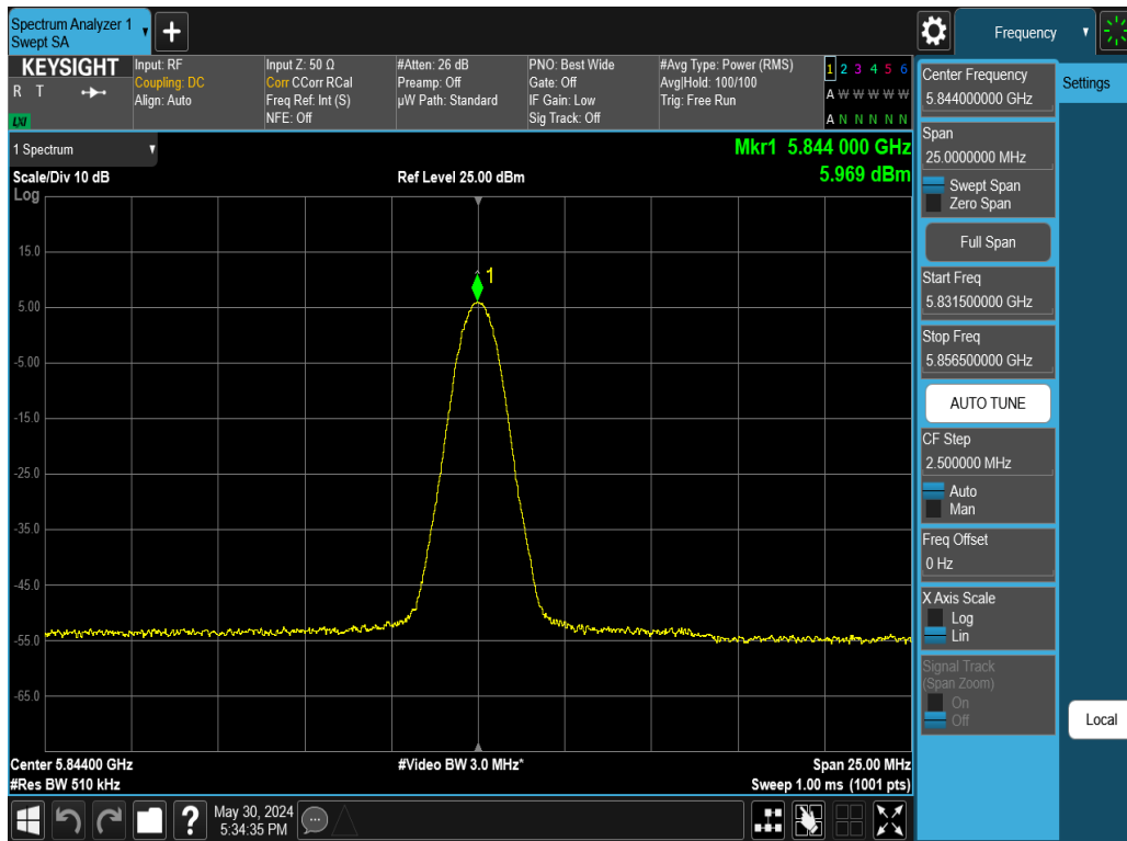
Plot 7-96. PSD Antenna WF2 (NB UNII BDR, iPA - 5844MHz)
