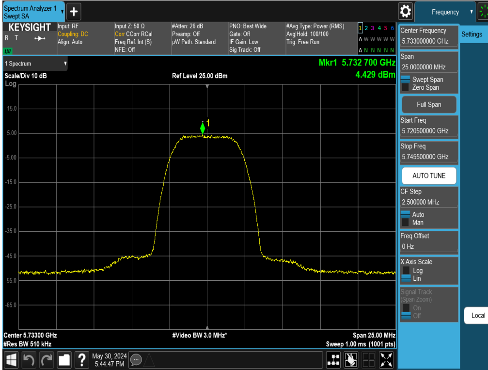
Plot 7-103. PSD Antenna WF2 (NB UNII HDR8, ePA – 5733MHz)
