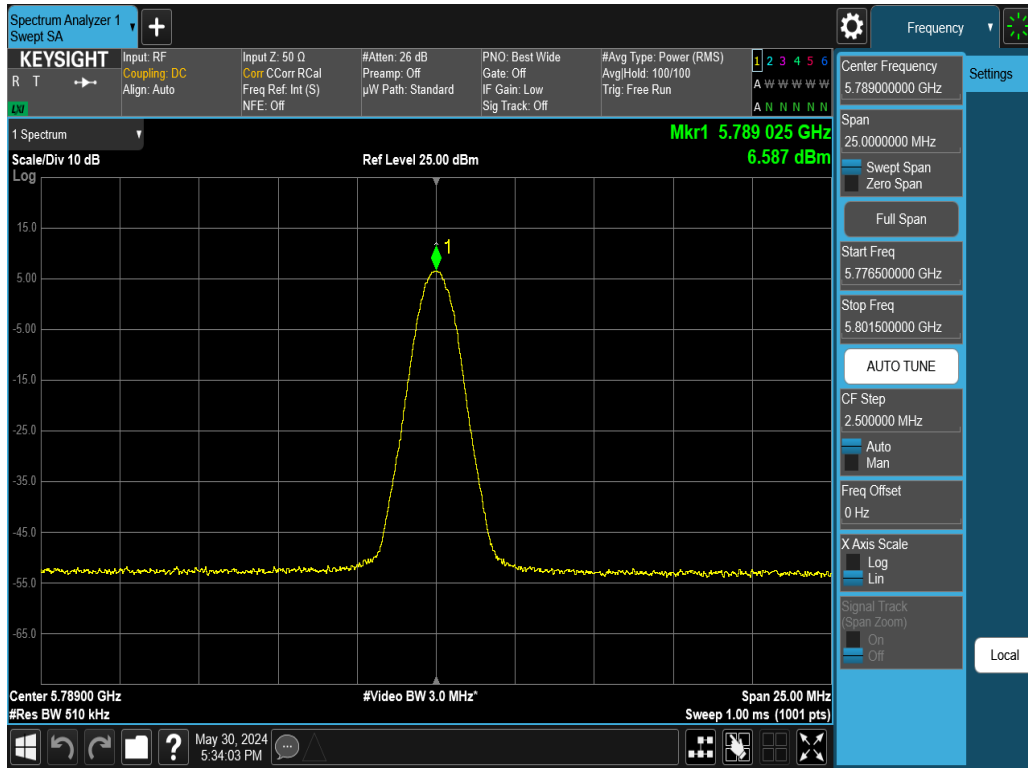
Plot 7-95. PSD Antenna WF2 (NB UNII BDR, iPA - 5789MHz)
