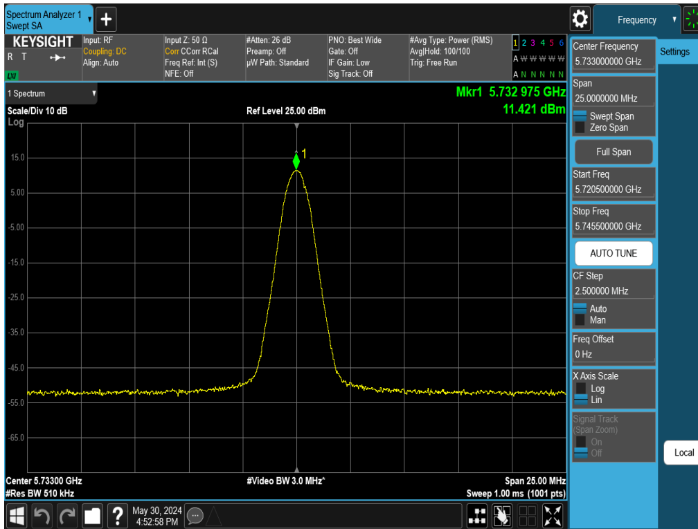
Plot 7-145. PSD TxBF Antenna WF5T (NB UNII BDR, ePA 5733MHz)
