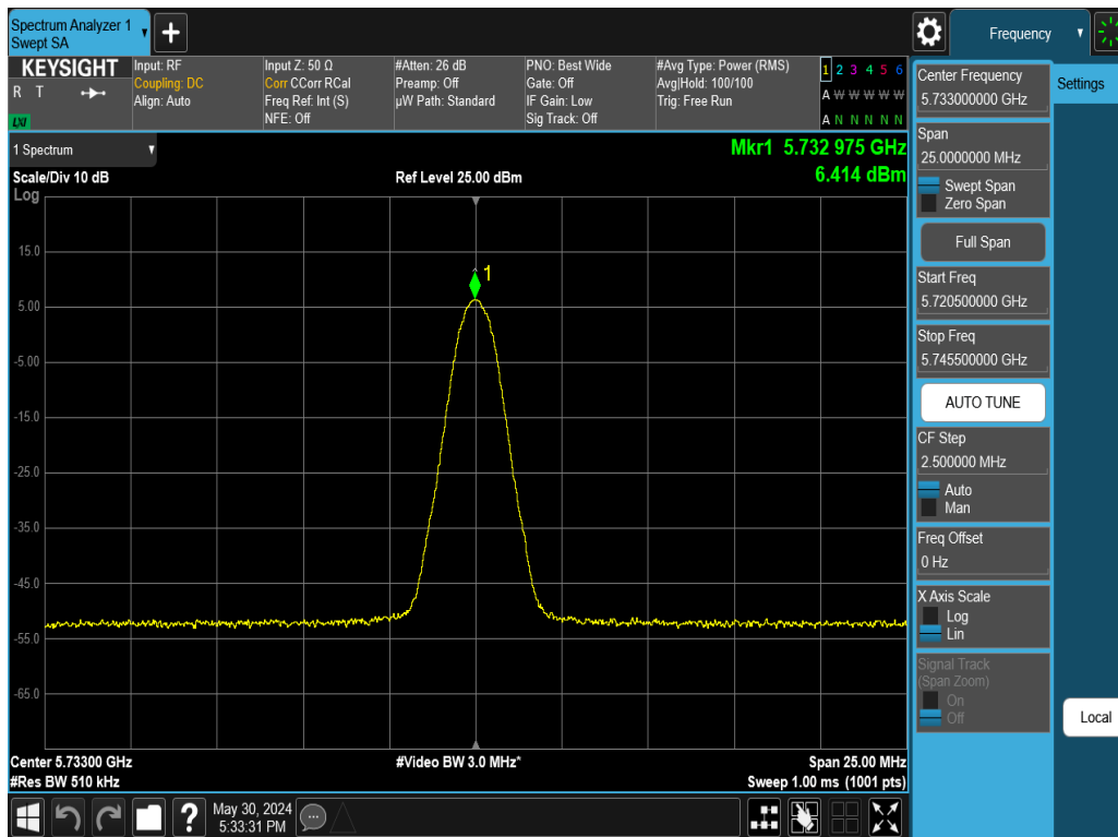
Plot 7-94. PSD Antenna WF2 (NB UNII BDR, iPA – 5733MHz)
