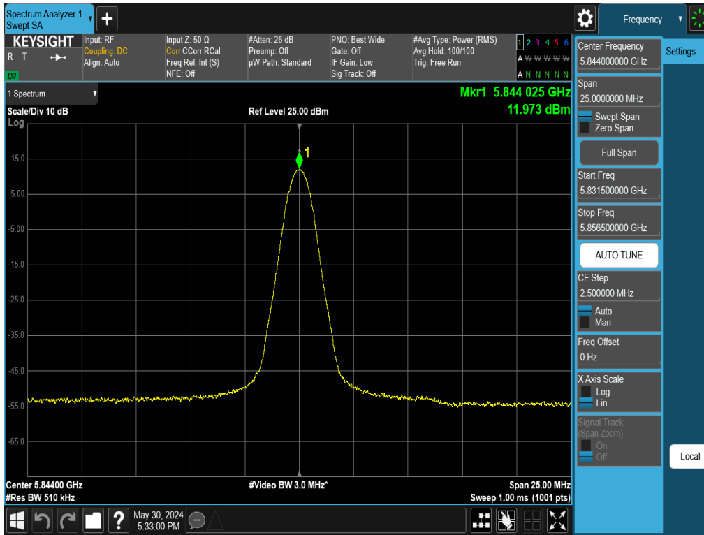
Plot 7-93. PSD Antenna WF2 (NB UNII BDR, ePA – 5844MHz)
