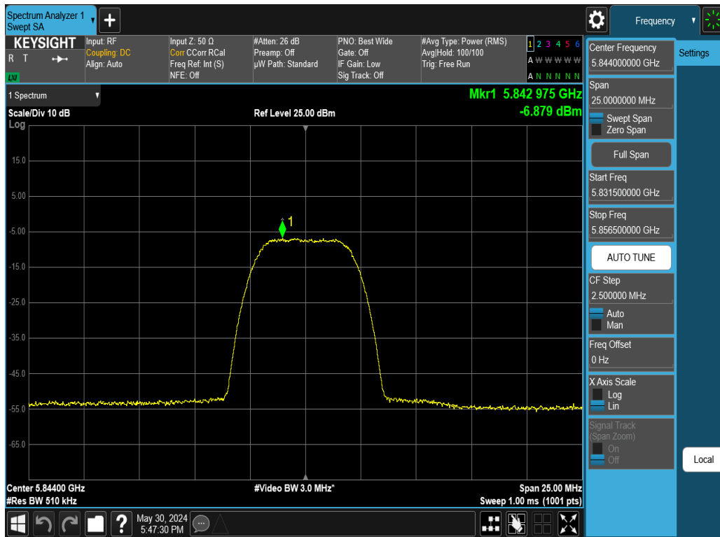
Plot 7-108. PSD Antenna WF2 (NB UNII HDR8, iPA – 5844MHz)
