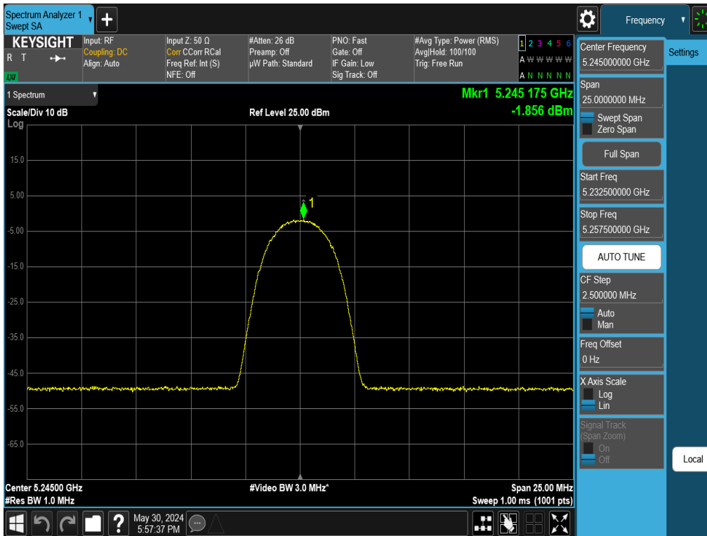
Plot 7-132. PSD TxBF Antenna WF2 (NB UNII HDR4, iPA- 5245MHz)
