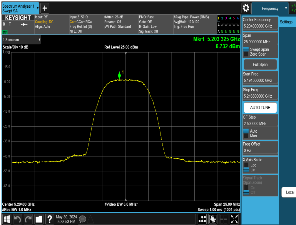
Plot 7-86. PSD Antenna WF2 (NB UNII HDR8, ePA – 5204MHz)
