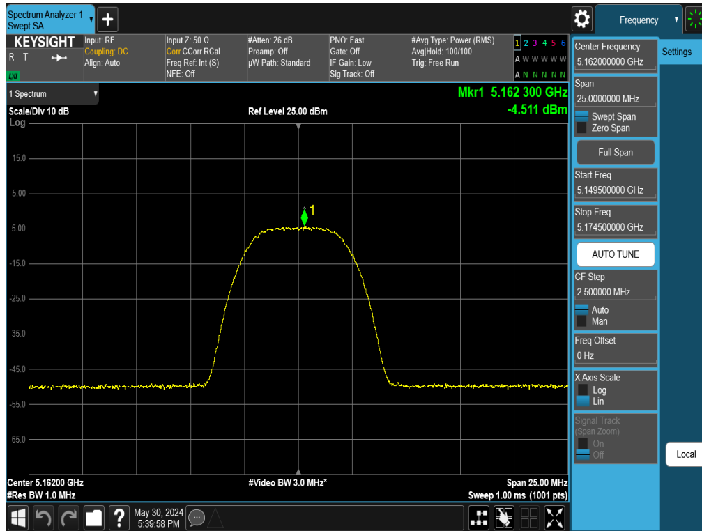
7-88. PSD Antenna WF2 (NB UNII HDR8, iPA - 5162MHz)
