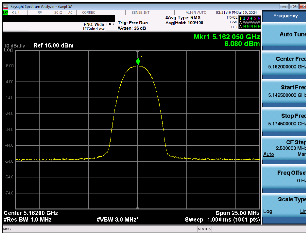
7-122. PSD Tx BF Antenna WF2 (NB UNII HDR4, ePA – 5162MHz)
