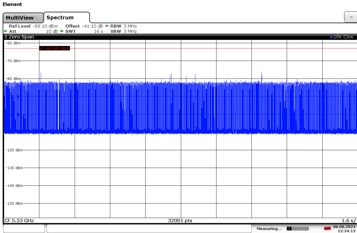
Figure 9-1. 5530MHz - Channel Loading - Mode 1 (80MHz)
