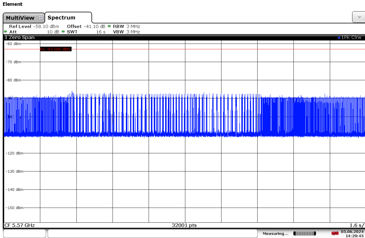
Figure 9-3. 5570MHz - Channel Loading - Mode 1 (160MHz)
