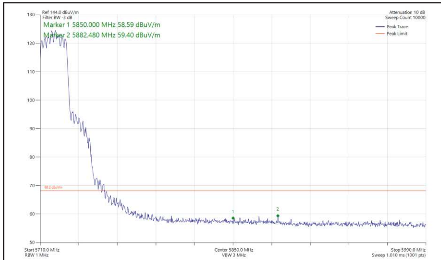
Figure 402 - 802.11ax HE20, SU, CDD, Core 0 + Core 1 - 5720 MHz Band Edge Frequency 5850 MHz
