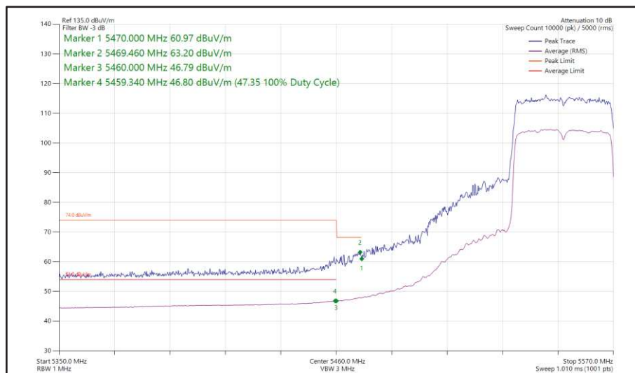
Figure 462 - 802.11ax HE40, SU, SISO, Core 1 - 5550 MHz Band Edge Frequency 5470 MHz
