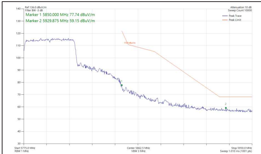
Figure 456 - 802.11ax HE40, SU, SISO, Core 0 - 5795 MHz Band Edge Frequency 5850 MHz
