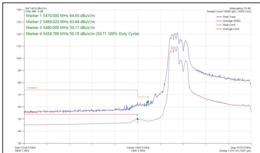
Figure 554 - 802.11ax HE80, RU 106-53, CDD, Core 0 + Core 1 - 5530 MHz Band Edge Frequency 5470 MHz
