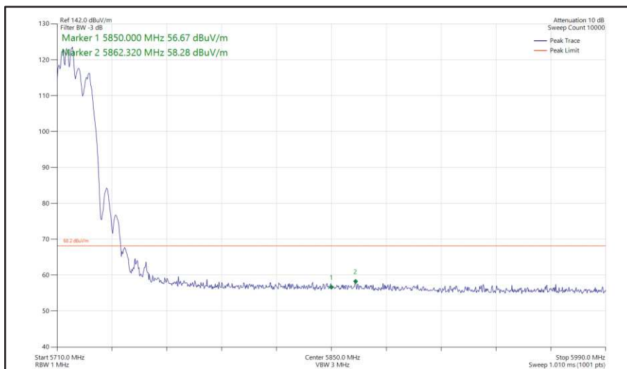
Figure 403 - 802.11ax HE20, RU 106-53, CDD, Core 0 + Core 1 - 5720 MHz Band Edge Frequency 5850 MHz
