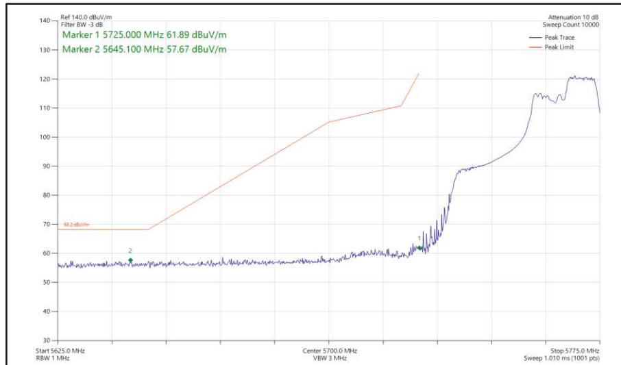
Figure 465 - 802.11ax HE40, RU 106-56, SISO, Core 1 - 5755 MHz Band Edge Frequency 5725 MHz
