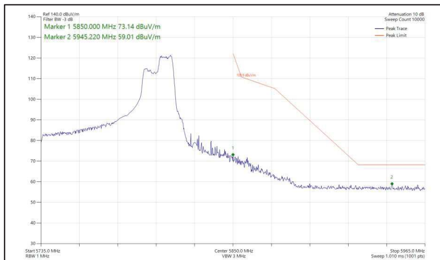
Figure 551 - 802.11ax HE80, RU 106-60, SISO, Core 1 - 5775 MHz Band Edge Frequency 5850 MHz
