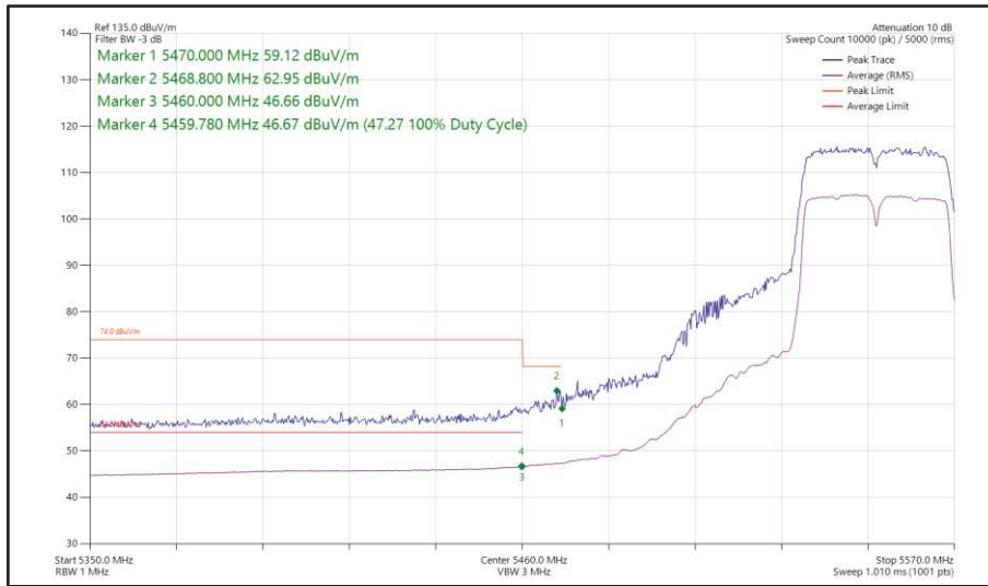
Figure 459 - 802.11n HT40, SISO, Core 1 - 5550 MHz Band Edge Frequency 5470 MHz
