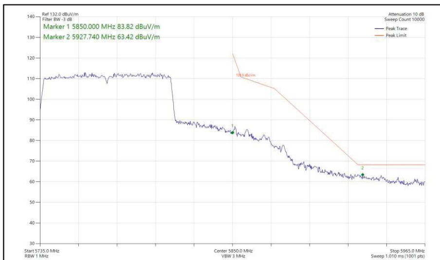
Figure 532 - 802.11ac VHT80, SISO, Core 0 - 5775 MHz Band Edge Frequency 5850 MHz
