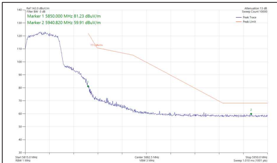
Figure 438 - 802.11ac VHT20, TxBF, Core 0 + Core 1 - 5825 MHz Band Edge Frequency 5850 MHz
