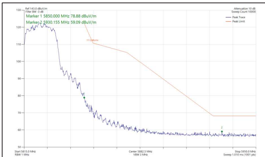
Figure 401 - 802.11n HT20, CDD, Core 0 + Core 1 - 5825 MHz Band Edge Frequency 5850 MHz
