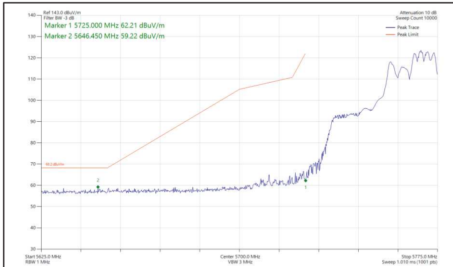
Figure 484 - 802.11ax HE40, RU 106-56, CDD, Core 0 + Core 1 - 5755 MHz Band Edge Frequency 5725 MHz
