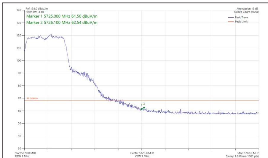
Figure 434 - 802.11ac VHT20, TxBF, Core 0 + Core 1 - 5680 MHz Band Edge Frequency 5725 MHz
