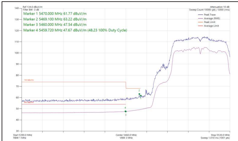
Figure 515 - 802.11ac VHT40, TxBF, Core 0 + Core 1 - 5510 MHz Band Edge Frequency 5470 MHz
