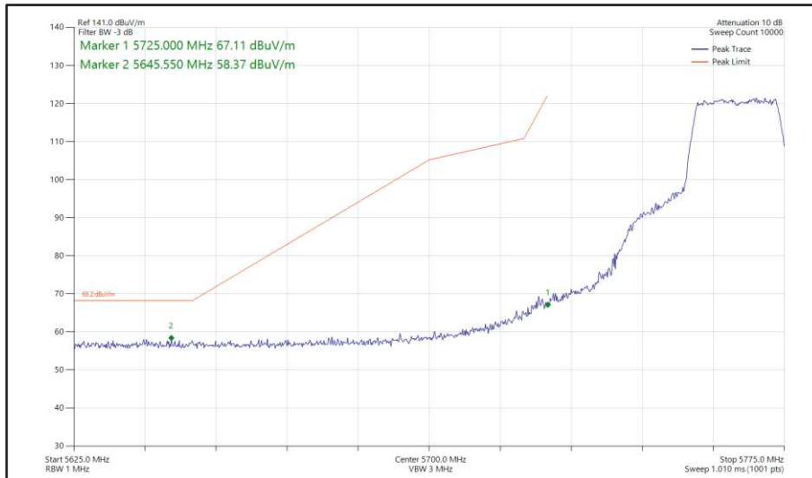
Figure 413 - 802.11n HT20, SDM, Core 0 + Core 1 - 5765 MHz Band Edge Frequency 5725 MHz
