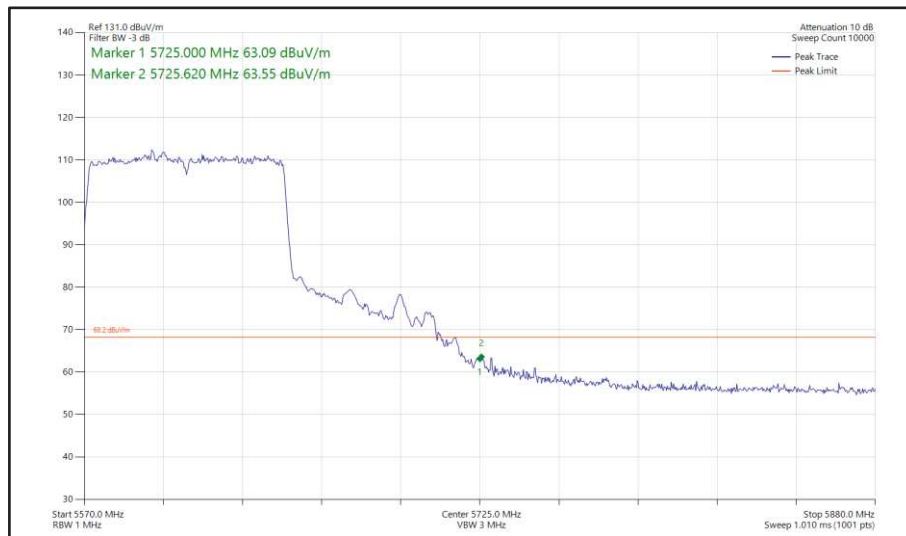
Figure 543 - 802.11ac VHT80, SISO, Core 1 - 5610 MHz Band Edge Frequency 5725 MHz
