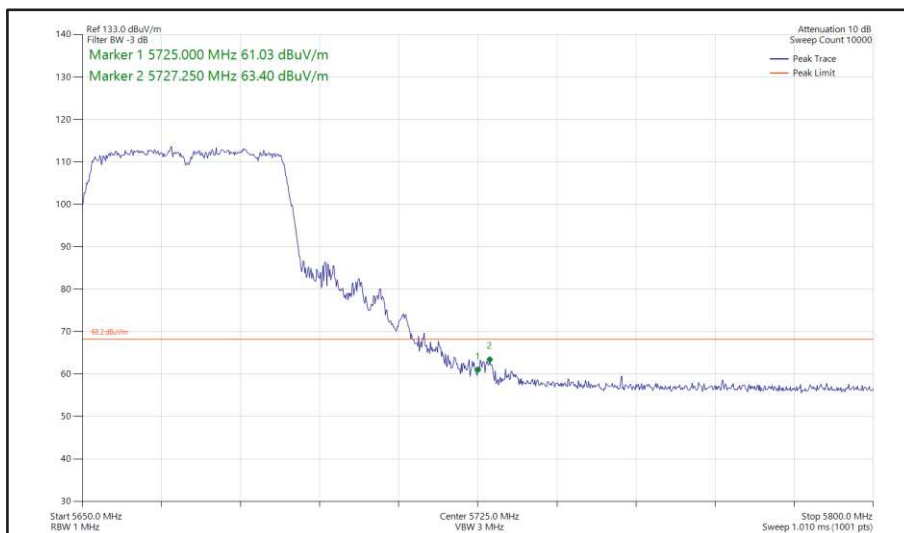
Figure 519 - 802.11ac VHT40, TxBF, Core 0 + Core 1 - 5670 MHz Band Edge Frequency 5725 MHz
