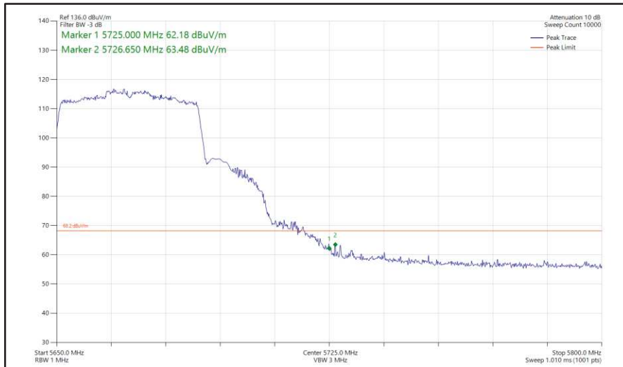
Figure 469 - 802.11ax HE40, SU, SISO, Core 1 - 5670 MHz Band Edge Frequency 5725 MHz
