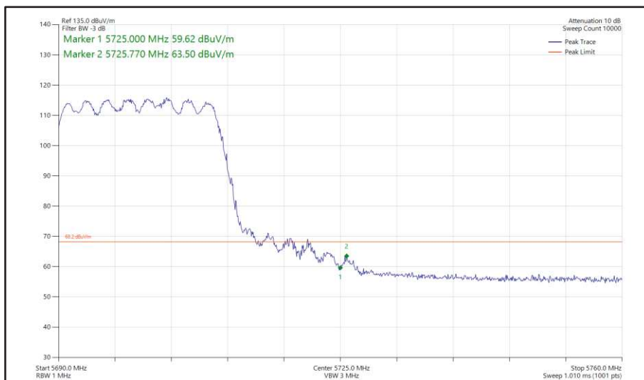
Figure 397 - 802.11ax HE20, SU, CDD, Core 0 + Core 1 - 5700 MHz Band Edge Frequency 5725 MHz
