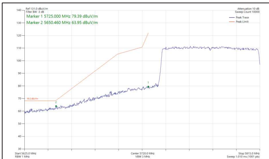
Figure 541 - 802.11ax HE80, SU, SISO, Core 1 - 5775 MHz Band Edge Frequency 5725 MHz
