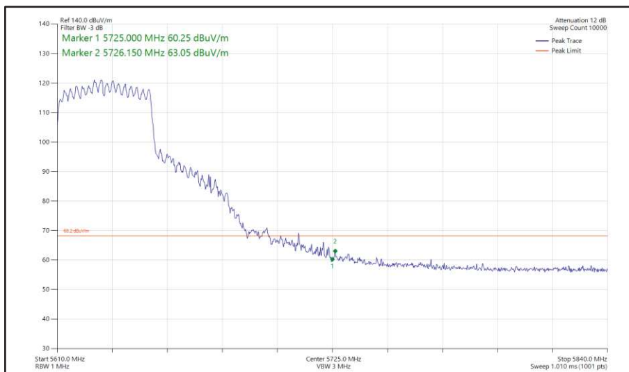
Figure 487 - 802.11ax HE40, SU, CDD, Core 0 + Core 1 - 5630 MHz Band Edge Frequency 5725 MHz
