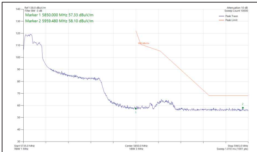
Figure 536 - 802.11ax HE80, RU 106-53, SISO, Core 0 - 5775 MHz Band Edge Frequency 5850 MHz
