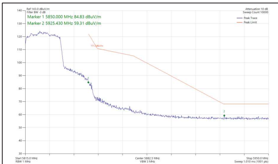
Figure 428 - 802.11ax HE20, SU, SDM, Core 0 + Core 1 - 5825 MHz Band Edge Frequency 5850 MHz
