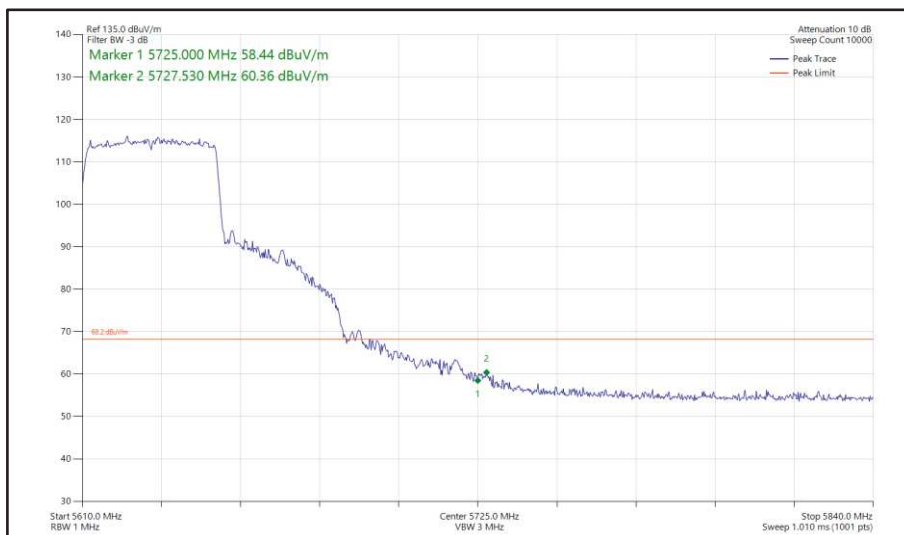
Figure 449 - 802.11ax HE40, SU, SISO, Core 0 - 5630 MHz Band Edge Frequency 5725 MHz
