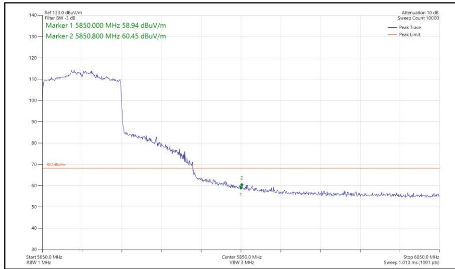
Figure 533 - 802.11ax HE80, SU, SISO, Core 0 - 5690 MHz Band Edge Frequency 5850 MHz
