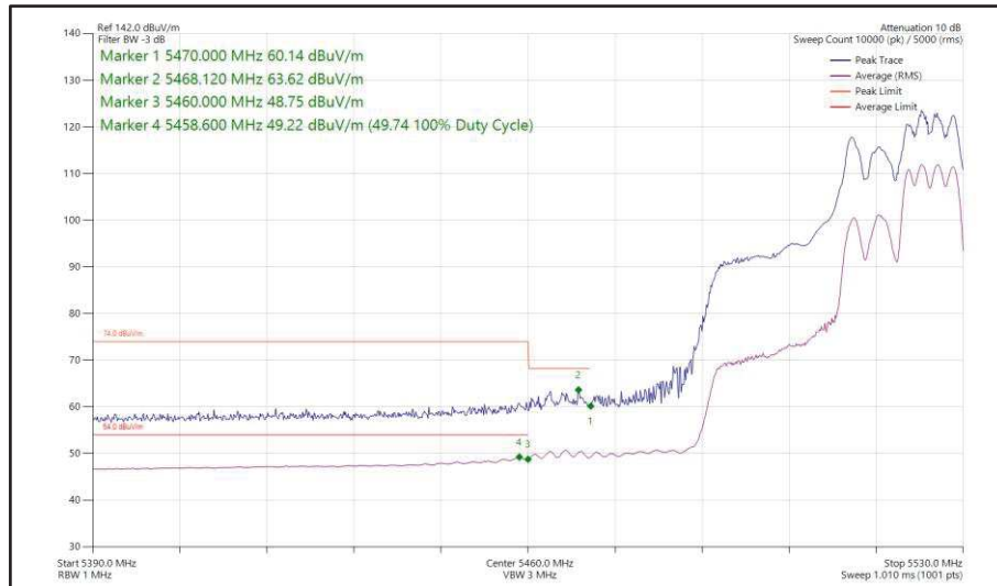
Figure 480 - 802.11ax HE40, RU 106-56, CDD, Core 0 + Core 1 - 5510 MHz Band Edge Frequency 5470 MHz
