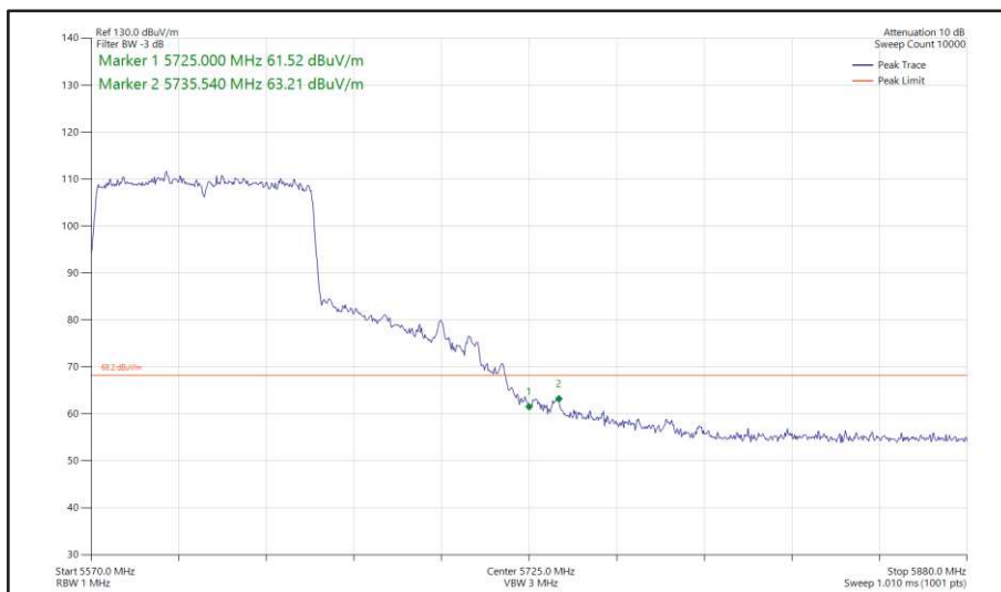
Figure 528 - 802.11ac VHT80, SISO, Core 0 - 5610 MHz Band Edge Frequency 5725 MHz
