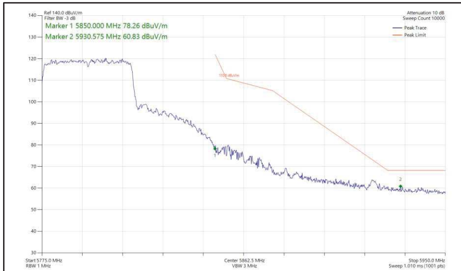
Figure 513 - 802.11ax HE40, SU, SDM, Core 0 + Core 1 - 5795 MHz Band Edge Frequency 5850 MHz
