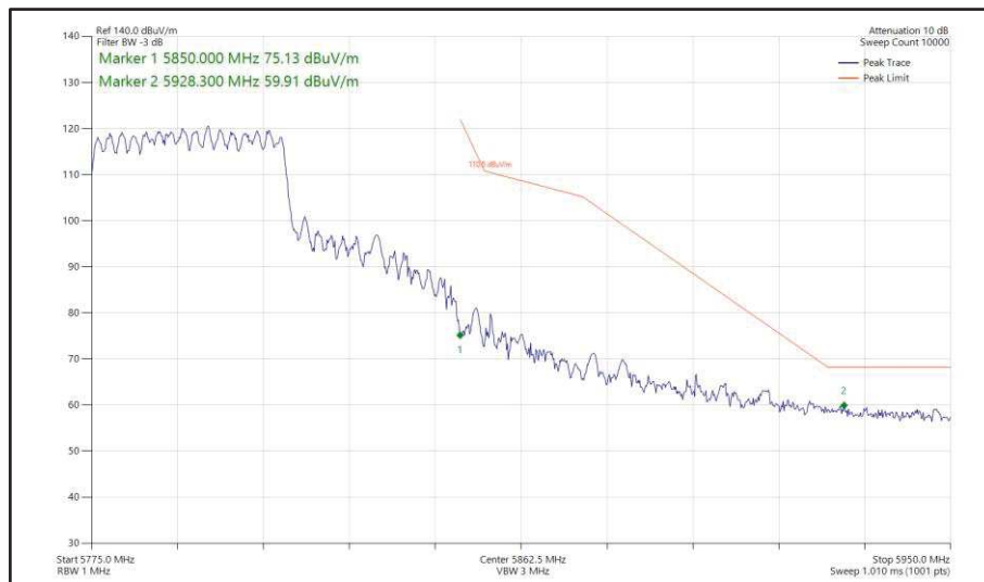
Figure 494 - 802.11ax HE40, SU, CDD, Core 0 + Core 1 - 5795 MHz Band Edge Frequency 5850 MHz
