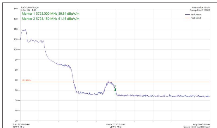
Figure 451 - 802.11ax HE40, RU 52-37, SISO, Core 0 - 5670 MHz Band Edge Frequency 5725 MHz
