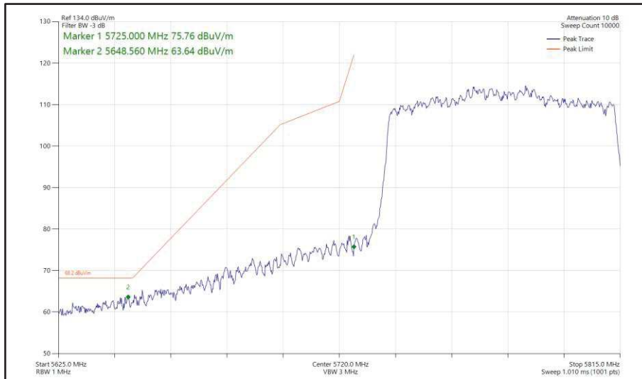
Figure 555 - 802.11ac VHT80, CDD, Core 0 + Core 1 - 5775 MHz Band Edge Frequency 5725 MHz
