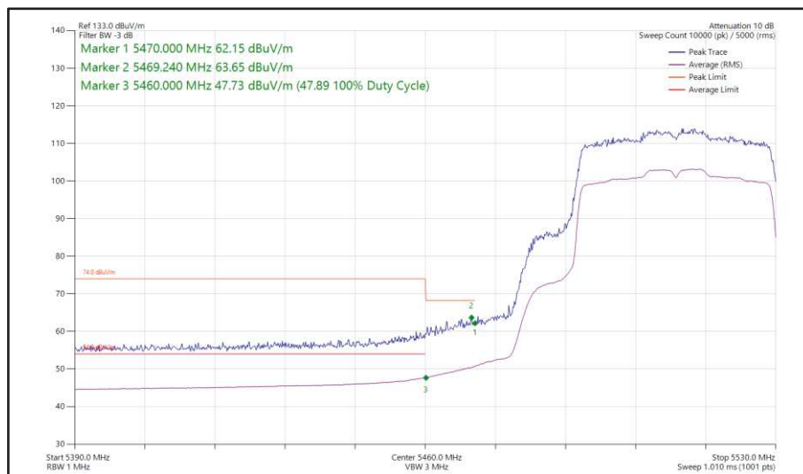
Figure 441 - 802.11ax HE40, SU, SISO, Core 0 - 5510 MHz Band Edge Frequency 5470 MHz
