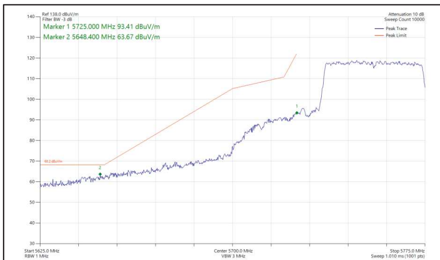
Figure 502 - 802.11ax HE40, SU, SDM, Core 0 + Core 1 - 5755 MHz Band Edge Frequency 5725 MHz
