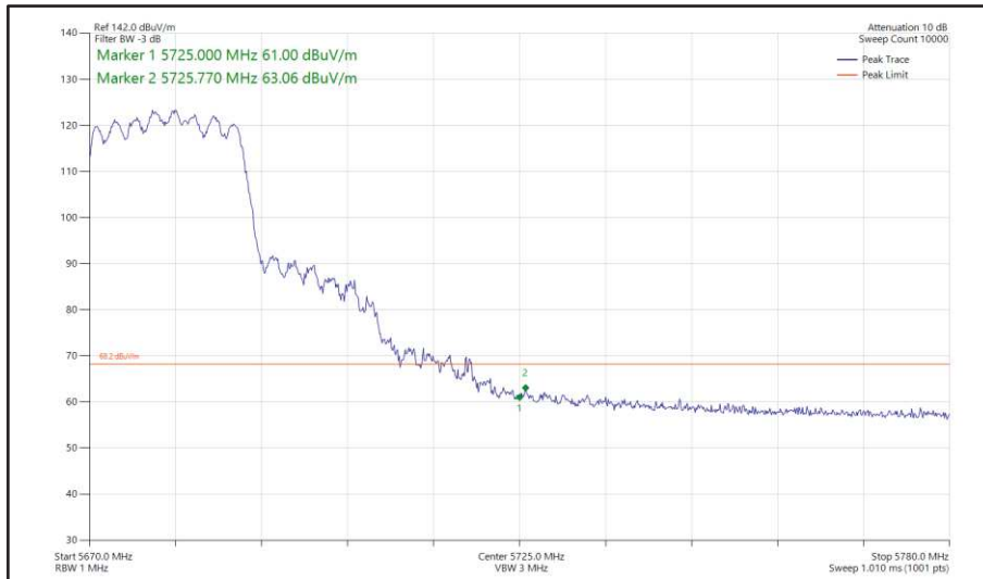
Figure 396 - 802.11ax HE20, SU, CDD, Core 0 + Core 1 - 5680 MHz Band Edge Frequency 5725 MHz
