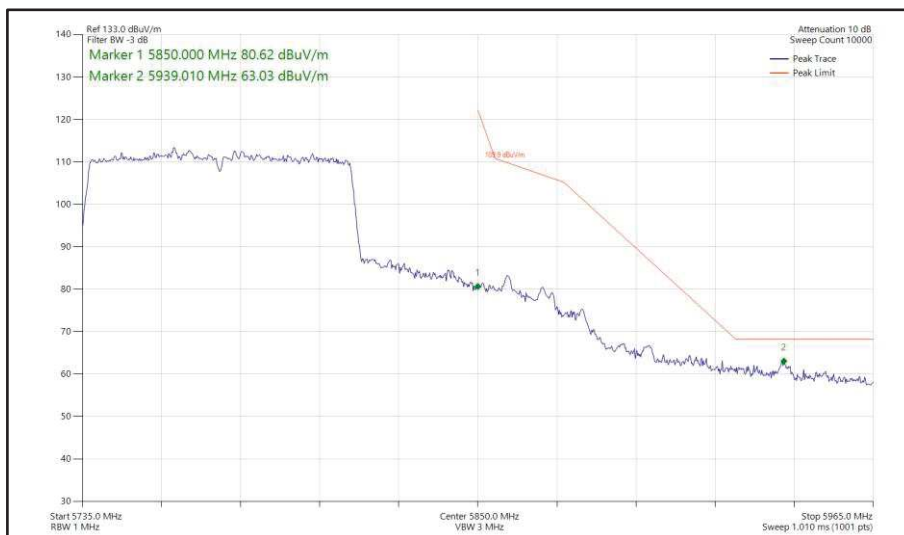
Figure 547 - 802.11ac VHT80, SISO, Core 1 - 5775 MHz Band Edge Frequency 5850 MHz
