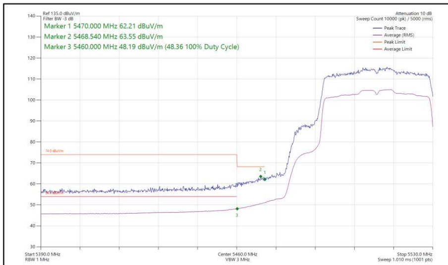
Figure 460 - 802.11ax HE40, SU, SISO, Core 1 - 5510 MHz Band Edge Frequency 5470 MHz
