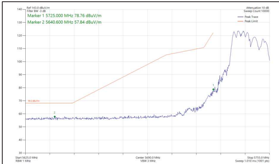
Figure 415 - 802.11ax HE20, RU 106-53, SDM, Core 0 + Core 1 - 5745 MHz Band Edge Frequency 5725 MHz
