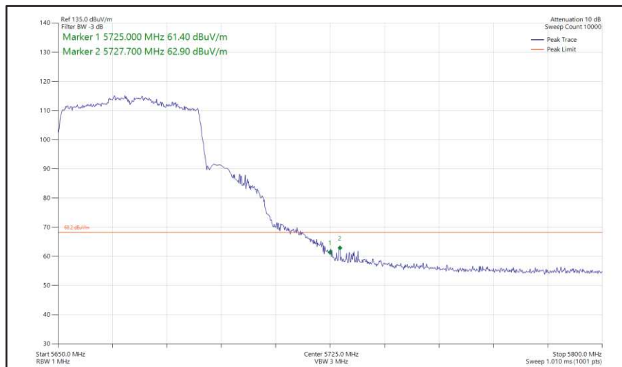
Figure 450 - 802.11ax HE40, SU, SISO, Core 0 - 5670 MHz Band Edge Frequency 5725 MHz
