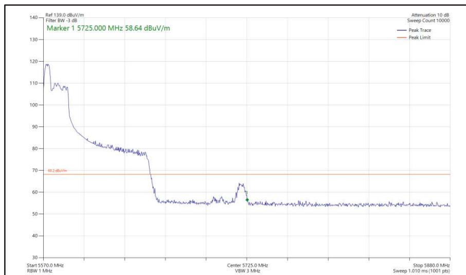
Figure 530 - 802.11ax HE80, RU 52-37, SISO, Core 0 - 5610 MHz Band Edge Frequency 5725 MHz
