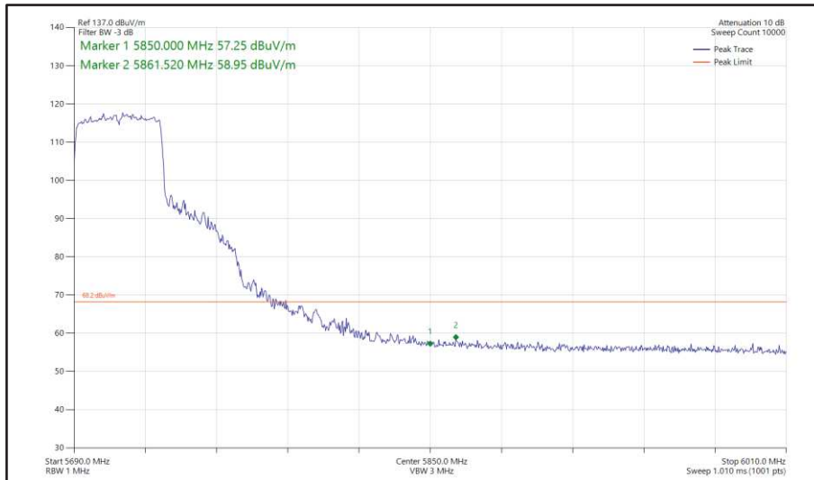
Figure 473 - 802.11ax HE40, SU, SISO, Core 1 - 5710 MHz Band Edge Frequency 5850 MHz
