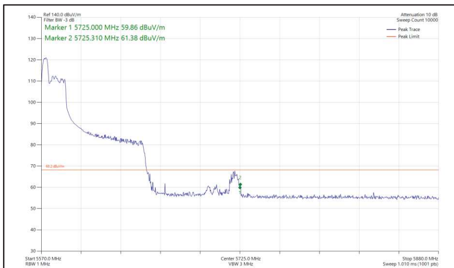
Figure 545 - 802.11ax HE80, RU 52-37, SISO, Core 1 - 5610 MHz Band Edge Frequency 5725 MHz
