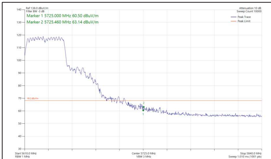
Figure 485 - 802.11n HT40, CDD, Core 0 + Core 1 - 5630 MHz Band Edge Frequency 5725 MHz
