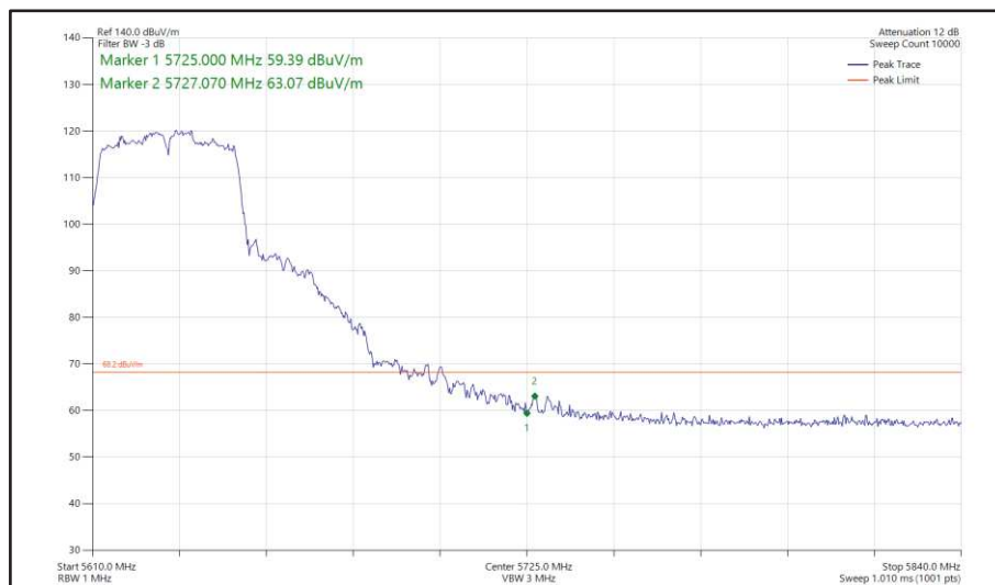
Figure 504 - 802.11n HT40, SDM, Core 0 + Core 1 - 5630 MHz Band Edge Frequency 5725 MHz
