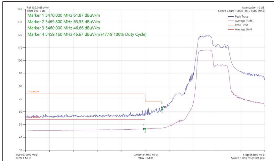
Figure 461 - 802.11ax HE40, RU 106-53, SISO, Core 1 - 5510 MHz Band Edge Frequency 5470 MHz
