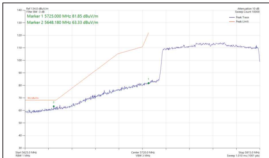
Figure 526 - 802.11ax HE80, SU, SISO, Core 0 - 5775 MHz Band Edge Frequency 5725 MHz
