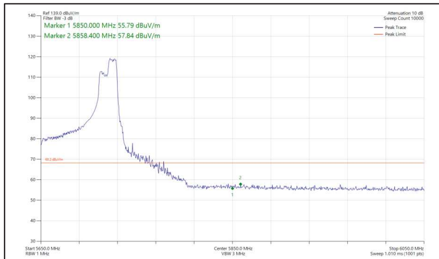
Figure 534 - 802.11ax HE80, RU 106-60, SISO, Core 0 - 5690 MHz Band Edge Frequency 5850 MHz
