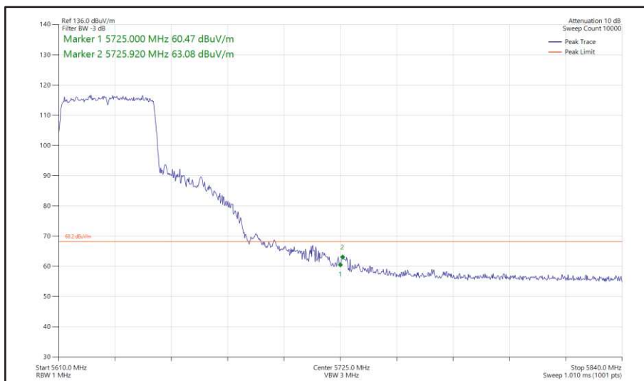
Figure 468 - 802.11ax HE40, SU, SISO, Core 1 - 5630 MHz Band Edge Frequency 5725 MHz
