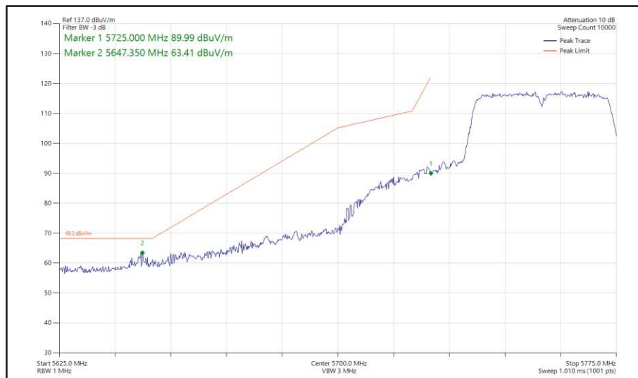
Figure 463 - 802.11n HT40, SISO, Core 1 - 5755 MHz Band Edge Frequency 5725 MHz
