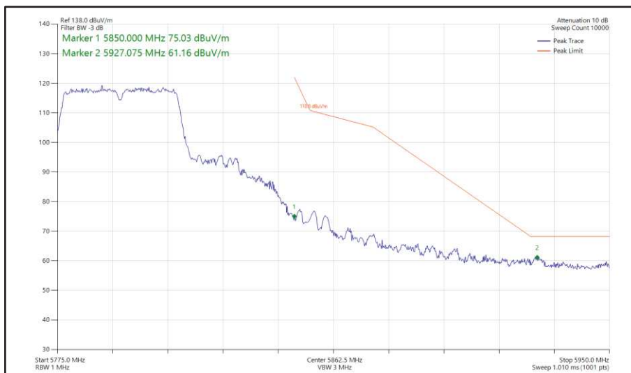
Figure 510 - 802.11n HT40, SDM, Core 0 + Core 1 - 5795 MHz Band Edge Frequency 5850 MHz
