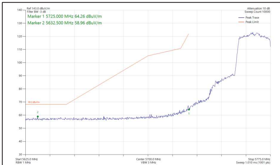
Figure 416 - 802.11ax HE20, SU, SDM, Core 0 + Core 1 - 5765 MHz Band Edge Frequency 5725 MHz
