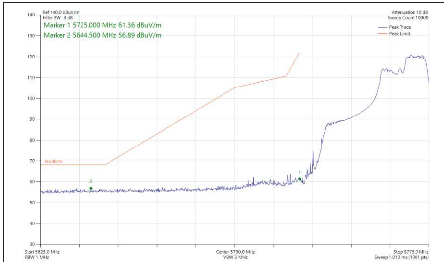
Figure 446 - 802.11ax HE40, RU 106-56, SISO, Core 0 - 5755 MHz Band Edge Frequency 5725 MHz
