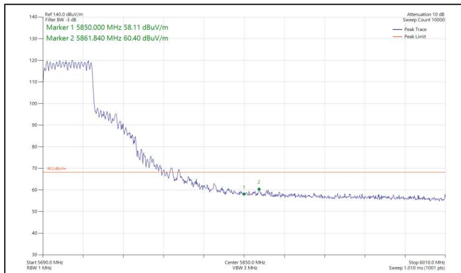
Figure 492 - 802.11ax HE40, SU, CDD, Core 0 + Core 1 - 5710 MHz Band Edge Frequency 5850 MHz
