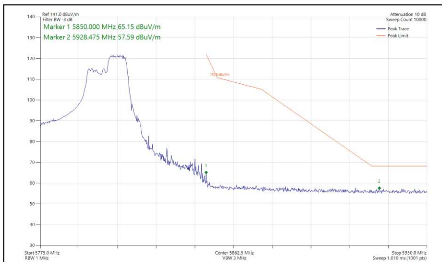
Figure 476 - 802.11ax HE40, RU 106-56, SISO, Core 1 - 5795 MHz Band Edge Frequency 5850 MHz
