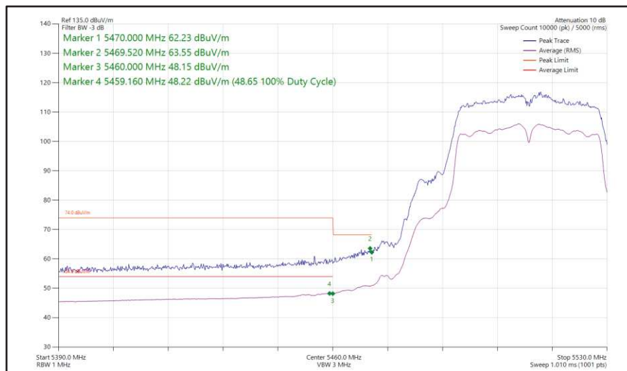
Figure 496 - 802.11n HT40, SDM, Core 0 + Core 1 - 5510 MHz Band Edge Frequency 5470 MHz
