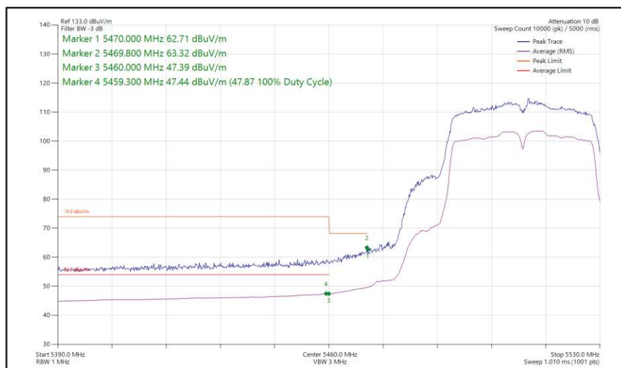
Figure 458 - 802.11n HT40, SISO, Core 1 - 5510 MHz Band Edge Frequency 5470 MHz
