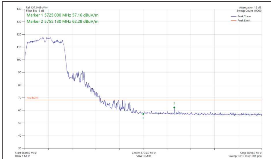
Figure 518 - 802.11ac VHT40, TxBF, Core 0 + Core 1 - 5630 MHz Band Edge Frequency 5725 MHz
