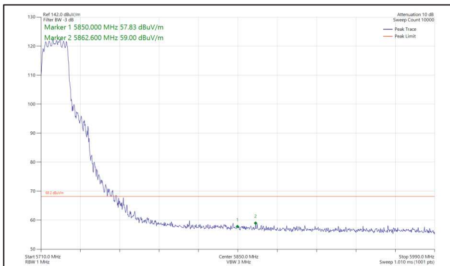
Figure 399 - 802.11n HT20, CDD, Core 0 + Core 1 - 5720 MHz Band Edge Frequency 5850 MHz
