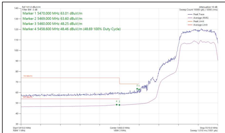
Figure 430 - 802.11ac VHT20, TxBF, Core 0 + Core 1 - 5500 MHz Band Edge Frequency 5470 MHz
