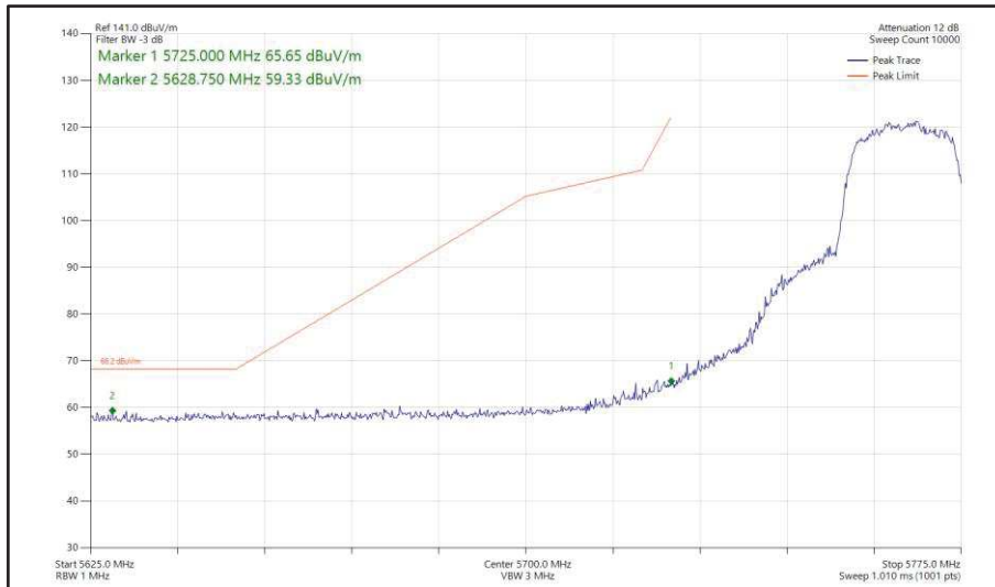
Figure 433 - 802.11ac VHT20, TxBF, Core 0 + Core 1 - 5765 MHz Band Edge Frequency 5725 MHz
