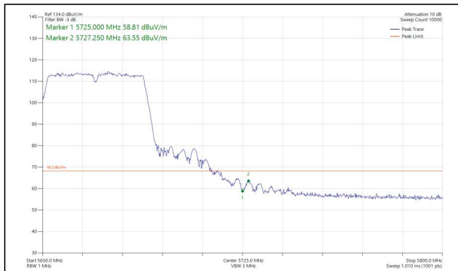
Figure 505 - 802.11n HT40, SDM, Core 0 + Core 1 - 5670 MHz Band Edge Frequency 5725 MHz
