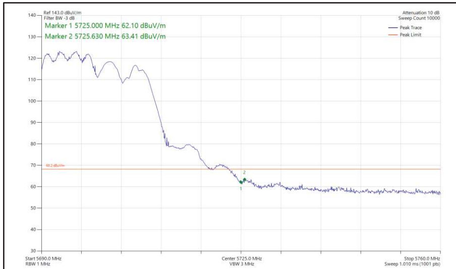
Figure 398 - 802.11ax HE20, RU 106-53, CDD, Core 0 + Core 1 - 5700 MHz Band Edge Frequency 5725 MHz
