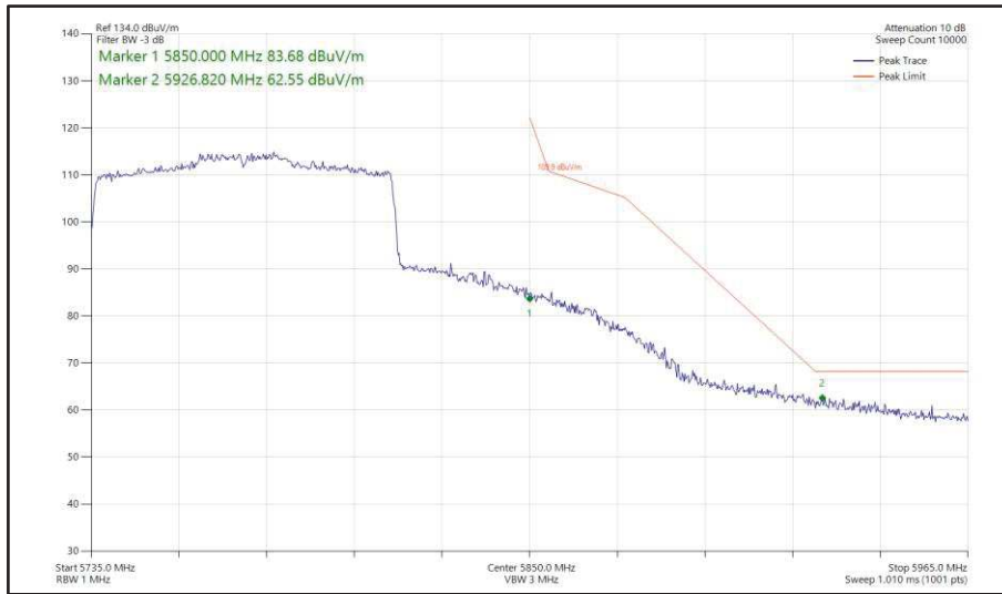
Figure 535 - 802.11ax HE80, SU, SISO, Core 0 - 5775 MHz Band Edge Frequency 5850 MHz
