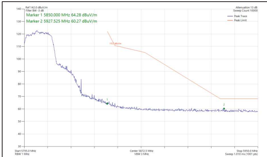
Figure 437 - 802.11ac VHT20, TxBF, Core 0 + Core 1 - 5805 MHz Band Edge Frequency 5850 MHz
