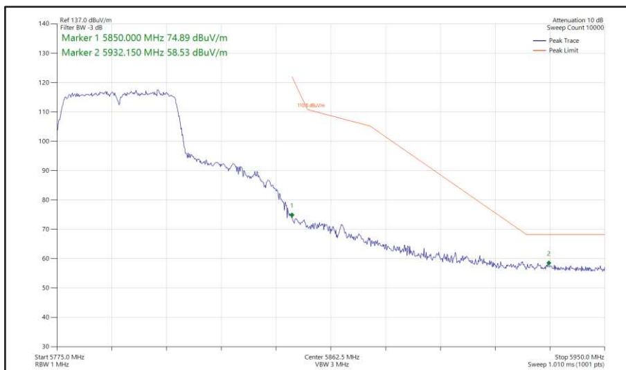
Figure 472 - 802.11n HT40, SISO, Core 1 - 5795 MHz Band Edge Frequency 5850 MHz
