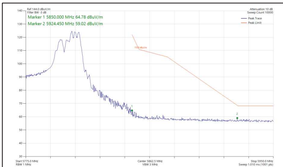
Figure 514 - 802.11ax HE40, RU 106-56, SDM, Core 0 + Core 1 - 5795 MHz Band Edge Frequency 5850 MHz
