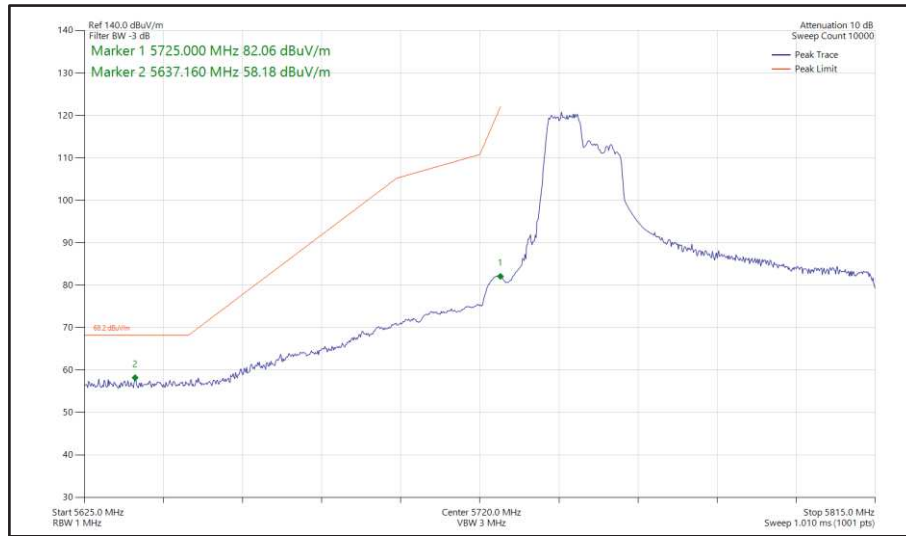
Figure 542 - 802.11ax HE80, RU 106-53, SISO, Core 1 - 5775 MHz Band Edge Frequency 5725 MHz
