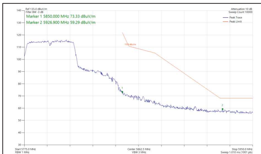
Figure 453 - 802.11n HT40, SISO, Core 0 - 5795 MHz Band Edge Frequency 5850 MHz
