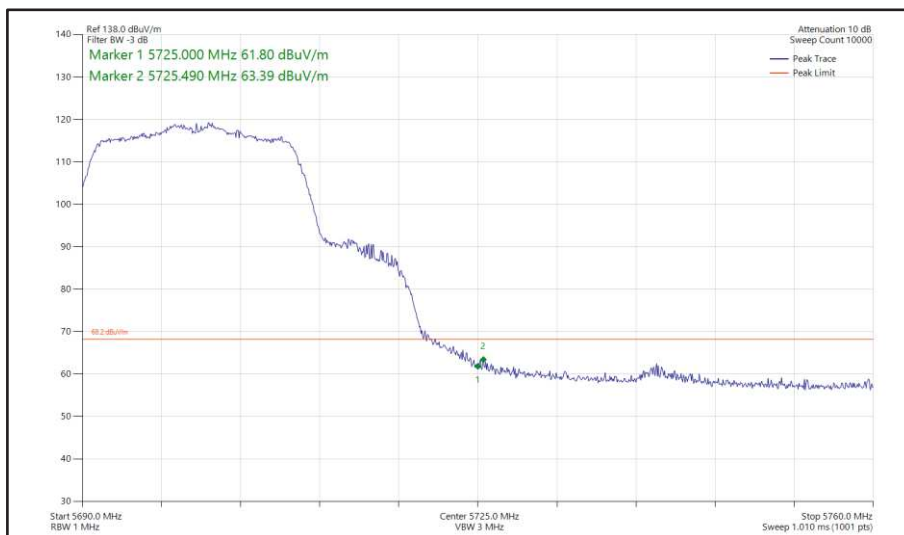
Figure 418 - 802.11n HT20, SDM, Core 0 + Core 1 - 5700 MHz Band Edge Frequency 5725 MHz
