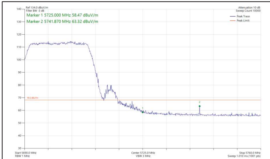
Figure 435 - 802.11ac VHT20, TxBF, Core 0 + Core 1 - 5700 MHz Band Edge Frequency 5725 MHz
