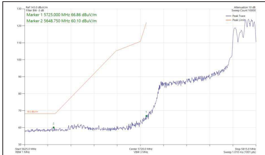
Figure 557 - 802.11ax HE80, RU 106-60, CDD, Core 0 + Core 1 - 5775 MHz Band Edge Frequency 5725 MHz
