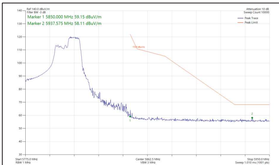
Figure 457 - 802.11ax HE40, RU 106-56, SISO, Core 0 - 5795 MHz Band Edge Frequency 5850 MHz
