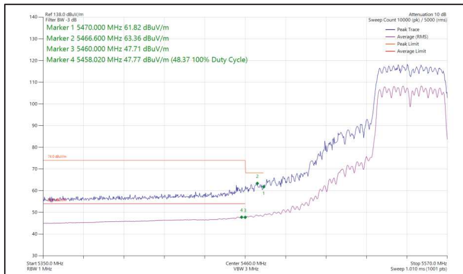
Figure 478 - 802.11n HT40, CDD, Core 0 + Core 1 - 5550 MHz Band Edge Frequency 5470 MHz
