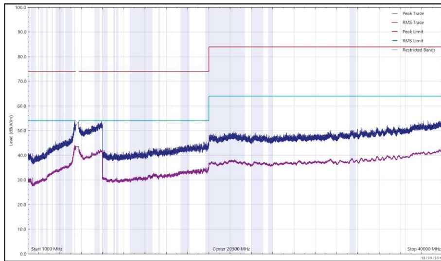
Figure 657 - U-NII-2C - 5700 MHz (CH140), 802.11a, Core 0, 1 GHz to 40 GHz, Vertical
