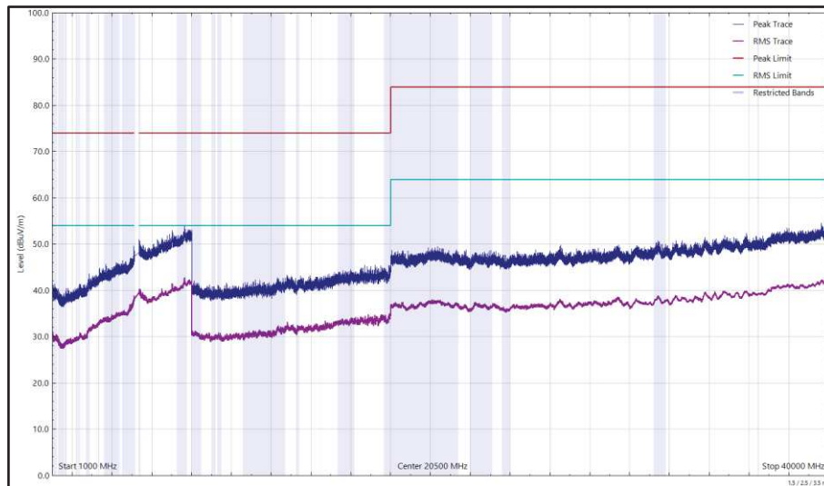
Figure 649 - U-NII-1 - 5180 MHz (CH36), 802.11a, Core 0, 1 GHz to 40 GHz, Horizontal
