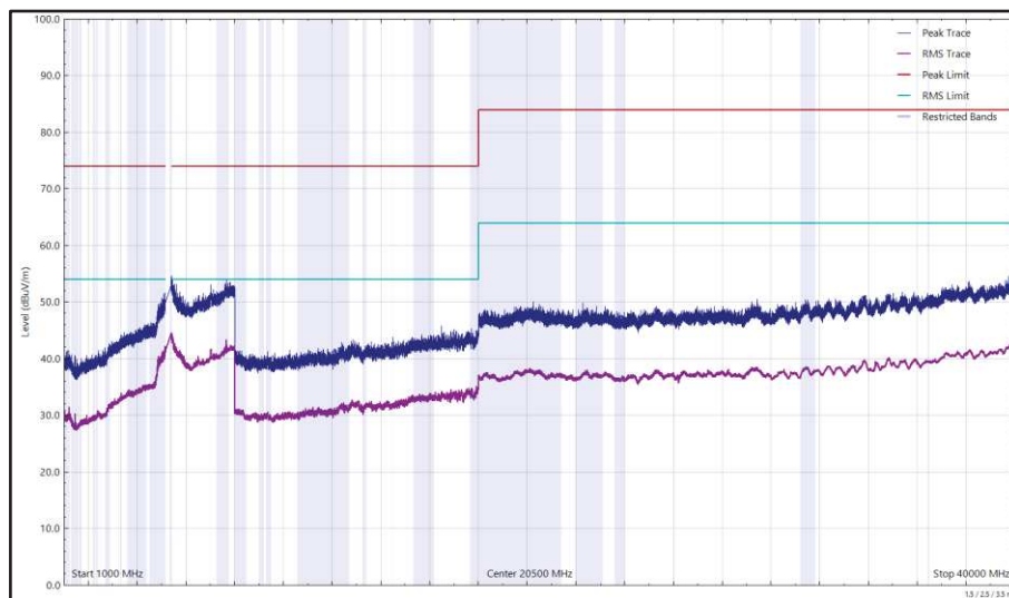
Figure 669 - U-NII-2A - 5320 MHz (CH64), 802.11a, Core 1, 1 GHz to 40 GHz, Vertical
