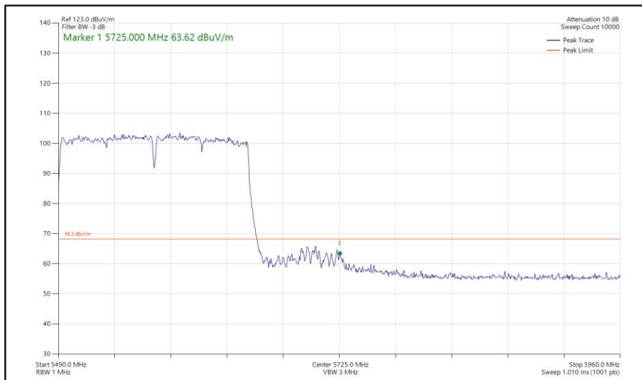
Figure 612 - 802.11ac VHT160, SDM, Core 0 + Core 1 - 5570 MHz Band Edge Frequency 5725 MHz
