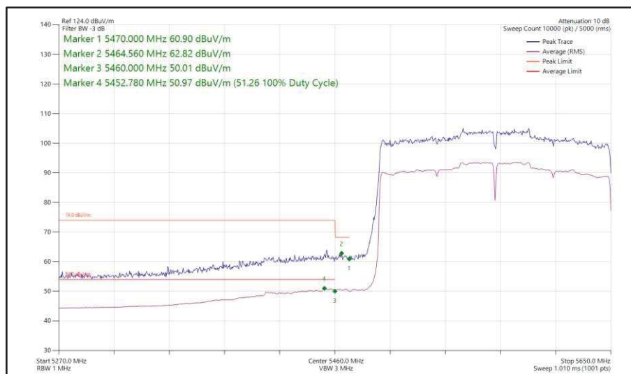
Figure 592 - 802.11ax HE160, SU, SISO, Core 0 - 5570 MHz Band Edge Frequency 5470 MHz
