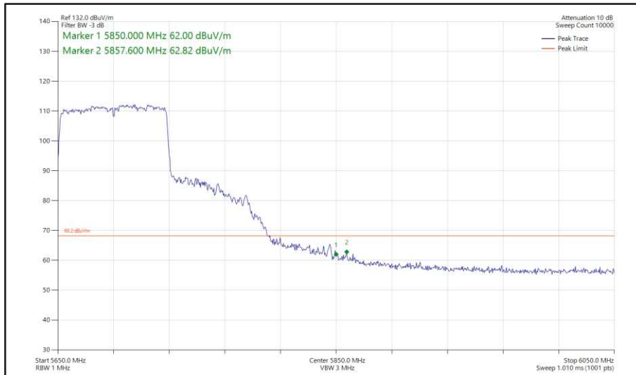
Figure 580 - 802.11ac VHT80, SDM, Core 0 + Core 1 - 5690 MHz Band Edge Frequency 5850 MHz
