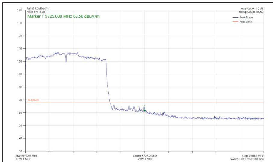
Figure 613 - 802.11ax HE160, SU, SDM, Core 0 + Core 1 - 5570 MHz Band Edge Frequency 5725 MHz
