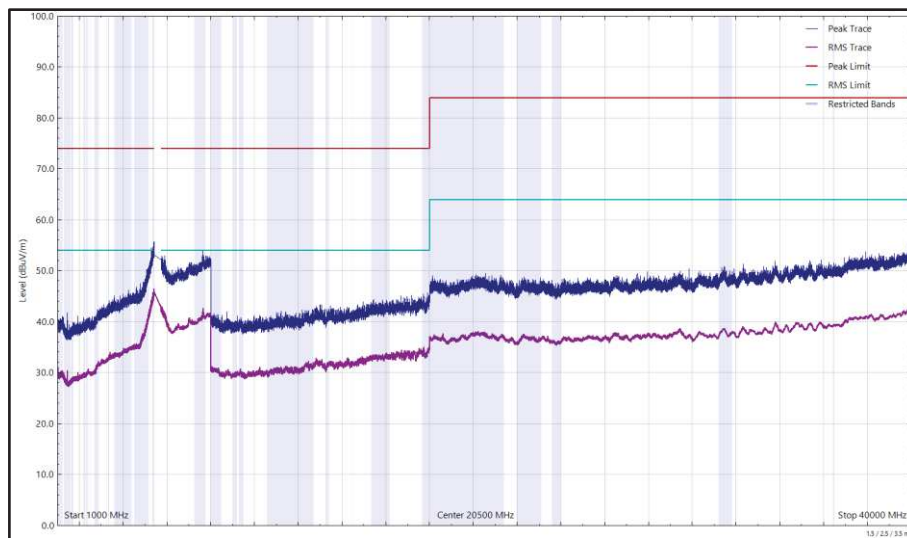
Figure 623 - U-NII-2C - 5500 MHz (CH100), HT20, CDD, Core 0 + Core 1, 1 GHz to 40 GHz, Vertical
