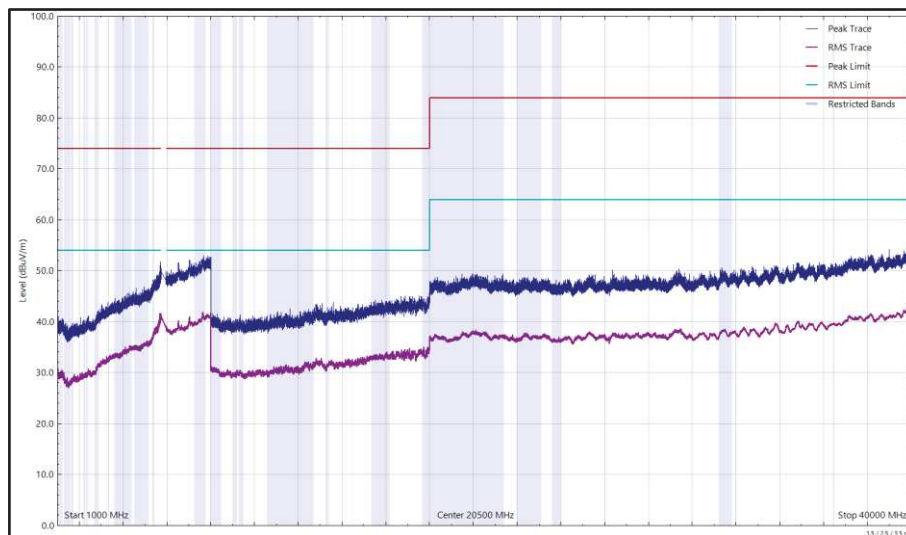
Figure 661 - U-NII-3 - 5825 MHz (CH165), 802.11a, Core 0, 1 GHz to 40 GHz, Horizontal
