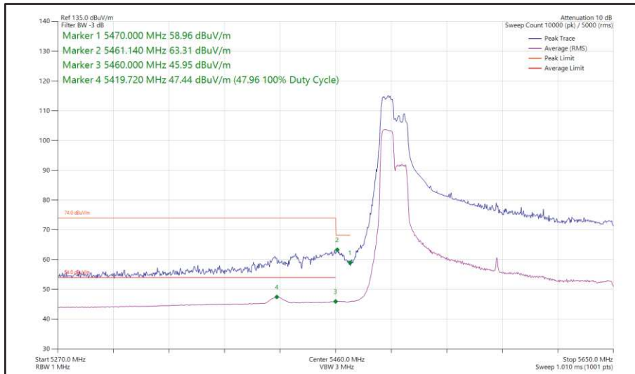
Figure 599 - 802.11ax HE160, RU 106-53, SISO, Core 1 - 5570 MHz Band Edge Frequency 5470 MHz
