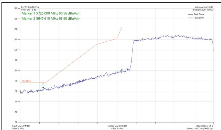
Figure 575 - 802.11ax HE80, SU, SDM, Core 0 + Core 1 - 5775 MHz Band Edge Frequency 5725 MHz
