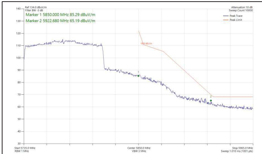
Figure 584 - 802.11ax HE80, SU, SDM, Core 0 + Core 1 - 5775 MHz Band Edge Frequency 5850 MHz
