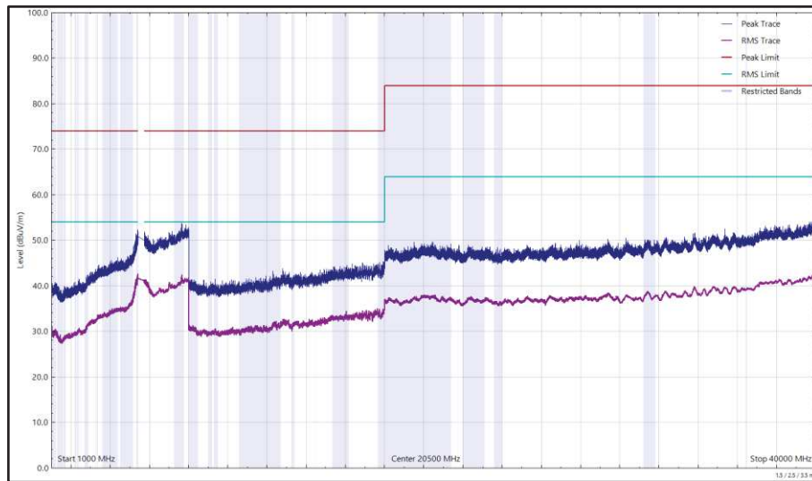
Figure 622 - U-NII-2C - 5500 MHz (CH100), HT20, CDD, Core 0 + Core 1, 1 GHz to 40 GHz, Horizontal
