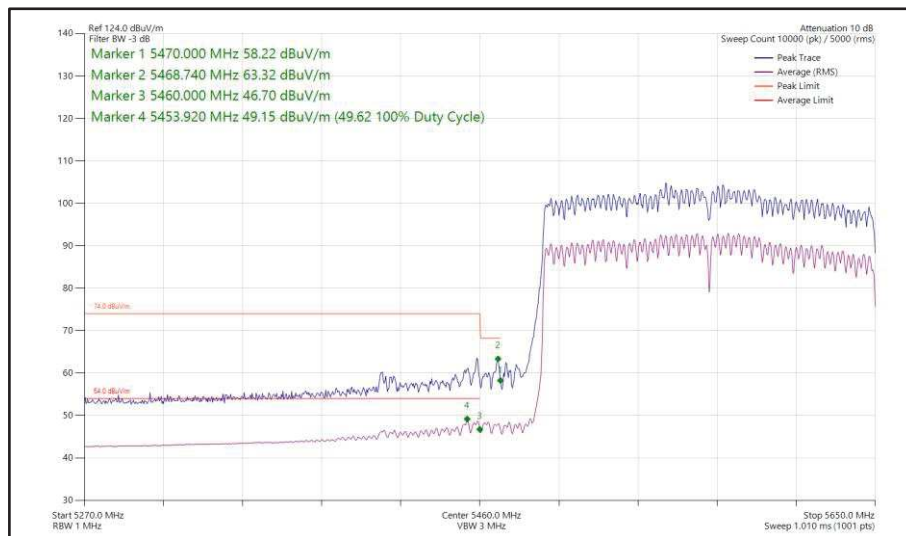
Figure 604 - 802.11ax HE160, SU, CDD, Core 0 + Core 1 - 5570 MHz Band Edge Frequency 5470 MHz
