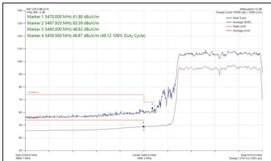
Figure 586 - 802.11ac VHT80, TxBF, Core 0 + Core 1 - 5530 MHz Band Edge Frequency 5470 MHz
