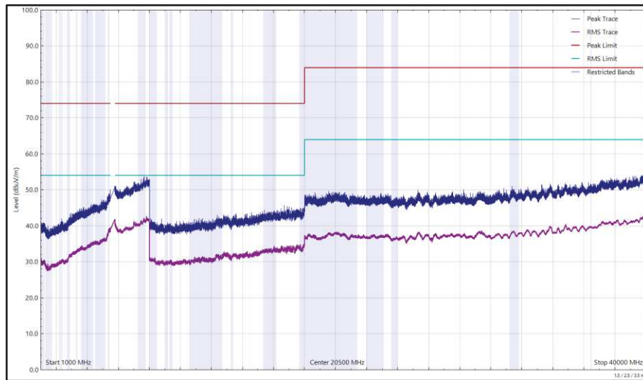
Figure 656 - U-NII-2C - 5700 MHz (CH140), 802.11a, Core 0, 1 GHz to 40 GHz, Horizontal
