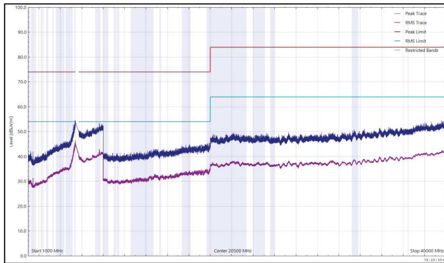
Figure 655 - U-NII-2C - 5500 MHz (CH100), 802.11a, Core 0, 1 GHz to 40 GHz, Vertical
