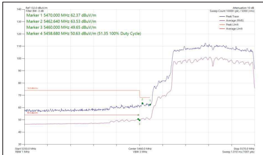
Figure 571 - 802.11ac VHT80, SDM, Core 0 + Core 1 - 5530 MHz Band Edge Frequency 5470 MHz
