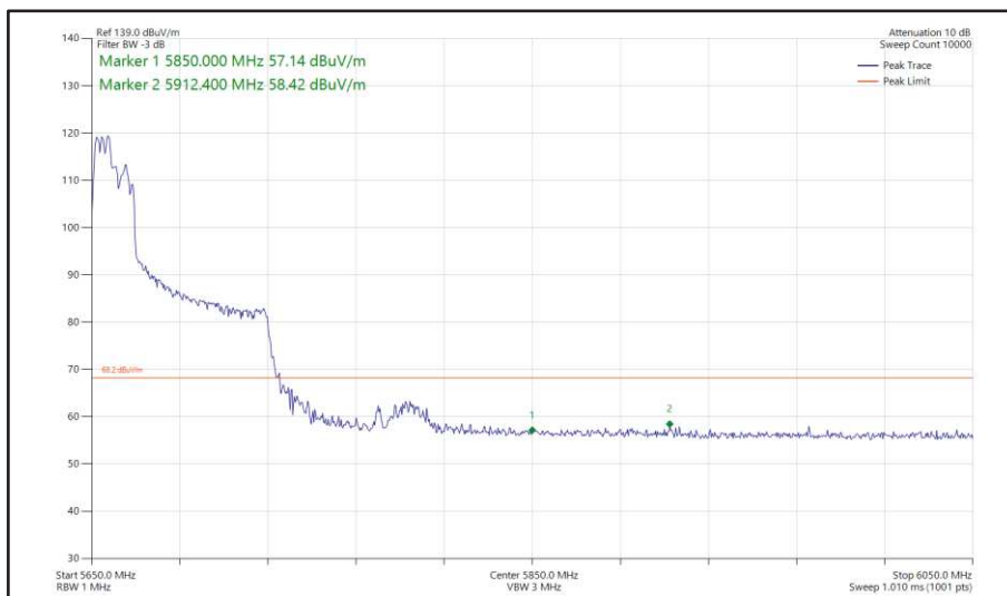
Figure 583 - 802.11ax HE80, RU 106-53, SDM, Core 0 + Core 1 - 5690 MHz Band Edge Frequency 5850 MHz
