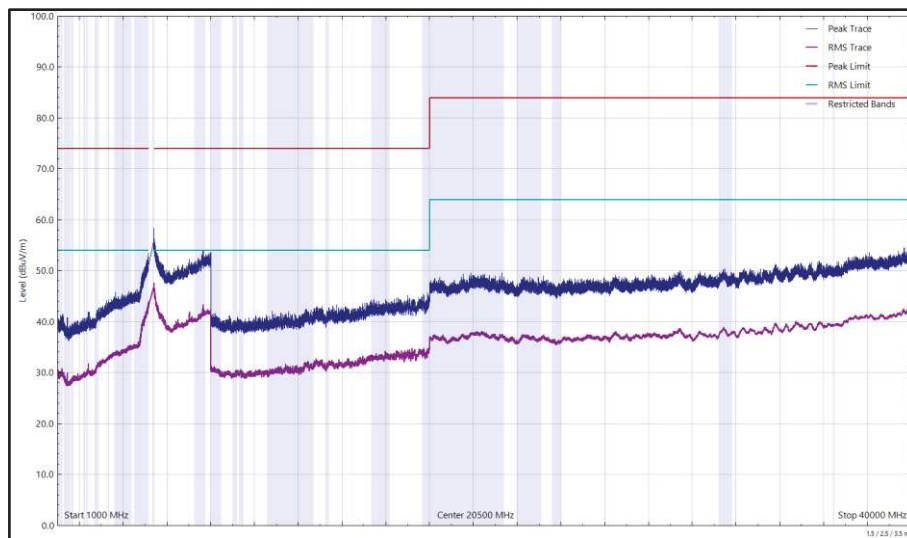
Figure 621 - U-NII-2A - 5320 MHz (CH64), HT20, CDD, Core 0 + Core 1, 1 GHz to 40 GHz, Vertical
