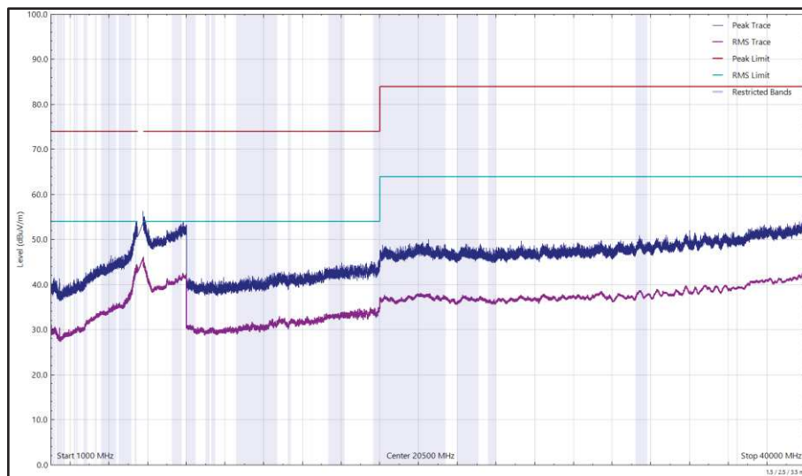
Figure 625 - U-NII-2C - 5700 MHz (CH140), HT20, CDD, Core 0 + Core 1, 1 GHz to 40 GHz, Vertical
