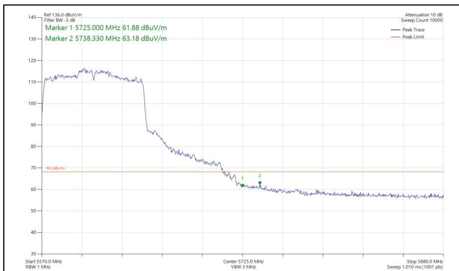
Figure 577 - 802.11ac VHT80, SDM, Core 0 + Core 1 - 5610 MHz Band Edge Frequency 5725 MHz
