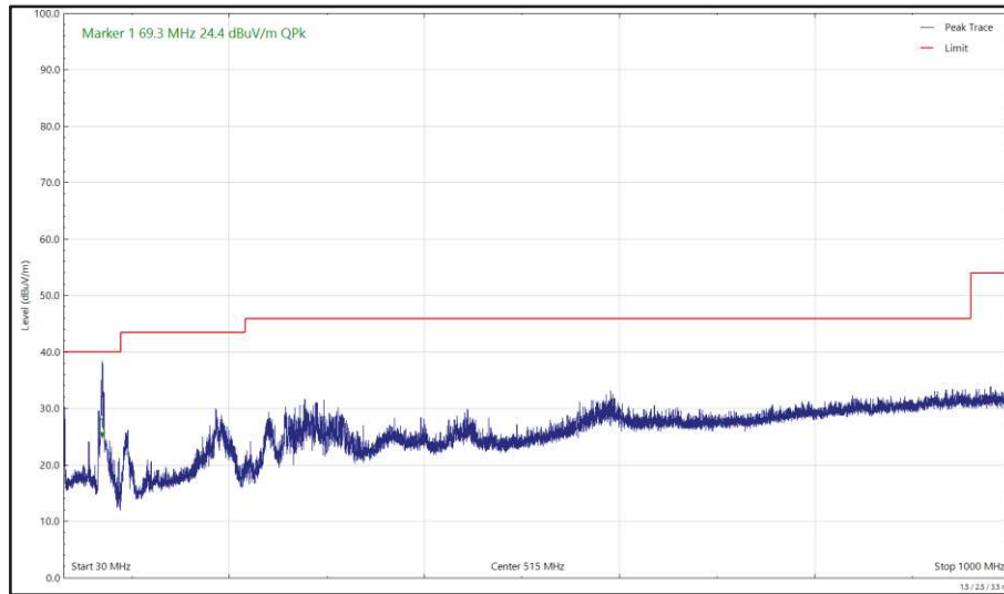
Figure 676 - U-NII-3 - 5825 MHz (CH165), 802.11a, Core 1, 30 MHz to 1 GHz, Horizontal (Peak)
