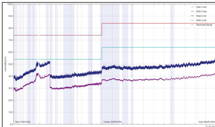
Figure 663 - U-NII-3 - 5825 MHz (CH165), 802.11a, Core 0, 1 GHz to 40 GHz, Vertical
