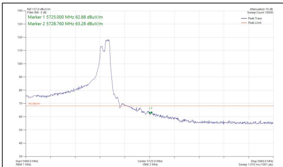
Figure 602 - 802.11ax HE160, RU 106-60, SISO, Core 1 - 5570 MHz Band Edge Frequency 5725 MHz
