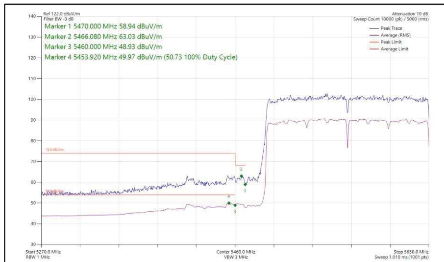
Figure 598 - 802.11ax HE160, SU, SISO, Core 1 - 5570 MHz Band Edge Frequency 5470 MHz
