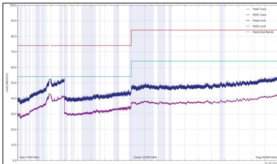
Figure 679 - U-NII-3 - 5825 MHz (CH165), 802.11a, Core 1, 1 GHz to 40 GHz, Vertical
