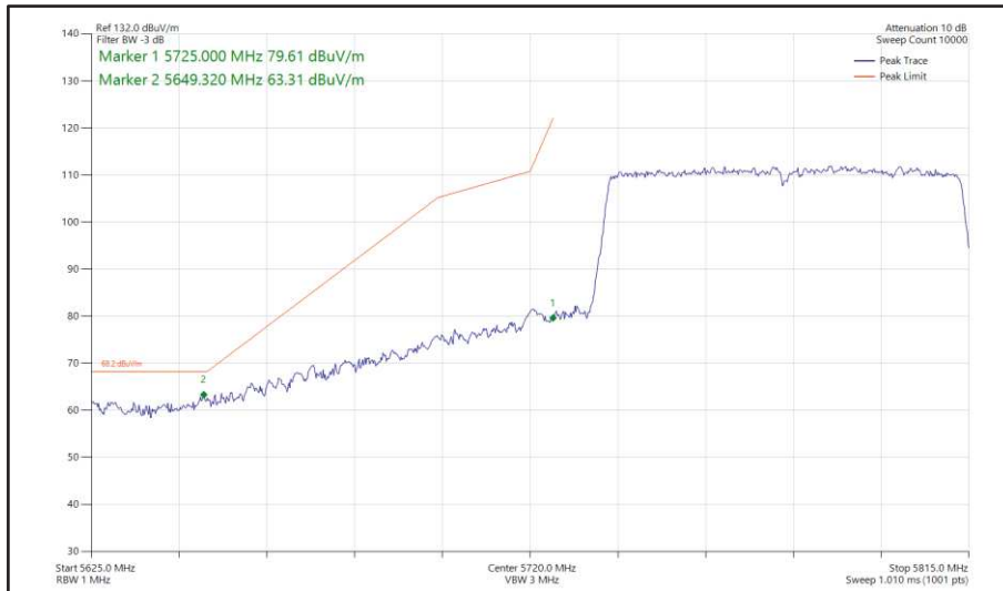
Figure 574 - 802.11ac VHT80, SDM, Core 0 + Core 1 - 5775 MHz Band Edge Frequency 5725 MHz
