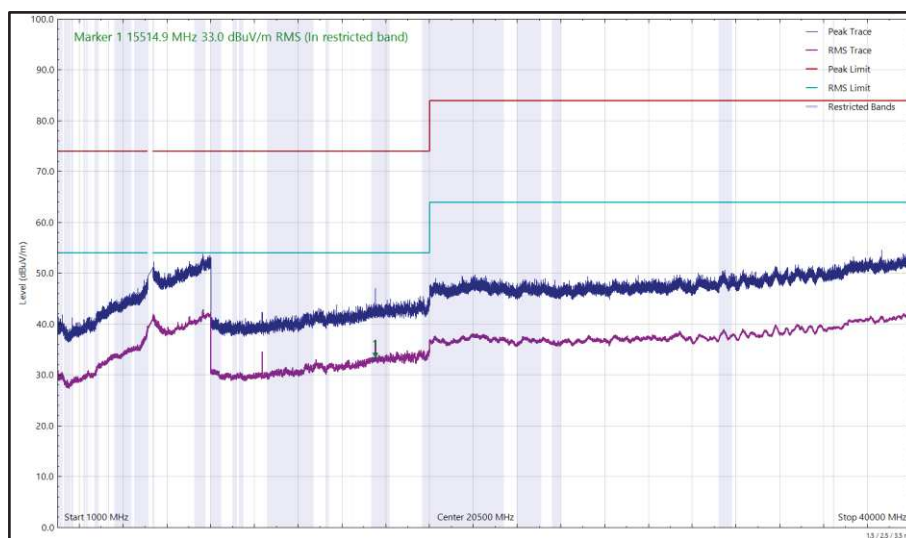
Figure 633 - U-NII-1 - 5180 MHz (CH36), HE20, RU26-0, CDD, Core 0 + Core 1, 1 GHz to 40 GHz, Horizontal
