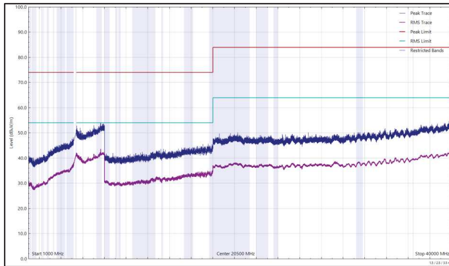
Figure 668 - U-NII-2A - 5320 MHz (CH64), 802.11a, Core 1, 1 GHz to 40 GHz, Horizontal
