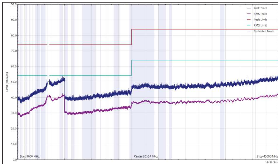
Figure 670 - U-NII-2C - 5500 MHz (CH100), 802.11a, Core 1, 1 GHz to 40 GHz, Horizontal
