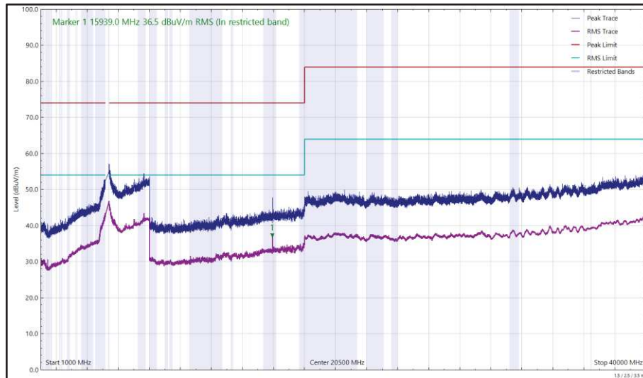
Figure 637 - U-NII-2A - 5320 MHz (CH64), HE20, RU52-37, CDD, Core 0 + Core 1, 1 GHz to 40 GHz, Vertical
