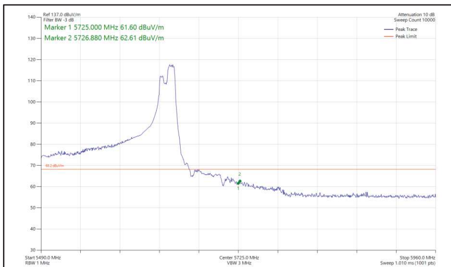
Figure 596 - 802.11ax HE160, RU 106-60, SISO, Core 0 - 5570 MHz Band Edge Frequency 5725 MHz
