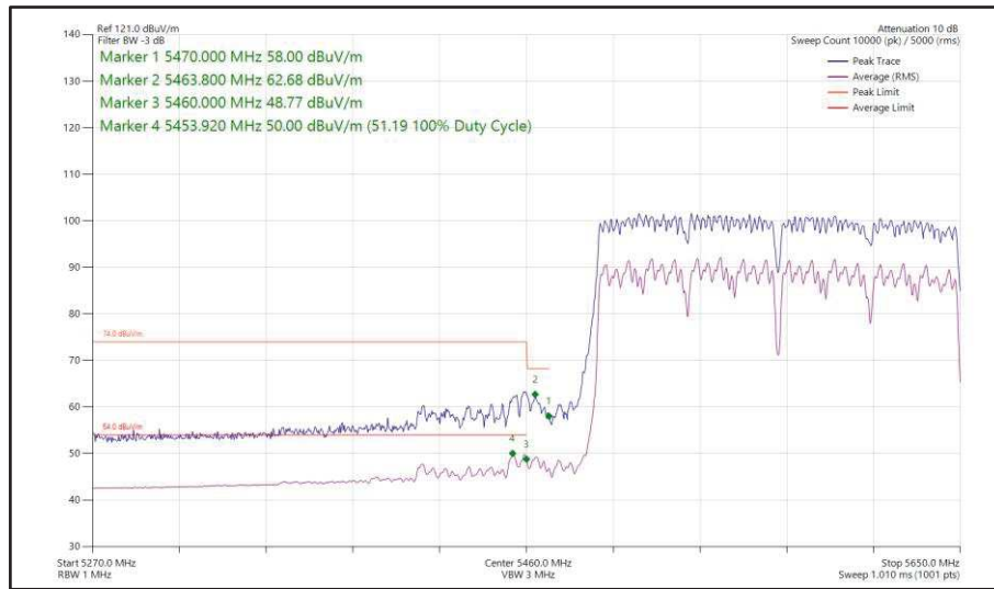
Figure 603 - 802.11ac VHT160, CDD, Core 0 + Core 1 - 5570 MHz Band Edge Frequency 5470 MHz
