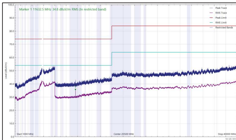
Figure 645 - U-NII-3 - 5825 MHz (CH165), HE20, RU26-0, CDD, Core 0 + Core 1, 1 GHz to 40 GHz, Horizontal
