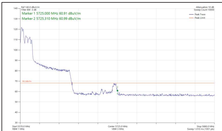
Figure 579 - 802.11ax HE80, RU 52-37, SDM, Core 0 + Core 1 - 5610 MHz Band Edge Frequency 5725 MHz
