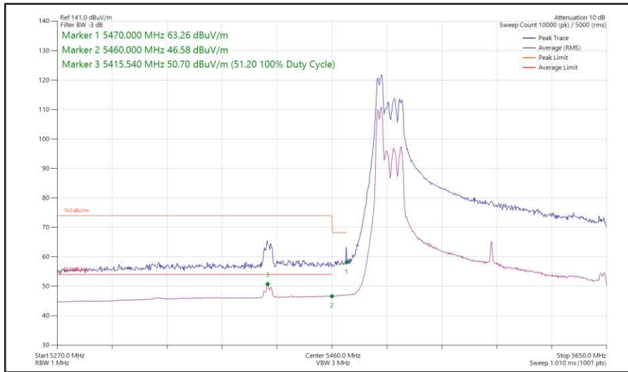
Figure 611 - 802.11ax HE160, RU 52-37, SDM, Core 0 + Core 1 - 5570 MHz Band Edge Frequency 5470 MHz
