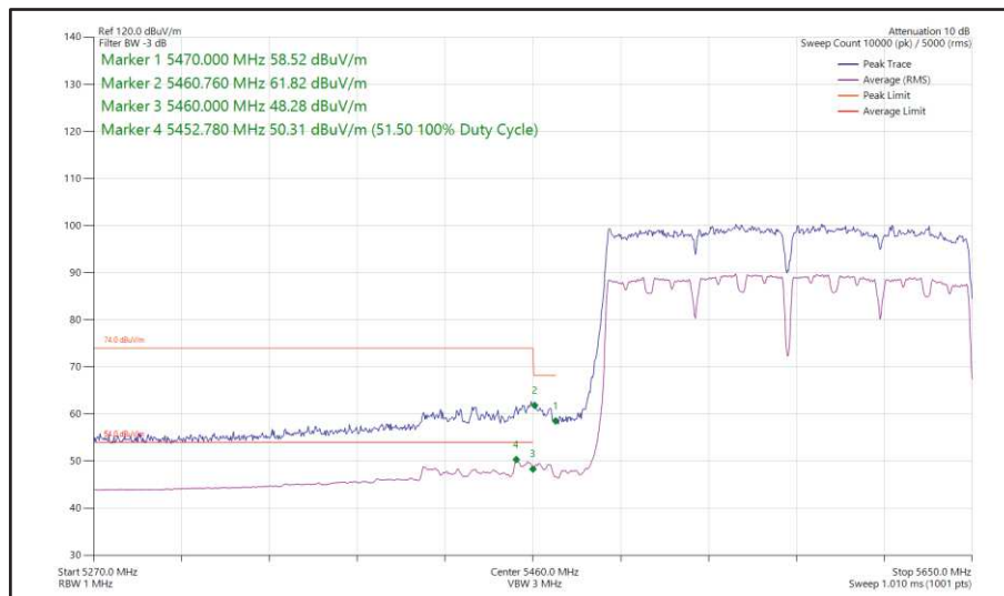
Figure 591 - 802.11ac VHT160, SISO, Core 0 - 5570 MHz Band Edge Frequency 5470 MHz
