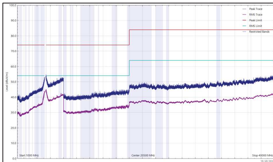
Figure 651 - U-NII-1 - 5180 MHz (CH36), 802.11a, Core 0, 1 GHz to 40 GHz, Vertical
