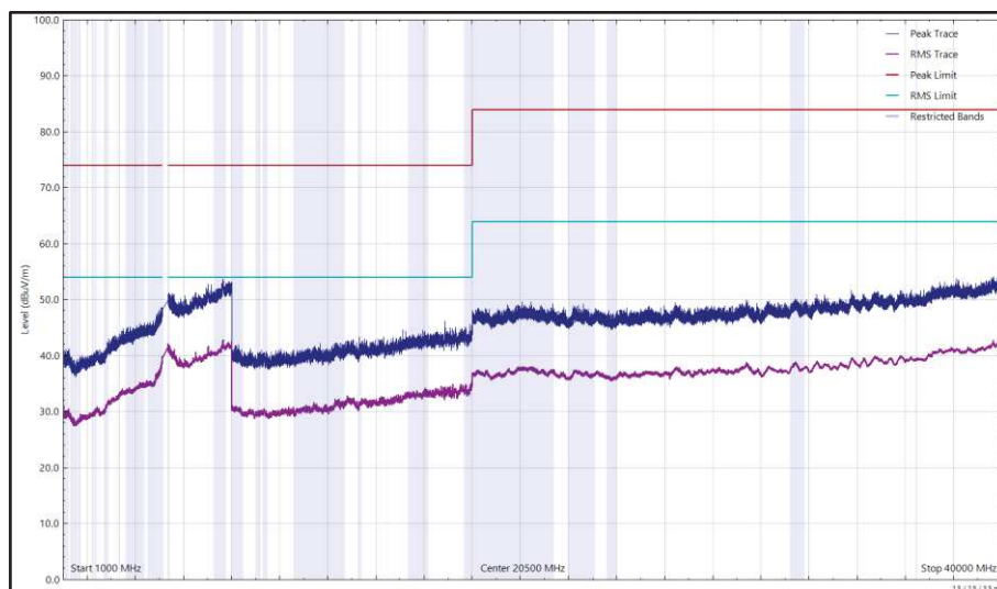
Figure 617 - U-NII-1 - 5180 MHz (CH36), HT20, CDD, Core 0 + Core 1, 1 GHz to 40 GHz, Horizontal
