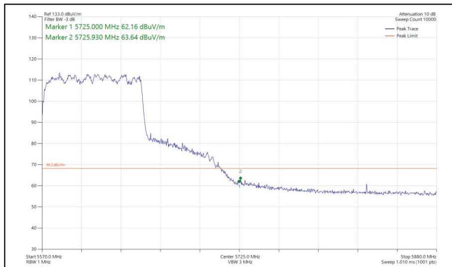
Figure 588 - 802.11ac VHT80, TxBF, Core 0 + Core 1 - 5610 MHz Band Edge Frequency 5725 MHz
