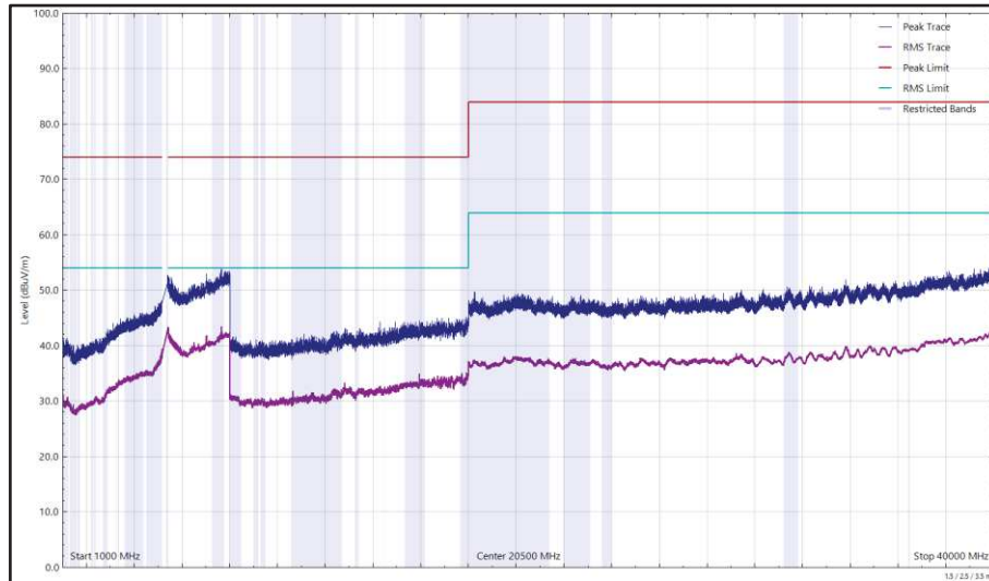
Figure 636 - U-NII-2A - 5320 MHz (CH64), HE20, RU52-37, CDD, Core 0 + Core 1, 1 GHz to 40 GHz, Horizontal
