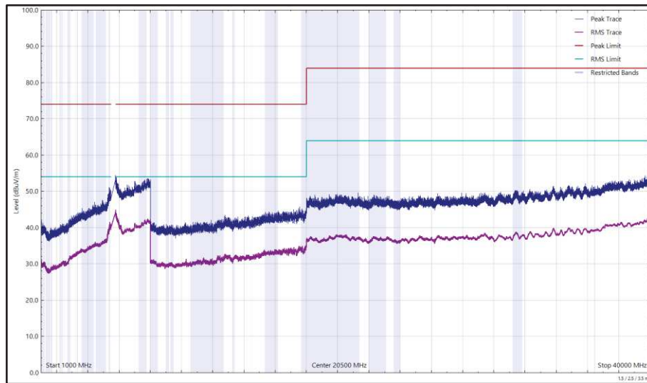
Figure 624 - U-NII-2C - 5700 MHz (CH140), HT20, CDD, Core 0 + Core 1, 1 GHz to 40 GHz, Horizontal
