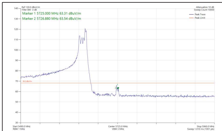
Figure 608 - 802.11ax HE160, RU 52-52, CDD, Core 0 + Core 1 - 5570 MHz Band Edge Frequency 5725 MHz
