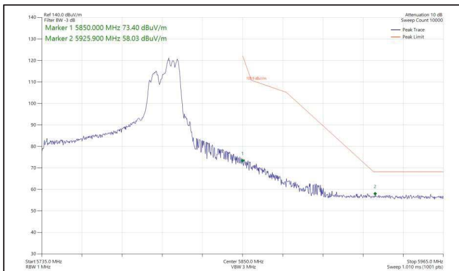
Figure 585 - 802.11ax HE80, RU 106-60, SDM, Core 0 + Core 1 - 5775 MHz Band Edge Frequency 5850 MHz
