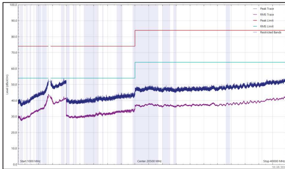
Figure 671 - U-NII-2C - 5500 MHz (CH100), 802.11a, Core 1, 1 GHz to 40 GHz, Vertical
