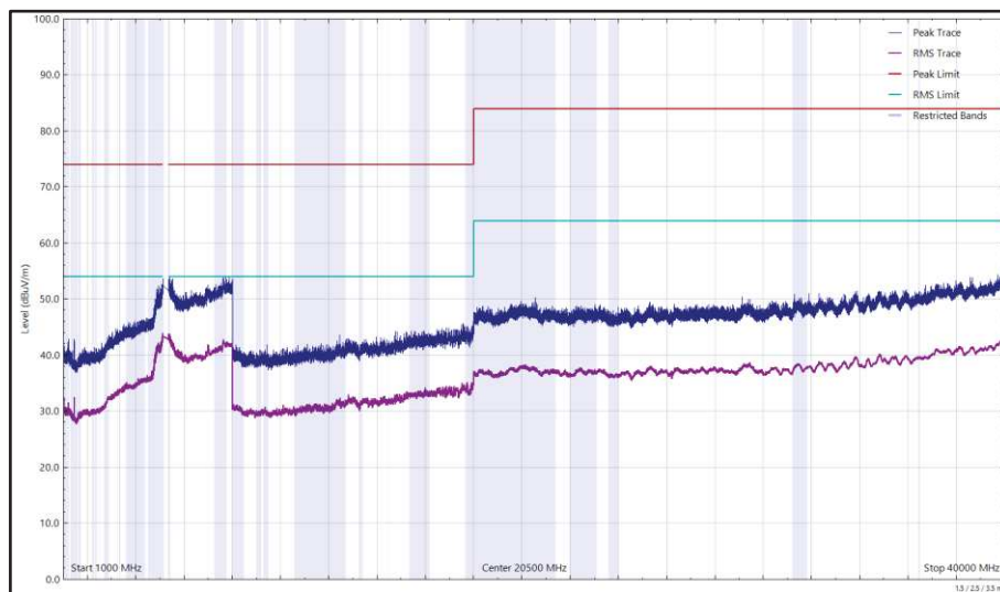
Figure 667 - U-NII-1 - 5180 MHz (CH36), 802.11a, Core 1, 1 GHz to 40 GHz, Vertical
