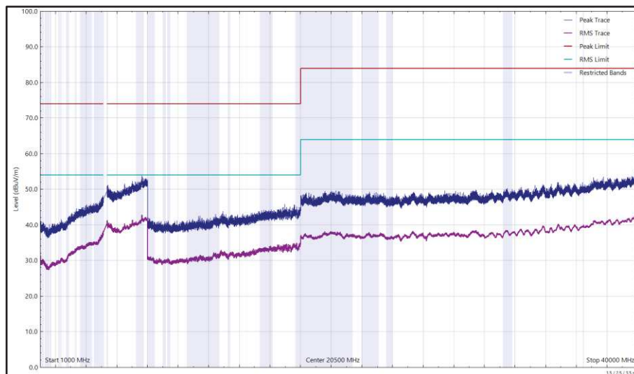
Figure 665 - U-NII-1 - 5180 MHz (CH36), 802.11a, Core 1, 1 GHz to 40 GHz, Horizontal
