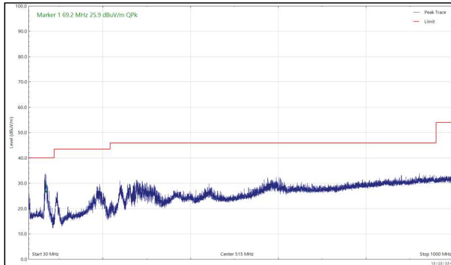
Figure 664 - U-NII-1 - 5180 MHz (CH36), 802.11a, Core 1, 30 MHz to 1 GHz, Horizontal (Peak)
